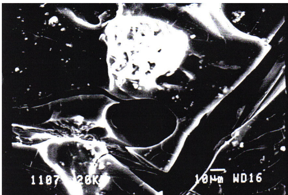
Figure 7.3.5 SEM image of Sample 4 (Tool 43). Red Ochre. Successful.
