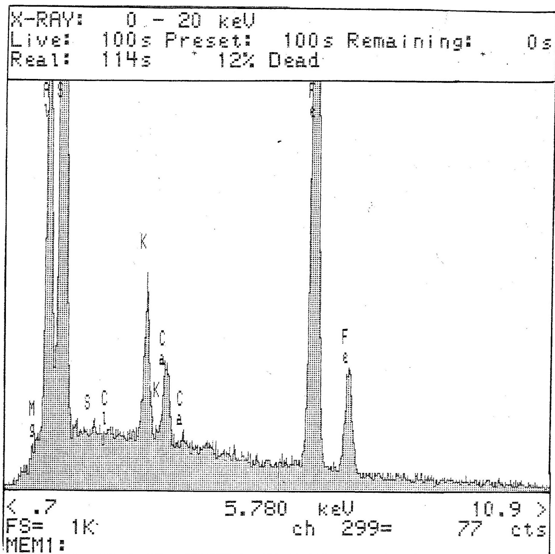
Figure 8.3.9 EDS Spectra IX: Red Ochre and Beeswax. Granular area.
