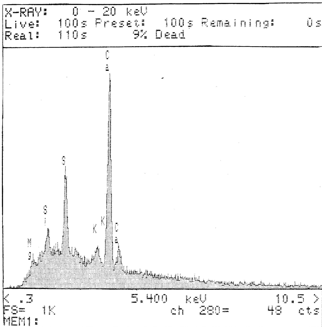
Figure 8.3.1 EDS Spectra I: Gypsum. Smooth, featureless section.
