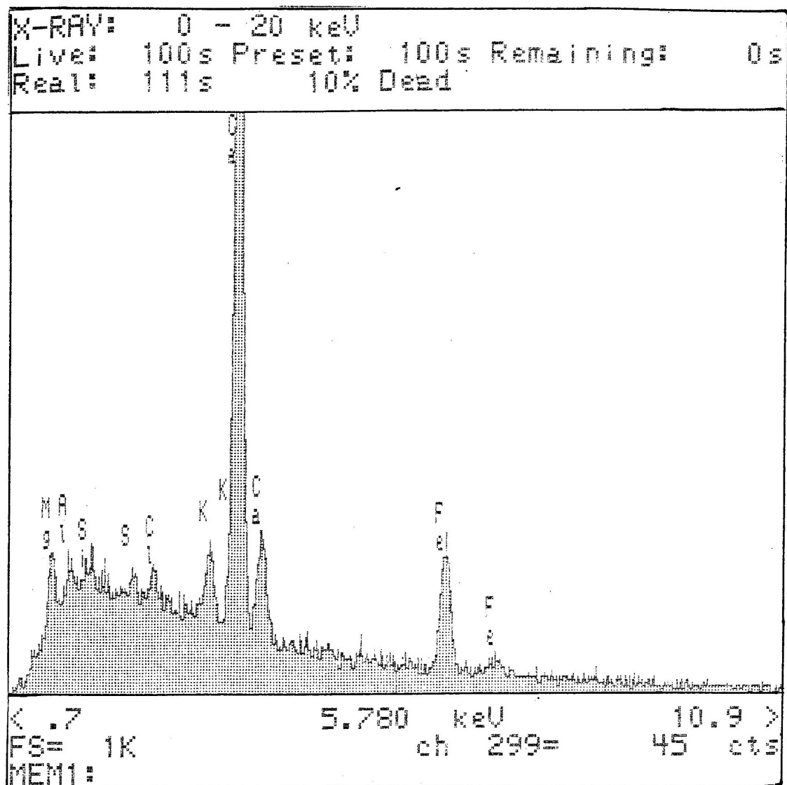
Figure 8.3.8 EDS Spectra VIII: Red Ochre and Beeswax. Smooth, featureless area.
