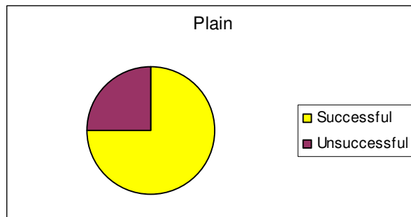
Figure 3.6.8 Success rate of tools made with no aggregate, i.e. plain resin.
