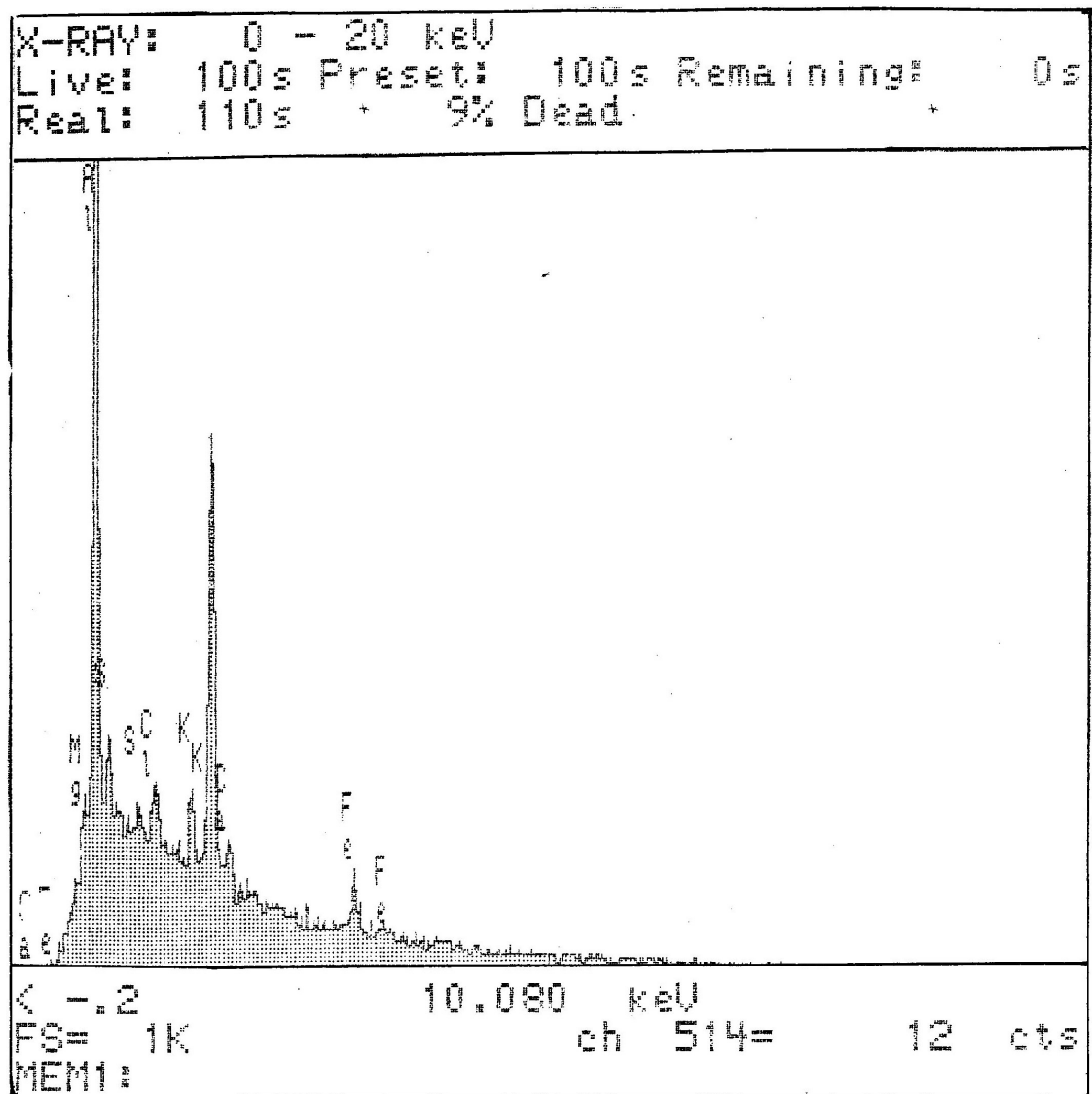
Figure 8.3.10 EDS Spectra X: Kaolinite. Smooth, featureless area.
