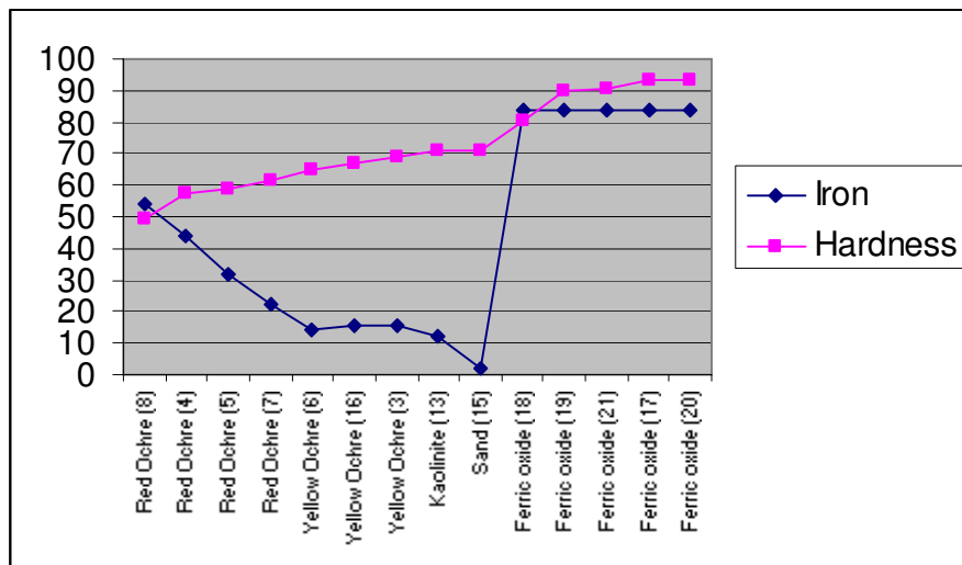
Figure 6.4.2 HRT readings versus percentage of iron (in the aggregates). Hardness test sample numbers are given after the aggregate.
