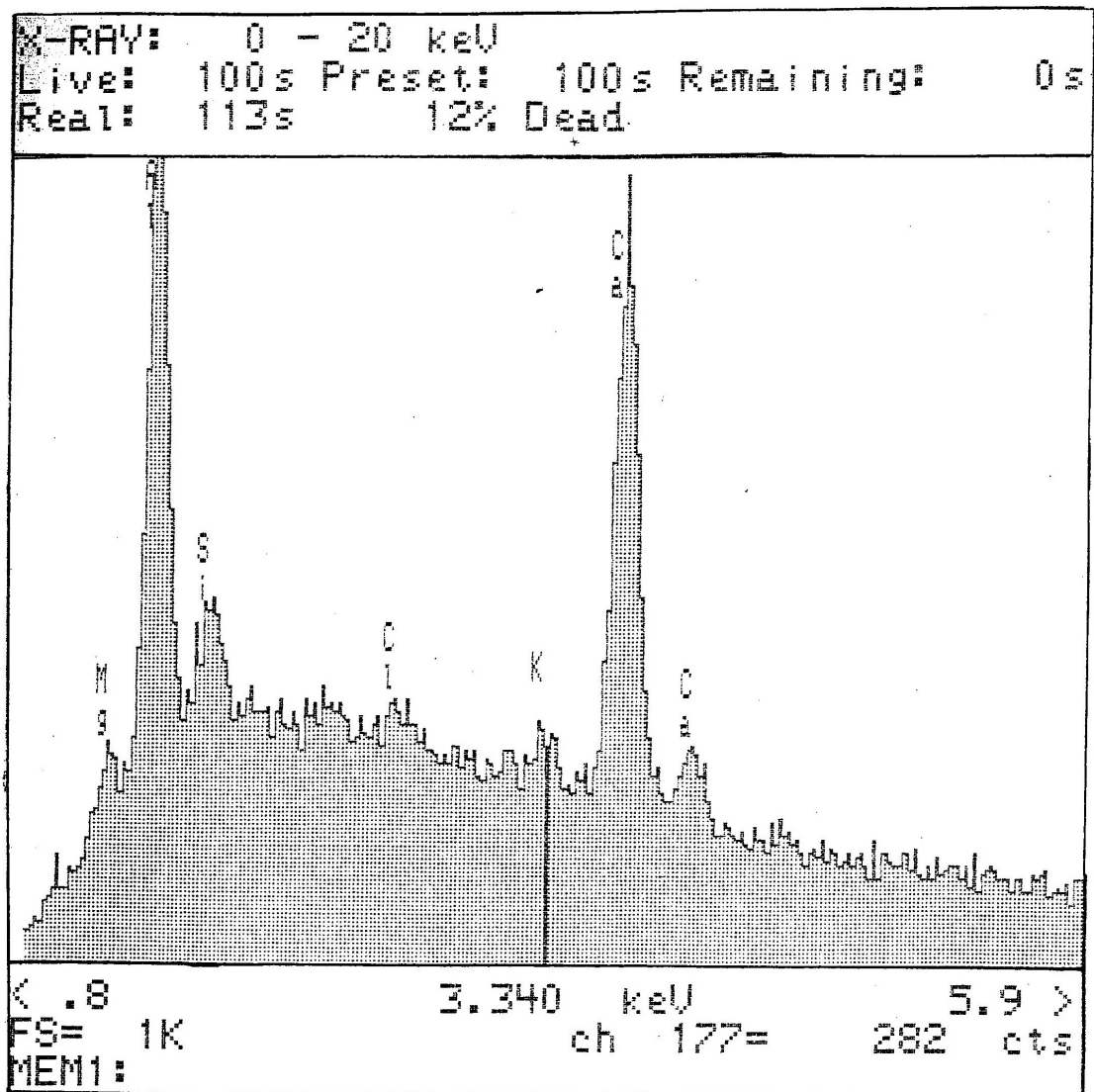
Figure 8.3.3 EDS Spectra III: Plain Resin. Smooth, featureless area.
