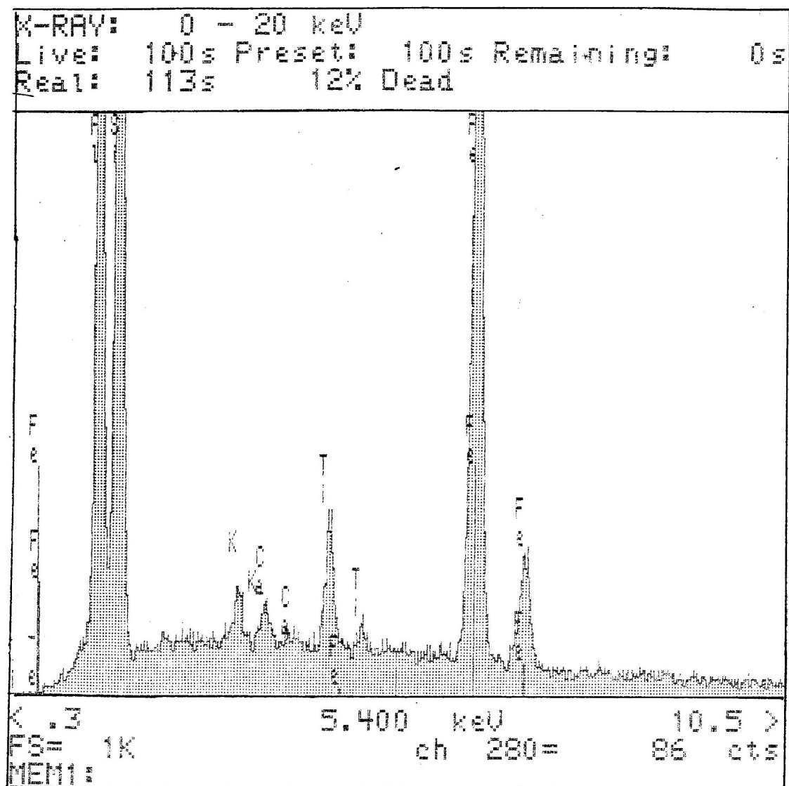
Figure 8.3.11 EDS Spectra XI: Kaolinite. Granular area.
