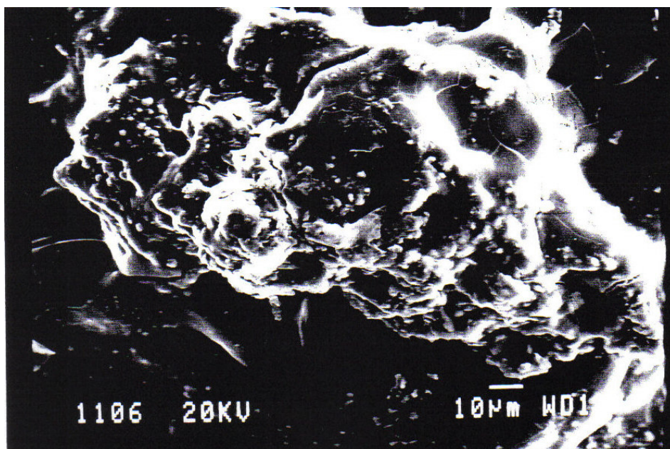
Figure 7.3.6 SEM image of Sample 4 (Tool 43). Red Ochre. Successful.
