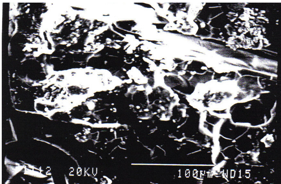
Figure 7.3.12 SEM image of Sample 13 (Tool 52). Kaolinite. Successful.
