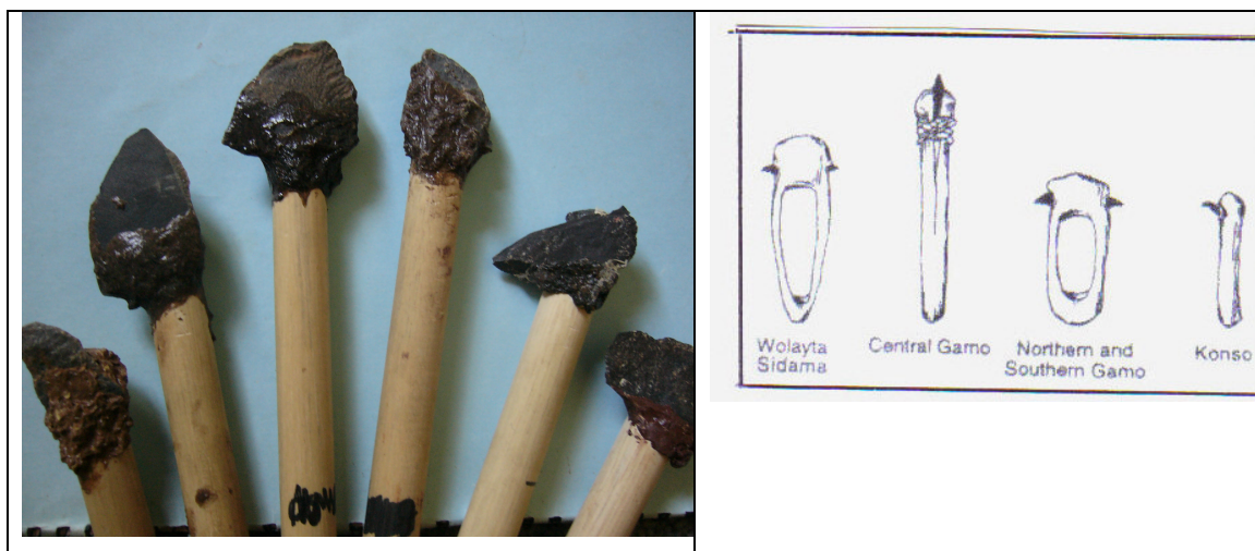
Figure 1.1 Chopping and sawing tools made in the current study (left), as opposed to the scraping tools used in southern Ethiopia (Brandt & Weedman, 1997). The tools on the left are all hafted with plain resin adhesives.
