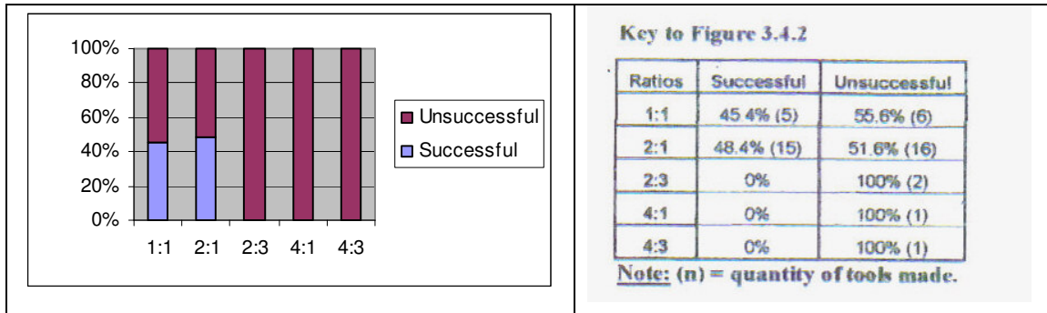
Figure 3.4.2 Success rate of adhesives made with different ratios of ingredients (not considering aggregate type).
