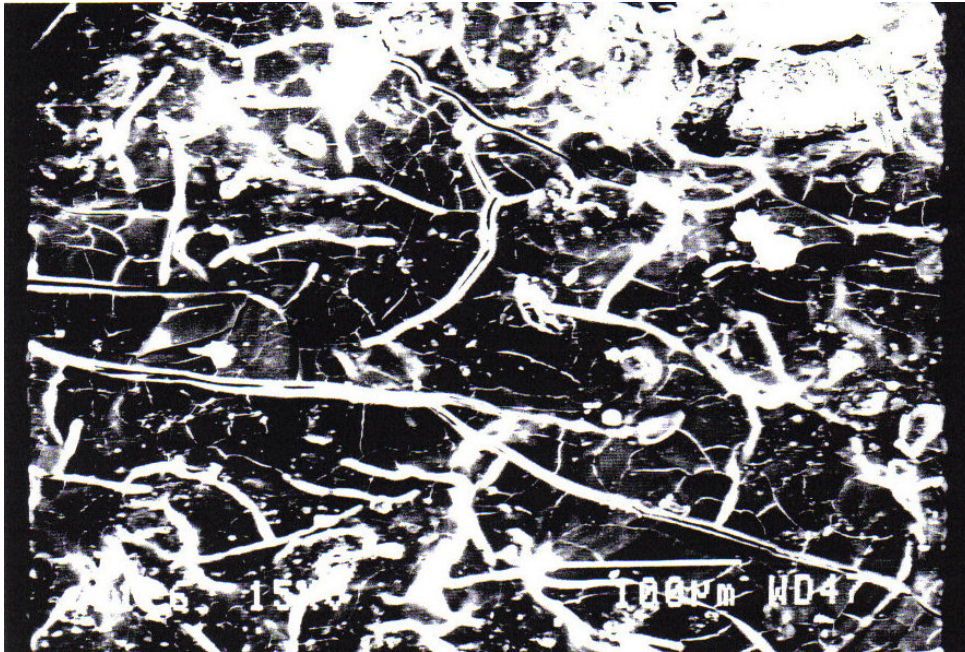
Figure 7.3.7 SEM image of Sample 8 (Tool 47). Red Ochre. Successful.
