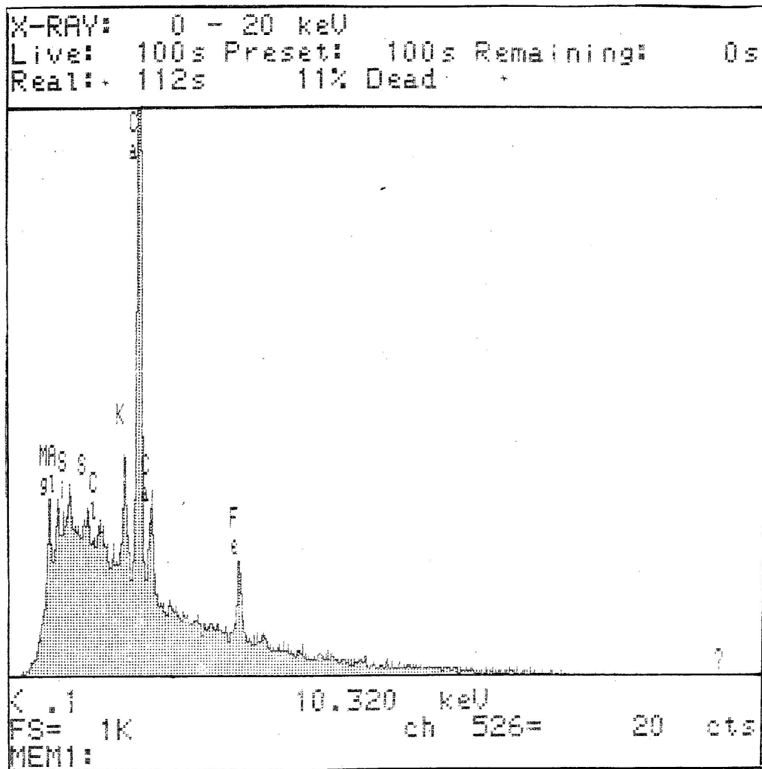
Figure 8.3.6 EDS Spectra VI: Red Ochre. Smooth, featureless area.
