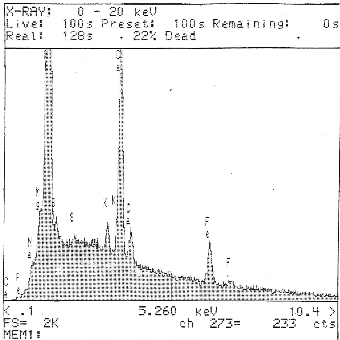
Figure 8.3.4 EDS Spectra IV: Yellow Ochre. Granular area.
