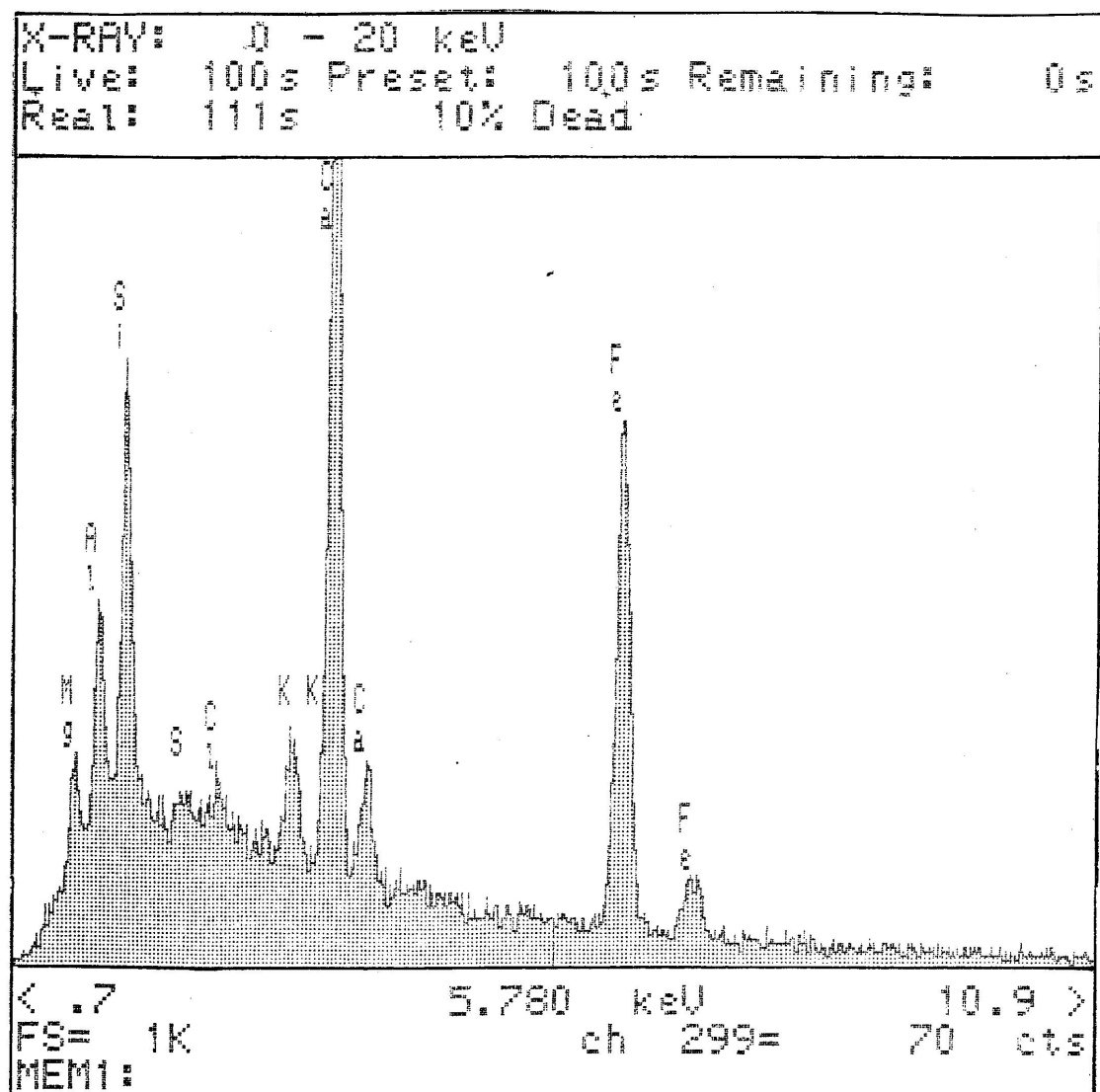
Figure 8.3.7 EDS Spectra VII: Red Ochre and Beeswax. Mixed area, some granules but quite smooth.
