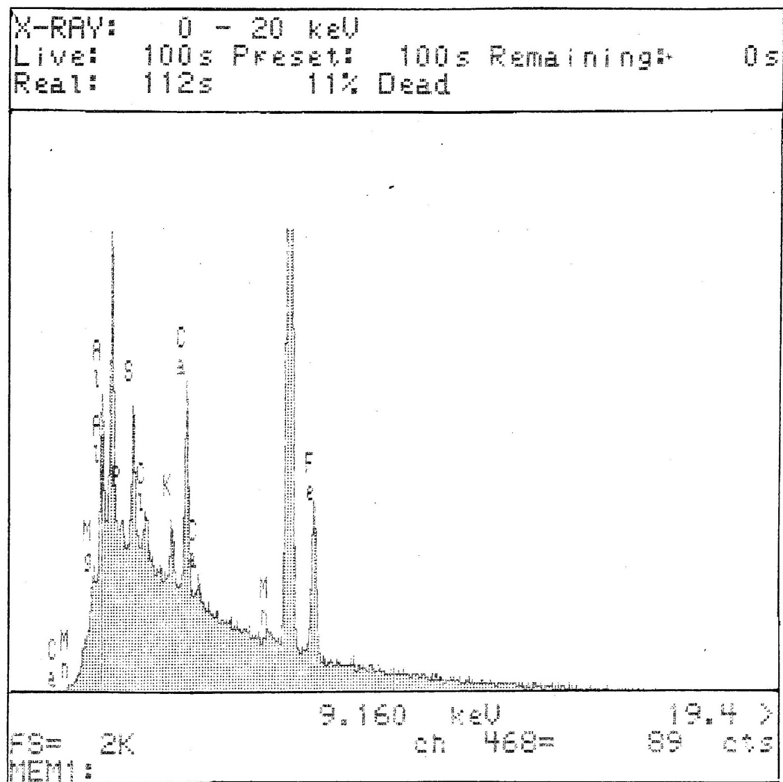
Figure 8.3.5 EDS Spectra V: Red Ochre. Granular area.
