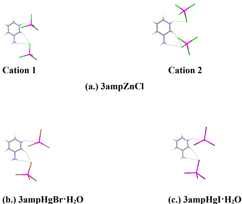
Figure 45: Identified synthons in (a.) 3ampZnCl , (b.) 3ampHgBr·H 2 O (Ali, 2008; TOBCOD) and (c.) 3ampHgI·H 2 O .
