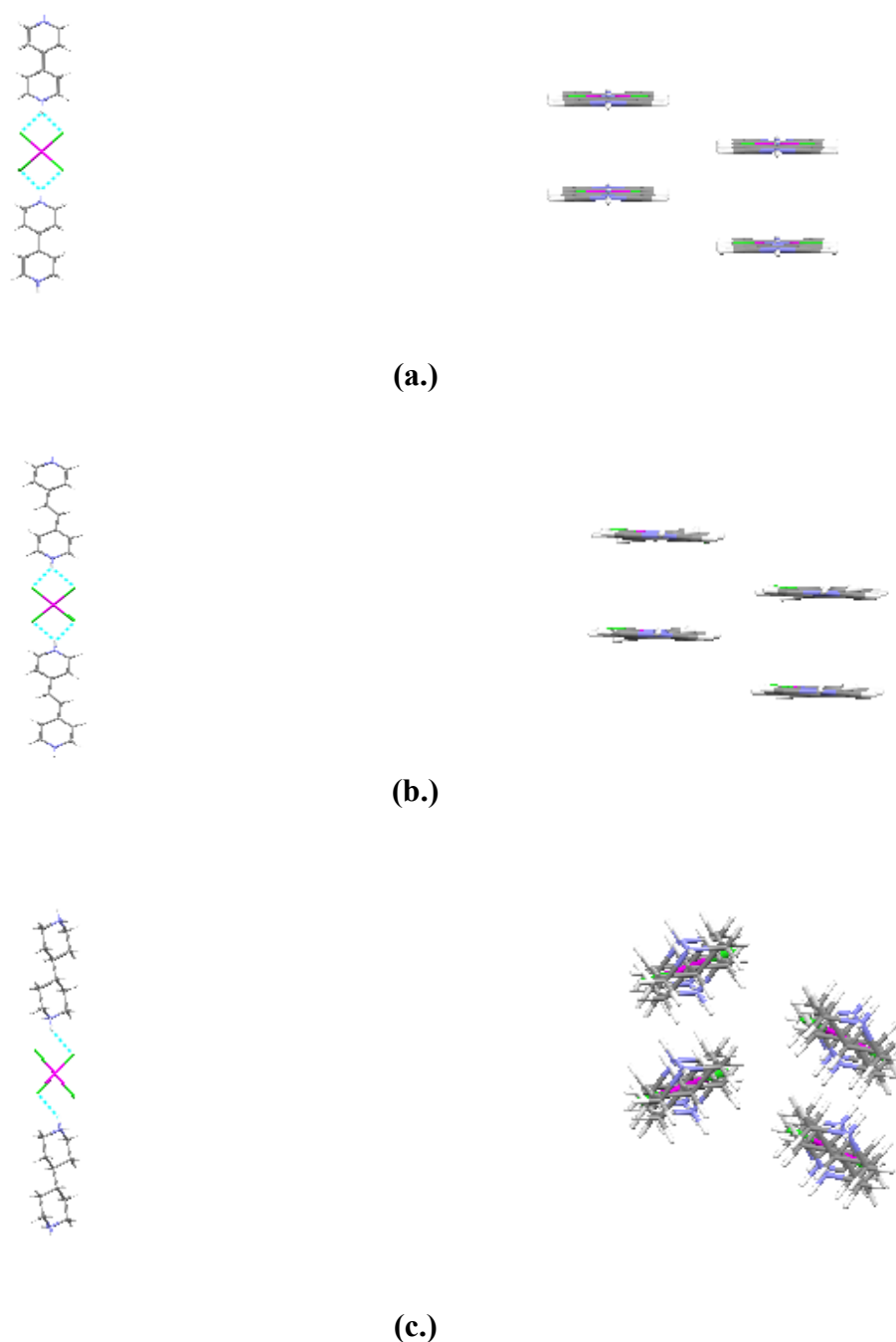
Figure 8: (a.) left: \text{NH}\cdots\text{Cl} hydrogen-bonded ribbon in A , right: ribbon packing in crystalline A . (Gillon and Orpen, 2000; Lewis and Orpen, 1998) (b.) left: \text{NH}\cdots\text{Cl} hydrogen-bonded ribbon in H , right: ribbon packing in crystalline H . Isostructural to I . (Adams and Orpen, 2006) (c.) left: \text{NH}\cdots\text{Cl} hydrogen-bonded ribbon in J , right: ribbon packing in crystalline J . (Adams and Orpen, 2006).
