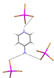
Cation 1
