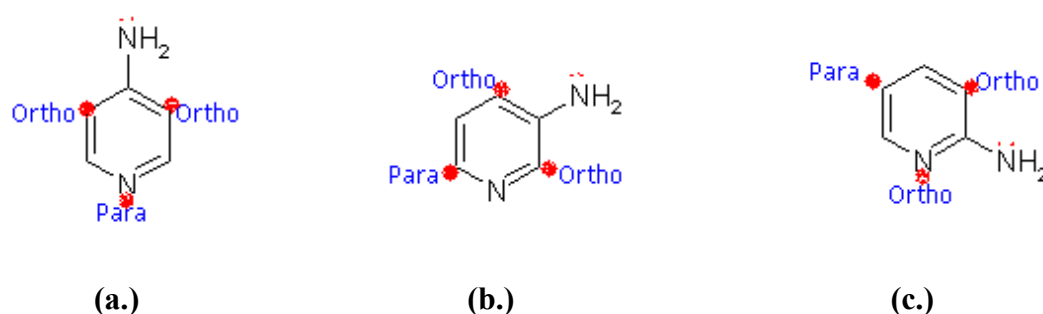
Figure 4: Additional negative charge at the ortho and para positions of (a.) 4-aminopyridine, (b.) 3-aminopyridine and (c.) 2-aminopyridine, indicated by red dots.
