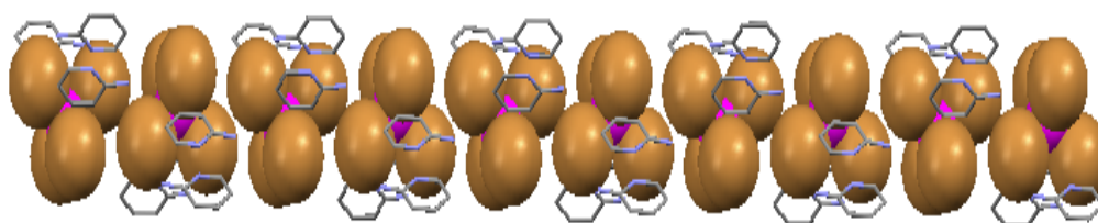
Figure 52: Anions packing in channel formed by 2-aminopyridinium cation in the structure 2ampZnBr . Isostructural to 2ampHgCl .
