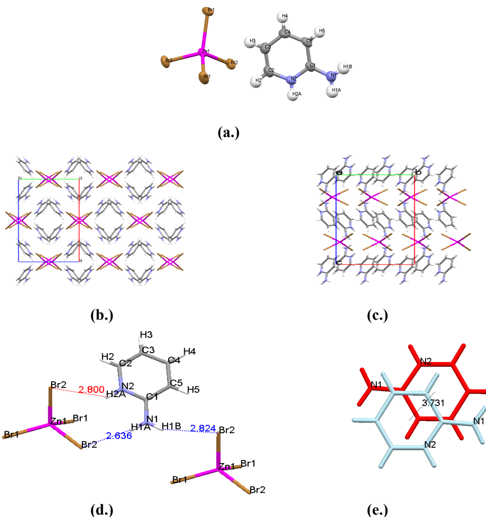
Figure 21: (a.) Asymmetric unit of 2ampZnBr (full anion is shown for clarity). (b.) Crystal structure of 2ampZnBr , viewed down the c -axis. Isostructural to 2ampZnCl and 2ampHgCl . (c.) Crystal structure of 2ampZnBr , viewed down the a -axis, showing the organic and inorganic layers. (d) Hydrogen bonding interactions. (e) Cation orientation.
