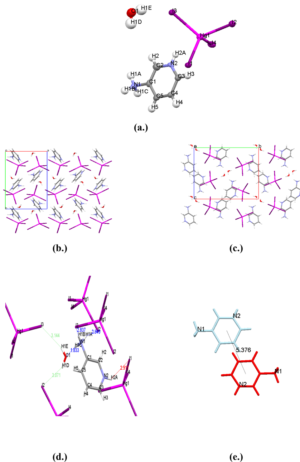
Figure 29: (a.) Asymmetric unit of 3ampHgI·H 2 O . (b.) Crystal structure of 3ampHgI·H 2 O , viewed down the c -axis. Space group P2 1 /n . (c.) Structure viewed down the a -axis. (d.) Charge assisted intermolecular interactions in the crystal structure of 3ampHgI·H 2 O . (e.) Cation orientation.
