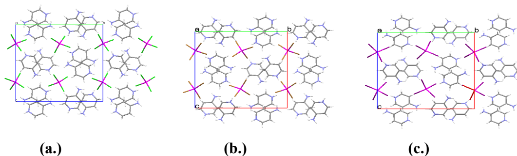
Figure 67: (a.) 4ampZnCl, viewed down the a -axis. (b.) 4ampZnBr, viewed down the a -axis (c.) 4ampZnI, viewed down the a -axis.
