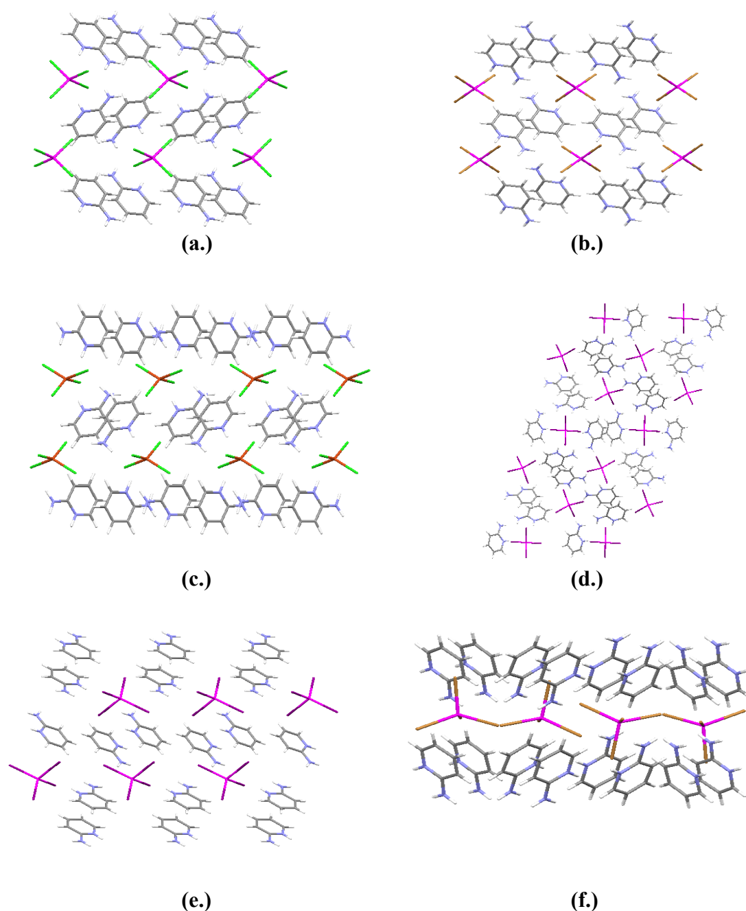
Figure 40: (a.) Structure of 2ampZnCl , viewed down the a -axis. Isostructural to 2ampCoCl (Jebas et al , 2006; DELPOA) number 3 in the literature survey. (b.) Structure of 2ampZnBr , viewed down the b -axis, isostructural to 2ampHgCl . (c.) Structure of 2ampCuCl (Kumar et al , 2005; YAPNAS01), viewed down the a -axis. Isostructural to 2ampCuBr (Luque et al , 1997; RIPWIW) and 3ampCuCl (Kumar et al , 2005; PATMUT) ( 1 , 2 and 6 in the literature survey). (d.) Structure of 2ampZnI , viewed down the b -axis. (e.) Structure of 2ampCdI , viewed down the a -axis, isostructural to 2ampHgI . (f.) Structure of 2ampHgBr .
