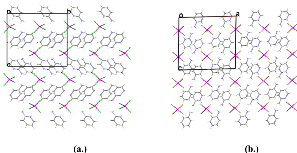
Figure 39: (a.) Structure 2ampZnCl ( Class 2A1 ), viewed down the a -axis, showing alternating orientation of cation pairs. (b.) Structure 2ampZnBr ( Class 2A2 ), viewed down the b -axis, illustrating the same orientation adopted by cation pairs.
