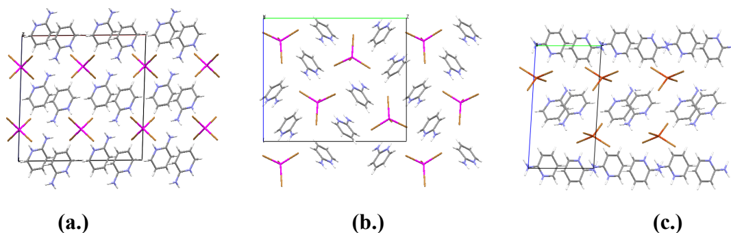
Figure 55: Packing in 2-aminopyridinium tetrabromometallates. (a.) 2ampZnBr , viewed down the b -axis. (b.) 2ampHgBr , viewed down the a -axis. (c.) 2ampCuBr , viewed down the a -axis (Luque et al , 1997; RIPWIW).
