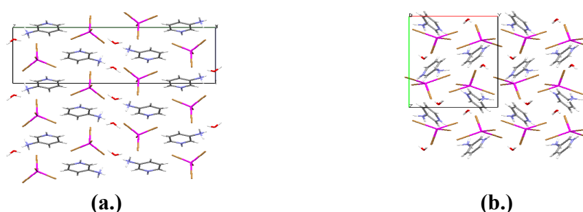
Figure 58: Packing in (a.) 3ampZnBr·H 2 O viewed down the a -axis and (b.) 3ampHgBr·H 2 O viewed down the c -axis (Ali et al , 2008; TOBCOD).
