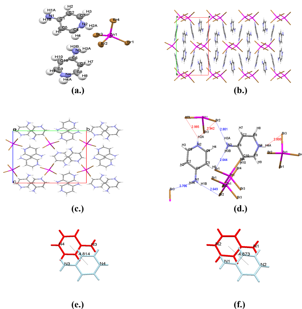
Figure 31: (a.) Asymmetric unit of 4ampZnBr . (b.) Crystal structure of 4ampZnBr , viewed down the c -axis. Space group P2_12_12_1 . Isostructural to 4ampZnCl and 4ampZnI . (c.) Structure viewed down a -axis. (d.) Intermolecular interactions. (e.) and (f.) Cation orientation.
