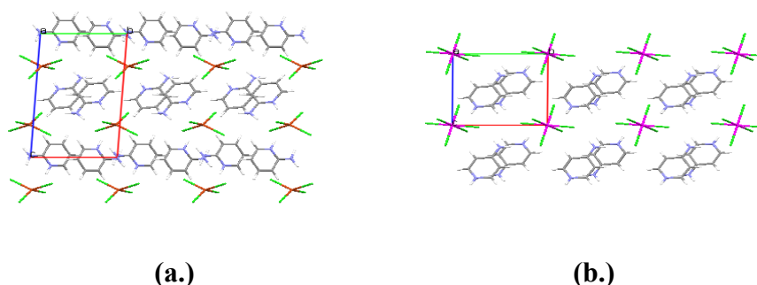
Figure 9: Crystal structures from literature in the space group P\bar{1} . (a.) Crystal structure of 2ampCuCl (1) (Kumar et al , 2005; YAPNAS01), viewed down the a -axis. Isostructural to 2ampCuBr (2) (Luque et al , 1997; RIPWIW) and 3ampCuCl (6) (Kumar et al , 2005; PATMUT). (b.) Crystal structure of 4ampSnCl (16) (Rademeyer et al , 2007; RIGDER), viewed down the a -axis.
