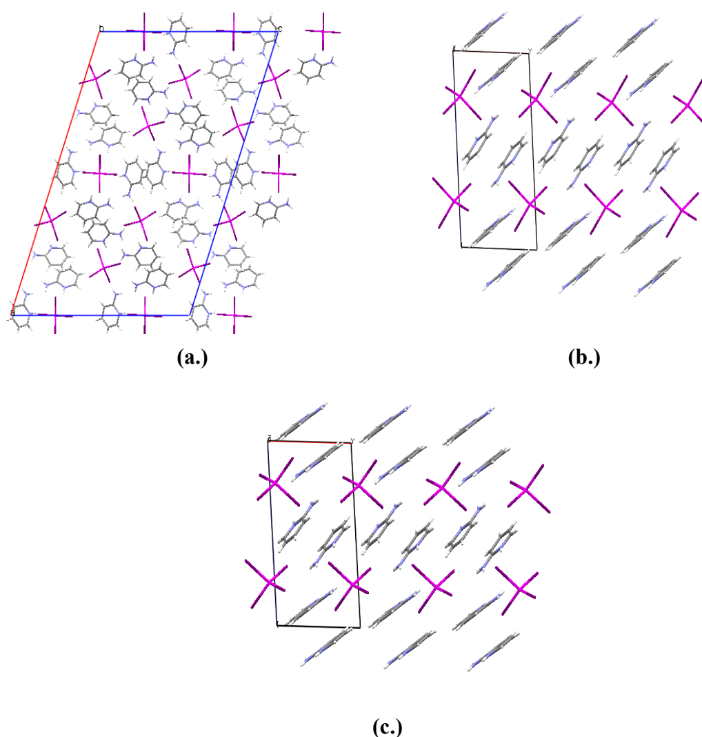
Figure 56: (a.) 2ampZnI viewed down the b -axis. (b.) 2ampCdI viewed down the b -axis and (c.) 2ampHgI viewed down the b -axis.
