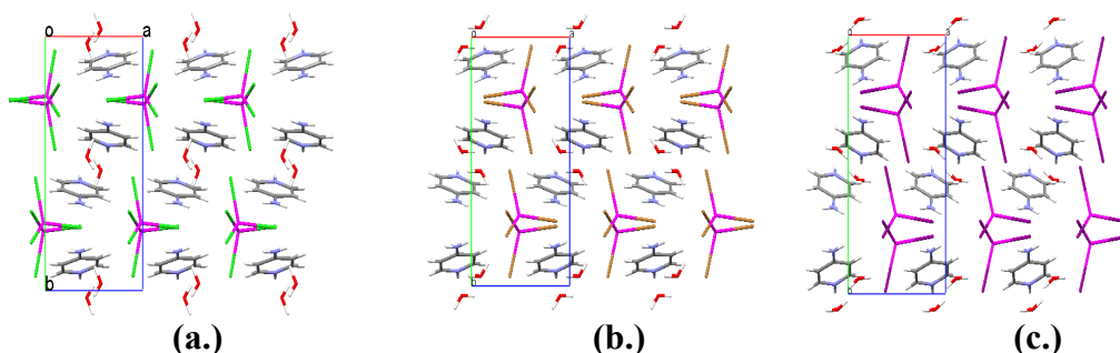
Figure 69: (a.) 4ampHgCl·H 2 O, viewed down the c -axis. (b.) 4ampHgBr·H 2 O, viewed down the c -axis and (c.) 4ampHgI·H 2 O, viewed down the c -axis.
