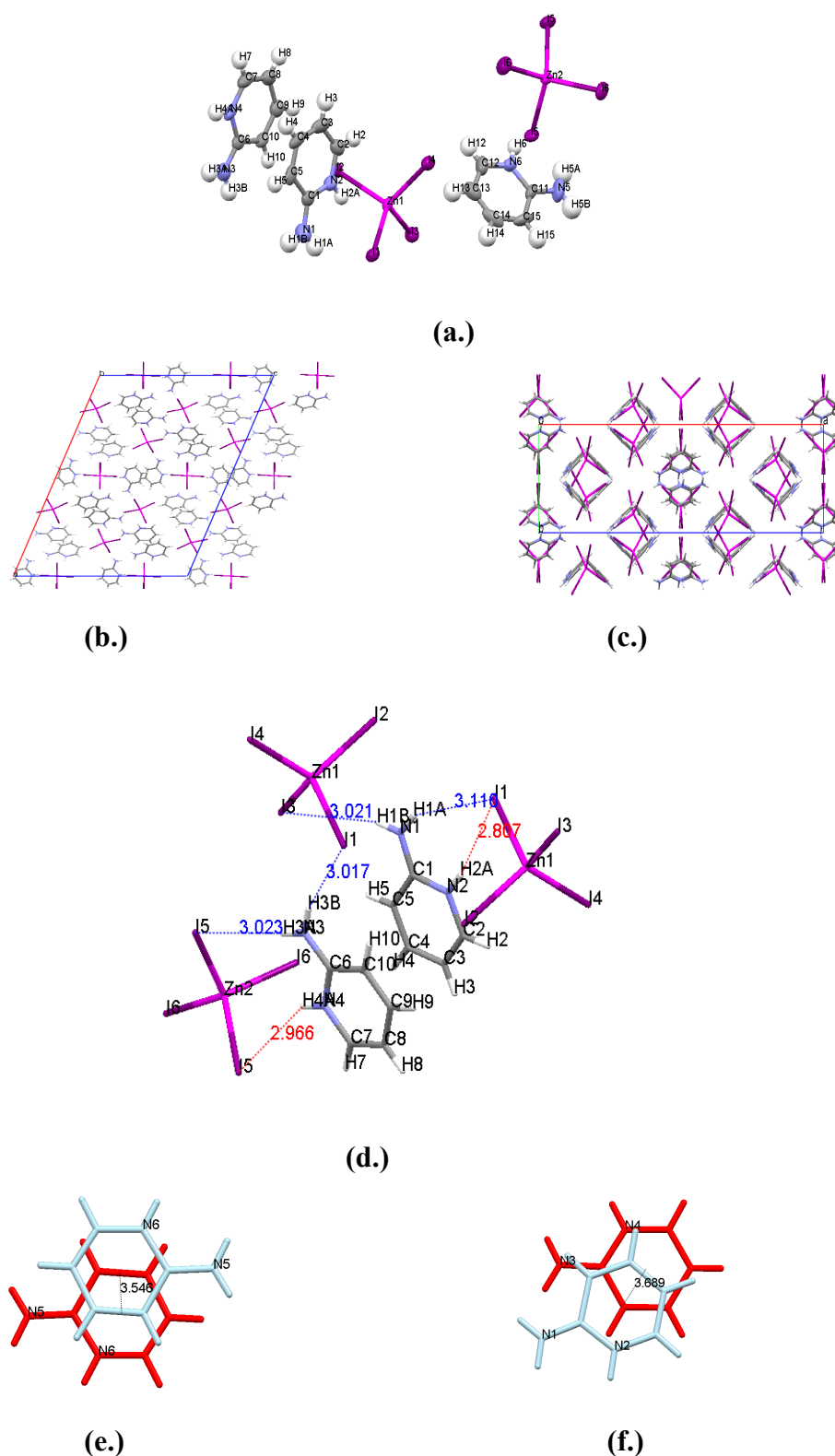
Figure 23: (a.) Asymmetric unit of 2ampZnI (full anion is shown for clarity). (b.) Crystal structure of 2ampZnI , viewed down the b -axis. (c.) Structure viewed down the c -axis. (d.) Hydrogen bonding interactions. (e.) and (f.) Cation orientation.
