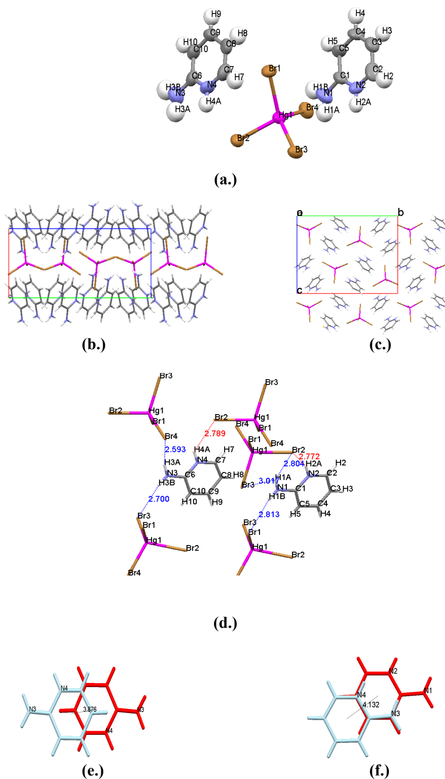
Figure 26: (a.) Asymmetric unit of 2ampHgBr . (b.) Crystal structure of 2ampHgBr , viewed down the c -axis. (c.) Structure viewed down the a -axis. (d.) Hydrogen bonding interactions. (e.) and (f.) Cation orientation.
