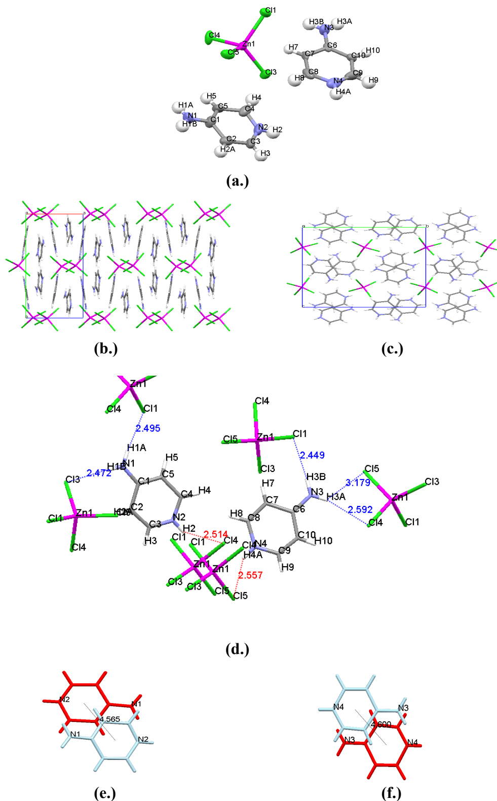
Figure 30: (a.) Asymmetric unit of 4ampZnCl . (b.) Crystal structure of 4ampZnCl , viewed down the c -axis. Space group P2_12_12_1 . Isostructural to 4ampZnBr and 4ampZnI . (c.) Structure viewed down the a -axis. (d.) Intermolecular interactions. (e.) and (f.) Cation orientation.
