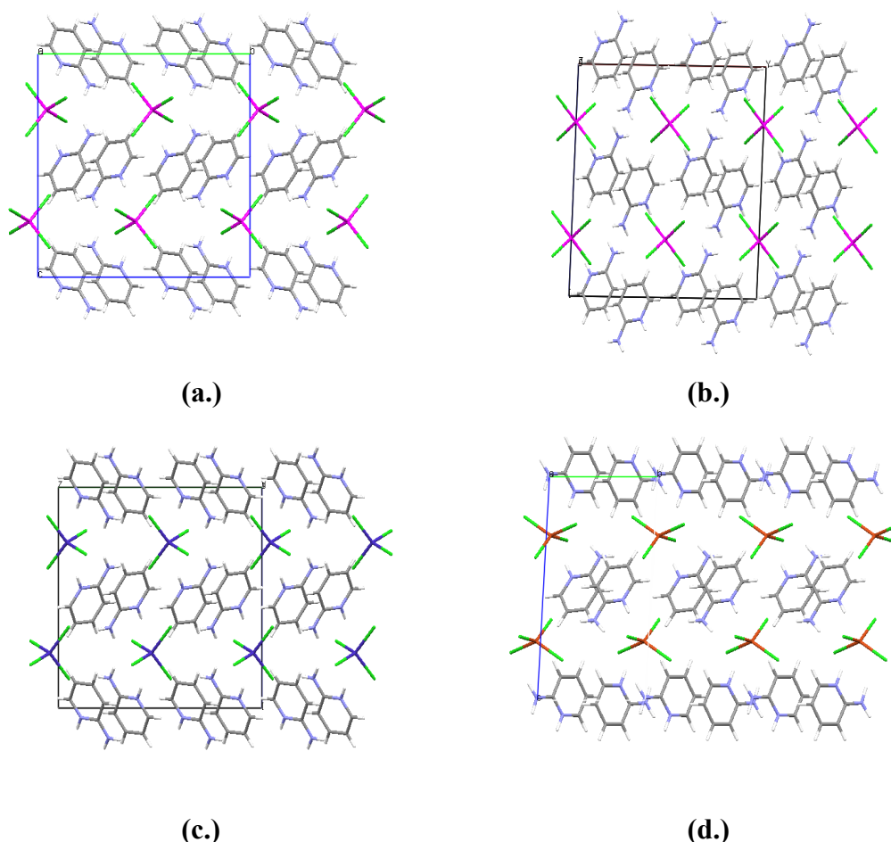
Figure 54: Packing in 2-aminopyridinium tetrachlorometallate structures. (a.) 2ampZnCl , viewed down the a -axis. (b.) 2ampHgCl , viewed down the b -axis. (c.) 2ampCoCl , viewed down the a -axis (Jebas et al , 2006; DELPOA), (d.) 2ampCuCl , viewed down the a -axis (Kumar et al , 2005; YAPNAS01).
