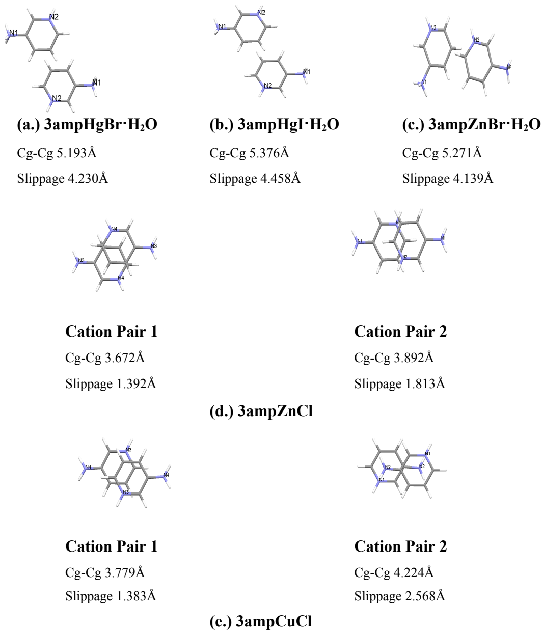
Figure 44: Cation pair orientation in (a.) 3ampHgBr·H 2 O (Ali, 2008; TOBCOD). (b.) 3ampHgI·H 2 O. (c.) 3ampZnBr·H 2 O. (d.) 3ampZnCl and (e.) 3ampCuCl.
