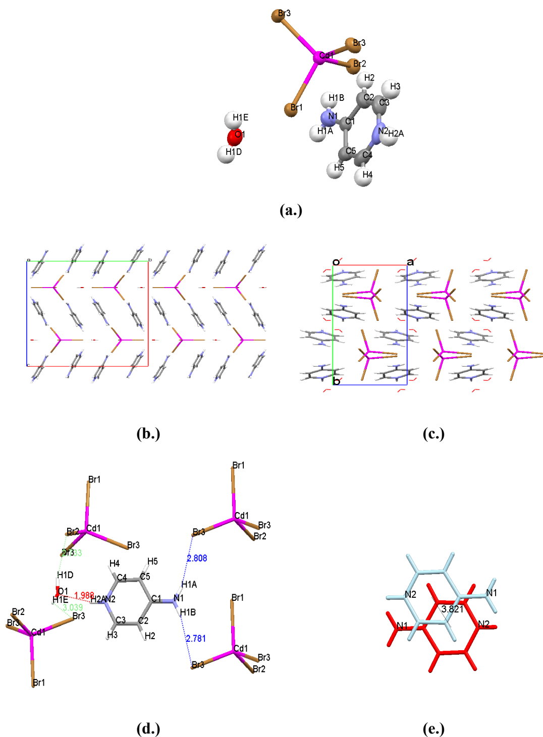
Figure 34: (a.) Asymmetric unit of 4ampCdBr·H 2 O (full anion showed for clarity). (b.) Crystal structure of 4ampCdBr·H 2 O , viewed down the a -axis. Space group Pbcm . Isostructural to 4ampCdI·H 2 O , 4ampHgCl·H 2 O , 4ampHgBr·H 2 O and 4ampHgI·H 2 O . (c.) Structure viewed down c -axis. (d.) Charge assisted intermolecular interactions. (e.) Cation orientation.
