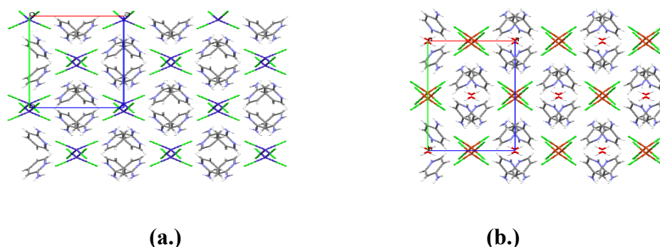
Figure 10: Crystal structures from literature in the space group C2/c . (a.) Crystal structure of 2ampCoCl (3) (Jebas et al , 2006; DELPOA), viewed down the c -axis. (b.) Crystal structure of 4ampCuCl·H 2 O (9) (Halvorson et al , 1990; SEZLEO), viewed down the c -axis. Isostructural to 4ampCuBr·H 2 O (10) (Román et al , 1996; ZUDKUE).
