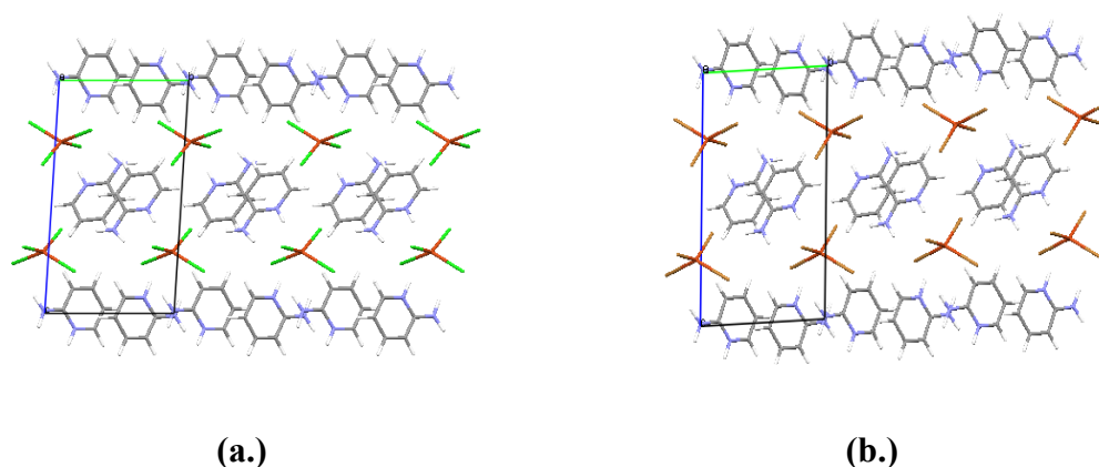
Figure 64: (a.) 2ampCuCl, viewed down the a -axis (Kumar et al , 2005; YAPNAS01) and (b.) 2ampCuBr, viewed down the a -axis (Luque et al , 1997; RIPWIW).
