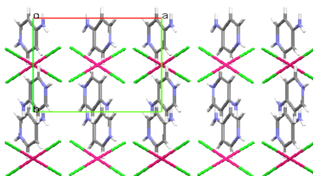
Figure 13: Crystal structure of 4ampCuBr (1) (Sertucha et al , 1998; LAHYAU), space group P4_2/n , viewed down the c -axis.
