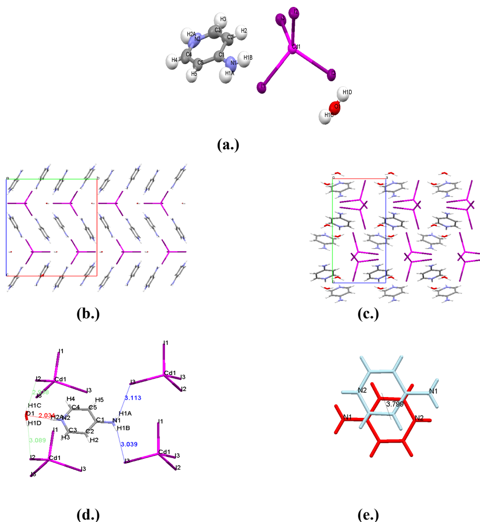
Figure 35: (a.) Asymmetric unit of 4ampCdI·H 2 O . (b.) Crystal structure of 4ampCdI·H 2 O , viewed down the a -axis. Space group Pbcm . Isostructural to 4ampCdBr·H 2 O , 4ampHgCl·H 2 O , 4ampHgBr·H 2 O and 4ampHgI·H 2 O . (c.) Structure viewed down c -axis. (d.) Charge assisted intermolecular interactions. (e.) Cation orientation.
