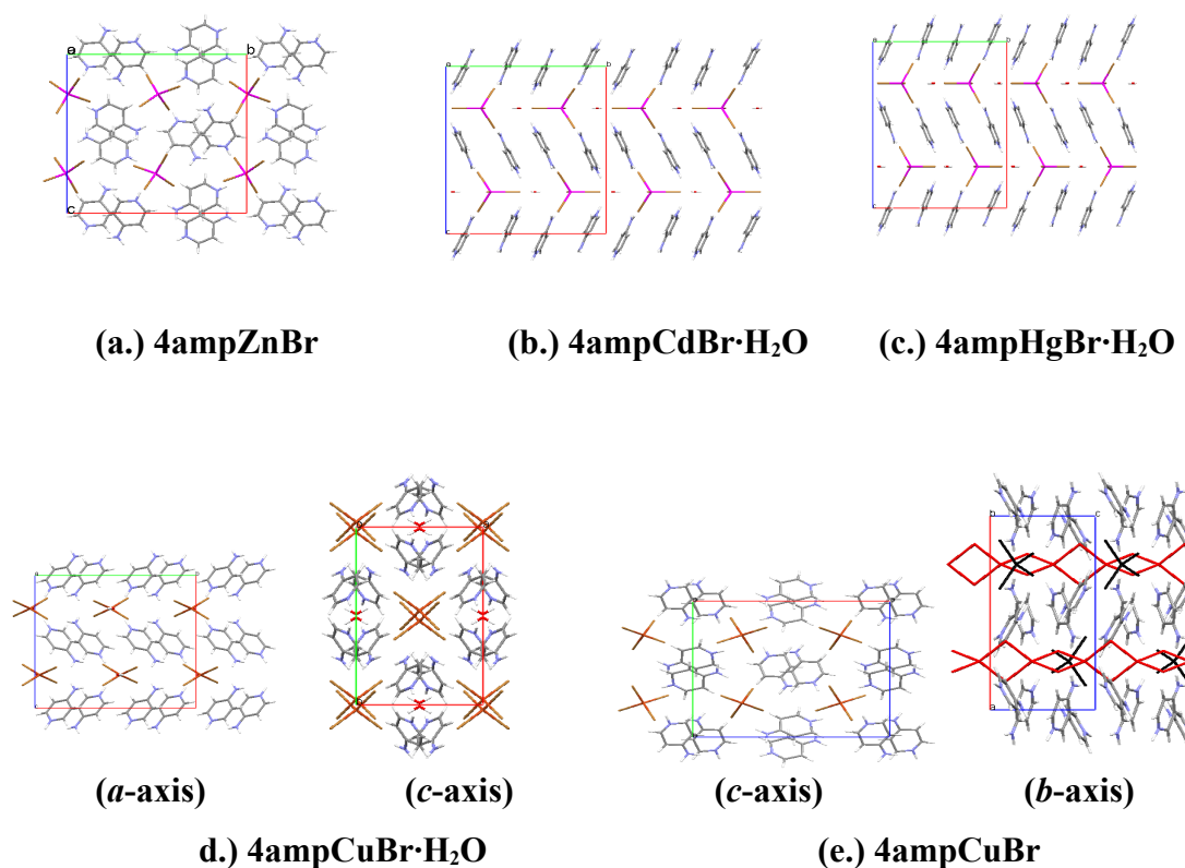
Figure 60: (a.) 4ampZnBr , viewed down the c -axis. (b.) 4ampCdBr·H 2 O , viewed down the a -axis. (c.) 4ampHgBr·H 2 O , viewed down the a -axis. (d.) 4ampCuBr·H 2 O , left: viewed down the a -axis, right: viewed down the c -axis (Román et al , 1996; ZUDKUE) and (e.) 4ampCuBr , left: viewed down the c -axis, right: viewed down the b -axis (Sertucha et al , 1998; LAHYAU).
