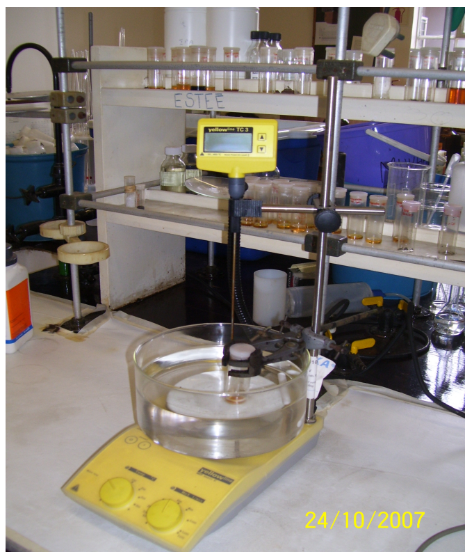
Figure 19: Apparatus for temperature controlled crystallization.
