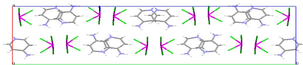
Figure 12: Crystal structure of 4ampSbCl (12) (Jakubas et al , 2003; XUQQAB), space group Cc , viewed down the c -axis. Similar to structures in Figure 11 , of space group P2_1/c .
