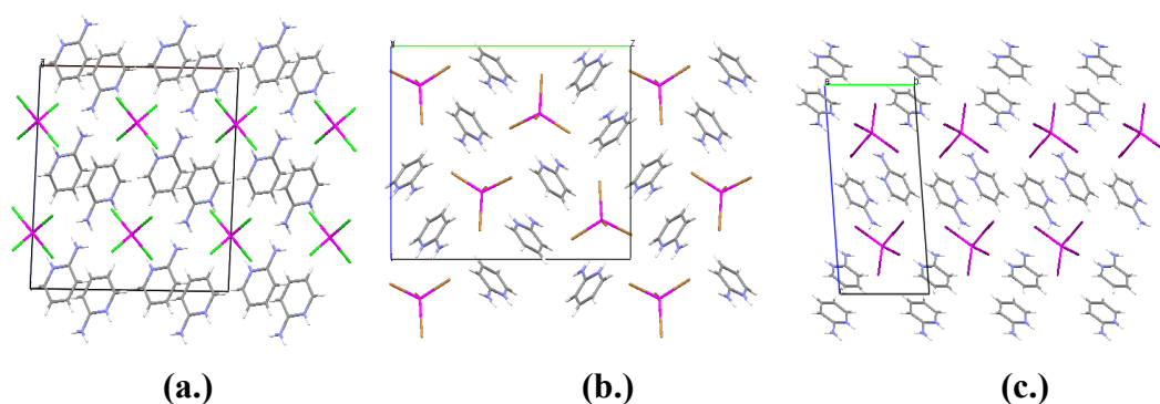
Figure 63: (a.) 2ampHgCl, viewed down the b -axis. (b.) 2ampHgBr viewed down the a -axis and (c.) 2ampHgI, viewed down the a -axis.
