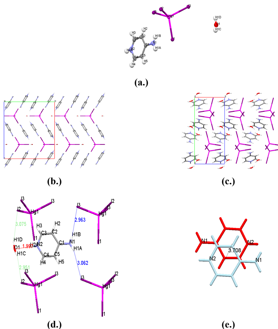
Figure 38: (a.) Asymmetric unit of 4ampHgI·H 2 O . (b.) Crystal structure of 4ampHgI·H 2 O , viewed down the a -axis. Space group Pbcm . Isostructural to 4ampHgCl·H 2 O , 4ampHgBr·H 2 O , 4ampCdBr·H 2 O and 4ampCdI·H 2 O . (c.) Structure viewed down c -axis. (d.) Charge assisted intermolecular interactions. (e.) Cation orientation.
