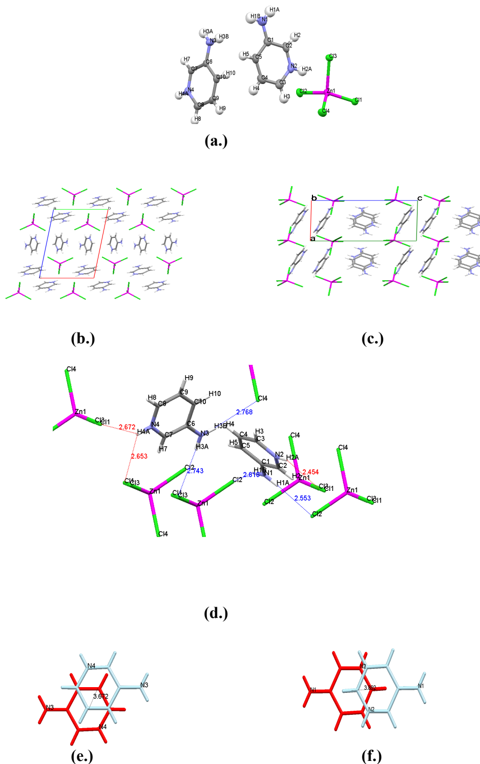
Figure 27: (a.) Asymmetric unit of 3ampZnCl . (b.) Crystal structure of 3ampZnCl , viewed down the a -axis, showing the organic and inorganic layers. (c.) Structure viewed down b -axis. (d.) Charge assisted intermolecular interactions in the crystal structure of 3ampZnCl . (e.) and (f.) Cation orientation.
