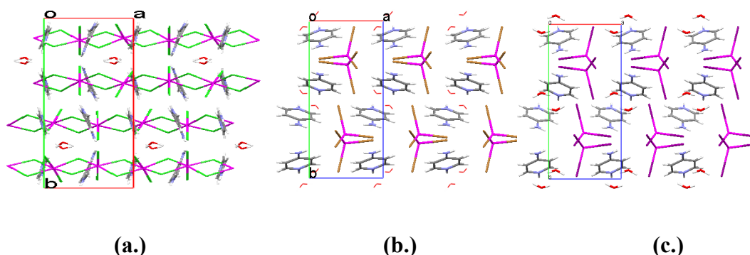
Figure 68: (a.) 4ampCdCl·H 2 O, viewed down the c -axis. (b.) 4ampCdBr·H 2 O, viewed down the c -axis and (c.) 4ampCdI·H 2 O, viewed down the c -axis.
