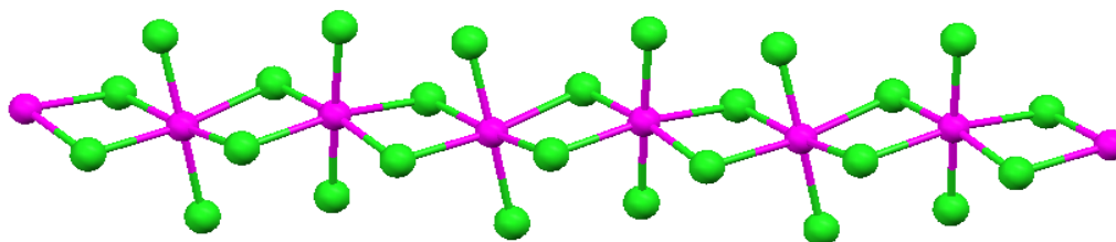
Figure 49: Polymeric anion observed for 4ampCdCl·H 2 O .
