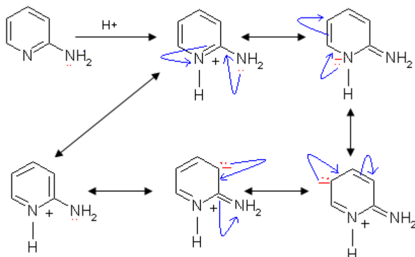
Figure 6: Resonance structures of 2-aminopyridinium. Adapted from Bordwell et al , 1992.
