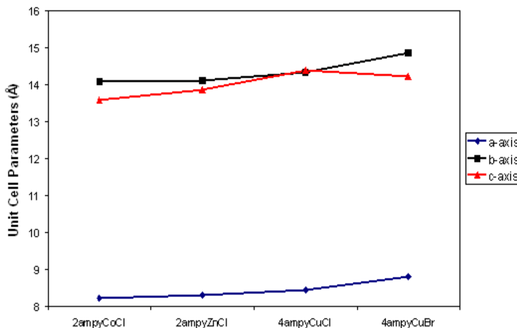
Figure 51: Unit cell parameters of isostructural compounds in the 2-aminopyridinium and 4-aminopyridinium family.
