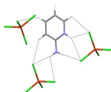
Cation 1
