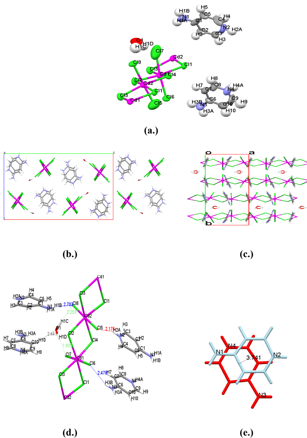
Figure 33: (a.) Asymmetric unit of 4ampCdCl·H 2 O . (b.) Crystal structure of 4ampCdCl·H 2 O , viewed down the a -axis. (c.) Structure viewed down c -axis. (d.) Charge assisted intermolecular interactions in the crystal structure of 4ampCdCl·H 2 O . (e.) Cation stacking, rotated relative to each other.
