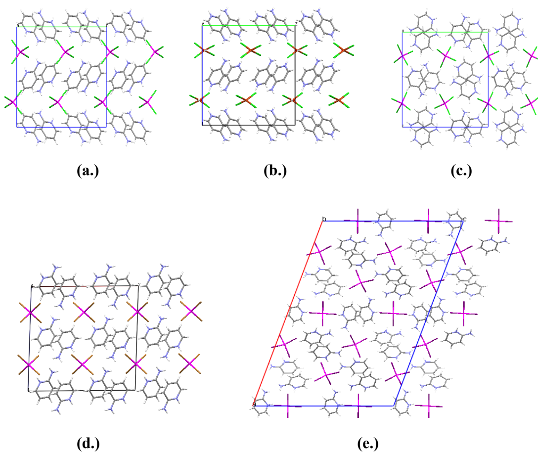
Figure 53: Layered structures with cation pairs in (a.) 2ampZnCl , viewed down the c -axis. (b.) 4ampCuCl·H 2 O (Halvorson et al , 1990; SEZLEO), viewed down the a -axis. (c.) 4ampZnCl , viewed down the a -axis. (d.) 2ampZnBr viewed down the b -axis and (e.) 2ampZnI viewed down the b -axis.
