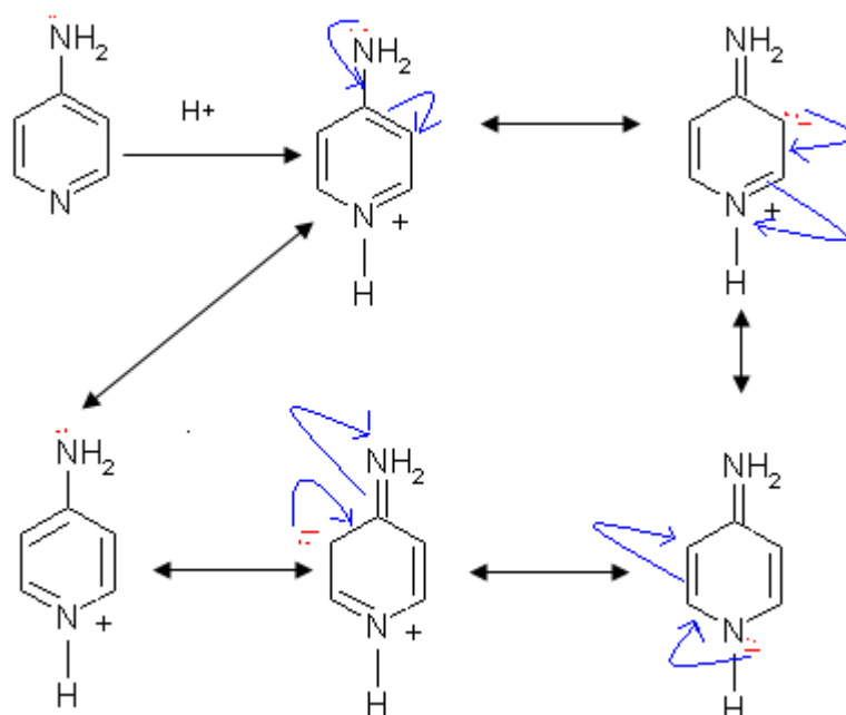
Figure 5: Resonance structures of 4-aminopyridinium. Adapted from Bordwell et al , 1992.
