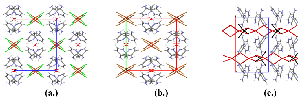
Figure 70: (a.) 4ampCuCl·H 2 O, viewed down the c -axis (Halvorson et al , 1990; SEZLEO). (b.) 4ampCuBr·H 2 O, viewed down the c -axis (Román et al , 1996; ZUDKUE) and (c.) 4ampCuBr, viewed down the c -axis (Sertucha et al , 1998; LAHYAU).
