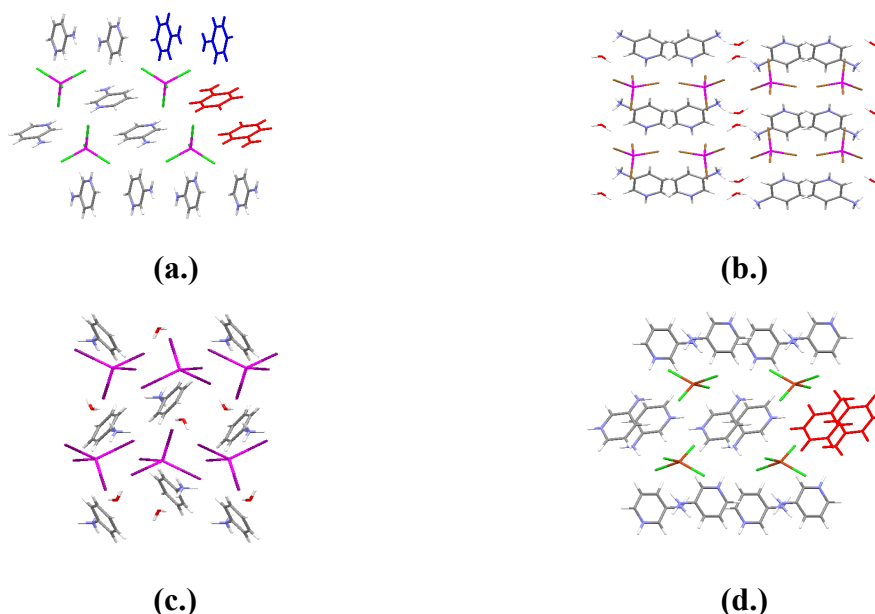
Figure 43: Layered structures observed for the 3-aminopyridinium and 3-ammoniopyridinium family. (a.) 3ampZnCl viewed down the a -axis. (b.) 3ampZnBr·H 2 O viewed down the b -axis. (c.) 3ampHgI·H 2 O , viewed down the c -axis. Isostructural to 3ampHgBr·H 2 O (Ali, 2008; TOBCOD). (d.) 3ampCuCl , viewed down the a -axis (Kumar et al , 2005; PATMUT).
