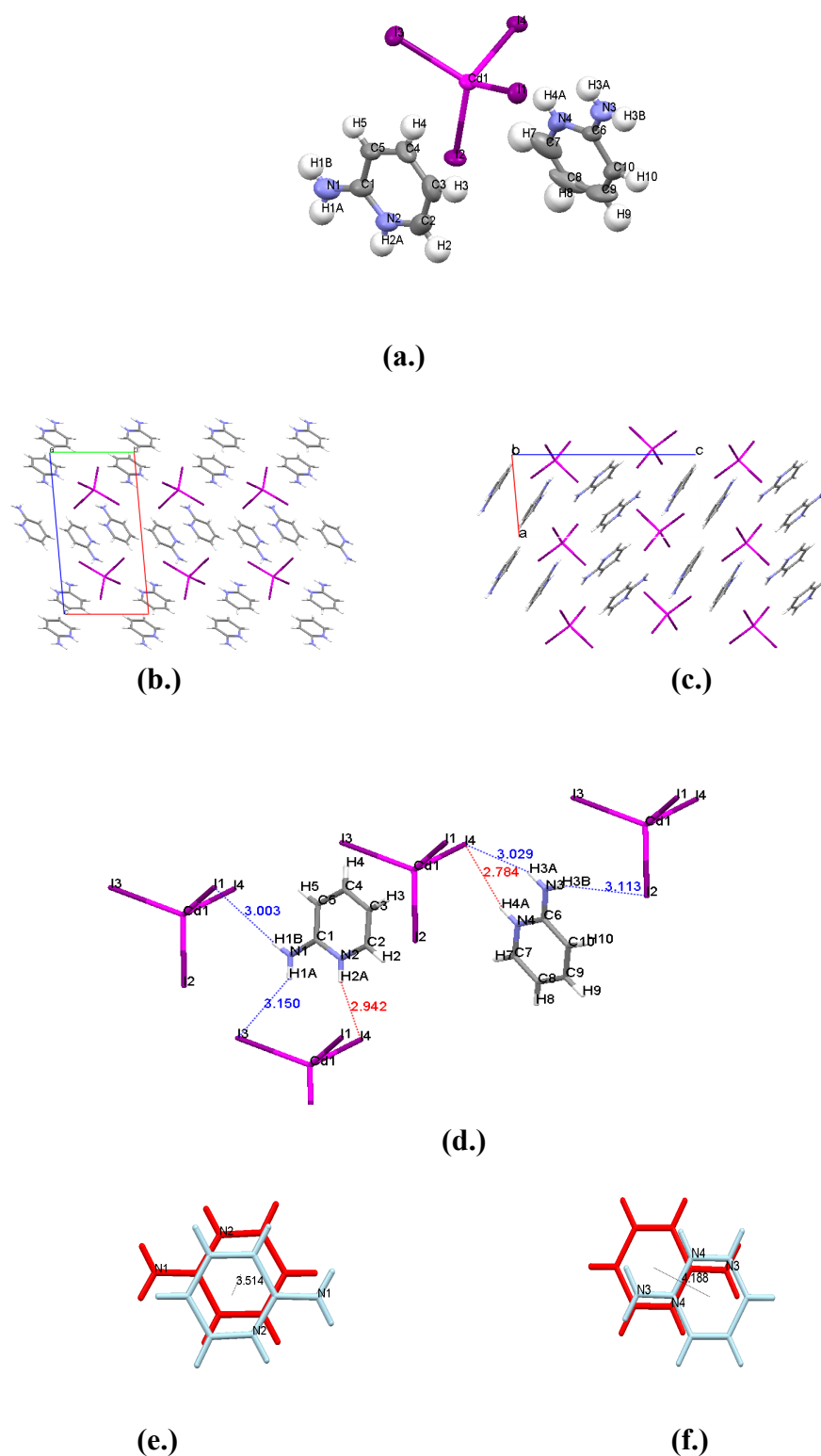
Figure 24: (a.) Asymmetric unit of 2ampCdI (full anion is shown for clarity). (b.) Crystal structure of 2ampCdI , viewed down the a -axis. Isostructural to 2ampHgI . (c.) Structure viewed down the b -axis. (d.) Hydrogen bonding interactions. (e.) and (f.) Cation orientation.
