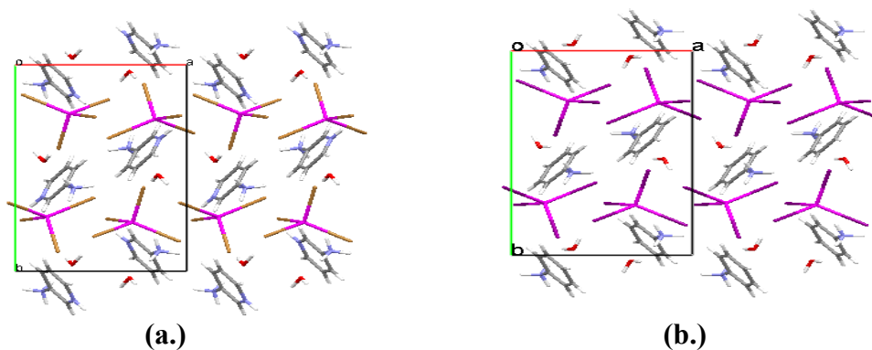
Figure 66: (a.) 3ampHgBr·H 2 O , viewed down the c -axis and (b.) 3ampHgI·H 2 O , viewed down the c -axis.
