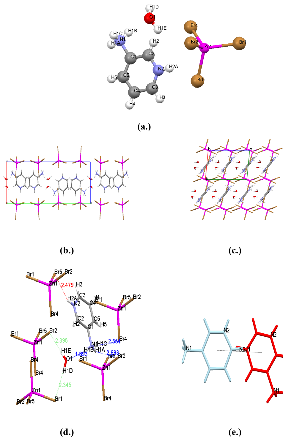
Figure 28: (a.) Asymmetric unit of 3ampZnBr·H 2 O . (b.) Crystal structure of 3ampZnBr·H 2 O , viewed down the c -axis (c.) Structure viewed down b -axis. (d.) Charge assisted intermolecular interactions in the crystal structure of 3ampZnBr·H 2 O . (e.) Cation orientation.
