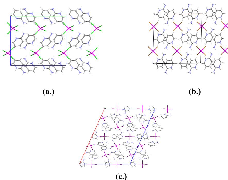
Figure 62: (a.) 2ampZnCl , viewed down the a -axis. (b.) 2ampZnBr , viewed down the b -axis and (c.) 2ampZnI viewed down the b -axis.
