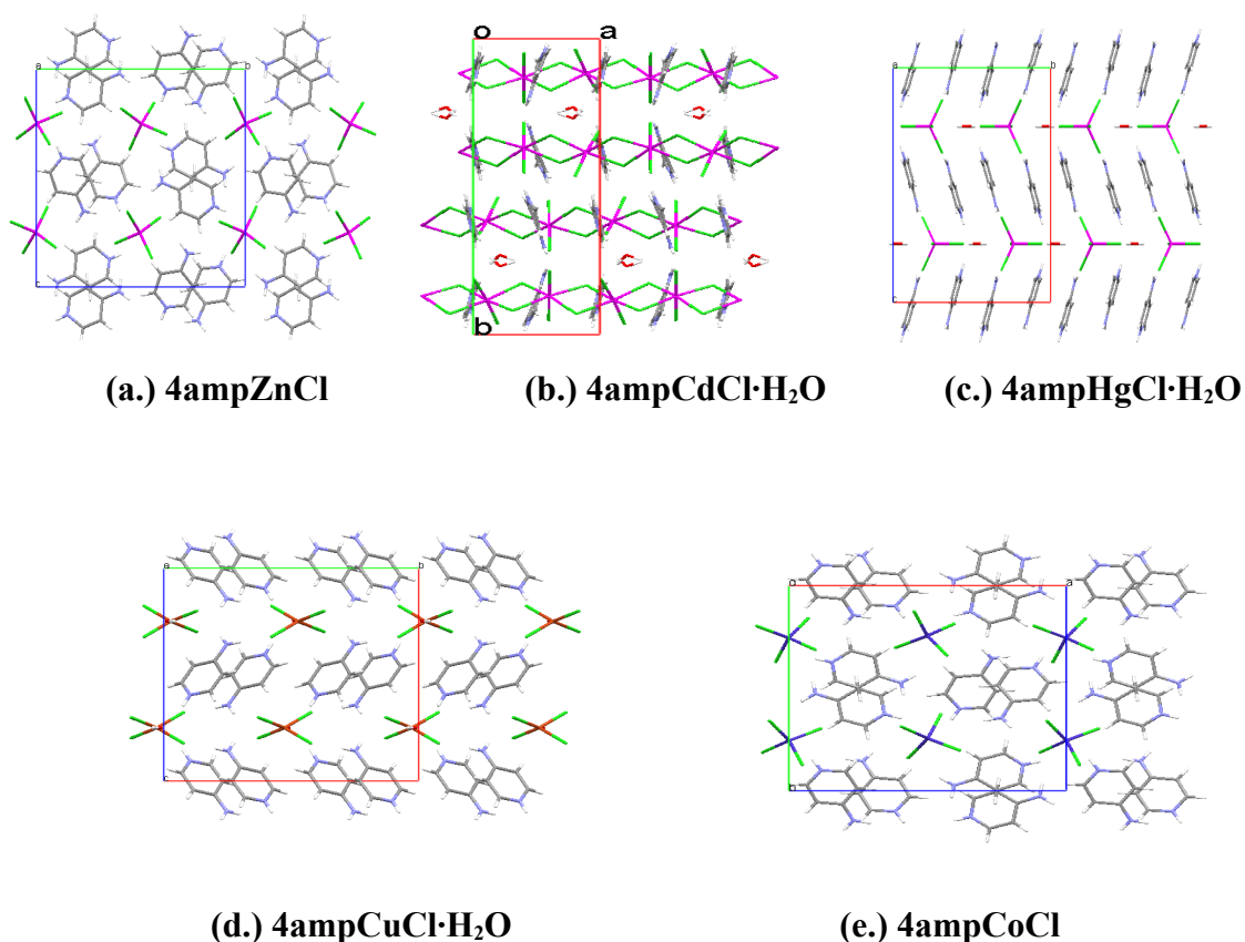
Figure 59: (a.) 4ampZnCl , viewed down the a -axis. (b.) 4ampCdCl·H 2 O , viewed down the c -axis. (c.) 4ampHgCl·H 2 O , viewed down the a -axis. (d.) 4ampCuCl·H 2 O , viewed down the a -axis (Halvorson et al , 1990; SEZLEO) and (e.) 4ampCoCl viewed down the c -axis (Jebas et al , 2009; HOSVIV).
