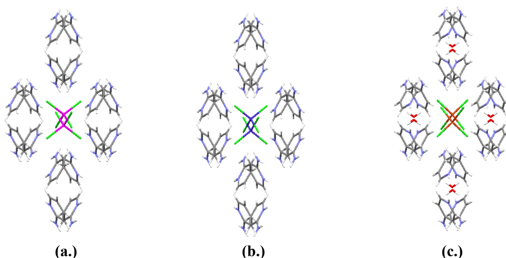
Figure 50: (a.) Crystal structure of 2ampZnCl , viewed down the c -axis (Class 2A1). (b.) Crystal structure of 2ampCoCl , viewed down the c -axis (Jebas et al , 2006; DELPOA). (c.) Crystal structure of 4ampCuCl·H 2 O , viewed down the c -axis (Halvorson et al , 1990; SEZLEO), isostructural to ( 4ampCuBr·H 2 O (Román, 1996; ZUDKUE), showing the incorporation of water molecules.
