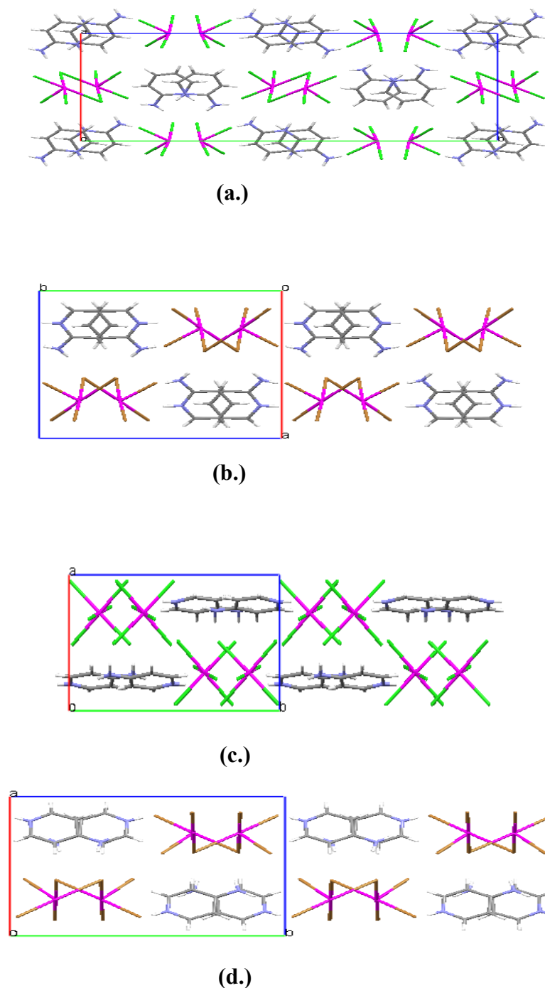
Figure 11: Crystal structures from literature in the space group P2_1/c , all viewed down the c -axis. (a.) Crystal structure of 2ampSbCl (4) (Kulicka et al , 2004; NAKLIV). (b.) Crystal structure of 2ampSbBr (5) (Kulicka et al , 2004; NAKLER). (c.) Crystal structure of 4ampSbCl (octahedron) (13) (Kulicka et al , 2006; ECAPUU). (d.) Crystal structure of 4ampSbBr (14) (Hashimoto et al , 2003; ENIKIV).
