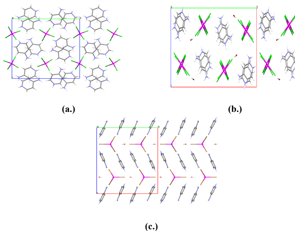
Figure 46: Layered structures observed for the 4-aminopyridinium family. (a.) 4ampZnCl , viewed down the a -axis, observed for Class 4A structures. (b.) 4ampCdCl·H 2 O , viewed down the a -axis, observed for Class 4B structures. (c.) 4ampCdBr·H 2 O , viewed down the a -axis, observed for Class 4C structures.
