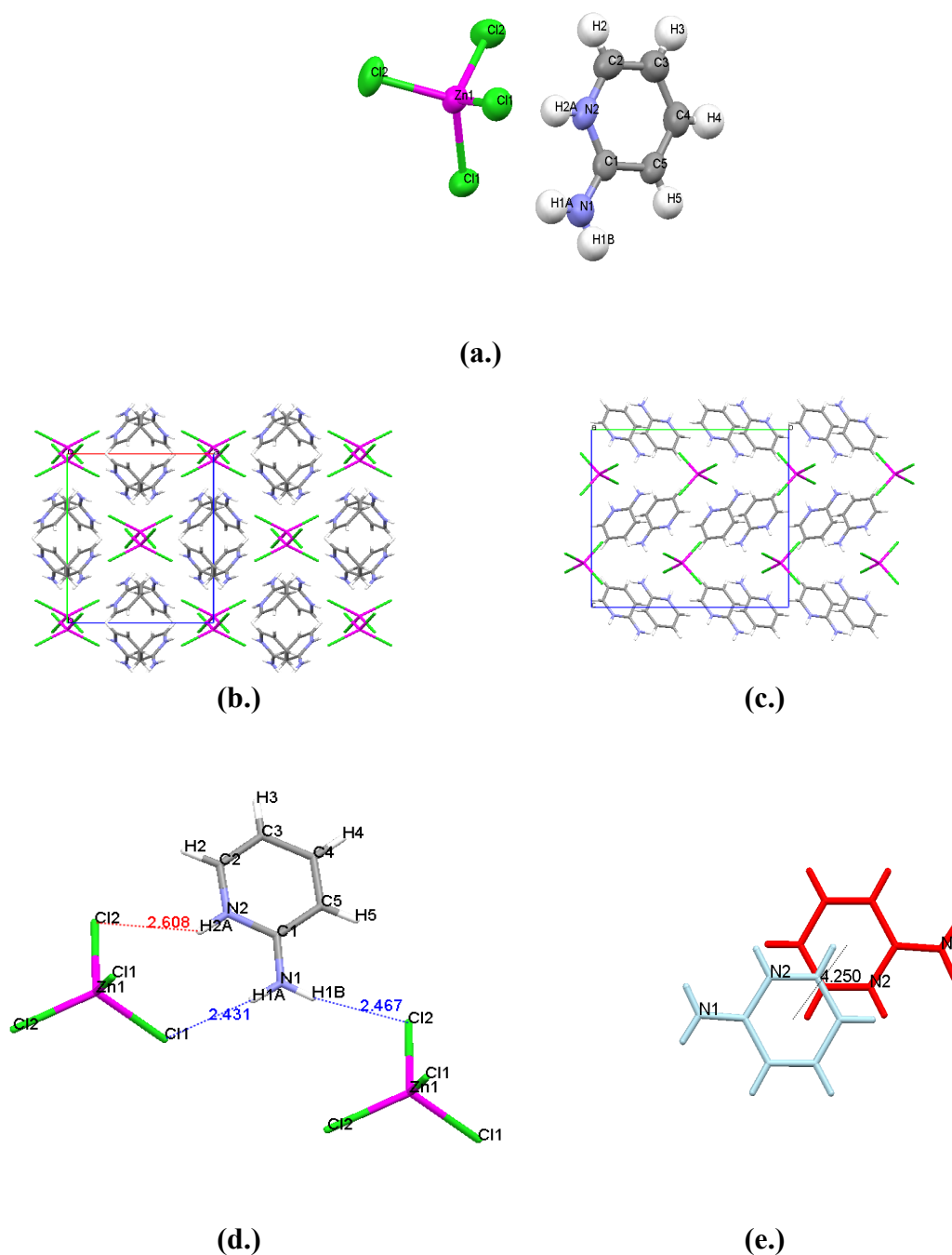
Figure 20: (a.) Asymmetric unit of 2ampZnCl (full anion is shown for clarity). (b.) Crystal structure of 2ampZnCl , viewed down the c -axis. Isostructural to 2ampZnBr and 2ampHgCl . (c.) Crystal structure of 2ampZnCl , viewed down the a -axis, showing the organic and inorganic layers. (d.) Hydrogen bonding interactions. (e.) Cation orientation.
