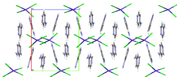
Figure 17: Crystal structure of 4ampCoCl (17) (Jebas et al , 2009; HOSVIV), space group P2_12_12_1 , viewed down the b -axis.
