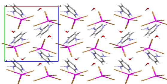
Figure 15: Crystal structure of 3ampHgBr·H 2 O (7) (Ali et al , 2008; TOBCOD), space group P2_1/n , viewed down the c -axis.
