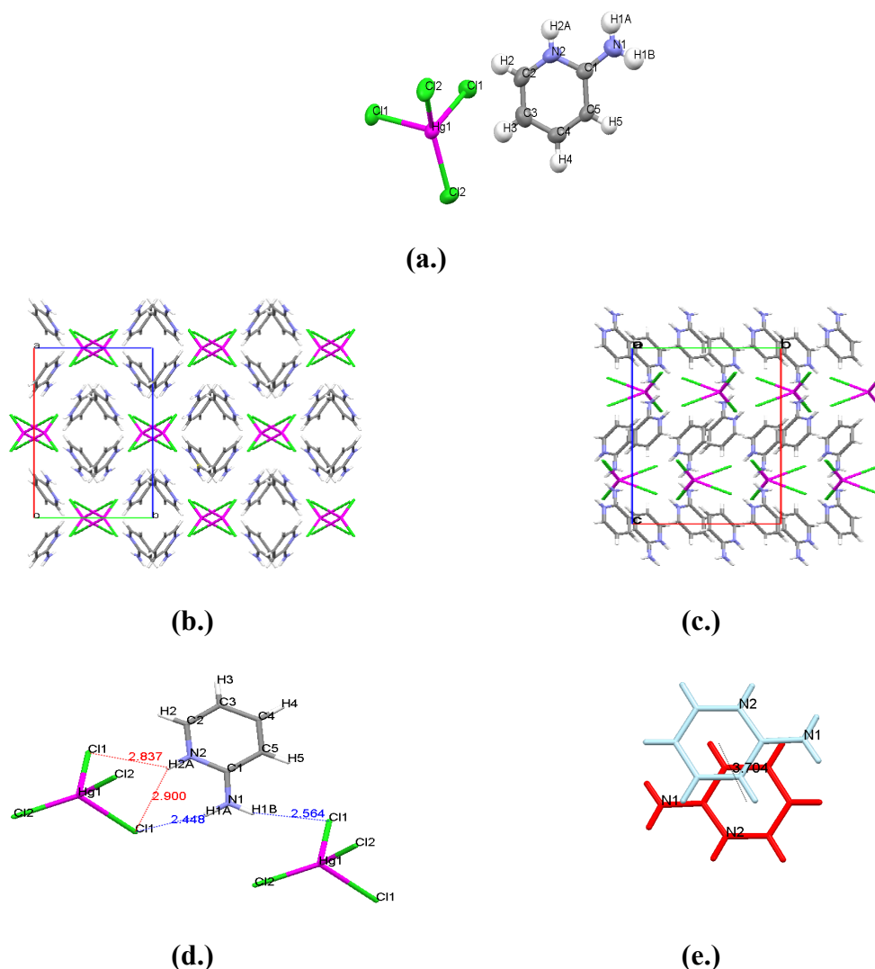
Figure 22: (a.) Asymmetric unit of 2ampHgCl (full anion is shown for clarity) (b.) Crystal structure of 2ampHgCl , viewed down the c -axis. Isostructural to 2ampZnCl and 2ampZnBr . (c.) Crystal structure of 2ampHgCl , viewed down the a -axis, showing the organic and inorganic layers (d.) Hydrogen bonding interactions. (e.) Cation orientation.
