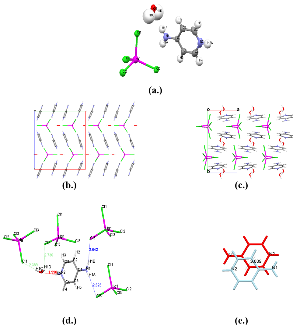
Figure 36: (a.) Asymmetric unit of 4ampHgCl·H 2 O . (b.) Crystal structure of 4ampHgCl·H 2 O , viewed down the a -axis. Space group Pbcm . Isostructural to 4ampCdBr·H 2 O , 4ampCdI·H 2 O , 4ampHgBr·H 2 O and 4ampHgI·H 2 O . (c.) Structure viewed down c -axis. (d.) Charge assisted intermolecular interactions. (e.) Cation orientation.
