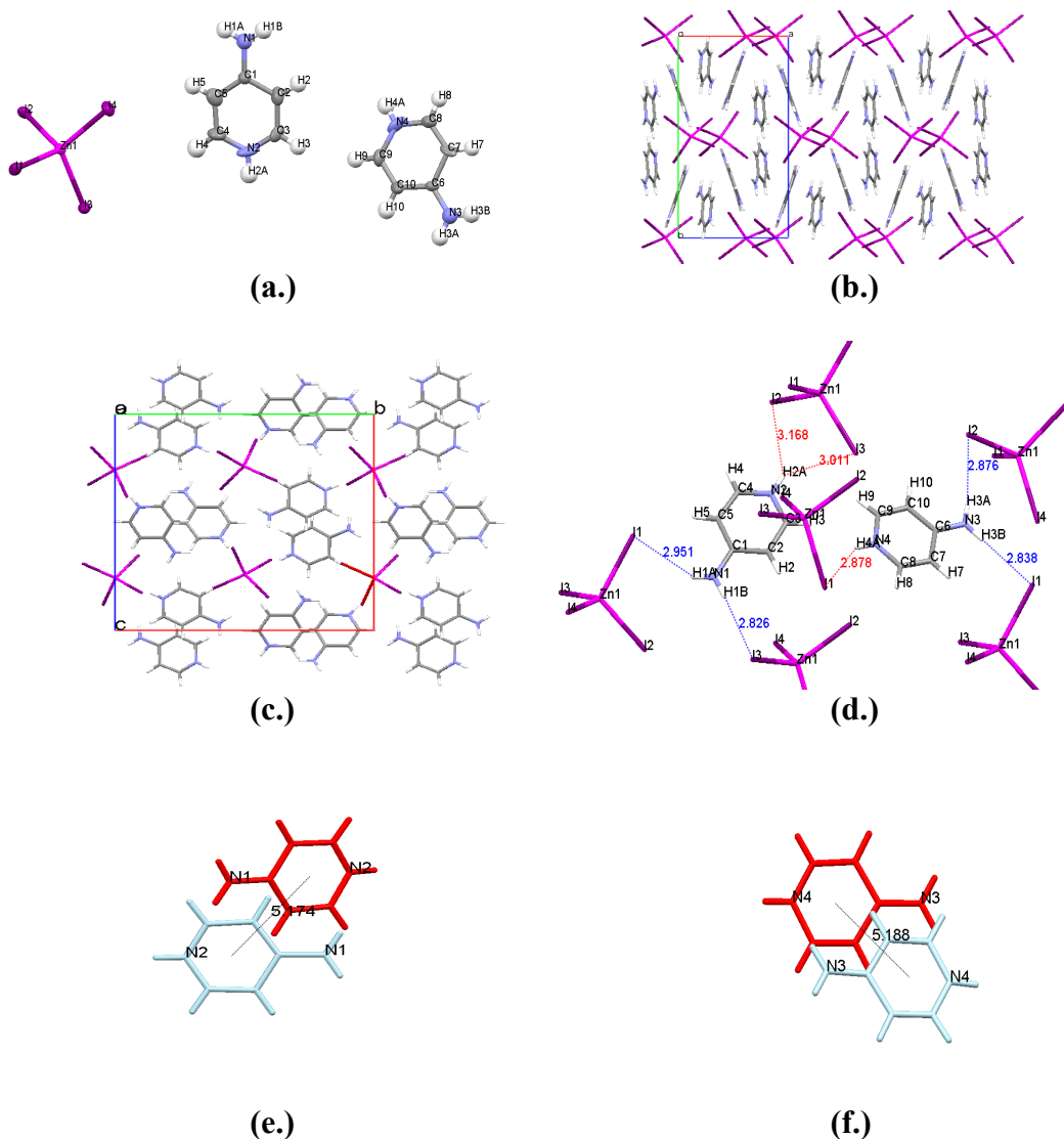
Figure 32: (a.) Asymmetric unit of 4ampZnI . (b.) Crystal structure of 4ampZnI , viewed down the c -axis. Space group P2_12_12_1 . Isostructural to 4ampZnCl and 4ampZnBr . (c.) Structure viewed down a -axis. (d.) Intermolecular interactions. (e.) and (f.) Cation orientation.
