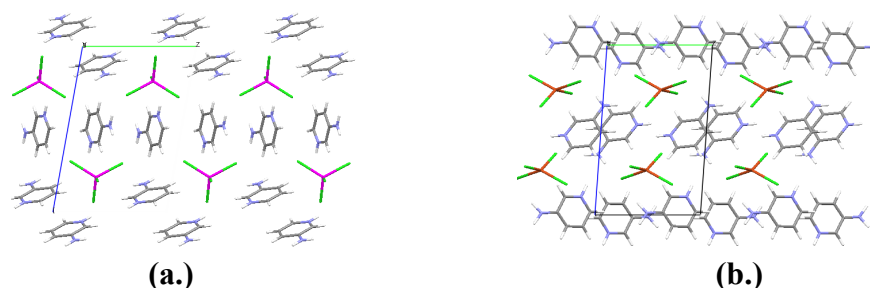
Figure 57: Packing in (a.) 3ampZnCl viewed down the a -axis and (b.) 3ampCuCl viewed down the a -axis (Kumar et al , 2005; PATMUT).
