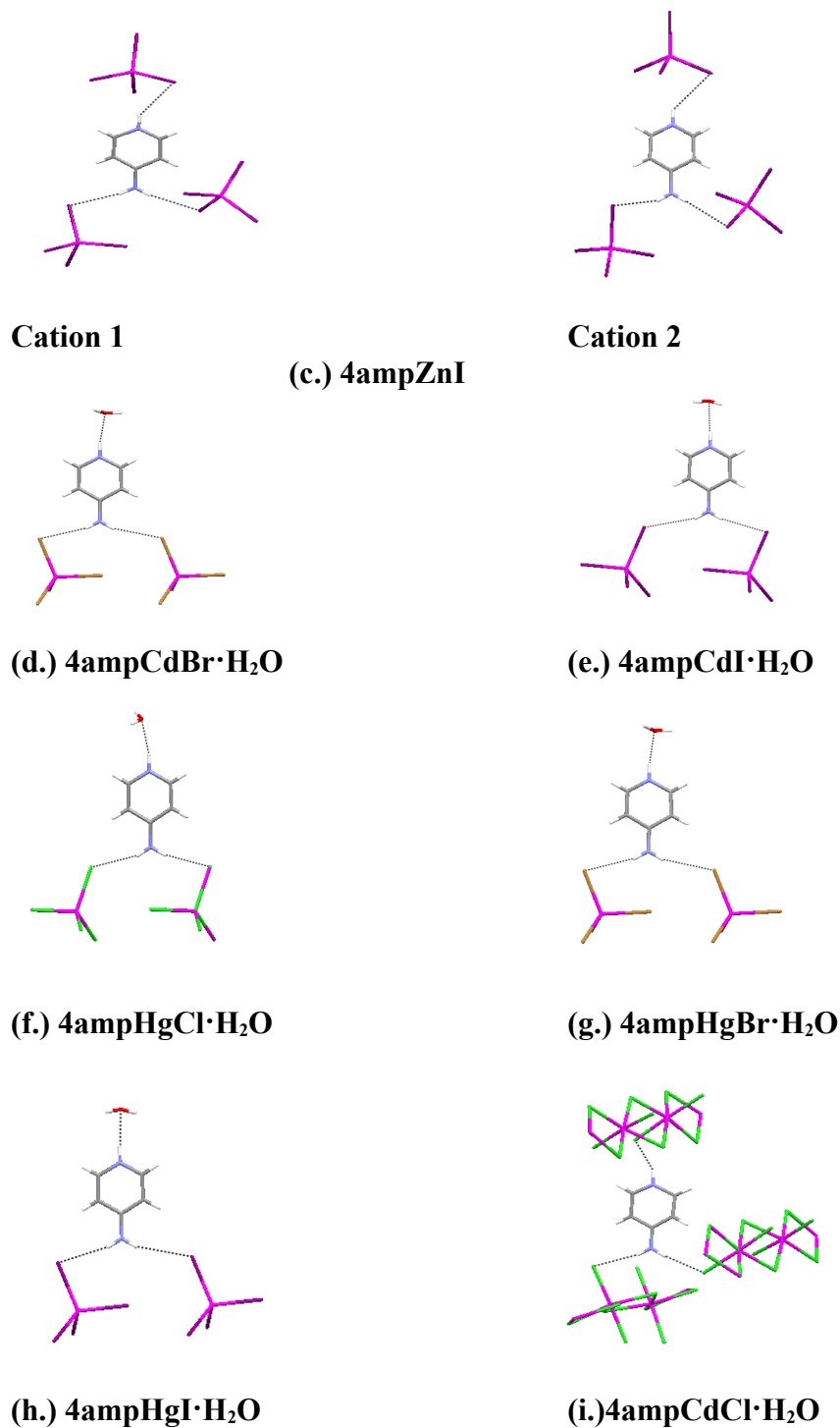
Figure 48: Identified synthons in (a.) 4ampZnCl, (b.) 4ampZnBr, (c.) 4ampZnI, (d.) 4ampCdBr·H 2 O, (e.) 4ampCdI·H 2 O, (f.) 4ampHgCl·H 2 O, (g.) 4ampHgBr·H 2 O, (h.) 4ampHgI·H 2 O and (i.) 4ampCdCl·H 2 O.
