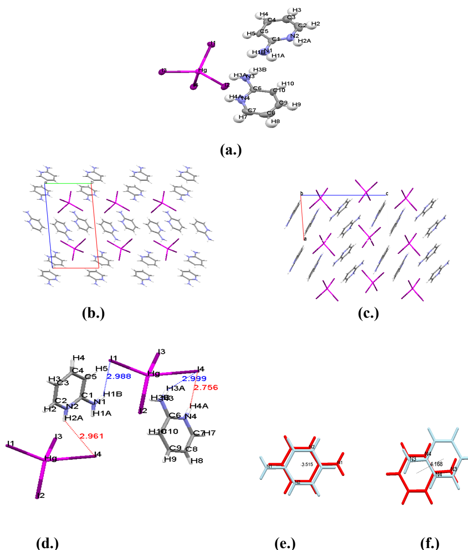
Figure 25: (a.) Asymmetric unit of 2ampHgI . (b.) Crystal structure of 2ampHgI , viewed down the a -axis. (Isostructural to 2ampCdI ). (c.) Structure viewed down the b -axis. (d.) Hydrogen bonding interactions. (e.) and (f.) Cation orientation.
