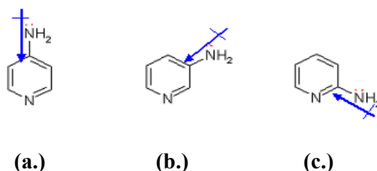
Figure 3: Illustration of the electron donating effect of \text{-NH}_2 in (a.) 4-aminopyridine, (b.) 3-aminopyridine and (c.) 2-aminopyridine.
