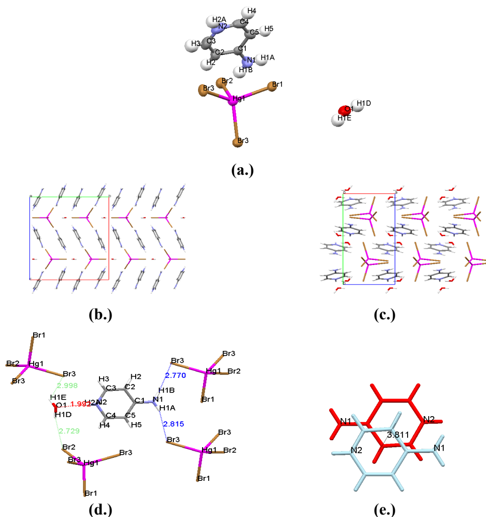
Figure 37: (a.) Asymmetric unit of 4ampHgBr·H 2 O . (b.) Crystal structure of 4ampHgBr·H 2 O , viewed down the a -axis. Space group Pbcm . Isostructural to 4ampHgCl·H 2 O , 4ampCdBr·H 2 O , 4ampCdI·H 2 O and 4ampHgI·H 2 O . (c.) Structure viewed down the c -axis. (d.) Charge assisted intermolecular interactions. (e.) Cation orientation.
