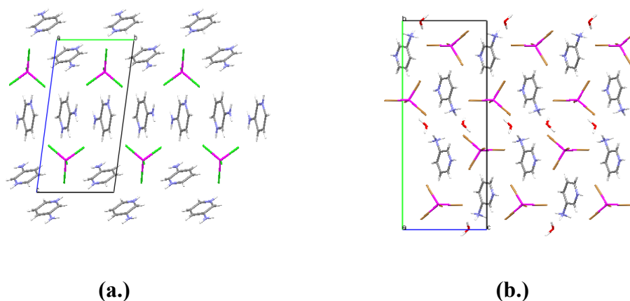
Figure 65: (a.) 3ampZnCl , viewed down the a -axis and (b.) 3ampZnBr·H 2 O , viewed down the a -axis.
