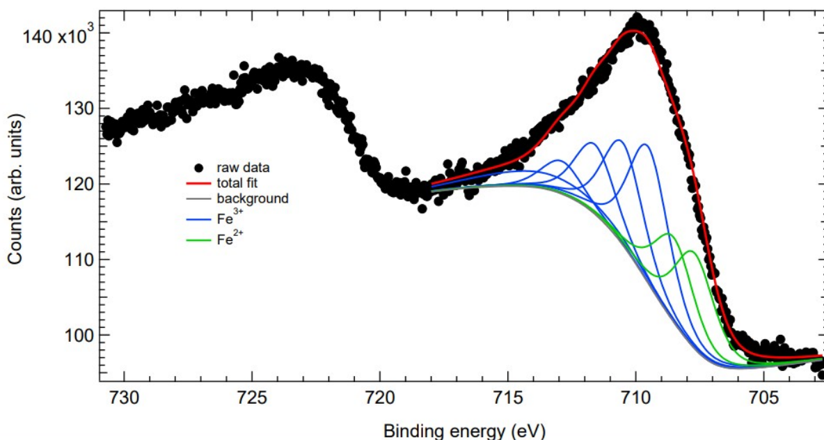
Figure 5. 3: XPS spectra of the Fe 2p core level.
