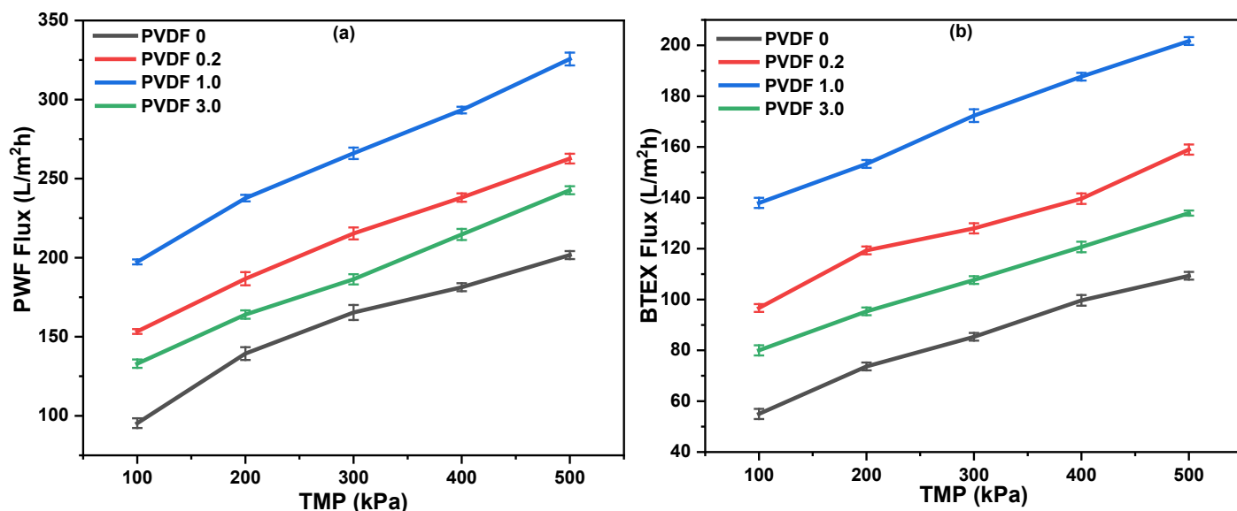
Figure 5. 12: (a) Pure water flux and (b) BTEX flux of the tested membranes.
