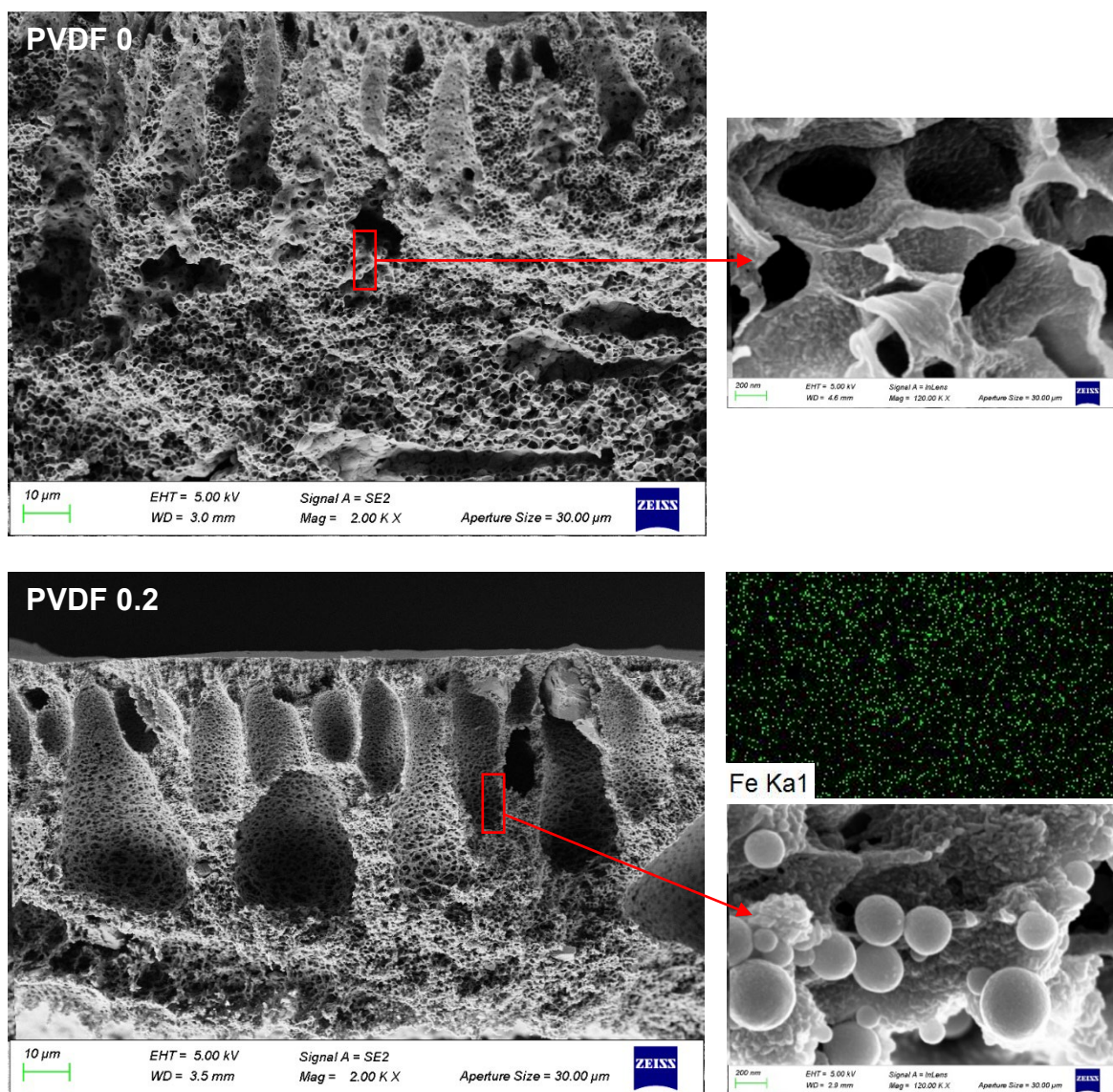
Figure 5. 7a: Cross-section SEM images of fabricated membranes with their respective EDX mapping images
