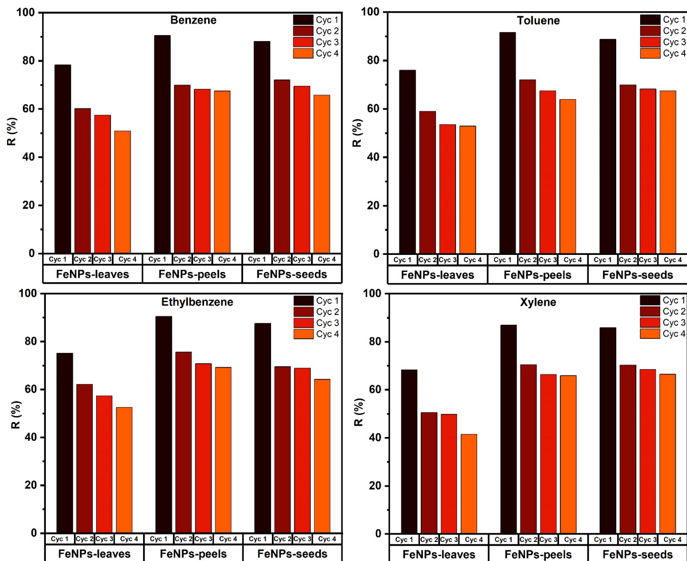
Figure 4. 14: Regeneration of the various FeNPs in BTEX adsorption.
