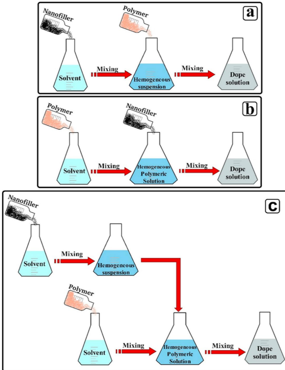
Figure 2. 6: Methods of incorporating inorganic nanoparticles into a membrane (Esfahani et al., 2019)
