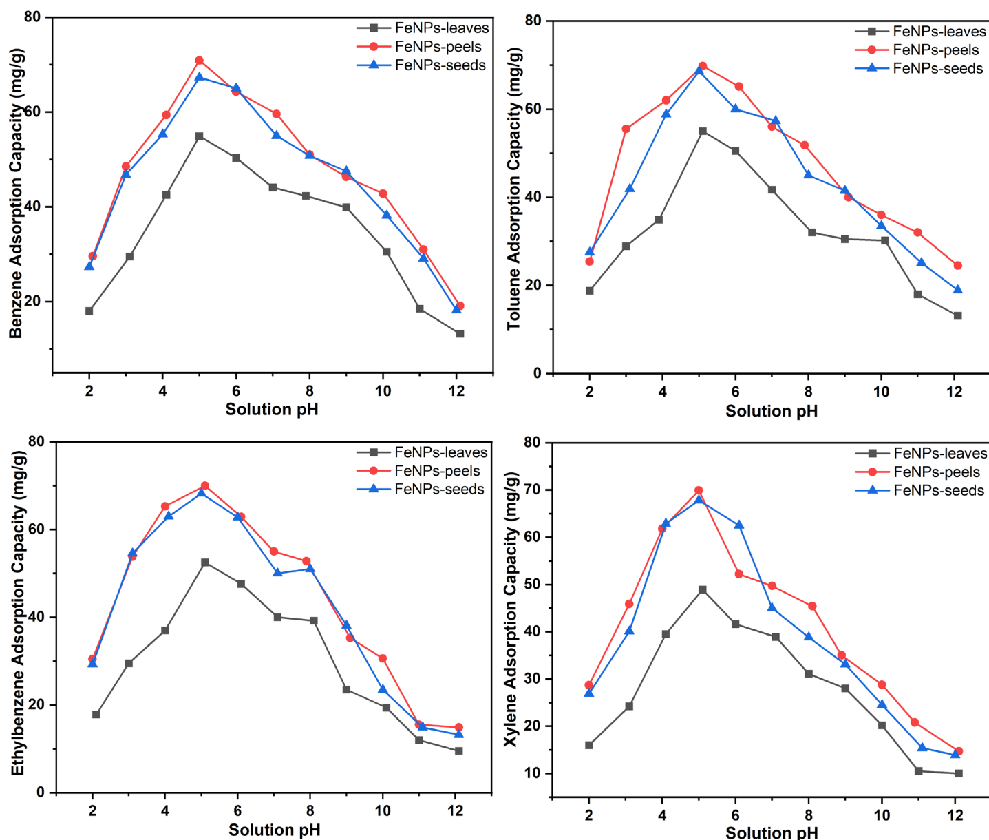
Figure 4. 8: Effect of solution pH on BTEX adsorption onto the FeNPs.
