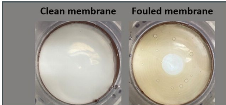
Figure 2. 11: Images of cleaned and fouled membrane (Dardor et al., 2021). This Figure is openly licensed via https://creativecommons.org/licenses/by-nc-nd/4.0/
