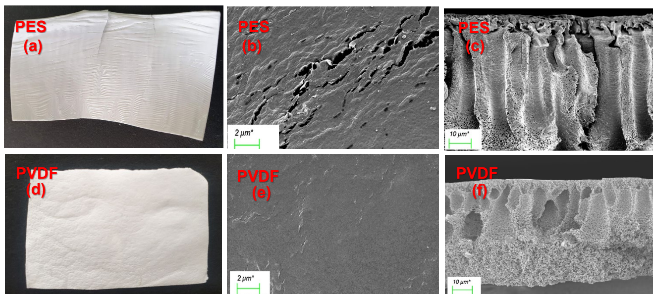
Figure 6. 1: The outcome of BTEX exposure of PES and PVDF membrane depicted by (a, d) photographs, (b, e) SEM image of membrane top surface, and (c, f) SEM image of membrane cross-section.
