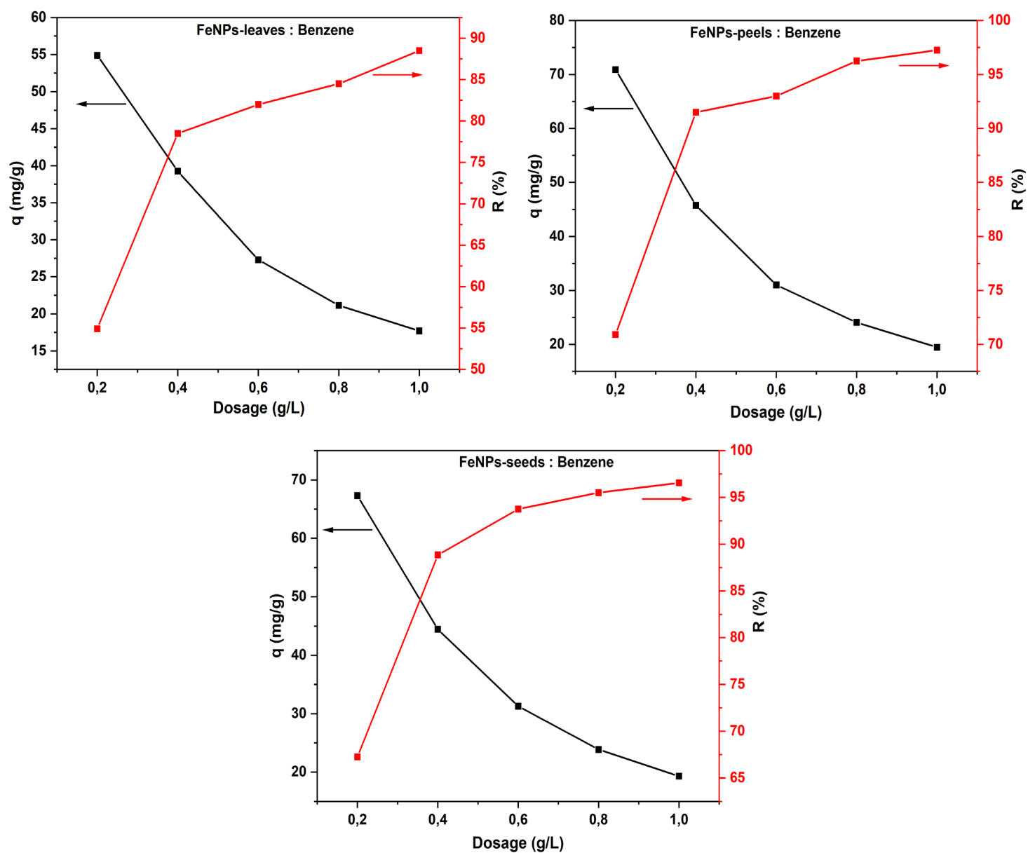
Figure 4. 9: Effect of FeNPs dosage on benzene adsorption.
