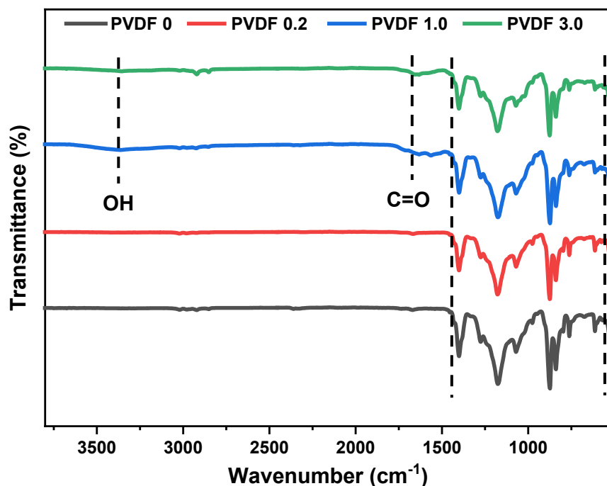
Figure 5. 6: FTIR spectra of the fabricated membranes
