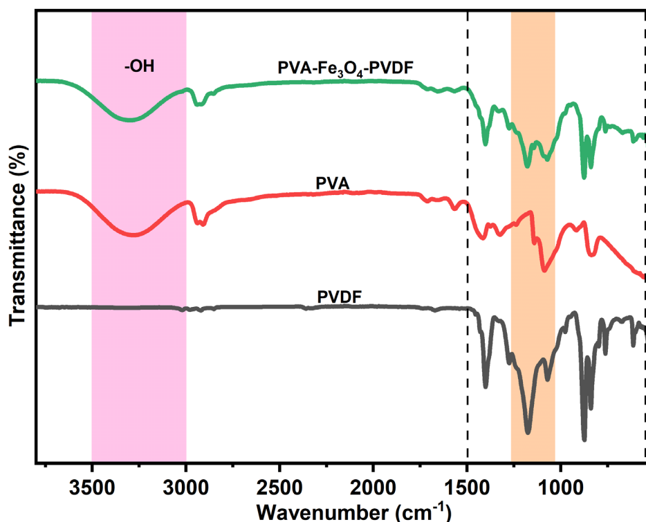
Figure 6. 2: FTIR spectra of PVDF, PVA, and PVA-Fe 3 O 4 -PVDF.
