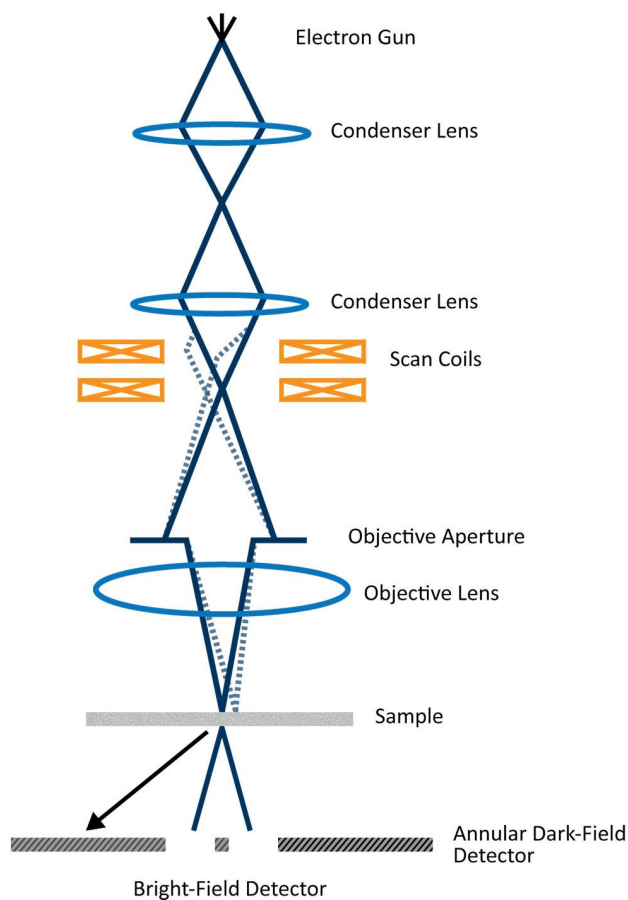
Figure 3. 4: Schematic depiction of the TEM principle (Nanoscience Instruments, 2020)
