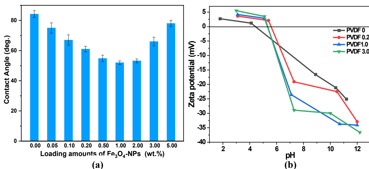
Figure 5. 10: (a) Contact angle values as a function of the \text{Fe}_3\text{O}_4 -NPs loadings and (b) zeta potential of the tested membranes
