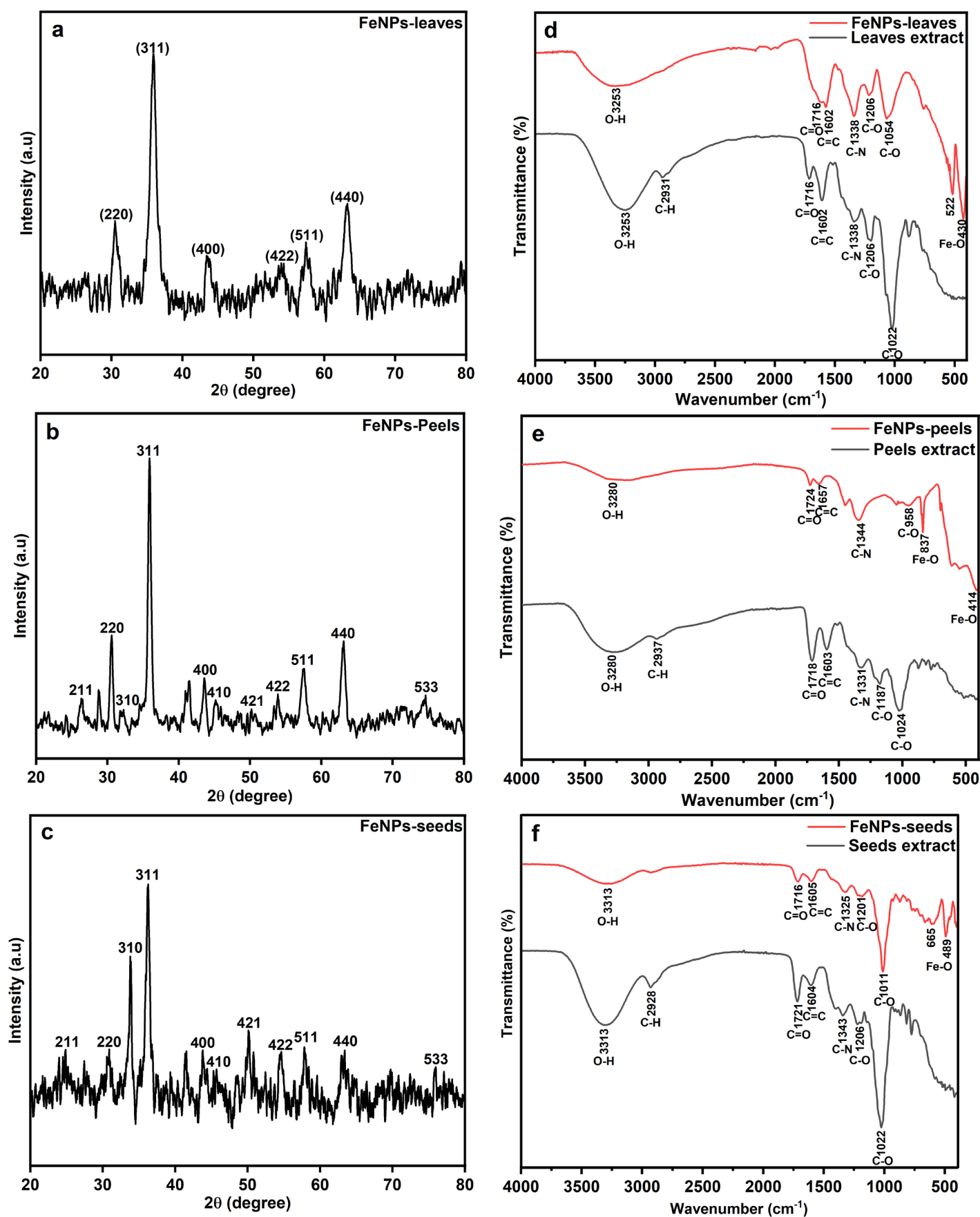
Figure 4. 4: (a,b,c) XRD patterns of the FeNPs, and (d,e,f) FTIR spectra of the FeNPs and the pomegranate extracts.
