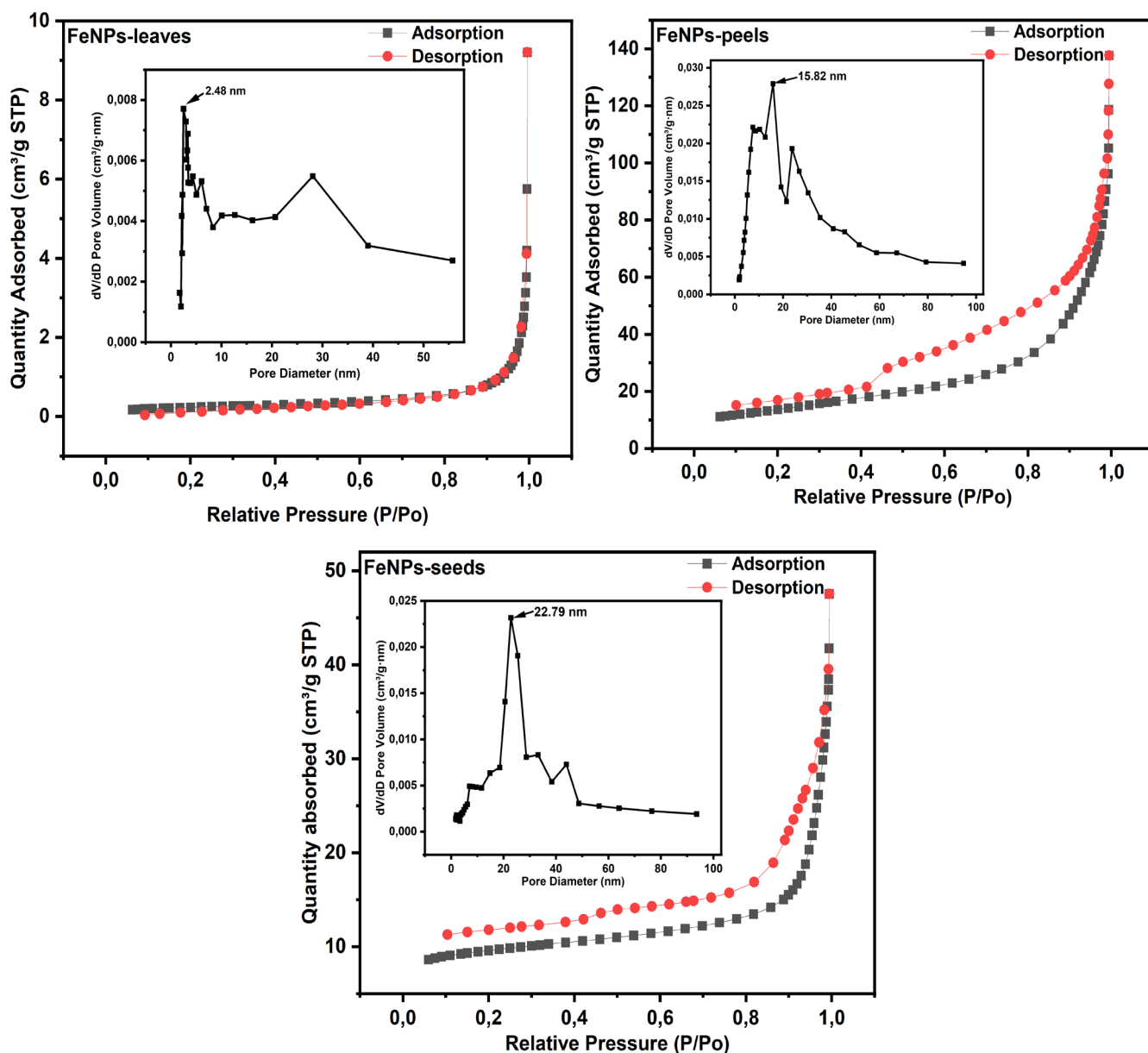
Figure 4. 6: The N 2 adsorption-desorption isotherms and pore size distributions (inset) of the FeNPs.
