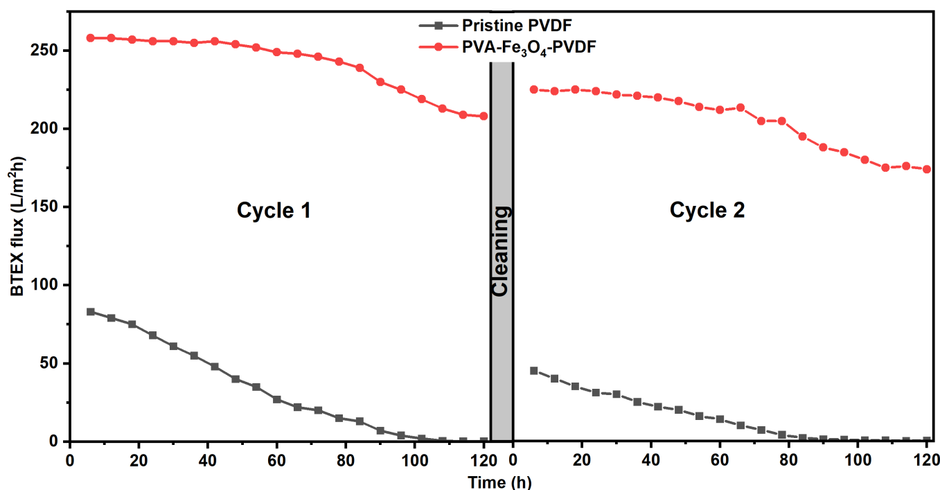
Figure 6. 10: Reusability of the membrane.
