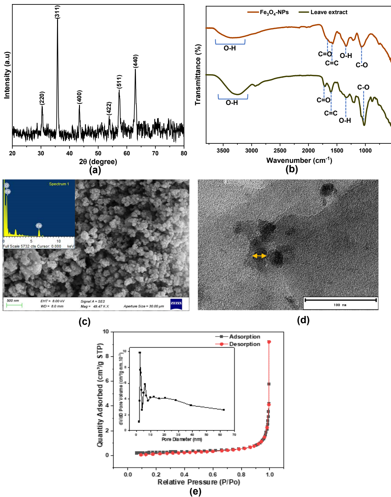
Figure 5. 2: (a) XRD pattern, (b) FTIR spectra, (c) SEM image, (d) TEM image, and (e) N 2 adsorption-desorption isotherm and pore size distribution (inset) of the Fe 3 O 4 -NPs.
