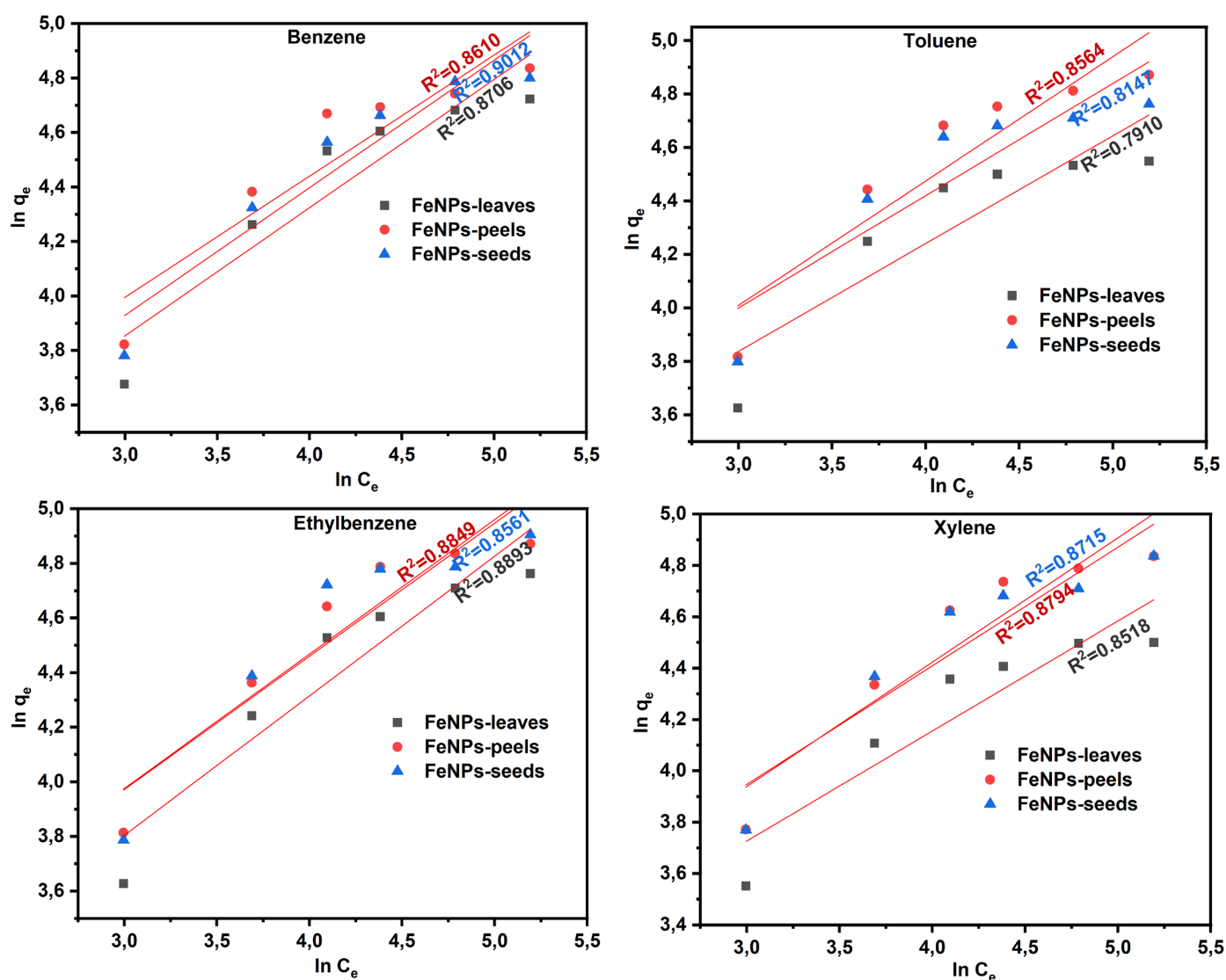
Figure 4. 12: The linear fit of Freundlich isotherm model for BTEX adsorption on FeNPs.
