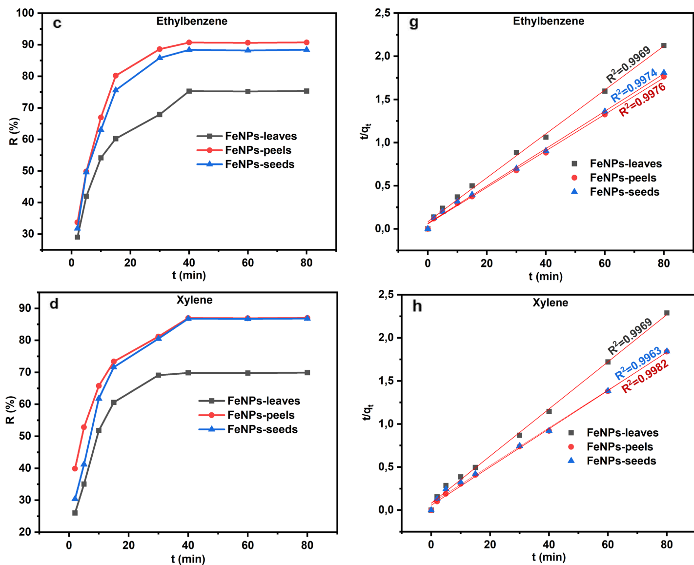
Figure 4. 10: (e, f, g, h) their respective linear fit for pseudo-second-order kinetic model.
