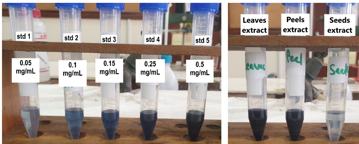
Figure 4. 2: The prepared standards and pomegranate extracts for total phenolic content measurements.
