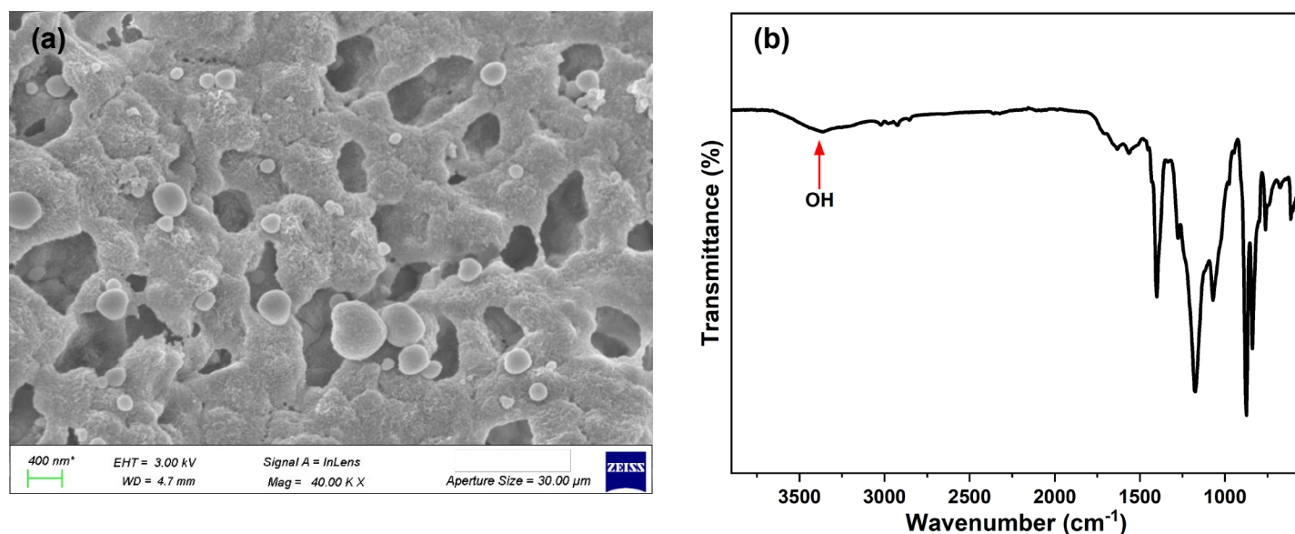
Figure 6. 11: (a) SEM image, and (b) FTIR spectrum of the PVA- \text{Fe}_3\text{O}_4 -PVDF membrane after long-term filtration test.
