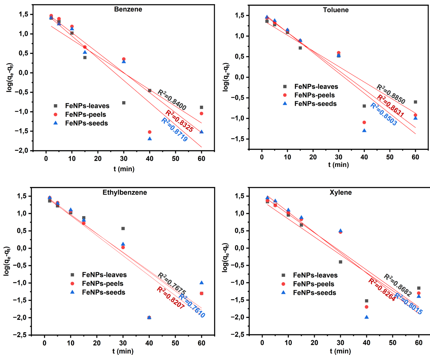
Figure 4. 101: Linear fit for the pseudo-first-order kinetic model for BTEX adsorption on FeNPs
