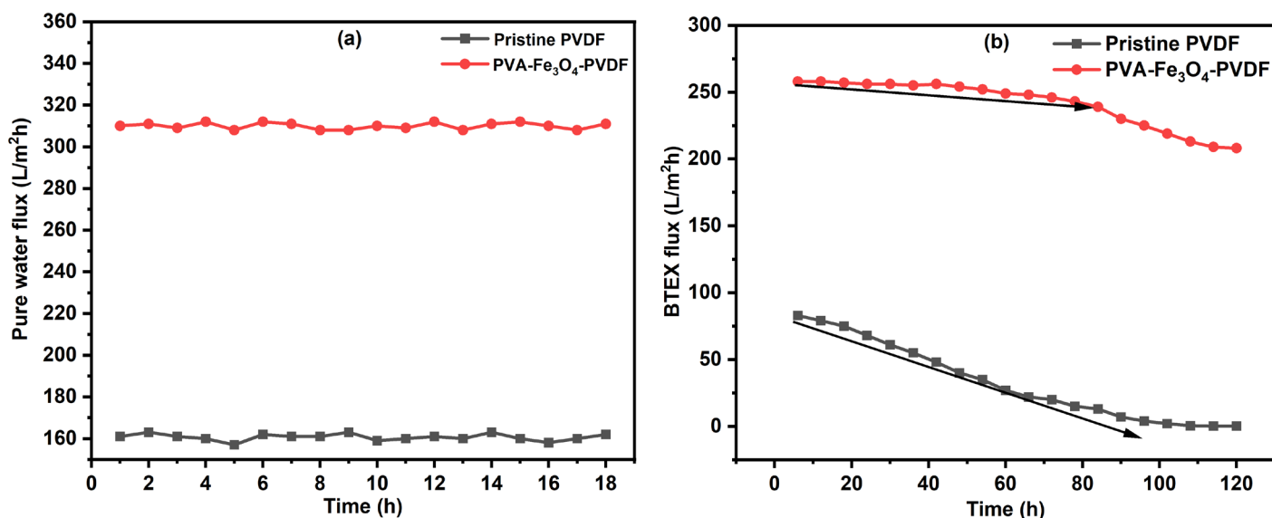
Figure 6. 8: Variation of (a) pure water flux, and (b) BTEX flux during the long-term filtration tests.
