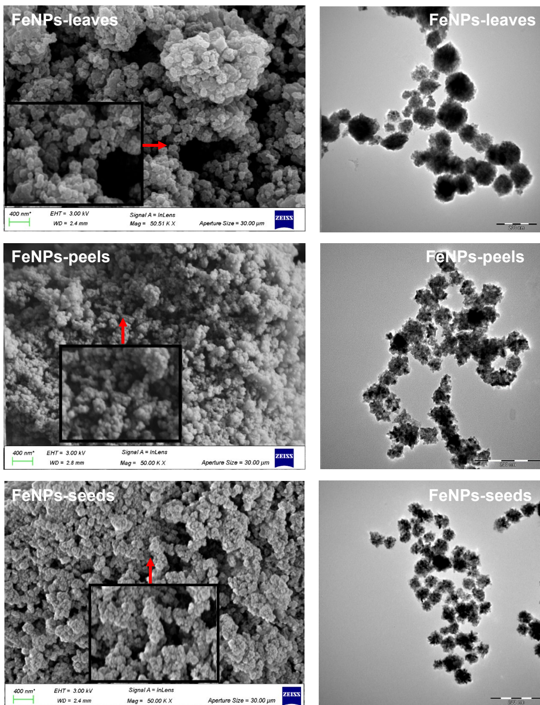
Figure 4. 5: SEM and TEM image of the FeNPs.
