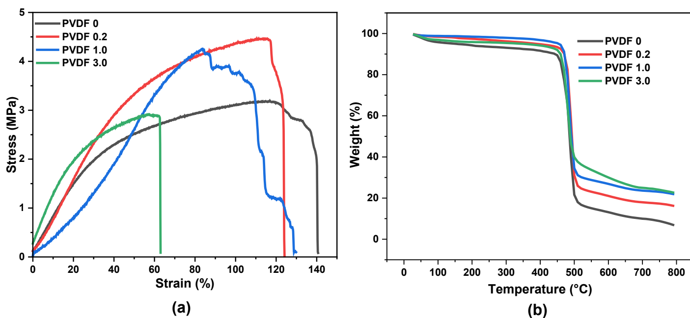
Figure 5. 11: (a) Stress-strain curves, and (b) TGA curves of the tested membranes.
