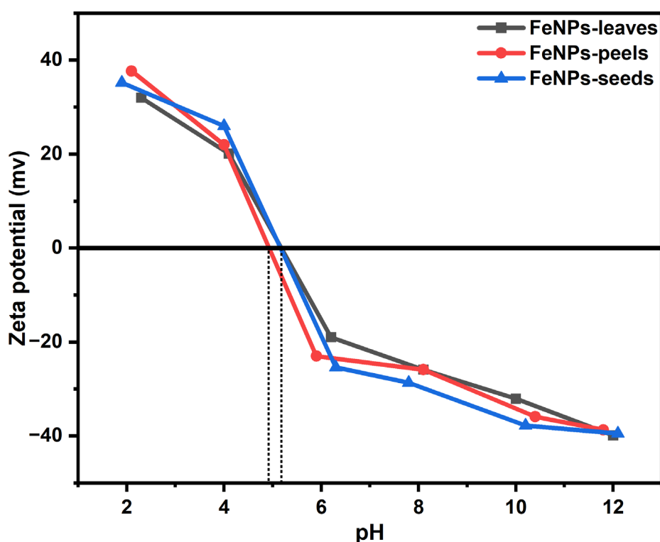
Figure 4. 7: Zeta potential of the FeNPs.
