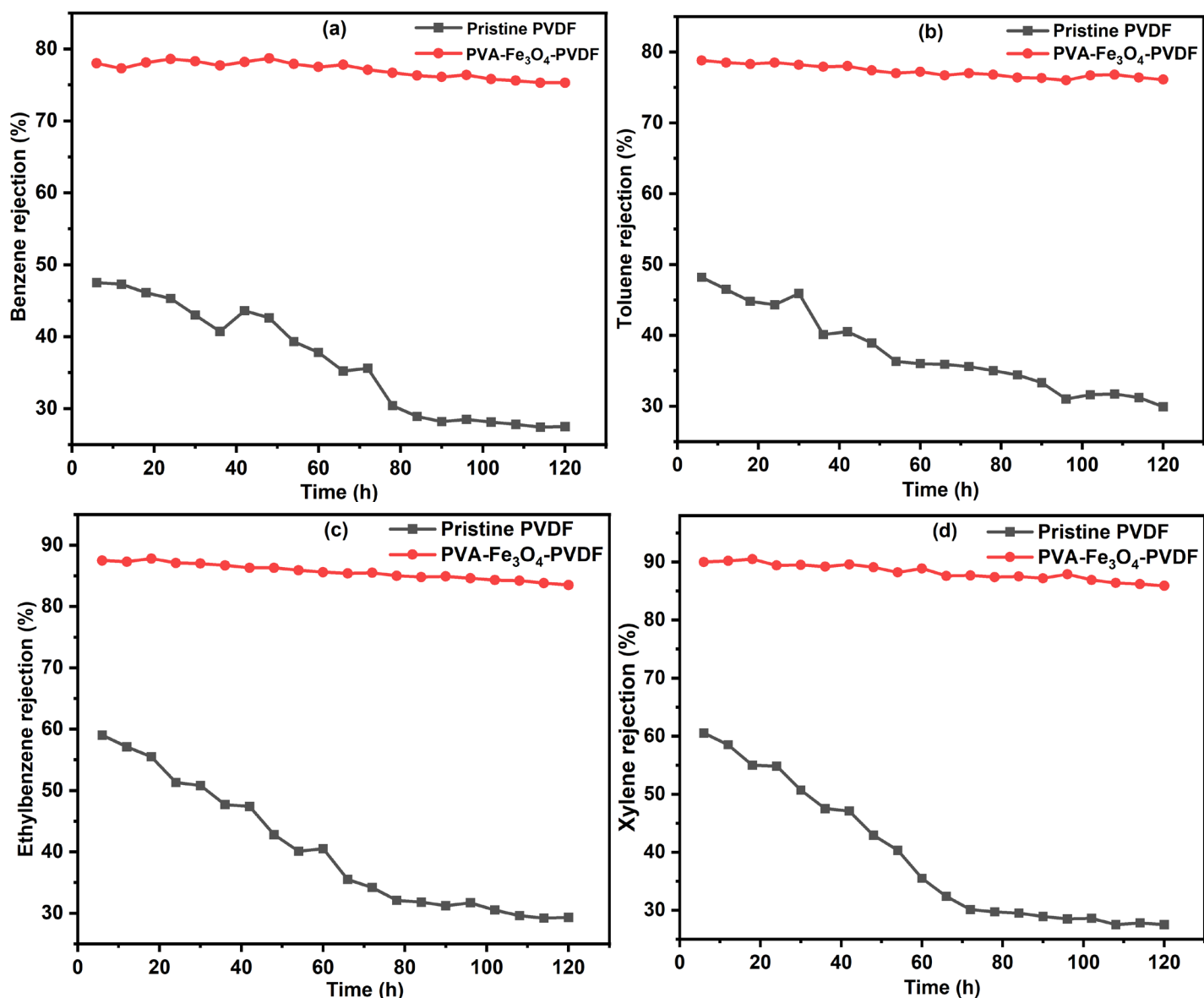
Figure 6. 9: Variation of the rejection of (a) benzene, (b) toluene, (c) ethylbenzene, and (d) xylene over long-term crossflow filtration.
