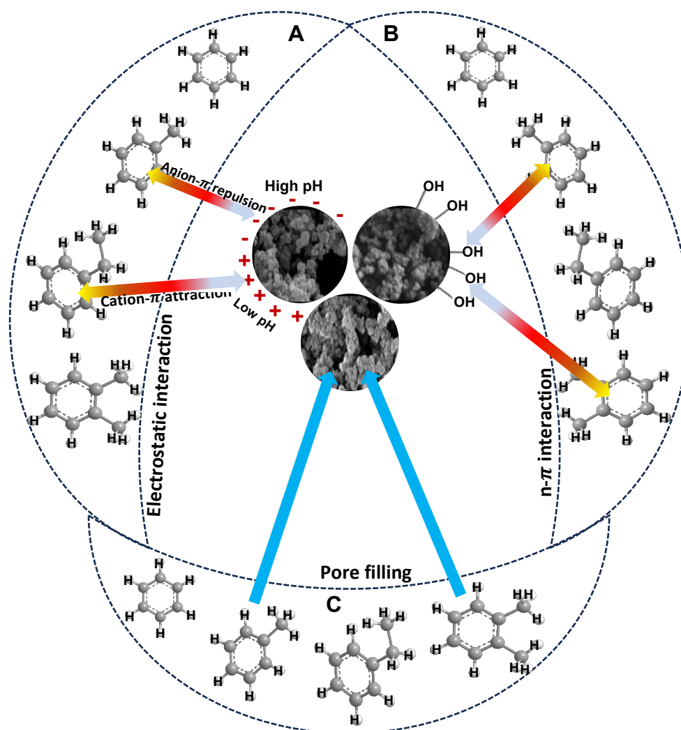
Figure 4. 13: Schematic diagram of the possible adsorption mechanism of BTEX on the FeNPs.
