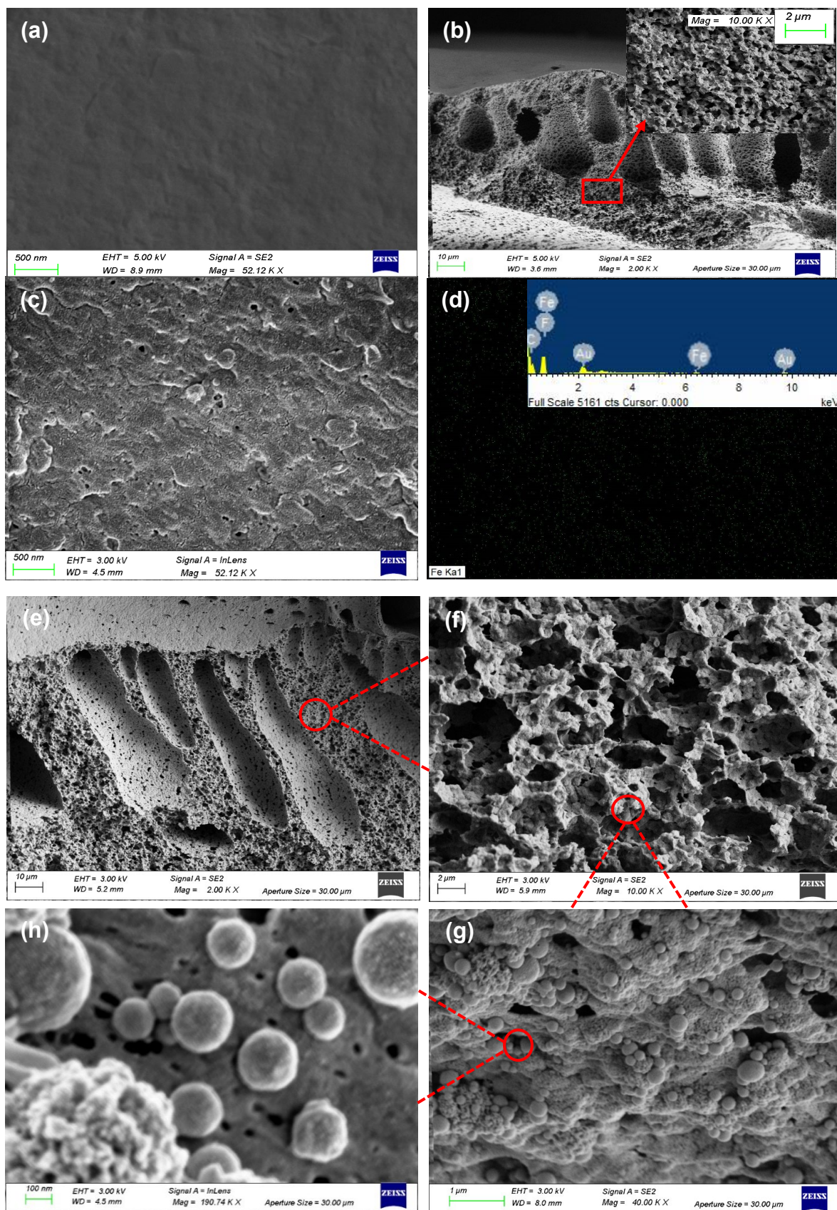
Figure 6.3: SEM image of the (a) surface of pristine PVDF, (b) inner structure of pristine PVDF, (c) surface of PVA-Fe 3 O 4 -PVDF, (d) EDX mapping image of PVA-Fe 3 O 4 -PVDF, and the inner structure of PVA-Fe 3 O 4 -PVDF at magnification (e) 2.00 KX, (f) 10.00KX, (g) 40.00KX, and (h) 190.74KX.
