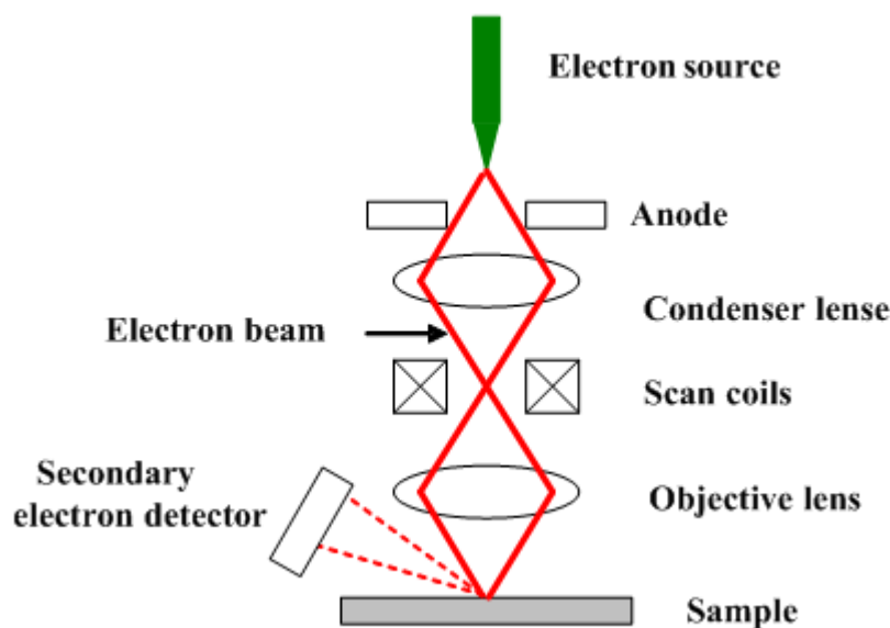
Figure 3. 3: Schematic depiction of the principle of SEM (SubsTech, 2015).
