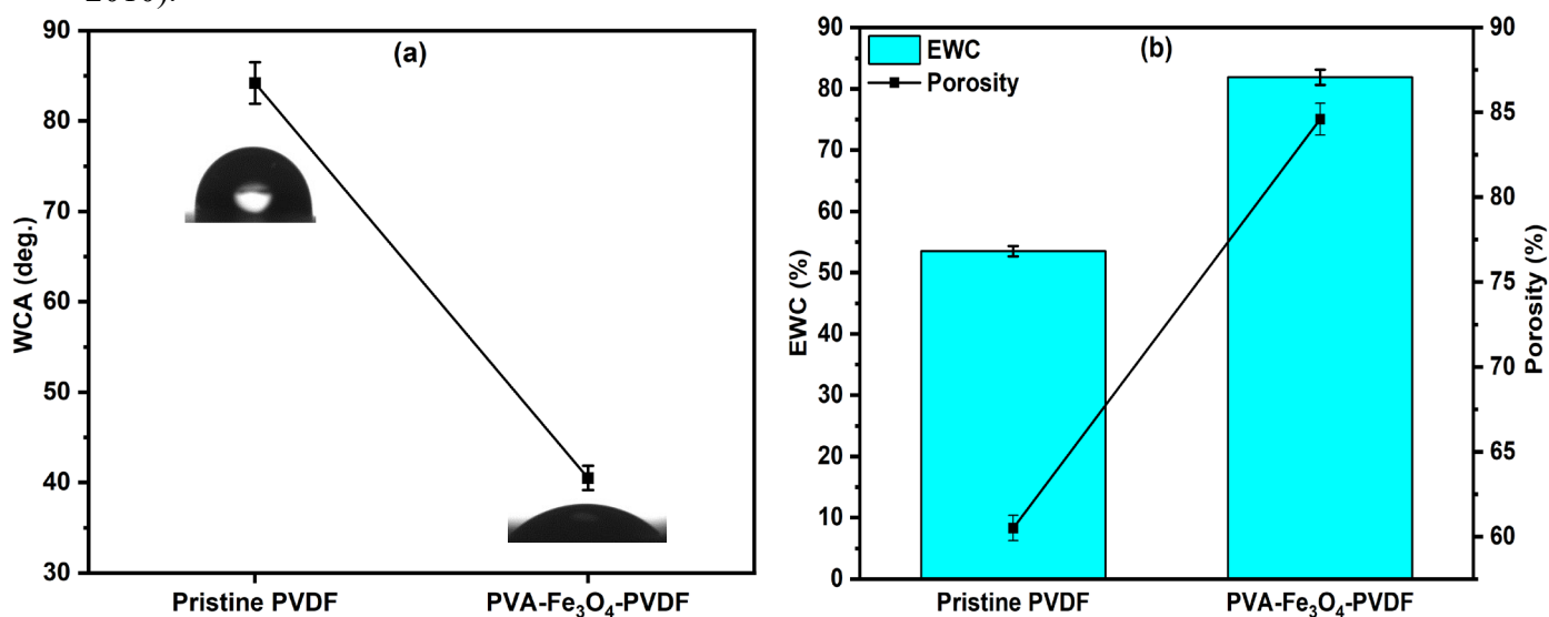
Figure 6. 5: (a) WCA, and (b) EWC and porosity of the pristine PVDF and PVA-Fe 3 O 4 -PVDF membrane.
