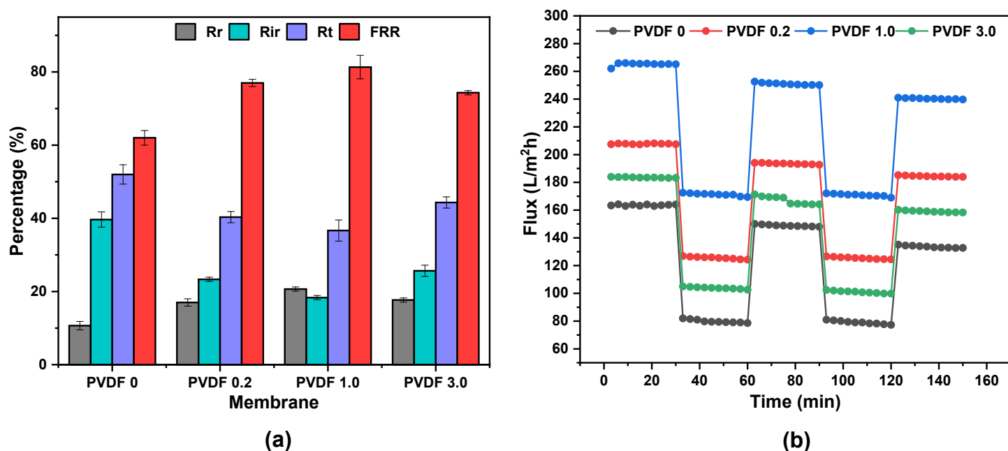
Figure 5. 15: (a) fouling resistance of the membranes, (b) Fluctuation of the flux of pure water and BTEX water over time.
