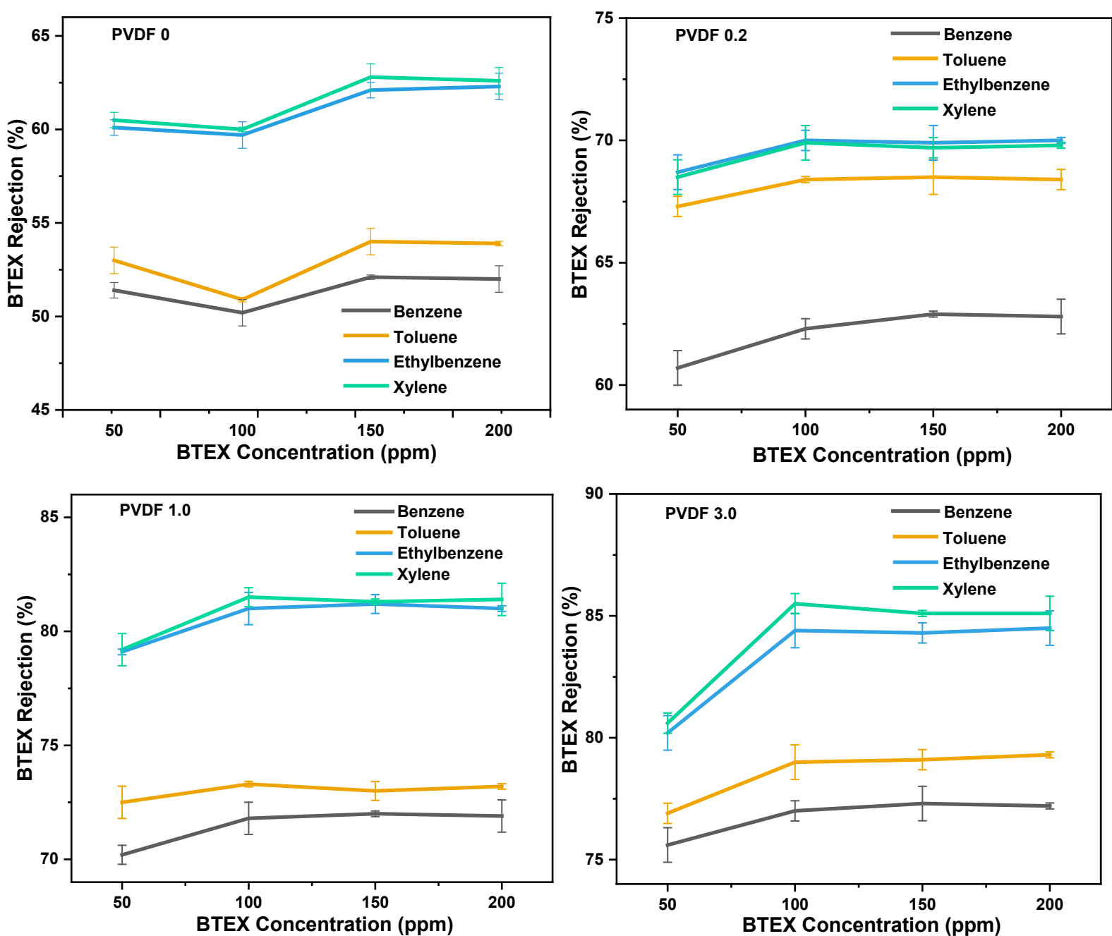
Figure 5. 14: Effect of BTEX concentrations on membranes' rejection capacity.
