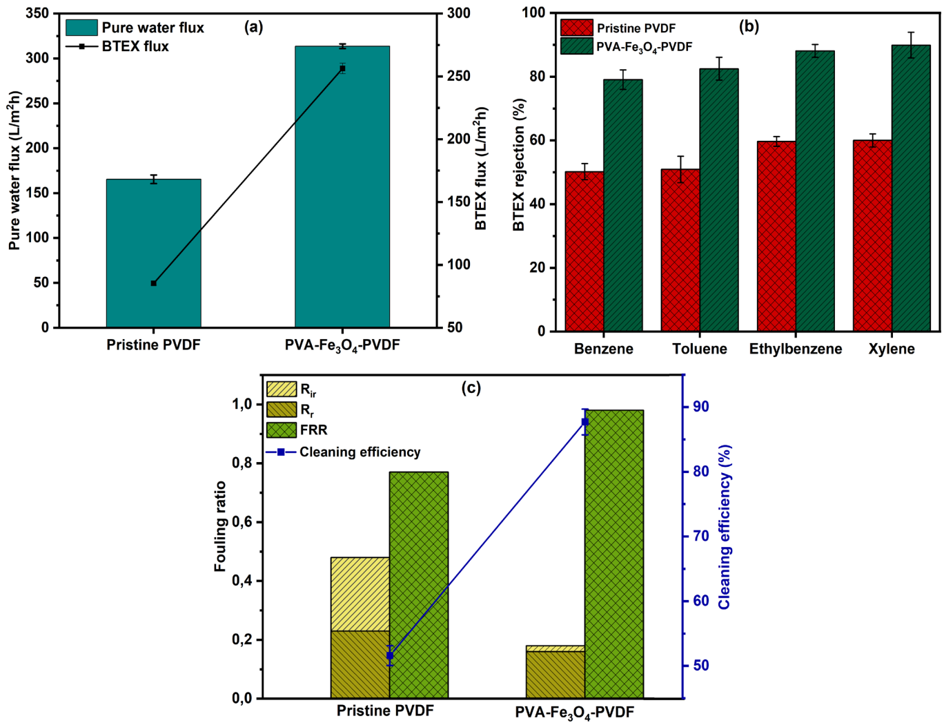
Figure 6. 7: (a) Permeate fluxes, (b) BTEX rejections, and (c) fouling ratios and cleaning efficiency of the membranes.
