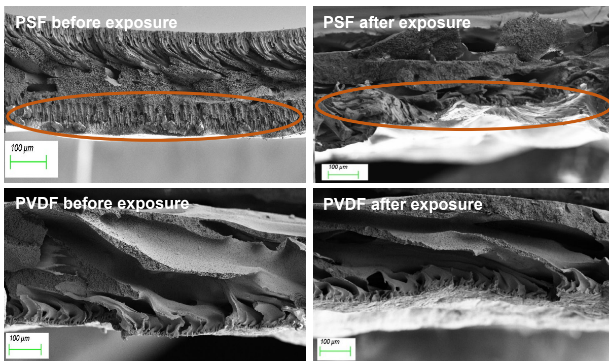
Figure 5. 5: SEM images of the before and after-exposure of PSF and PVDF membrane to BTEX solution.
