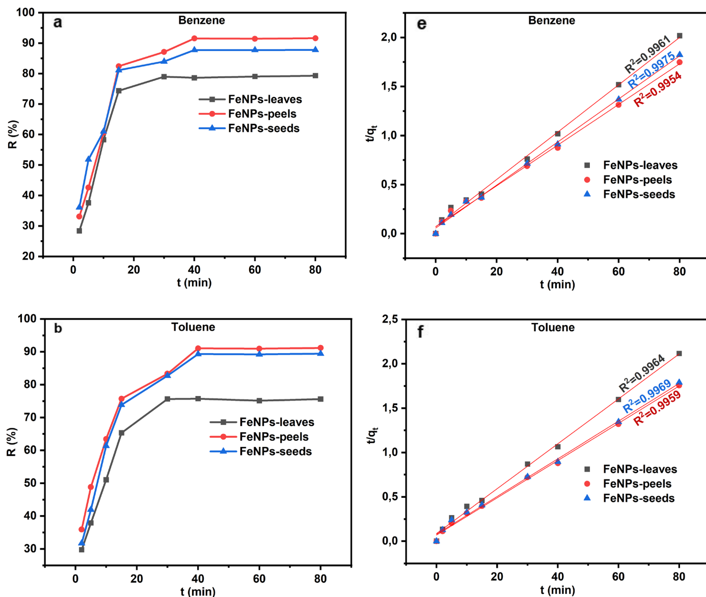
Figure 4. 10: (a, b, c, d) Effect of contact time on BTEX adsorption on the FeNPs
