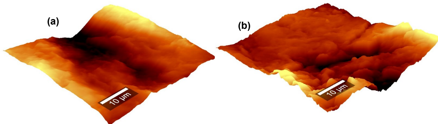
Figure 6. 4: AFM images of the (a) pristine PVDF membrane, and (b) PVA-Fe 3 O 4 -PVDF membrane.
