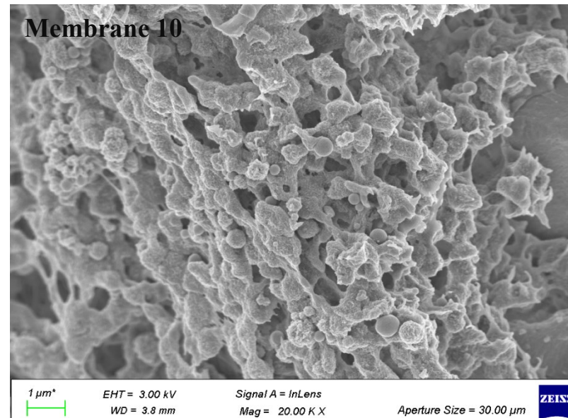
Figure 7. 1: The SEM image of the inner structure of the membranes shows the dispersion of the \text{Fe}_3\text{O}_4 -NPs in the membrane matrix.
