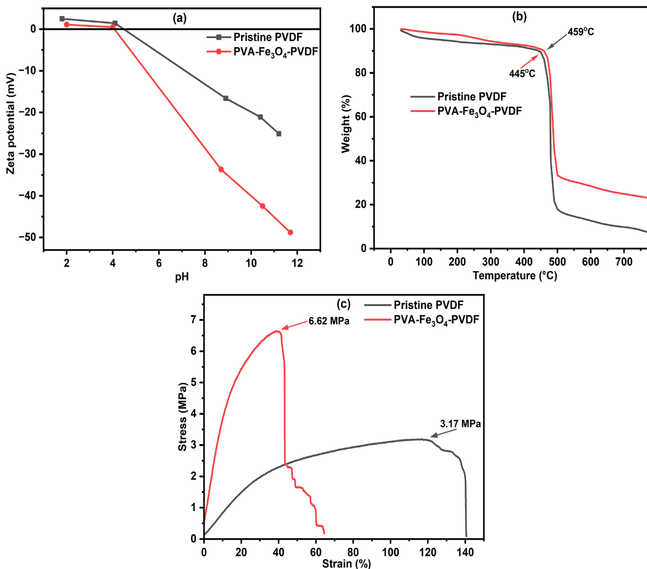
Figure 6. 6: (a) surface zeta potentials, (b) TGA curves, and (c) stress-strain curves of the pristine PVDF and PVA-Fe 3 O 4 -PVDF membrane.
