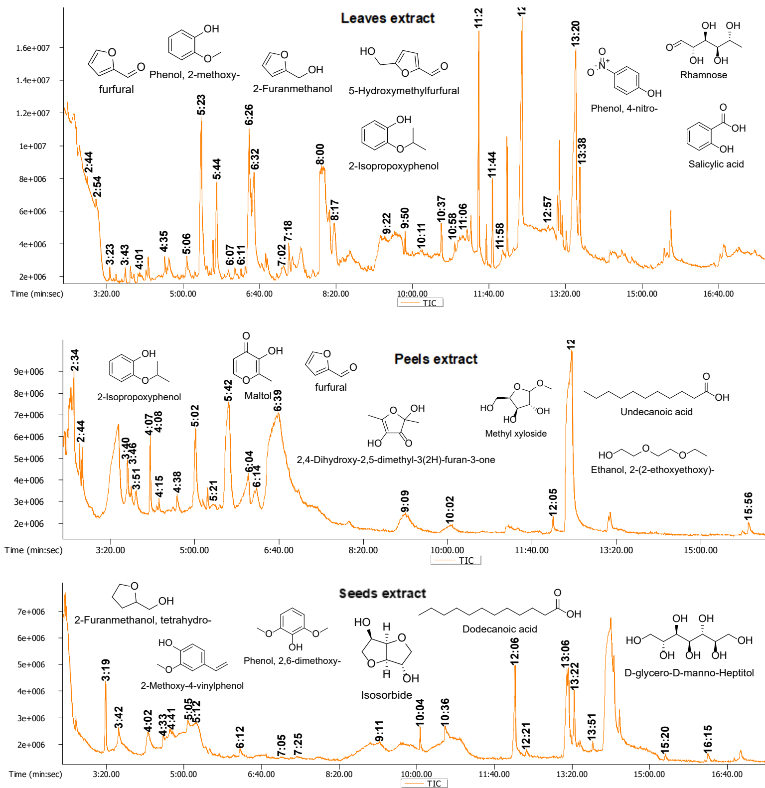
Figure 4. 3: GC-MS chromatograms of the pomegranate leaves, peels, and seeds extract.
