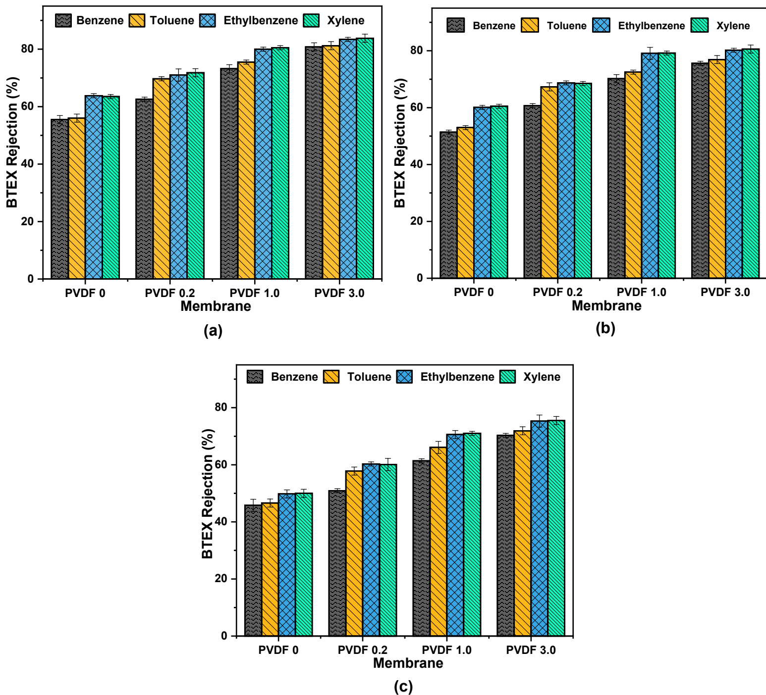
Figure 5. 13: Effect of TMP on the BTEX rejection of the membranes at (a) 100 kPa, (b) 300 kPa, and (c) 500 kPa.
