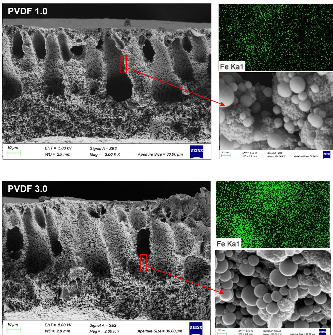
Figure 5. 8b: Cross-section SEM images of fabricated membranes with their respective EDX mapping images.
