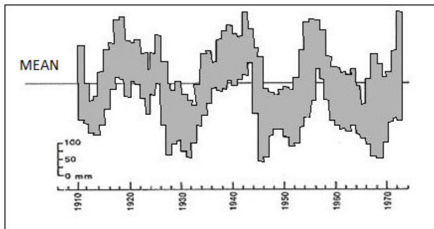
Figure 4.1: Showing superimposed deviations from mean annual rainfall smoothed with a 5-term binomial filter for some stations in the summer rainfall region. Based on Tyson (1987: 69).
