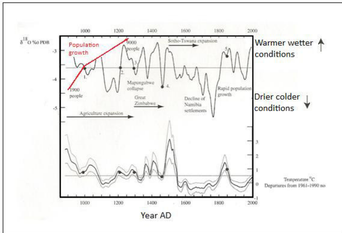
Figure 4.3: Climate time series are derived from analyses of stalagmites from Cold Air Cave together with historical information. The top series show \delta^{18}\text{O} variations reflecting relative changes in temperature and moisture and the bottom series shows temperature changes in ^{\circ}\text{C} anomalies from 1961-1990. Based on Holmgren and Öberg (2005: 188).
