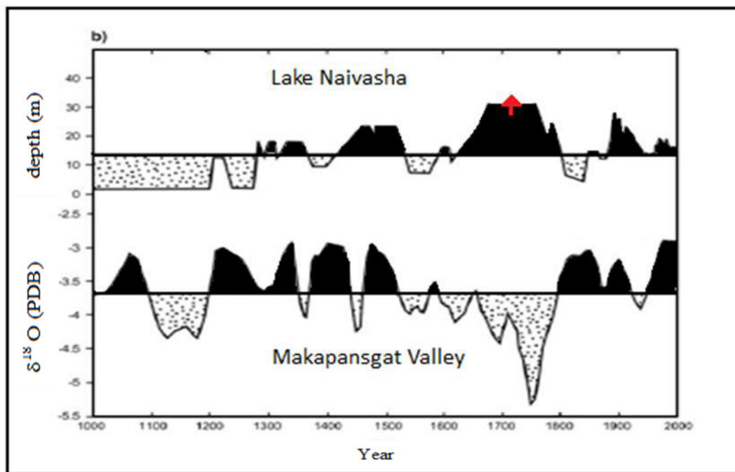
Figure 4.2: Correlation between lake levels in East Africa and speleothems in southern Africa, based on Tyson et al. 2002.
