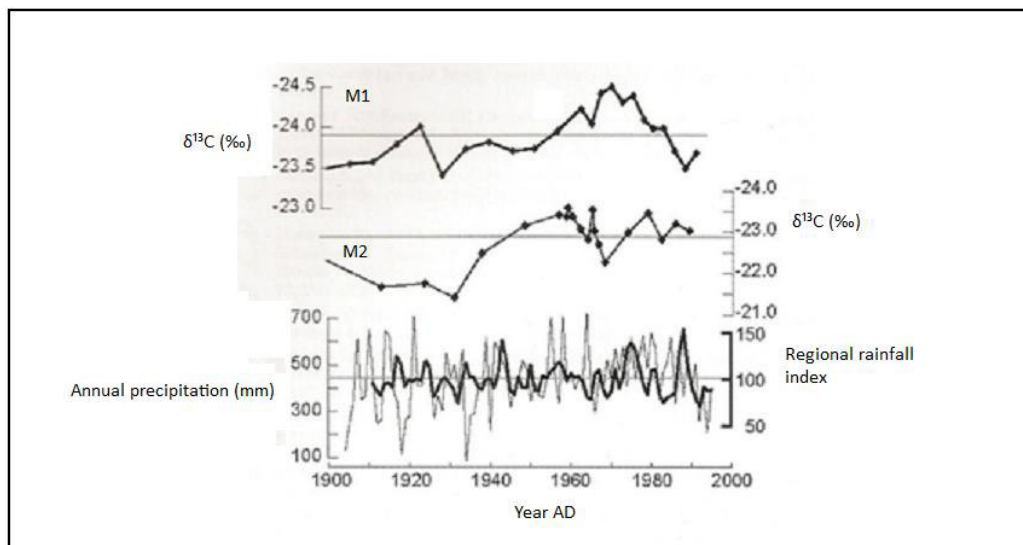
Figure 4.4: Properties of M1 and M2 plotted together with rainfall variations at Polokwane weather station and a regional rainfall index. Based on Norström et al. 2005: 167.
