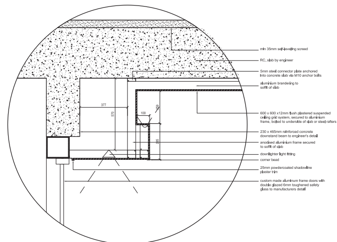
Detail 2: Concrete downstand beam
