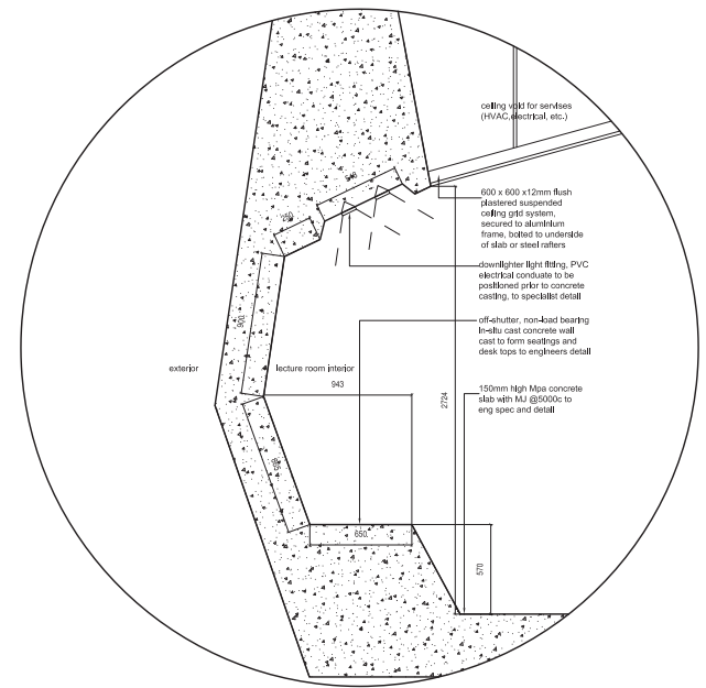
Detail 3: Moulded seating
