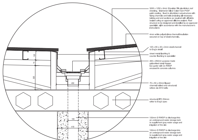
Detail 1: Hopper box gutter
