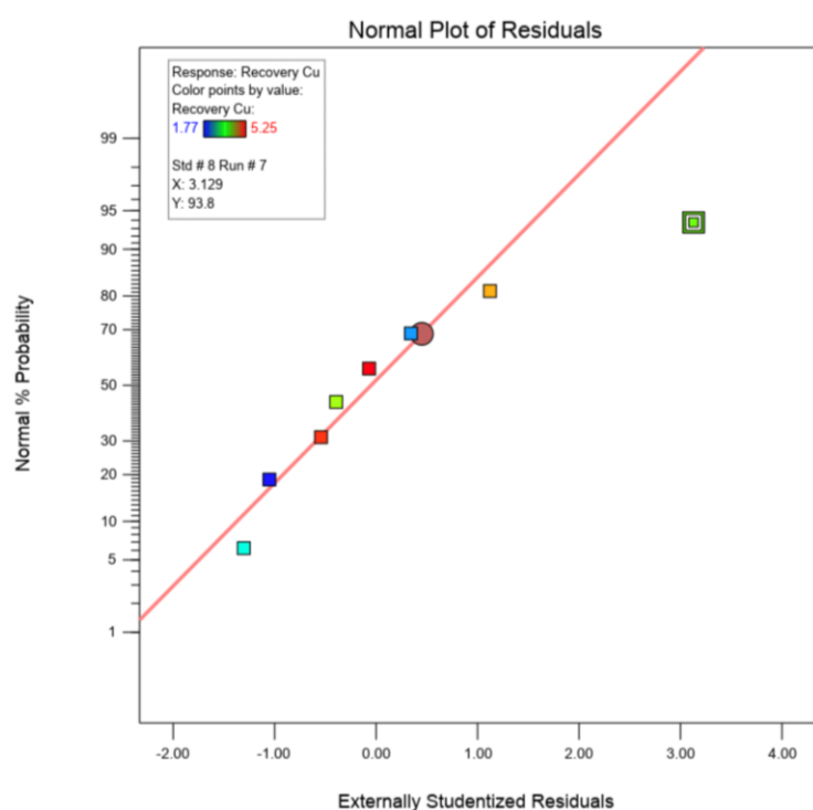
Figure 5-4 Normal plot of residuals for Cu recovery
