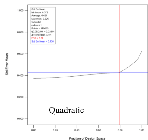
Figure 6-8 FDS plot for quadratic model
