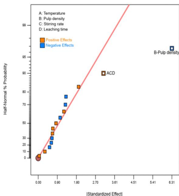
Figure 5-5 Half normal plot for Ni recovery
