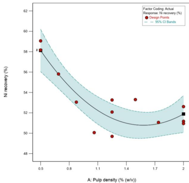
Figure 6-4 Response surface plot for Ni recovery
