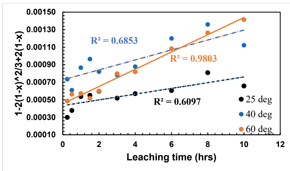
Figure 7-5 Plot of 1 - 3(1 - x)^{2/3} + 2(1 - x) vs time for Cu Dissolution at 25°C to 60 °C
