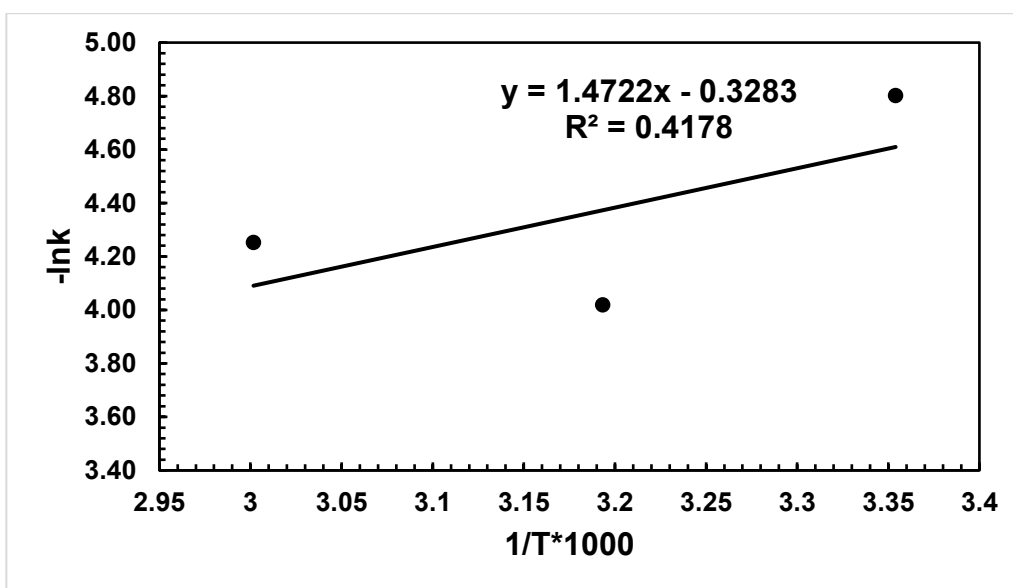
Figure 7-12 Arrhenius plot showing the linear relationship between \ln k and 1/T for Ni extraction in the DES, ethaline (1ChCl:2EG).
