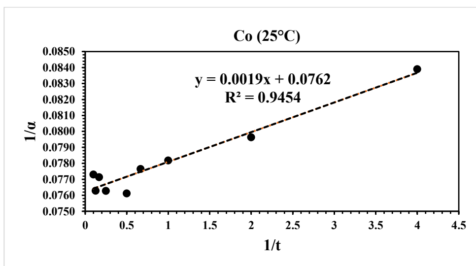
Figure 7-8 Plot of \frac{1}{\alpha} vs \frac{1}{t} for the proposed SPM-PSO Co kinetic model at 25°C
