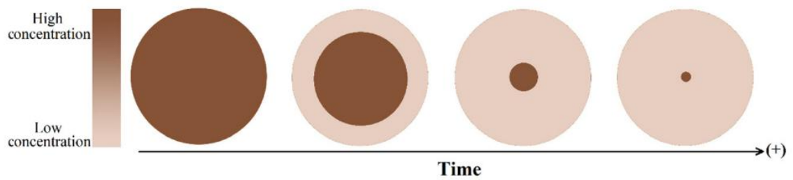
Figure 2-4 Leaching of particles based on the Shrinking-Core-Model – Constant Size (Faraji et al. , 2022)
