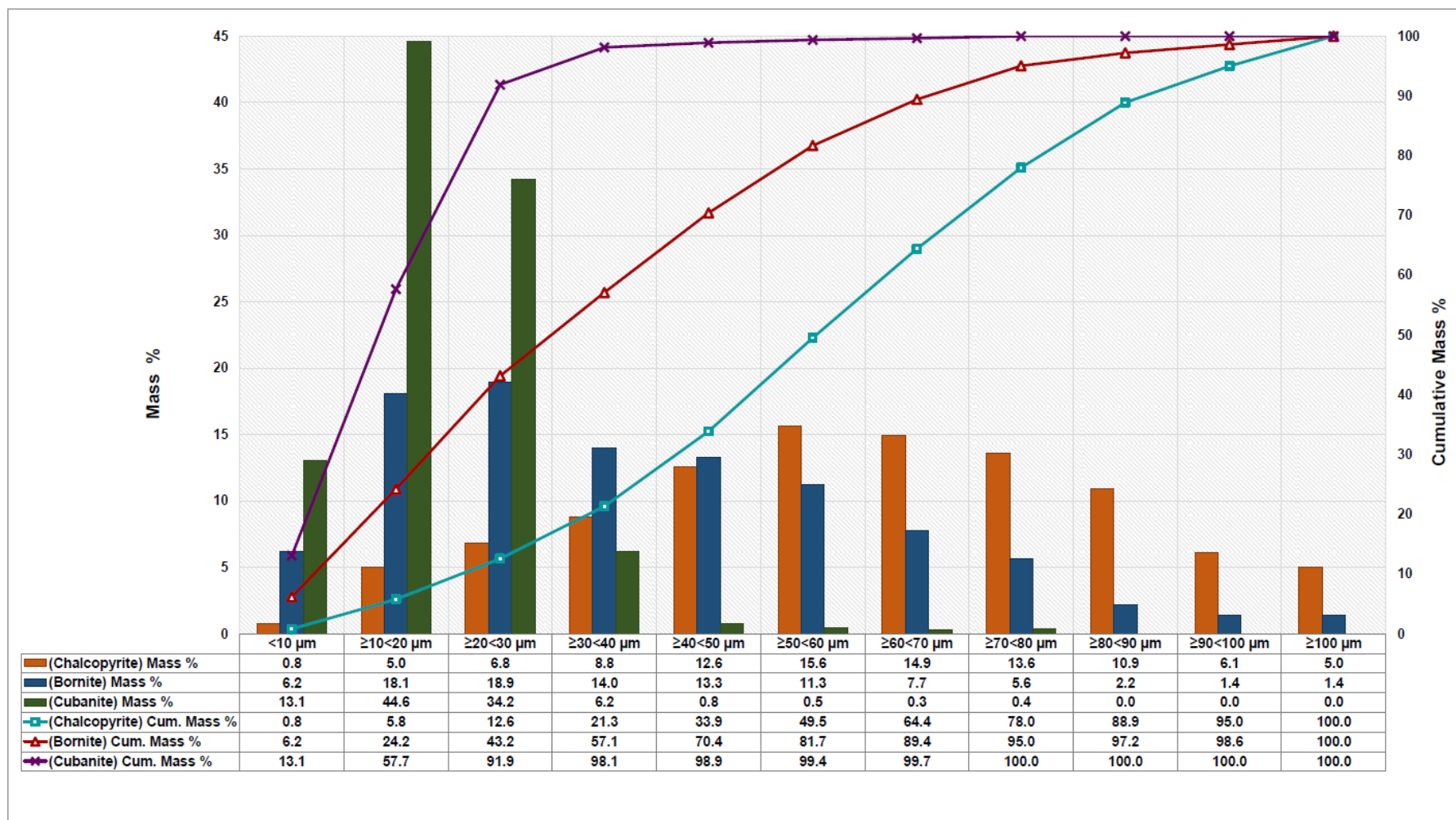
Figure A3 GSD data for the Cu-bearing samples
