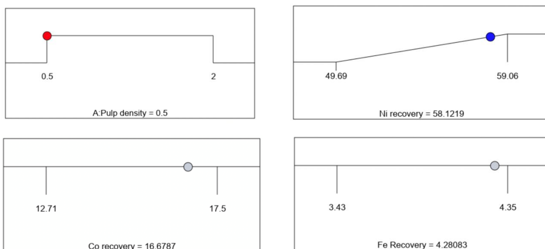
Figure 6-11 Solution to Ni recovery maximization via numerical optimization
