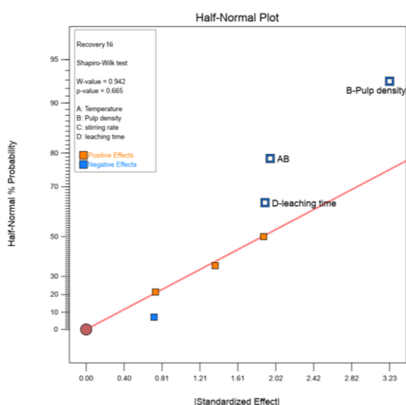
Figure 5-1 Half Normal plot of estimated factor effects of Ni recovery using ethaline
