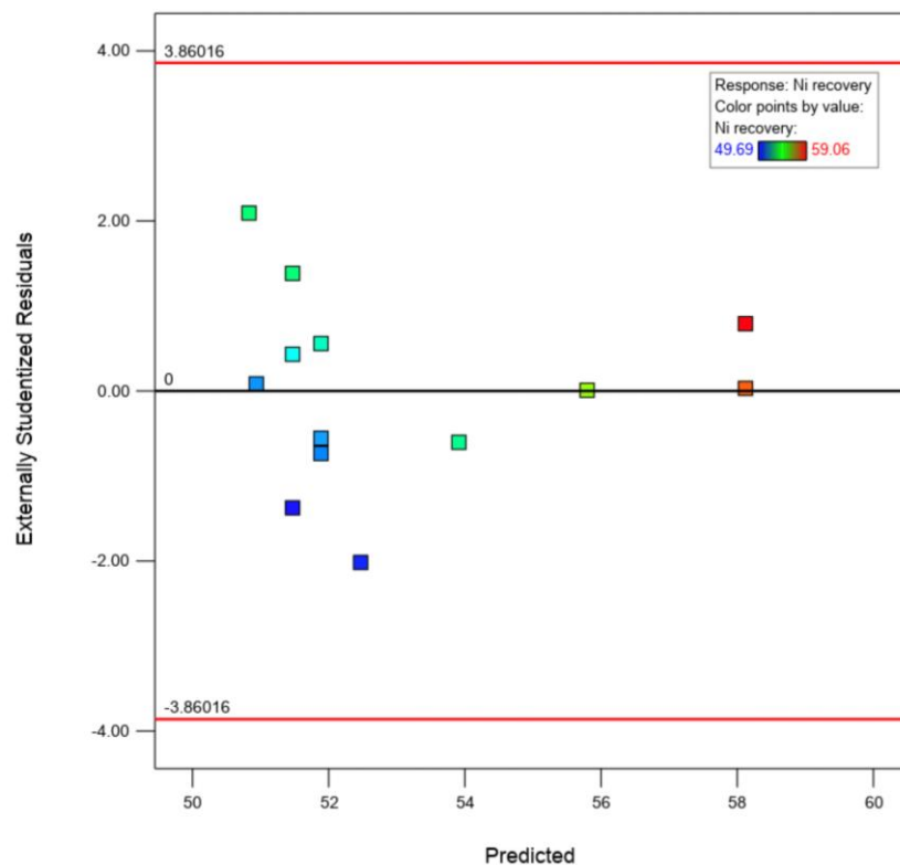
Figure 6-3 Residuals vs Predicted response
