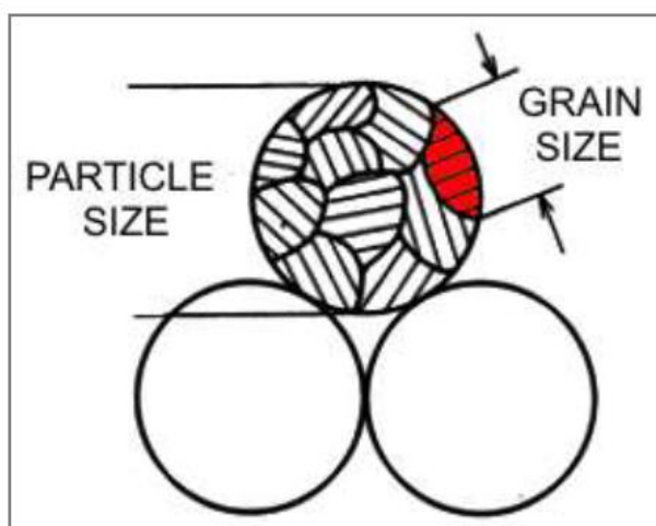
Figure 4-1 Explanation of grain versus particle (BITRI, 2023)
