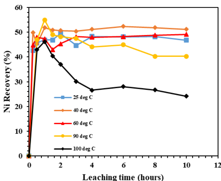
Figure 7-1 Nickel (pentlandite) dissolution from a Cu-Ni sulphide ore concentrate in terms of recovery at different temperatures
