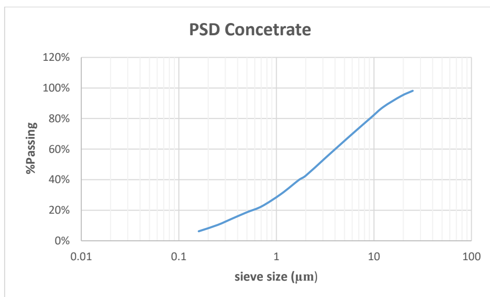
Figure A1. Sieve analysis plot of the head sample.
