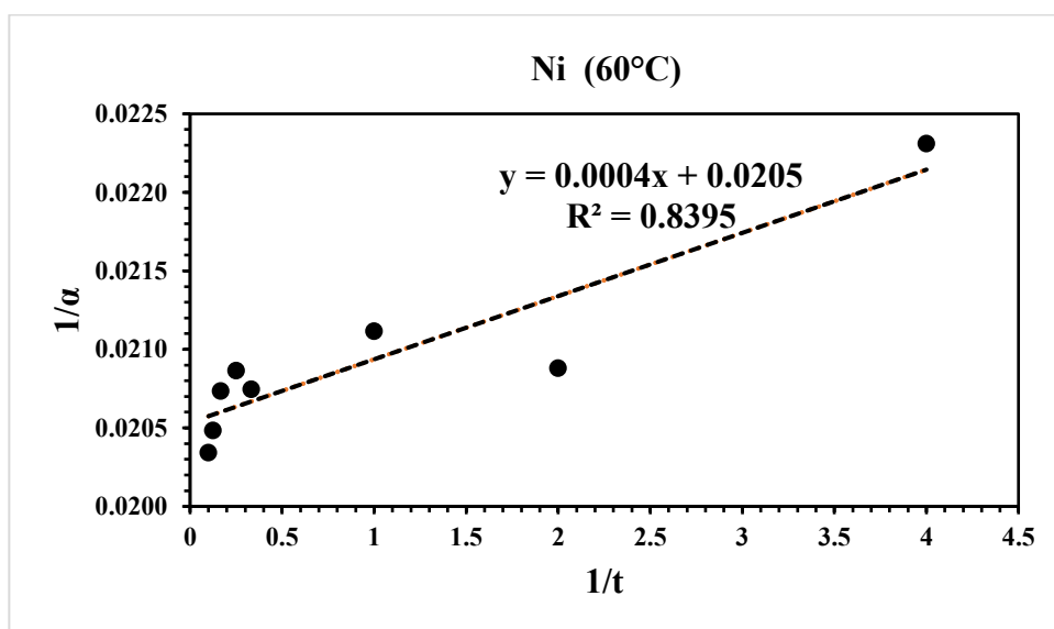
Figure 7-11 Plot of \frac{1}{\alpha} vs \frac{1}{t} for the proposed SPM-PSO Ni kinetic model at 60°C
