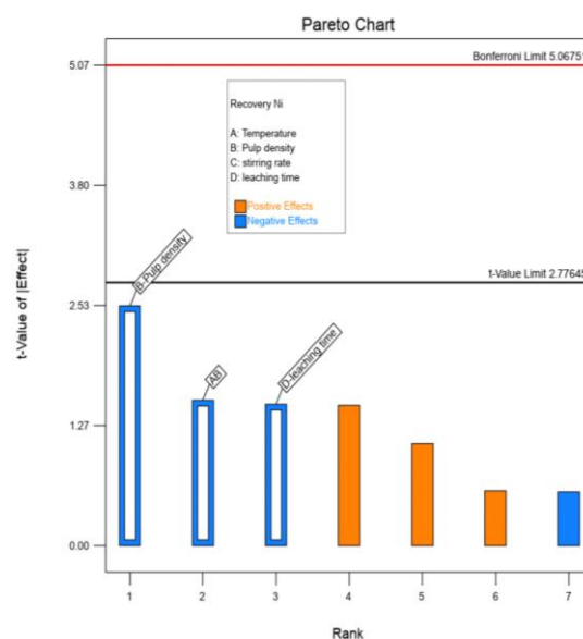
Figure 5-2 Pareto chart for ranking of main and interactive effects (Ni recovery)
