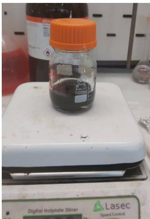
Figure 3-1 Leaching test setup
