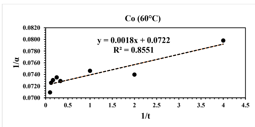
Figure 7-9 Plot of \frac{1}{\alpha} vs \frac{1}{t} for the proposed SPM-PSO Co kinetic model at 60°C
