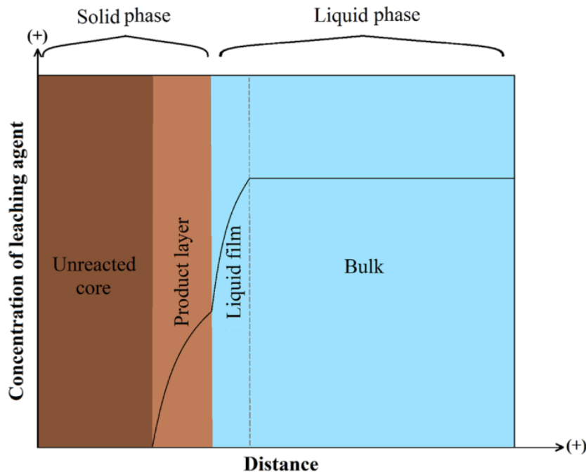
Figure 2-3 Graphic representation of leaching steps
