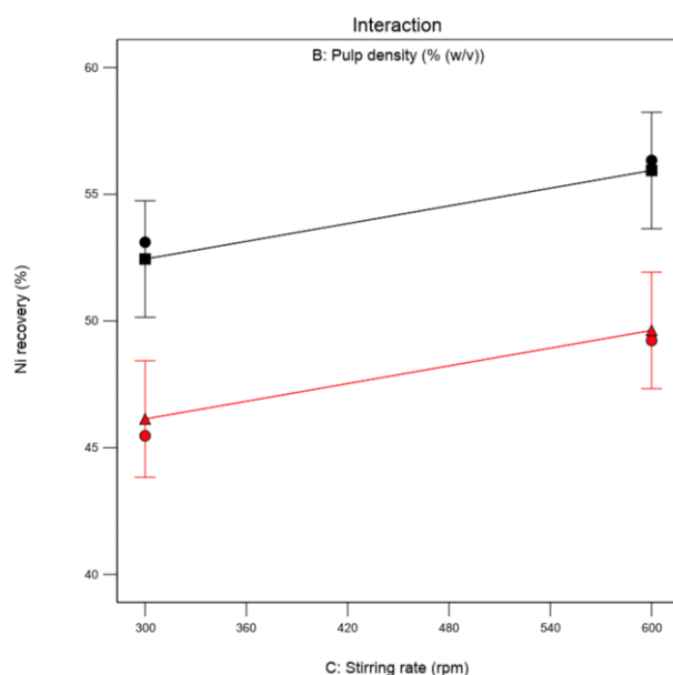
Figure 5-9 Two-way interaction plot for Ni recovery vs stirring rate and pulp density: red graph (B=10% w/v) and black graph (B=2% w/v)
