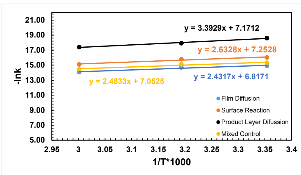
Figure 7-13 Arrhenius plot showing the linear relationship between \ln k and 1/T for Cu extraction in the DES, ethaline (1ChCl:2EG).
