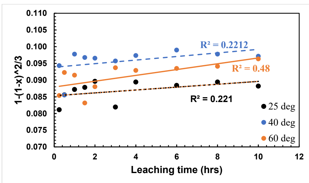
Figure 7-4 Plots of 1 - (1 - x)^{2/3} vs time for Co Dissolution at 25°C to 60 °C
