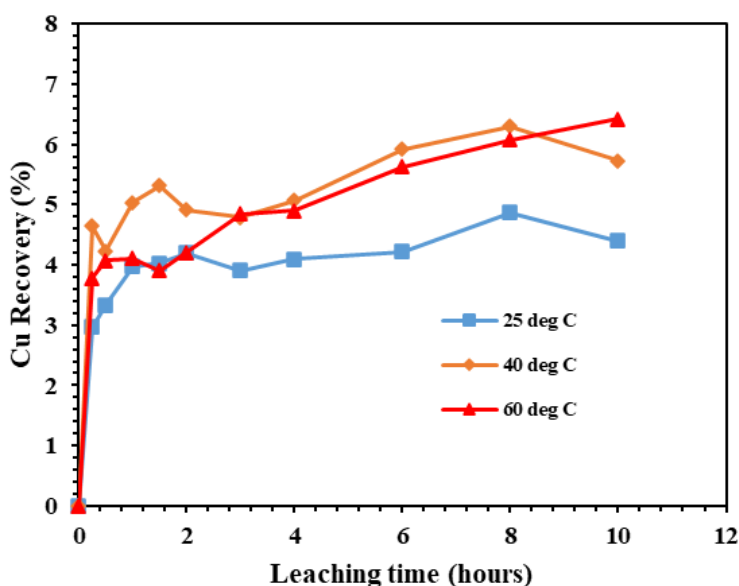
Figure 7-3 Copper (chalcopyrite) dissolution from a Cu-Ni sulphide ore concentrate in terms of recovery at different temperatures
