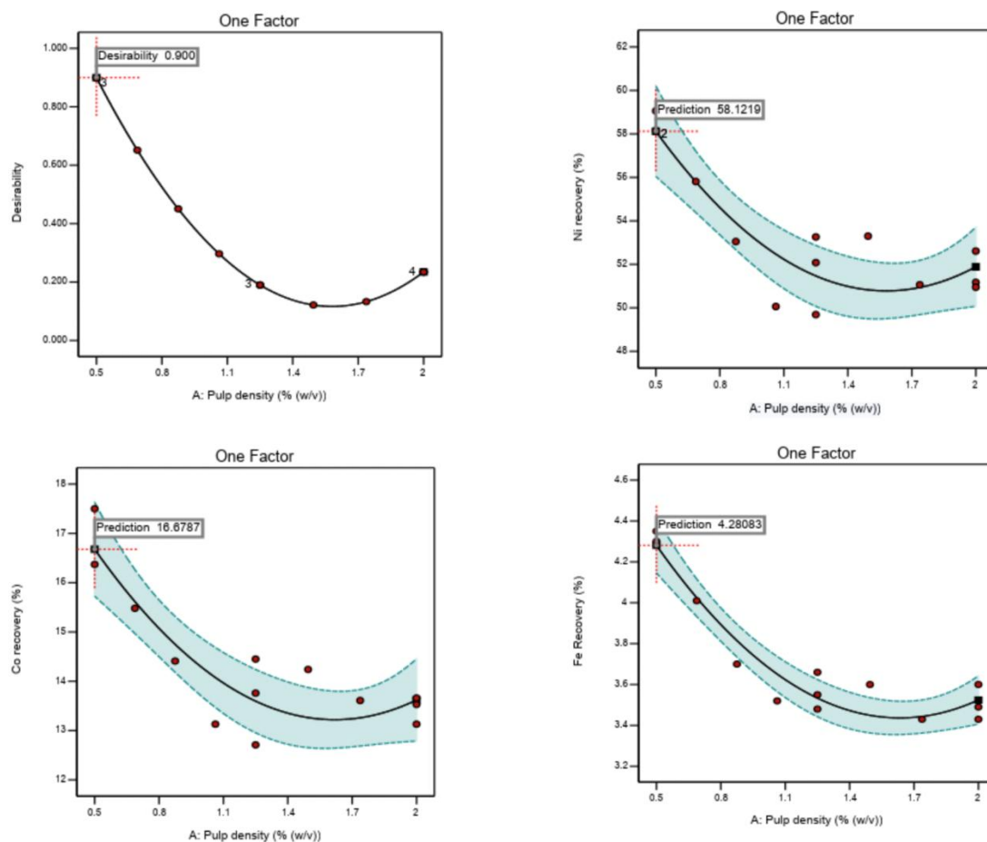
Figure 6-12 Numerical optimization graphs indicating the predicted responses and factor levels
