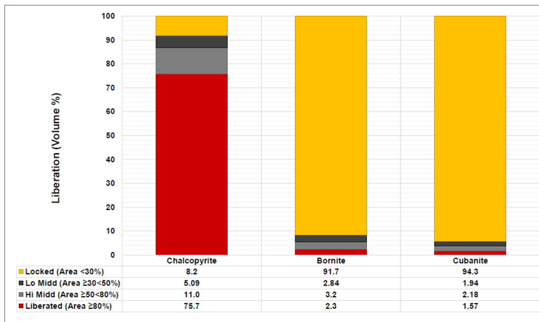
Figure 4-4 Liberation of Cu-bearing Minerals
