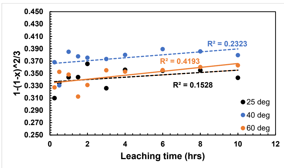
Figure 7-7 Plot of 1 - (1 - x)^{2/3} vs time for Ni Dissolution at 25°C - 60°C
