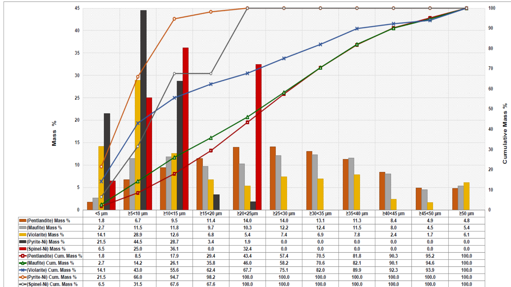
Figure A2 GSD data for the Ni-bearing samples.
