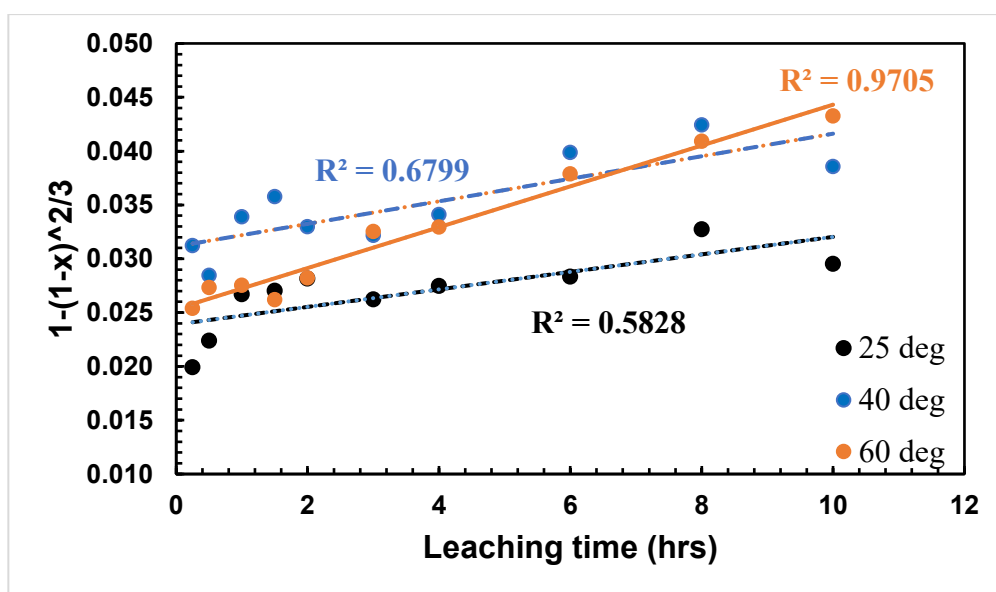
Figure 7-6 Plot of 1 - (1 - x)^{1/3} vs time for Cu Dissolution at 25°C - 60°C
