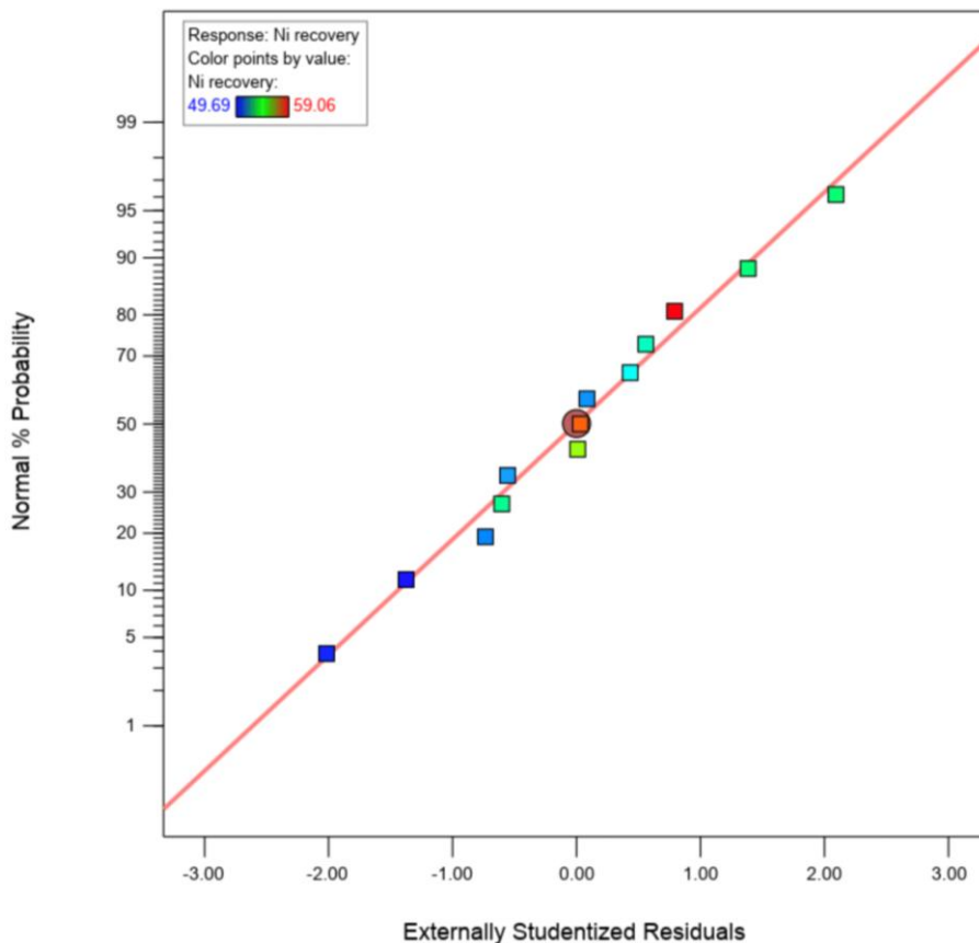
Figure 6-2 Normal plot of residuals for Ni recovery
