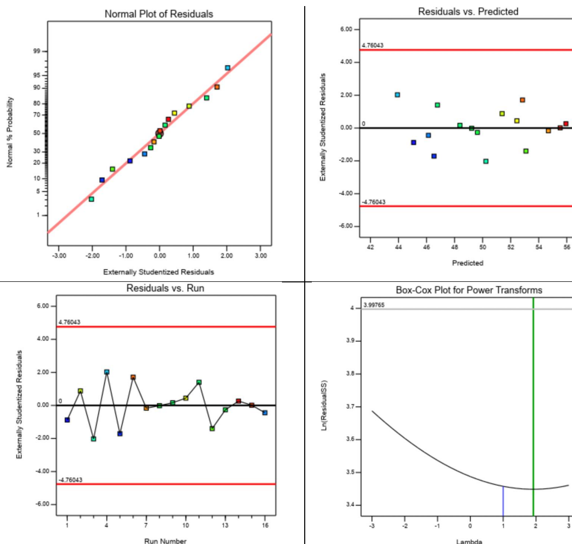
Figure 5-7 Diagnostic plots, top left (Normal plot of residuals), top right (Residuals vs Predicted), bottom left (Residuals vs Run) and bottom right (Box-Cox Plot)
