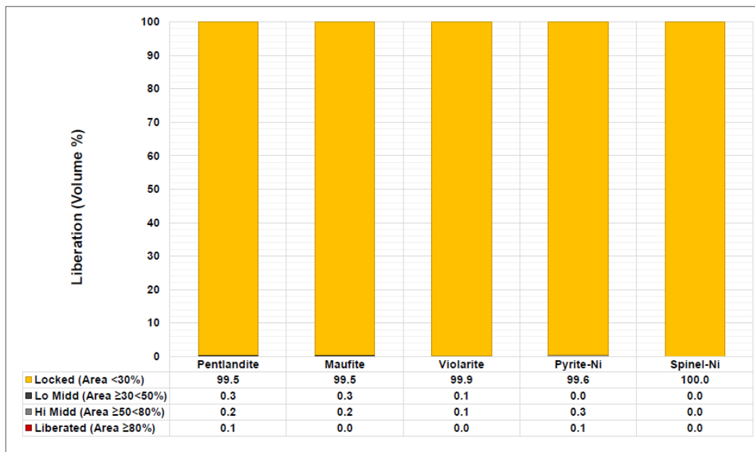
Figure 4-3 Liberation of Ni-bearing Minerals
