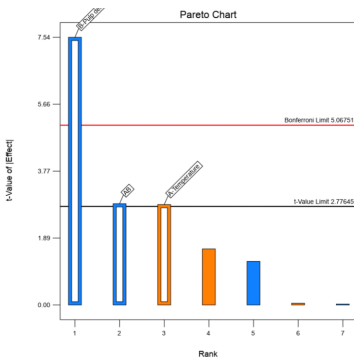
Figure 5-3 Pareto chart for ranking of main and interactive effects (Co recovery)
