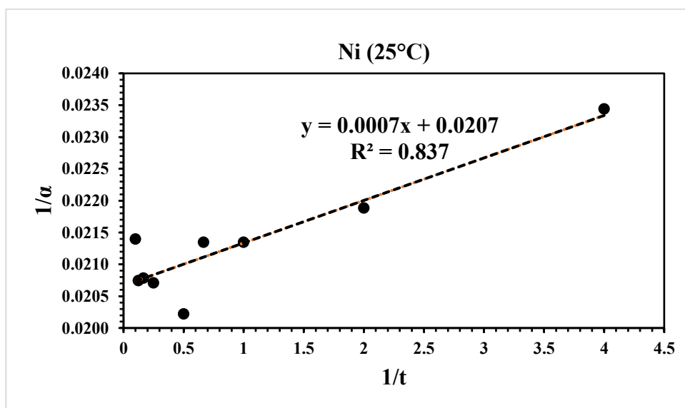
Figure 7-10 Plot of \frac{1}{\alpha} vs \frac{1}{t} for the proposed SPM-PSO Ni kinetic model at 25°C
