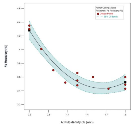
Figure 6-6 Response surface plot for Fe recovery
