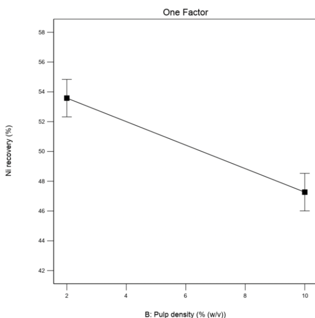
Figure 5-8 An interaction plot of pulp density vs Ni recovery
