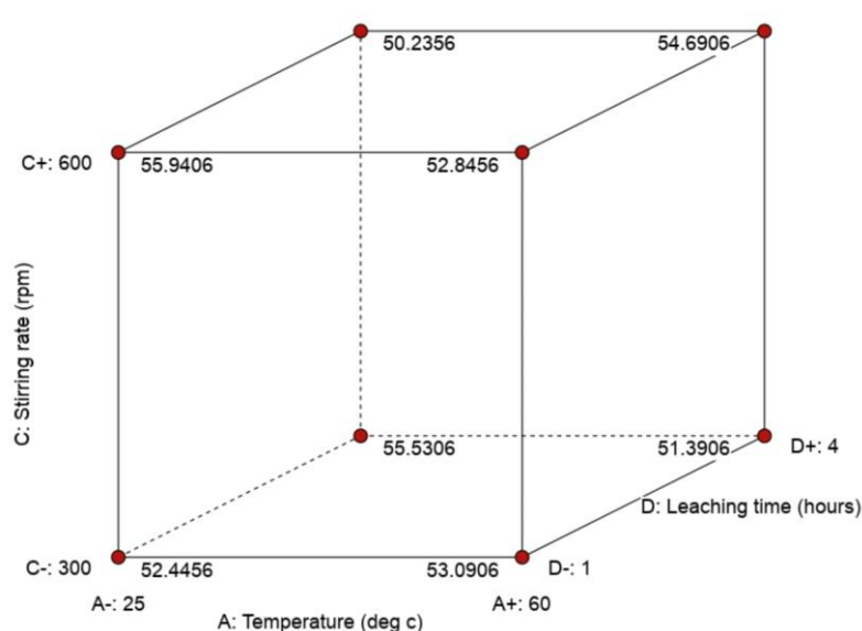
Figure 5-10 Cube plot for Ni recovery
