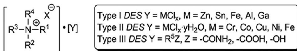
Figure 2-2 Basic formula for quaternary ammonium salt-based DES (García Álvarez, 2014)
