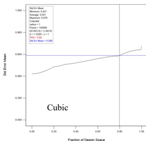
Figure 6-7 FDS plot for cubic model
