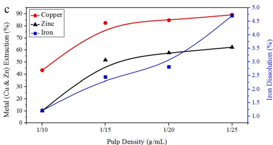
Figure 2-5 Effect of solids to liquid ratio (pulp density) on the extraction of base metals from converter slag (Topçu, Rüşen and Küçük, 2021)
