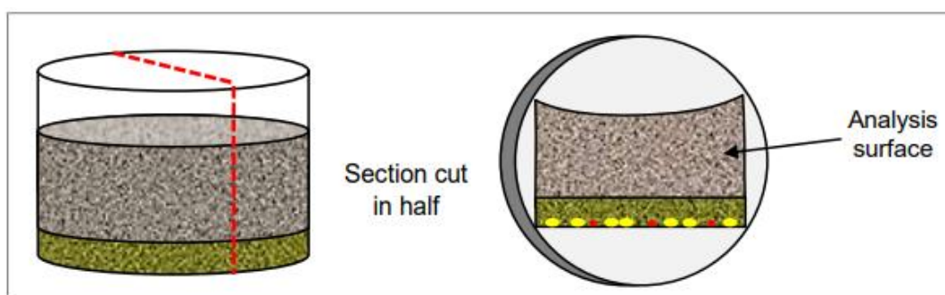
Figure 3-3 A diagram representing a transverse-cut polished block.
