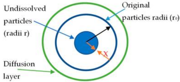
Figure C1 Diagram of an ideal mineral particle undergoing leaching
