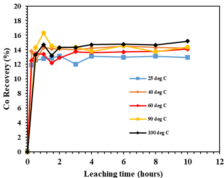
Figure 7-2 Cobalt (pentlandite inclusion) dissolution from a Cu-Ni sulphide ore concentrate in terms of recovery at different temperatures
