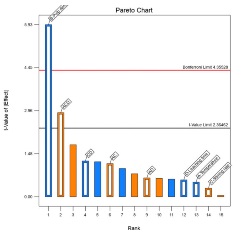
Figure 5-6 Pareto chart for ranking of effects on Ni recovery
