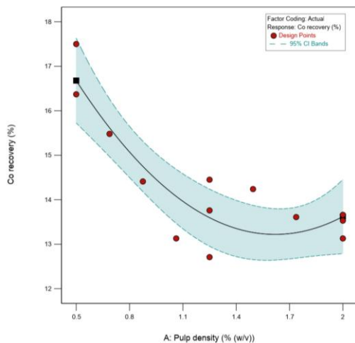
Figure 6-5 Response surface plot for Co recovery
