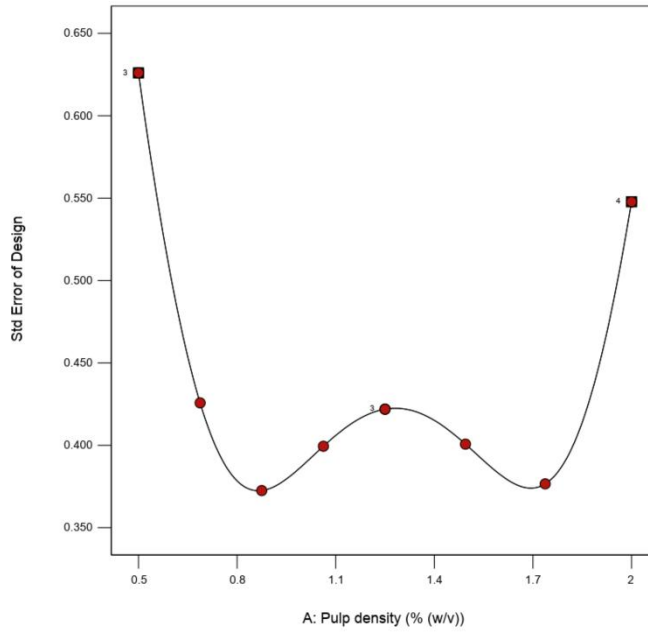
Figure 6-9 Standard error of design for quadratic model
