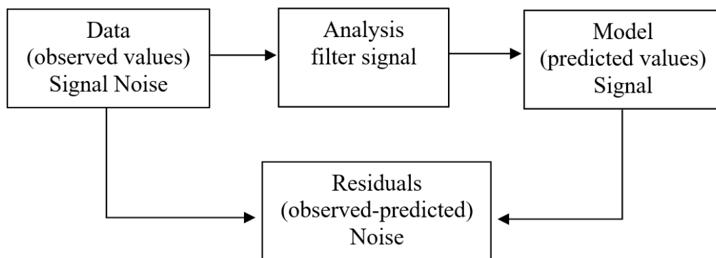
Figure 6-1 Derivation of residuals
