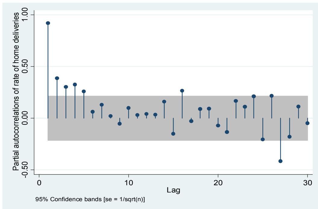
Figure 12: The partial autocorrelations function with 95% confidence band
