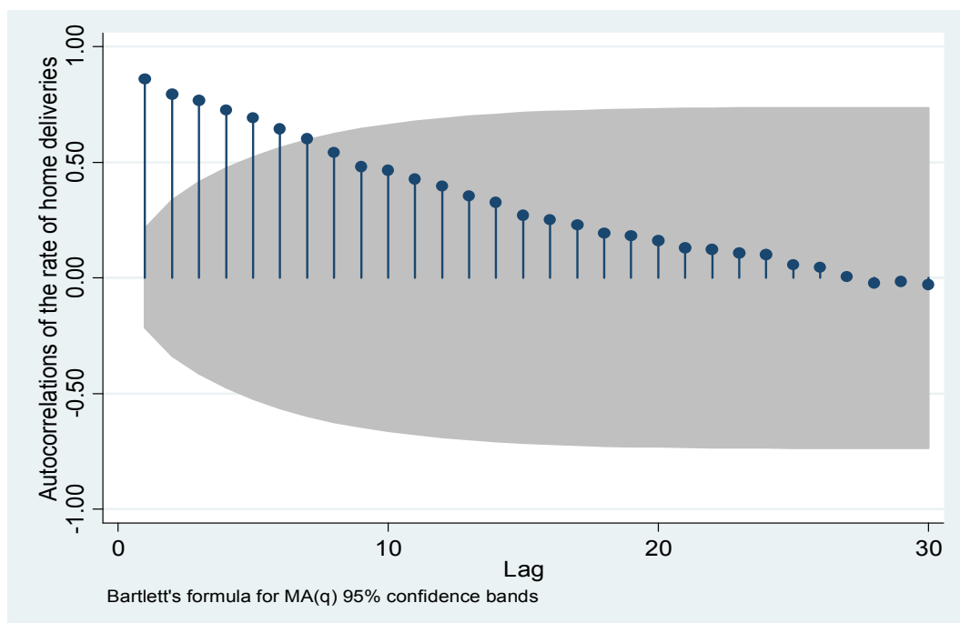
Figure 13: The autocorrelations function with 95% confidence band
