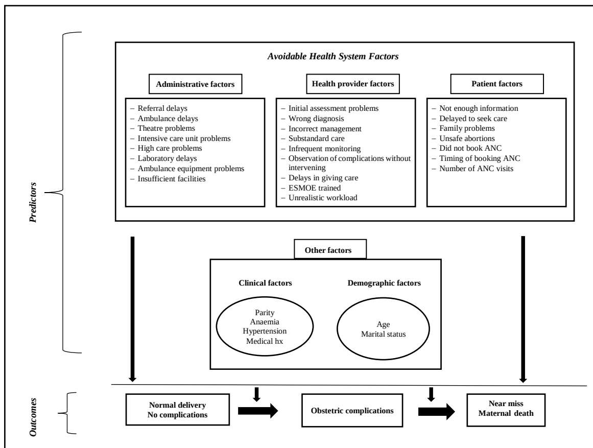
Figure 1: Analytical framework
