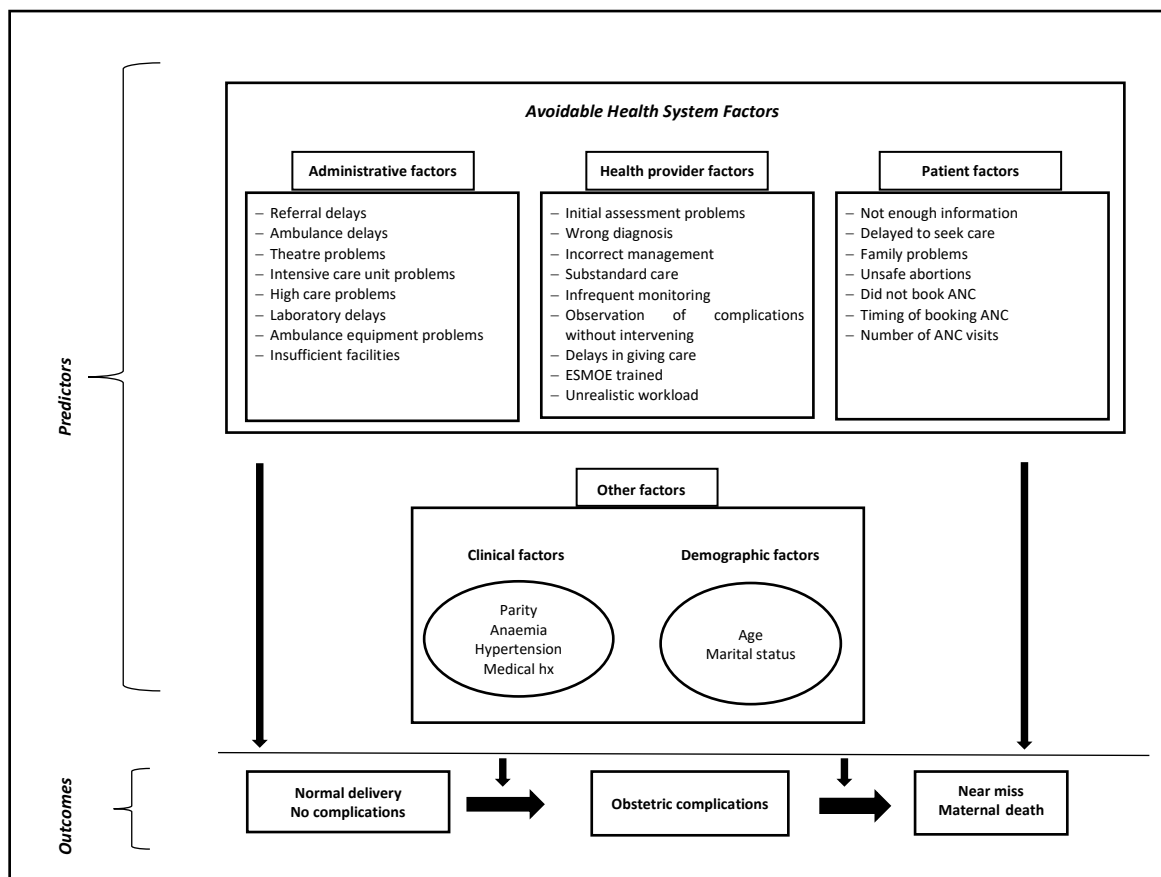
Figure 3: Analytical framework
