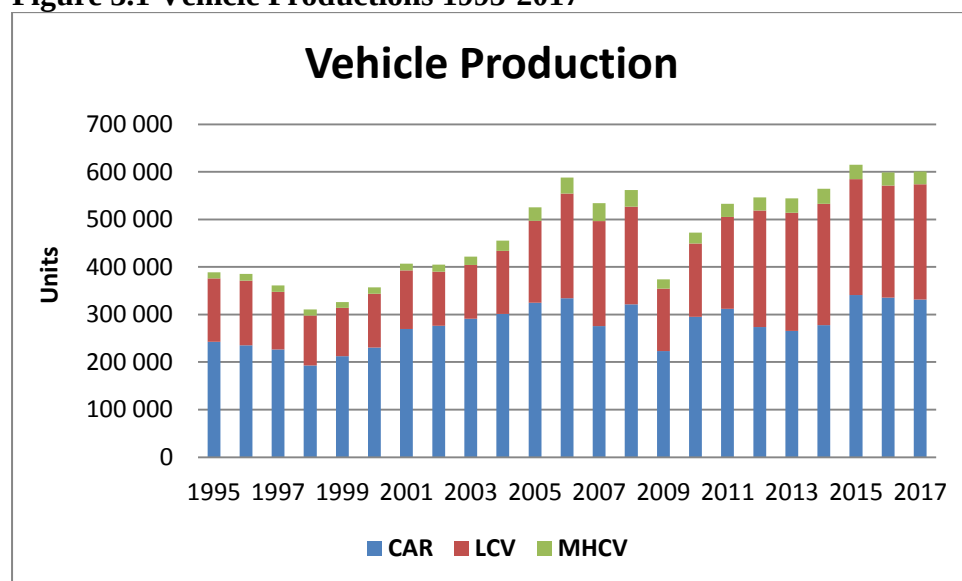
Figure 3.1 Vehicle Productions 1995-2017
