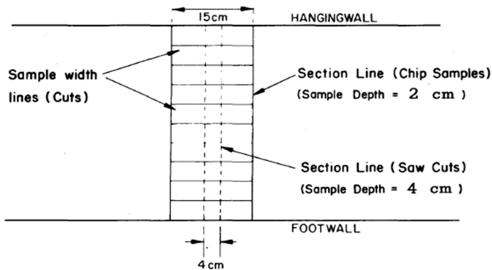
Figure 2.11: Sampling method applied at the Randfontein Estate Gold Mine for chip sampling and diamond –saw (Magri and McKenna, 1986:338).
