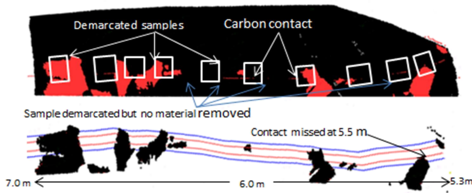
Figure 3.9: A software plot of points generated by the Faro laser scan, the irregular shapes of the samples removed during the extraction process highlights the irregular extraction compared to extracting pre-defined sample shapes from hard quartz reefs.
