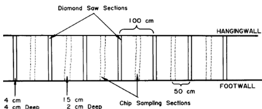
Figure 2.13: Sampling method at the Western Areas Gold Mine. (Magri and McKenna, 1986:344)
