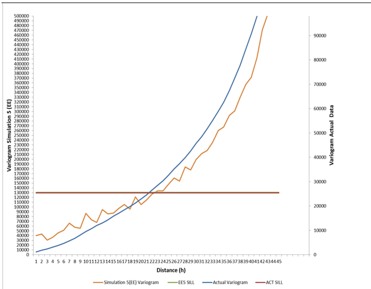
Figure 6.18: Actual shape of the semi-variograms with their sills aligned.
