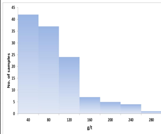
Figure 4.2: Positively skew distribution of chip sampling data
