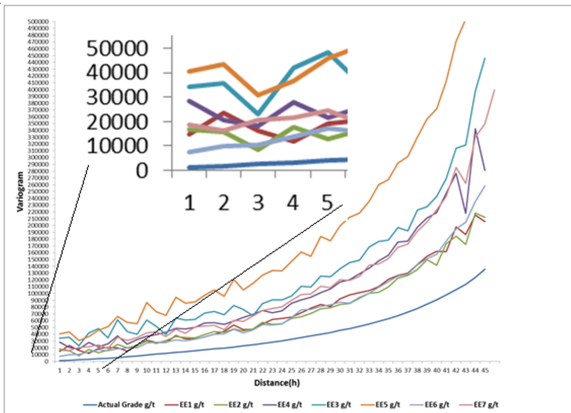
Figure 6.16: Semi-variograms for each of the simulated samples calculated; the inset shows the nugget effect of the variograms near the origin.
