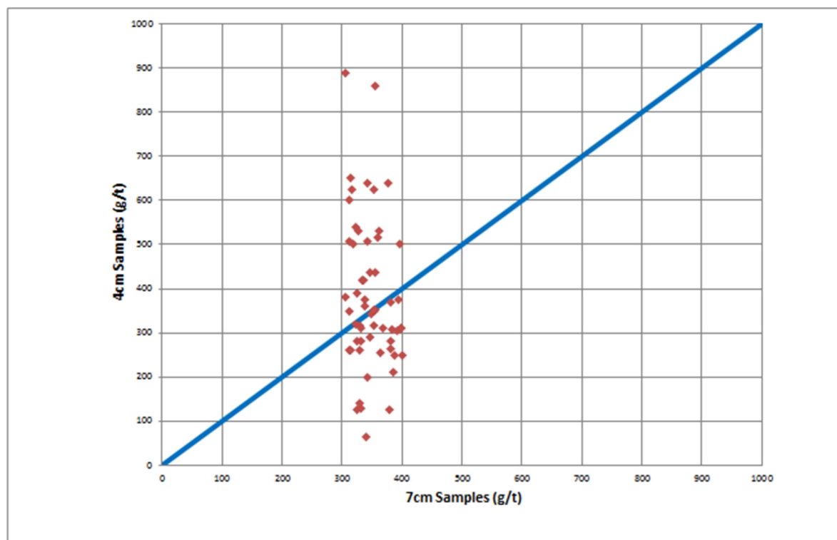
Figure 2.6: New comparisons between samples of different dimensions indicate something artificial happening in the 7cm data.
