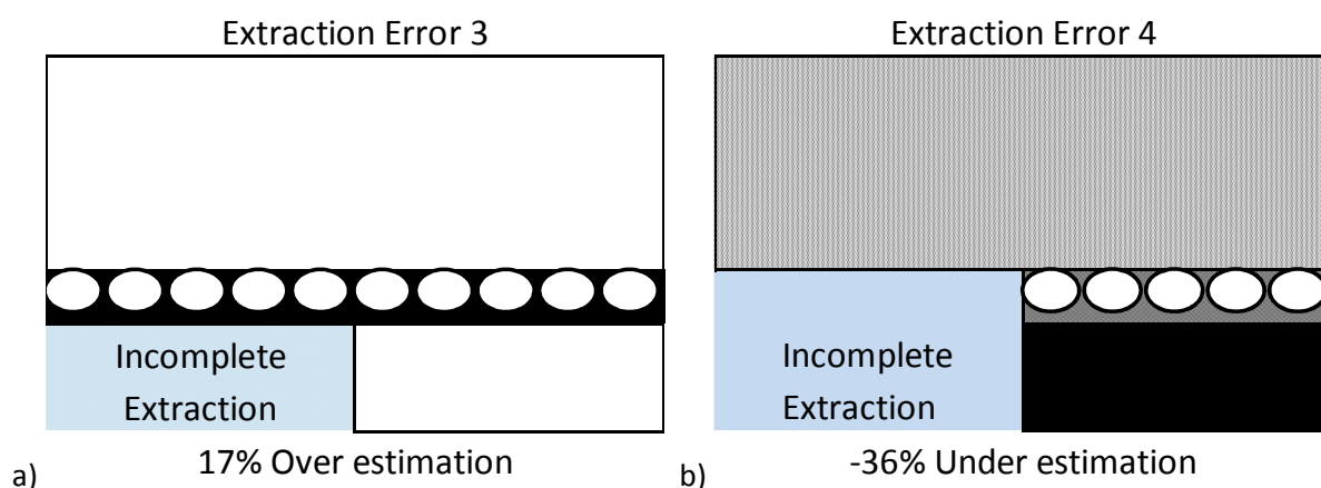
Figure 6.3: Diagram indicating the probable area of under extraction for a) Extraction Error 3 and b) Extraction Error 4
