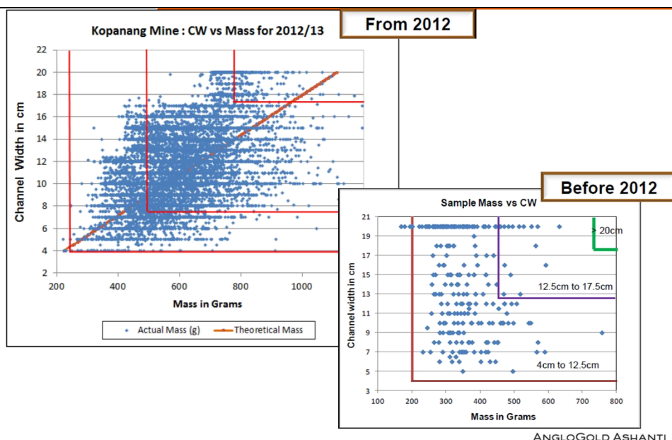
Figure 2.21: Comparison of the improved correlation observed between the actual mass and the theoretical mass before and after implementing the quality index (Freeze, 2013)
