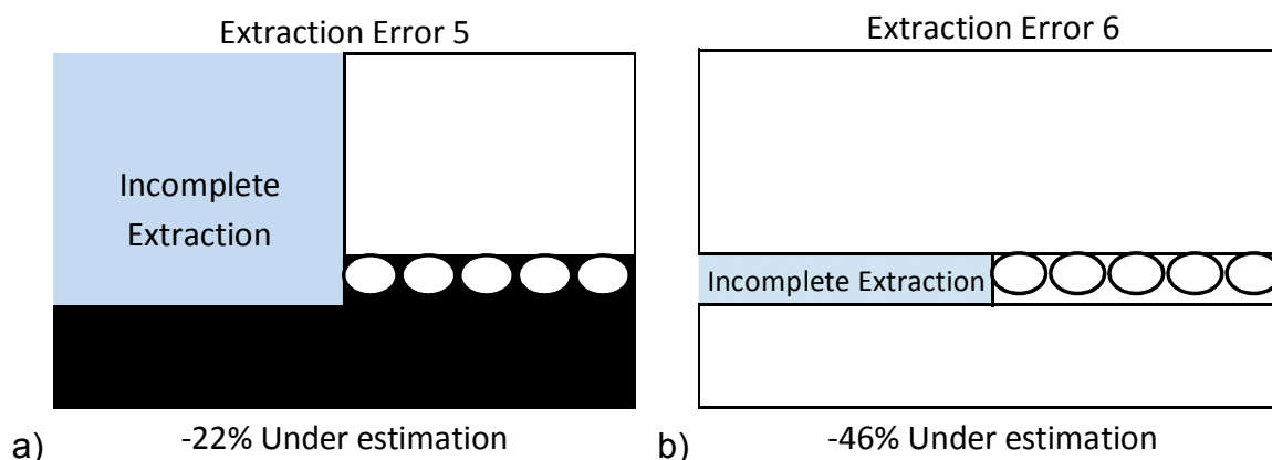
Figure 6.4: Diagram indicating the area of under extraction for a) Extraction Error 5 and b) Extraction Error 6
