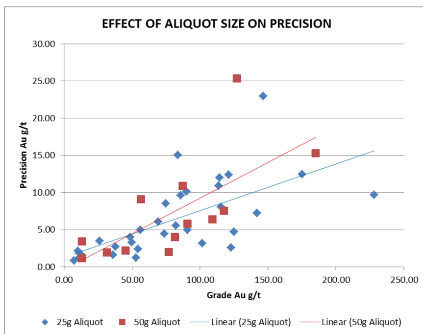
Figure 4.4: Effect of aliquot size on precision
