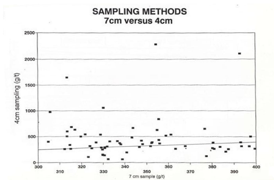
Figure 2.5: Grade comparison done between samples taken at different sample dimensions (De Jager, 1997: 92)
