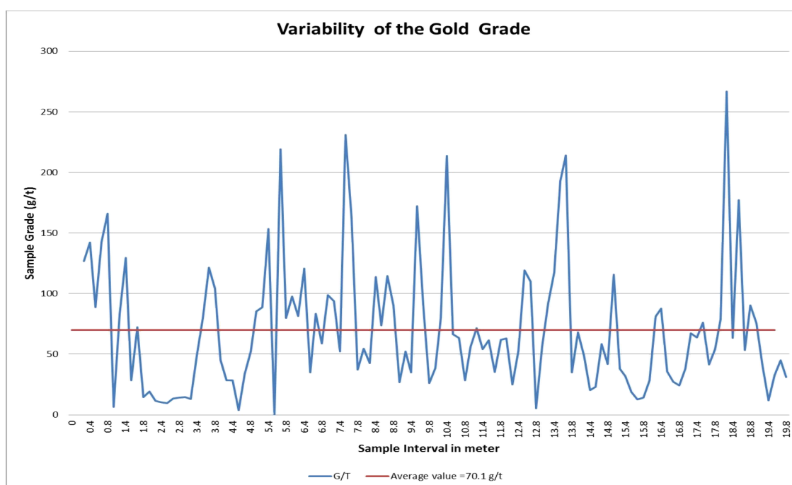
Figure 4.3: Variability of the 120 samples gold grade in the development raise
