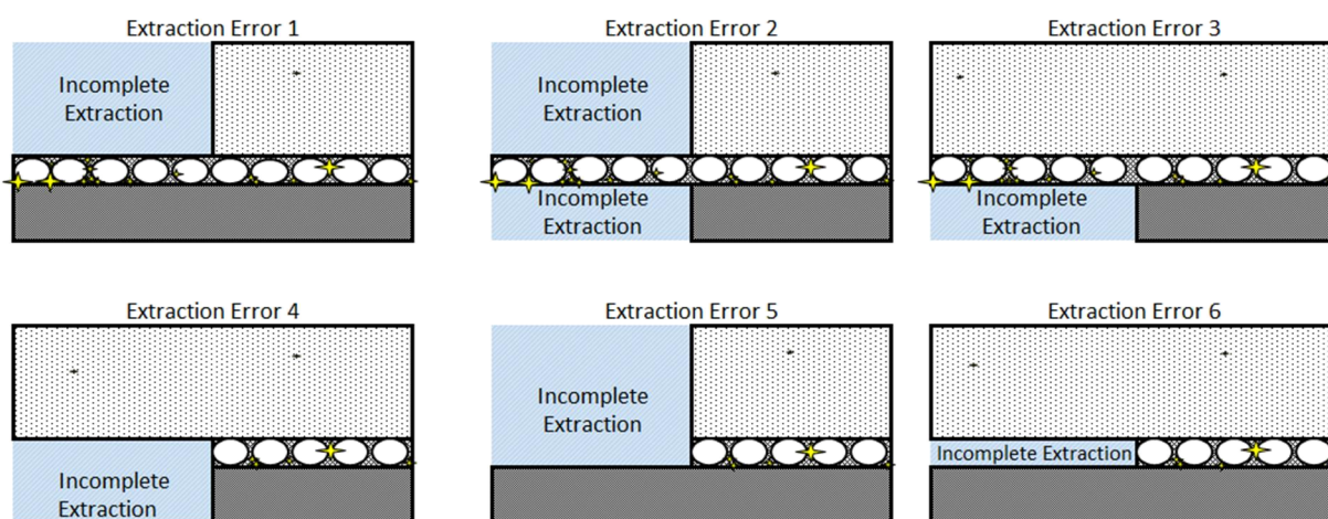
Figure 6.15: Six probable combinations of lithological components illustrate the effect that incomplete extraction may have on the true “nugget effect” of a sample
