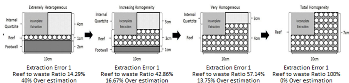
Figure 6.12: Percentage extraction error decreases as the sample becomes more homogenous.
