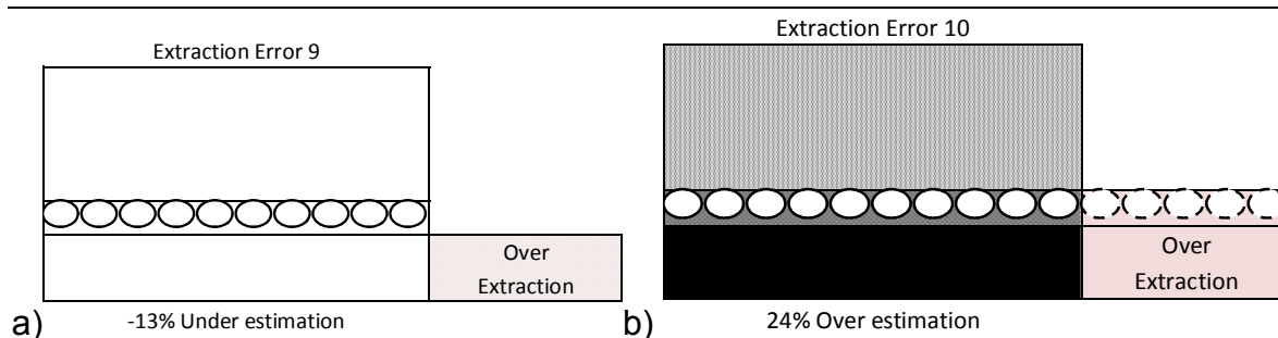
Figure 6.6: Diagram indicating the area of under extraction for a) Extraction Error 9 and b) Extraction Error 10
