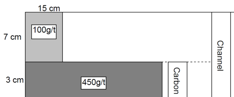
Figure 5.4: Diagram explaining the new method of sampling and how the variance could be reduced by simply increasing the sample width of the high grade contact portion (Cawood, 2003:28)
