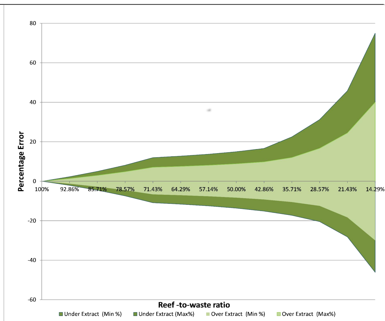
Figure 6.13: Graphical depictions on how errors increase from a very homogenous (on the left) to a highly heterogeneous (on the right composition).
