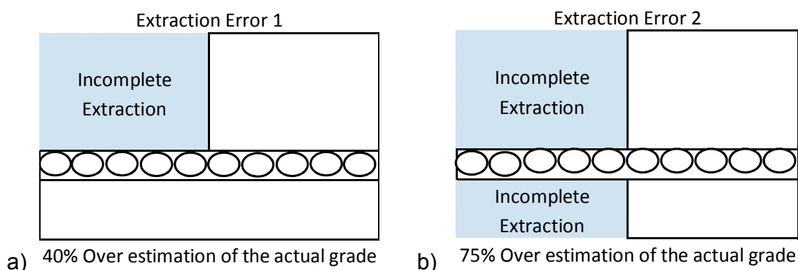
Figure 6.2: Diagram indicating the area of under extraction for; a) Extraction Error 1 and b) Extraction Error 2.
