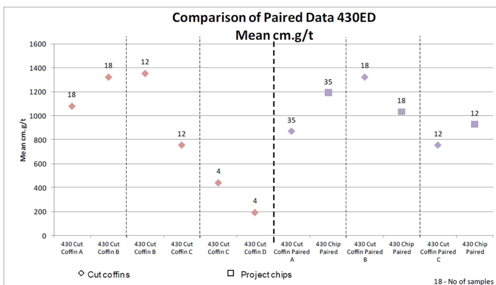
Figure 2.16: Comparison of mean cm.g/t paired data for the 430 estimation domains (Flitton, 2011:11).
