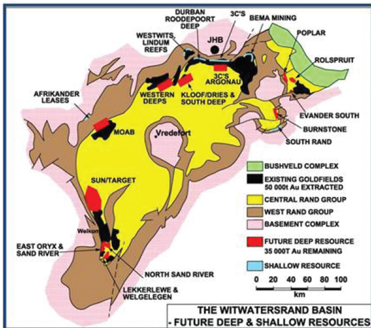
Figure 2.2: Major geological features of the Witwatersrand basin showing major goldfields (Viljoen, 2009:131)
