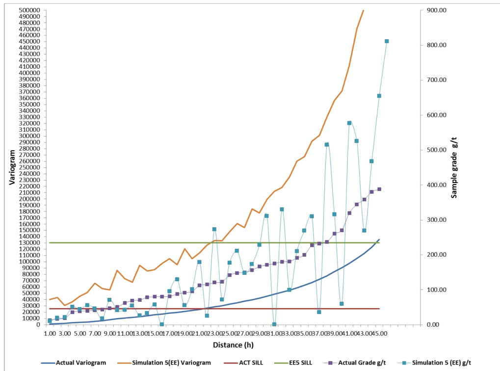
Figure 6.17: Comparing the differences of two semi-variograms and their grades at individual distances.
