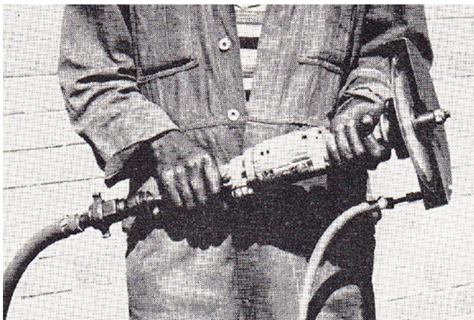
Figure 2.9: The then modern version of the St. Clair sample cutter used to compare with conventional chip sampling. (Sichel, 1961:567)
