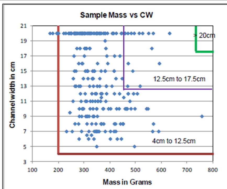
Figure 2.18: Chip data not indicating any relationship between the width extracted and the sample mass. Source: Freeze, 2013:16
