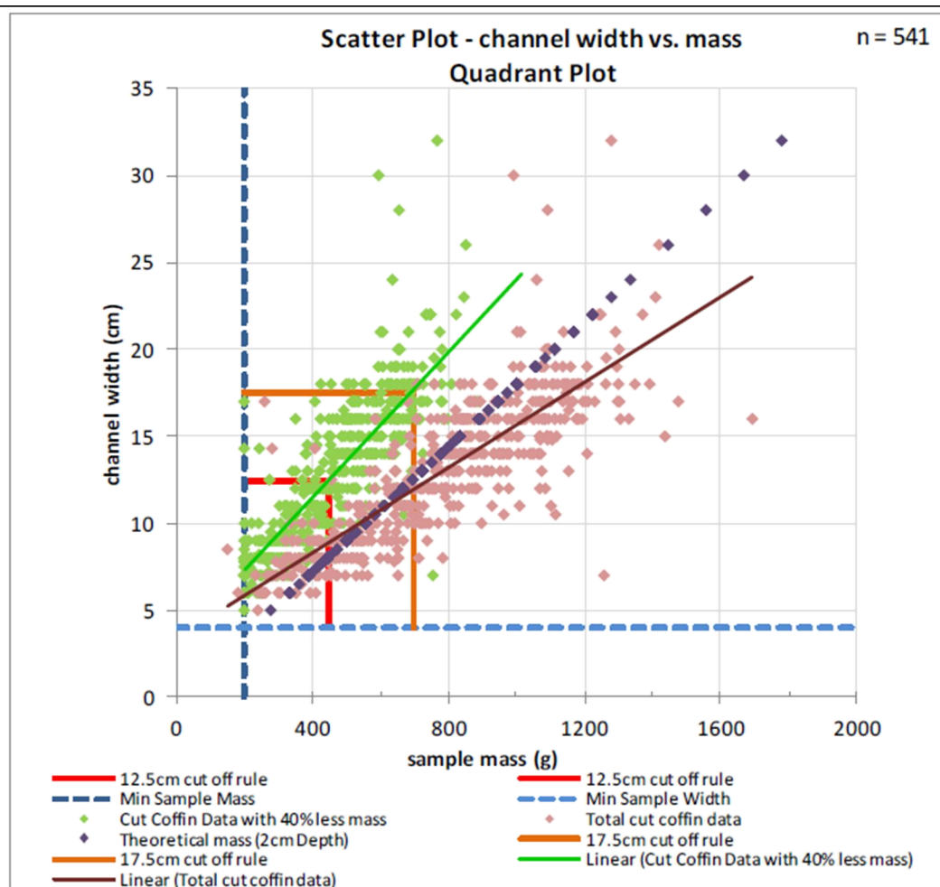
Figure 2.19: Quadrant Cw-Mass plot used for quality control (Flitton, 2011:15)
