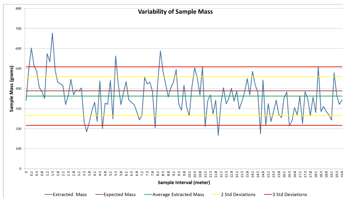
Figure 4.1: Variability of the individual mass of samples.
