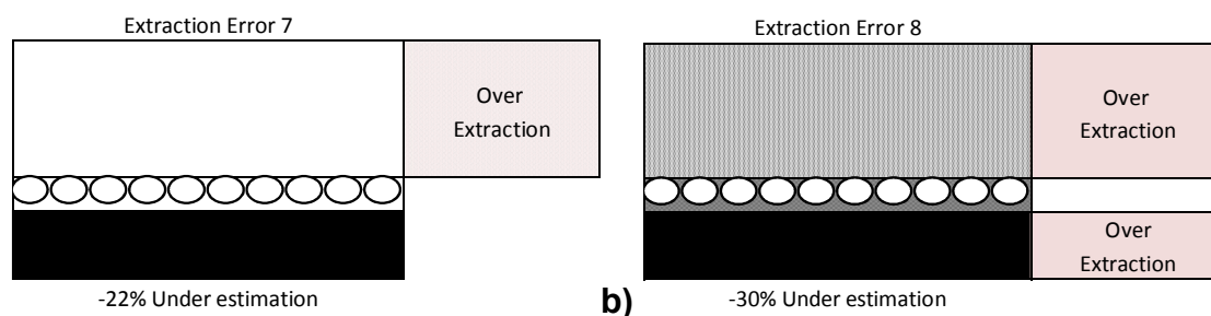
Figure 6.5: Diagram indicating the area of under extraction for a) Extraction Error 7 and b) Extraction Error 8
