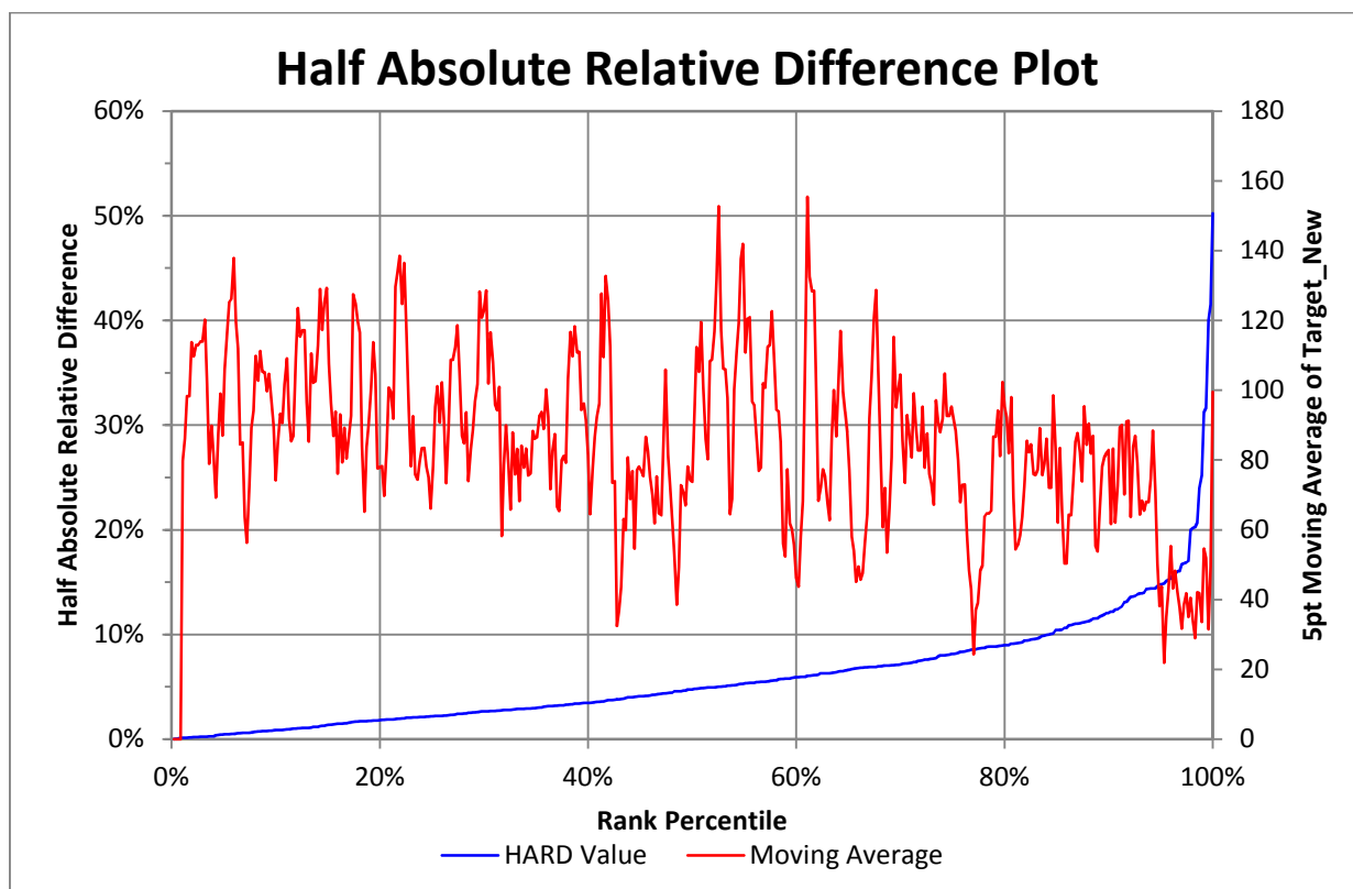
Figure 4.5: Half absolute relative difference plot for duplicate assays
