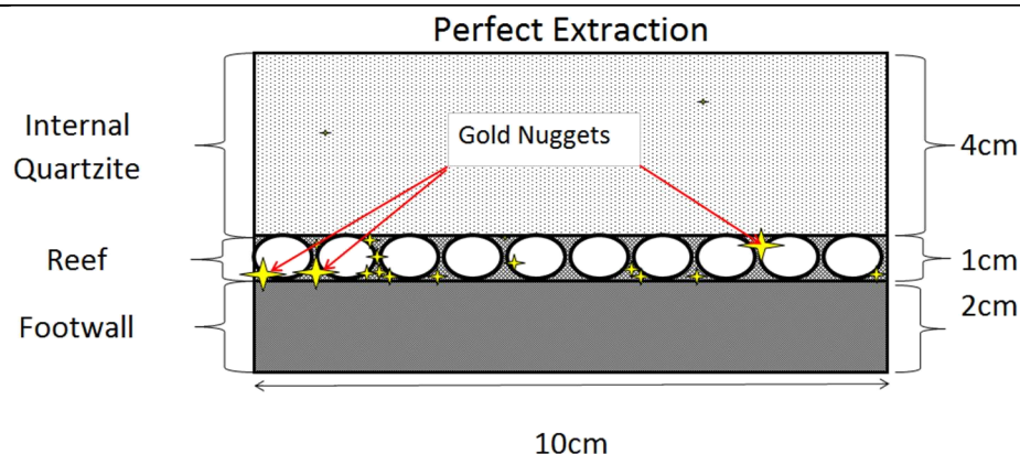
Figure 6.14: Illustration of gold nuggets (gold stars) in a correctly demarcated sample
