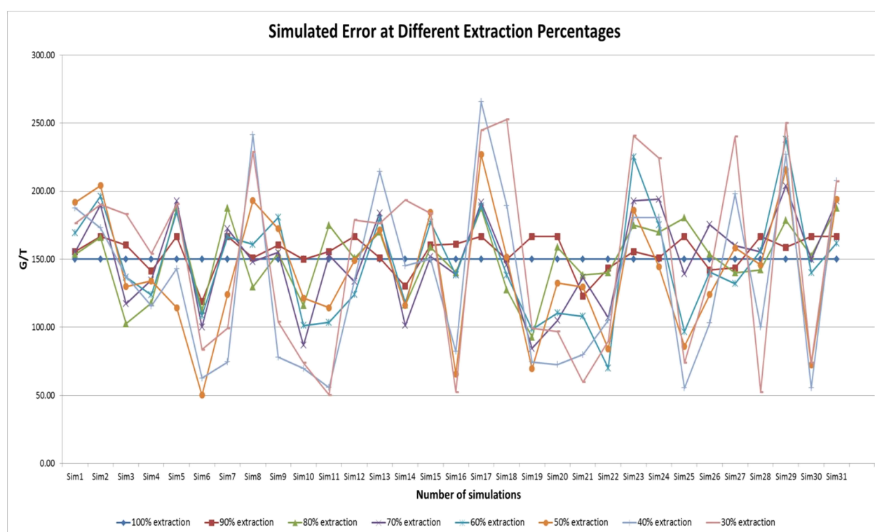
Figure 6.9: A graphical presentation on how the percentage material extracted from a delimited sample is affecting the precision of the grade.
