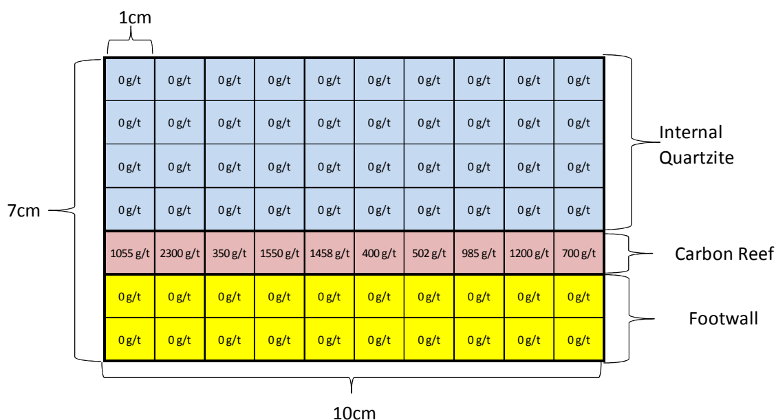
Figure 6.8: New “Simulated Chip Sample Model” generated and split into 1\text{cm}^3 with corresponding grades.
