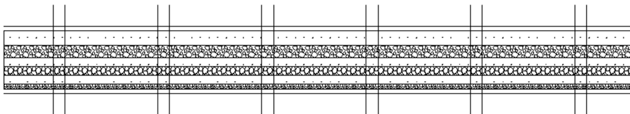
Figure 5.1: The underground stope face actually represents a heterogeneous 1-D 'stream' and the vertical lines represent the sample section (Fourie and Minnitt, 2013)
