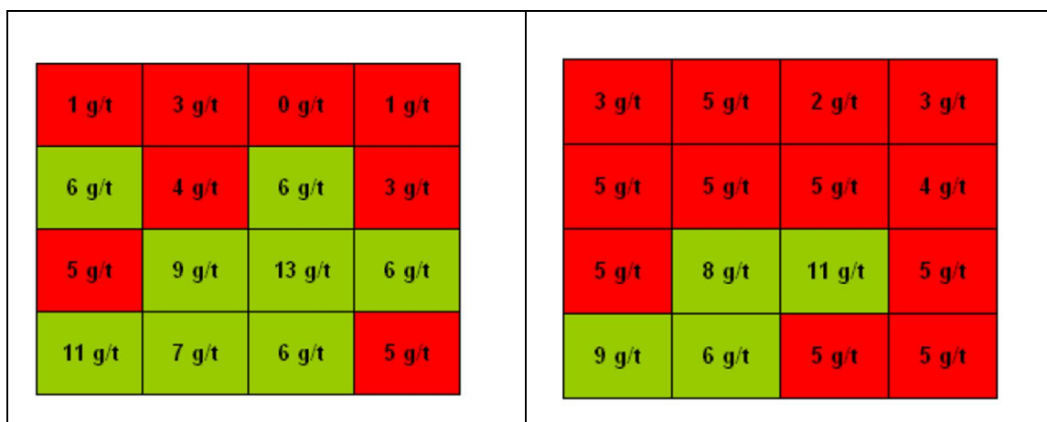
Figure 6.19: a) Estimated grade distribution of the 16 minable block, assuming that the semi-variogram is accurately estimated and modelled b) Estimated grade estimation of the 16 minable blocks, assuming that the semi-variogram's nugget effect is now too highly estimated (Morgan, 2005:41).
