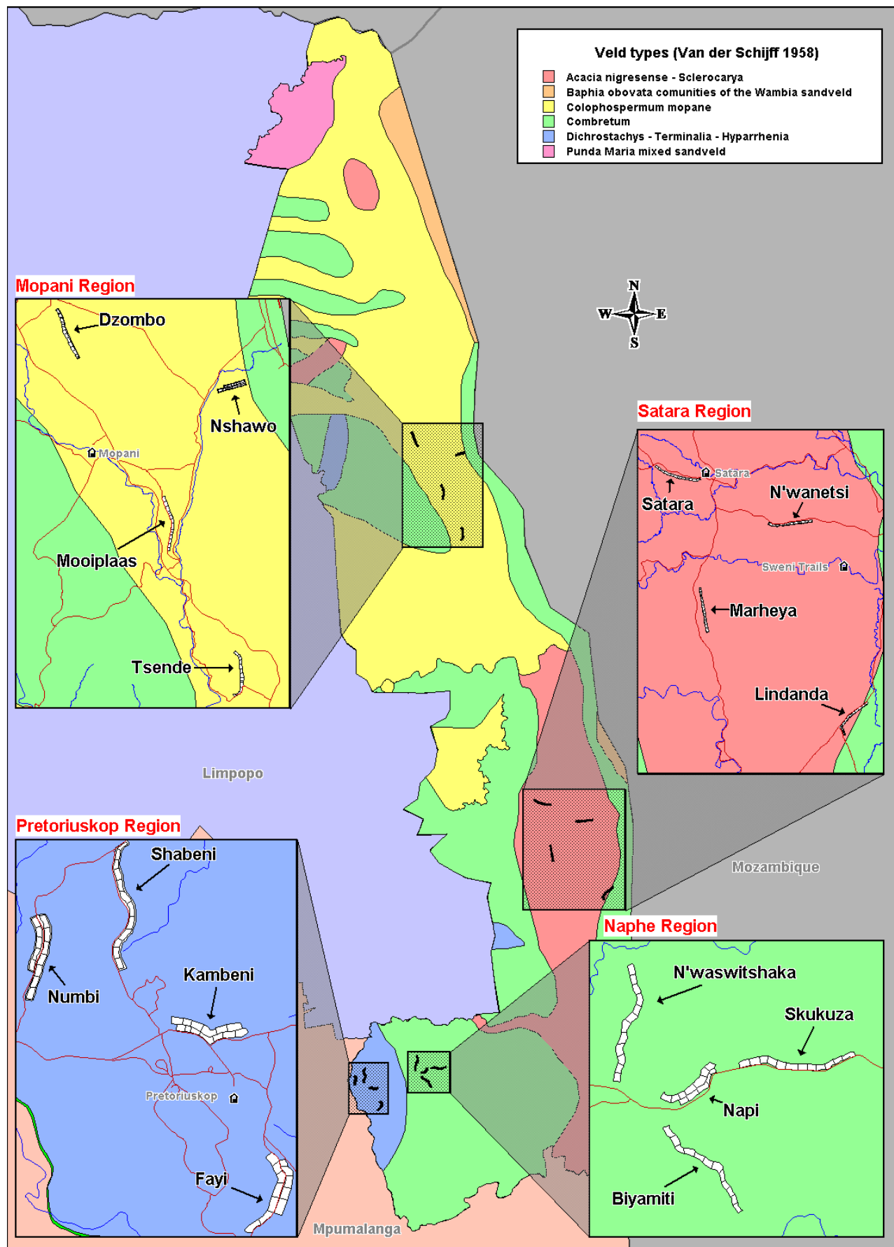
Figure 6-1: The layout of the Experimental Burn Plot experiment in the four vegetation communities in the Kruger National Park.
