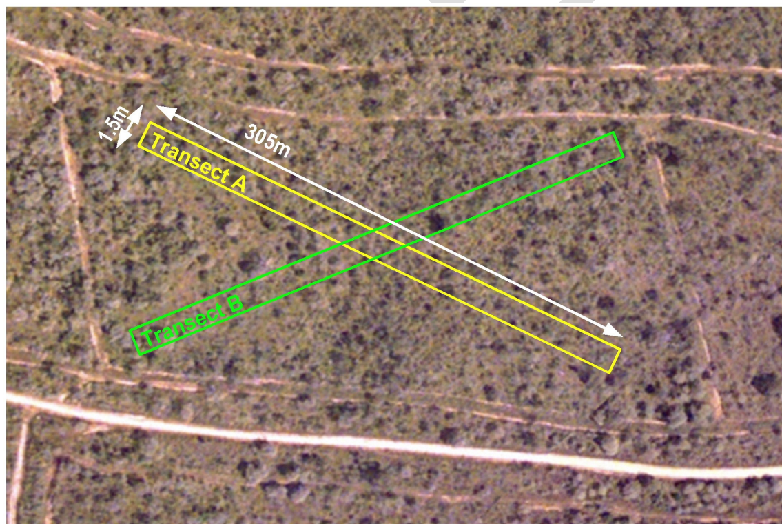
Figure 6-4: Showing the placement of the two transects along the diagonals of a treatment plot in the baseline woody vegetation survey of the EBPs in 1954.
