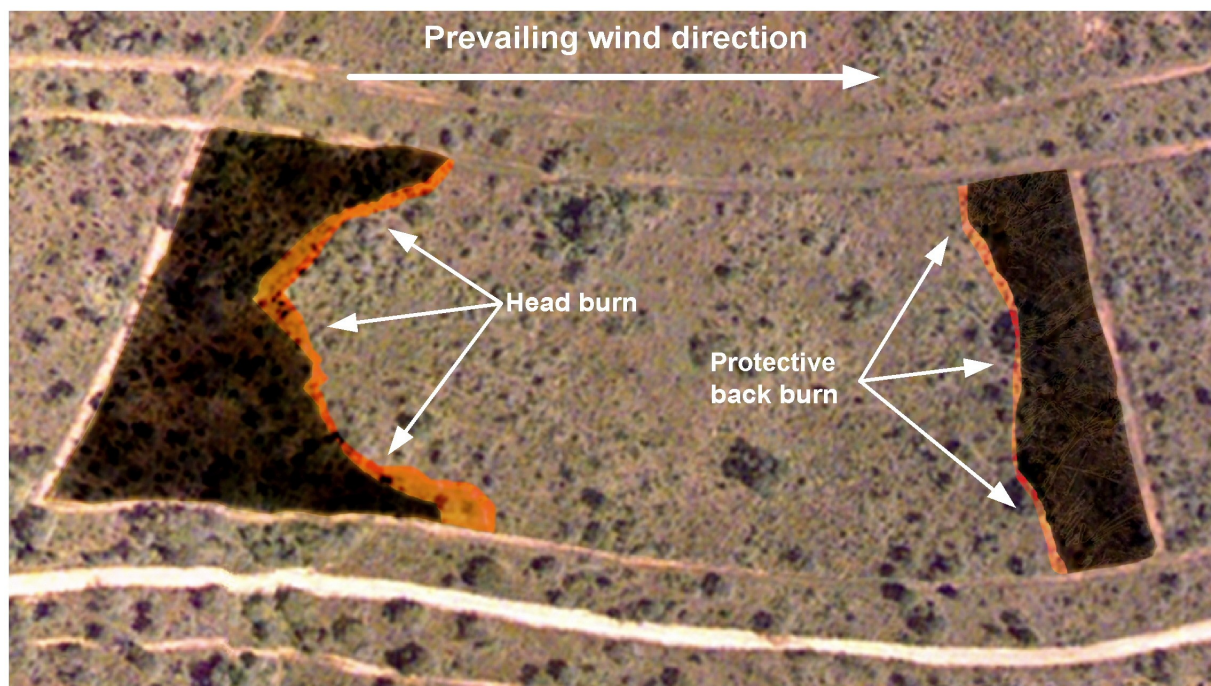
Figure 6-3: Showing the typical application of a fire treatment to an EBP, with a protective back burn to prevent the head burn from jumping the firebreak and burning the neighbouring plot or the surrounding landscape.
