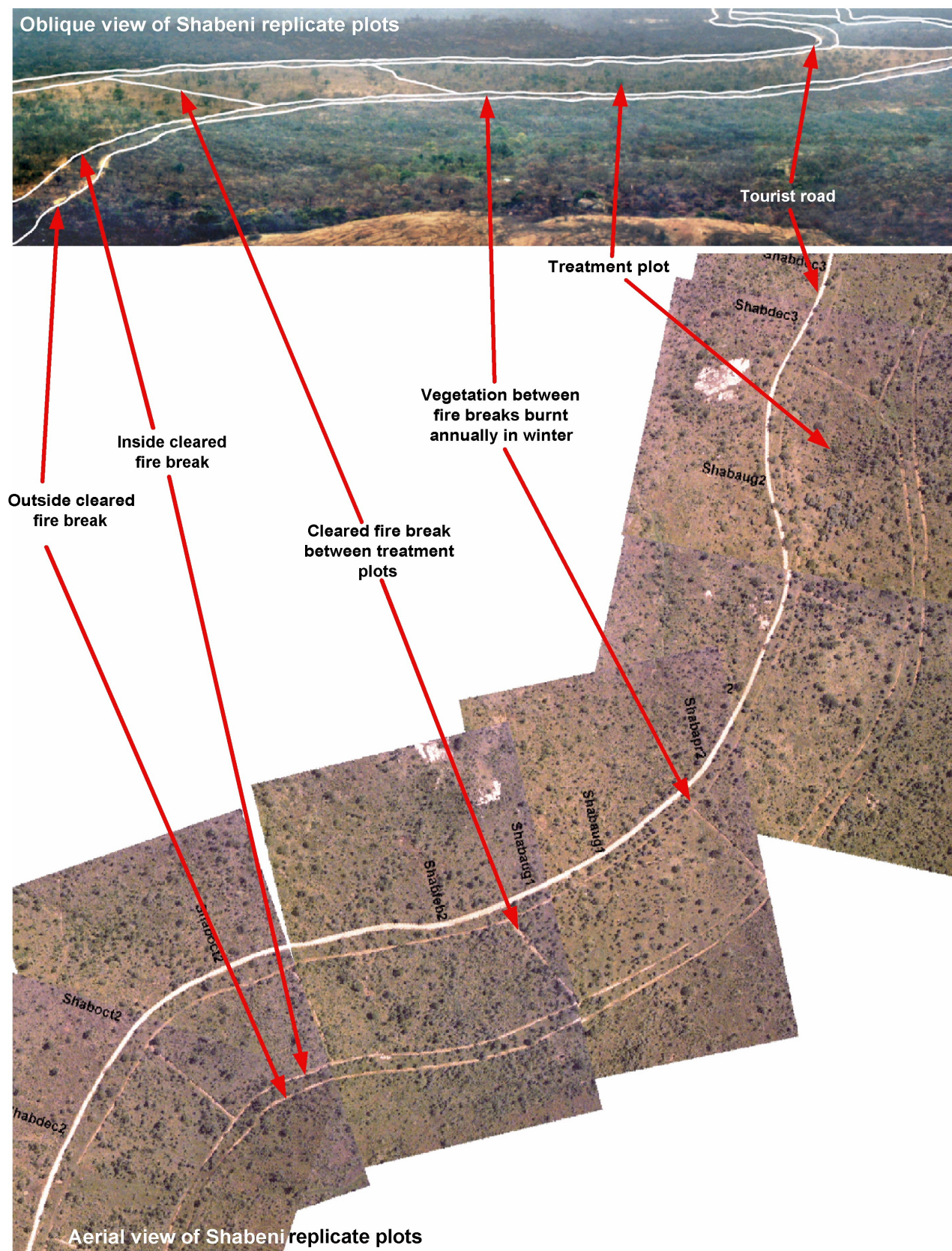
Figure 6-2: Oblique and aerial view of the Shabeni replicate, showing how the treatment plots were setup with the single cleared fire breaks between the plots and the two cleared fire breaks surrounding the replicate.
