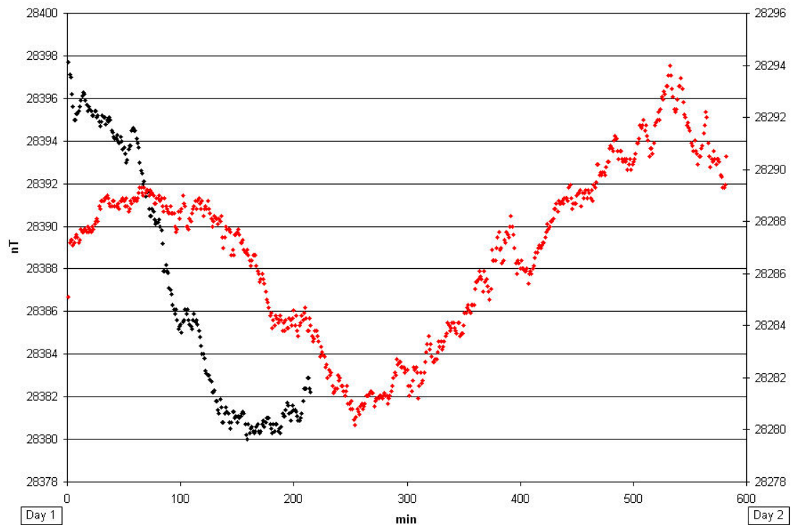
Figure 4.9 – Plot of base station data for the two days spent on the ground magnetic survey. Note: surveys were approximately one year apart, accounting for the \sim 100 nT shift from Day 1 to Day 2. This shift was corrected for in the survey data.
