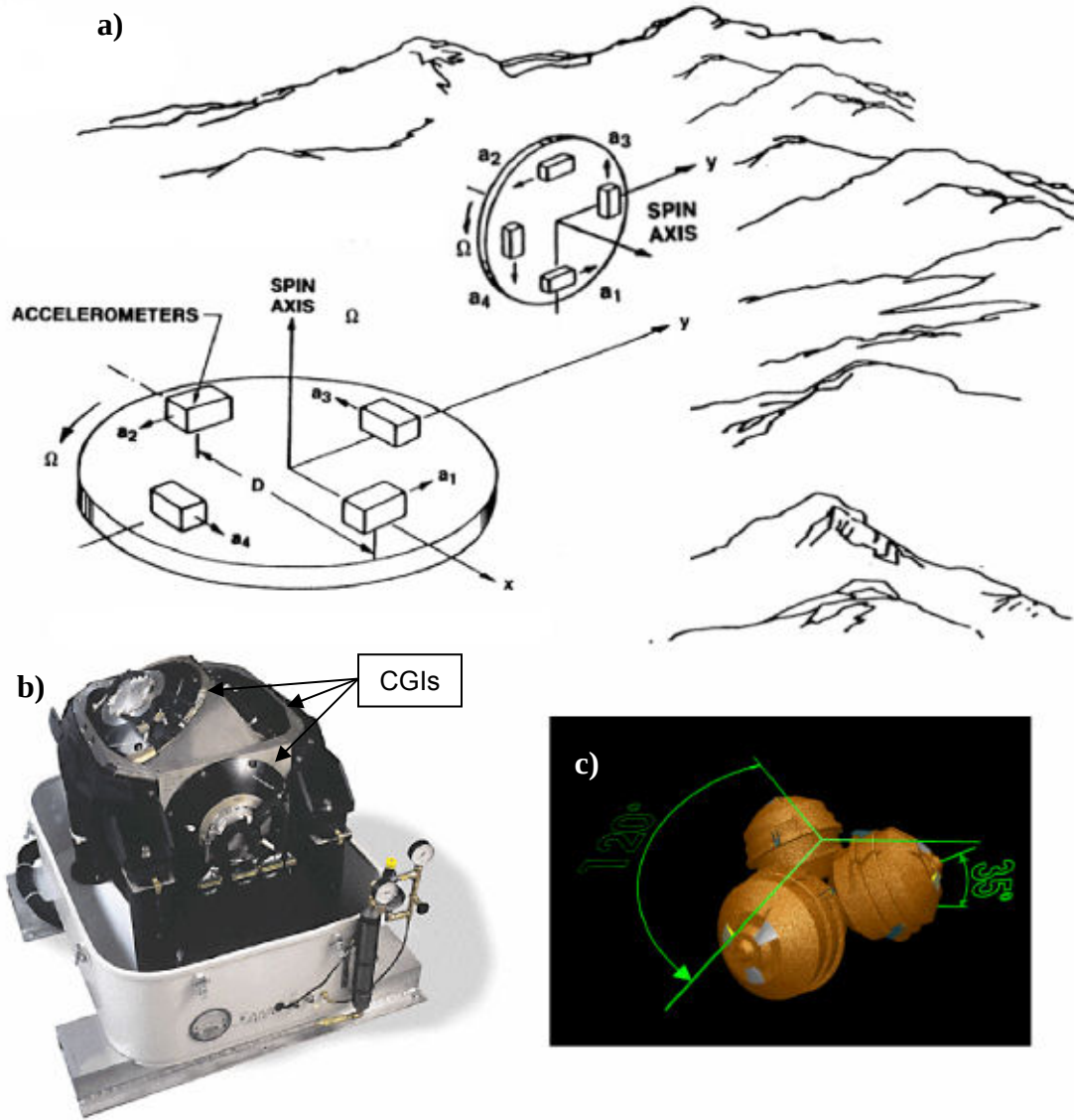
Figure 3.4 – a) Schematic diagram of the Air-FTG ® instrument, showing the arrangement of the accelerometers within each spinning disk, b) image of the Air-FTG ® system, showing positioning of CGIs, and c) geometric arrangement of the GGIs (Murphy, 2004).
