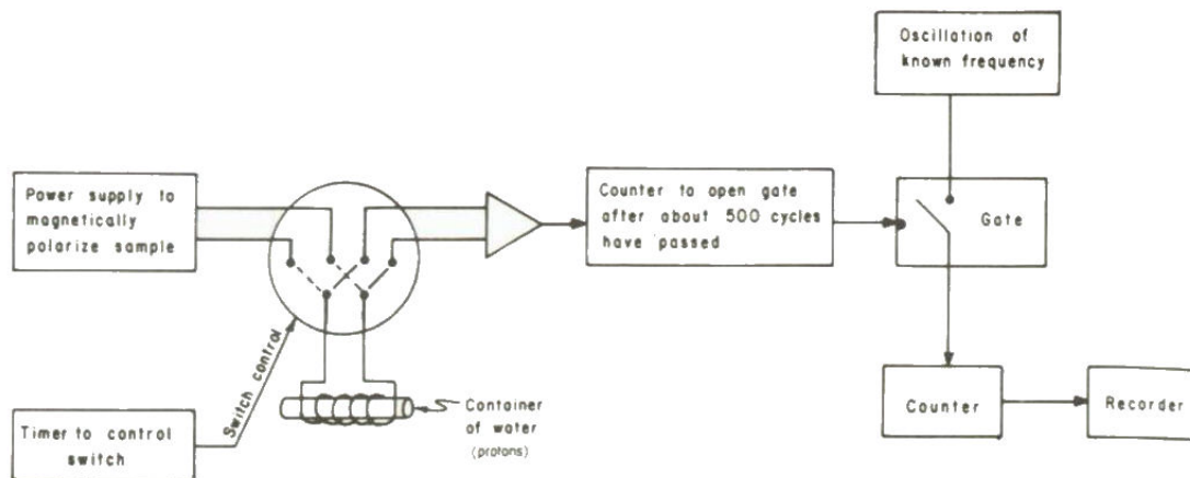
Figure 4.7 – Circuit diagram of a proton precession magnetometer (Telford et al. , 1990).
