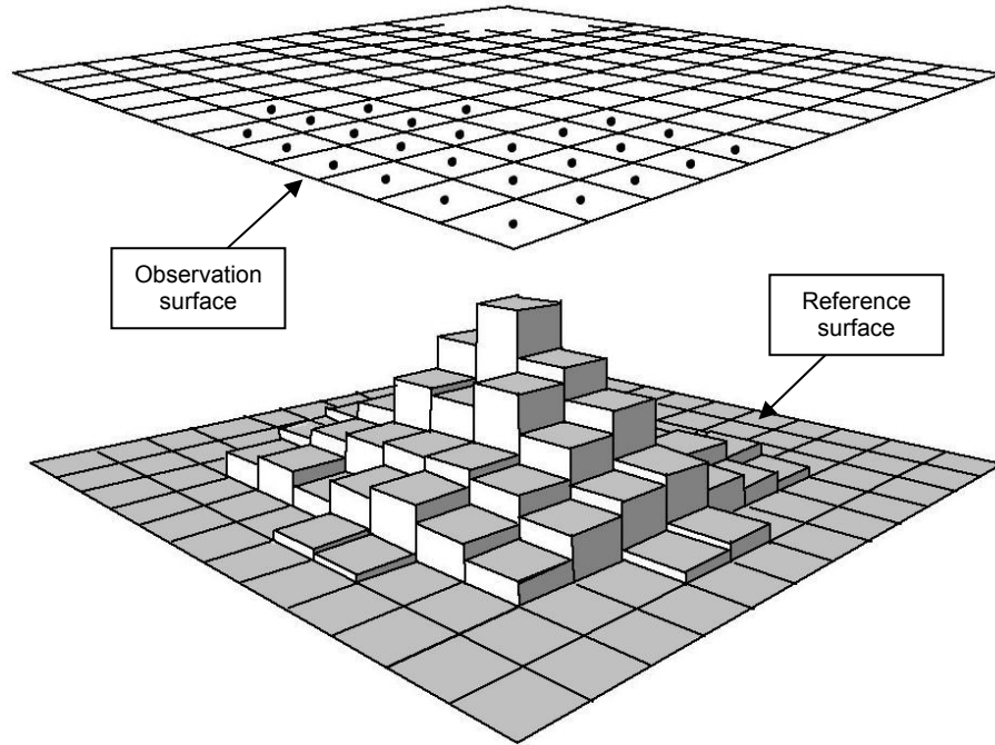
Figure 7.5 – 3D model, defined by Cordell and Henderson (1968), for iterative inversions. Block thicknesses are relative to a reference surface and the calculated gravity data occur on an observation surface.
