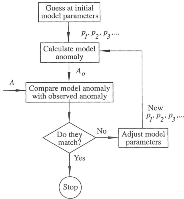
Figure 7.1 – Comparing the forward and inverse method. A represents the measured anomaly, and A_o the calculated anomaly. Parameters p_1, p_2, \dots are the source attributes (e.g. depth, thickness, density), Blakely (1995).
