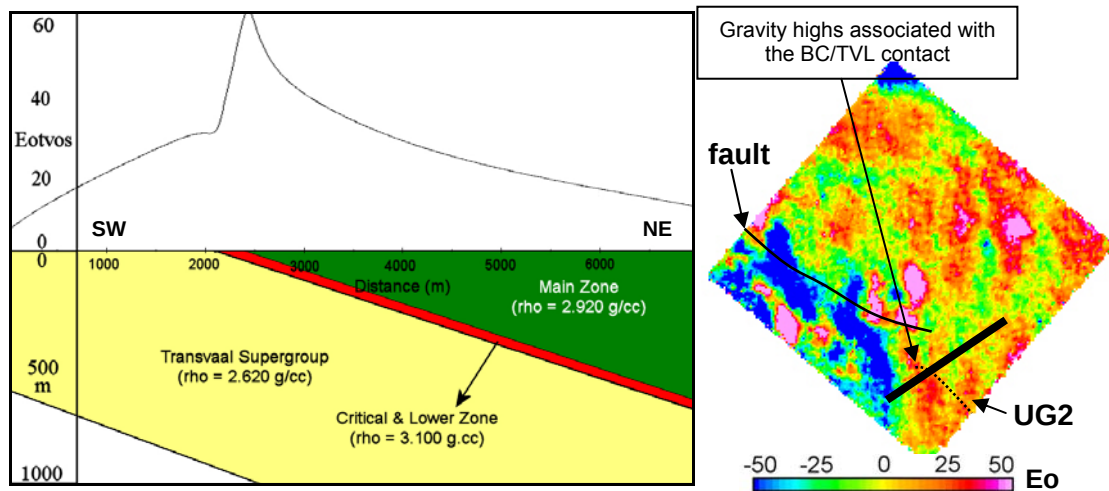
Figure 9.3 – (left) Synthetic 2D T_{zz} response across a Bushveld Complex layered with the Transvaal Supergroup (after Antoine (2004)) using Grav2DC (Cooper, 2003) and SignProc (Cooper, 2000), (right) Gridded T_{zz} map over the study area, showing the response across a similar geological scenario (black line), from AGG data.
