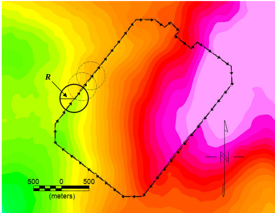
Figure 5.2 – The suture method, with circle (radius: R ) traversing the boundary of the ground gravity survey, interpolating between the ground gravity and calculated airborne G_z data. Note: this figure does not show the final sutured image.
