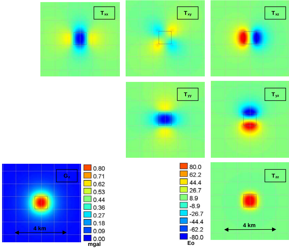
Figure 3.2 – Total gravity field ( G_z ) and FTG gravity components for a buried synthetic cube (outline of cube presented). Parameters: dimensions 1 000 m x 1 000 m x 1 000 m; depth 25 m; density contrast 1.0 \text{ g.cm}^{-3} ).
