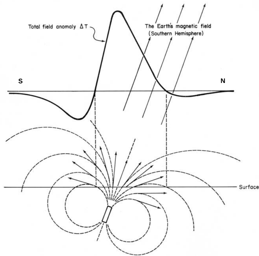
Figure 4.1 – South-North schematic profile of a magnetic anomaly over a magnetic dyke with a dipolar field. The dyke is striking E-W, and situated in the southern hemisphere (Roux, 1980).
