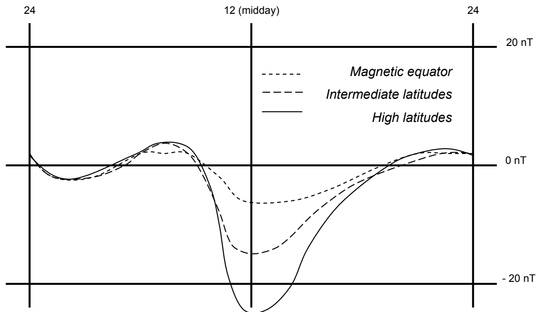
Figure 4.4 – Schematic diurnal variation, showing the vertical component of the magnetic field through a 24 hour period at varying magnetic latitudes (Roux, 1980).
