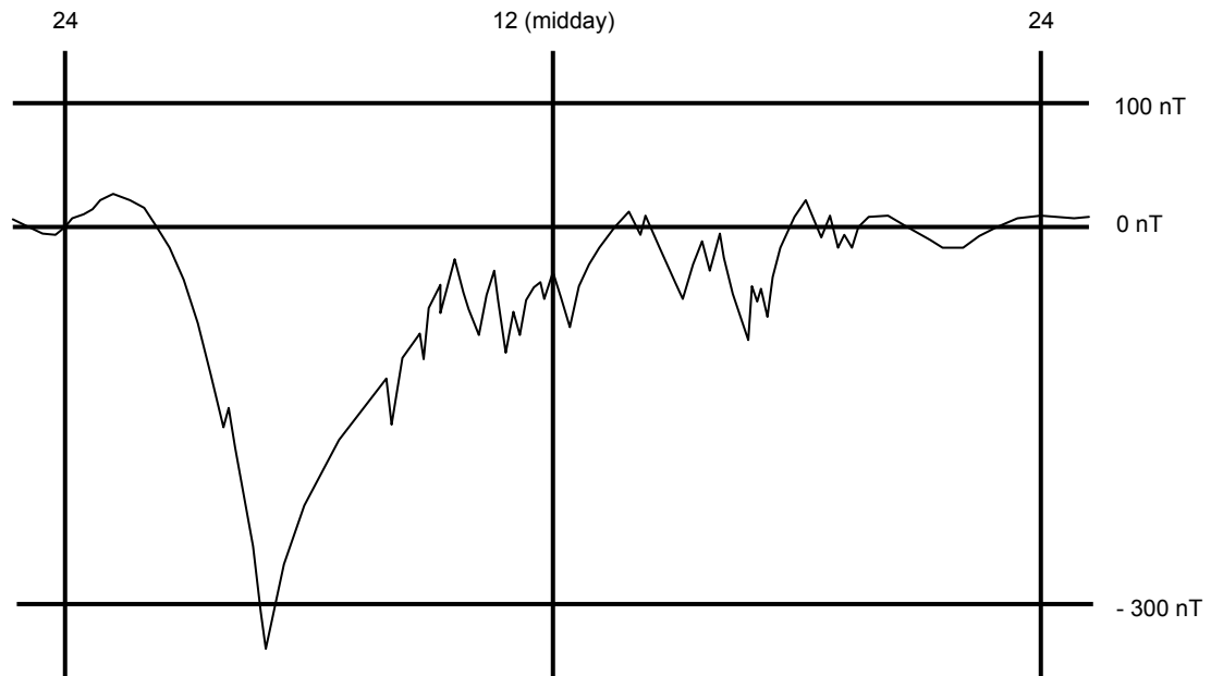
Figure 4.5 – Schematic magnetic storm, showing the vertical component of the magnetic field. Note the erratic nature of the field and the change in scale from Figure 4.4.
