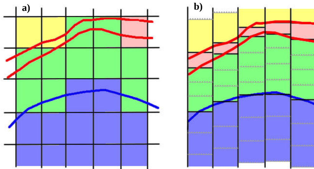
Figure 7.6 – Comparing geometry variation methods for two sets of similar geological units (lithological boundaries represented by red and blue lines). a) Conventional fixed mesh (black lines), with invariable horizontal cell divisions and cells assigned according to the lithology occupying the greatest percentage of the cell. b) Adaptive mesh with variable horizontal cell divisions (solid horizontal lines) and sub-cells (dotted horizontal lines), after Fullagar and Pears (2007). Note how the adaptive mesh represents the geology more closely.
