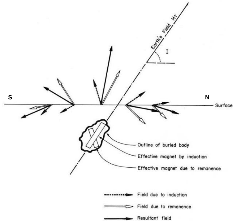
Figure 4.2 – The effect of remanence on S-N profile: the induced magnetization vector and remanent magnetization vector combine to produce a resultant vector, commonly different to the present-day field (Roux, 1980).
