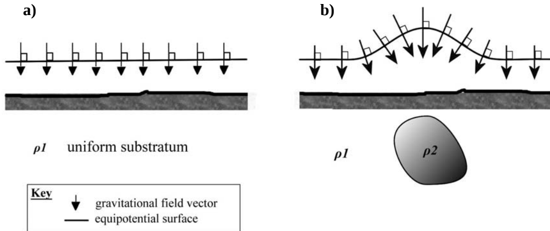
Figure 2.1 – Equipotential surfaces caused by different substratum. (a) Uniform substratum causes equal gravitational field vectors across the equipotential surface. (b) An ore body of arbitrary shape and with density greater than the substratum (i.e. \rho_2 > \rho_1 ) results in a mass excess causing unequal field lines across an up-warped equipotential surface (after Corner, 1993).
