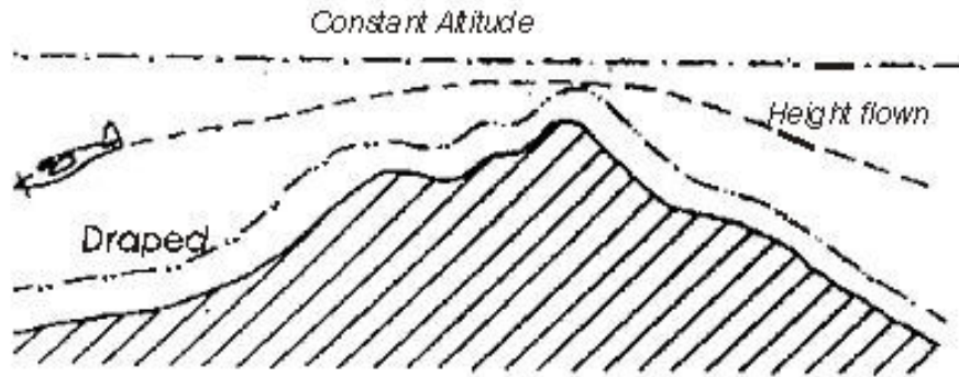
Figure 3.5 – Comparing surveys flown at a constant height or draped, as well as the actual height flown for a draped survey in regions of steep topography (Syberg, 1972).
