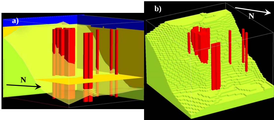
Figure 8.7 – a) 3D voxel of the starting model, with the transparent Transvaal Supergroup contact and cross-sections showing the prisms defining the geophysical units: air (blue), Bushveld Complex (orange), Transvaal Supergroup (lime) and IRUPs (red). b) 3D voxel model showing the discretized 200 x 200 m prisms of the Transvaal Supergroup (lime) and IRUPs (red). Vertical Exaggeration: 3.
