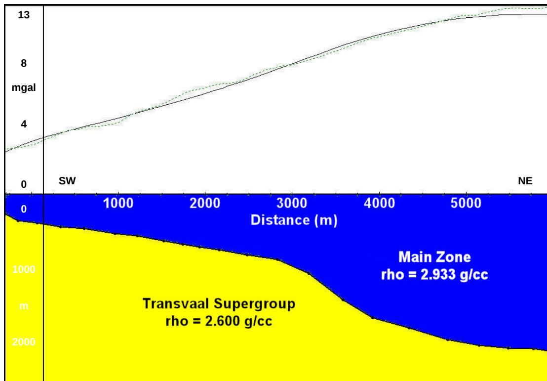
Figure 8.1 – 2.5D gravity model of Line 1, with measured data (green line) and calculated data (black line). Inversions produced a density contrast of 0.333 \text{ g.cm}^{-3} .
