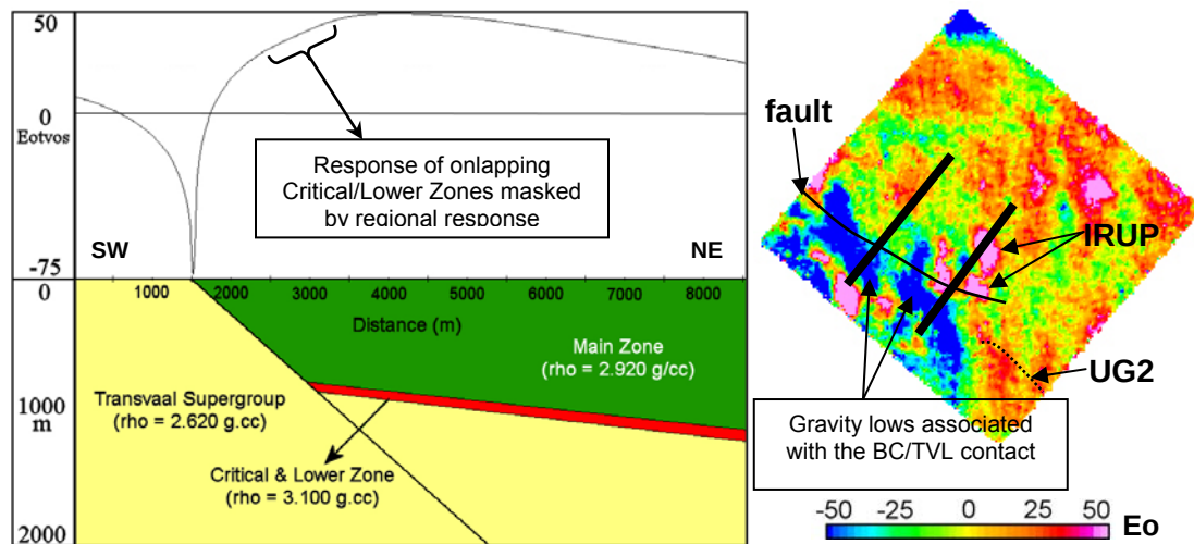
Figure 9.4 – (left) Synthetic 2D T_{zz} response from a Bushveld Complex onlapping the Transvaal Supergroup (after Antoine (2004)) using Grav2DC (Cooper, 2003) and SignProc (Cooper, 2000), (right) Gridded T_{zz} map over the study area, showing the response across a similar geological scenario (black lines), from AGG data.
