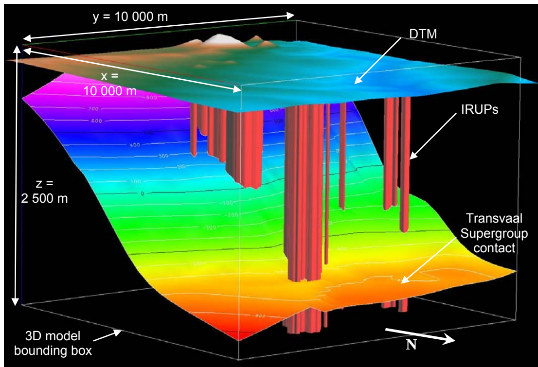
Figure 8.6 – 3D geological starting model of the study region, showing topographic surface (i.e. surface separating air from the Bushveld Complex and Transvaal Supergroup), IRUPs, and Transvaal Supergroup contact. Dimensions of the bounding box are shown and apply to all subsequent images of the regional model. Vertical exaggeration: 3.
