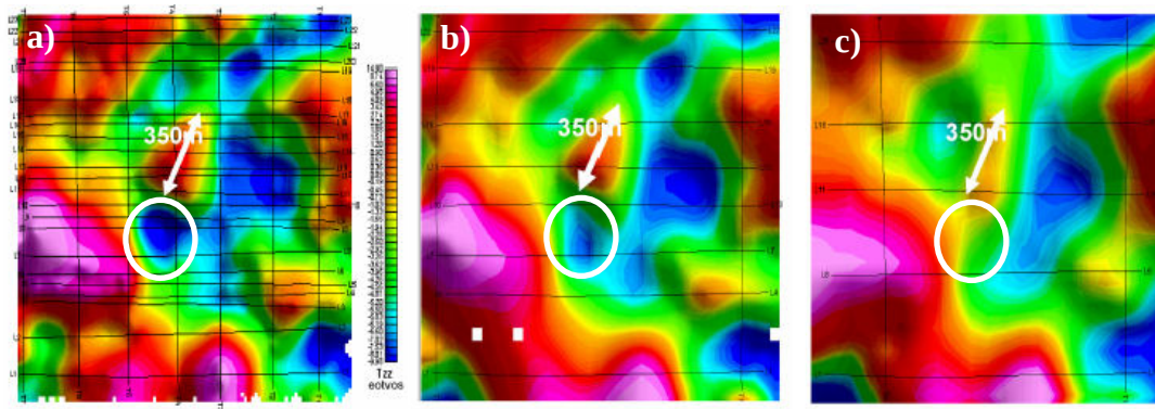
Figure 3.6 – The effect of line-spacing on T_{zz} data, where lines have been removed from an original survey. a) Original survey using 50 m line-spacing, b) simulated survey using 150 m line-spacing, and c) simulated survey using 250 m line-spacing. The target anomaly (length: 350 m) is still resolved in b) but already shows aliasing in c). The negative anomaly (circled) all but disappears in c), (Murphy, 2004).
