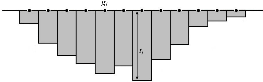
Figure 7.4 – Cross-section model of a sedimentary basin. Basin is approximated by rectangular blocks, extending infinitely perpendicular to the profile and with one block per gravity station (Bott, 1960).
