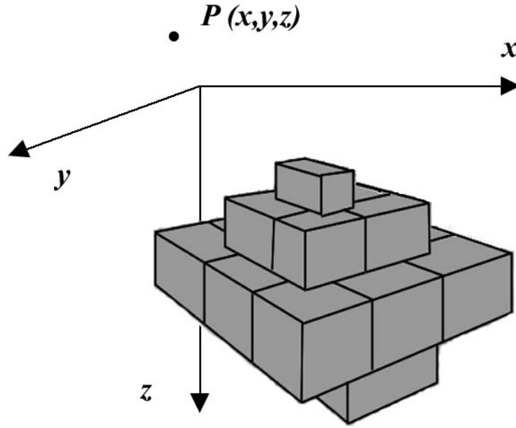
Figure 7.3 – Schematic diagram of a 3D approximation of a body, using rectangular prisms (Blakely, 1995).
