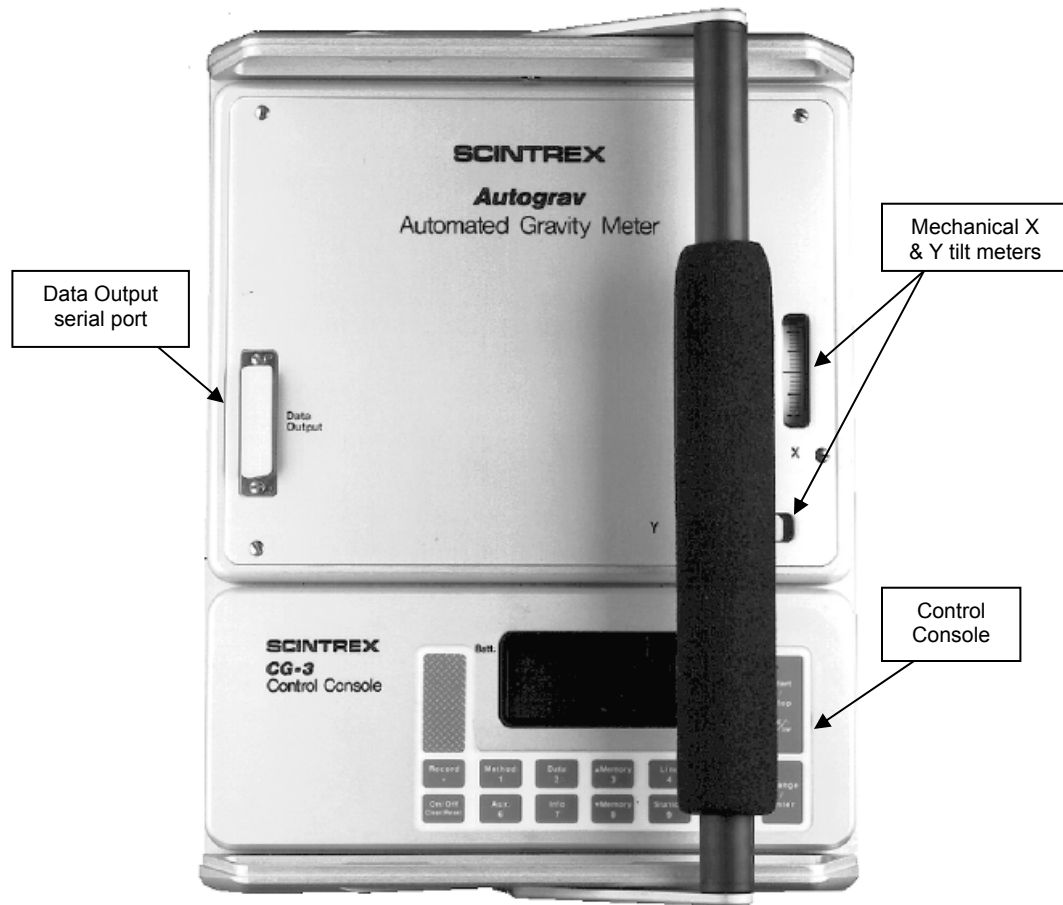
Figure 2.2 – Overhead view of the Scintrex Autograv CG-3, showing Control Console, Mechanical Tilt Meters (X and Y axis) and Data Output serial port (Scintrex, 1995).
