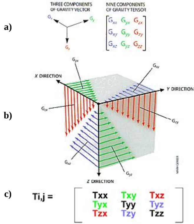
Figure 3.1 – a) Schematic co-ordinate system showing the three principle components of the gravity field ( G_x – blue, G_y – green, G_z – red), with derivatives in the x , y and z direction of each component creating the nine components of the gravity tensor. b) The components of the FTG gravity field, which describe the rate of change of the gravity vector as one moves in the direction of the vector. c) The FTG matrix, T_{ij} , showing the components which are equal (i.e. T_{xy} = T_{yx} , T_{xz} = T_{zx} , and T_{yz} = T_{zy} ), hence one of each of these components can be considered redundant (Bell Geospace, 2006).
