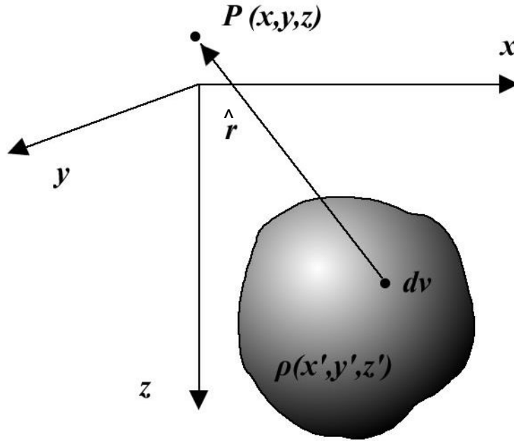
Figure 7.2 – Arbitrary 3D body with density \rho(x', y', z') and unit vector \hat{\mathbf{r}} pointing from an element of the body to the calculation point P(x, y, z) , (Blakely, 1995).
