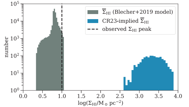
Figure 3. Implied mean H I mass surface density, \Sigma_{\text{H I}} (grey), within r_{\text{disc}} for all Monte Carlo realizations using the Blecher et al. (2019) source model. The black dashed vertical line indicates the typical peak H I mass surface density measured in the local Universe with sub-kpc spatial resolution (e.g. Bigiel et al. 2008). In blue, we show the implied \Sigma_{\text{H I}} distribution, if one assumes the quoted CR23 H I flux density and only considers those realizations with magnifications \mu > 23 (i.e. within one standard deviation of their quoted magnification). This demonstrates that the CR23 implementation of the Blecher et al. (2019) model and claimed H I detection cannot both be correct.
