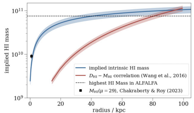
Figure 5. Implied intrinsic H I mass and quoted uncertainty (blue curve and shading) based on the reported CR23 apparent H I mass (i.e. claimed intrinsic mass multiplied by their magnification of 29) and the implementation of the Shu et al. (2017) lens model in this work. The red curve and shading correspond to the M_{\text{H I}}-D_{\text{H I}} relation (Wang et al. 2016) and scatter (which the Blecher et al. 2019 method enforces). These two curves only intersect at a radius r > 90 kpc, corresponding to magnifications \mu < 3 and M_{\text{H I}} larger than the highest H I masses recorded in the ALFALFA survey (dashed horizontal line; Jones et al. 2018). The CR23 H I mass and magnification are indicated by the black square.
