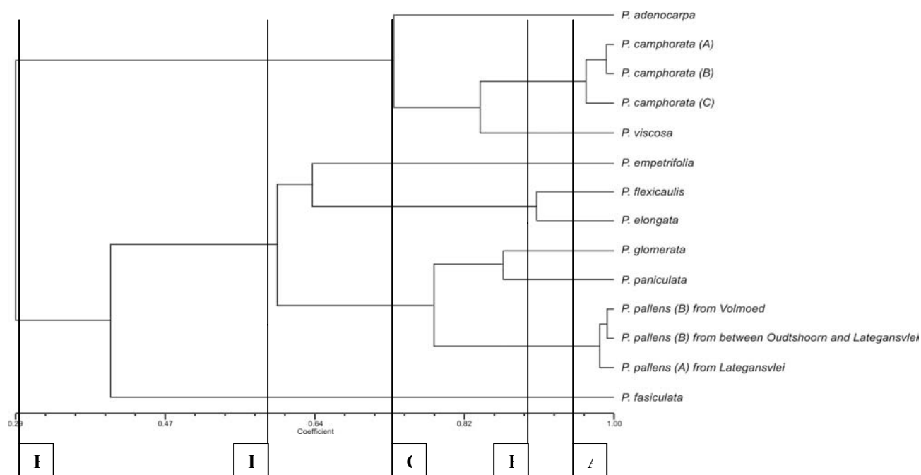
Figure 9: Cluster analysis of essential oil composition.
