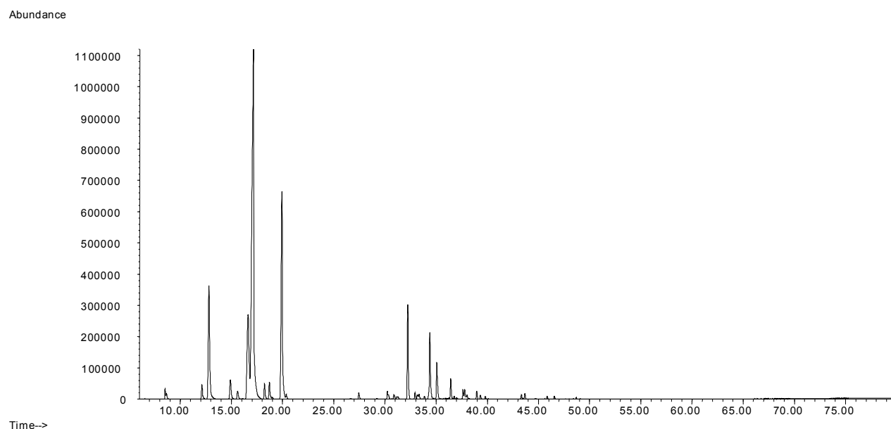
Figure 17: Total ion chromatogram of the hydrodistilled essential oil from P. camphorata var. camphorata (individual A).
