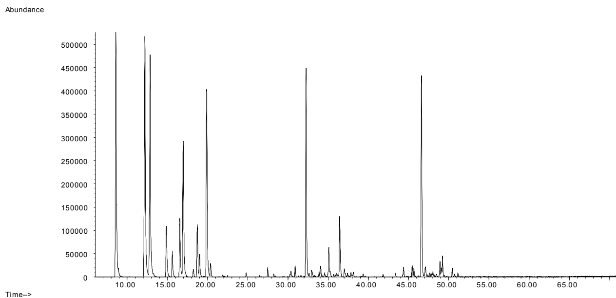
Figure 34: Total ion chromatogram of the hydrodistilled essential oil from P. glomerata .
