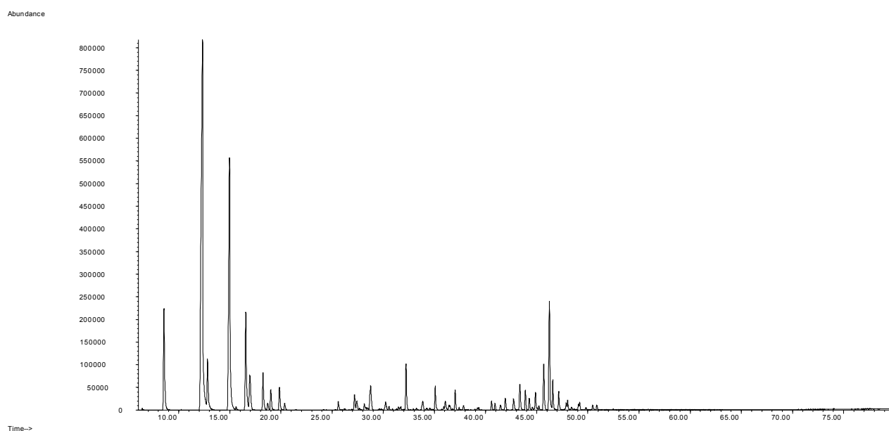
Figure 32: Total ion chromatogram of the hydrodistilled essential oil from P. flexicaulis .
