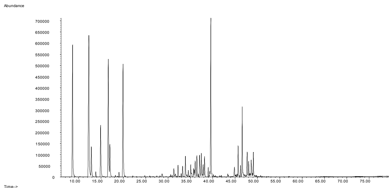
Figure 25: Total ion chromatogram of the hydrodistilled essential oil from P. empetrifolia .
