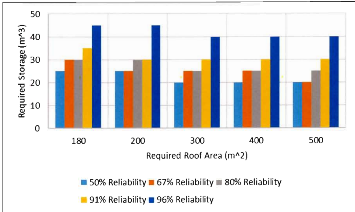
Figure 6.5: Storage-roof area-reliability relationship for Homestead 1 when the required demand is maximized (thus 25 l/d/capita over 365 days of supply in a year).
