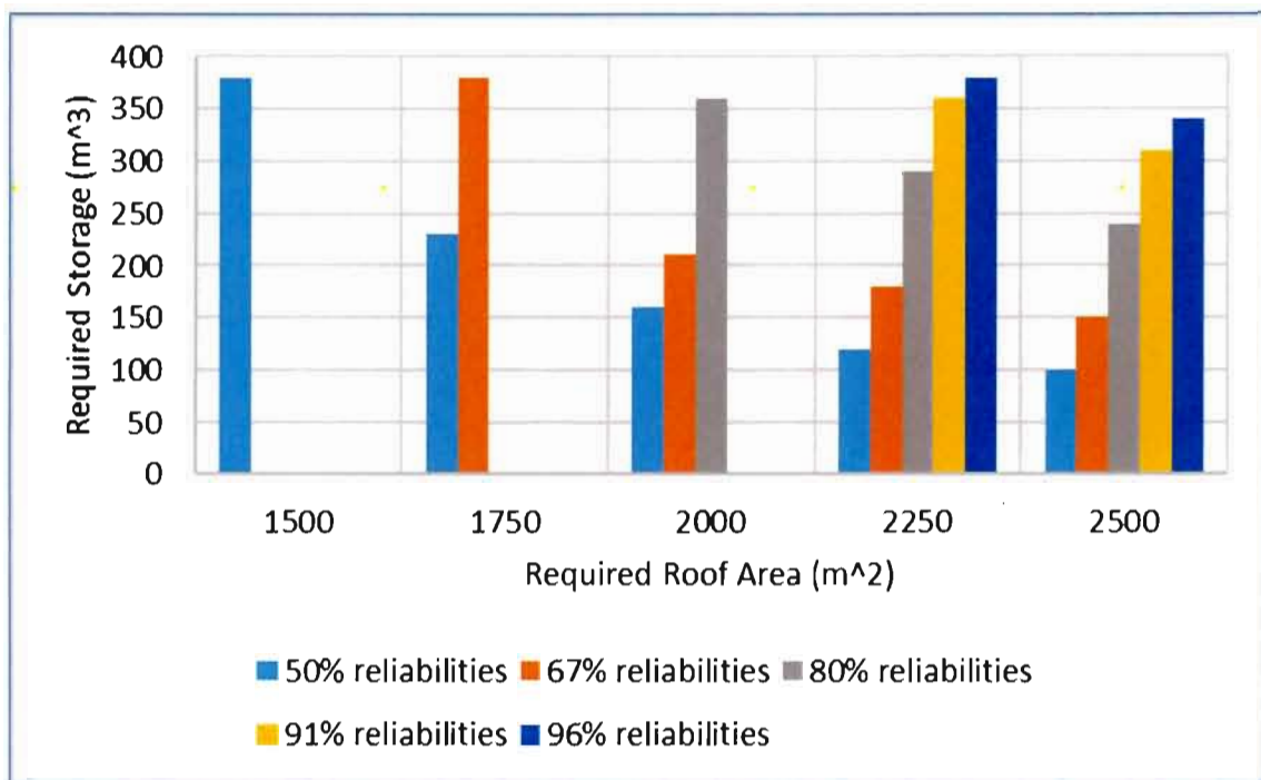
Figure 6.17: Storage-roof area-reliability relationship for the school when the required demand is maximized (thus 5 l/d/capita over 250 days of supply in a year).
