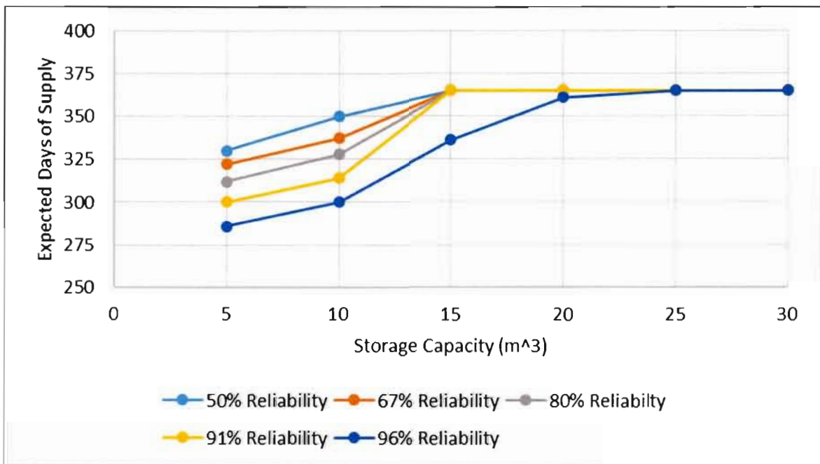
Figure 6.7: Storage-yield-reliability relationship for Homestead 2 based on measured consumption (13 l/d/capita applied variably).
