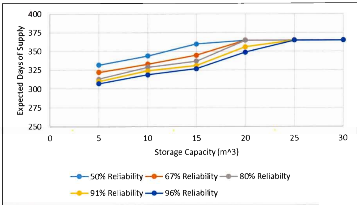
Figure 6.2: Storage-yield-reliability relationship for Homestead 1 based on measured consumption (14.4 l/d/capita applied variably).
