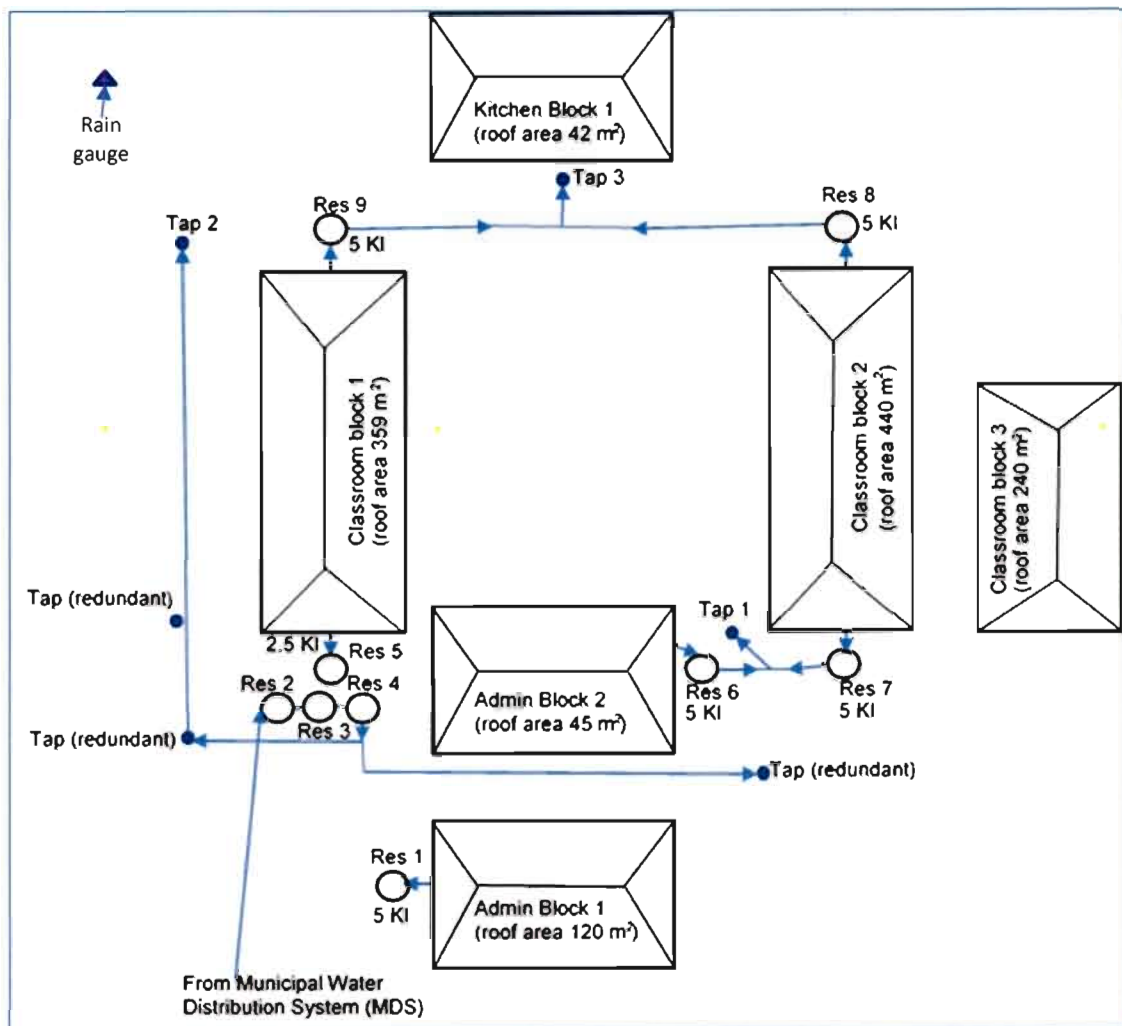
Figure 4.7: Schematic layout for the school's water supply and distribution.
