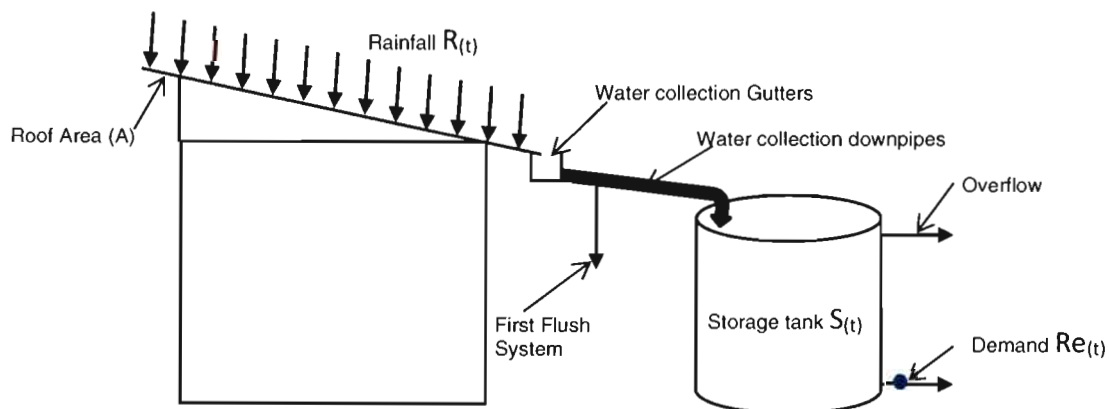
Figure 3.1: Typical Rainwater Harvesting system
