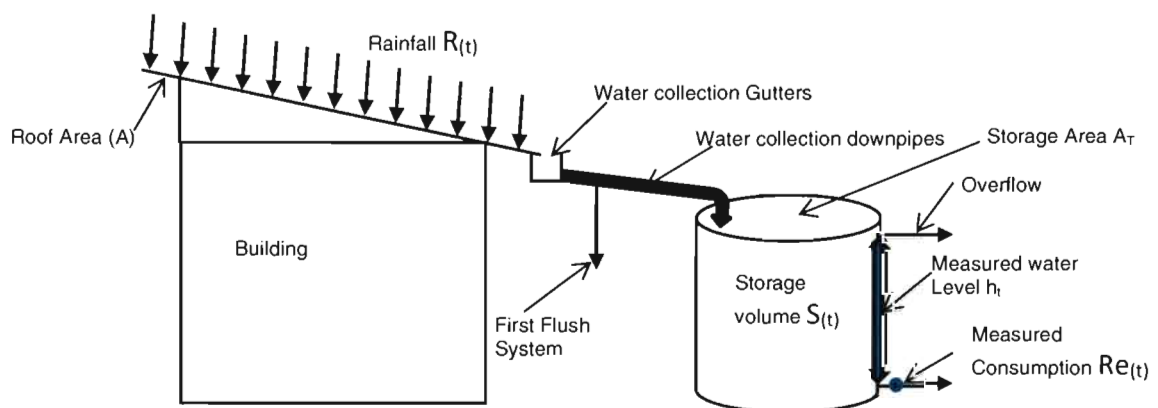
Figure 4.1: Typical RWH system in the identified water users
