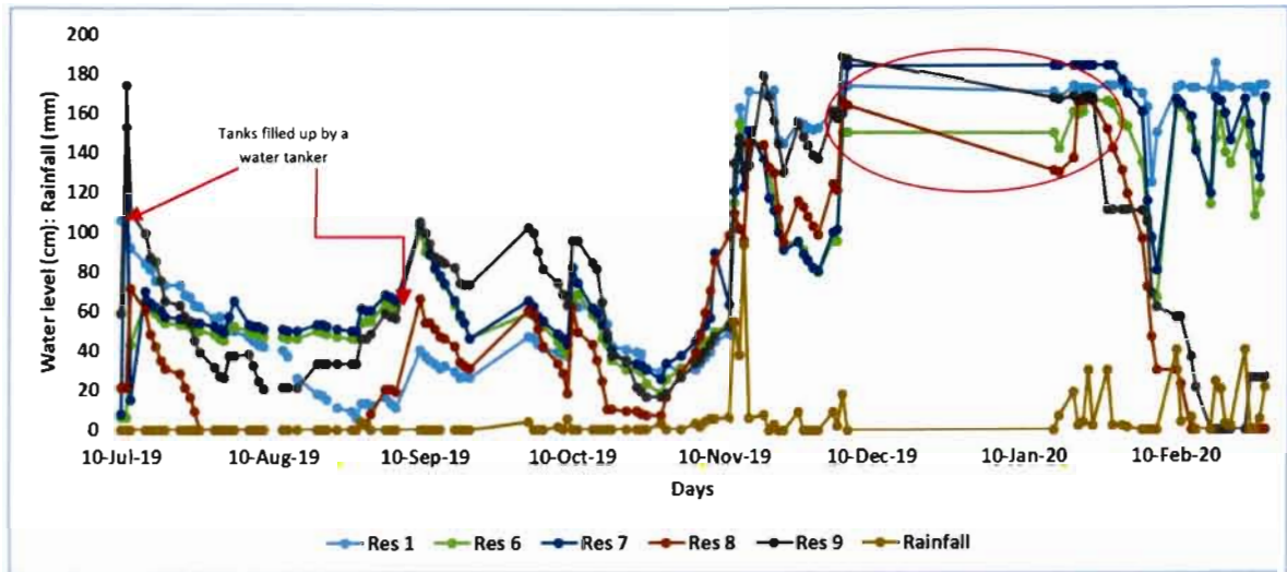
Figure 5.11: Reservoir storage water levels and rainfall for the School.
