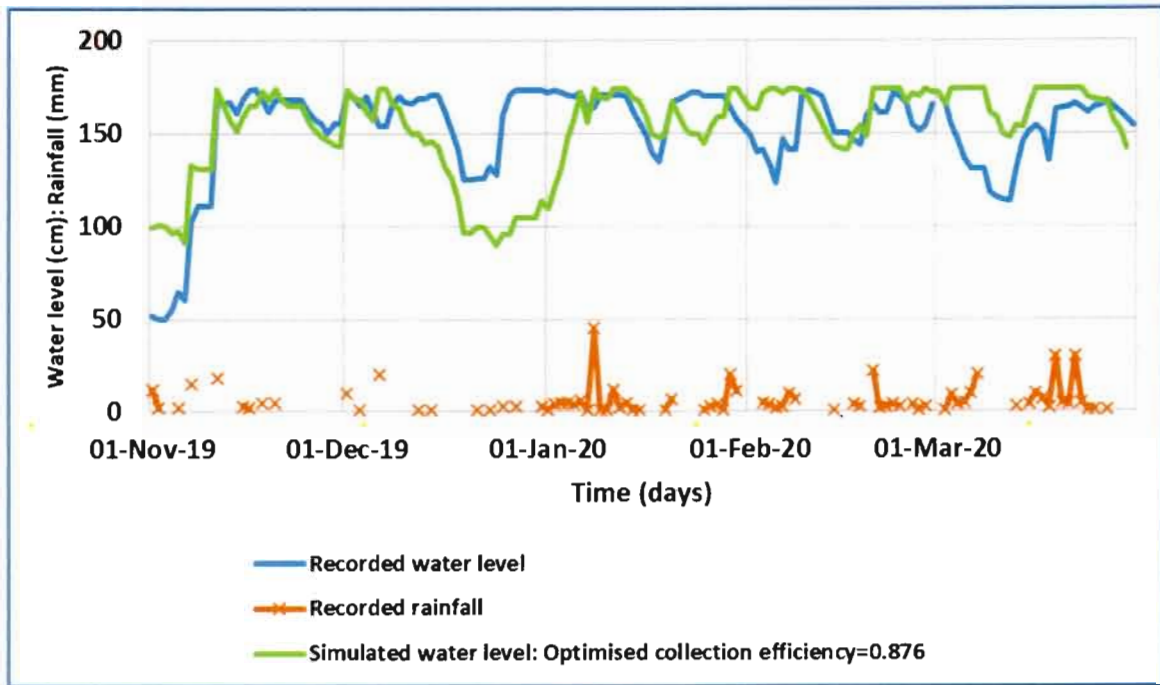
Figure 5.19: Recorded and simulated storage water level trajectories for the optimal rainwater collection efficiency for reservoir 3 of the Clinic.
