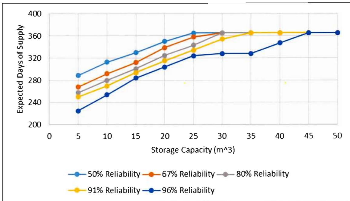
Figure 6.8: Storage-yield-reliability relationship for Homestead 2 based on required demand (25 l/d/capita applied constantly).
