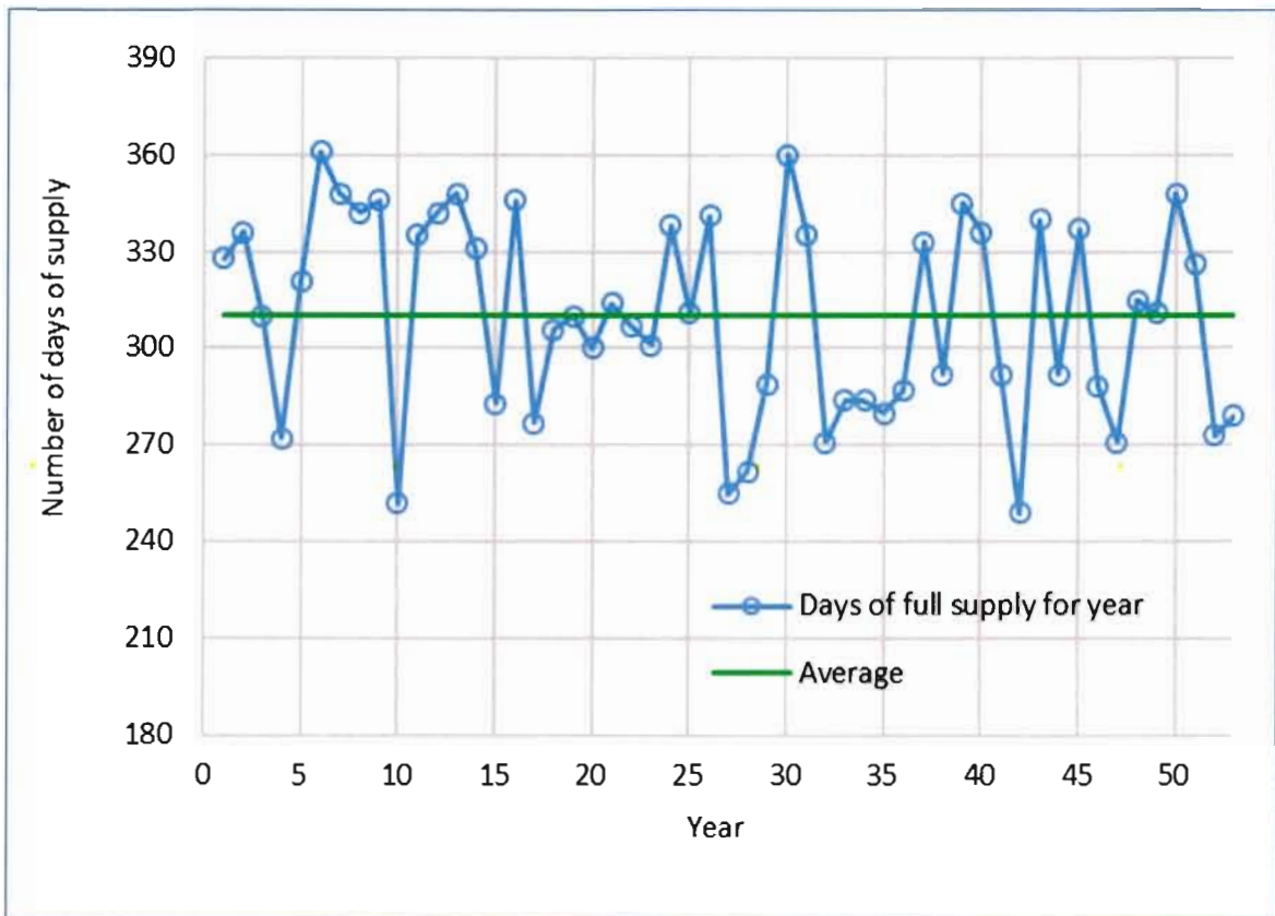
Figure 4.13: Time series of annual number of days of supply for a storage of 10m³ for household 1
