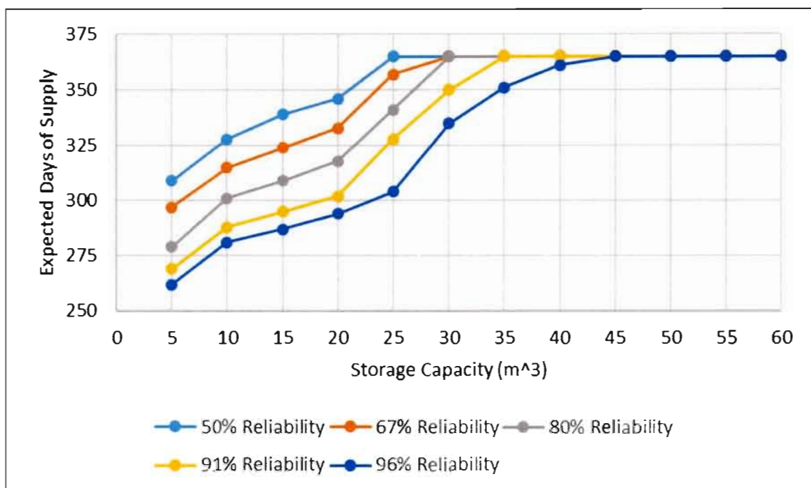
Figure 6.9: Storage-yield-reliability relationship for Homestead 2 based on required demand (25 l/d/capita applied variably).
