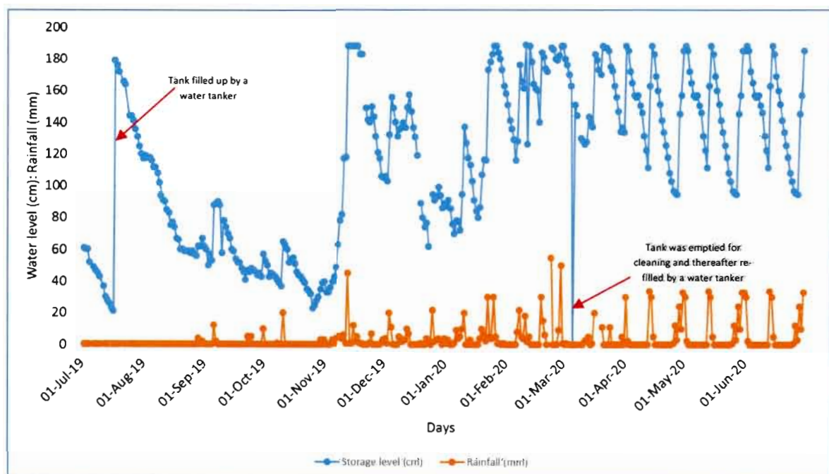
Figure 5.8: Reservoir storage water levels and rainfall for Homestead 1.
