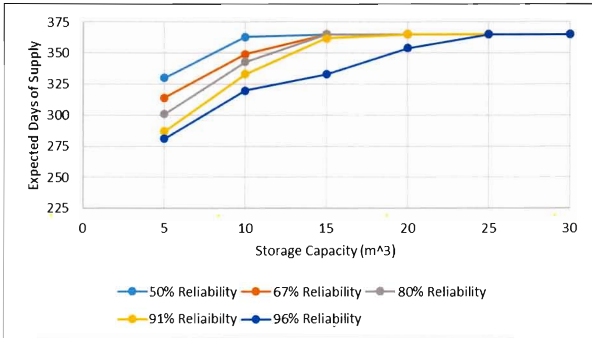
Figure 6.6: Storage-yield-reliability relationship for Homestead 2 based on measured consumption (13 l/d/capita applied constantly).
