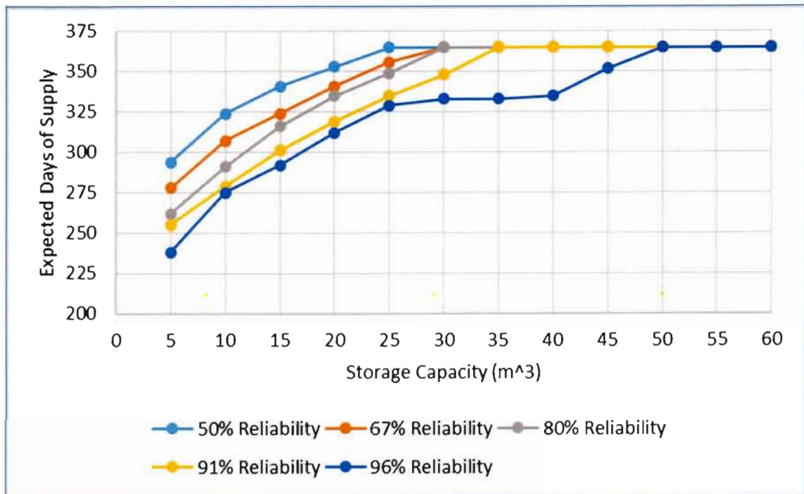
Figure 6.11: Storage-yield-reliability relationship for the Clinic based on measured consumption (4.3 l/d/capita applied constantly).
