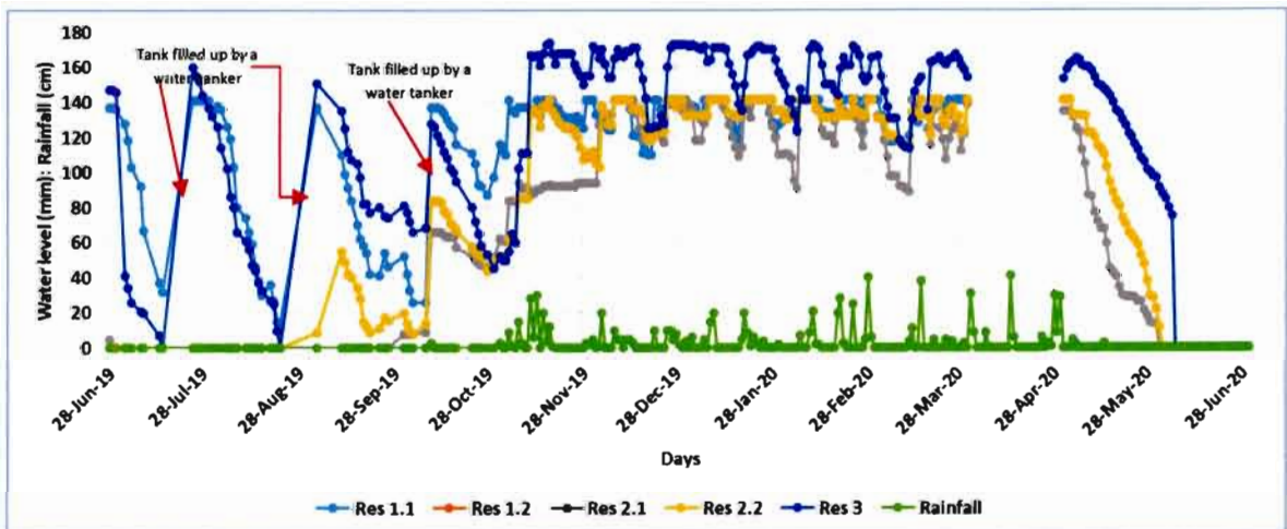
Figure 5.10: Reservoir storage water levels and rainfall for the Clinic
