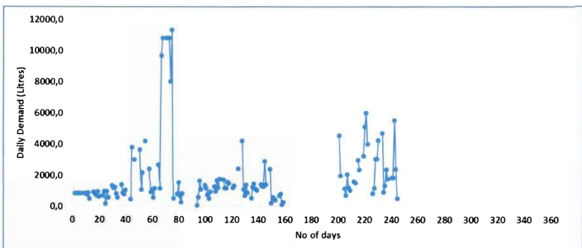
Figure 5.7: Daily water consumption at the school.
