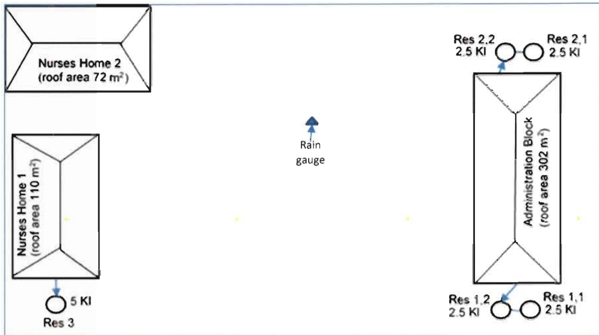
Figure 4.9: Schematic layout of RWH at the Clinic
