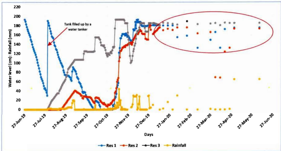
Figure 5.9: Reservoir storage water levels and rainfall for Homestead 2.
