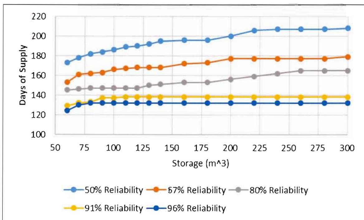
Figure 6.16: Storage-yield-reliability relationship for the school based on required demand (5 l/d/capita applied constantly).
