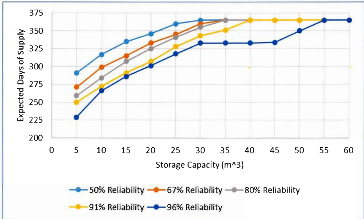
Figure 6.13: Storage-yield-reliability relationship for the Clinic based on required demand (5 l/d/capita applied constantly).
