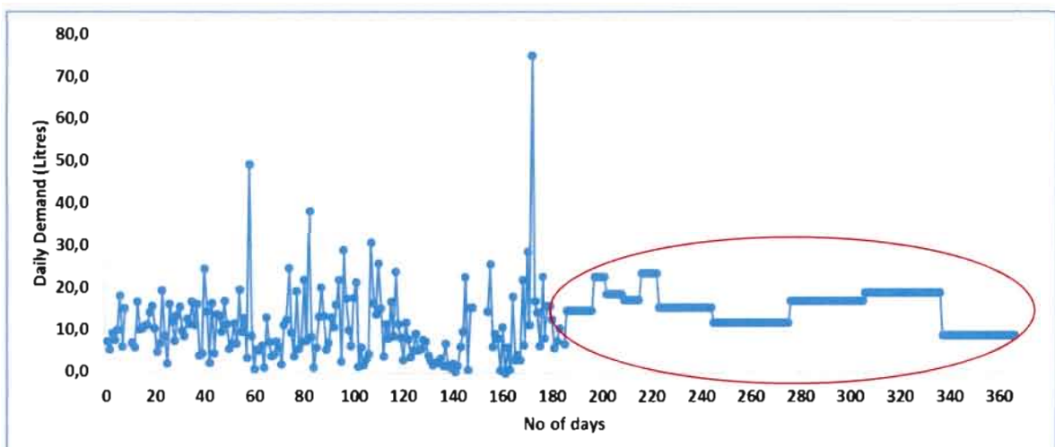
Figure 5.3: Daily water consumption in Homestead 2.
