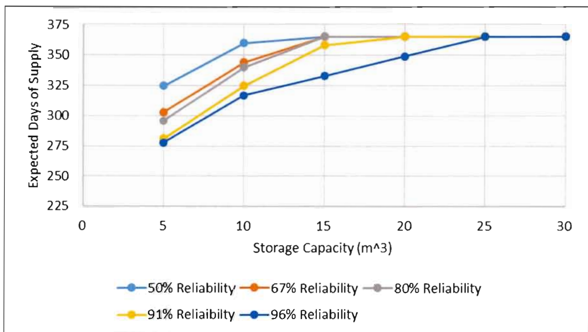
Figure 6.1: Storage-yield-reliability relationship for Household 1 based on measured consumption ( 14.4\text{ l/d/capita} applied constantly).
