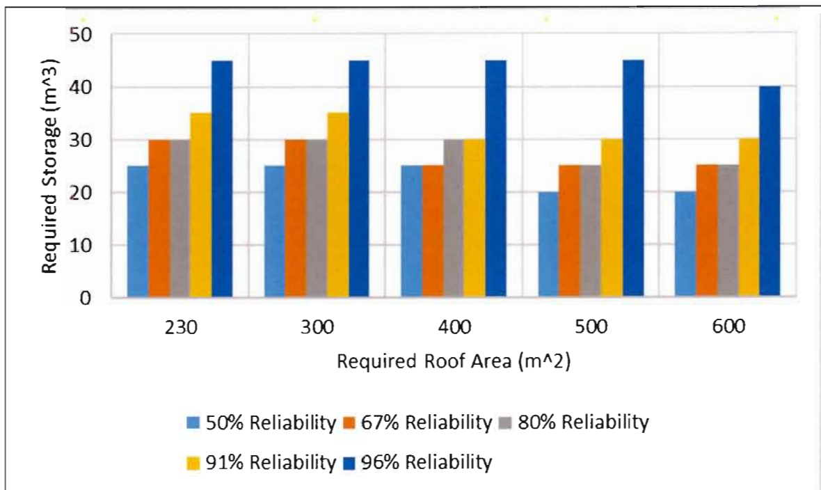
Figure 6.10: Storage-roof area-reliability relationship for Homestead 2 when the required demand is maximized (thus 25 l/d/capita over 365 days of supply in a year).
