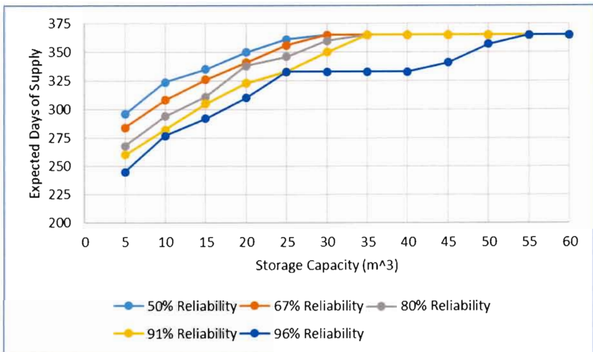
Figure 6.12: Storage-yield-reliability relationship for the clinic based on measured consumption (4.3 l/d/capita applied variably).
