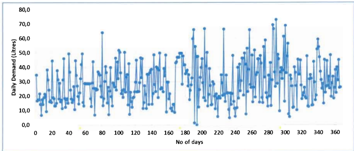
Figure 5.4: Daily water consumption in Homestead 3.
