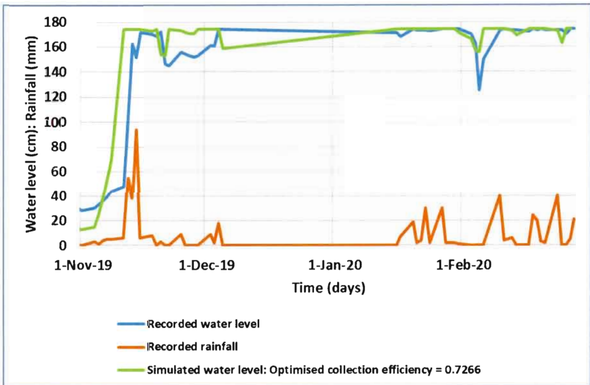
Figure 5.20: Recorded and simulated storage water level trajectories for the optimal rainwater collection efficiency for reservoir 1 of the School.
