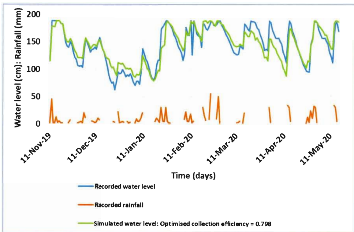
Figure 5.18: Recorded and simulated storage water level trajectories for the optimal rainwater collection efficiency for reservoir 1 of Household 1.
