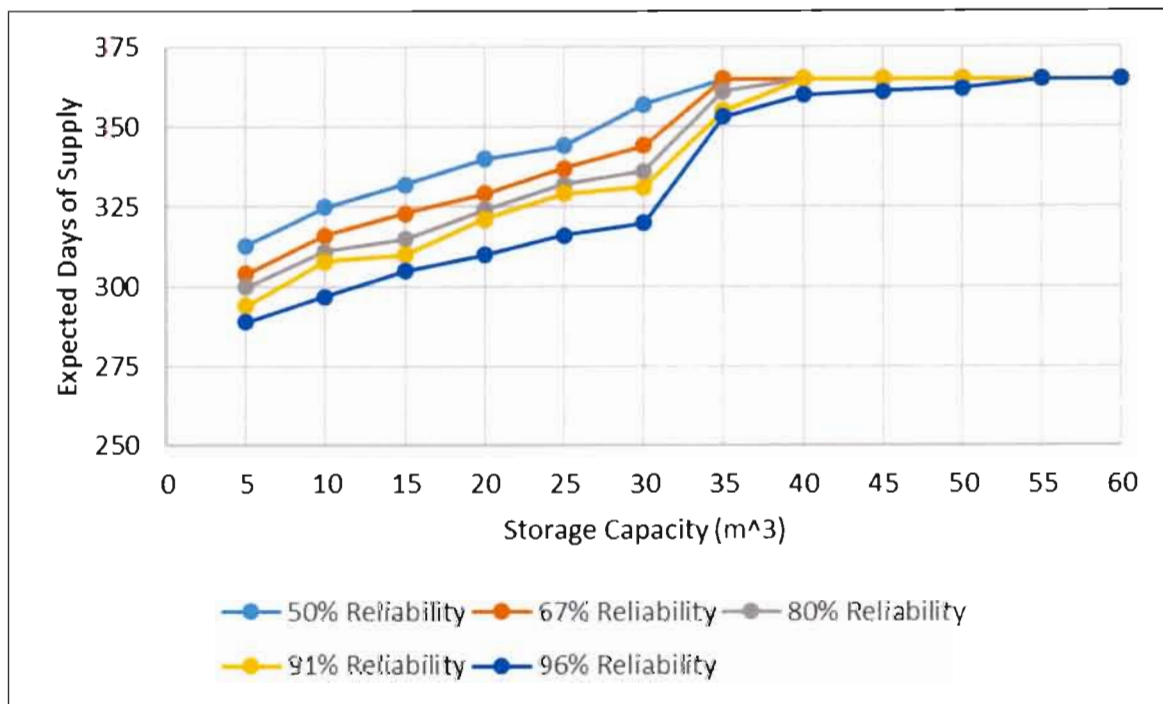
Figure 6.4: Storage-yield-reliability relationship for Homestead 1 based on required demand (25 l/d/capita applied variably)
