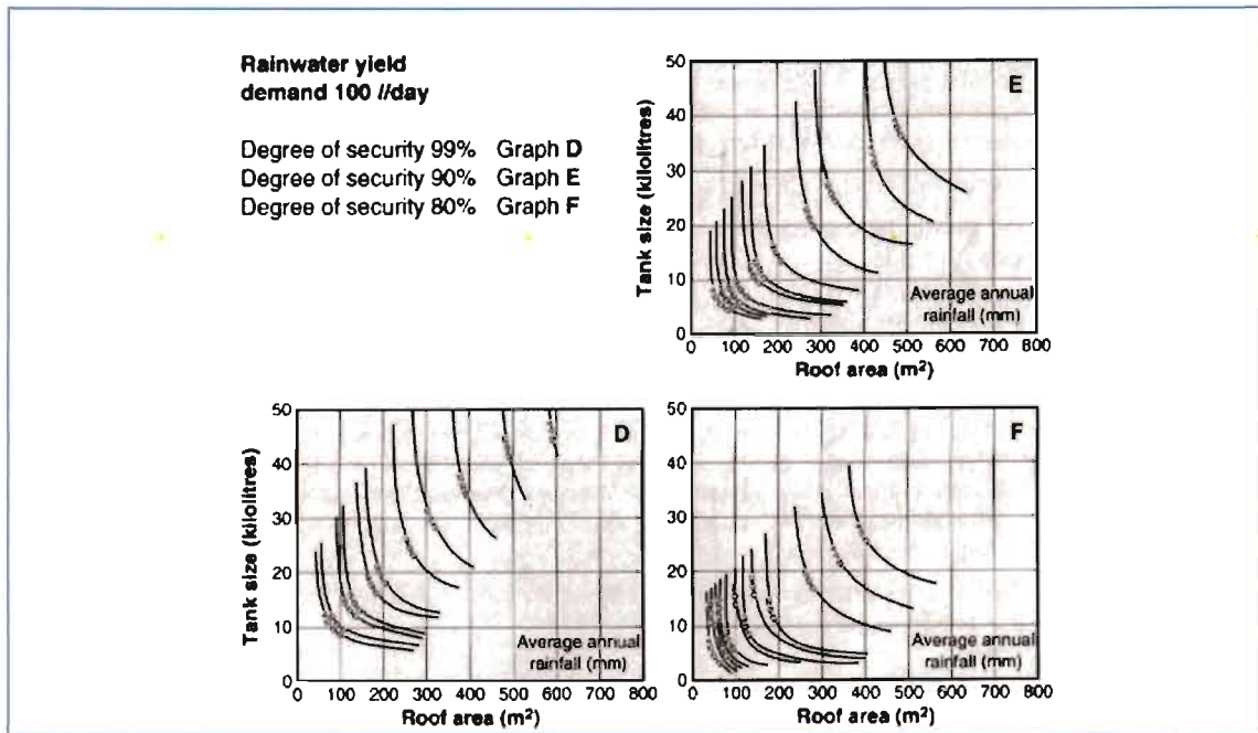
Figure 3 3: Simplified approach to sizing RWH systems using average annual rainfall Basinger et al., (2010)
