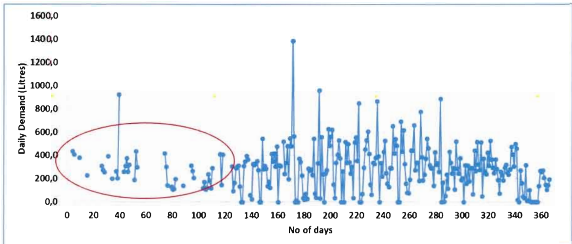
Figure 5.6: Measured daily water consumption at the Clinic.
