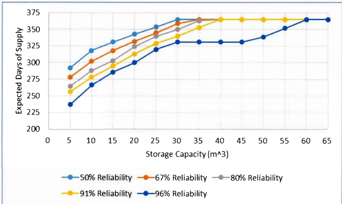
Figure 6.14: Storage-yield-reliability relationship for the Clinic based on required demand (5 l/d/capita applied variably).
