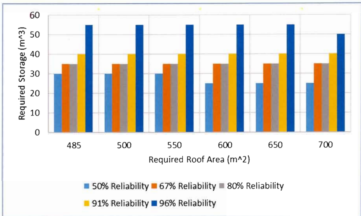
Figure 6.15: Storage-roof area-reliability relationship for the Clinic when the required demand is constantly maximized (thus 5 l/d/capita over 365 days of supply in a year).
