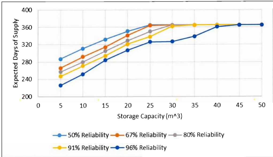
Figure 6.3: Storage-yield-reliability relationship for Homestead 1 based on required demand (25 l/d/capita applied constantly).
