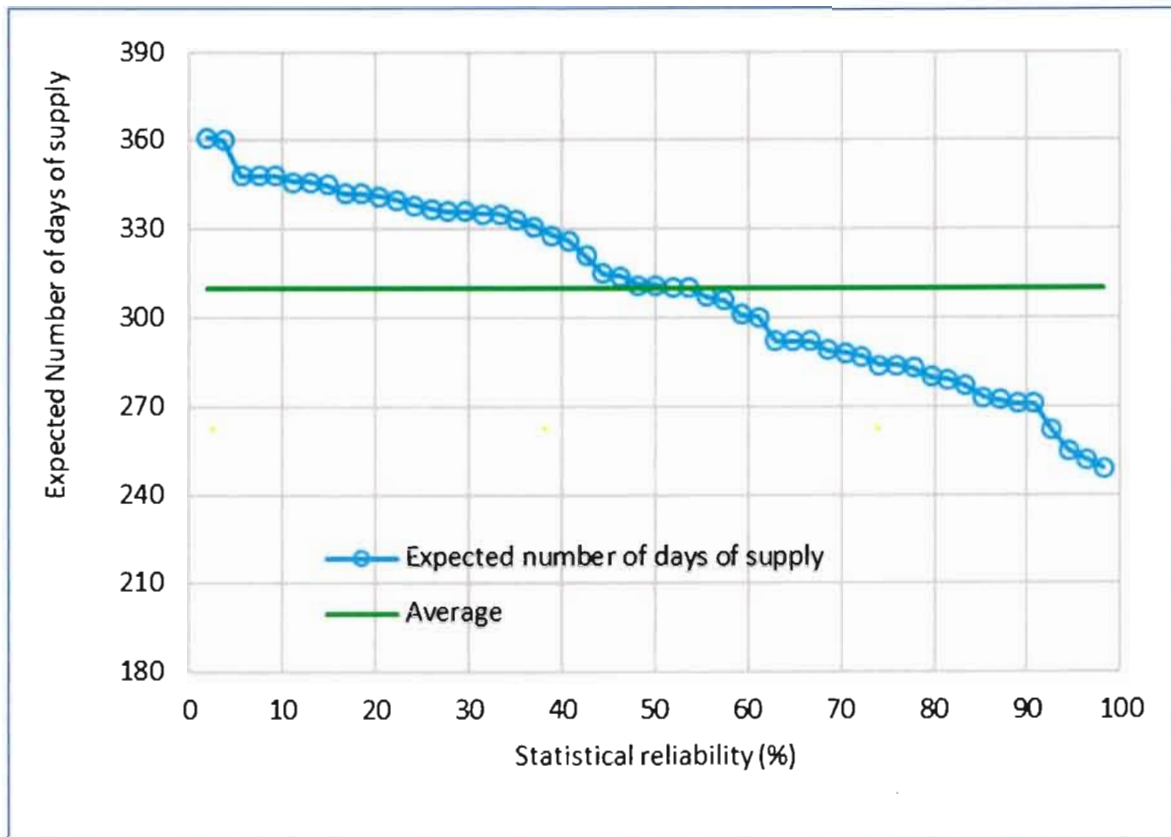
Figure 4.14: Relationship between statistical reliability and level of supply for a storage of 10m 3 for household 1.
