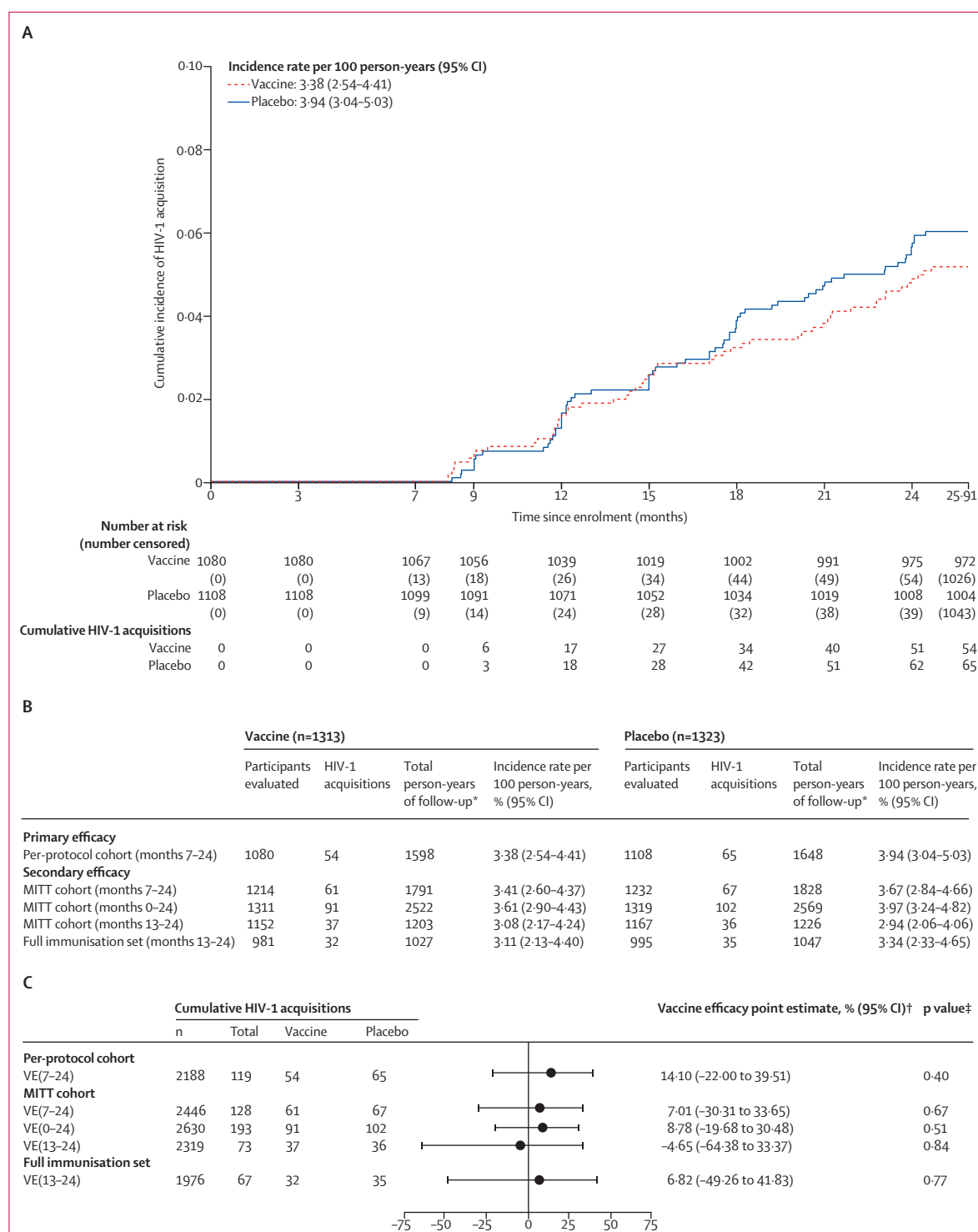
Figure 3: Vaccine efficacy
