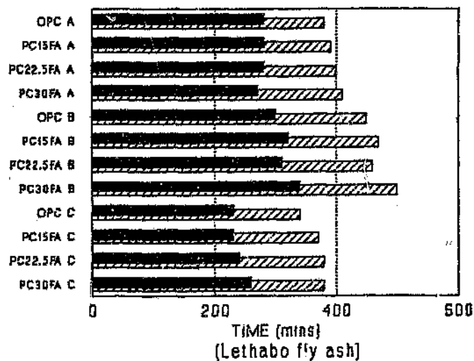
Figure 5.17a Initial and final setting times for equivalent 28 day mixes (hot curing)
