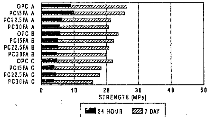
Figure 7.3b Compressive strength Standard cured direct replacement mixes
