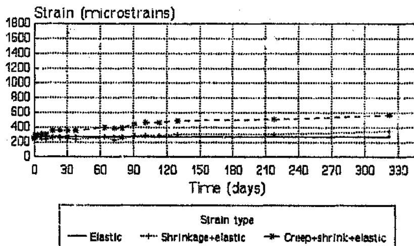
Figure 8.6c Creep, shrinkage and elastic deformation of PC30FA mix (13 mm stone, sealed)
