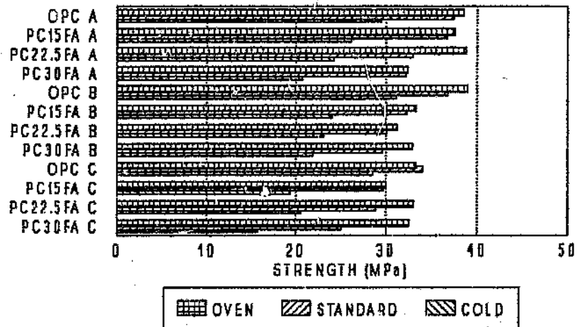
Figure 7.5h 28 Day Compressive strength DR cured at different temperatures
