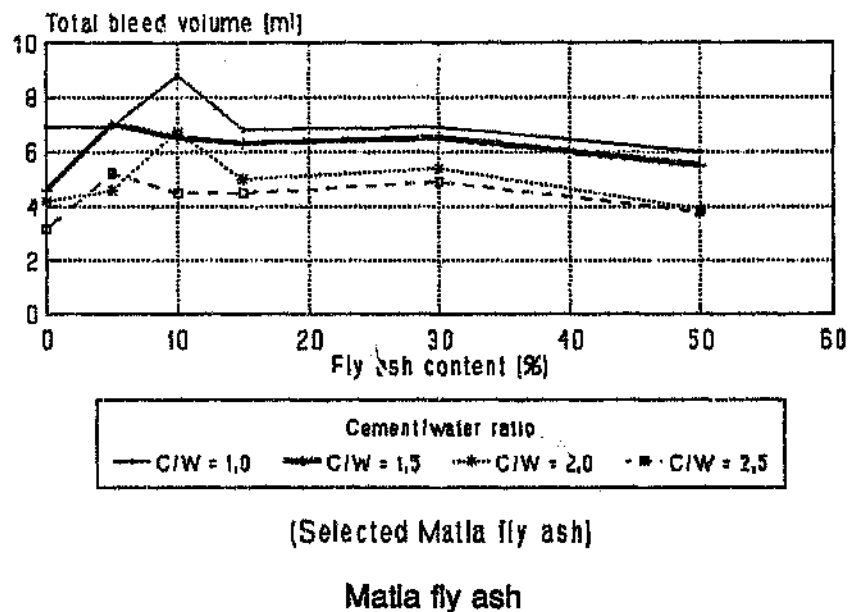
Figure 5.18f Bleed volume of mortar mixes with and without fly ash
