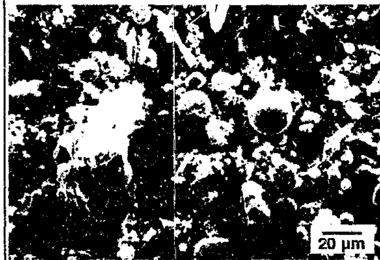
Figure 4.5 Photomicrograph of Duvha fly ash
