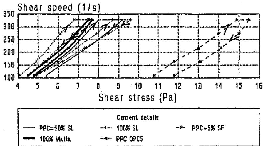
Figure 5.9b Viscous behaviour of other cementitious materials (c/w=1.67)
