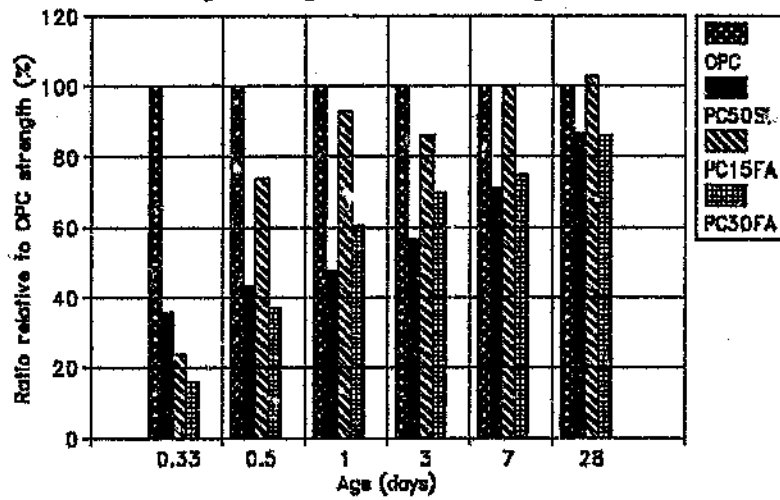
Figure 7.5d Age strength ratio at 30 degrees
