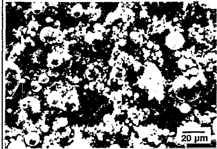
Figure 4.4 Photomicrograph of Matla fly ash
