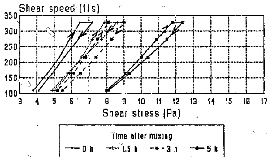
Figure 5.10b Change of viscosity with time for PPC OPC + 15% Matla at c/w = 1.67
