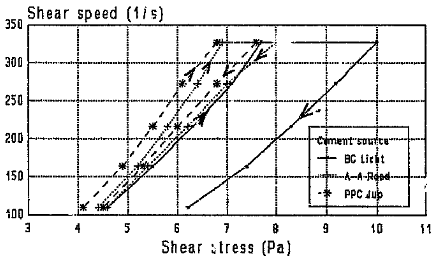
Figure 5.3b Viscous behaviour of OPC's Cement/water ratio = 1.67
