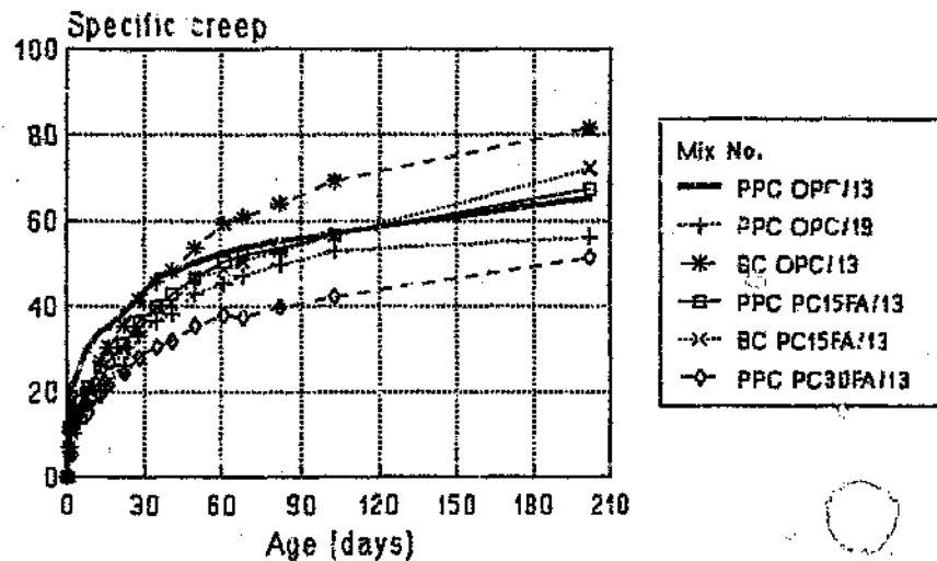
Figure 8.5 Specific creep : Series I for opc and fly ash mixes
