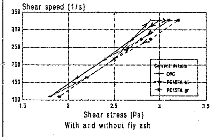
Figure 5.7a Viscous behaviour of PPC blends Cement/water ratio = 1.3
