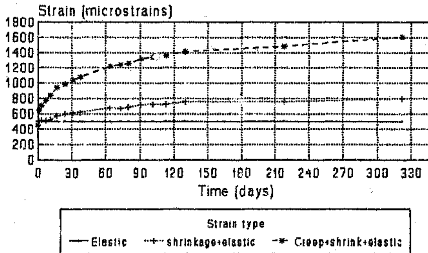
Figure 8.6d Creep, shrinkage and elastic deformation of PC30FA mix (13 mm stone, unsealed)
