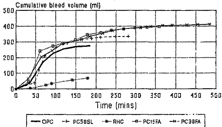
Figure 5.20 Bleeding of mortars made with different cementitious materials
