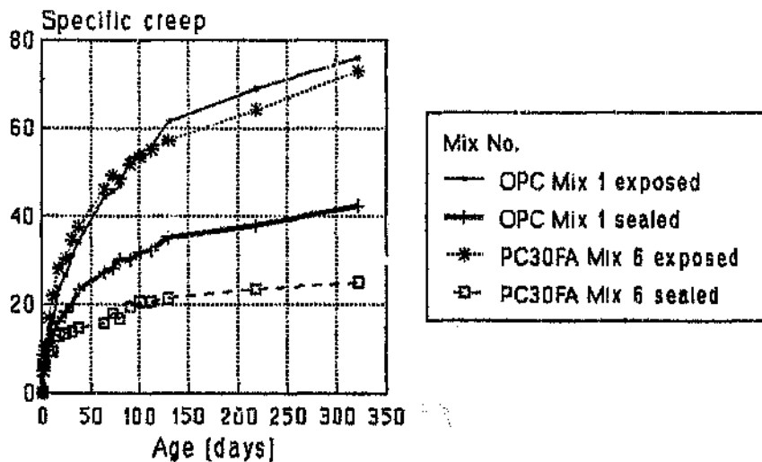
Figure 8.7 Specific creep : Series II for opc, fa mixes (sealed and exposed)
