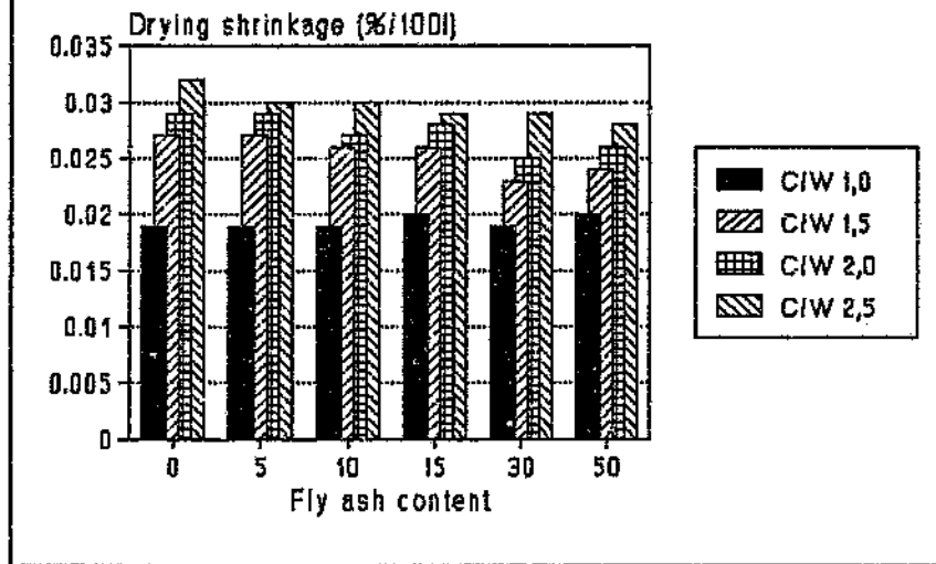
Figure 8.3b Proportion of drying shrinkage to water content of mortars with/out fly ash
