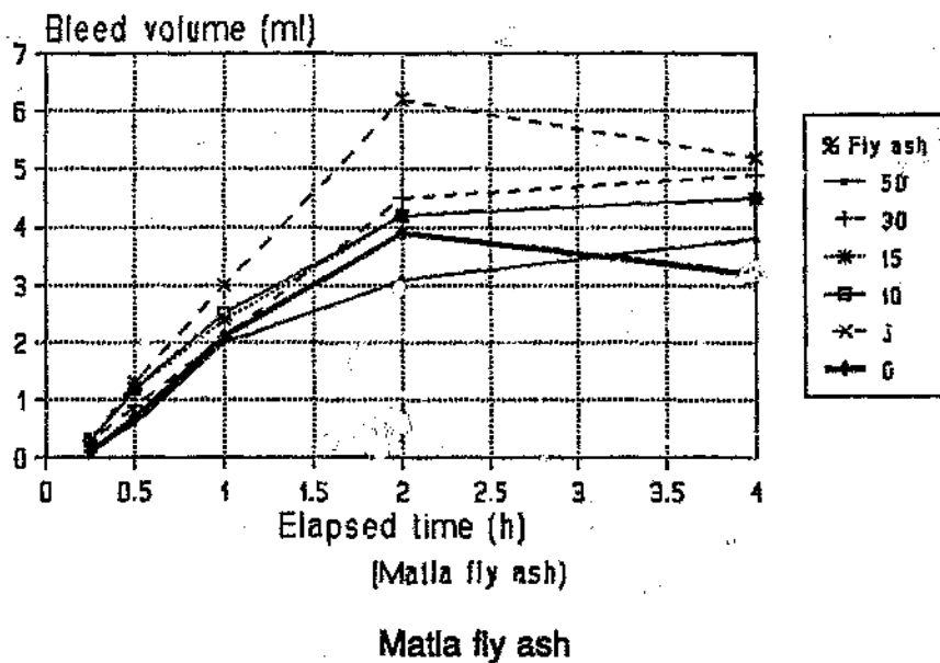
Figure 5.18d Bleed volume at c/w = 2.5 For varying fly ash contents
