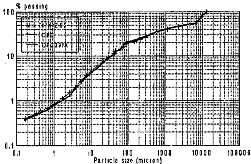
Figure 5.1e Grading curves of opc and pc30fa mixes
