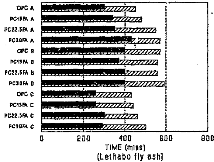
Figure 5.17c Initial and final setting times for equivalent 28 d mixes (standard curing)
