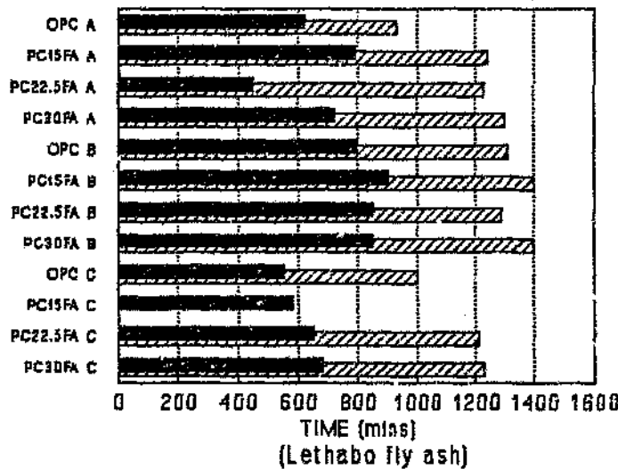
Figure 5.17f Initial and final setting times for direct replacement mixes (cold curing)
