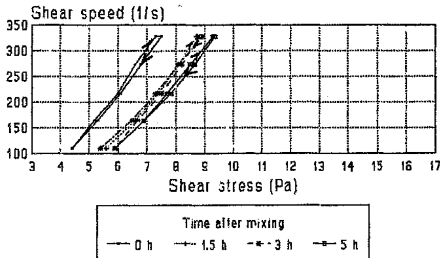
Figure 5.10c Change of viscosity with time for PPC OPC + 50% Matla at c/w = 1.67
