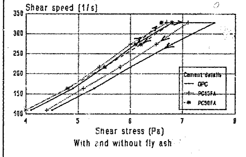
Figure 5.6b Viscous behaviour of PPC OPC Cement/water ratio = 1.67
