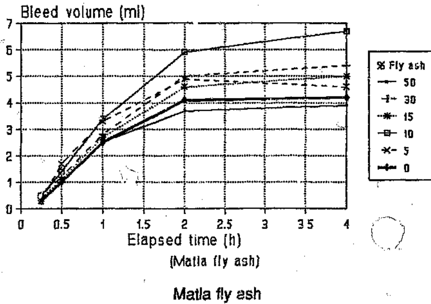
Figure 5.18c Bleed volume at c/w = 2.0 For varying fly ash contents
