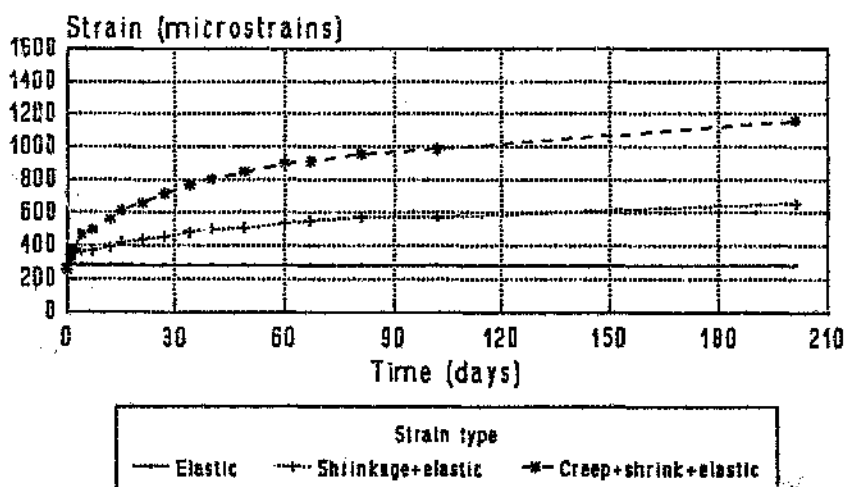
Figure 8.4f Creep, shrinkage and elastic deformation of PPC Jup. opc 30% fa mix with 13 stone
