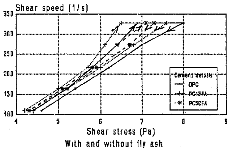
Figure 5.5b Viscous behaviour of Anglo-Alpha OPC Cement/water ratio = 1.67
