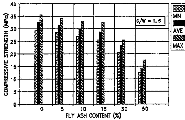
Figure 7.2b 28day compressive strength range
