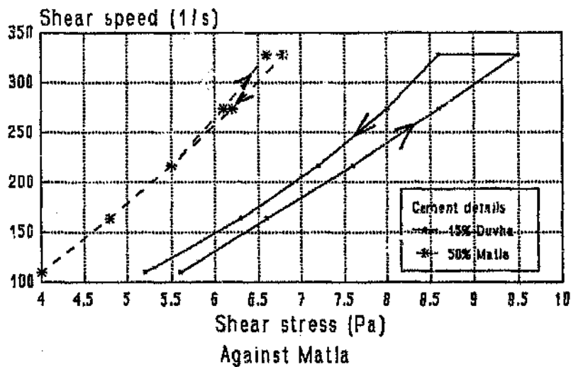
Figure 5.8b Viscous behaviour of Duvha blends Cement/water ratio = 1.67
