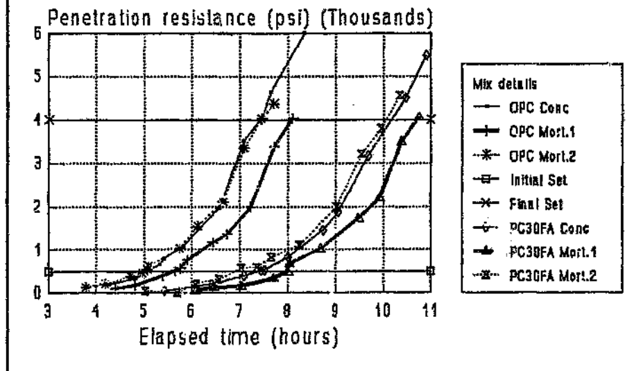
Figure 5.11 Comparison of concrete and mortar setting time methods for OPC & PC30FA
