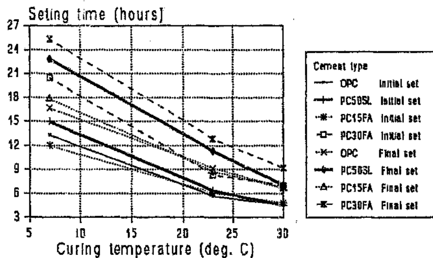
Figure 5.16b Setting times of OPC, SL and FA mortar at different temperatures
