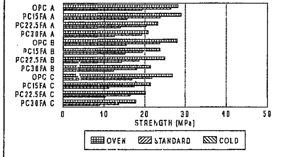
Figure 7.5j 7 Day Compressive strength DR cured at different temperatures
