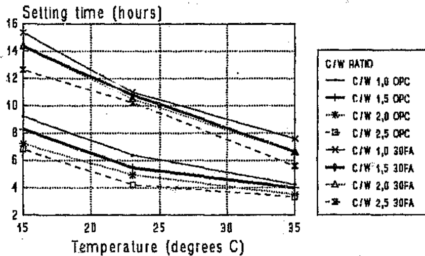
Figure 5.16a Setting time of OPC and FA mortar at different temperatures
