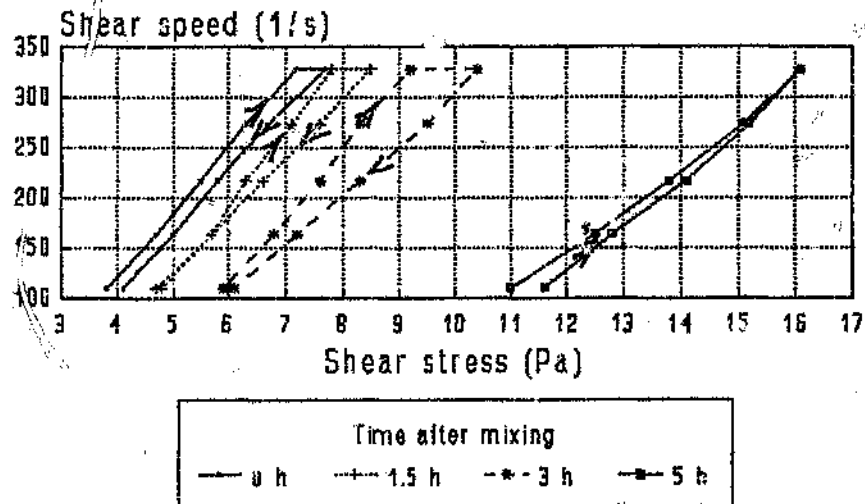
Figure 5.10a Change of viscosity with time for PPC OPC at c/w = 1.67
