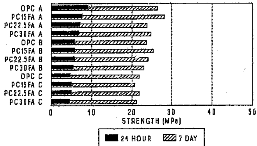
Figure 7.3a Compressive strength Standard cured equivalent 28 day mixes
