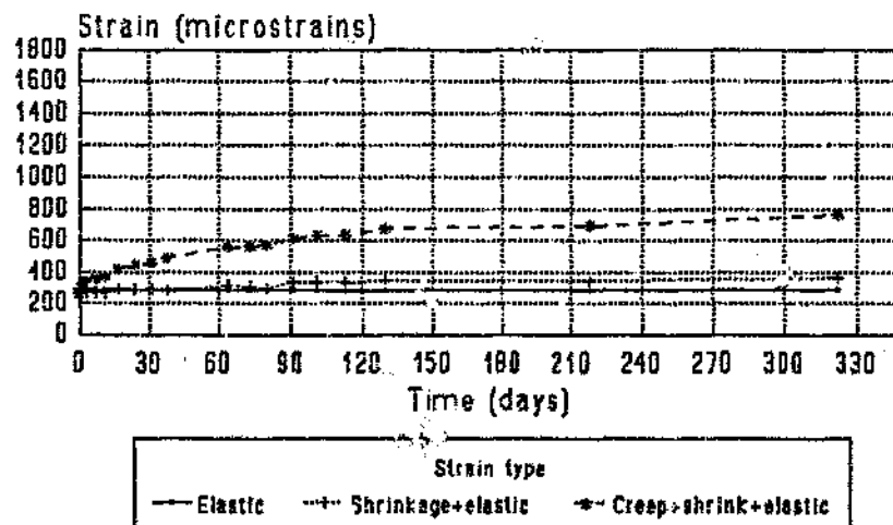
Figure 8.6a Creep, shrinkage and elastic deformation of PPC Jup opc mix (13 mm stone, sealed)
