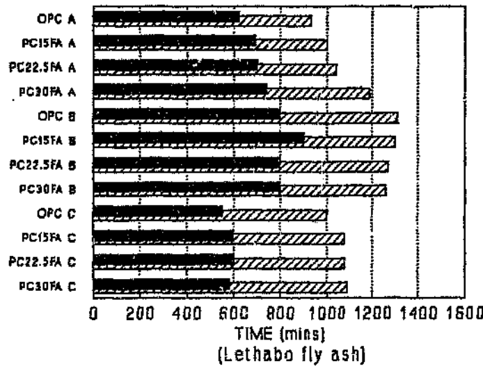
Figure 5.17e Initial and final setting times for equivalent 28 day mixes (cold curing)
