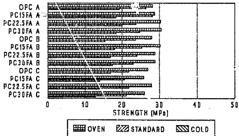
Figure 7.5i 7 Day Compressive strength EQ 28 cured at different temperatures
