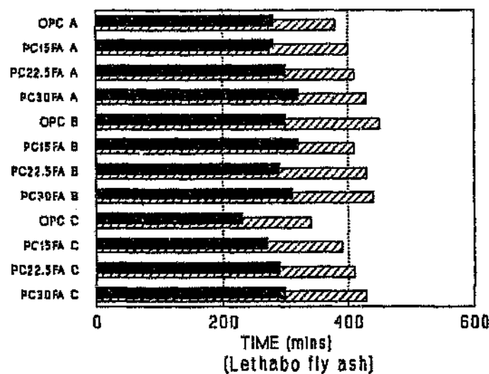
Figure 5.17b Initial and final setting times for direct replacement mixes (hot curing)
