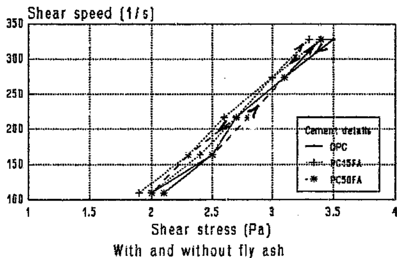
Figure 5.5a Viscous behaviour of Anglo-Alpha OPC Cement/water ratio = 1.3
