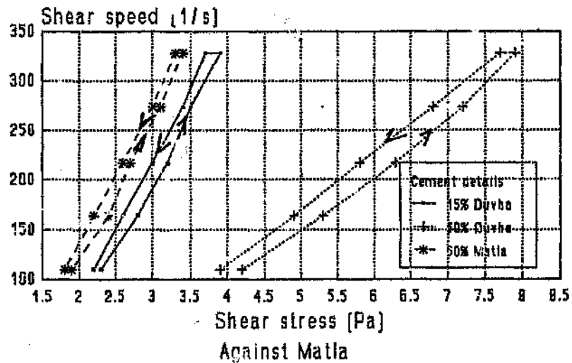
Figure 5.8a Viscous behaviour of Duvha blends Cement/water ratio = 1.3
