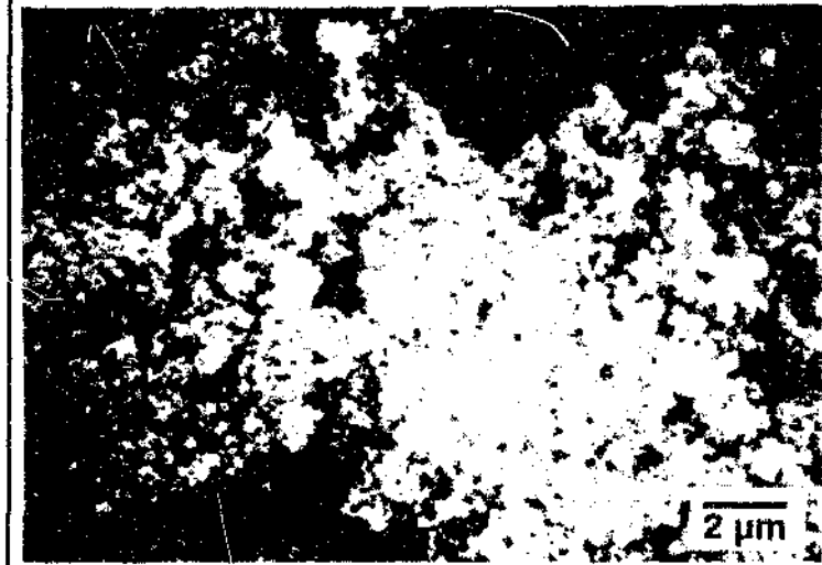
Figure 4.10 Photomicrograph of silica fume
