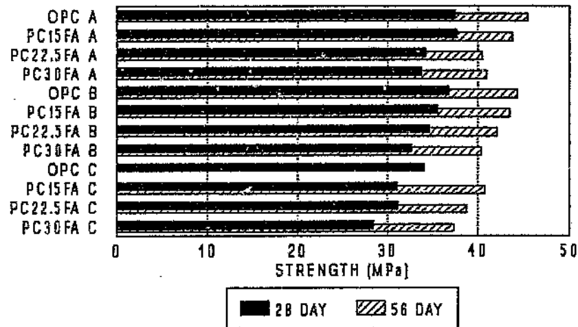
Figure 7.3d Compressive strength Standard cured direct replacement mixes
