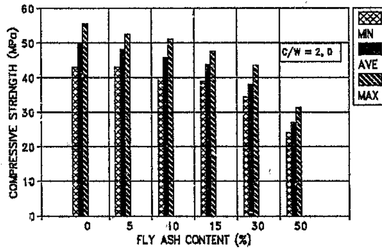
Figure 7.2c 28 day compressive strength range
