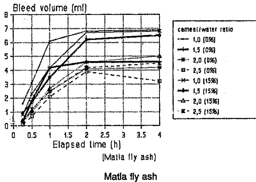
Figure 5.18e Bleed volume at FA = 0 and 15% For varying c/w ratios
