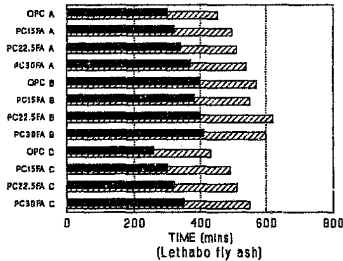
Figure 5.17d Initial and final setting times for direct replacement mixes (standard cure)
