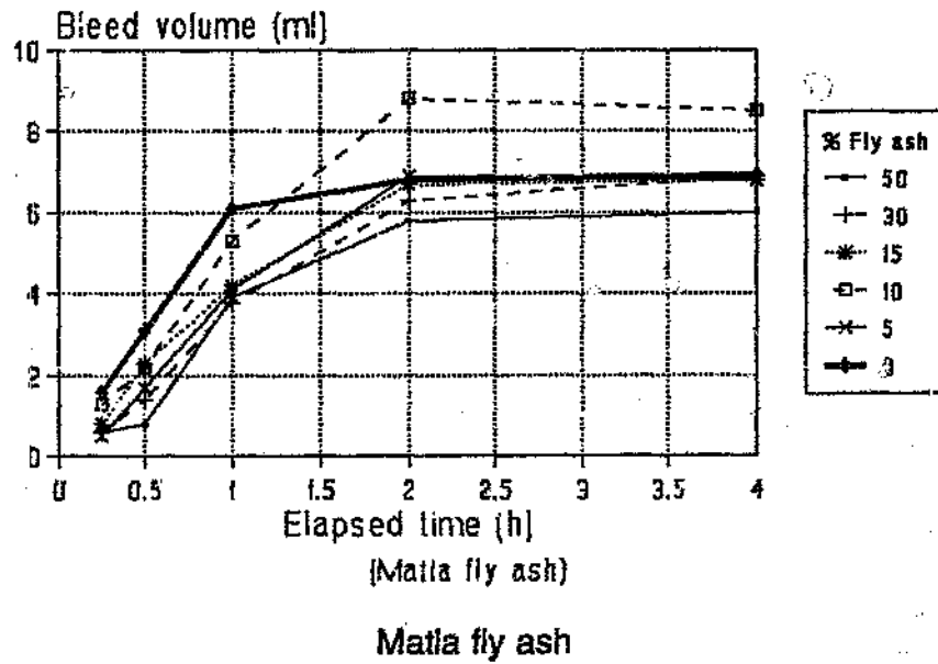
Figure 5.18a Bleed volume at c/w = 1,0 For varying fly ash contents
