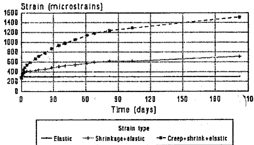
Figure 8.4c Creep, shrinkage and elastic deformation of BC Light. opc mix with 13 mm stone
