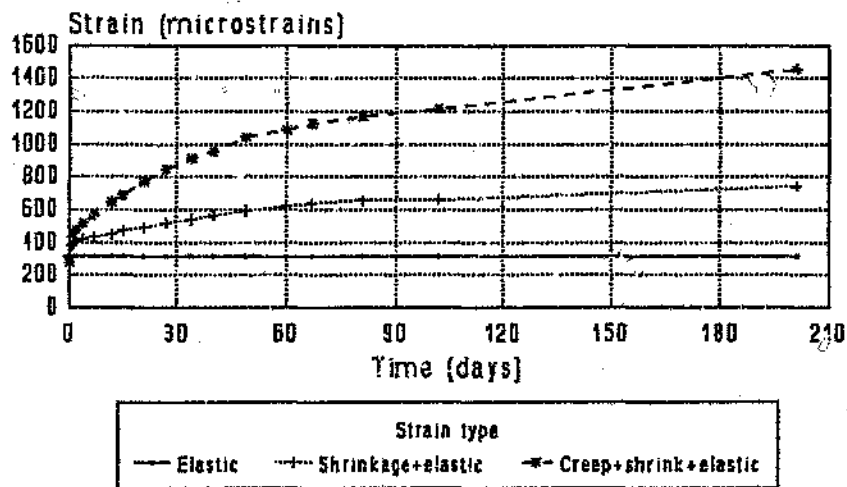
Figure 8.4e Creep, shrinkage and elastic deformation of BC Light opc 15% fa mix with 13 stone
