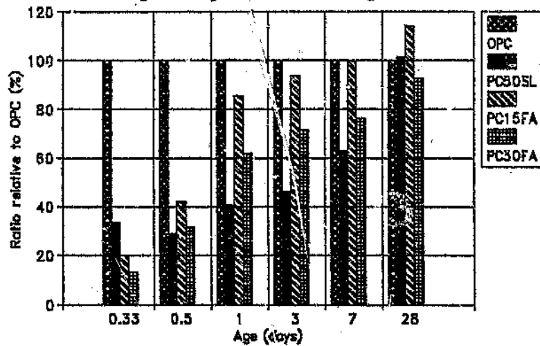
Figure 7.5e Age strength ratio at 23 degrees
