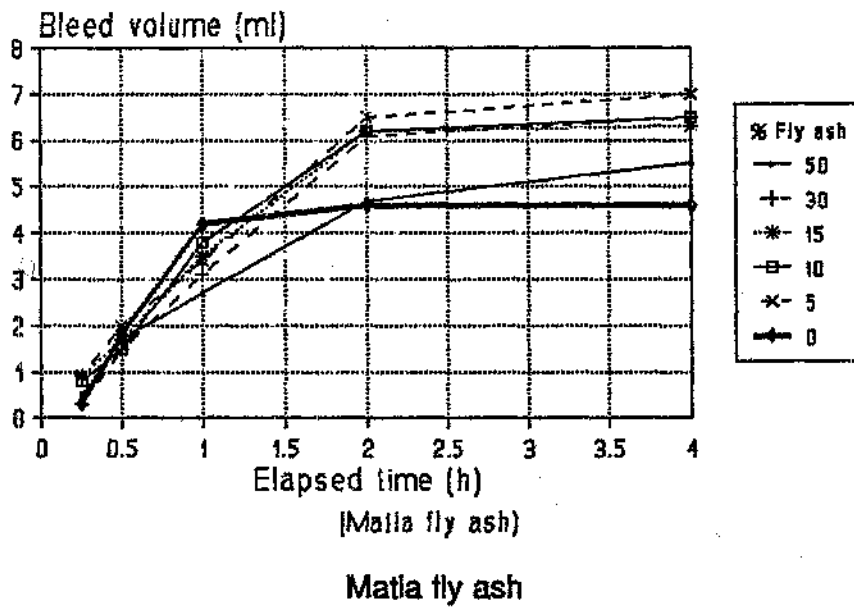
Figure 5.18b Bleed volume at c/w = 1,5 For varying fly ash contents
