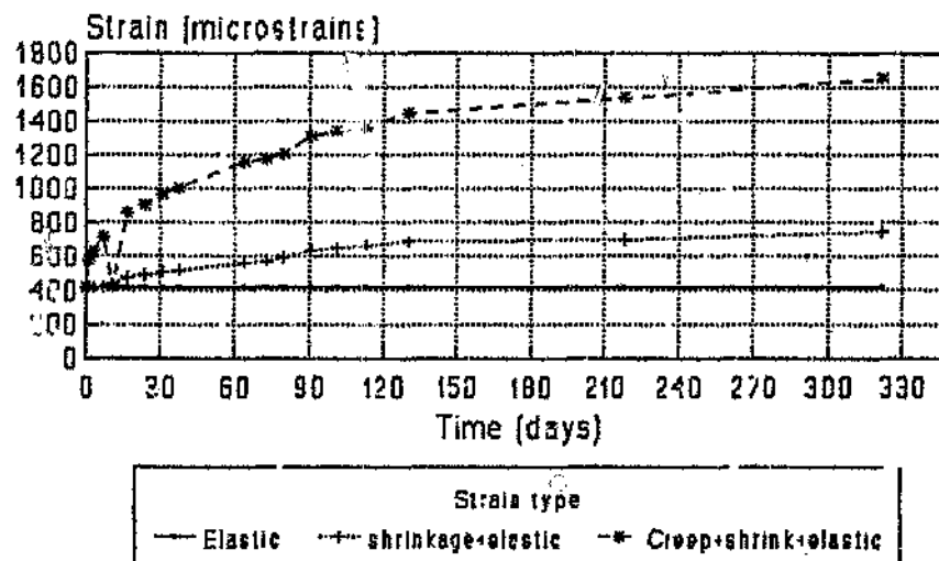
Figure 8.6b Creep, shrinkage and elastic deformation PPC Jup cpc (13 mm stone, unsealed)
