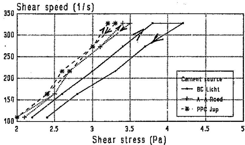
Figure 5.3a Viscous behaviour of OPC's Cement/water ratio = 1.3
