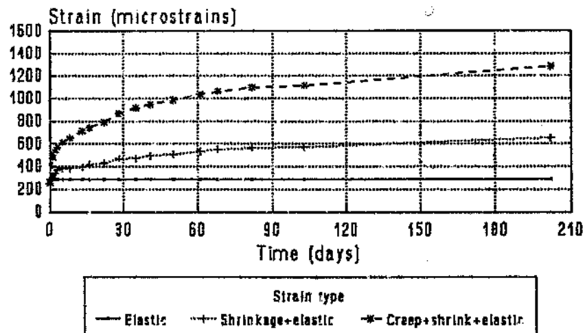
Figure 8.4d Creep, shrinkage and elastic deformation of PPC Jup opc 15% fa mix with 13 stone
