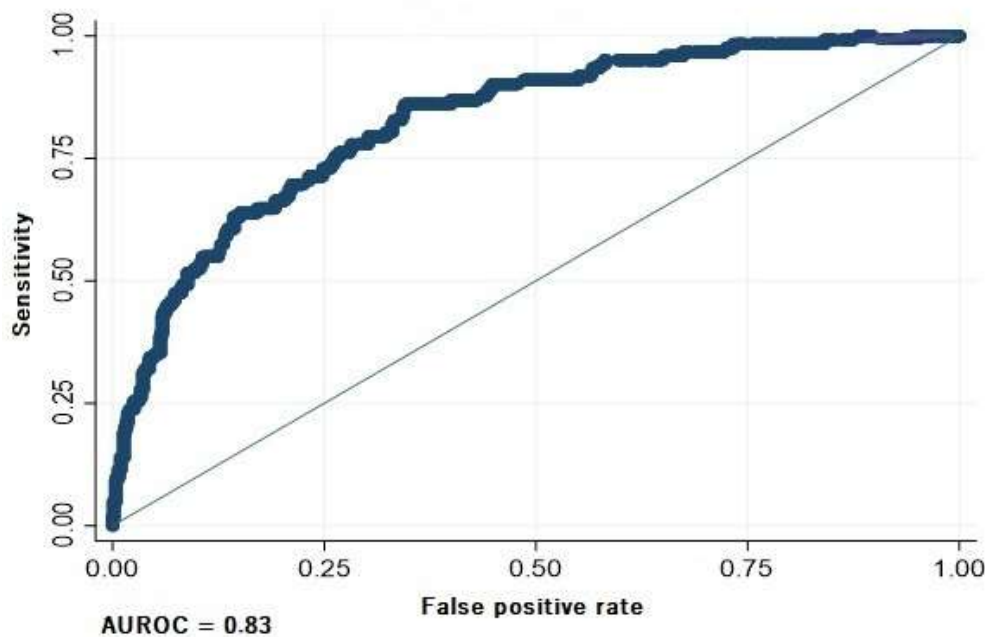
Figure 9: Receiver operating characteristic curve of the prediction model
