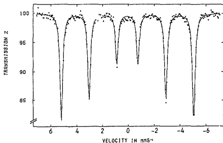
Fig. 3.2 A room temperature Mössbauer spectrum with a ^{57}\text{Co(Rh)} source and a 25% natural iron absorber.
