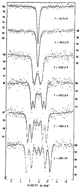
Fig. 5.5 Spectra with a stainless steel absorber and ^{57}\text{Co}(\text{}^{57}\text{Fe}) source close to the Curie temperature.
