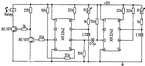
Fig. A.1 Circuit diagram for liquid nitrogen timer/filler
