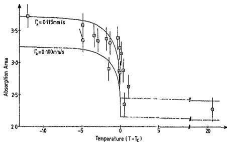
Fig. 5.6 Absorption area of a 25 \mu natural iron foil recorded with a ^{57}\text{Co(Rh)} source at temperatures near the Curie point.
