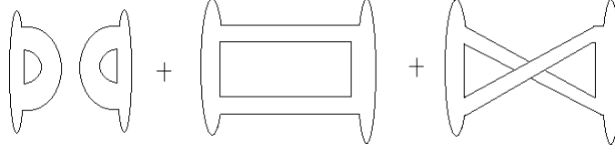
Figure 4.3: \langle Tr(X^2)Tr(X^2) \rangle
