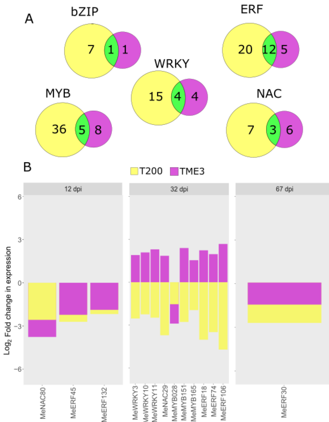
Figure 3-2: The comparison between (A) the number of different DE members belonging to the five TF families of interest and (B) the expression profiles of the common TFs DE at the same time point in both T200 and TME3 landraces.
