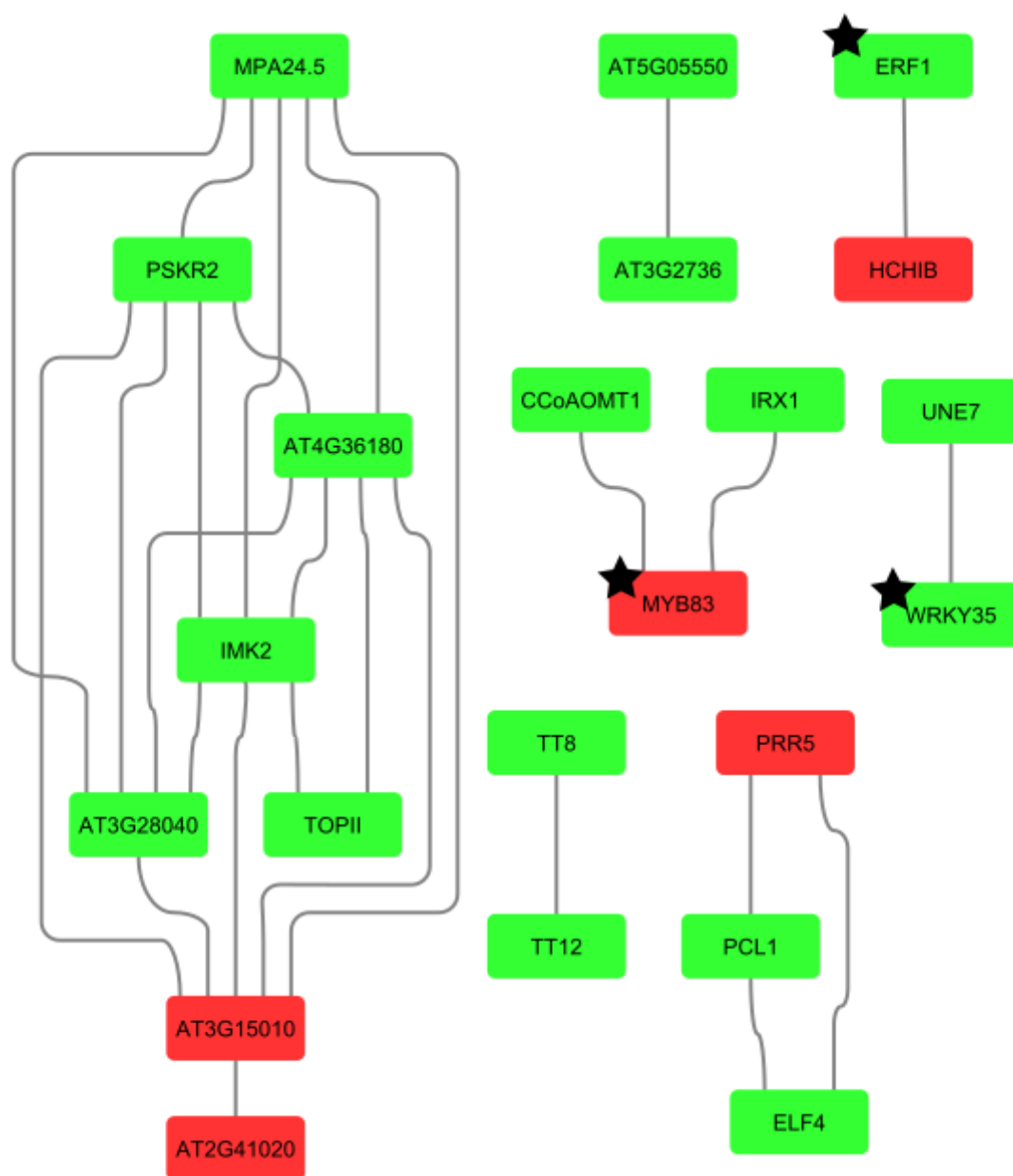
Figure 3-5: Protein-protein interaction network centring around the unique Arabidopsis homologs only identified to be DE in T200 at 67 dpi. TFs in the network are designated with a black star. Red genes represent down-regulation while green represents up-regulation of genes in response to SACMV. Disconnected nodes were removed. Only interaction occurring between at least two DEGs are shown and all unconnected DEGs were removed from the network.
