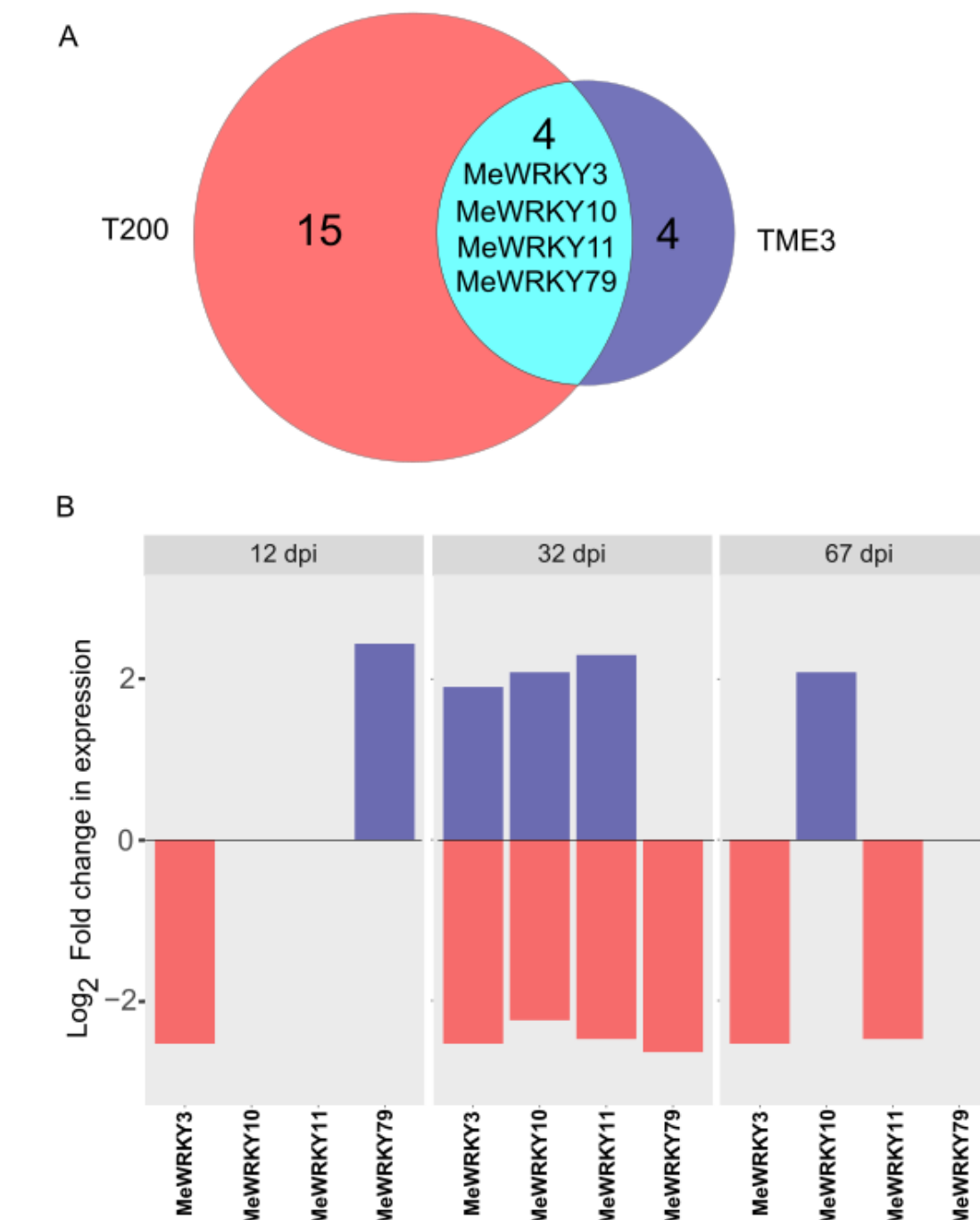
Figure 2-2: Differential expression of MeWRKY transcription factors common to T200 and TME3. A. The total number of identified DE MeWRKY s in T200 (15), TME3 (4), and those common (4) to both landraces, landrace throughout disease progression. B. Log 2 -fold change in expression of the four common MeWRKY s identified in T200 and TME3 at 12, 32 and 67 dpi.
