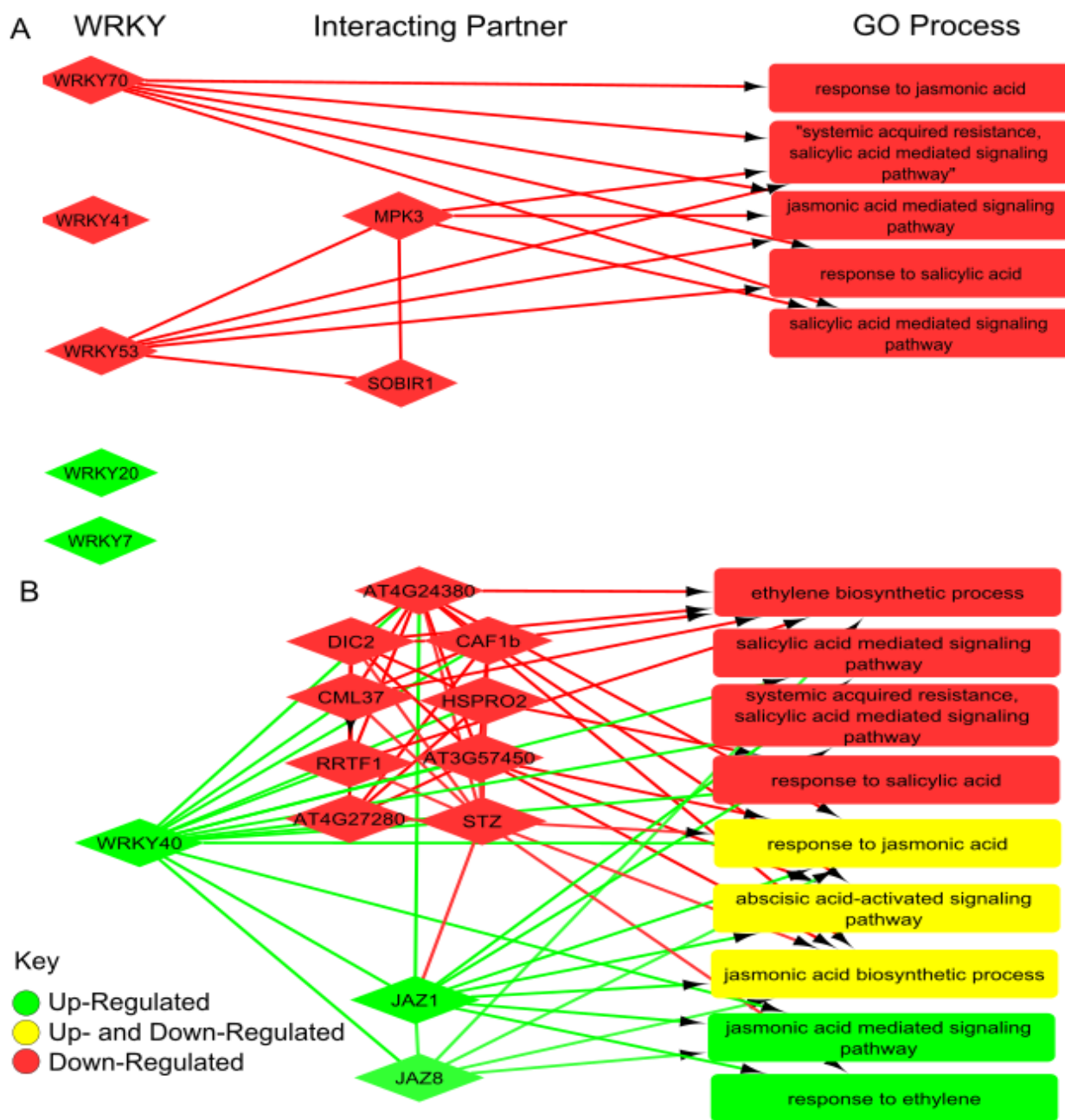
Figure 2-6: Predicted pathways and hormone responses of the differentially expressed (DE) WRKYs identified in (A) T200 and (B) TME3 at 12 dpi. From left to right: the DE WRKY TFs identified at 12 dpi, their differentially expressed interacting partners from STRING, and on the right the enriched GO biological process (hormone responses) derived from the DE WRKYs and DEGs. Red and green represent the relative Log 2 -fold change expression, down-regulation and up-regulation, respectively, at 12 dpi at each of the nodes, and the GO terms enriched with only the down-regulated genes. Yellow represents GO processes that were found to be enriched in both up- and down-regulated genes at 12 dpi.
