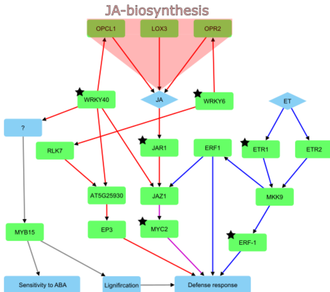
Figure 3-9: The proposed model of the network in TME3 at 32 that induces an ISR-like response which leads to SACMV tolerance. Genes shown in green boxes represent up-regulation of the cassava homologs in TME3 at middle infection. Diamond blue nodes represent hormone molecules, while the different colour edges represent the transduction of signal associated with each hormone signaling pathway (red for JA signaling, blue for ET signaling, and purple representing the intersection of both signals). Stars represent not TFs but rather proteins that have been previously described to be associated with ISR.
