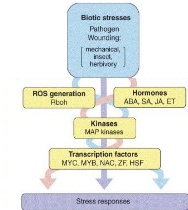
Figure 1-3: Overview of the signal transduction involved in biotic and abiotic stress responses in plants and the various components involved with mounting the appropriate response. Both biotic and abiotic stress pathways incorporate the use of ROS, hormones and kinases to transduce the signal to TFs. It is then up to TFs to lead to changes in expression of targeted to genes in order to respond to the stress in an appropriate manner (adapted from Fujita et al. , 2006).
