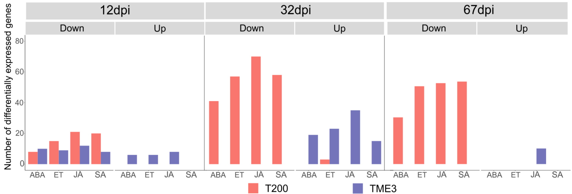
Figure 2-9: The number of up- and down-regulated DEGs involved in phytohormone processes in TME3 and T200. The bar graph shows the number of up- and down-regulated DEGs found to be involved in the ABA, ET, JA, and SA signaling based on the infection stage and relative log 2 -fold change in expression. These numbers were determined by counting all unique genes involved in any enriched GO process associated with phytohormones
