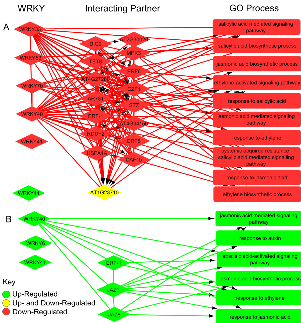
Figure 2-7: Predicted pathways and hormone responses of the differentially expressed (DE) WRKYs identified in (A) T200 and (B) TME3 at 32 dpi. From left to right: the DE WRKY TFs identified at 12 dpi, their differentially expressed interacting partners from STRING, and on the right the enriched GO biological process (hormone responses) derived from the DE WRKYs and DEGs. Yellow represents a single Arabidopsis gene that has two cassava homologs that show contrasting differential expression.
