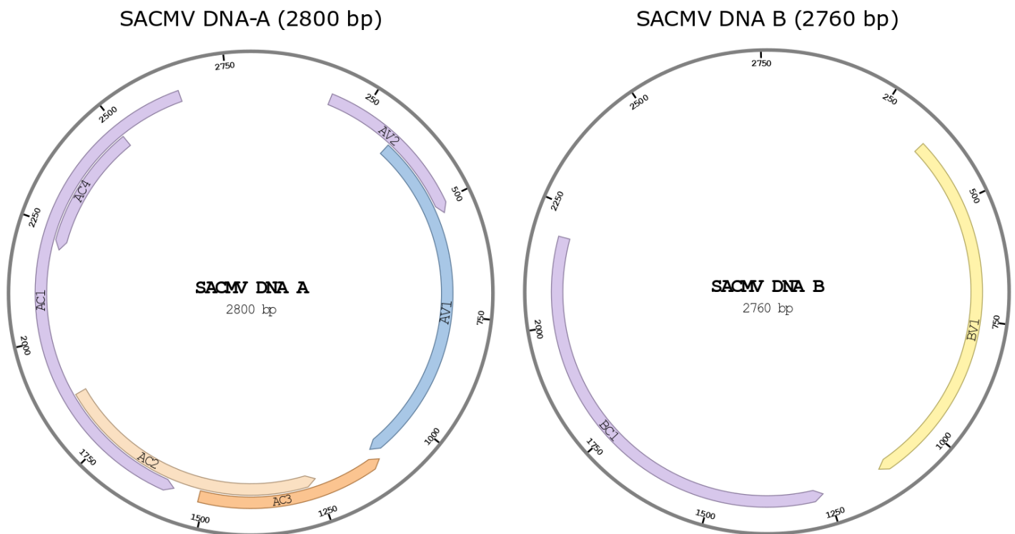
Figure 1-1 The bi-partite genome of SACMV showing the open reading frames and their positions
