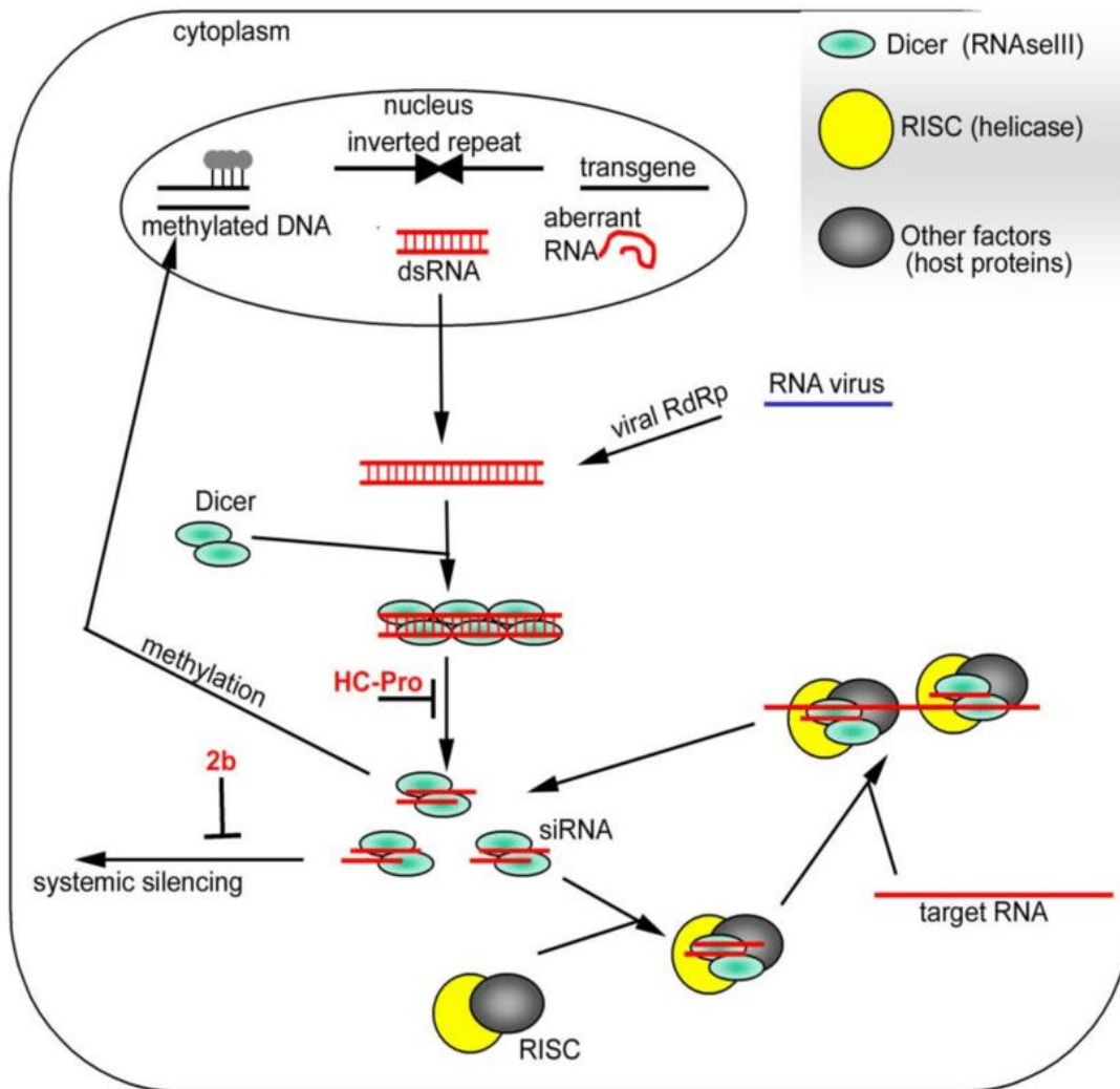
Figure 1-7: Overview of RNAi and the proteins involved. RNAi can either be induced from dsRNA derived from exogenous viral RNA (blue) or dsRNA synthesised in the nucleus. This either leads to PTGS, once the processed RNA is incorporated into the RISC complex, or TGS can occur leading to methylation of targeted DNA. (SURGONDA, 2015)
