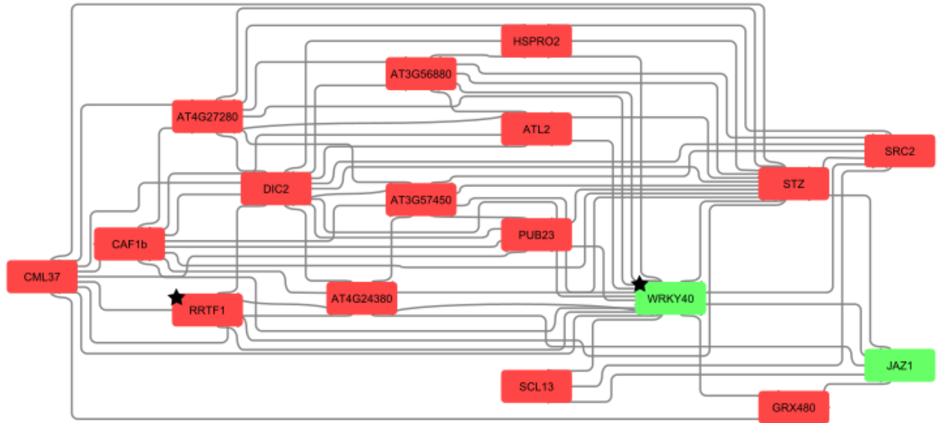
Figure 3-6: Protein-protein interaction network centring around the Arabidopsis homologs of identified DE TFS in TME3 at 12 dpi. TFs in the network are designated with a black star. Red genes represent down-regulation while green represents up-regulation of genes
