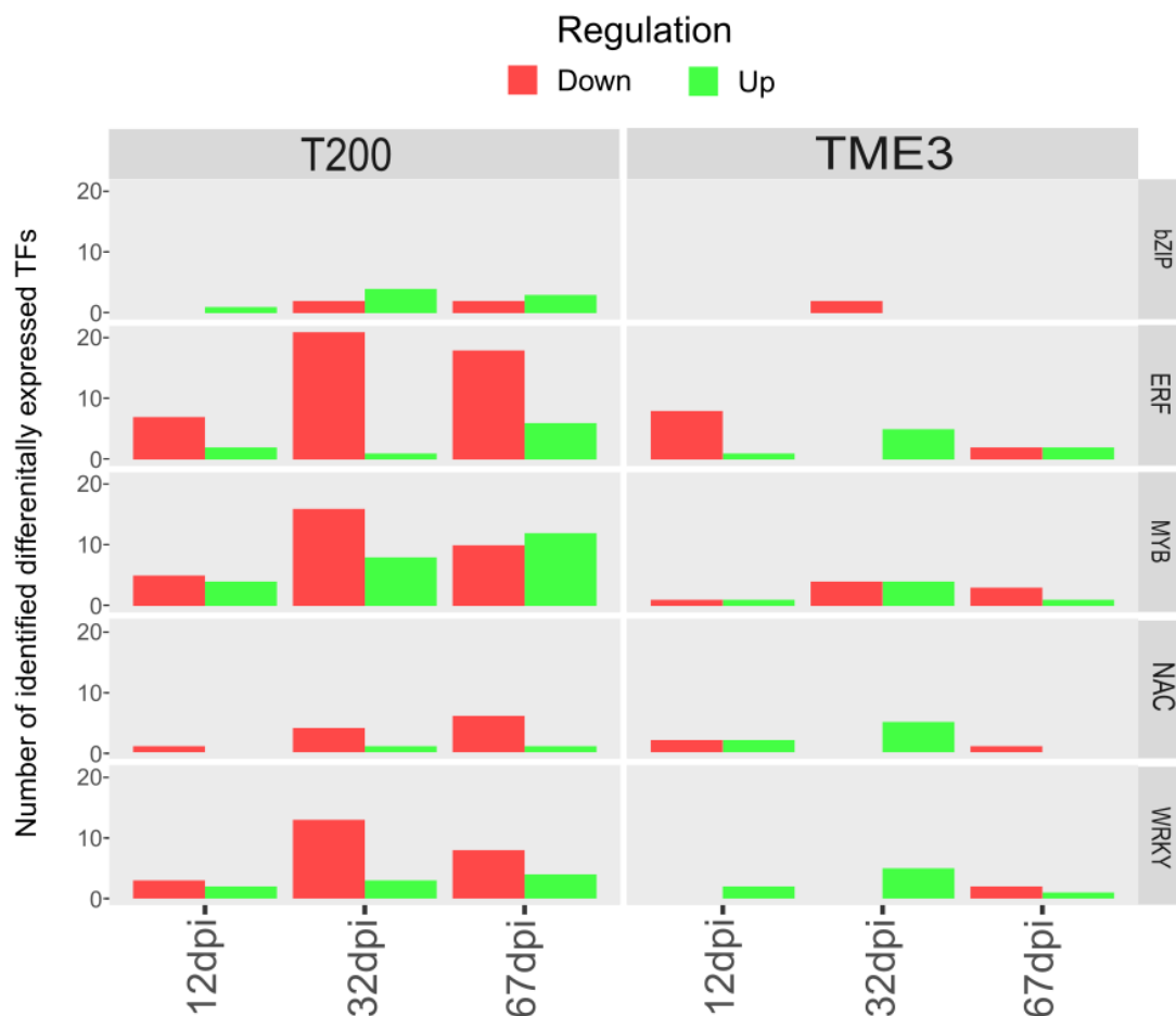
Figure 3-1: The global representation of the number of DE TFs belonging to the bZIP, ERF, MYB, NAC and WRKY families in T200 and TME3 during the time course of SACMV infection. Green and red represent up- and down-regulation, respectively.
