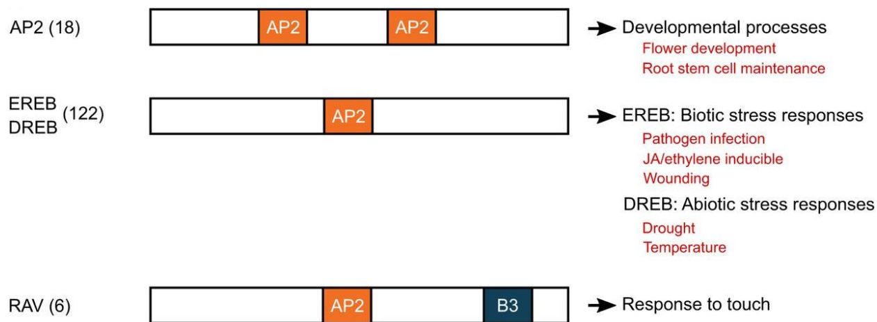
Figure 1-4: A structural overview of the subgroups within the AP2/ERF TF family with their associated conserved motifs and biological functions. The number in brackets shows the number of proteins identified in A. thaliana in each group (adapted from Heyman et al. , 2018).
