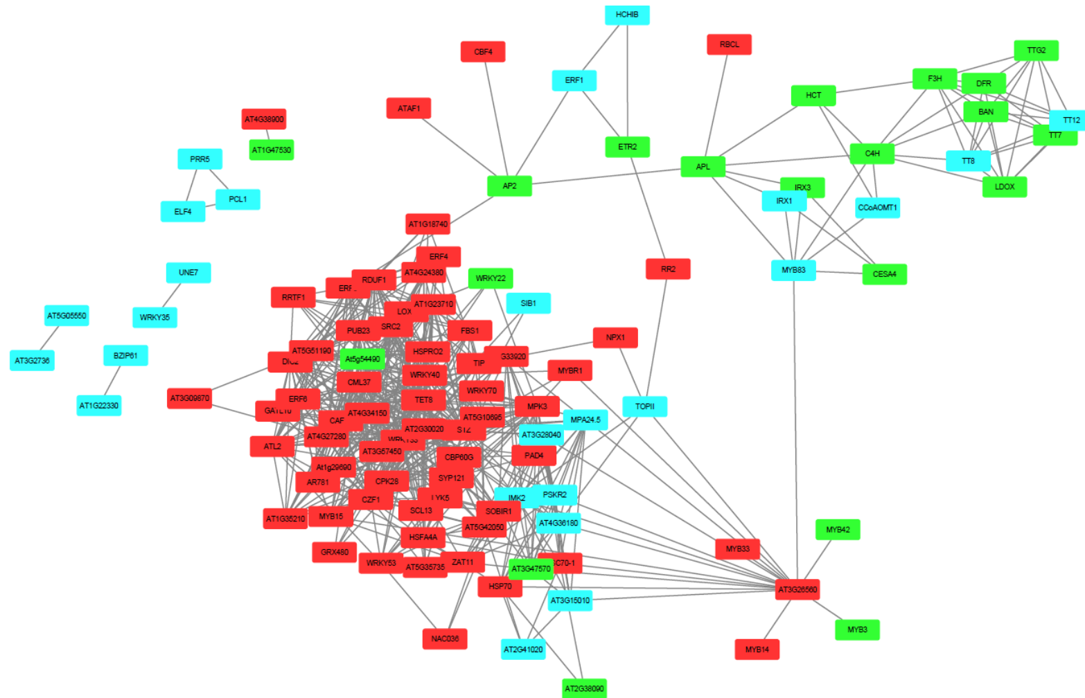
Supplementary Figure 2: Full network of interacting proteins in T200 at 67 dpi around the proteins found uniquely to that time point (Blue). Green and red nodes represent up-and down-regulation respectively
