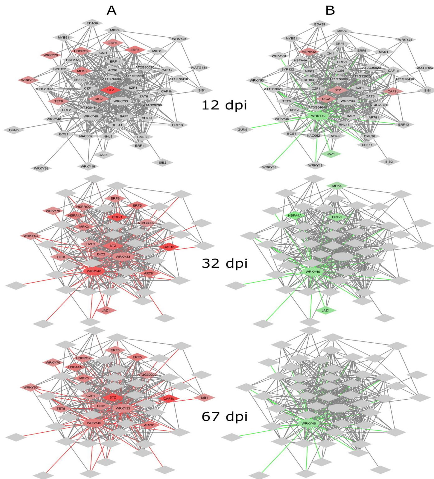
Figure 2-5: STRING protein-protein interaction network centring around AtWRKY33 and 40 and their interacting partners. Differentially expressed (DE) genes from T200 (A) and TME3 (B) at early, middle and late infection are mapped to the network. Red and green genes refer to instances of down- and up-regulation respectively, while shading represents the magnitude of differential expression. Genes that were not DE in 32 and 67 dpi were removed from the network to simplify it.
