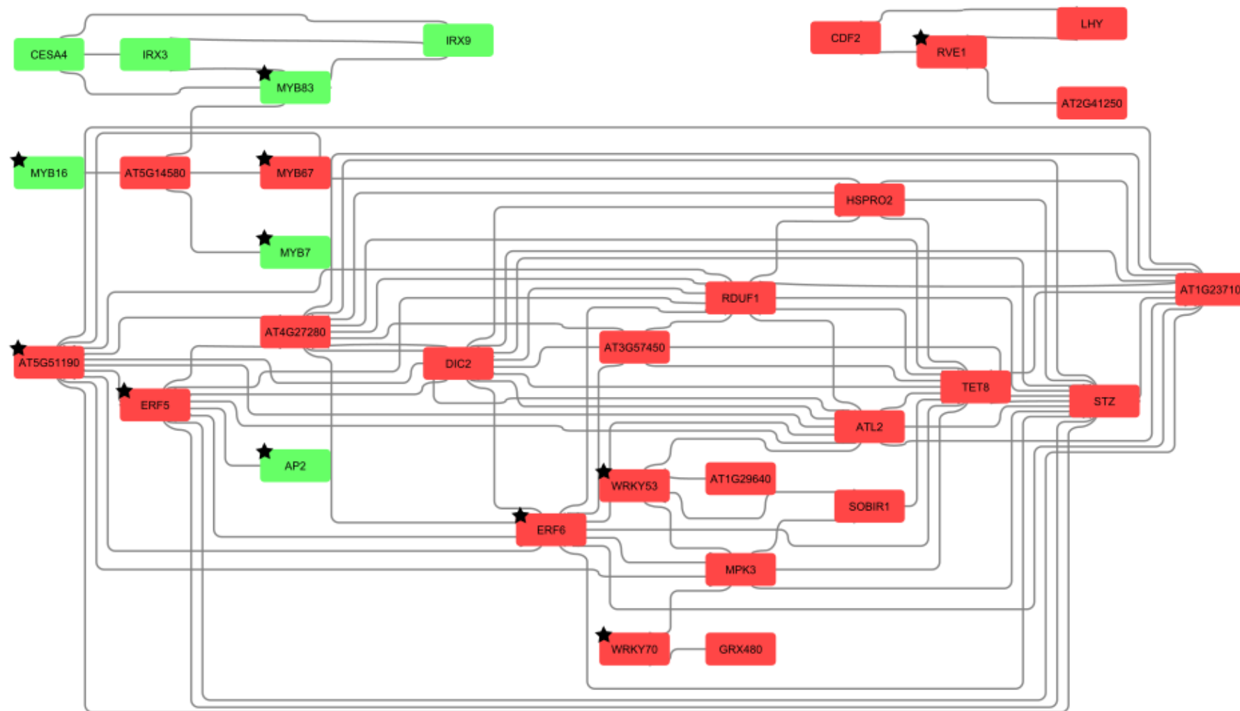
Figure 3-3: Protein-protein interaction network centring around the Arabidopsis homologs of identified DE TF in T200 at 12 dpi.
