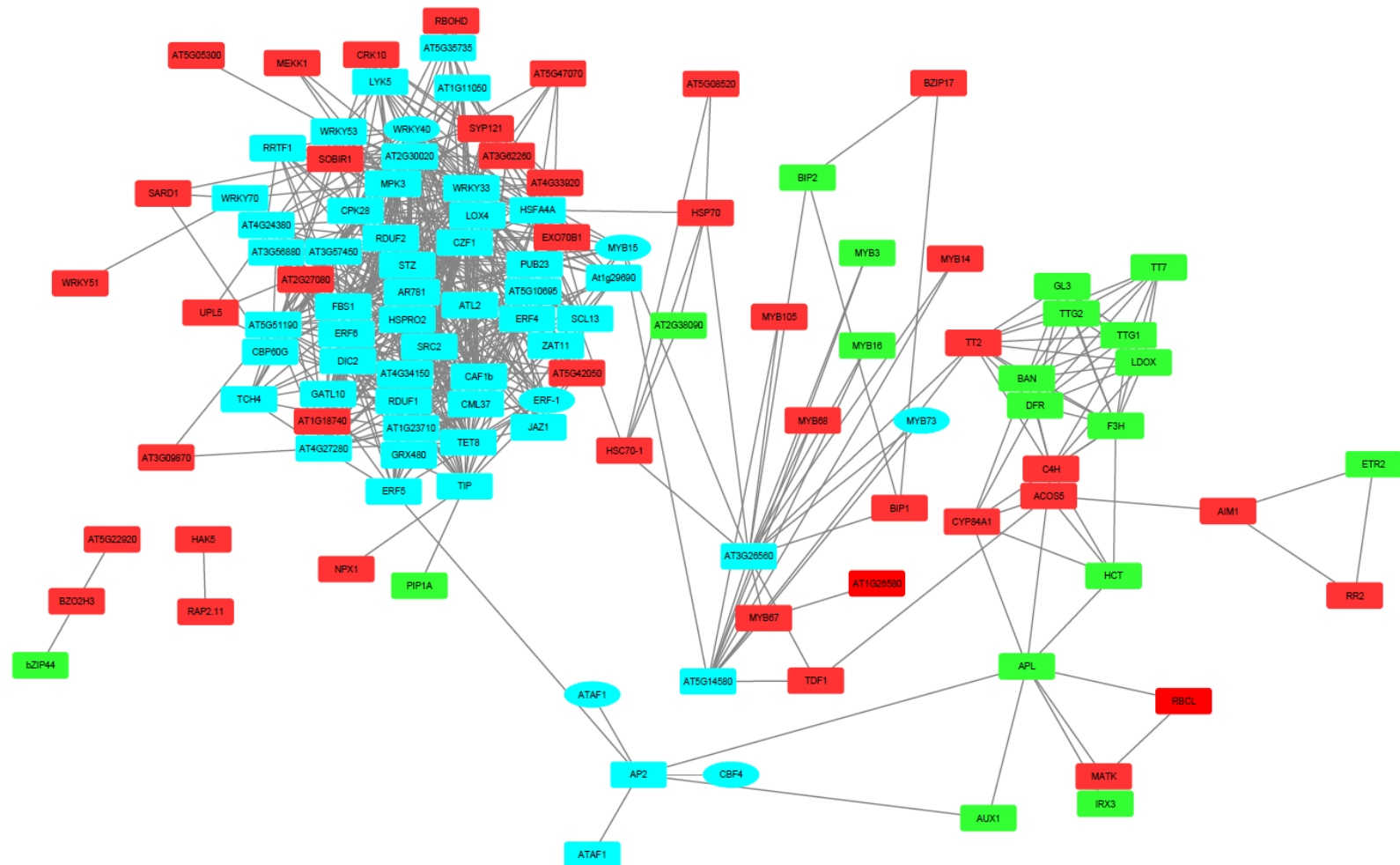
Supplementary Figure 1: Full network of interacting proteins in T200 at 32 dpi around the proteins found in Figure 3-4 (Blue) . Green and red nodes represent up-and down-regulation respectively
