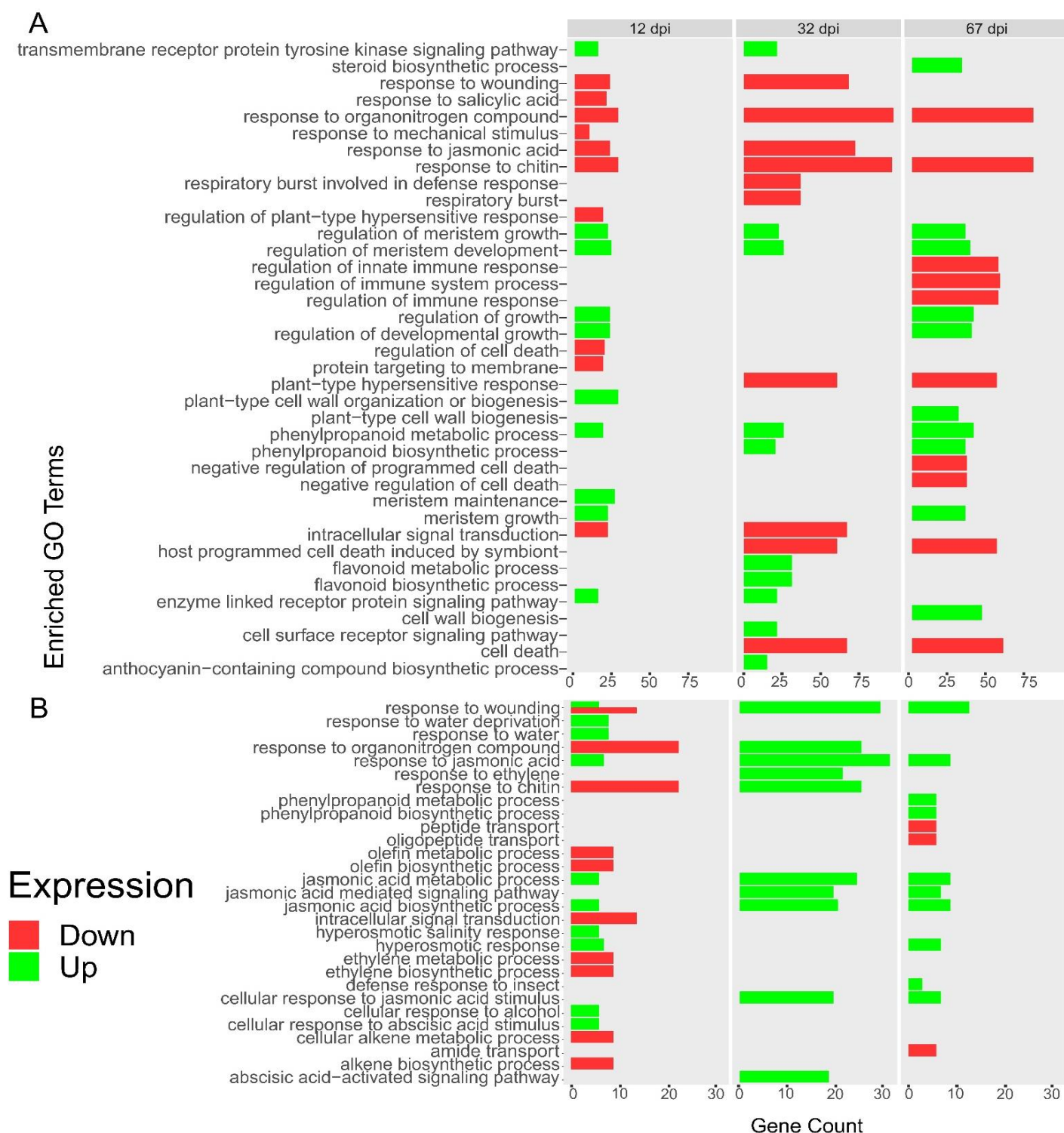
Figure 2-4: Top 10 most enriched biological processes associated in up- and down-regulated genes in T200 and TME3 throughout SACMV infection. The top 10 biological GO terms were taken based on the significance (p-value) of the GO terms in (A) T200 and (B) TME3, plotted against the counts of genes that fell into the GO category. Green represents the process found to be enriched among the up-regulated genes and red are processes enriched among down-regulated genes.
