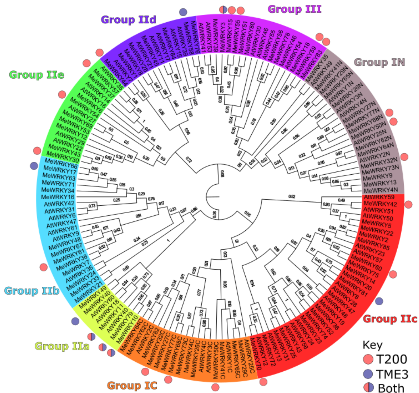
Figure 2-3: A phylogenetic tree of WRKY transcription factors from Arabidopsis thaliana (At) and cassava [ Manihot esculenta (Me)] sorted into taxonomic groups based on amino acid sequences (bootstrap value of a 1000). The tree demonstrates the three main groups that WRKY transcription factors belong to. Group I is characterized by two WRKY domains, Group II by one WRKY domain and a C2H2 zinc finger motif, and Group 3 has one WRKY domain and a C2HC Zn finger motif. Group 1 has been subdivided into two sub-groups (Group IC and Group IN) representing the alignment of the C and N terminus of the protein respectively. The tree is annotated (dots) with the differentially expressed WRKYs in SACMV-infected Arabidopsis. The phylogenetic tree was provided by Hu et al. , 2016 and altered in the Inkscape program to show DE WRKYs in T200 and TME3 at all 3 time points.
