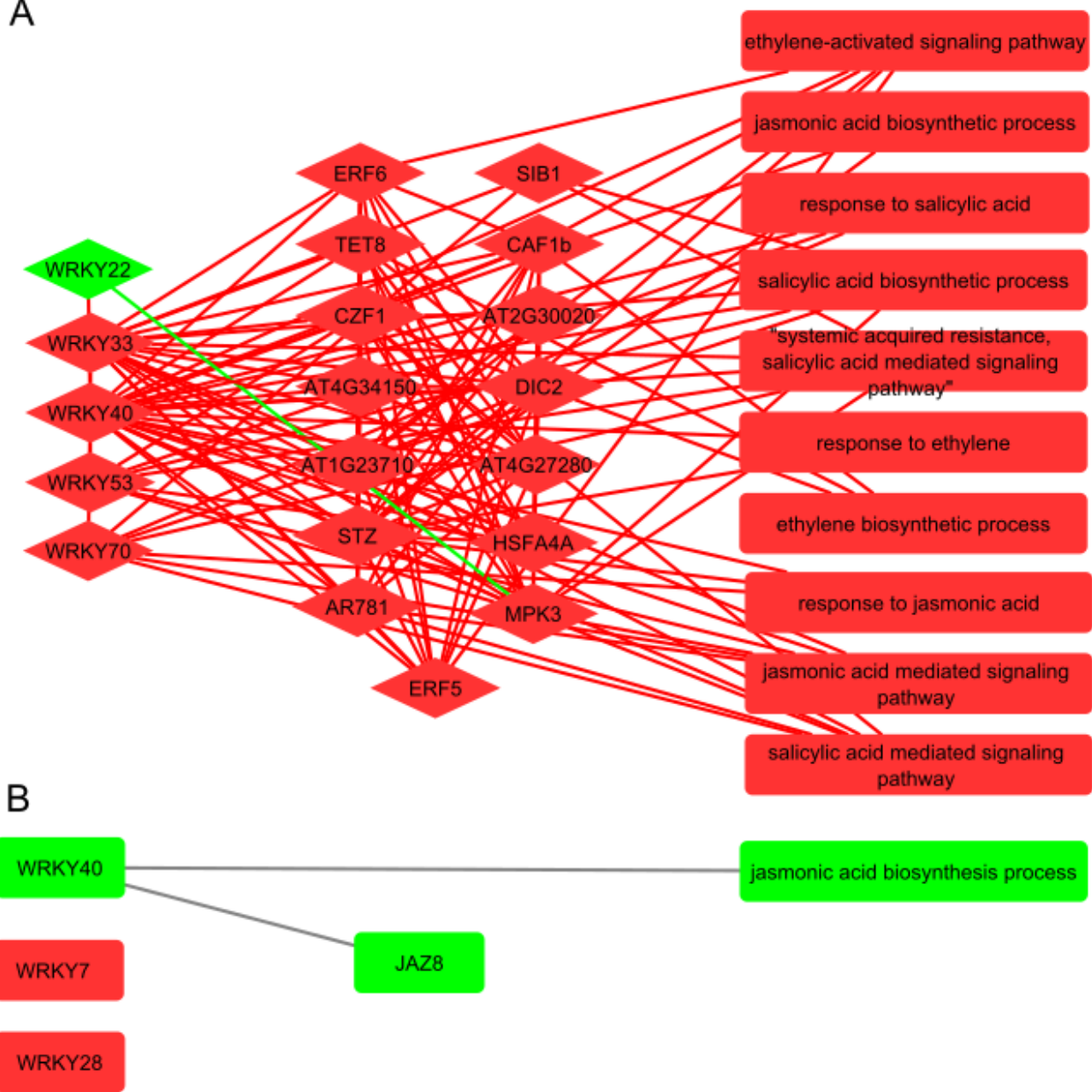
Figure 2-8: Predicted pathways and hormone responses of the differentially expressed (DE) WRKYs identified in (A) T200 and (B) TME3 at 67 dpi. From left to right: the DE WRKY TFs identified at 12 dpi, their differentially expressed interacting partners from STRING, and on the right the enriched GO biological process (hormone responses) derived from the DE WRKYs and DEGs.
