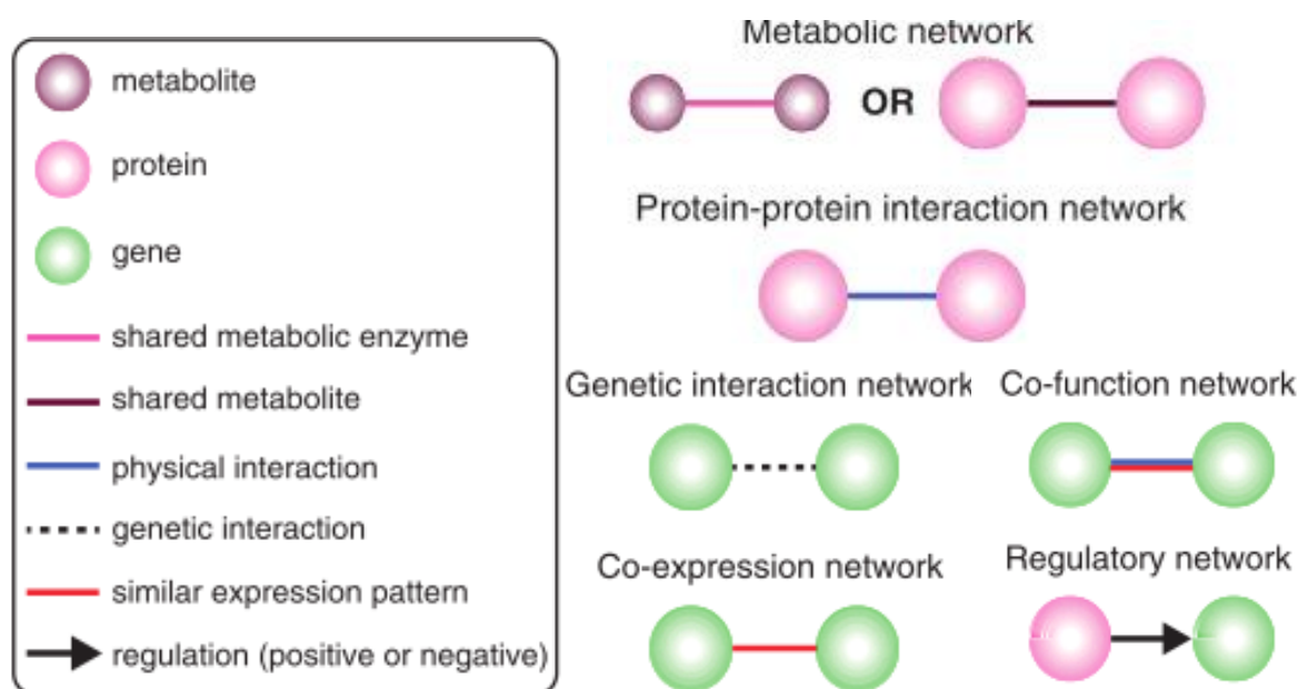
Figure 1-8: Schematic summary of the different types of nodes (circles) and edges (lines) which make up various biological networks. Adapted from Chae et al. , 2012.
