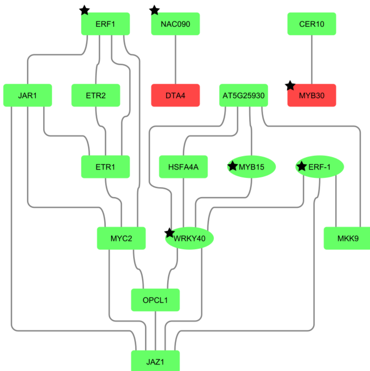
Figure 3-7: Protein-protein interaction network centring around the Arabidopsis homologs of DE TFS in TME3 at 32 dpi. TFs in the network are designated with a black star. Red genes represent down-regulation while green represents up-regulation of genes in response
