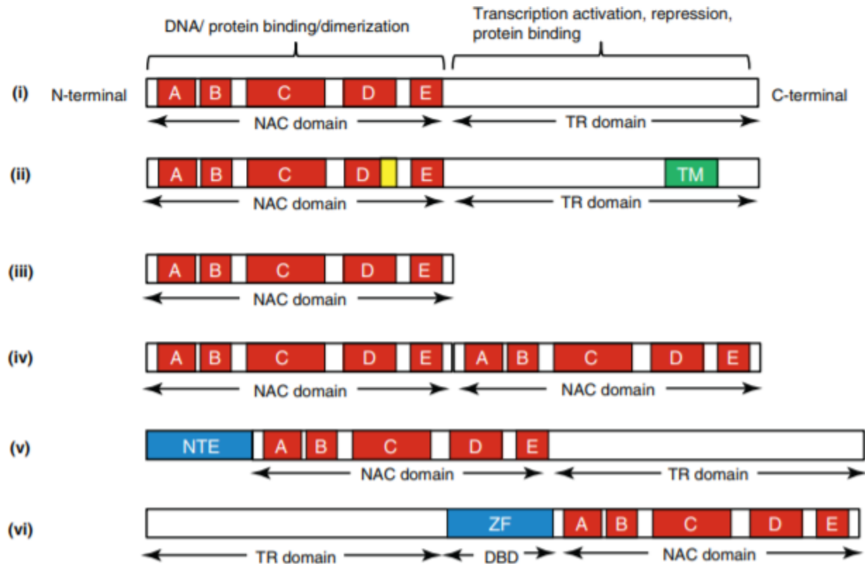
Figure 1-5: An overview of the NAC TF family showing the (i) typical domain figuration of the NAC domain that is further divided into five different repetitive domains (A-E). Sometimes variation can be seen in the family, where some TFs display (ii) a repressor domain (yellow) and a transmembrane domain (TM) at the C terminal. Further variation can be seen in NAC proteins containing (iii) only the NAC domain or (iv) a duplicated NAC domain. Lastly (v) N-terminally extended (NTE) and (vi) zinc finger (ZF) motifs have also been known to make an appearance with some NAC proteins (Prochnik et al. , 2012b).
