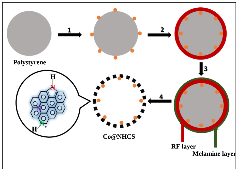
Figure 4.12 Schematic representation of the synthesis methodology. (1) loading Co metal onto a polystyrene template; (2) resorcinol-formaldehyde (carbon precursor) coating; (3) melamine (nitrogen precursor) coating and (4) template decomposition and annealing
