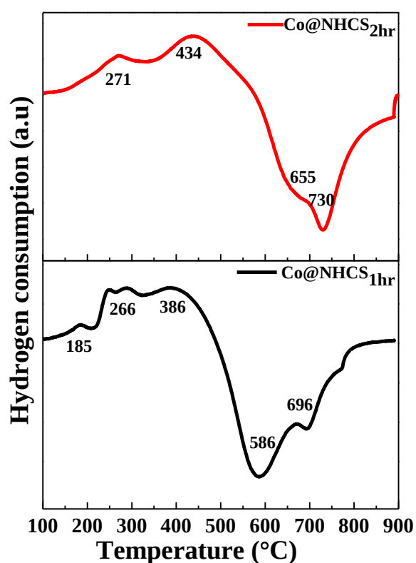
Figure 4.16 TPR profile for supported catalysts. (1hr) 1 hour annealing time; (2hr) 2 hours annealing time.
