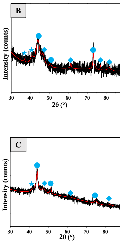
Figure 4.10 PXRD patterns of Co catalysts, reduced in H 2 gas at 450 °C for 3 hours. (A) Co@NHCS, (B) Co@NHCS@Ru, (C) Co-Ru@NHCS; CoO (★), Co hcp (◆), Co fcc (●)
