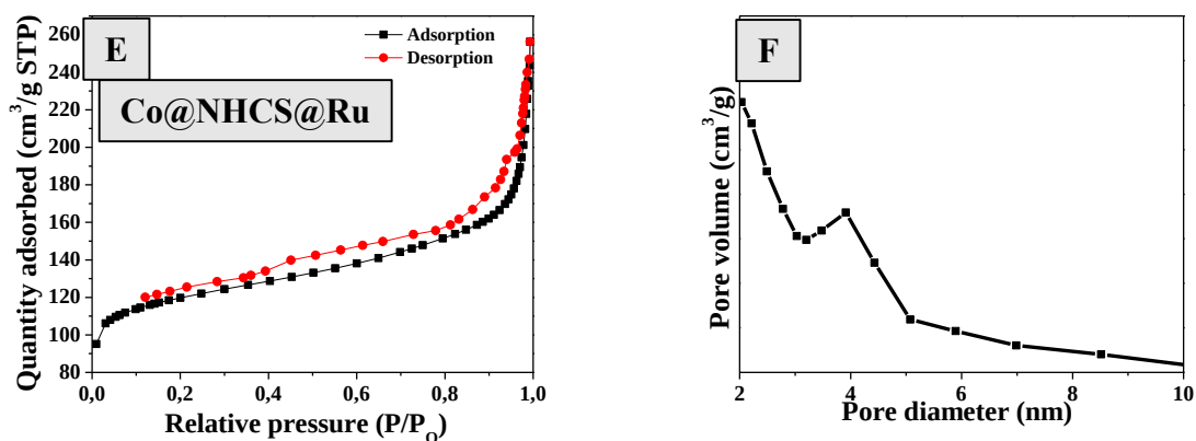
Figure 4S.3 N 2 adsorption-desorption isotherm (A, C, E) and the corresponding adsorption pore size distribution (B, D, F) for catalysts Co@NHCS, Co-Ru@NHCS and Co@NHCS@Ru, respectively.
