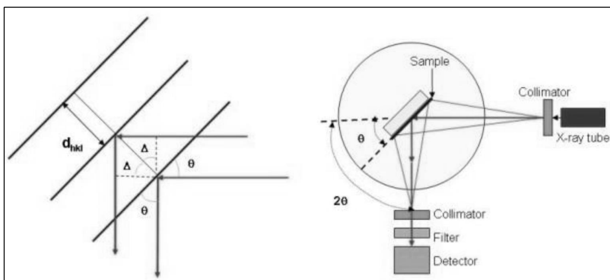
Figure 3.2 Bragg's schematic and a typical setup on an XRD diffractometer. 12
