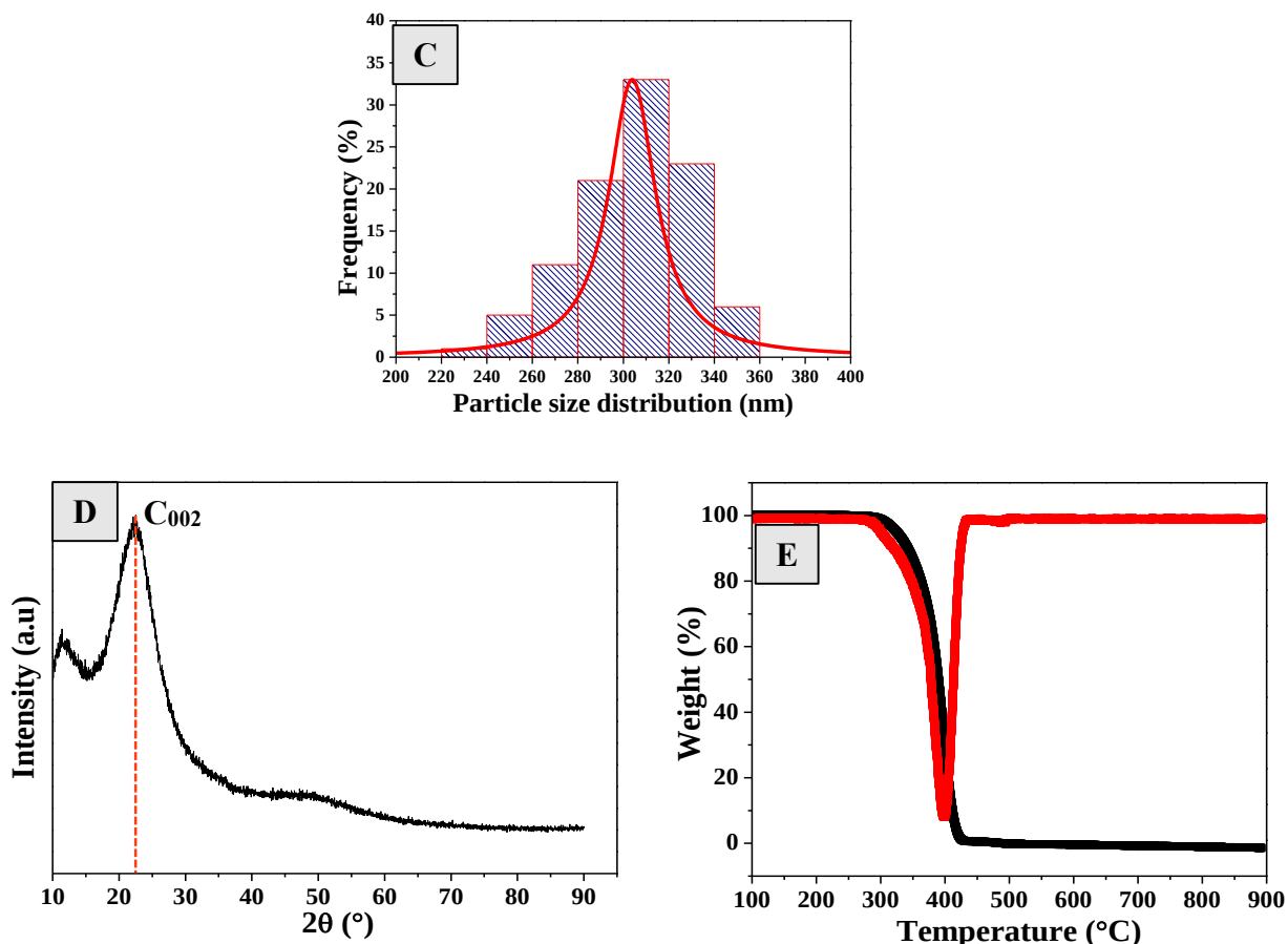
Figure 4.3 SEM image (A), TEM image (B), particle size distribution (C), PXRD pattern (D) and TGA with DTG (E) for polystyrene spheres.
