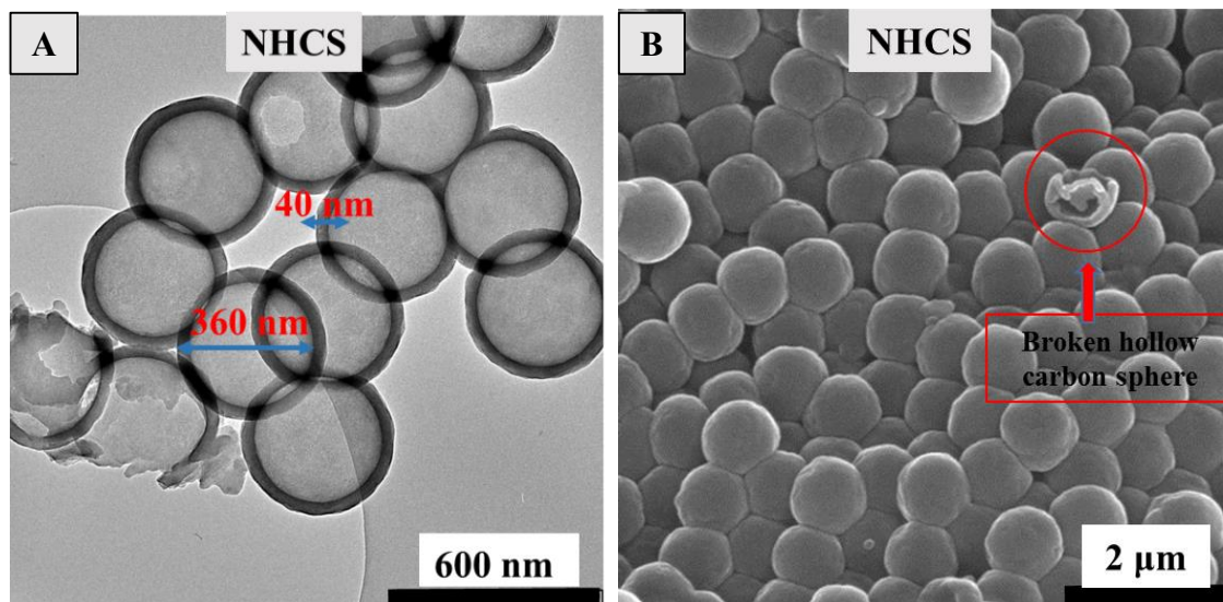
Figure 4.4 TEM (A) and SEM (B) image of N-doped hollow carbon spheres (NHCSs).
