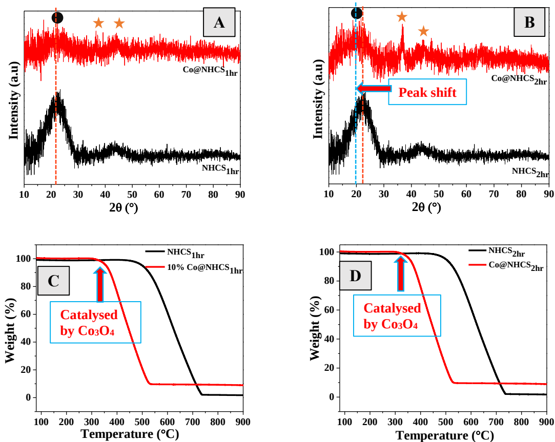
Figure 4.14 PXRD patterns (A, B) and TGA profiles (C, D) of catalysts. (1hr) 1 hour annealing time; (2hr) 2 hours annealing time; Carbon (●); Co 3 O 4 (★)
