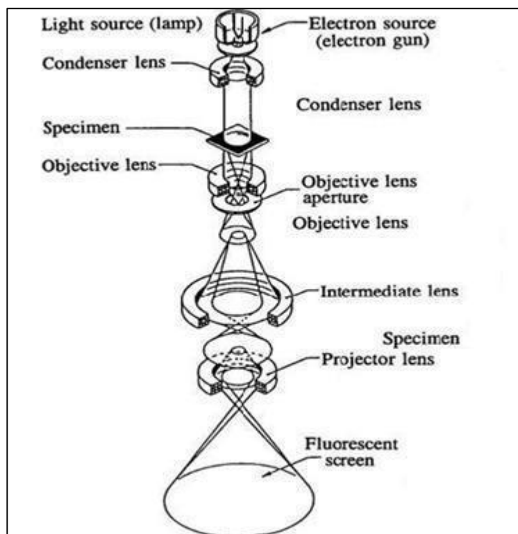
Figure 3.7 Schematic of main components found in a TEM instrument. 18
