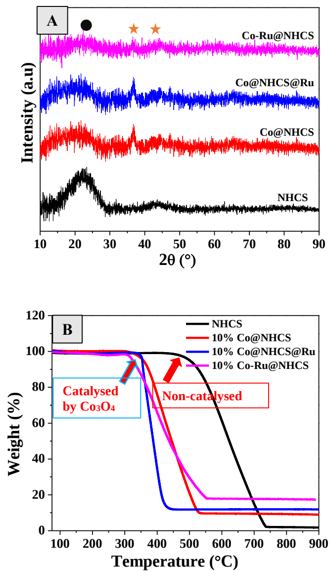
Figure 4.6 PXRD patterns (A) and TGA profiles (B) of catalysts. Carbon (●); \text{Co}_3\text{O}_4 (★)
