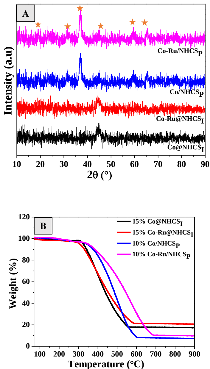
Figure 4.19 PXRd spectra (A) and TGA thermographs (B) of the catalysts. (I) in situ nitrogen doping; (P) post nitrogen doping. \text{Co}_3\text{O}_4 (★)
