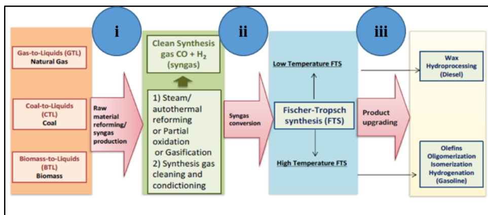
Figure 2.2 The schematic representation of the FTS process from feedstocks to products. 4
