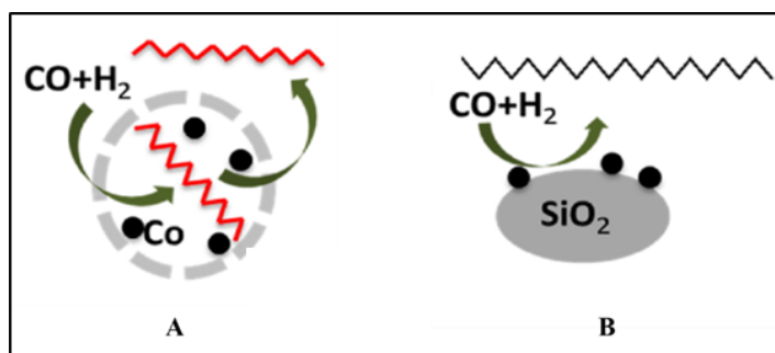
Figure 2.4 A FTS reaction occurring in a nanoreactor (A) and on a conventional oxidic support (B). 43
