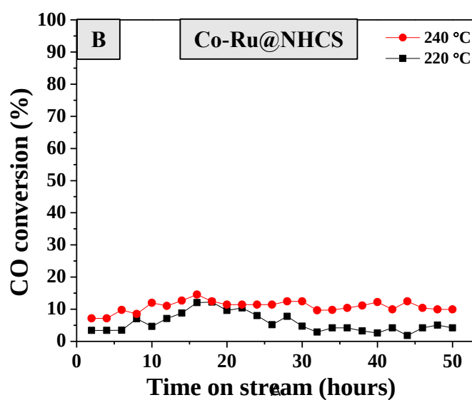
Figure 5.1 CO conversion (%) as a function of time in FTS of Co catalysts, (A) Co@NHCS, (B) Co-Ru@NHCS, at different FTS temperature.
