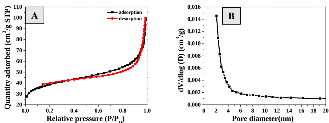
Figure 4.8 N 2 adsorption-desorption isotherm (A) and the corresponding adsorption pore size distribution (B) for the NHCSs.
