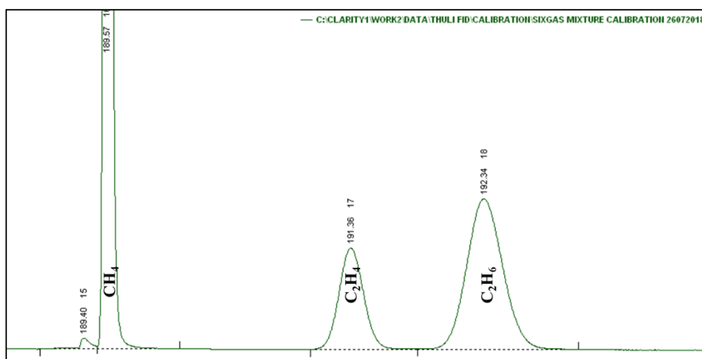
Figure 3.15 A GC-FID trace recorded during six gas mixture calibration.
