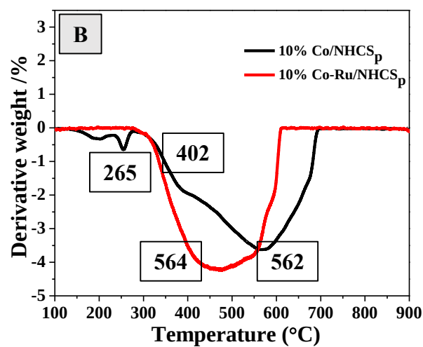
Figure 4S.6 Derivative TGA profiles of catalysts supported (A) inside the in situ nitrogen doped carbon and (B) on the post nitrogen doped carbon.
