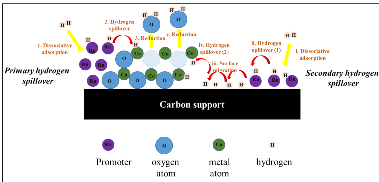
Figure 2.7 Diagrammatic presentation of the hydrogen spillover process, detailing primary and secondary spillover. 92
