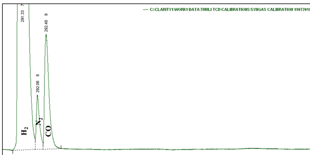
Figure 3.14 A GC-TCD trace recorded during syngas calibration.
