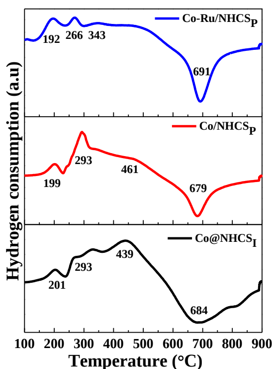
Figure 4.20 TPR profiles of supported catalysts. (i) in situ nitrogen doping; (p) post nitrogen doping.
