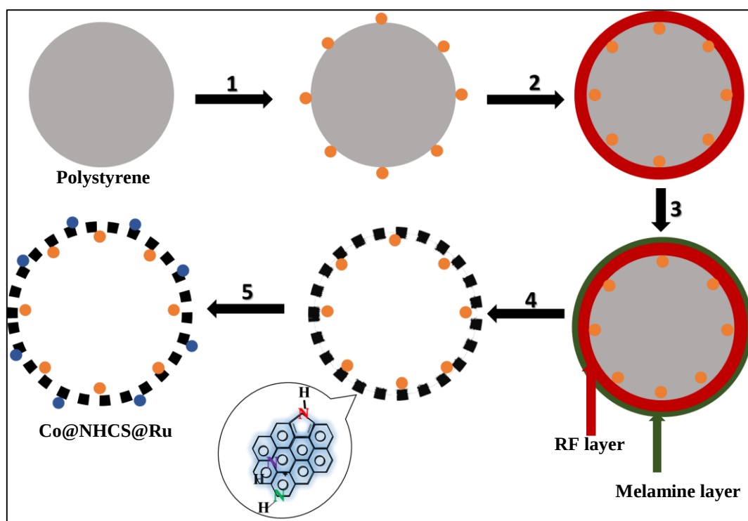
Figure 4.2 Schematic representation of the synthesis methodology. (1) metal (Ru and Co) onto a polystyrene template; (2) resorcinol-formaldehyde (carbon precursor) coating; (3) melamine (nitrogen precursor) coating, (4) template decomposition and annealing and (5) Ru metal loaded onto the carbon support.
