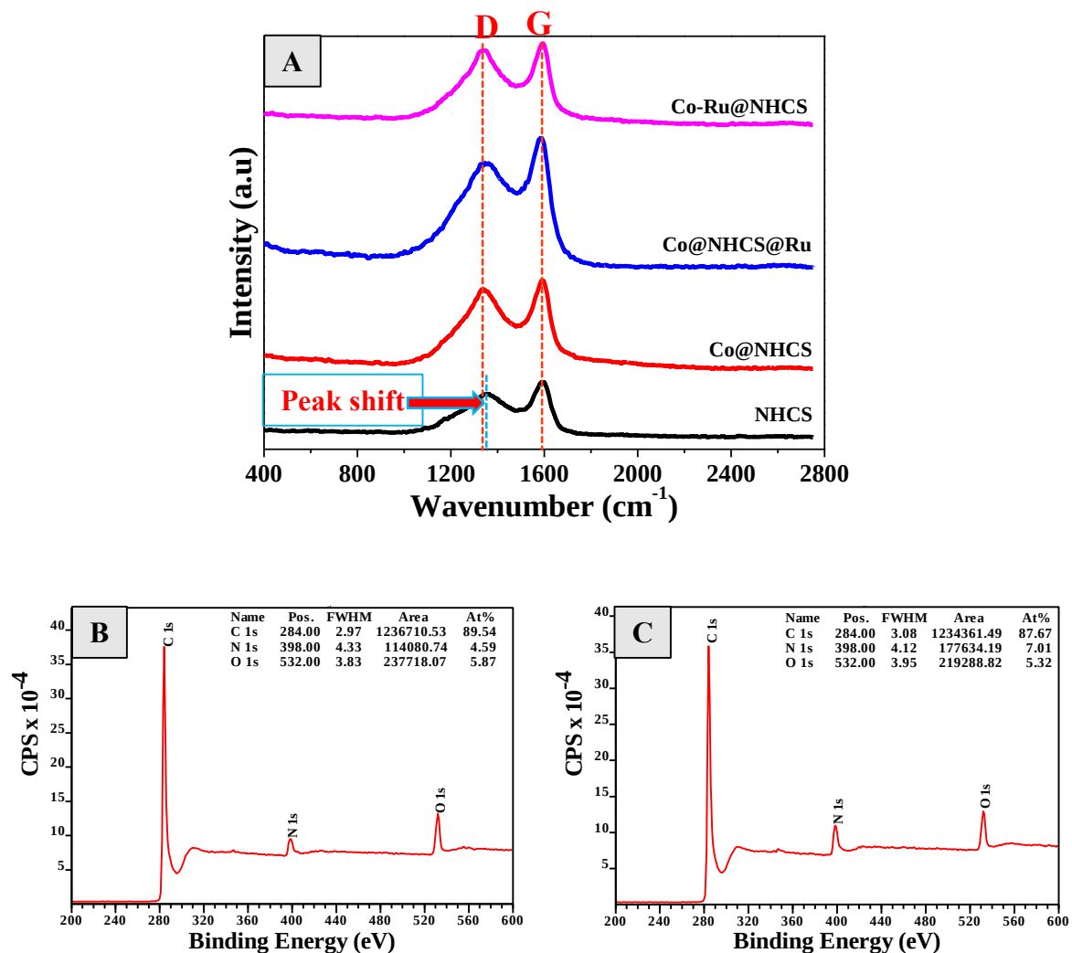
Figure 4.7 Raman spectra of catalysts (A) and survey XPS spectra of 10% Co@NHCS (B) and survey XPS spectra of NHCS (C).
