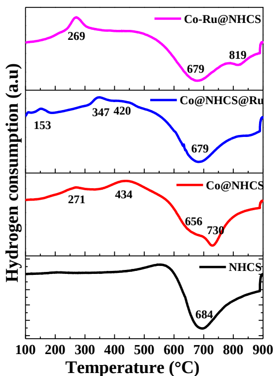
Figure 4.9 TPR reduction profiles for Co catalysts and catalyst support.
