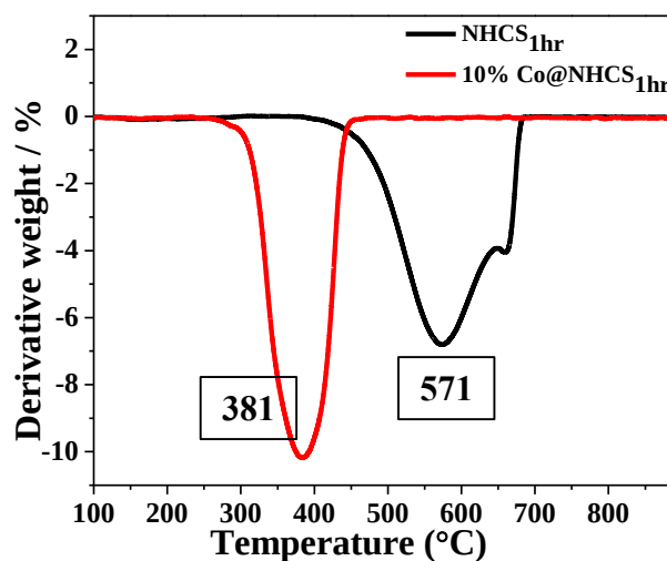
Figure 4S.4 Derivative TGA profiles of catalysts annealed for 1 hour.
