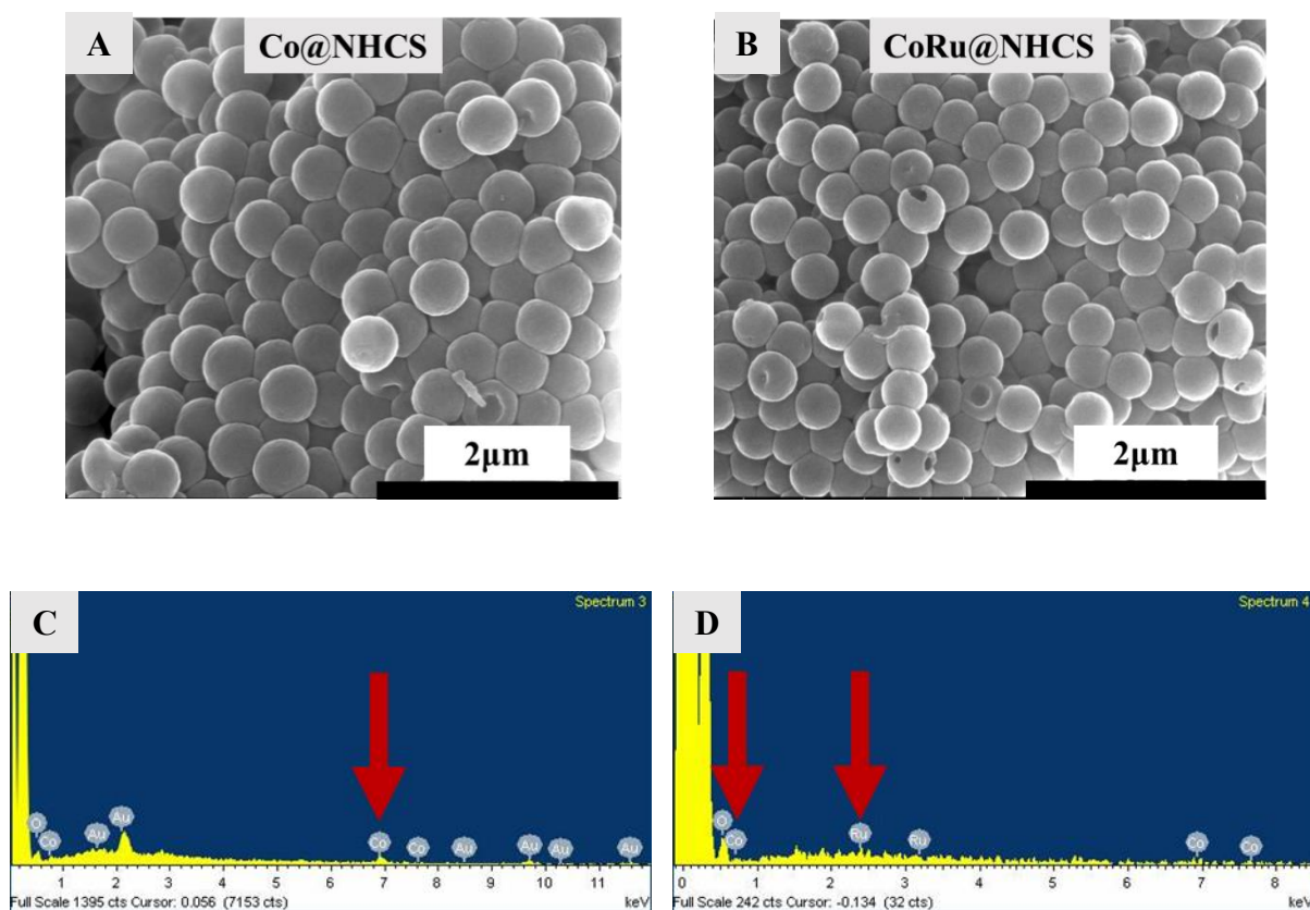
Figure 4S.1 SEM image with respective EDX spectrum of the catalysts, ( A and C ) 10% Co@NHCS; ( B and D ) 10% Co-Ru@NHCS.
