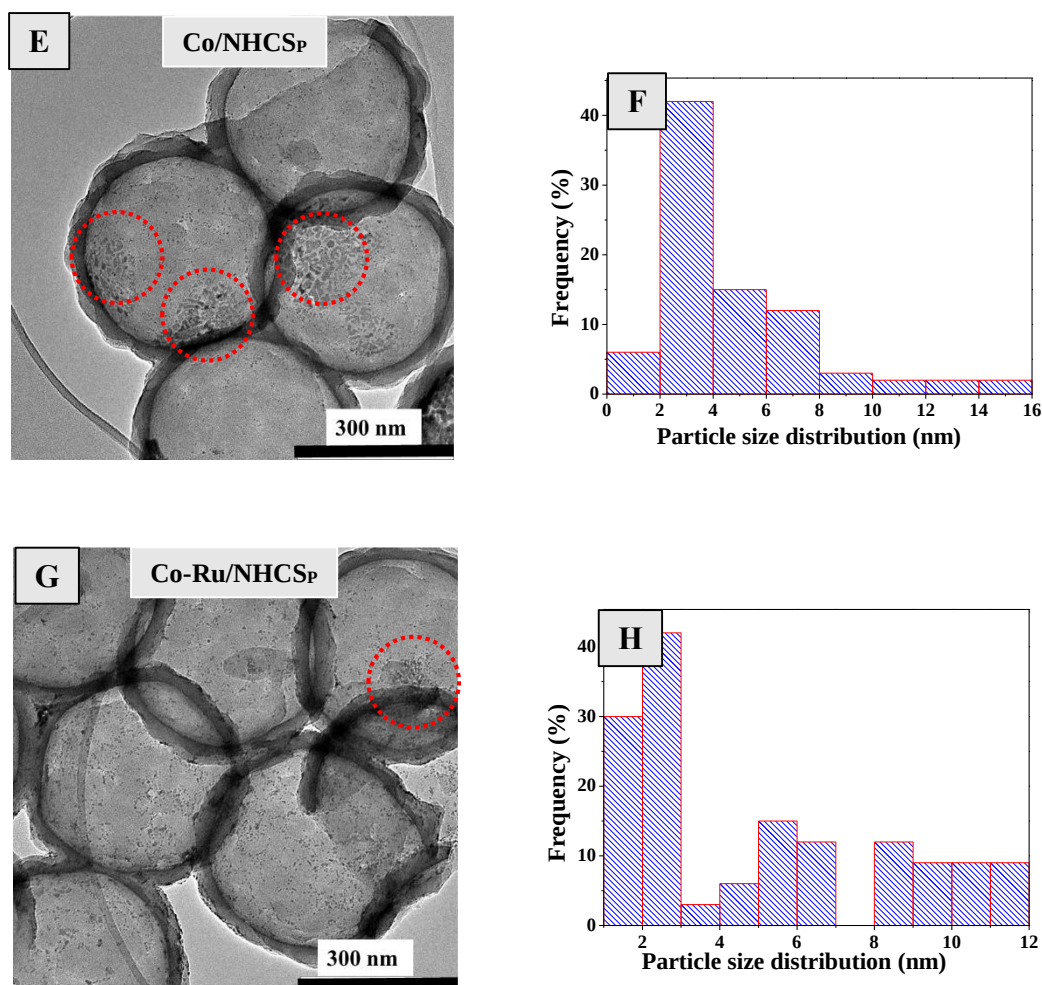
Figure 4.18 TEM images and particle size distributions of the supported catalysts. (i) in situ nitrogen doping; (p) post nitrogen doping.
