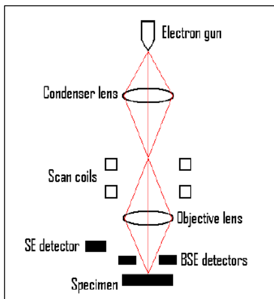
Figure 3.9 Schematic of main components found in a SEM instrument. 19
