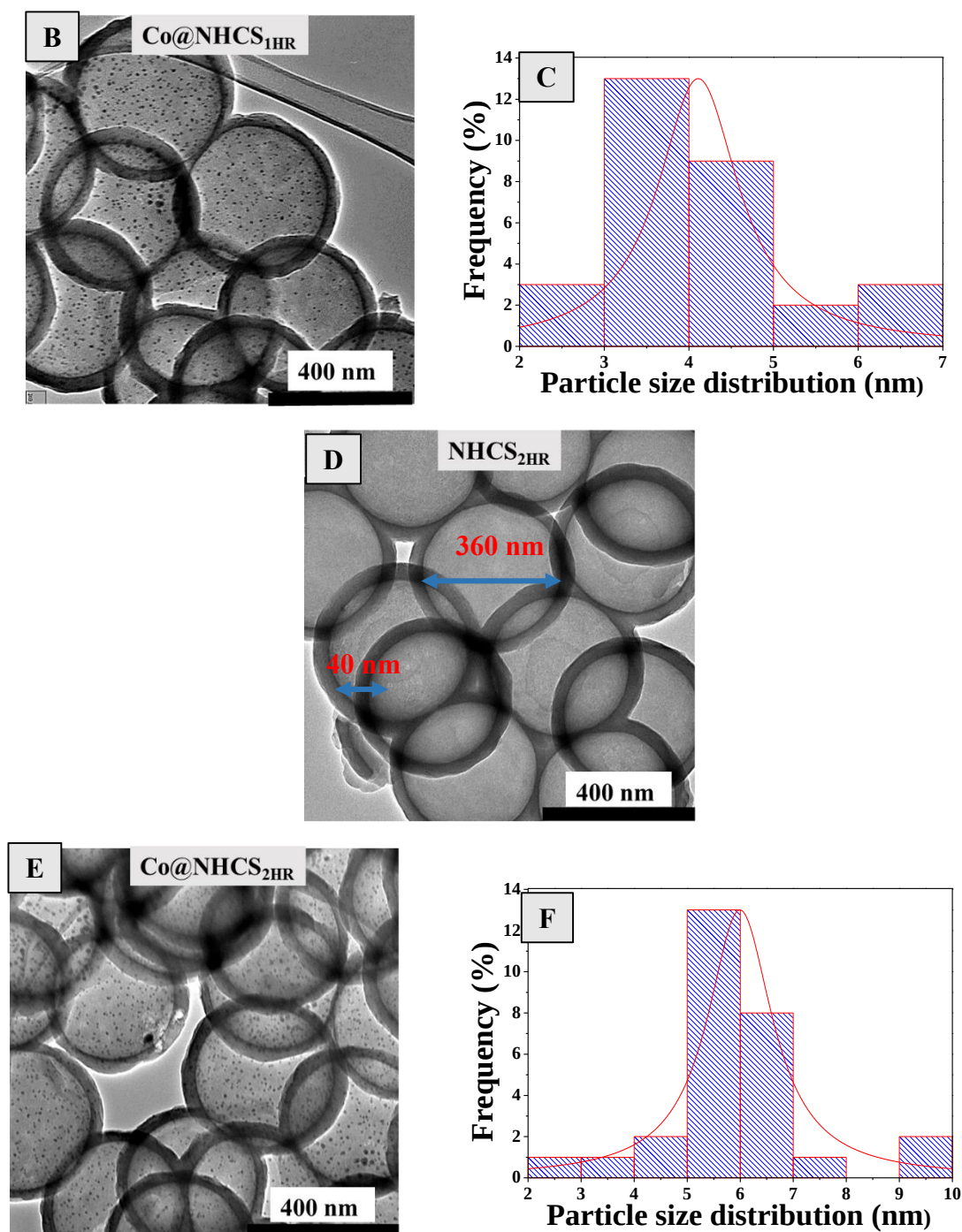
Figure 4.13 TEM images of catalyst supports and supported catalysts with corresponding metal particle size distribution when annealed for 1 hour ( A, B, C ) and 2 hours ( D, E, F ). (1hr) 1 hour annealing time; (2hr) 2 hours annealing time.
