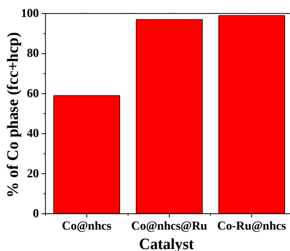
Figure 4.11 Degree of reduction for Co catalysts.
