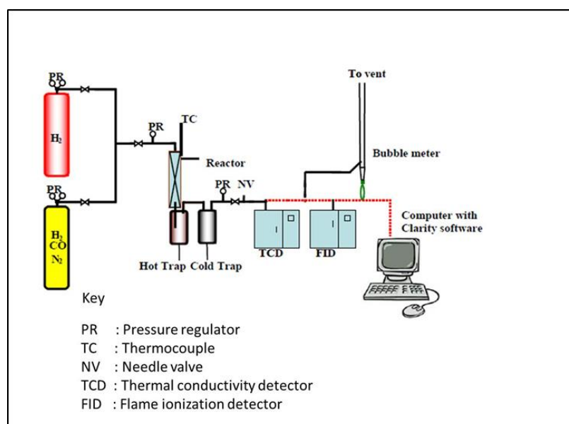
Figure 3.13 A schematic illustration of the rig reactor design. 24
