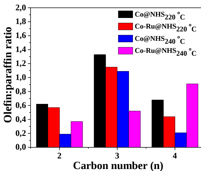
Figure 5.2 Olefin to paraffin ratio of Co catalysts, Co@NHCS and Co-Ru@NHCS, at different FTS temperature.
