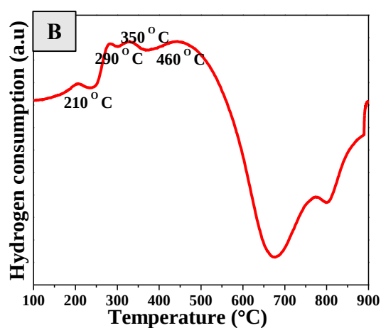
Figure 4S.7 TPR profiles of catalysts supported ( A &B ) of Co@NHCS 1hr .
