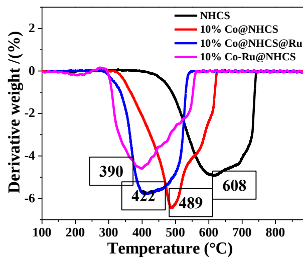
Figure 4S.2 Derivative TGA profiles of catalysts.
