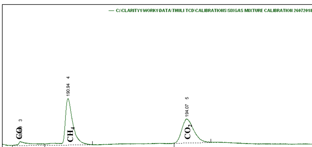
Figure 3.16 A GC-TCD trace recorded during six gas mixture calibration.
