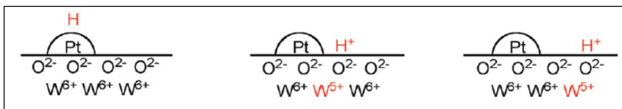
Figure 2.8 Schematic diagram of the production of the proton and electron upon adsorption of H 2 on Pt and subsequent spillover of H atoms to the reducible WO 3 support. 95, 96
