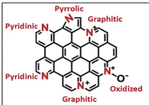
Figure 2.6 Nitrogen configurations incorporated into the carbon matrix. 23
