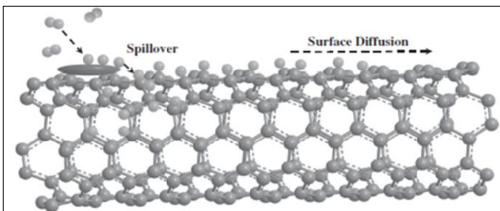
Figure 2.10 Hydrogen spillover on carbon supports through surface diffusion. 3
