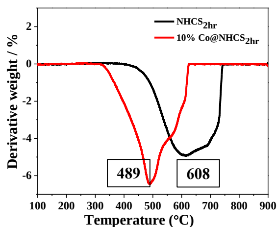
Figure 4S.5 Derivative TGA profiles of catalysts annealed for 2 hours.
