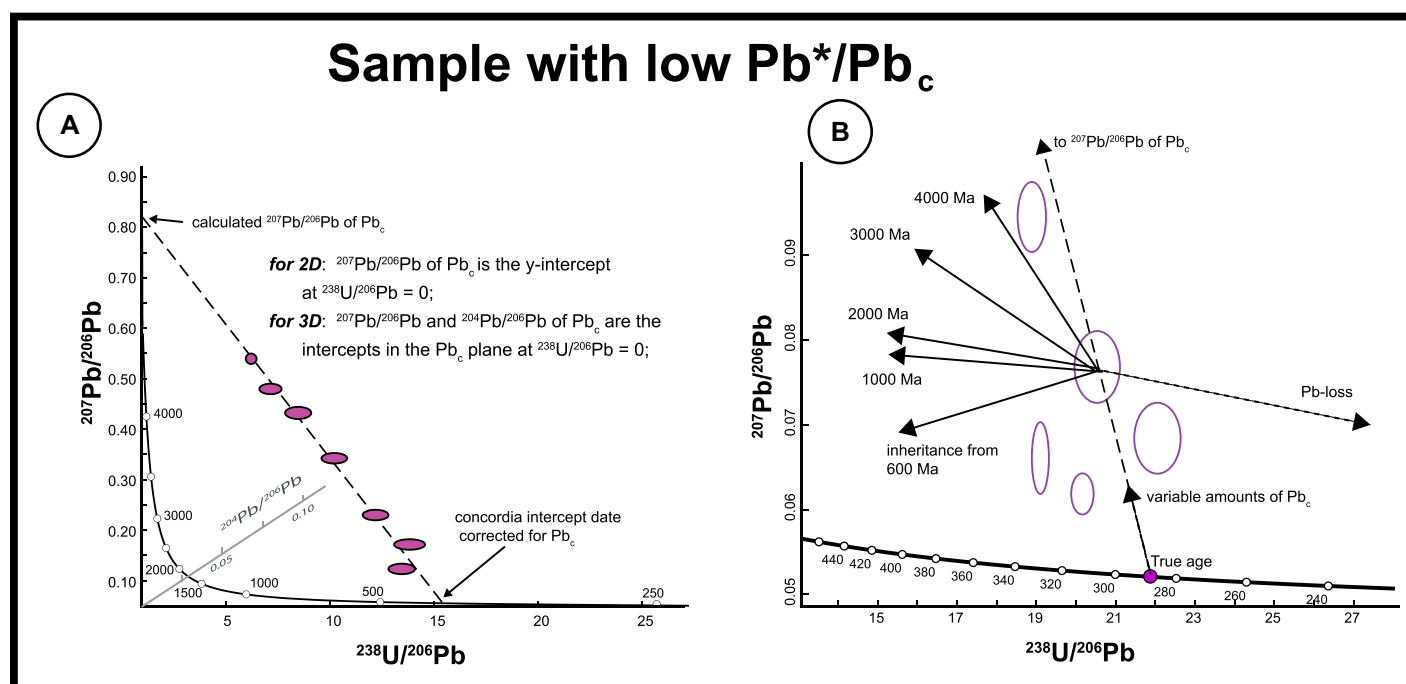
Figure 4. Impact of different types of system complexity on U-Pb dates from minerals with high abundance of common Pb (Pb c ) in Tera-Wasserburg Concordia plots. (A) Standard 3-D Tera-Wasserburg diagram illustrating means of calculating an age and the initial ^{207}\text{Pb}/^{206}\text{Pb} and ^{204}\text{Pb}/^{206}\text{Pb} isotope compositions of Pb c for a set of low Pb*/Pb c analyses. (B) Enlargement of the Pb* intercept area of a standard 3-D Tera-Wasserburg diagram illustrating the effects of various sources of scatter in low Pb*/Pb c minerals (inherited Pb components of different age, variable amounts of Pb c , and loss of Pb*).
