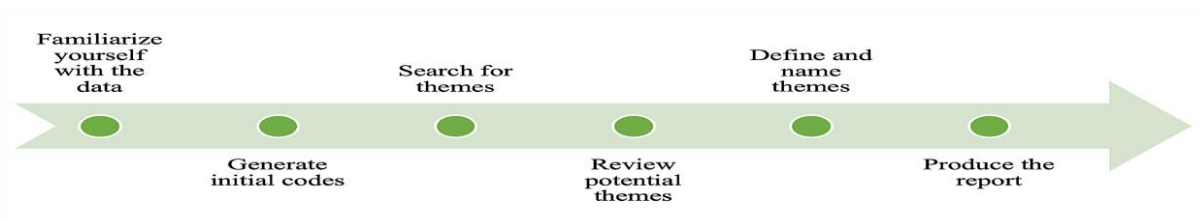
Figure 6.1: Thematic data analysis steps
