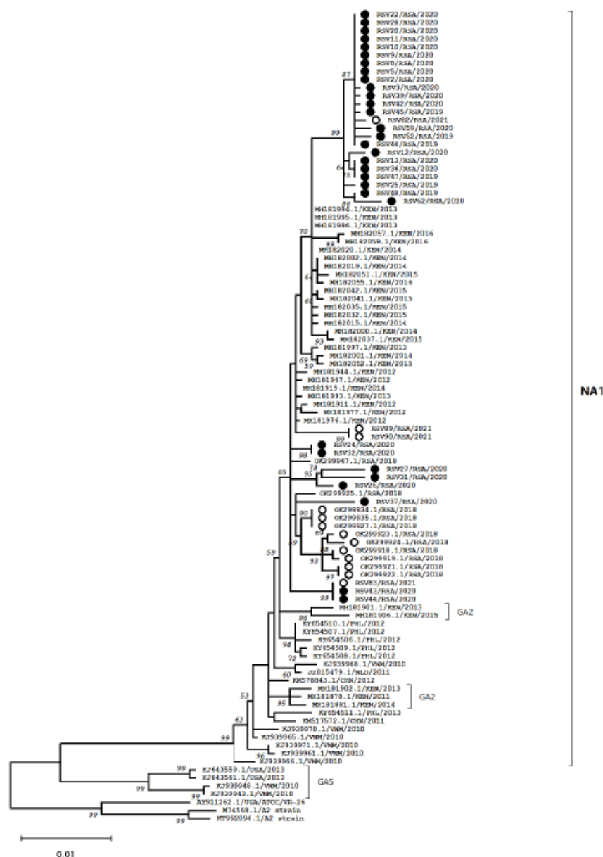
Figure 1. Maximum-likelihood phylogenetic tree based on the 1716 bp long F gene sequences of RSV-A strains from South Africa that circulated in 2019 and 2020 (filled black circles). Reference South African strains are indicated by open black circles. A2 Long strains were used as root. Genotype classification used are based on G protein gene sequence genotypes assigned to reference sequences.
