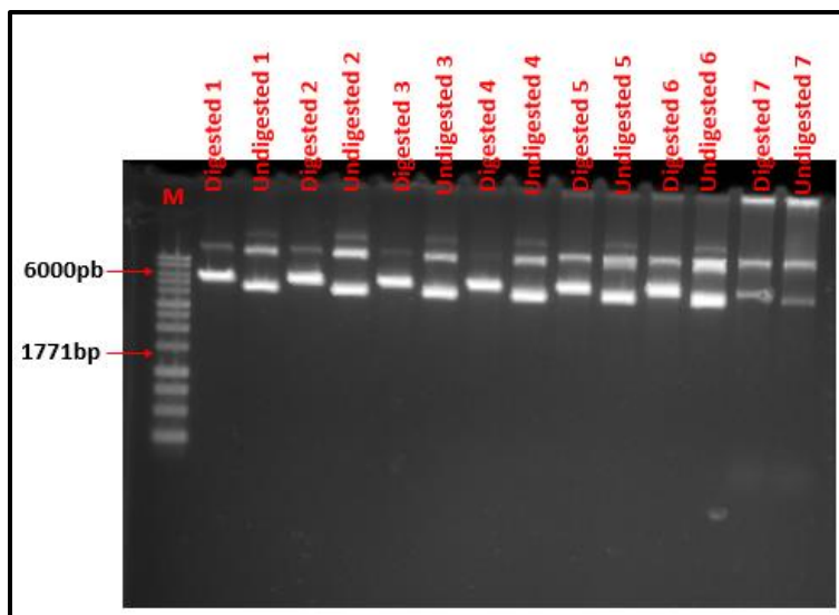
Figure 3.3 A 0.6% agarose gel electrophoresis picture for double restriction digestion of the purified plasmid DNA.
