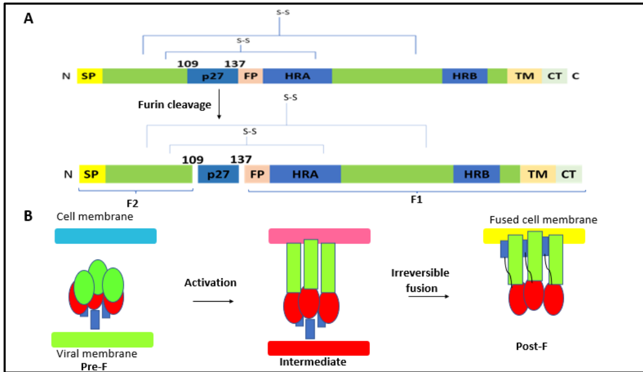
Figure 1.3. Activation and refolding of RSV pre-F into post-F conformation. (A) The biologically inactive F0 precursor is post-translationally cleaved by furin proteases at amino acids 109 and 137, to form two fragments (F2 and F1), resulting in the release of p27 peptide that separates C-terminus F1 and N-terminus F2. (B) Upon triggering, pre-F partially refolds and integrates its hydrophobic F peptide into the host cell membrane to form a pre-hairpin intermediate. The refolding of the pre-hairpin intermediate into the post-F conformation facilitates further viral F protein-host cell membrane fusion, adapted from [31].
