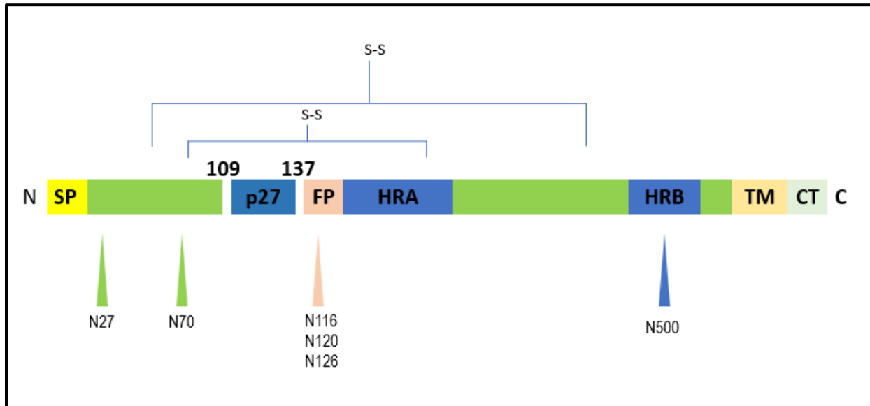
Figure 1.2. Structure of RSV F protein. The F protein is made of a cytoplasmic tail, the transmembrane domain, the two heptad-repeat regions (HR-A and HR-B), a fusion peptide (FP), and the SP. The furin cleavage sites (109 and 137) are indicated. Approximate positions of the N-glycosylation sites are shown by arrows, adapted from [16].
