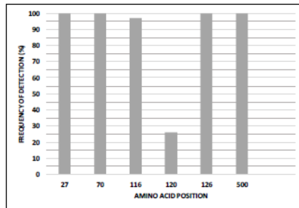
Figure 2. A graphic representation of N-glycosylation site positions across the South African RSV F protein sequences and the frequency of detection of NX(T/S)X sequons, 2019 to 2020.
