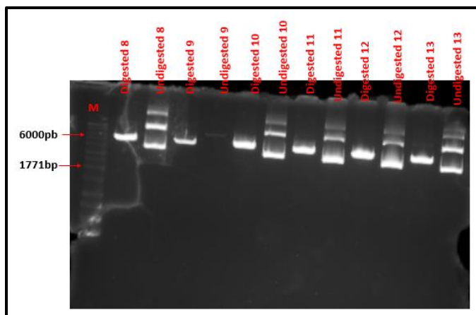
Figure 3.4. A 0.6% agarose gel electrophoresis picture for double restriction digestion of the purified plasmid DNA.
