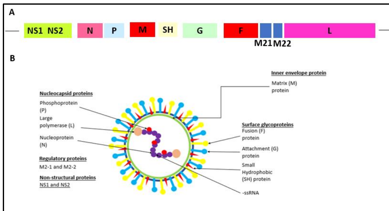
Figure 1.1. (A) RSV gene arrangement. (B) RSV virion structure. The virus consists of three envelope proteins, the G, F and SH proteins. The M protein is located below the envelope as the inner envelope protein. The nucleocapsid is made of -ssRNA that is encapsulated by the N protein. Associated with the nucleocapsid are the L protein and the P protein, adapted from [12].
