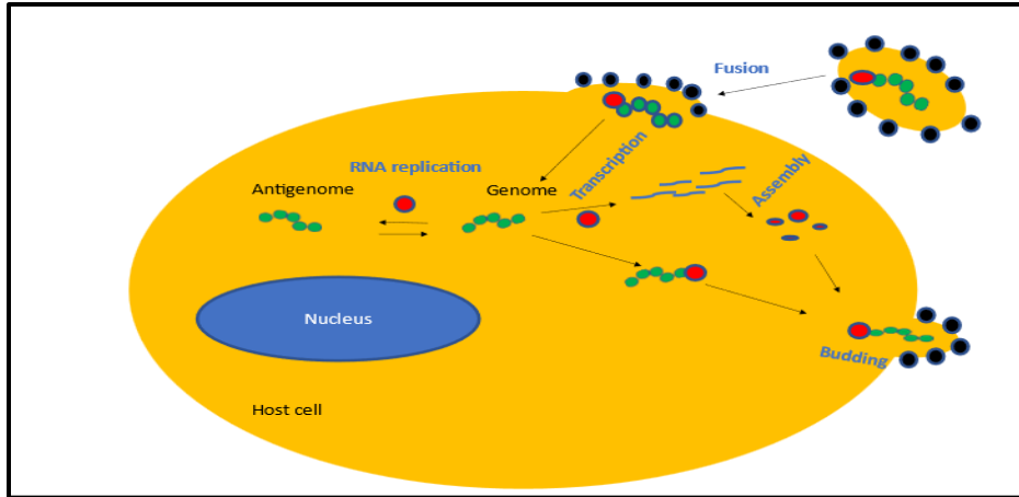
Figure 1.4. RSV life cycle. Firstly, viral-host cell attachment and fusion occurs when the virus enters the cell . The viral genome is released to start . Transcription occurs and it is followed by assembly and budding to generate new virions,adapted from [50].
