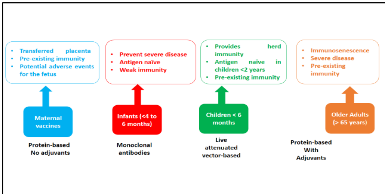
Figure 1.5. Summary of RSV vaccine types in development and clinical trials with target populations also indicated, adapted from [78].
