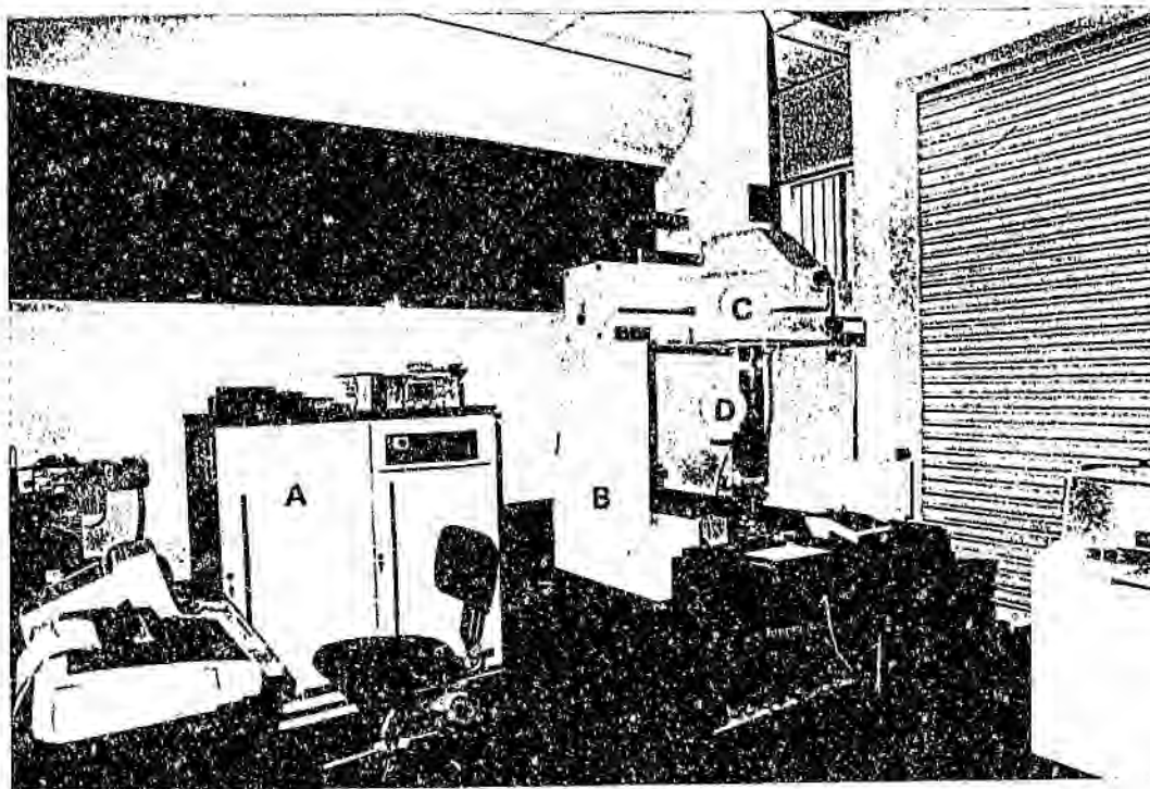
Figure 19. Three-dimensional coordinate measuring centre. (A) Minicomputer which controls the measuring machine (B) Travelling bridge (x-axis) (C) Horizontal carriage (y-axis) (D) Vertical ram (z-axis)
