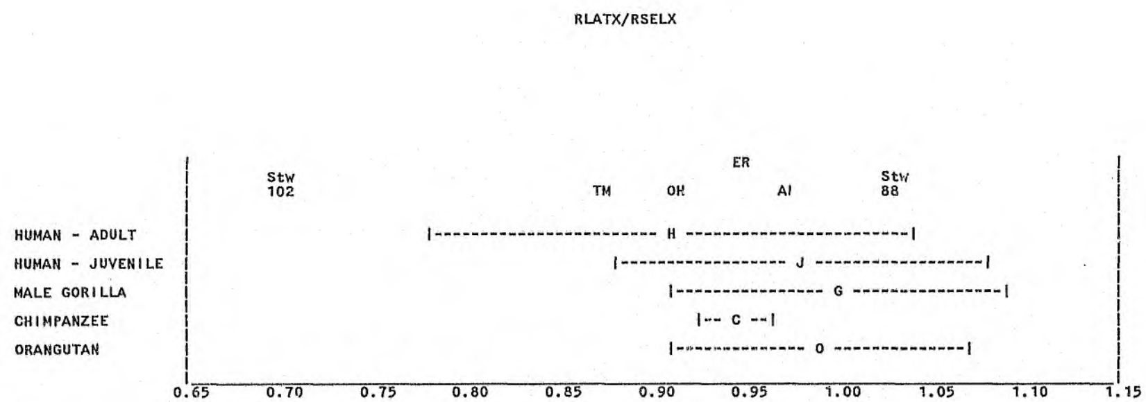
Figure 54. RLATX/RSELX - Samples of Modern Humans and Great Apes (Mean \pm Standard Deviation) and Fossil Specimens.
