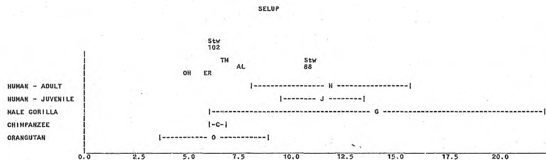
Figure 48. SELUP - Samples of Modern Humans and Great Apes (Mean \pm Standard Deviation) and Fossil Specimens.
