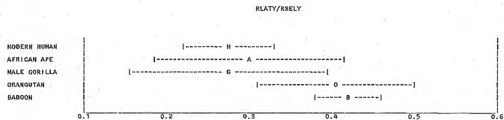
Figure 38. RLATY/RSELY - Samples of Extant Primates (Mean \pm Standard Deviation).
