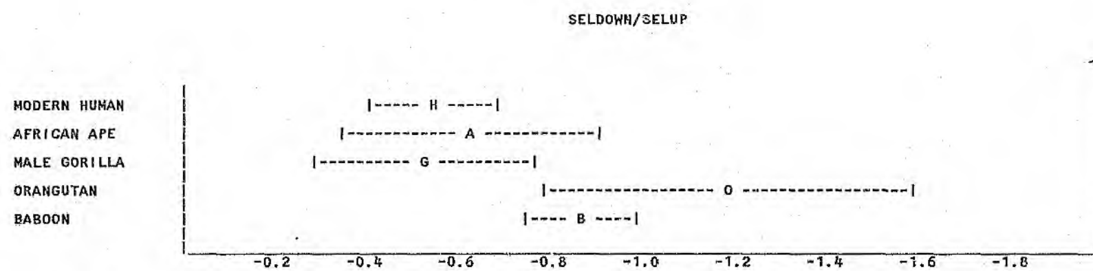
Figure 40. SELDOWN/SELUP - Samples of Extant Primates (Mean \pm Standard Deviation).
