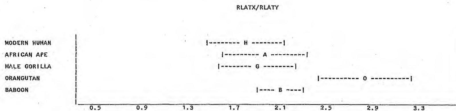
Figure 41. RLATX/RLATY - Samples of Extant Primates (Mean \pm Standard Deviation).
