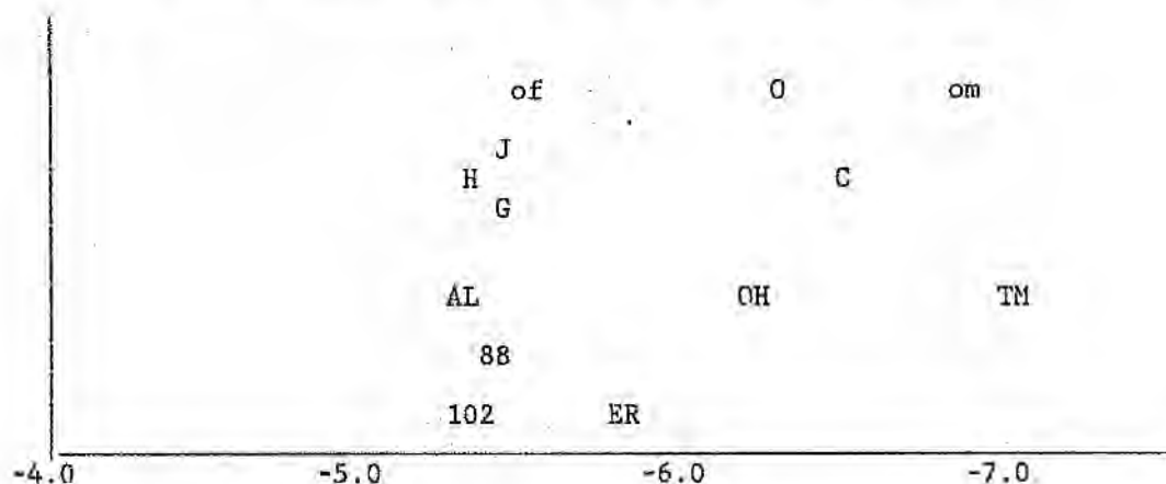
Figure 61. Average of Sample Means of RMEDX, SELDOWN and RLATX. Samples of Extant Primates (H = modern human adults, J = modern human juveniles, G = male gorillas, C = chimpanzees, O = orangutans, of = female orangutans, om = male orangutans) and Fossil Specimens (OH = OH 8, TM = TM 1517, ER = KNM ER-813, AL = AL 288-1as, 88 = Stw 88, 102 = Stw 102).
