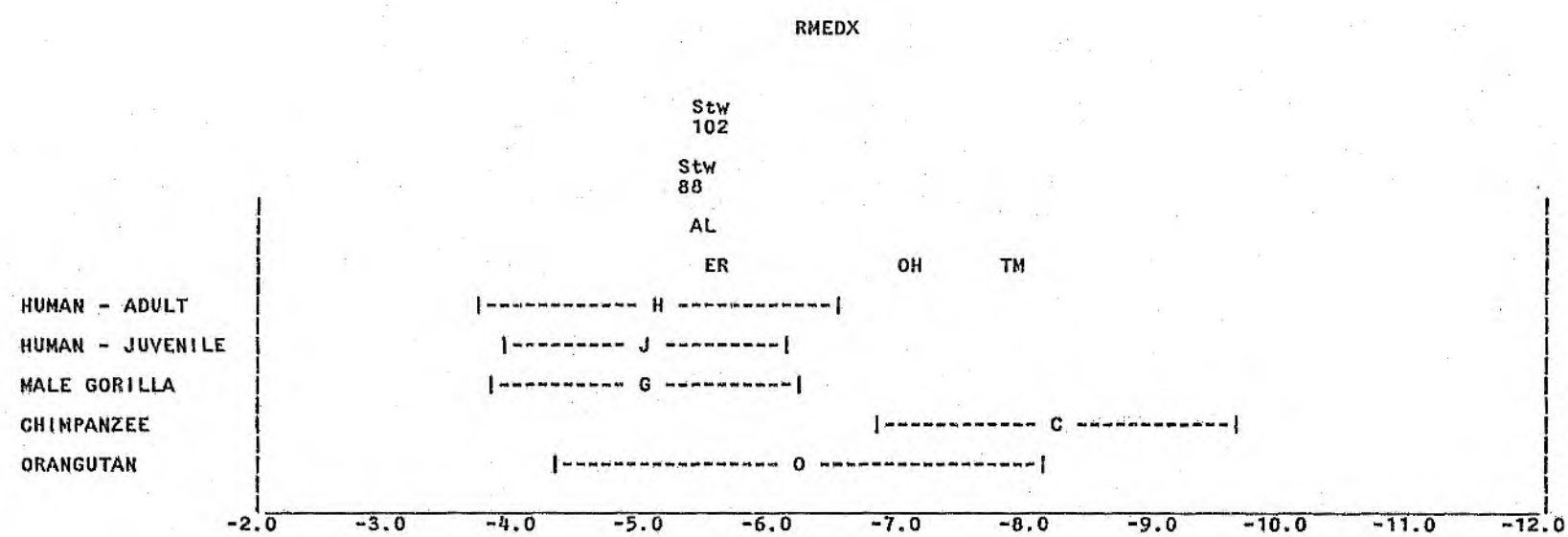
Figure 44. RMEDX - Samples of Modern Humans and Great Apes (Mean \pm Standard Deviation) and Fossil Specimens.
