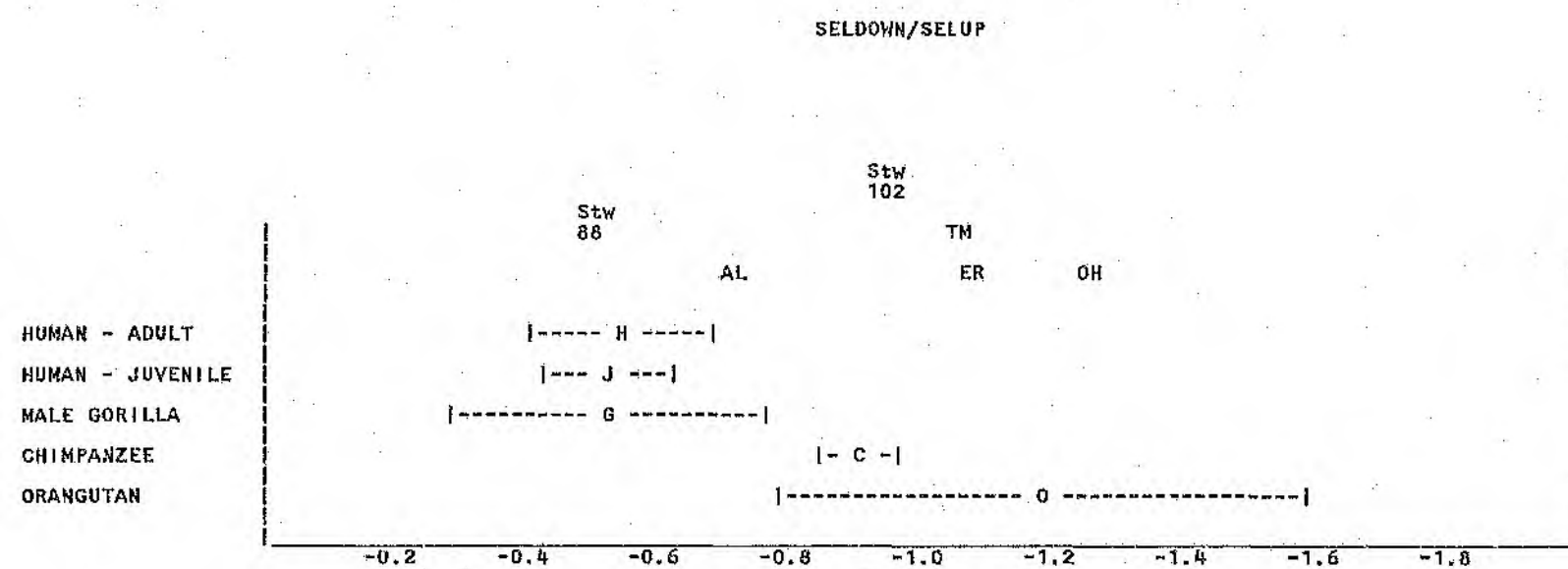
Figure 59. SELDOWN/SELUP - Samples of Modern Humans and Great Apes (Mean \pm Standard Deviation) and Fossil Specimens.
