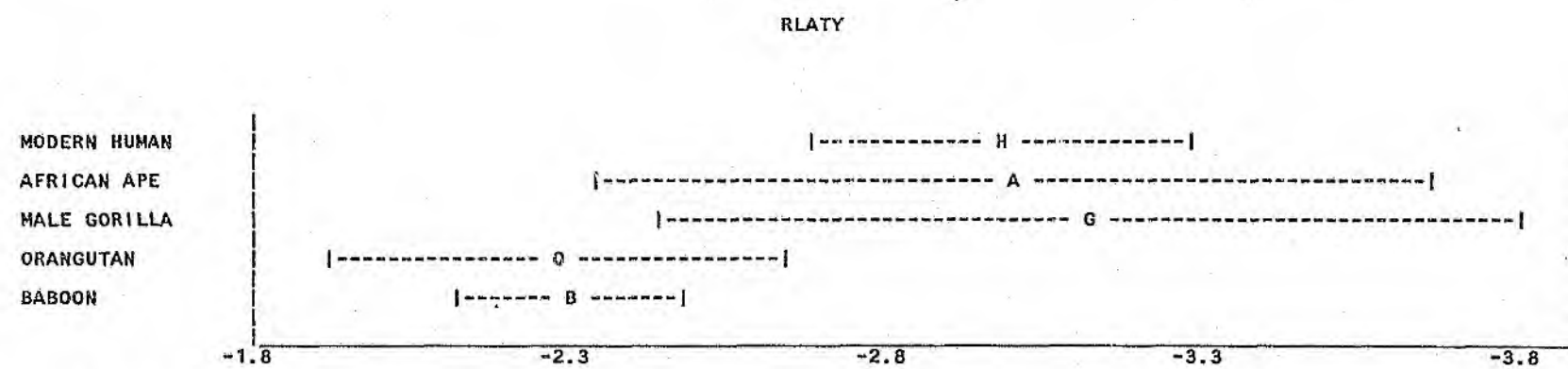
Figure 30. RLATY - Samples of Extant Primates (Mean \pm Standard Deviation).
