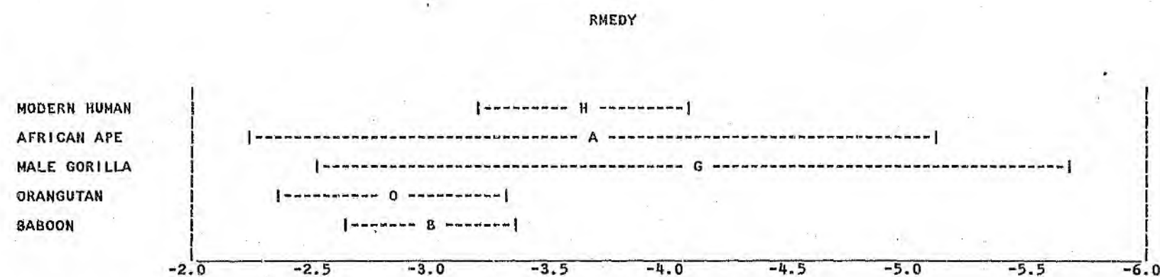
Figure 28. RMEDY - Samples of Extant Primates (Mean \pm Standard Deviation).
