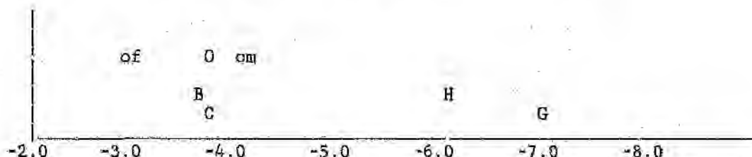
Figure 43. Average of Sample Means of RMEDY, SELUP and RLATY. Samples of Extant Primates (B = baboons, H = modern humans, G = male gorillas, C = chimpanzees, O = orangutans, of = female orangutans, om = male orangutans).
