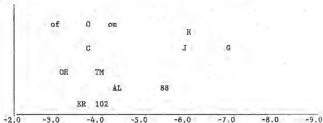
Figure 63. Average of Sample Means of RMEDY, SELUP and RLATY. Samples of Extant Primates (H = modern human adults, J = modern human juveniles, G = male gorillas, C = chimpanzees, O = orangutans, of = female orangutans, om = male orangutans) and Fossil Specimens (OH = OH 8, TM = TM 1517, ER = KNM ER-813, AL = AL 288-las, 88 = Stw 88, 102 = Stw 102).
