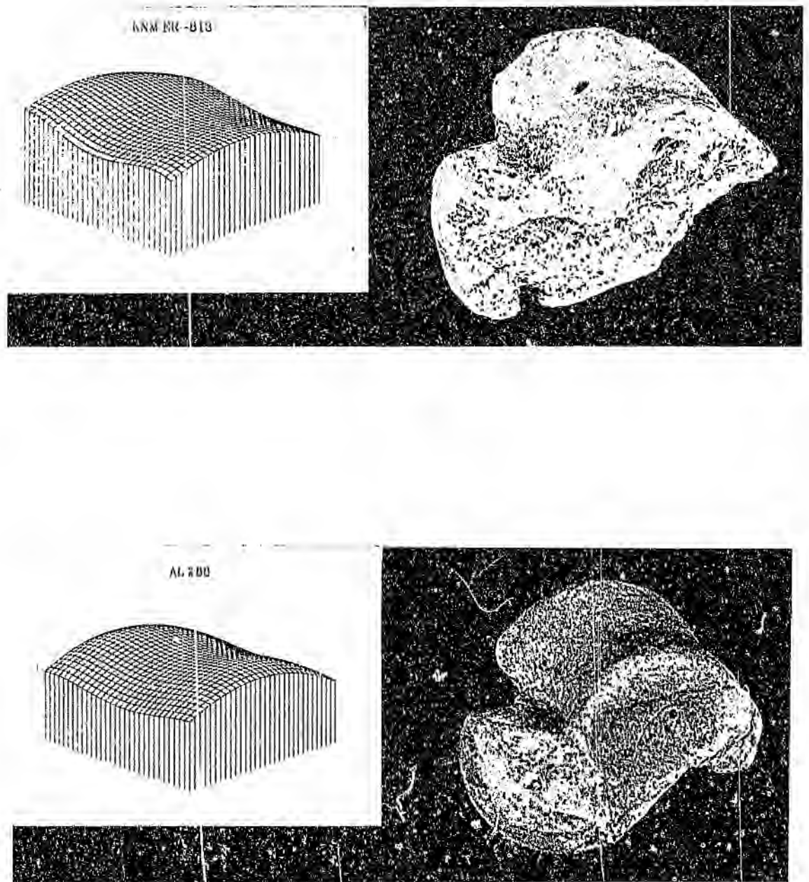
Figure 9. B. Early hominid talii from East Turkana (KNM ER-813) and Hadar (AL 288) (medial view, larger than natural size).
