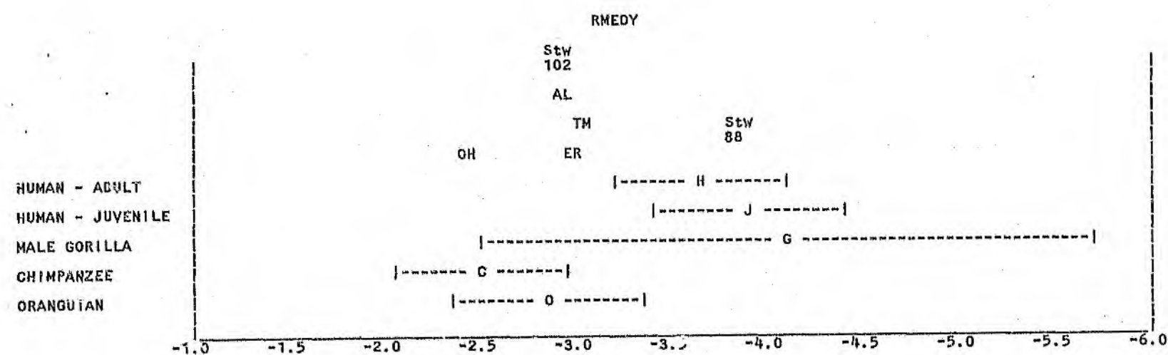
Figure 47. RMEY - Samples of Modern Humans and Great Apes (Mean \pm Standard Deviation) and Fossil Specimens.
