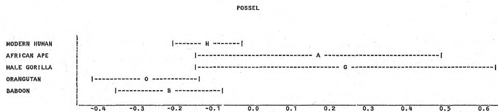
Figure 31. POSSEL - Samples of Extant Primates (Mean \pm Standard Deviation).
