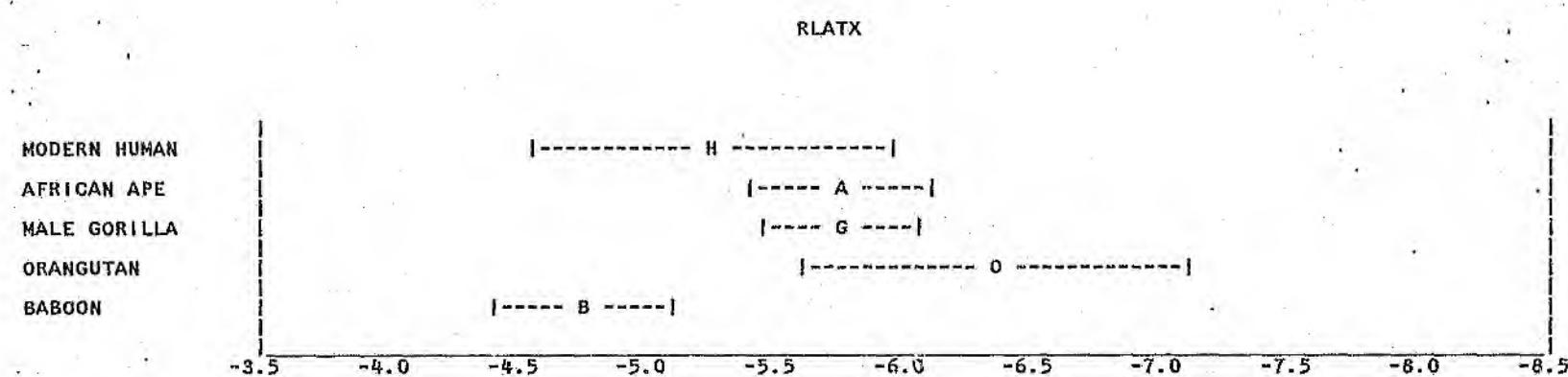
Figure 27. RLATX - Samples of Extant Primates (Mean \pm Standard Deviation).
