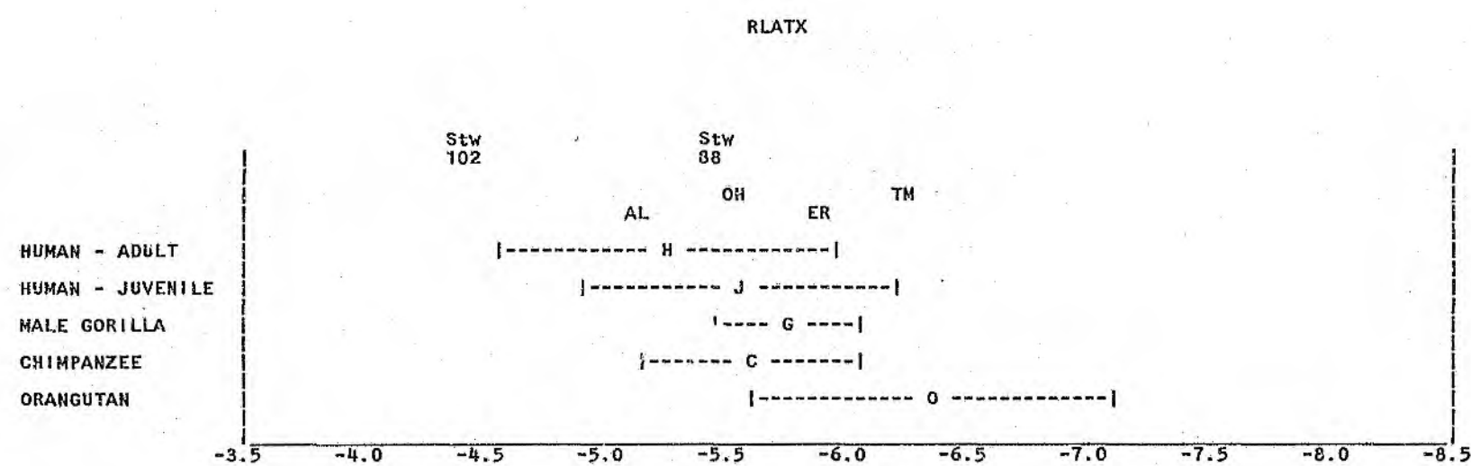
Figure 46. RLATX - Samples of Modern Humans and Great Apes (Mean \pm Standard Deviation) and Fossil Specimens.
