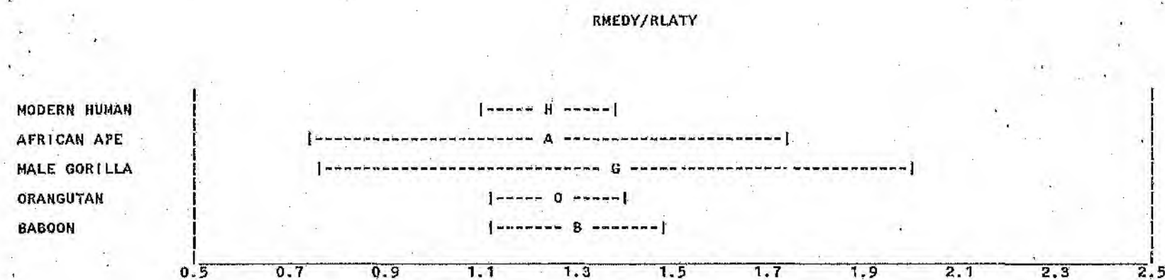
Figure 36. RMEDY/RLATY - Samples of Extant Primates (Mean \pm Standard Deviation).
