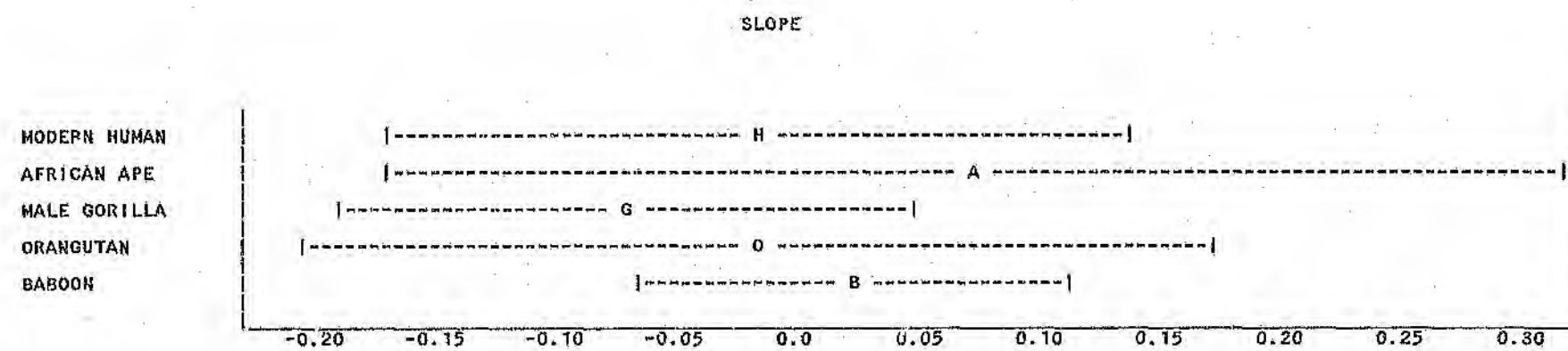
Figure 32. SLOPE - Samples of Extant Primates (Mean \pm Standard Deviation).
