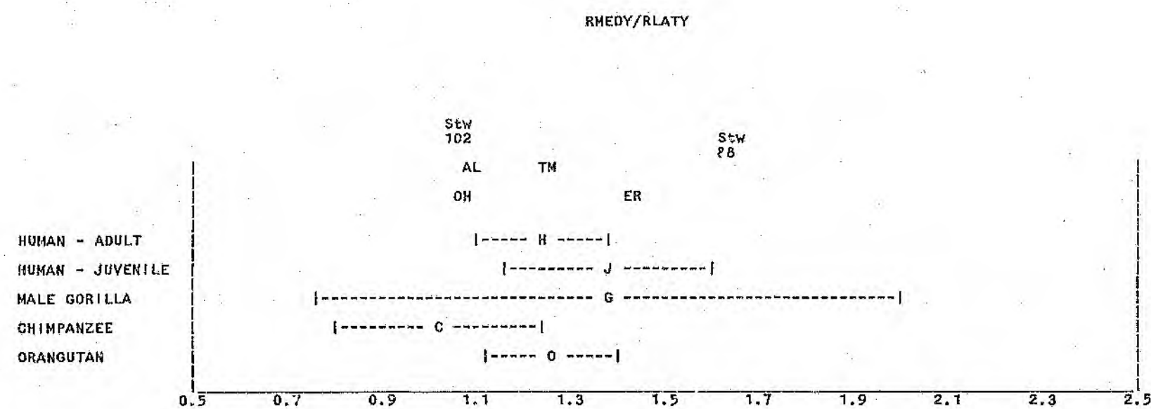
Figure 55. RMDY/RLATY - Samples of Modern Humans and Great Apes (Mean \pm Standard Deviation) and Fossil Specimens.
