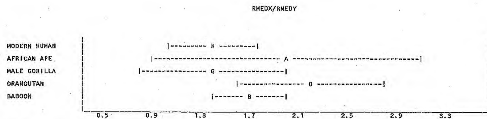
Figure 39. RMEDX/RMEDY - Samples of Extant Primates (Mean \pm Standard Deviation).
