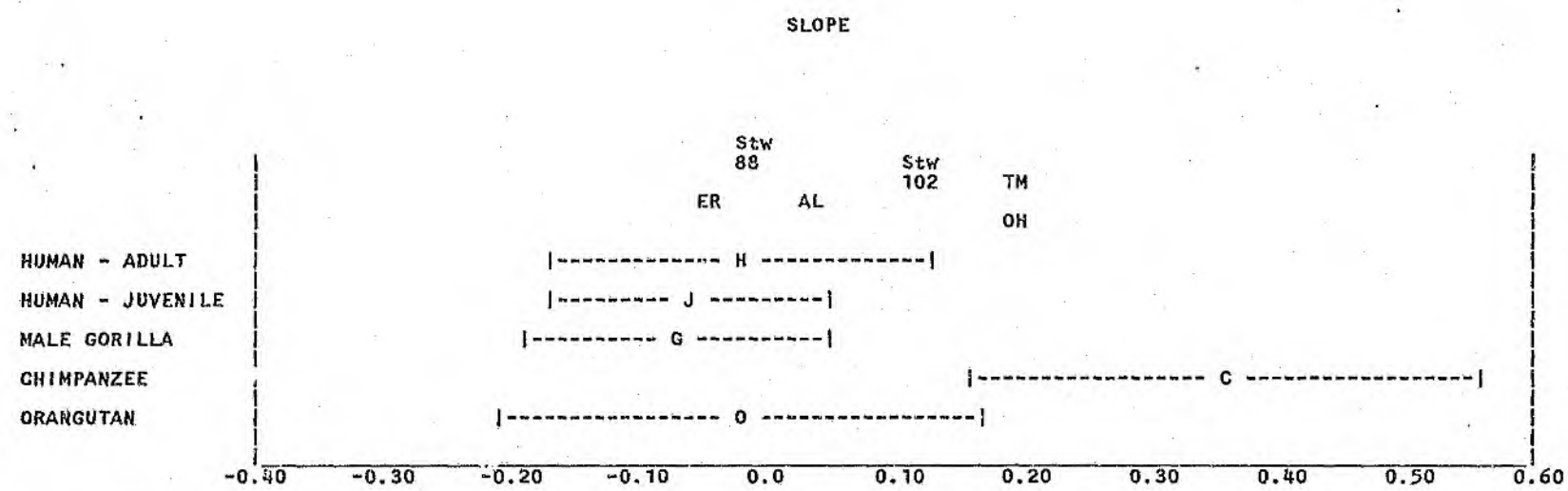
Figure 51. SLOPE - Samples of Modern Humans and Great Apes (Mean \pm Standard Deviation) and Fossil Specimens.
