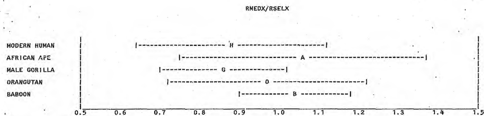
Figure 34. RMDX/RSELX - Samples of Extant Primates (Mean \pm Standard Deviation).
