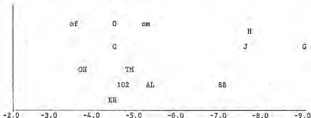
Figure 64. Average of Sample Means of RMEDY and SELUP. Samples of Extant Primates (H = modern human adults, J = modern human juveniles, G = male gorillas, C = chimpanzees, O = orangutans, of = female orangutans, om = male orangutans) and Fossil Specimens (OH = OH 8, TM = TM 1517, ER = KNM ER-813, AL = AL 288-las, 88 = Stw 88, 102 = Stw 102).
