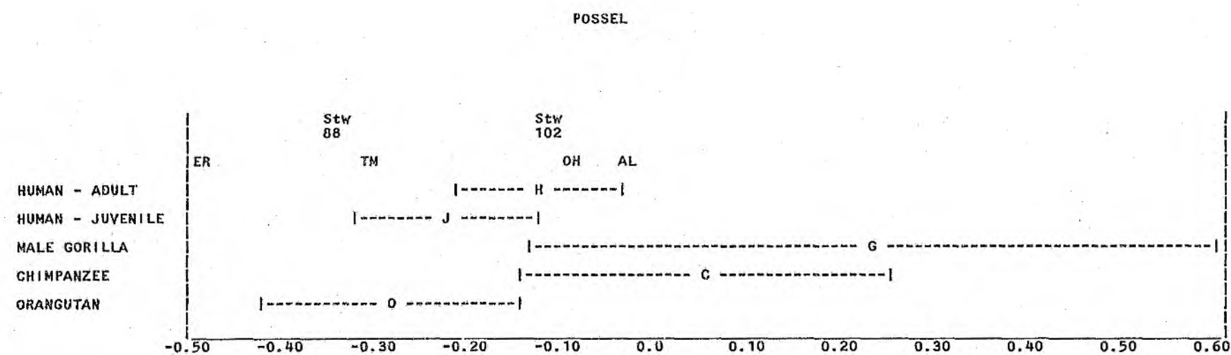
Figure 50. POSSEL - Samples of Modern Humans and Great Apes (Mean \pm Standard Deviation) and Fossil Specimens.
