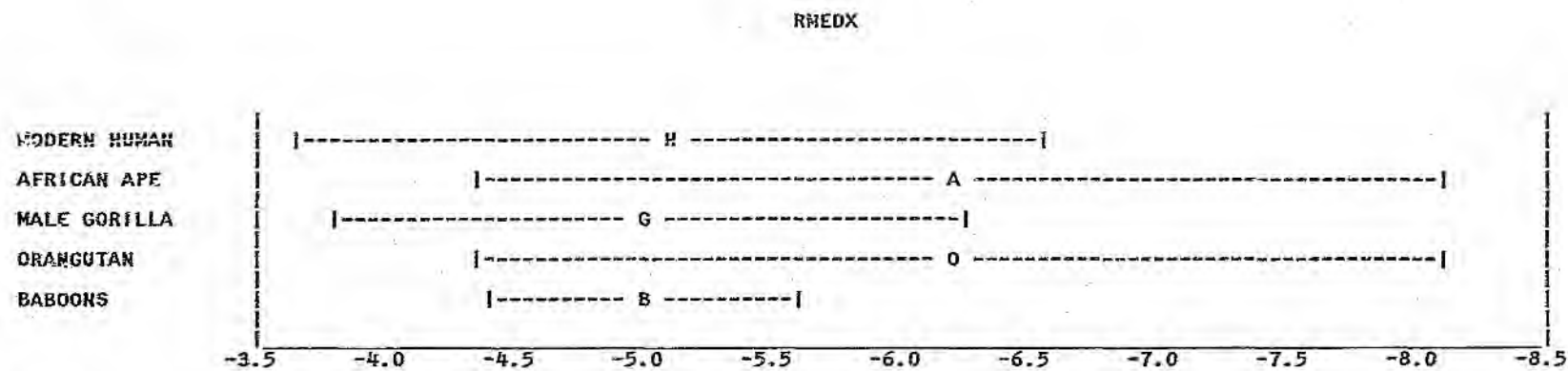
Figure 25. RMEDX - Samples of Extant Primates (Mean \pm Standard Deviation).
