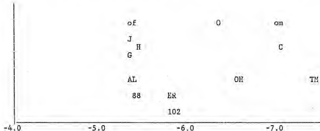
Figure 62. Average of Sample Means of RMEDX and SELDOWN. Samples of Extant Primates (H = modern human adults, J = modern human juveniles, G = male gorillas, C = chimpanzees, O = orangutans, of = female orangutans, om = male orangutans) and Fossil Specimens (OH = OH 8, TM = TM 1517, ER = KNM ER-813, AL = AL 288-1as, 88 = Stw 88, 102 = Stw 102).
