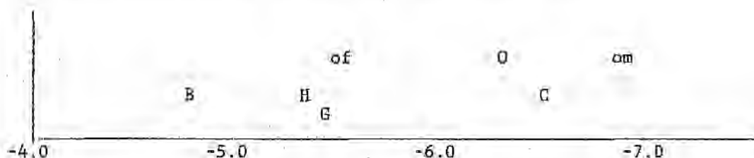
Figure 42. Average of Sample Means of RMEDX, SELDOWN and RLATX. Samples of Extant Primates (B = baboons, H = modern humans, G = male gorillas, C = chimpanzees, O = orangutans, of = female orangutans, om = male orangutans).
