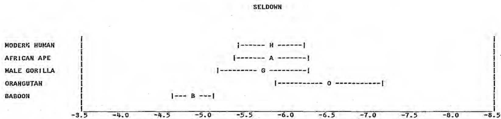
Figure 26. SELDOWN - Samples of Extant Primates (Mean \pm Standard Deviation).
