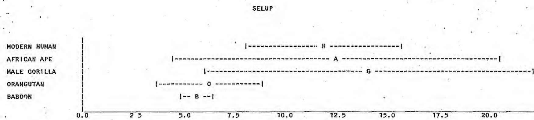
Figure 29. SELUP - Samples of Extant Primates (Mean \pm Standard Deviation).
