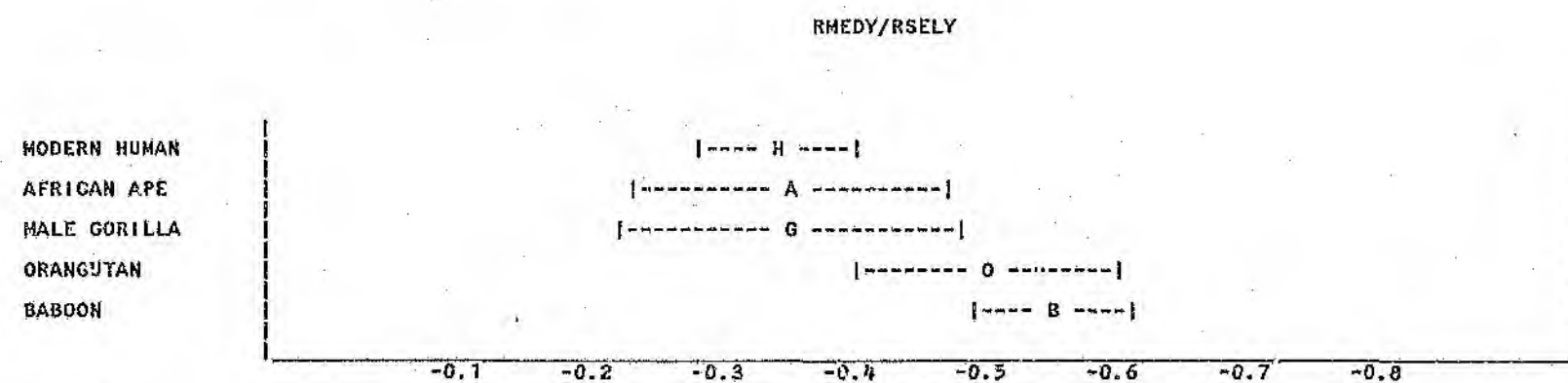
Figure 37. RMEDY/RSELY - Samples of Extant Primates (Mean \pm Standard Deviation).
