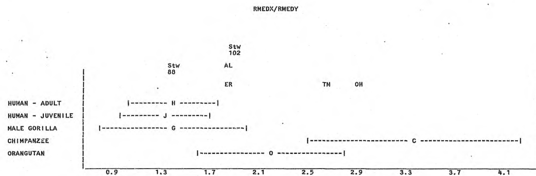
Figure 58. RMEDX/RMEDY - Samples of Modern Humans and Great Apes (Mean \pm Standard Deviation) and Fossil Specimens.
