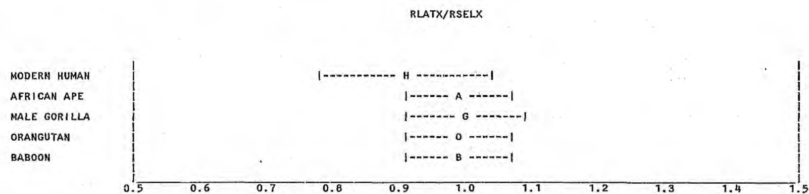
Figure 35. RLATX/RSELX - Samples of Extant Primates (Mean \pm Standard Deviation).
