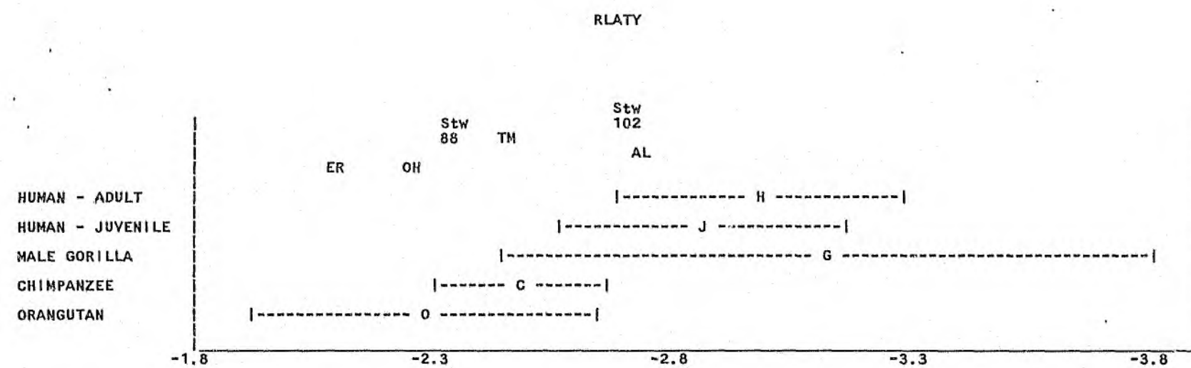
Figure 49. RLATY - Samples of Modern Humans and Great Apes (Mean \pm Standard Deviation) and Fossil Specimens.
