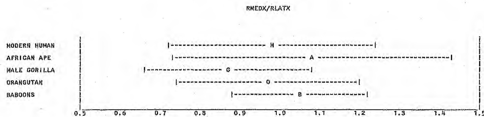
Figure 33. RMEDX/RLATX - Samples of Extant Primates (Mean \pm Standard Deviation).
