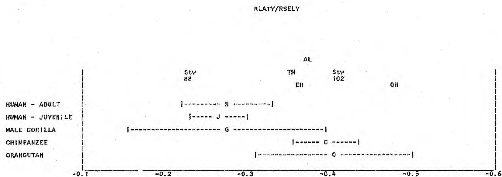
Figure 57. RLATY/RSELY - Samples of Modern Humans and Great Apes (Mean \pm Standard Deviation) and Fossil Specimens.
