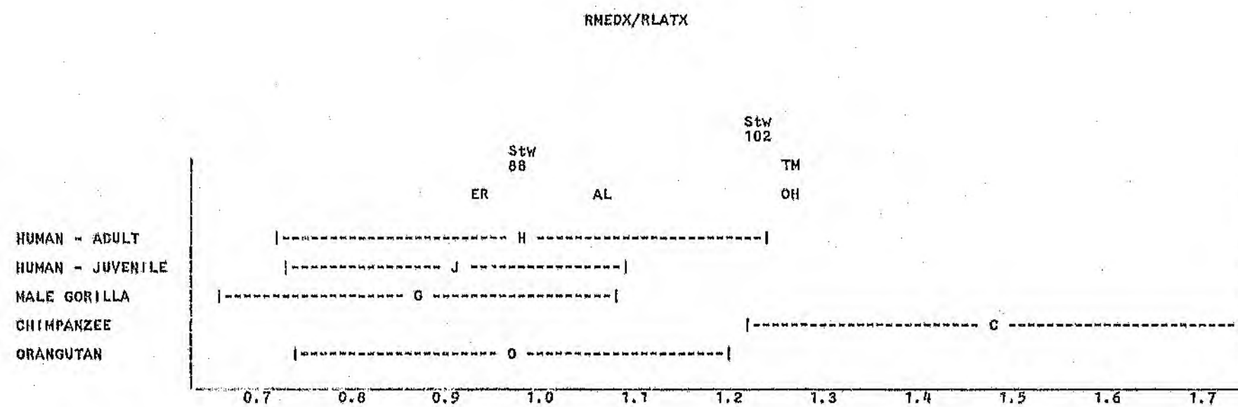
Figure 52. RMEDX/RLATX - Samples of Modern Humans and Great Apes (Mean \pm Standard Deviation) and Fossil Specimens.
