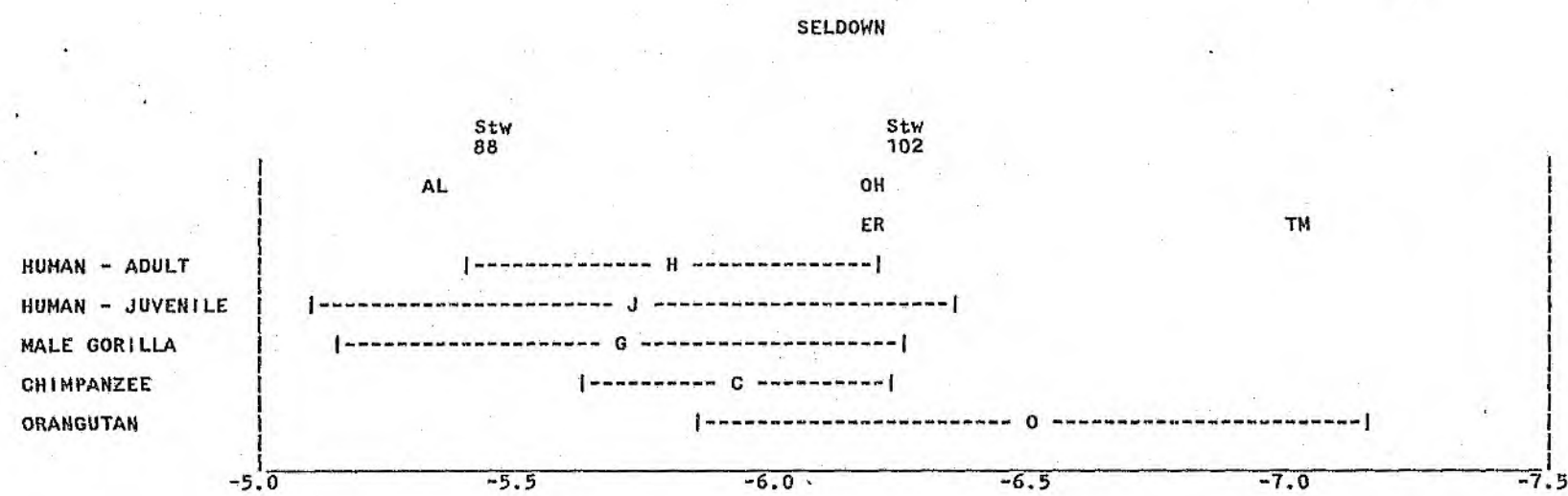
Figure 45. SELDOWN - Samples of Modern Humans and Great Apes (Mean \pm Standard Deviation) and Fossil Specimens.
