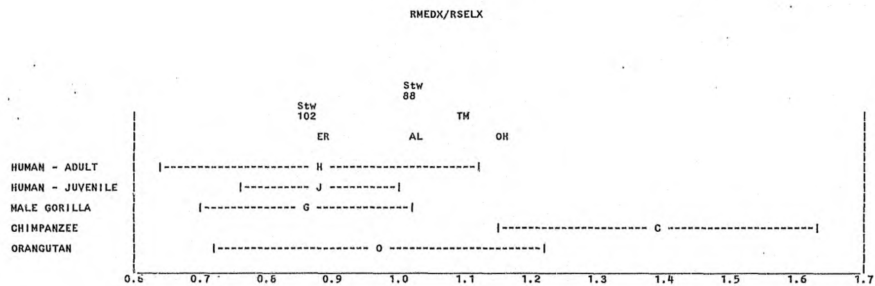
Figure 53. RMEDX/RSELX - Samples of Modern Humans and Great Apes (Mean \pm Standard Deviation) and Fossil Specimens.
