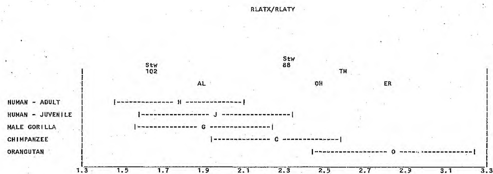
Figure 60. RLATX/RLATY - Samples of Modern Humans and Great Apes (Mean \pm Standard Deviation) and Fossil Specimens.
