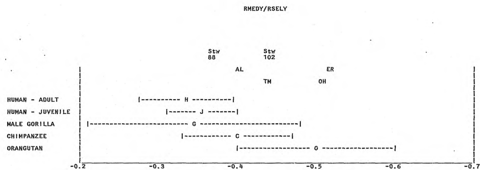
Figure 56. RMEDY/RSELY - Samples of Modern Humans and Great Apes (Mean \pm Standard Deviation) and Fossil Specimens.
