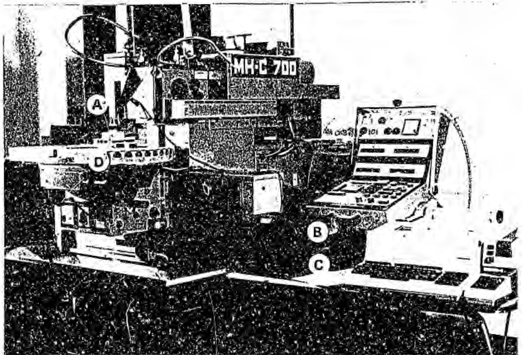
Figure 12. Computer numerical control milling machine modified by the attachment of: (A) Digital length transducer, (B) Printer, (C) Display monitor. (D) indicates the machine's movable table.
