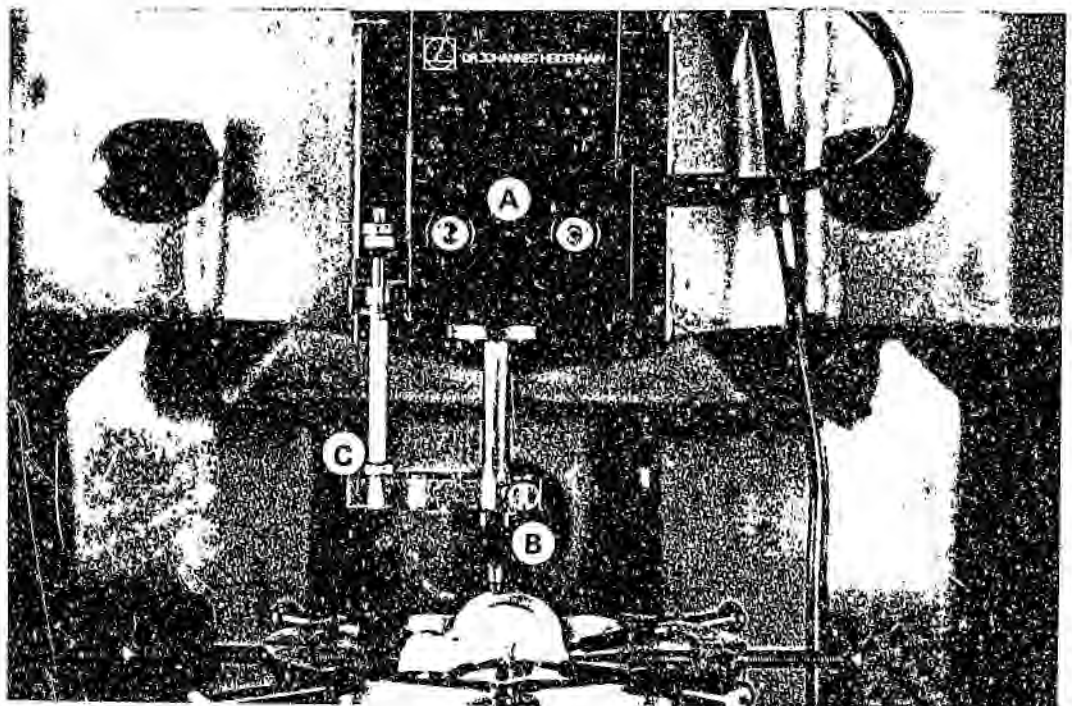
Figure 13. (A) Digital length transducer, (B) Probe with spherical tip, (C) Vertical guiding device.
