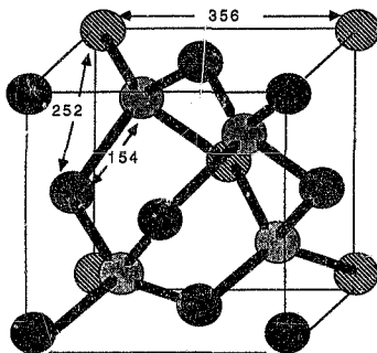
fig 1 the diamond unit cell
