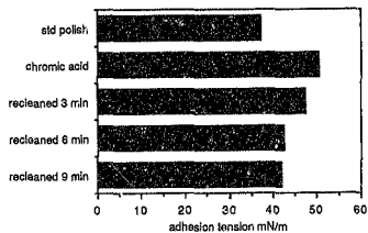
fig 27 effect of chromic acid and attrition
