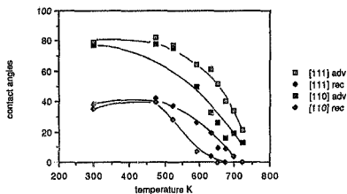
fig 24a oxidation effects on contact angles
