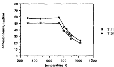
fig 28b effect of hydrogen on adhesion tension
