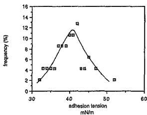
fig 23a distribution of adhesion tension on polished [111]
