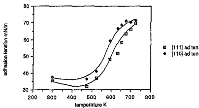
fig 24b oxidation effects on adhesion tension
