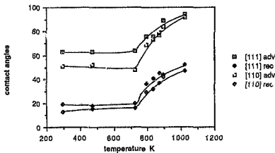
fig 28a effect of hydrogen on contact angles
