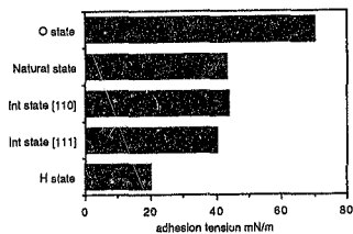
fig 32 relative wettability of natural surface
