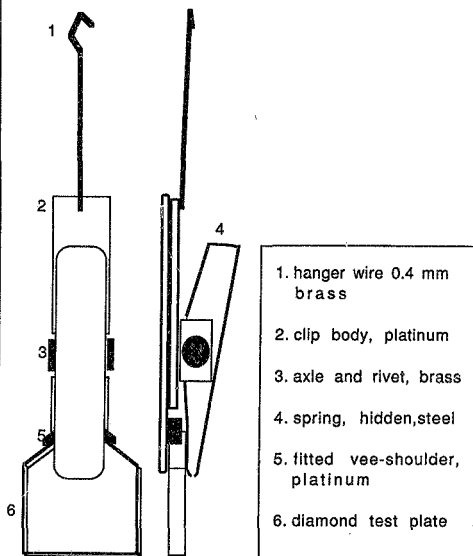
fig 10 detail of clip for diamond test plates
