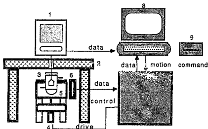
fig 8 capillarographic apparatus - schematic
