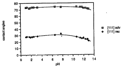
fig 40a effect of pH on contact angles
