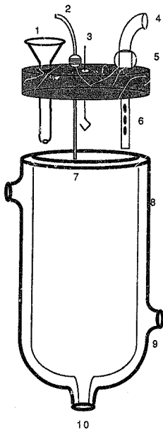
fig 9 detail of capillarographic cell and lid
