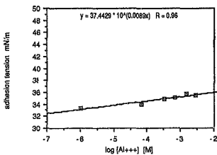
fig 46 effect of aluminium ion concentration
