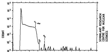
101 FIGURE 33 R B SPECTRA
