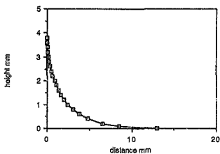
fig 7 numerical solution of meniscus curve for water
