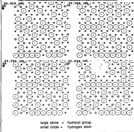
fig 38 simulation of randomized surface coverage
