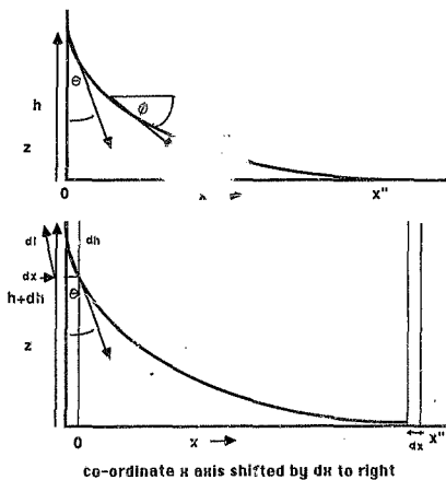
fig A1 derivation of Young's equation by energy method vertical plate with gravitational potential
