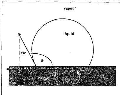
fig 4 the mechanical equilibrium of Thos Young (1804)
