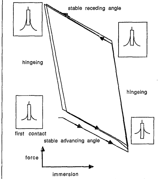
fig 19 stages in the wetting hysteresis loop
