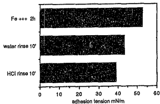
fig 50 removal of ferric ion by water and acid rinse
