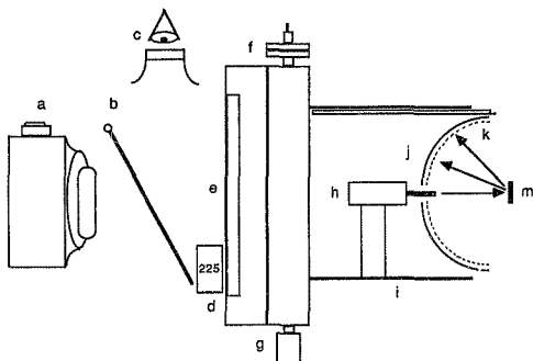
fig 17 low energy electron diffraction apparatus
