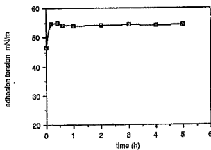
fig 44 Long exposure to Venetia water
