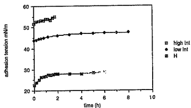
fig 39 hydration effect in water
