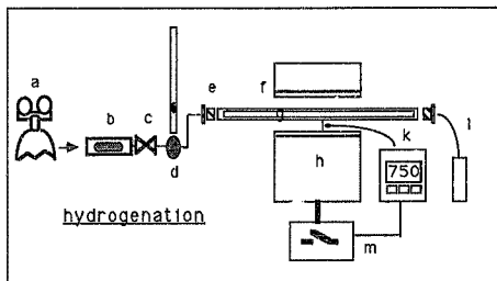
fig 15 tube reactor for gas reaction
