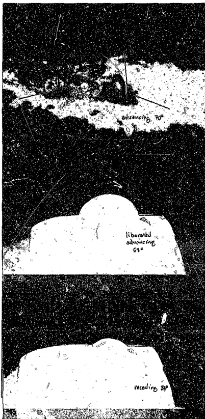
fig 31 photographs from optical contact angle studies
