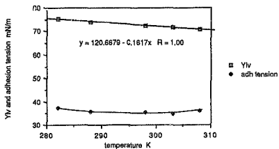
fig 41 effect of temperature on Ylv and adhesion tension
