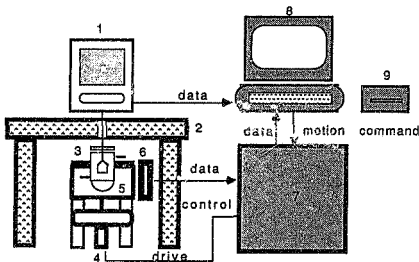
fig 8 capillarographic apparatus - schematic
