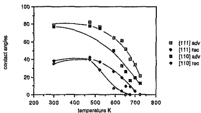
fig 24a oxidation effects on contact angles
