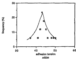
fig 23b distribution of adhesion tension for polished [110]
