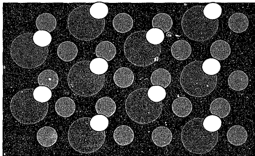
fig 37 ideal 1/3 monolayer coverage by oxygen on the [111] surface
