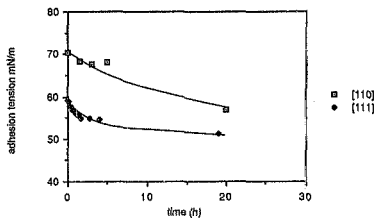
fig 25 recovery from hydrophilic state
