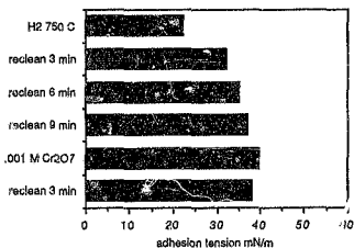
fig 29 effect of attrition on hydrogenated surface
