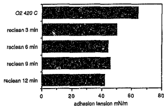
fig 26 effect of attrition on oxidized surface
