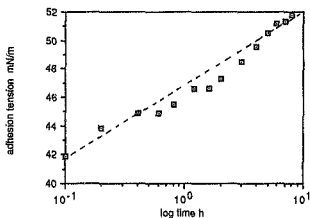
fig 49 effect of ferric ion with time
