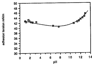
fig 40b effect of pH on adhesion tension
