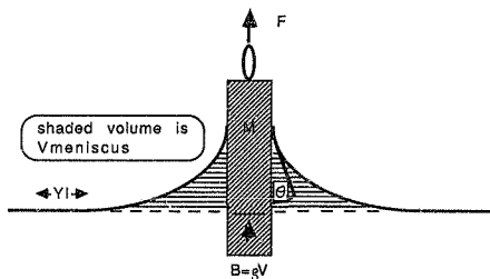
fig 6 Basis of the capillarographic method
