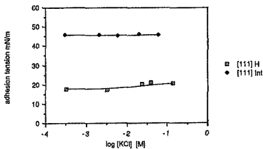
fig 42 effect of ionic strength
