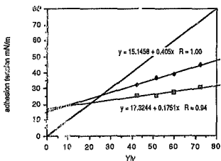
fig 30 Zisman plots for [111]H and [110]Int
