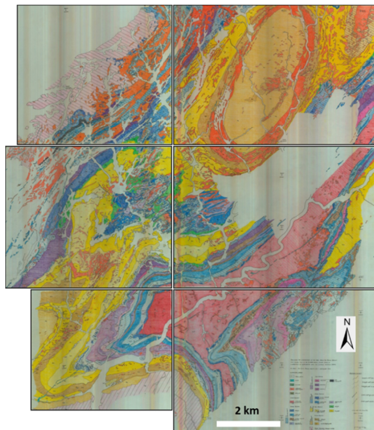
Figure 2.20. Interpretation at 1:10 000 scale of the project area. Note the hole in the interpretation is where detailed ground mapping exists (the SJ map of Golder Associates (1978) and the geological mapping of Laberge (2008a, 2008b) in the SK and SJ south areas described in Chapter 2.5.1. The Nose Structure portion of the bottom left sheet was subsequently re-interpreted as shown in Figure 2.22. See Appendix II for location and explanation of ornaments used.
