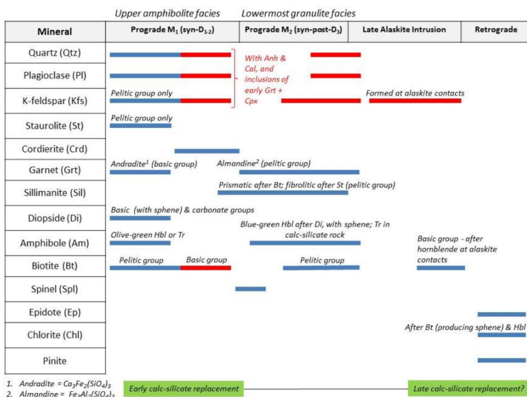
Figure 5.5. Diagram showing a revised mineral paragenesis after Nash (1971) with additional observations from this project. These include the presence of cordierite and almandine garnet earlier than that interpreted by Nash, and pulses of calc-silicate replacement ( \pm brecciation) associated with faulting. The mineral assemblage suggests that M 2 reached lowermost granulite facies metamorphism (Figure 5.6). An explanation to mineral abbreviations where not given in the figure is shown in Appendix I.
