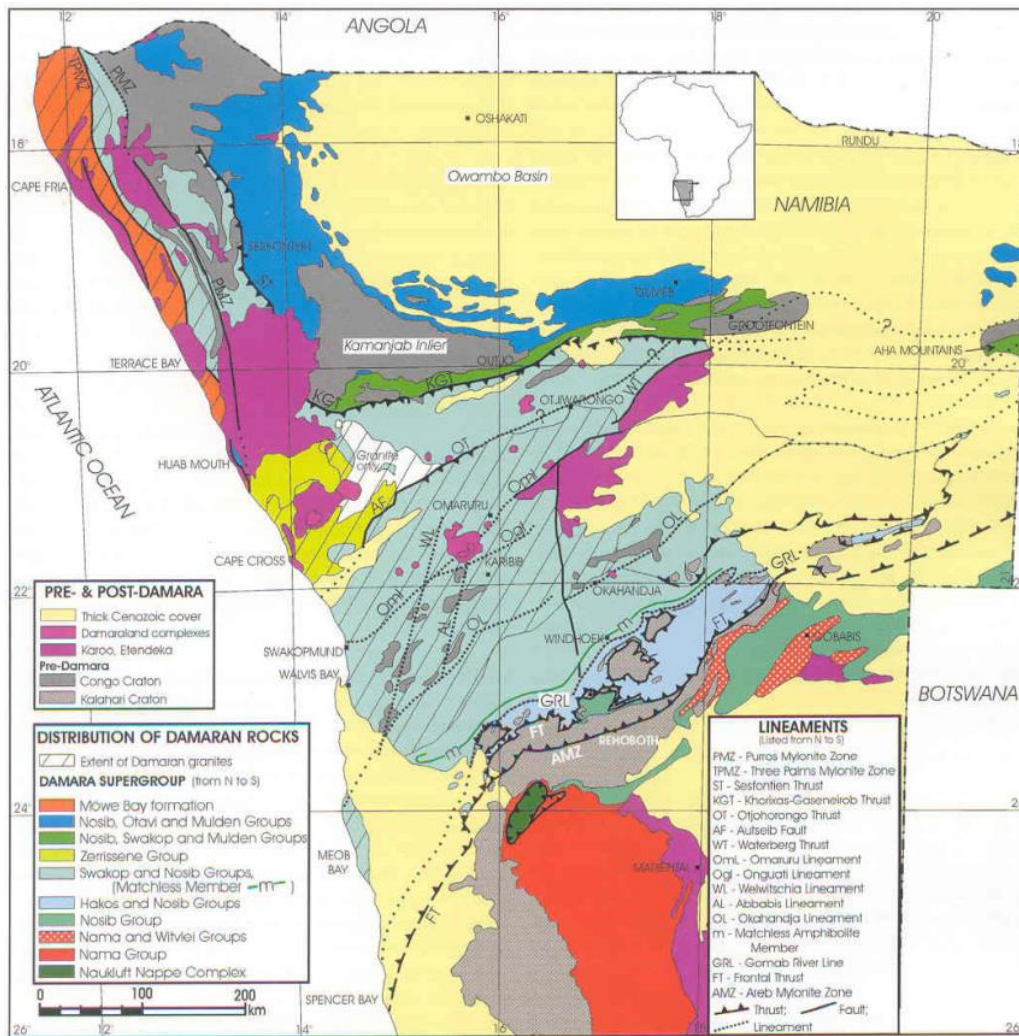
Figure 1.5. Schematic geological map showing the distribution of the main stratigraphic units of the Damara Supergroup (from Miller, 2008).
