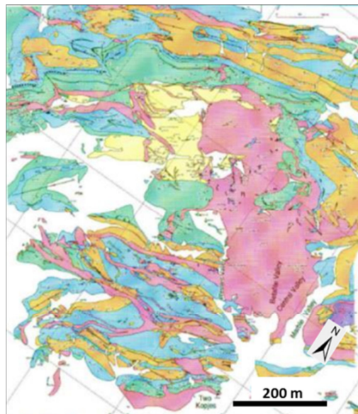
Figure 2.18. Geological map of the SH area of Mestres-Ridge (1992). For the location of the SH area see Figure 1.2. Figure is centred on 503000 mE, 7512000 mN.
