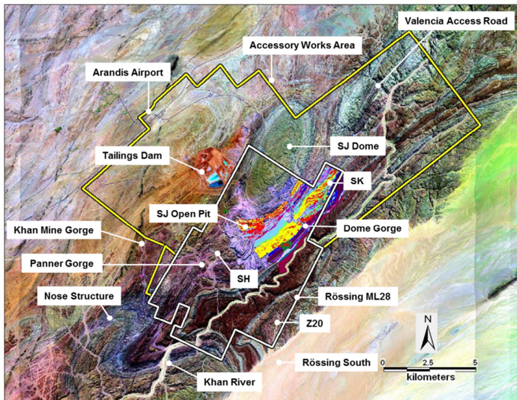
Figure 1.2. Hyperspectral imagery showing the Rössing Uranium Ltd. ML28 mine lease area (white border) and accessory works area (yellow border) showing the location of the SJ, SK, SH and Z20-Rössing South uranium deposits and extent of detailed geological mapping around the SJ open pit. The image is processed hyperspectral line data with RGB band combinations 108-26-2 (equivalent to Landsat bands 7-4-1). Some physiographic features referred to in the text are shown. Figure is centred on 506000 mE, 7516000 mN.
