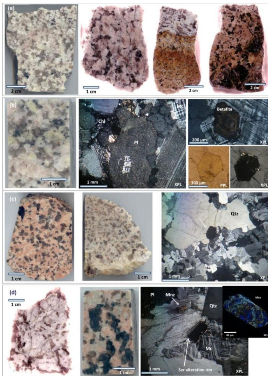
Figure 6.3. Examples of textural and mineralogical variability in uraniferous alaskites equated to the D and E types of Nex (1997). (a) examples of hand specimens from the SJ Pit from left to right: granodiorite D type RSS098, alkali feldspar granite D type RPS048 from the Trolley 10 area, quartz syenite E type RSS003 from Phase 2 exhibiting an iron oxide 'front' where this fills fracture planes, and ilmenite-bearing syenogranite E type RSS005 from Phase 2. (b) SJ Pit syenogranite RSS097 D type in hand specimen (left) and thin section (middle, right) showing typical minor clay alteration of plagioclase and strong chloritisation of biotite, and betafite detail shown on the three right hand images (c) syenogranite RSS025 D type from the SH alaskite plug (left) which appears in the field to cross-cut granodiorite RSS022 D type (middle, right – note betafite indicated by arrow). (d) alkali feldspar granite RPS005 D type from the northeastern extremity of Z19 (left), syenogranite RSS093 D type from SK drill hole SK07D041 in hand specimen (middle) illustrating the smokiness of the quartz and thin section (right) showing an opaque phase with a clay alteration rim and euhedral monazite zonation detail. PPL – plain polarised light, XPL – cross polarised light. For an explanation of mineral abbreviations refer to Appendix I.
