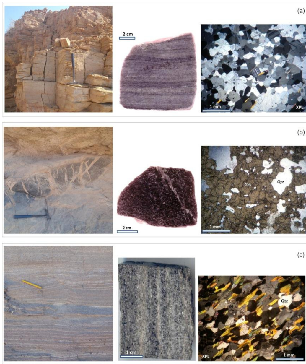
Figure 3.3. Mapped units of the Etusis Formation. (a): bedded meta-arkose outcropping on the SJ Dome (left), in hand specimen RSS051 (middle) showing heavy mineral-rich laminae, and exhibiting moderately developed granoblastic texture in a thin section of the same sample (right); (b): interbed of plagioclase-quartz-garnet calc-silicate in meta-arkose of the SJ Dome cut by alaskite (left), and in RPS042 hand specimen and thin section (middle, right); (c): outcrop of biotite gneiss on the SJ Dome showing the effects of shearing as tension gashes in the orientation of the swing magnet (left) and hand specimen and thin section of RSS011 (right), an ilmenite-phlogopite-plagioclase-microcline-quartz-gneiss. PPL – plain polarised light, XPL – cross polarised light. For an explanation of mineral abbreviations refer to Appendix I.
