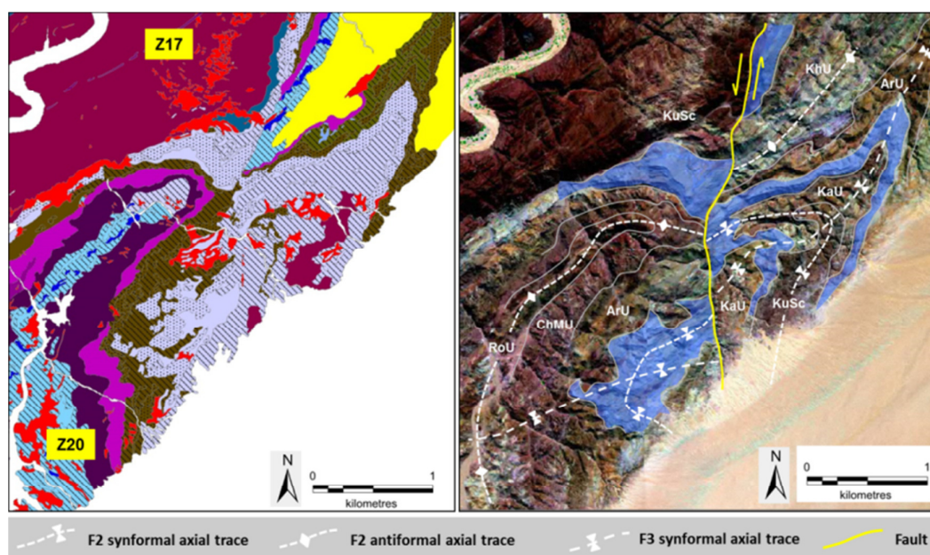
Figure 4.5. Left – lithological interpretation of the area northeast of the Z20 anomaly and Rössing South Zone 1 as per the attached map. Right – structural interpretation that uses marble of the Karibib Formation (blue) to highlight a type 3 fold interference structure comprising F_3 folds superimposed on earlier F_2 structures; the geology is further complicated by the presence of a left-lateral D_4 fault offsetting the closure of the central F_2 syncline by a distance of approximately 600 m. Base image is hyperspectral line data with RGB band combinations 108-26-2 (equivalent to Landsat bands 7-4-1). See Figure 4.2 for location. KhU – undifferentiated Khan Formation; RoU – undifferentiated Rössing Formation; ChMU – undifferentiated Chuos Formation diamictite; ArU – undifferentiated Arandis Formation; KaU – undifferentiated Karibib Formation; KuSc – Kuiseb Formation schist. Figure is centred on 508000 mE, 7509000 mN.
