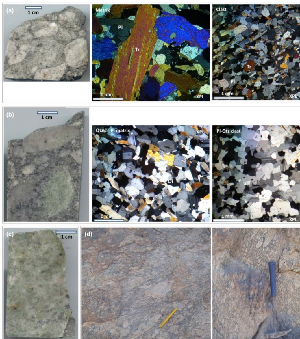
Figure 5.4. Calc-silicate rock exhibiting characteristic quartz-tremolite-plagioclase mineralogy. (a) RSS068 in hand specimen (left) and thin section (middle and right showing matrix and clast respectively), from southwest of Dome Gorge; (b) diopside-bearing RSS030 from SH hand specimen (left) and thin section (middle and right showing matrix and clast respectively); (c) RSS067 from southwest of Dome Gorge, exhibiting a fine-grained massive texture; (d) outcropping matrix-supported calc-silicate breccia from Panner Gorge. PPL – plain polarised light, XPL – cross polarised light. For an explanation of mineral abbreviations refer to Appendix I.
