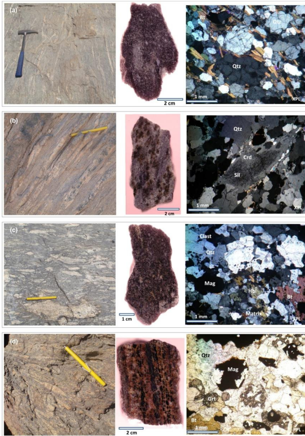
Figure 3.11. Mapped units of the Chuos Formation, in each case shows outcrop (left), hand specimen (middle) and corresponding thin section (right). (a) Facies 1, RPS031 K-feldspar-biotite-quartz diamictite; (b) Facies 2, RPS040 sillimanite-cordierite-biotite-K-feldspar-quartz diamictite; (c) Facies 3, RPS041 magnetite-hornblende-biotite-K-feldspar-quartz diamictite; (d) Facies 3, sample RPS068 biotite-garnet-magnetite-quartz iron formation outcropping between Arandis Airport and Panner Gorge. PPL – plain polarised light, XPL – cross polarised light. For an explanation of mineral abbreviations refer to Appendix I.
