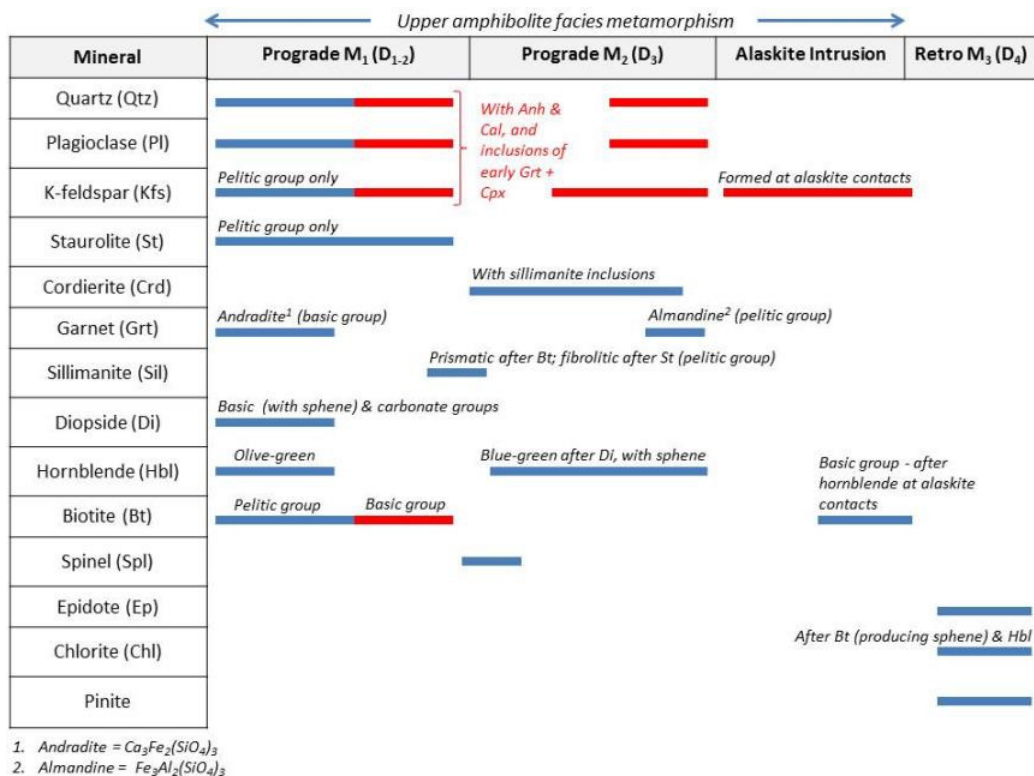
Figure 5.1. Diagram showing the paragenesis of selected minerals compiled from Nash (1971) shown as blue bars and occurring within four compositional groups (psammitic, basic, pelitic and carbonate groups). The current author's correlation of M 1 and M 2 with regional D 1-2 and D 3 events respectively is clear from Nash's description, however in the case of correlating M 3 with D 4 this is tentative. Note that Nash (1971) interprets two phases of migmatisation during both prograde M 1 and M 2 pulses, where the resulting partial melt material is shown as red bars. An explanation to mineral abbreviations is provided in the left column and in Appendix I.
