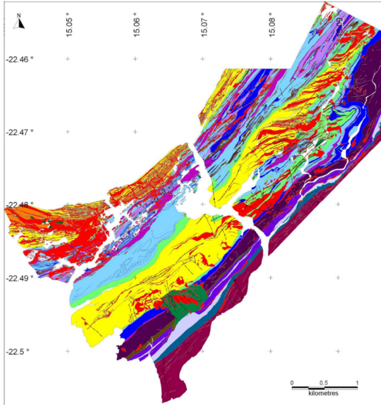
Figure 2.17. Geological map of the SJ-SK area comprising the original SJ geological map of Golder Associates (1978) and the geological mapping of Laberge (2008a, 2008b) in the SK and SJ south areas. Figure from Laberge (2008b). For explanation of colours see Appendix II.
