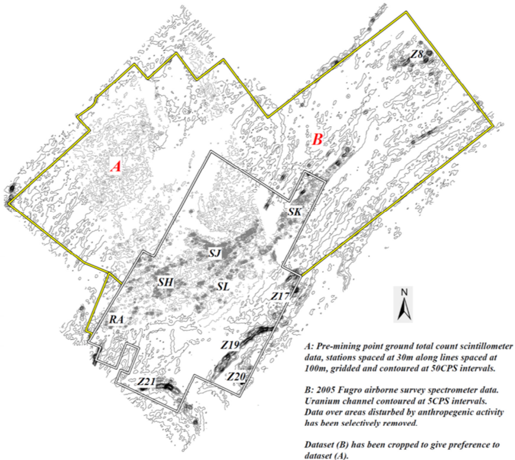
Figure 7.1. Location of radiometric anomalies within the Rössing mine lease ML28 shown on contoured radiometric data compiled as part of this project (see inset and Chapter 2.2 for explanation). Figure is centred on 506000 mE, 7516000 mN.
