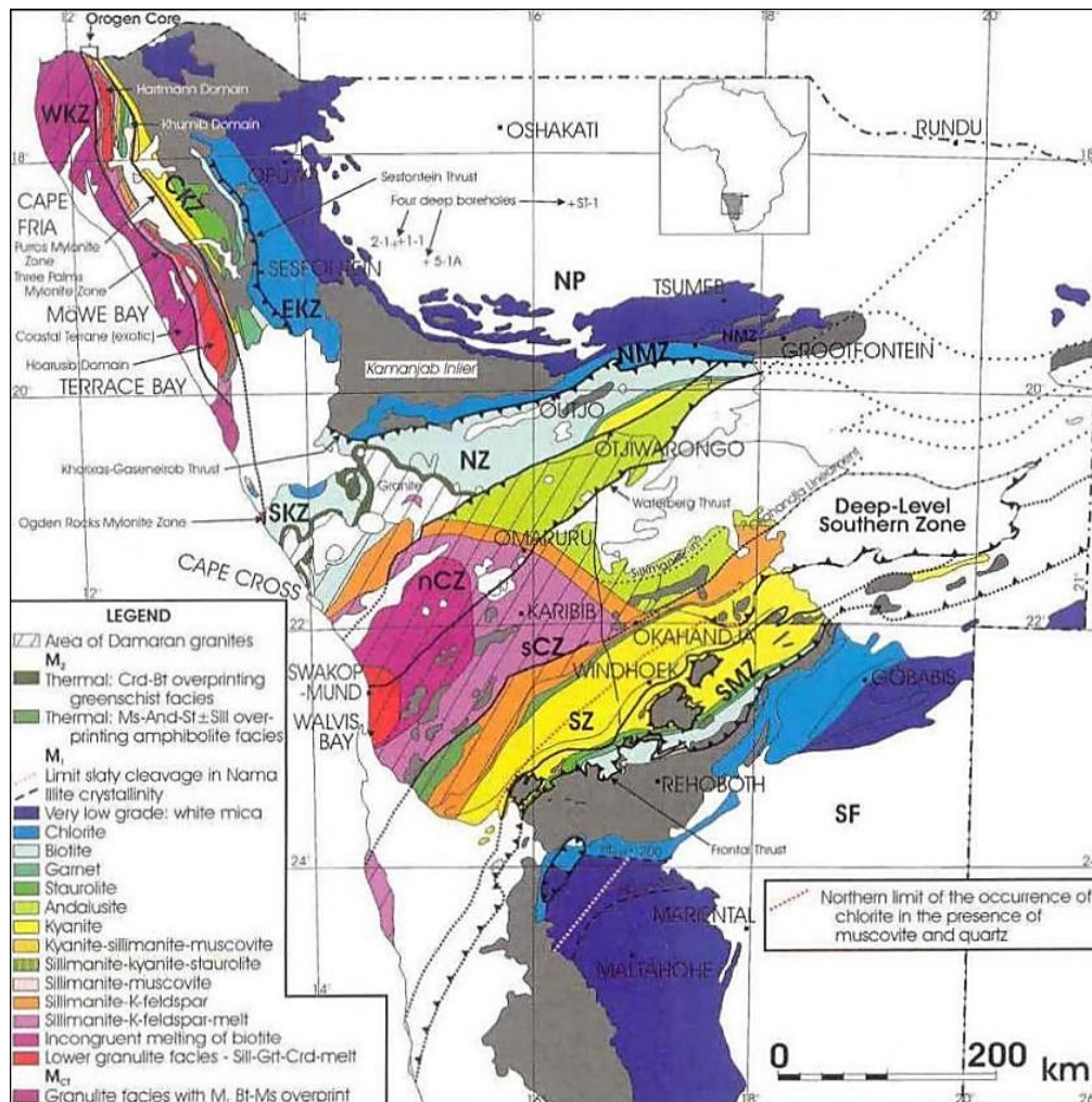
Figure 1.7. Schematic geological map showing the metamorphic zonation of the Damara Orogen based on metapelite assemblages (from Miller, 2008, and references therein).
