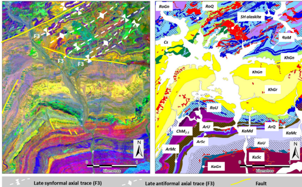
Figure 3.4. Left - HyMap imagery band combination 10-11-12 with M.N.F. transform in the Panner Gorge area (see Figure 1.2). This image distinguishes virtually every mapped unit at member scale (right). Fold structures are dominantly F_3 synform-antiforms superimposed on the larger Rössing synclinorium F_2 - F_3 fold interference structure (Chapter 4, Figure 4.2). Major faults are evident from map relations at the Khan-Rössing Formation contact zone with minor northwest-trending faults parallel to possible F_4 fold axial planes. Right – lithological interpretation of the same area with map unit annotations as follows: KhGn Khan Formation clinopyroxene gneiss; KhGr Khan Formation Granofels; KhMg Khan Formation Biotite Gneiss; RoM Rössing Formation marble; RoGn Rössing Formation cordierite gneiss; RoQ Rössing Formation feldspathic quartzite; RoU undifferentiated Rössing Formation; ChM 2-3 Chuos Formation diamictite facies 2-3; ArMc Arandis Formation calcitic marble; ArSc Arandis Formation biotite schist; ArQ Arandis Formation calc-silicate gneiss; ArU undifferentiated Arandis Formation; KaMc Karibib Formation calcitic marble; KaMd Karibib Formation dolomitic marble; KaGn Karibib Formation biotite gneiss; KaU undifferentiated Karibib Formation; KuSc Kuiseb Formation schist; Cs cross-cutting calc-silicate replacement. The SH uraniferous alaskite plug intrudes an intensely ( F_3 ) folded Khan-Rössing Formation contact hence is demonstrably post- D_3 . Note that the Chuos Formation pinches out completely in the southern part of Panner Gorge. Figure is centred on 503000 mE, 7511000 mN.
