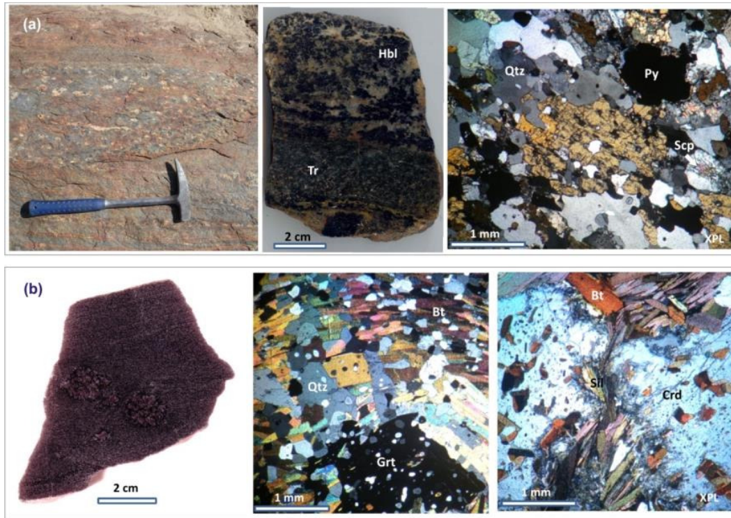
Figure 3.12. Lithologies of the Arandis Formation. (a) calc-silicate gneiss in outcrop (left) from the Karub Member at Z19 and 20008980 (middle) with corresponding thin section (right), a pyrrhotite-scapolite-tremolite-quartz gneiss also from the Z19 area; (b) Okawoyo Member biotite schist RPS011 in hand specimen and thin section (left, middle), a garnet-biotite-quartz schist from Panner Gorge showing biotite wrapping around pre-tectonic garnet poikiloblasts, and thin section of RSS060 (right) from the Khan River, a sillimanite-plagioclase-biotite-quartz-cordierite schist. PPL – plain polarised light, XPL – cross polarised light. For an explanation of mineral abbreviations refer to Appendix I.
