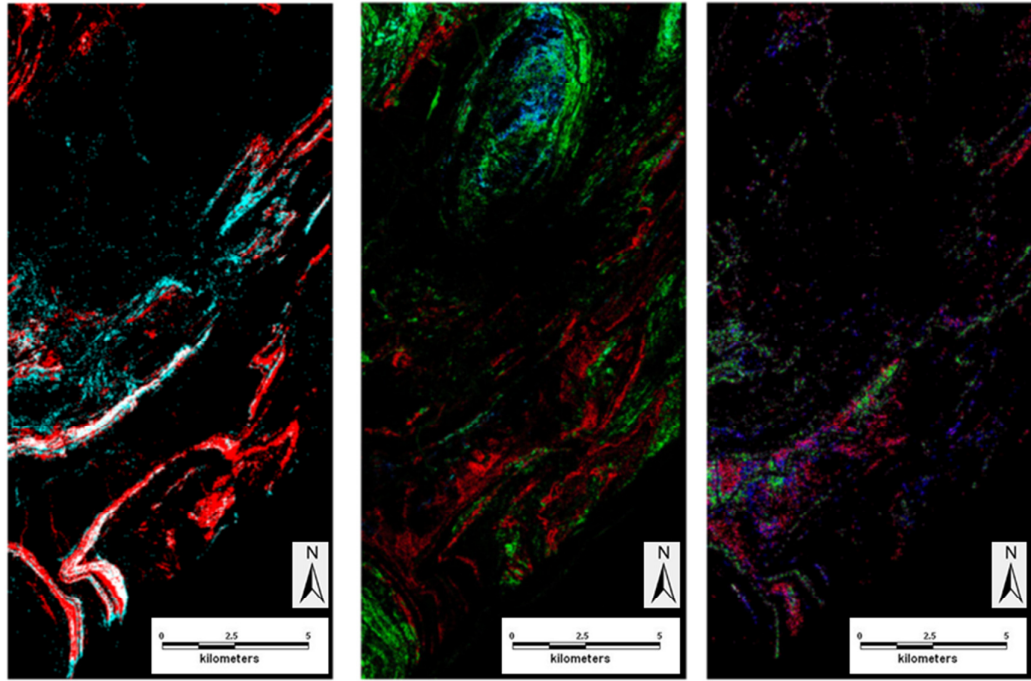
Figure 2.13. Mineral end-member images derived from the Rössing area HyMap data. Left – calcite (light blue) and dolomite (red); centre – illite composite consisting of montmorillonite (green) and a kaolinite-halloysite mixture (red); right – epidote-chlorite (from Caballero, 2009). Figure is centred on 505000 mE, 7511000 mN.
