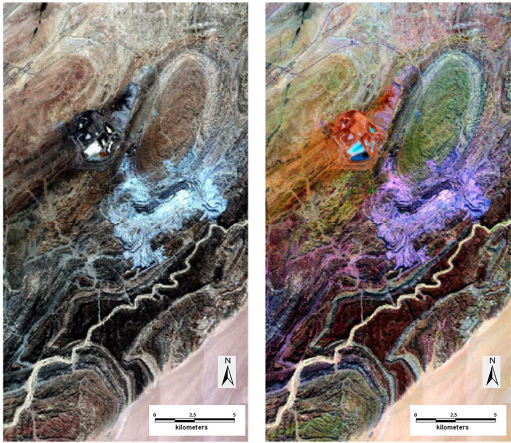
Figure 2.11. Colour combination images of portions of the HyMap survey data: left - real colour composite image bands 15-8-2 (equivalent to Landsat RGB 3-2-1); right - lithological contrast image using bands 108-26-2 (equivalent to Landsat RGB 7-4-1; from Caballero (2009). Figure is centred on 505000 mE, 7513000 mN.
