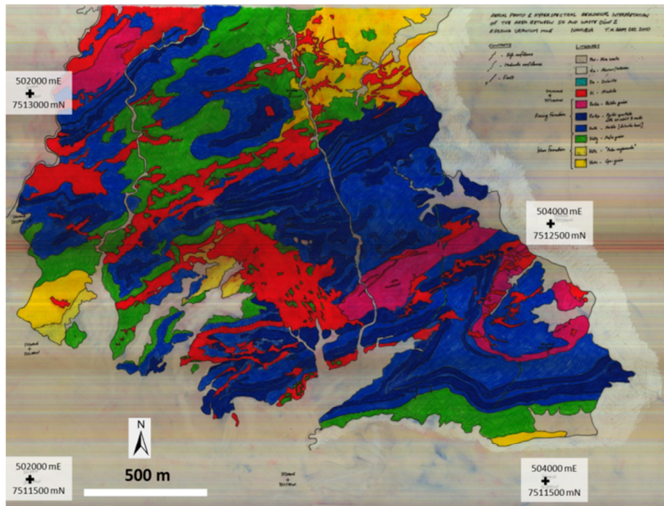
Figure 2.21. Interpretation at 1:3500 scale of the geology in the SH area. This interpretation was completed to better resolve the structural and stratigraphic detail of the area beyond that shown in the centre of Figure 2.20. The white shading on the interpretation indicates the extent of mine dumps. See appended map and legend for explanation of other ornaments used.
