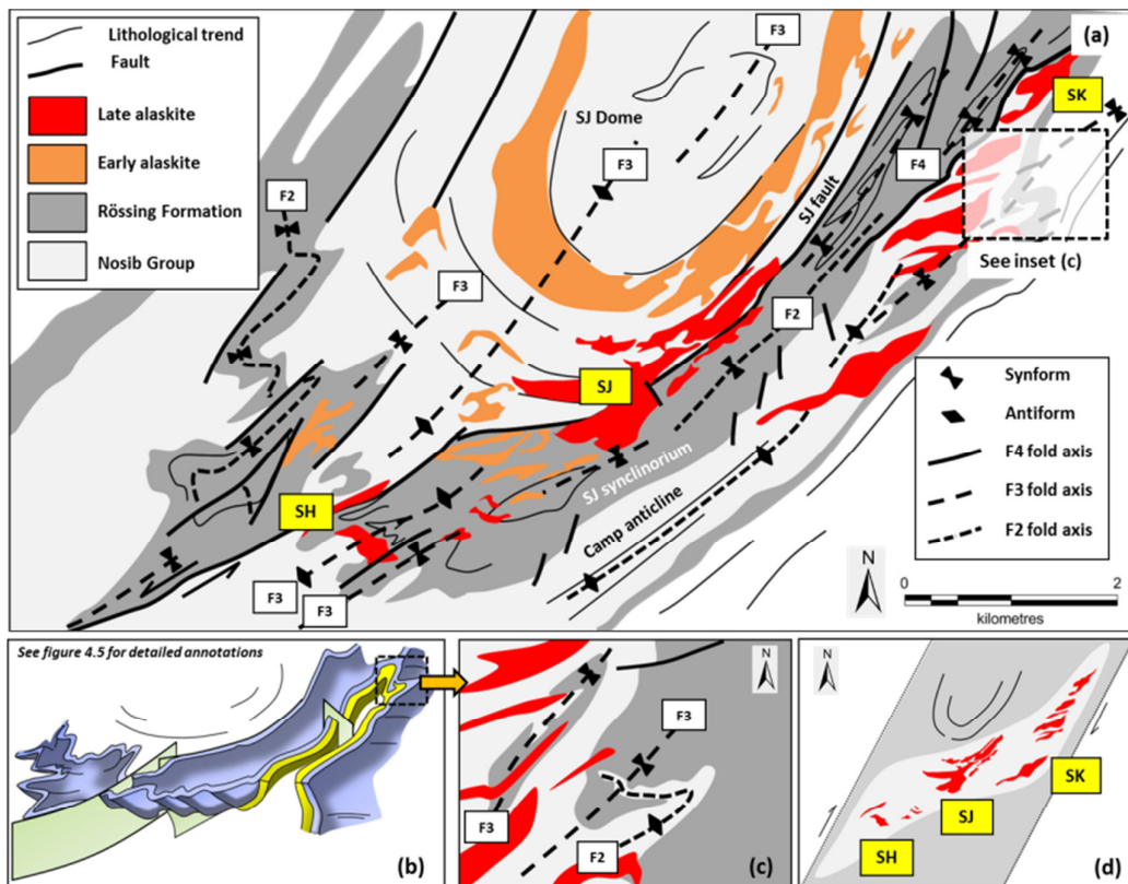
Figure 7.2. (a) Summary geological map after the appended detailed map showing the geological setting of the SJ, SH and SK uraniferous alaskite bodies. Note that early barren (C type of Nex, 1997) and late uraniferous (D-E type) alaskites are broadly differentiated, where these are either folded by, or cross-cut F_3 folds, respectively. (b) 3D sketch depicting fold interference structures in the area (see Figure 4.5 for detailed explanation). (c) Detail of an
