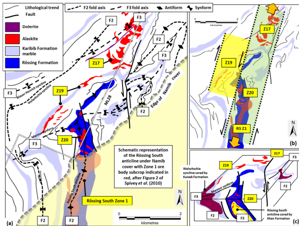
Figure 7.3. (a) Simplified geological setting and major structures in the Z20-Z19-Z17 (and Rössing South Zone 1) area. Major early isoclinal F_2 folds comprising the Rössing South anticline and Welwitschia anticline are refolded into upright northeast-plunging F_3 folds that include the Marmor synform, Blauer Heinrich syncline (see Figure 4.2) and the complex interference structure northeast of Z20 (see Figure 4.4 for detail); the fold interference structure has subsequently been disrupted by left-lateral north-northeast oriented strike slip movements ( D_4 sinistral faults). The locations of uraniferous alaskites are shown, including the subcrop of Rössing South Zone 1 under Namib cover taken from Figure 2 of Spivey et al. (2010). (b) Interpretation of district-scale mode of emplacement of uraniferous alaskites into syn- to post through-going north-northeast oriented transtensional zones that probably predate D_4 sinistral faulting, controlling emplacement of alaskites at Rössing South, Z20, Z17 and Z19. (c) Simple 3D block diagram of the area shown in Figure 7.3a illustrating the relationship between major folds and faults. Bedding parallel faults at the Rössing and Karibib Formation contacts are likely to have been early structures that formed during D_{1-2} and were subsequently reactivated. Figure is centred on 507000 mE, 7508000 mN.
