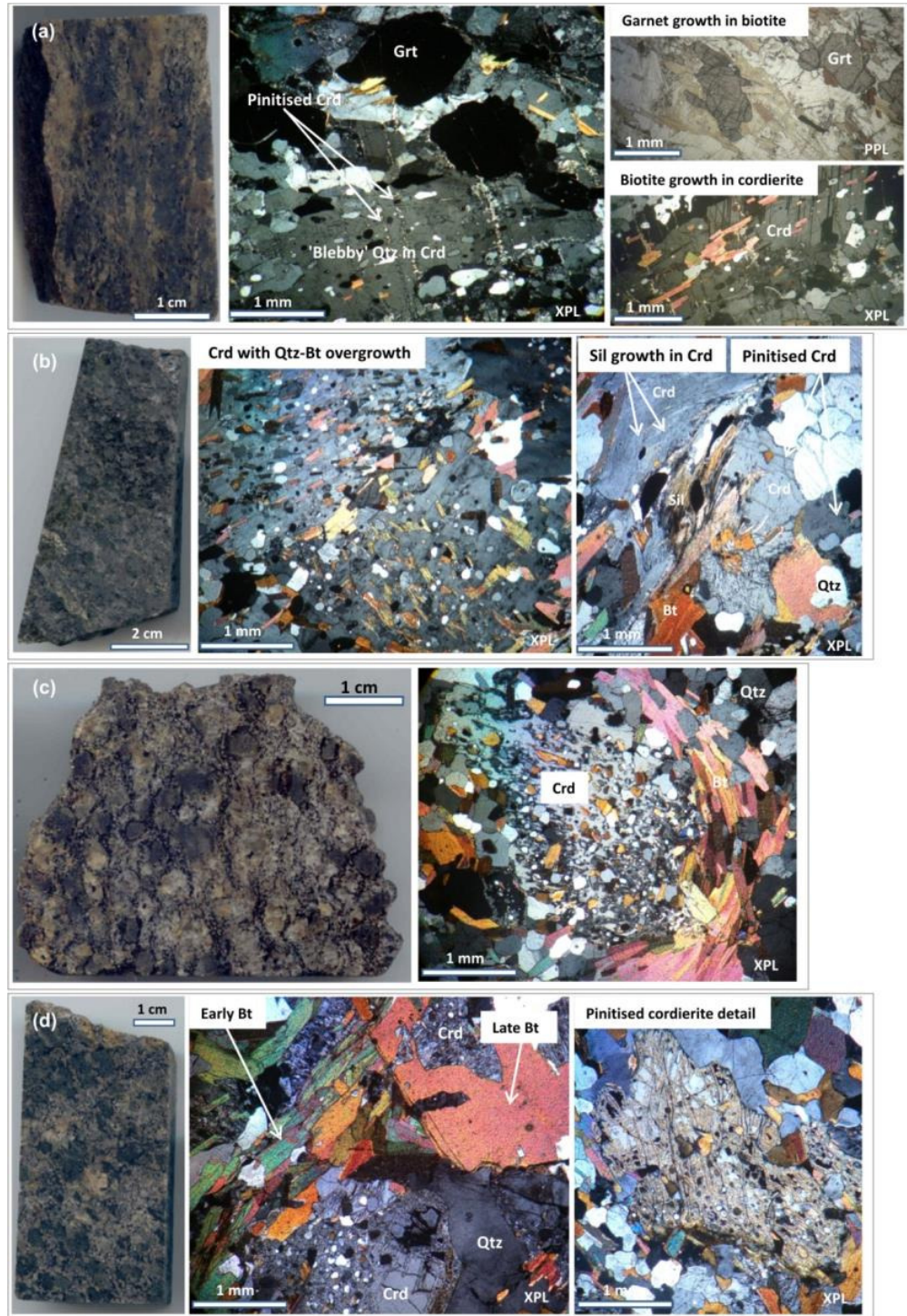
Figure 5.3. Textures and mineral parageneses within metapelites in hand specimen and thin section. (a) RSS036, Grt-Bt-Qtz-cordierite gneiss, Rössing Formation, exhibiting late garnet growth in early biotite bands, and late biotite growth in early cordierite; (b) RSS086, Py-Sil-Crd-Bt-Qtz-K-Fsp gneiss, Rössing Formation, showing late quartz, biotite and sillimanite overgrowing early cordierite; (c) RSS064, Pl-Qtz-Bt-Crd schist, Kuiseb Formation, showing early cordierite porphyroblasts enclosed by early biotite and late quartz-biotite overgrowing cordierite; (d) K-Fsp-Bt-Qtz-Crd schist, Kuiseb Formation, exhibiting both early and late biotite stages. PPL – plain polarised light, XPL – cross polarised light. For an explanation of mineral abbreviations refer to Appendix I.
