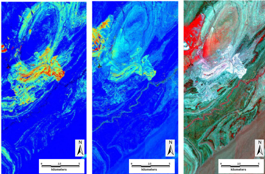
Figure 2.14. Iron oxide and hydroxide mineral end-member maps derived from Rössing area HyMap data. Left – goethite; centre – jarosite; right – goethite and hematite (blue-green) and jarosite (red). From Caballero (2009). Figure is centred on 505000 mE, 7511000 mN.
