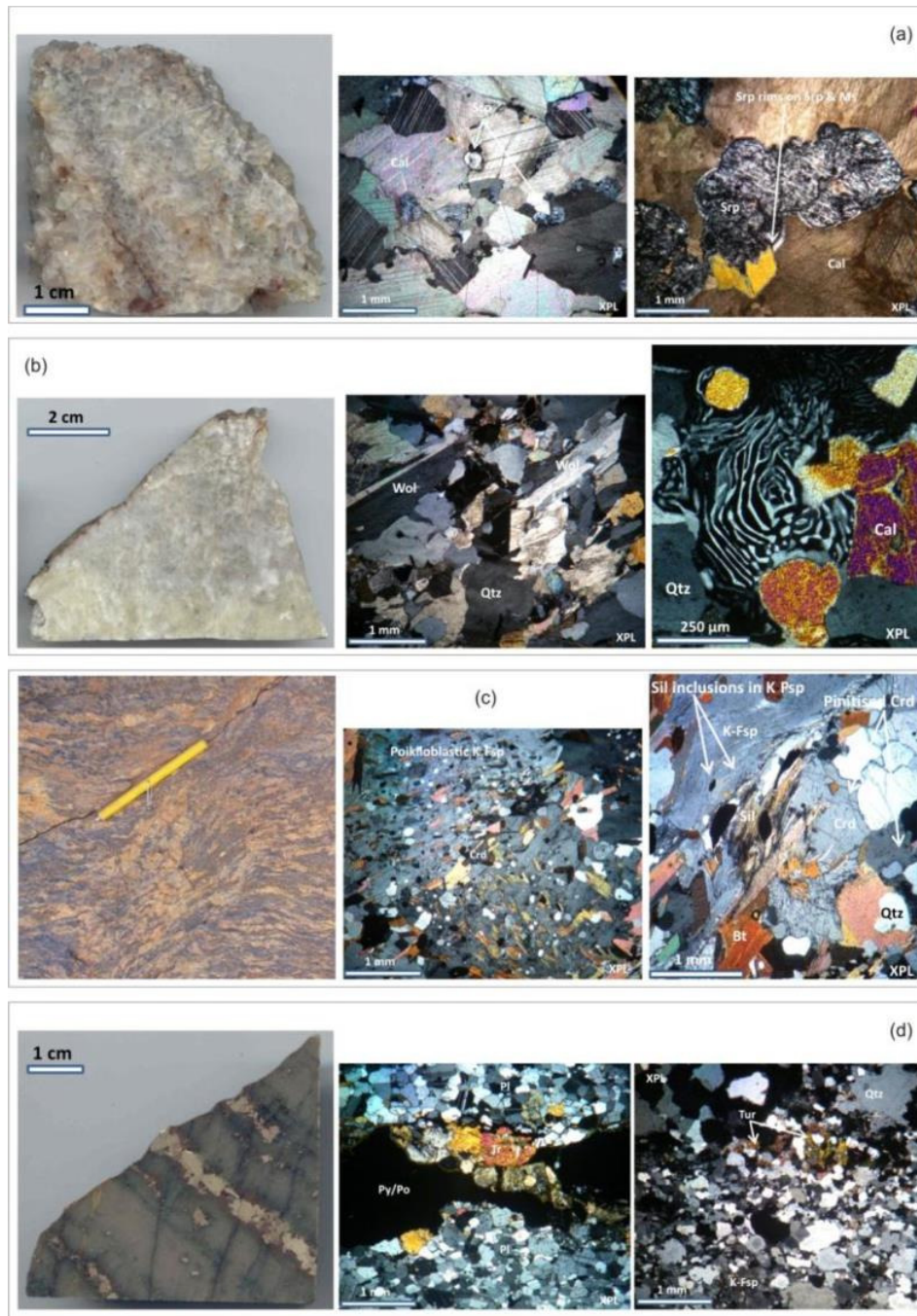
Figure 3.9. Mapped units of the Rössing Formation. (a) marble – graphitic, calcitic, scapolite-bearing marble RSS026 (left) and corresponding thin section (middle) from the SH area, and thin section of RSS084 (right), a serpentine calcitic marble from the SJ open pit; (b) RSS038 (left) and corresponding thin section (middle, right), representing wollastonite-scapolite-quartz skarn mineral development within the Rössing Formation marble; the central area of the right hand thin section photo shows a complex possible quartz-carbonate intergrowth texture; (c) cordierite gneiss outcrop (left) and thin section images of RSS086 from the SJ open pit (middle, right) showing poikiloblastic K-feldspar, pinitised cordierite and fibrous sillimanite; (d) pyrite-pyrrhotite bearing meta-arkose RSS087 from the SJ open pit (left), corresponding thin section (middle) and tourmaline bearing meta-arkose RSS047 from the hinge zone of the Blauer Heinrich Syncline (right). PPL – plain polarised light, XPL – cross polarised light. For an explanation of mineral abbreviations refer to Appendix I.
