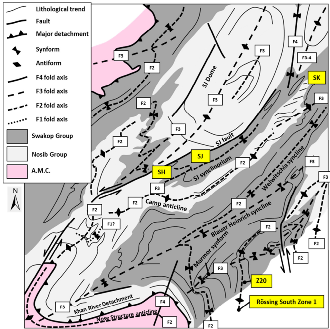
Figure 4.2. Selected structural elements of the Rössing area incorporated from previous work (Figure 4.1 and references therein) with modifications and additional detail added from this mapping. The location of the figure is coincident to the referenced area shown on the map in Appendix II. Figure is centred on 505000 mE, 7511000 mN.
