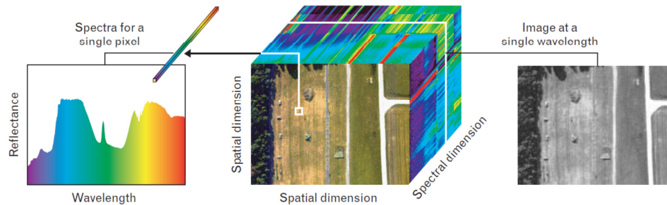
Figure 2.7. An example of the 'data-cube' (centre) structure of hyperspectral imaging illustrating the spatial and spectral nature of the data. The data cube can be visualised as a set of spectra for each individual pixel (left) or as a stack of images (right) for each single spectral channel. From Manolakis et al. (2003).
