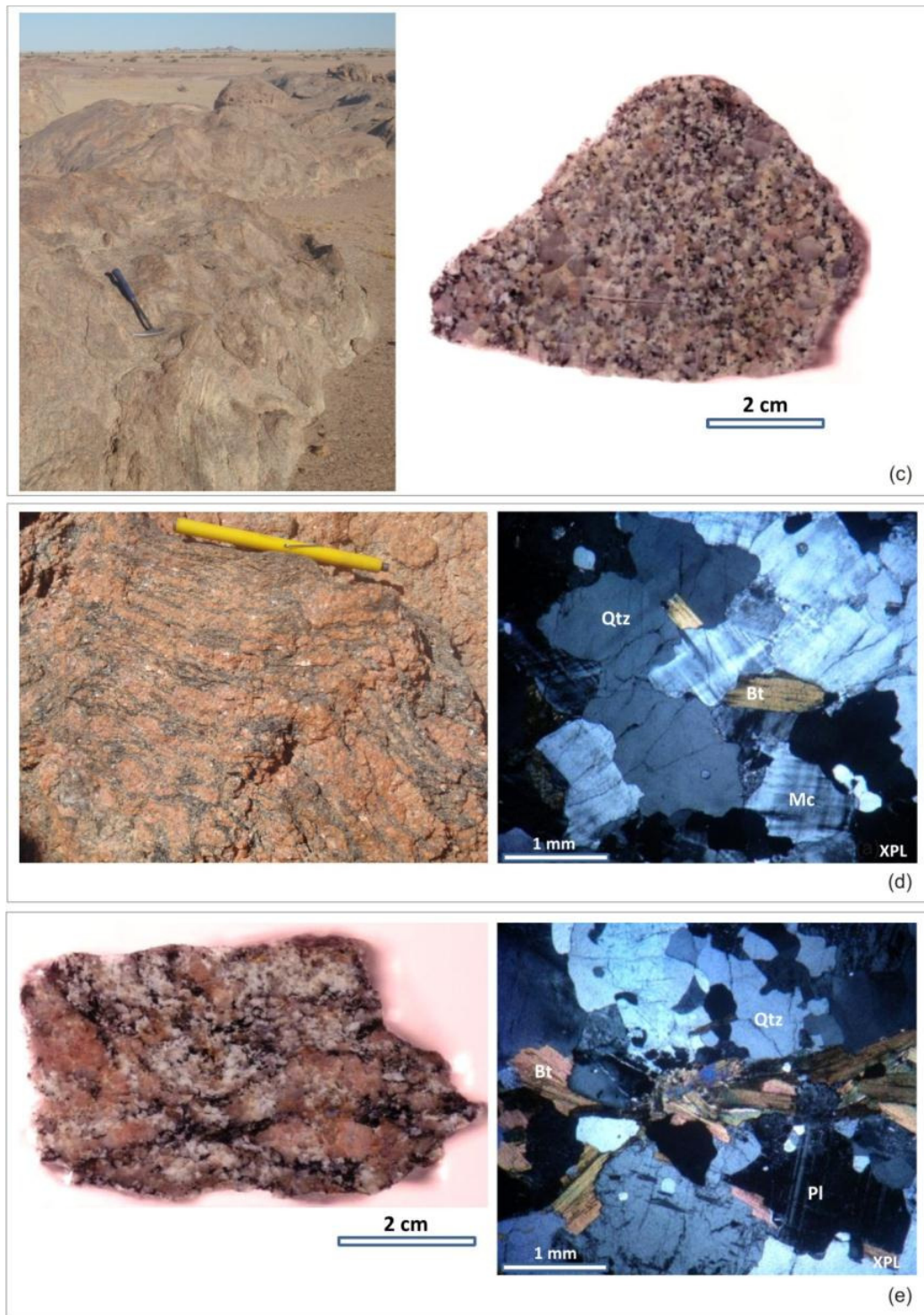
Figure 3.2 (Cont.). Granite and felsic gneisses of the A.M.C. (c) left – outcropping granite gneiss in the Arandis Airport area and, right - corresponding sample RPS071 (monzogranite); (d) left – outcropping foliated, biotite-bearing, red alkali feldspar granite in the Arandis Airport area and, right – corresponding thin section from RSS071; (e) left – augen gneiss sample RPS033 and, right – corresponding thin section. PPL – plain polarised light, XPL – cross polarised light. For an explanation of mineral abbreviations refer to Appendix I.
