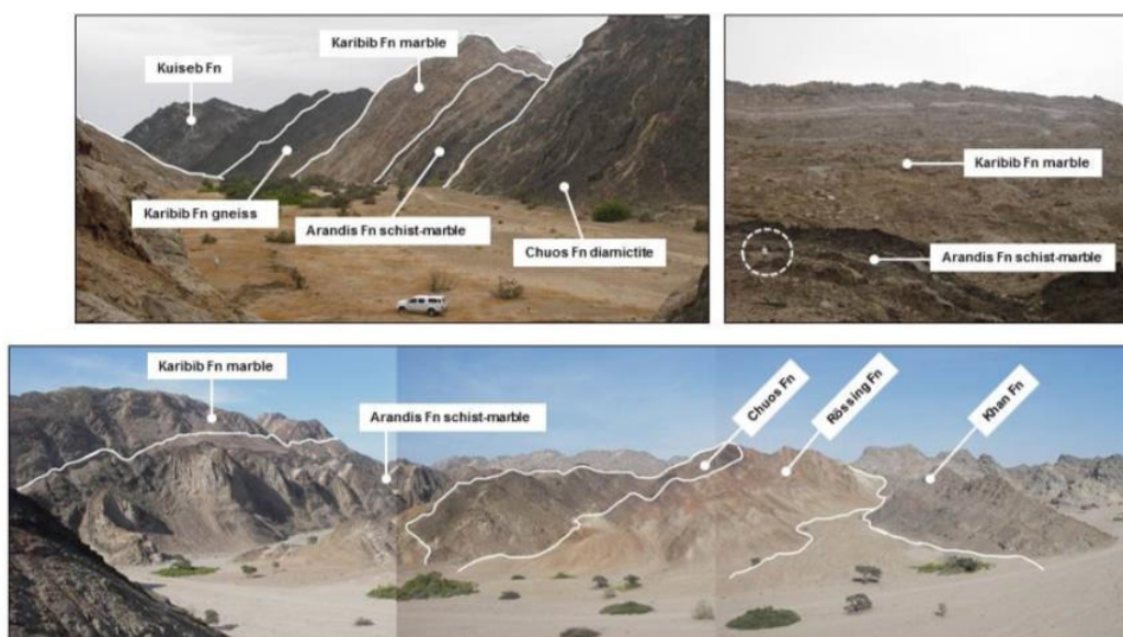
Figure 2.19. Photographs taken during field mapping showing colour and geomorphological expression of major Damaran metasedimentary units in the area. Top left – Chuos Formation and overlying units outcropping spectacularly in the Khan River area, view to the northeast; top right – distinctive outcrop morphology of Karibib Formation marbles and underlying stratigraphy (note Justin Laberge circled for scale), same locality as top left; bottom – section through the lower part of the Damaran stratigraphy as outcropping in the Panner Gorge area showing distinctive colour variations throughout the various formations, view to the west.
