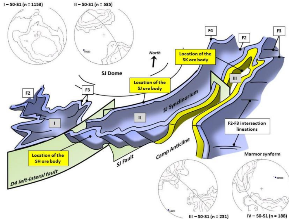
Figure 4.4. Fold interference relationships in the SH-SJ-SK area as determined from compilation of structural data. F_2 fold axes (cf. Figure 4.2) are reworked into northeast-southwest doubly plunging and sub-horizontal F_2 - F_3 interference structures that wrap around the SJ Dome (areas I, II, III and corresponding stereograms). Area I northwest of SH forms a subhorizontal doubly plunging basin-shaped syncline. Area II (SJ area) plunges gently southwest. Area III (SK area) is likely doubly plunging given the anticlinal fold closure to the northeast, with measurements indicating a gentle plunge southwest. Individual F_3 folds on the limbs of the F_2 structures predominantly plunge moderately northeast – an example is shown from S_0 - S_1 data from the F_3 Marmor synform (stereogram IV) to the south of this area. See also appended map for location of structural data. Note the presence of late left-lateral and locally right-lateral faulting. Yellow = top of the Khan Formation, blue = base of the Rössing Formation.
