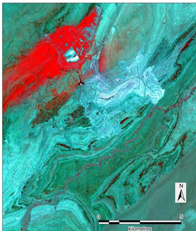
Figure 3.7. Hyperspectral end-member image showing the distribution of hematite-goethite (blue-green) and jarosite (red). Jarosite effectively maps the pyritic meta-arkose of the Rössing Formation and pyritic calc-silicate beds within the Arandis Formation. Jarosite forms through oxidation of pyrite and can be seen to be dispersed by wind to the southwest of the tailings area. Figure is centred on 505000 mE, 7511000 mN.
