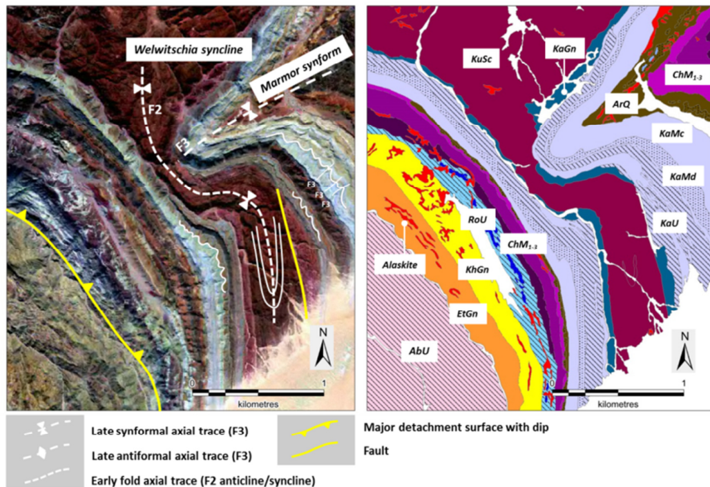
Figure 3.1. Left - HyMap imagery band combination 108-26-2 (equivalent to Landsat 7-4-1) covering the area south of the Khan River and corresponding map interpretation. The image shows that this band combination can spectrally distinguish the entire mapped sequence at a formation-scale, and locally at a member-scale. Major structures (see Chapter 4) are shown on the hyperspectral image and include the fold axial trace of the major refolded Welwitschia syncline (Smith, 1965) and the sheared contact between the A.M.C. and overlying Damaran sequence. Highlighted satellite F_3 fold trends in Karibib Formation marbles show west vergence or M-type concentric folds. A north-northwest trending faulted contact is present between Kuiseb Formation schists and the top of the Karibib Formation observable in the bottom right of the image. Note the isoclinal north-south F_{1-2} similar fold within the hinge zone
