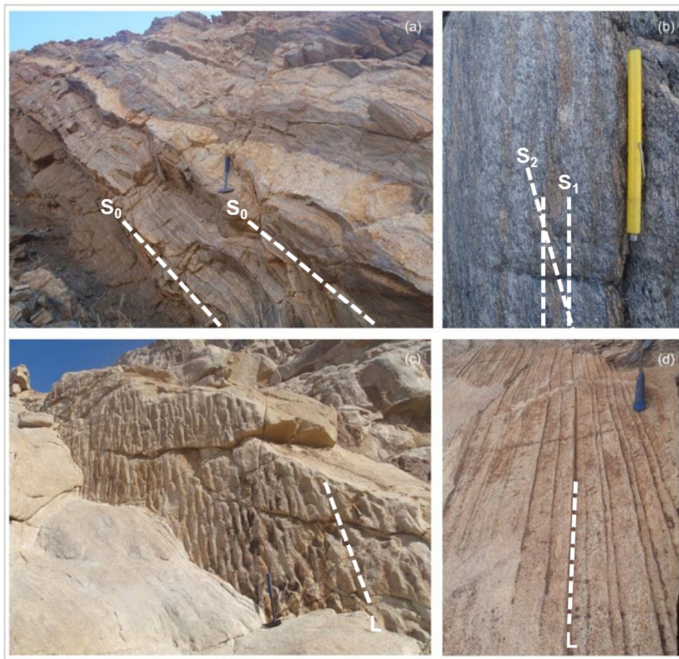
Figure 4.3. Examples of planar and lineation fabrics developed in the Damara succession. (a) bedding ( S_0 ) in quartzo-feldspathic gneisses of the Rössing Formation on the north margin of the Rössing SJ Dome, defined by sub-metric compositional changes in beds, between which gneissosity is developed overprinting original sedimentary features. (b) development of local gneissic fabric ( S_1 ) in Kuiseb cordierite schist of the Khan River with cross-cutting second cleavage ( S_2 ) at a shallow angle to the gneissosity. (c) Karibib marble bedding contact in Panner Gorge showing a crudely developed and steeply plunging bedding-cleavage intersection lineation (L), better defined in the outcrop shown in (d) from the same general locality.
