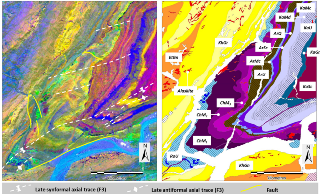
Figure 3.10. Left - HyMap imagery band combination 10-11-12 with M.N.F. transform in the area of the Blauer Heinrich syncline. As per Figure 3.7 this image distinguishes most mapped units at member scale (right). In particular the three members of the Chuos Formation are visible, whilst a complete section of the Arandis and Karibib Formations are also present. Late fold ( F_3 ) axial traces are shown. Right – lithological interpretation of the same area with map unit annotations as follows: EtU Etusis Formation biotite gneiss; KhGn Khan Formation clinopyroxene gneiss; KhGr Khan Formation Granofels; RoU undifferentiated Rössing Formation; ChM 1-3 Chuos Formation diamictite facies 1-3; ArMc Arandis Formation calcitic marble; ArSc Arandis Formation biotite schist; ArQ Arandis Formation calc-silicate gneiss; ArU undifferentiated Arandis Formation; KaMc Karibib Formation calcitic marble; KaMd Karibib Formation dolomitic marble; KaGn Karibib Formation biotite gneiss; KaU undifferentiated Karibib Formation; KuSc Kuiseb Formation schist. Note that on the northern limb of the Blauer Heinrich syncline the Chuos Formation appears to show internal boudinage of units and that this probably predates the F_3 fold structures. Note also the late N-S oriented sinistral faults. Figure is centred on 501000 mE, 7508000 mN.
