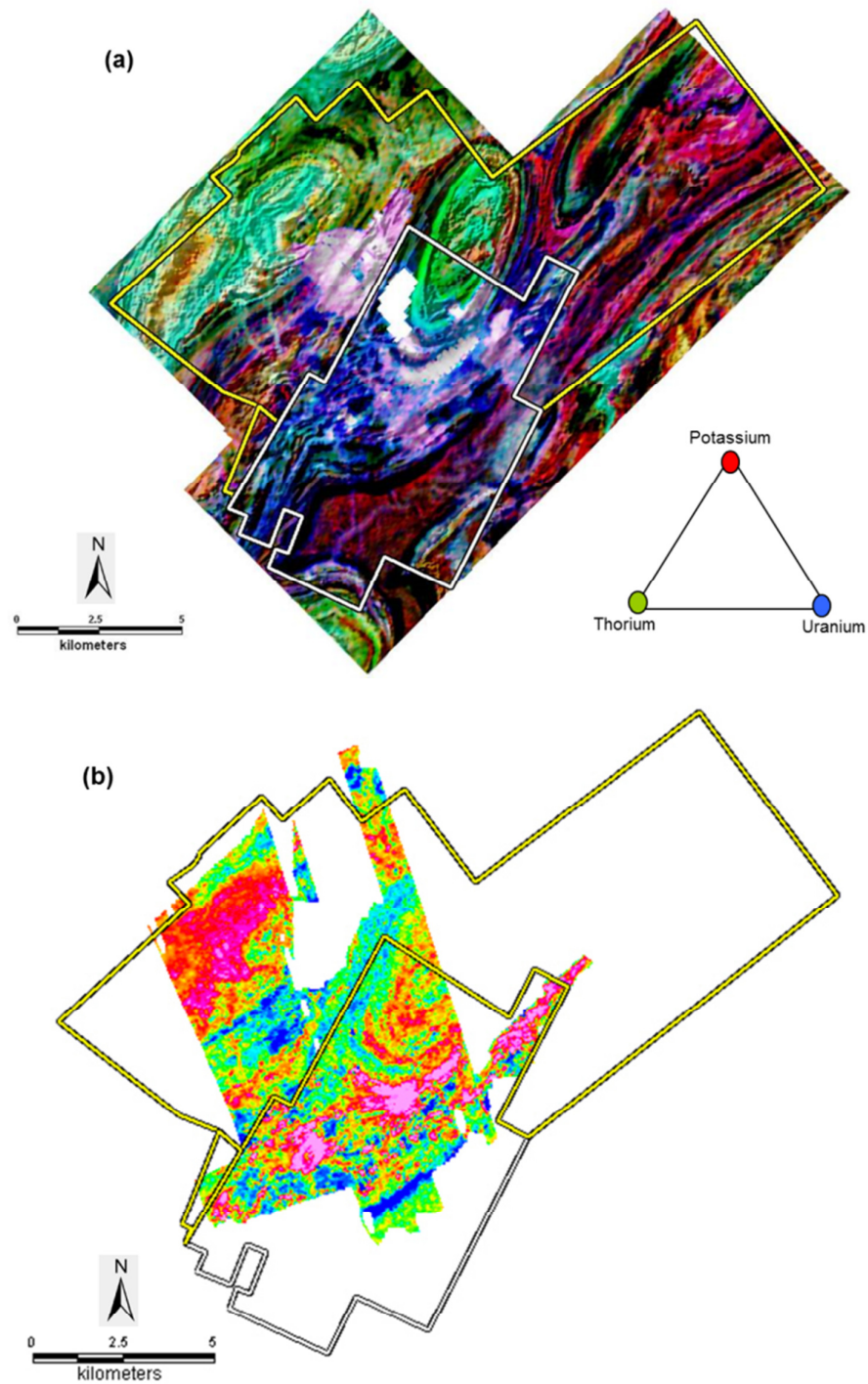
Figure 2.3. Radiometric data in the Rössing area. (a) Ternary image of heli-borne gamma ray spectrometer data. (b) Pre-mining ground scintillometer data, line spacing 100 m with stations spaced at 30 m data gridded to 20 m cell size (hot colours = higher count). Note the ground disturbance in the immediate vicinity of the mine (centre of the image) evident in (a) that masks the response of the sub-surface geology, whereas the total count data in (b) clearly shows the radiometric anomalies (hot colours) associated with the Rössing SJ ore body and surrounding uraniferous alaskites. Combined contoured data is shown on the attached map and on Figure 7.1. Figure is centred on 506000 mE, 7515000 mN.
