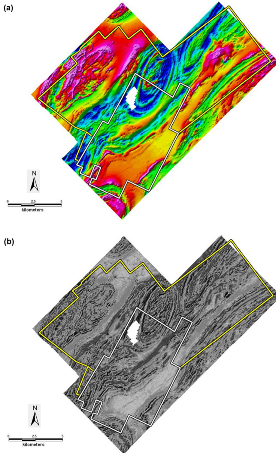
Figure 2.2. Gridded heli-borne gradiometric magnetic data over the Rössing mine lease (white border) and accessory works area (yellow border). (a) Total magnetic intensity reduced to pole (TMI RTP). (b) First vertical derivative of the TMI RTP. Gridded to 25 m and shaded with illumination from the northwest to highlight the principal structural trends. Figure is centred on 506000 mE, 7515000 mN.
