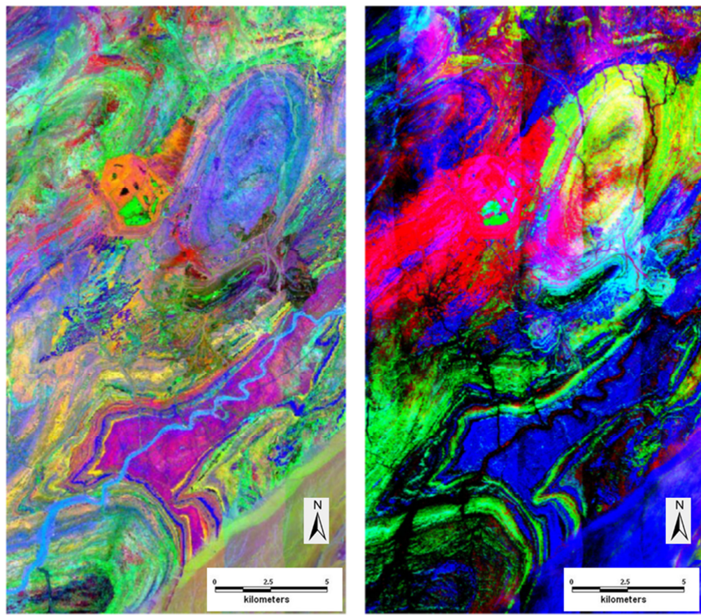
Figure 2.12. The minimum noise fraction (M.N.F.) transform applied to Rössing area HyMap data, bands 10-11-12 (left) and 7-8-9 (right); from Caballero (2009). See text for explanation. Figure is centred on 505000 mE, 7513000 mN.
