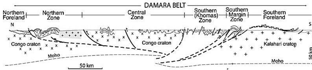
Figure 1.6. North-south simplified structural profile of the Damara Belt (from Hoffmann, P.F., 2005., 2008, after Miller and Grote, 1988)
