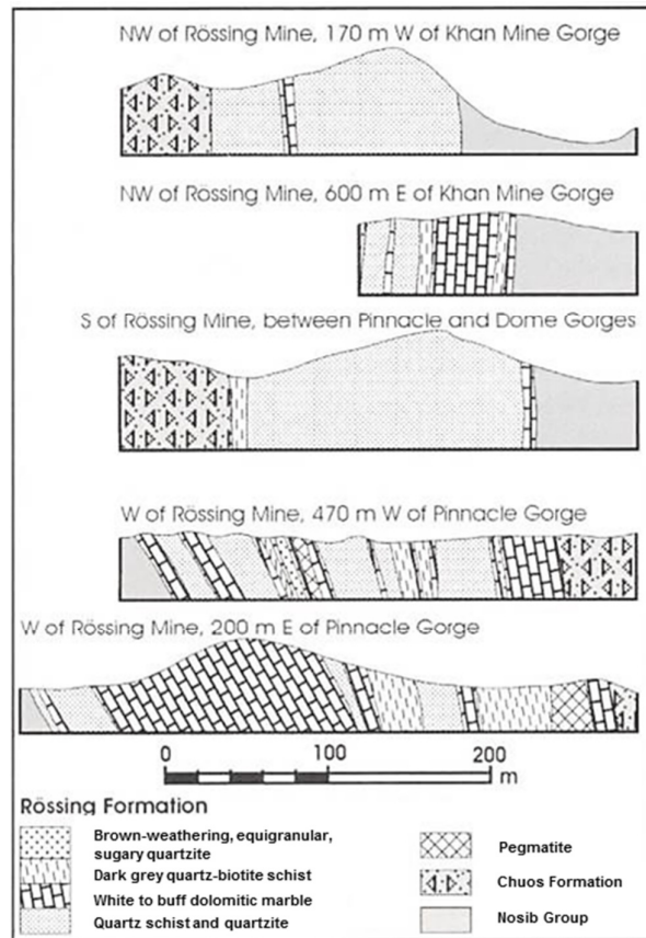
Figure 3.6. Lithological variability of the Rössing Formation in the vicinity of the Rössing mine. From Miller (2008) after Smith (1965). For locations see Figure 1.2; Pinnacle Gorge is assumed to be located between Panner Gorge and Rossing SJ.
