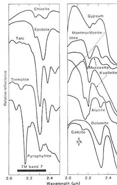
Figure 2.6. Selected laboratory mineral spectra showing diagnostic absorption and reflectance features. Spectra are arranged vertically for comparison. The bandwidth of band 7 of the Landsat T.M. sensor (see also Figure 2.4 and Chapter 2.3.2) is also shown and discussed in the text. Note the shift to the right in absorption features between calcite and dolomite which allows these minerals to be separated in hyperspectral imagery in the project area (see Figure 3.8). From Lillesand et al. (2008).
