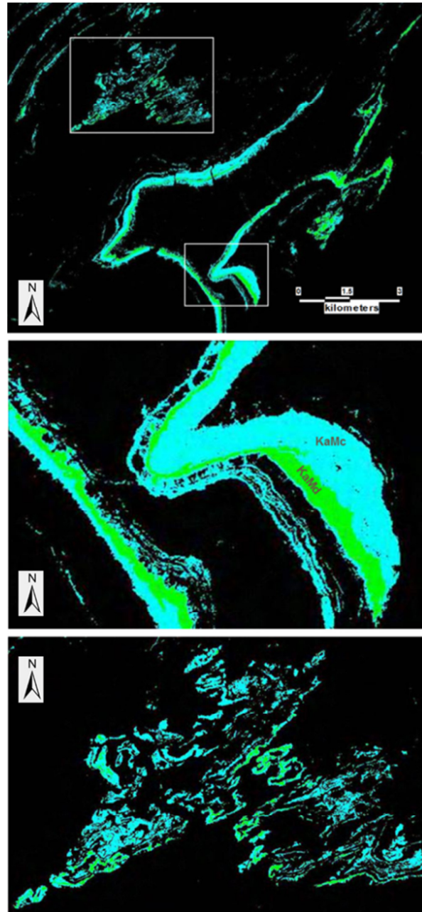
Figure 3.8. Hyperspectral carbonate end-member images showing examples of the distribution of calcite and dolomite in the Rössing and Karibib Formations. Upper image: overview of the areas shown in the lower two images; middle image: detail of the Karibib Formation marbles showing 1) a lower calcitic member (cyan, KaMc), 2) a middle dolomitic member (green, KaMd) and 3) an upper mixed calcitic marble-non-carbonate member; lower image: detail of calcite (cyan) versus dolomite (green) distribution in the general area of Panner Gorge and SH showing that the lower marble in the Rössing Formation is variably dolomitised. For location refer to Appendix II.
