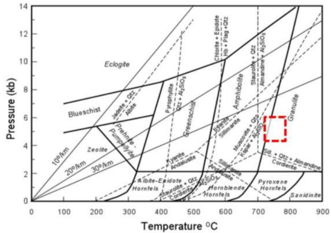
Figure 5.6. Temperature pressure mineral stability plot showing the approximate position of peak metamorphic assemblages in the Rössing area (red box) based on pelitic mineral paragenesis from Nash (1971) and this study, and thermobarometry of cordierite-bearing anatectic assemblages in Kuiseb schists of the project area indicating peak conditions of 750 °C and 5 kbar in the study of Ward et al. (2008).
