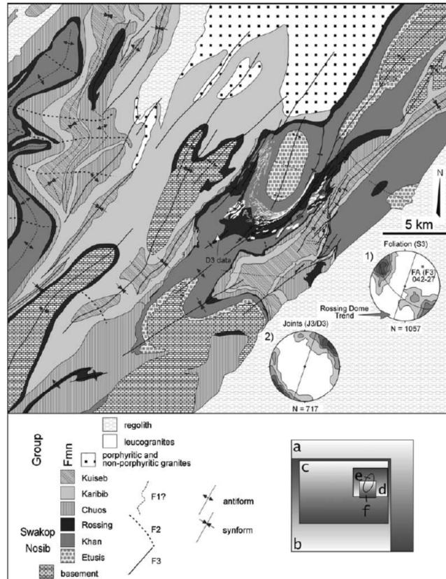
Figure 2.1. Compilation of geological mapping of the Rössing mine area encompassing the work of Basson and Greenway (2004), Smith (1965), Jacob (1974), Anderson and Nash (1997), Oliver and Kinnaird (1996) and Jacob and Kerber (1997); from Basson and Greenway (2004). Contoured equal area, best fit stereonet from Jacob and Kerber (1997) are: (1) S_3 data with best-fit F_3 fold axes of 042-27^\circ ; and (2) J_3 joint data, which defines a northwest-southeast trending joint set. The approximate source of this data is indicated as 'D 3 data' on the map – this data is included in this project compilation (see Chapter 2.5.1). Note that the Arandis Formation here is included in the Karibib Formation.
