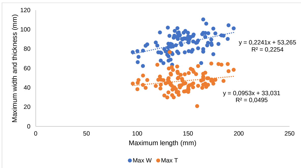
Figure 7.37: Correlation of maximum length (mm) and maximum width and thickness of LCTs (mm)
