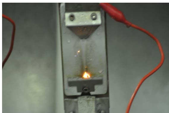
Figure C.4: Visible “track” marks
