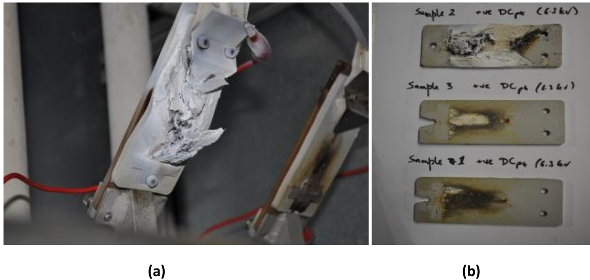
Figure 15: (a) Sample 2 burnt all the way through, and (b) all 3 samples after the test.
