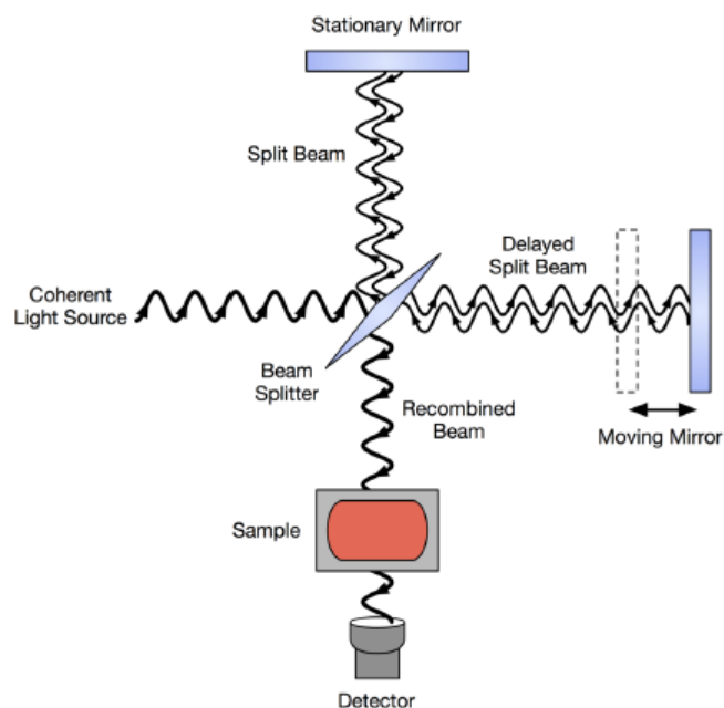
Figure B.8: Schematic diagram of a Michelson interferometer, configured for FTIR
