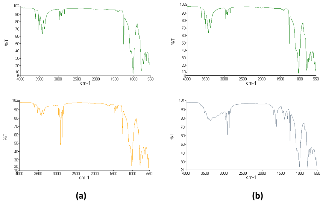
Figure 19: FTIR comparisons between (a) +6.3 kV dc (orange) and (b) -6.3 kV dc (blue) against the control (green)
