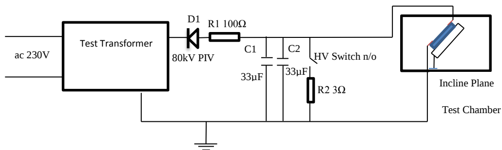
Figure B.4: Circuit diagram for negative dc setup
