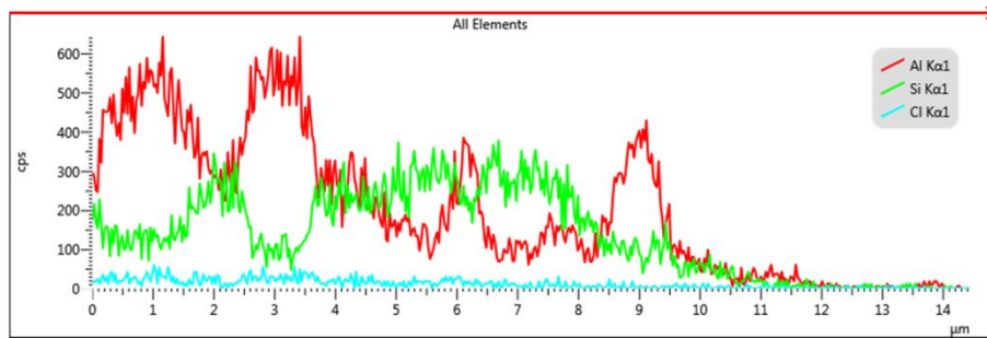
Figure D.22: EDS scan of positive 6.3 kV dc sample
