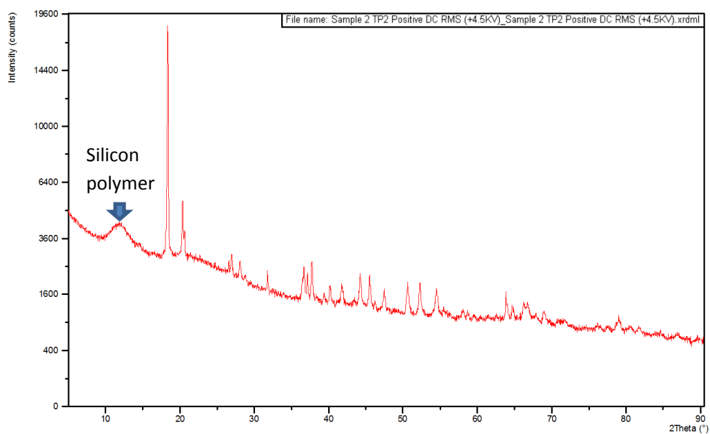
Figure D.26: XRD result for the positive 4.5 kV dc sample
