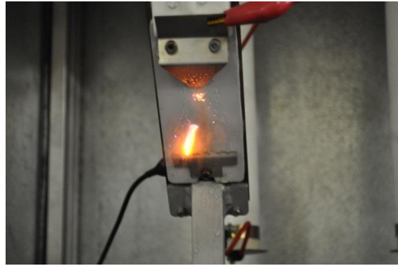
Figure C.39: “Long” arcs observed
