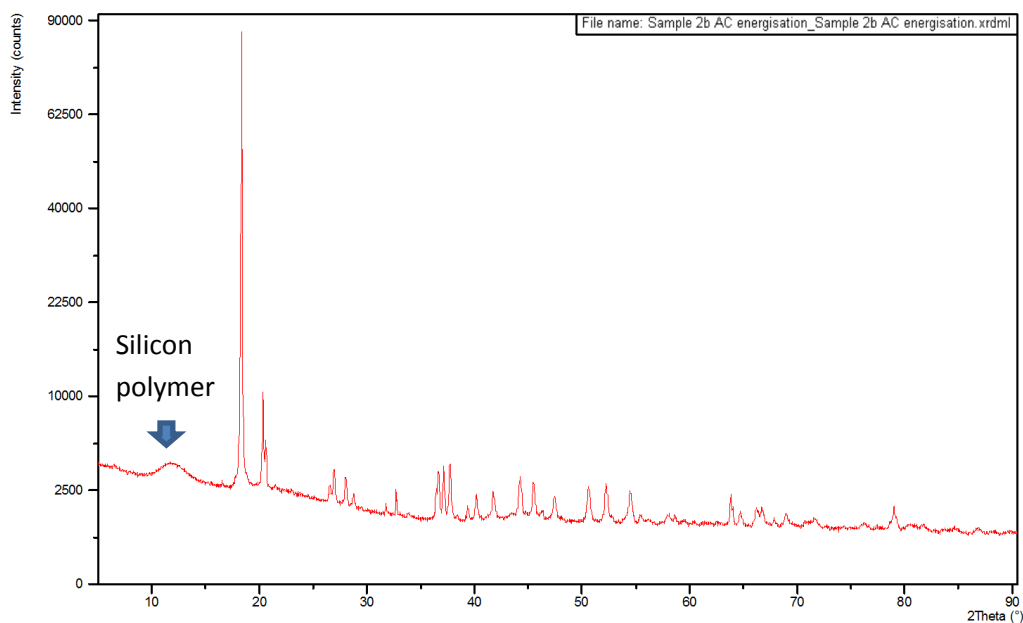
Figure D.25: XRD result for the ac sample
