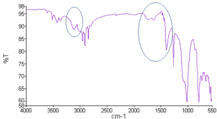
Figure D.8: FTIR spectrum of AC sample – 1cm away from damage area
