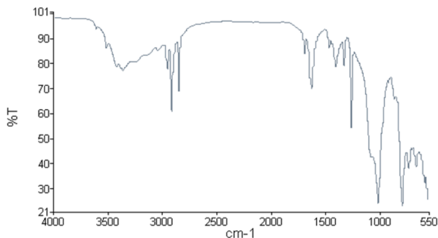
Figure D.16: FTIR of negative 6.3 kV dc sample – 1 cm away from damage area
