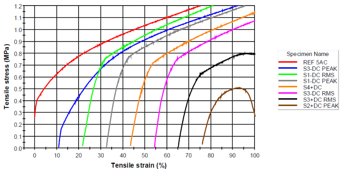
Figure D.30: Tensile test on damaged / aged samples
