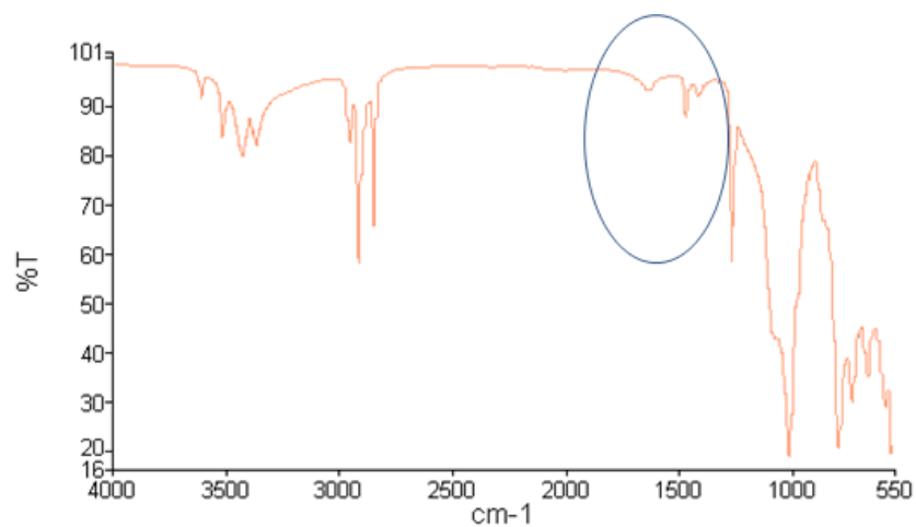
Figure D.9: FTIR spectrum of AC sample – damage area
