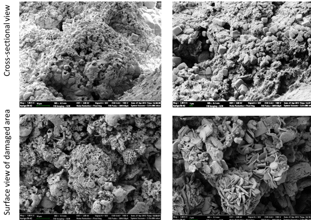
Figure D.2: SEM analysis of ac samples
