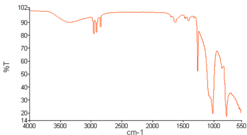
Figure D.17: FTIR of negative 6.3 kV dc sample – damage area
