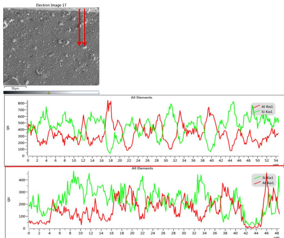
Figure D.18: EDS scan of the control sample with two linescans
