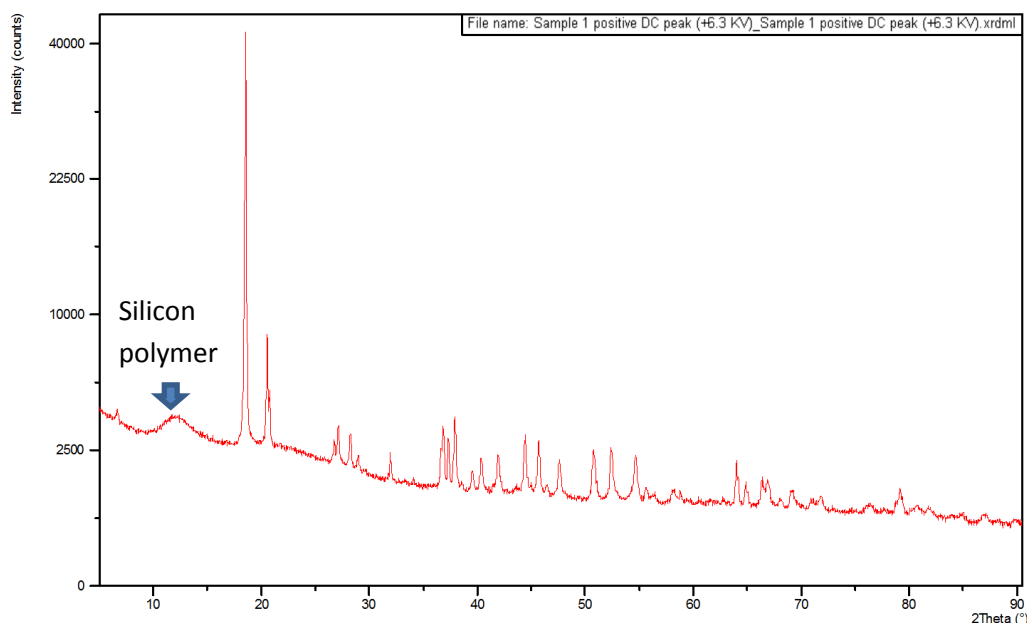
Figure D.28: XRD result for the positive 6.3 kV dc sample
