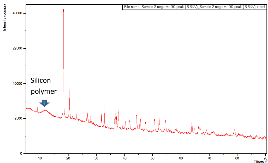
Figure D.29: XRD result for the negative 6.3 kV dc sample
