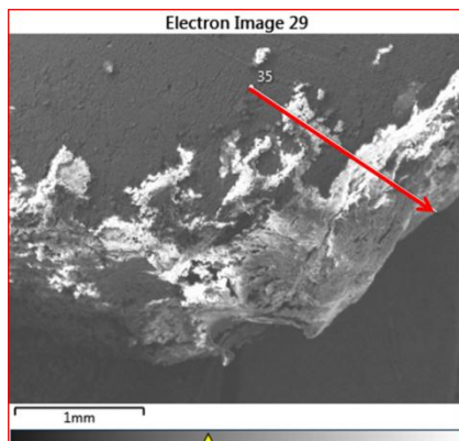
Figure D.20: EDS Scan of positive 4.5 kV dc sample
