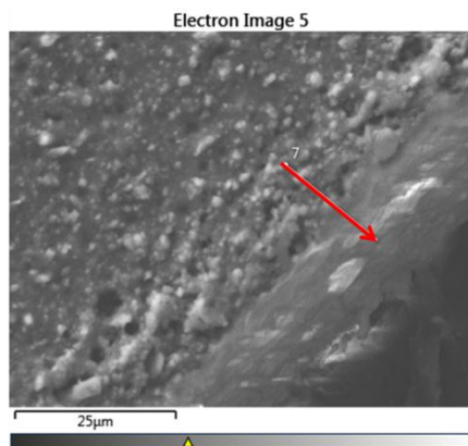
Figure D.22: EDS scan of positive 6.3 kV dc sample
