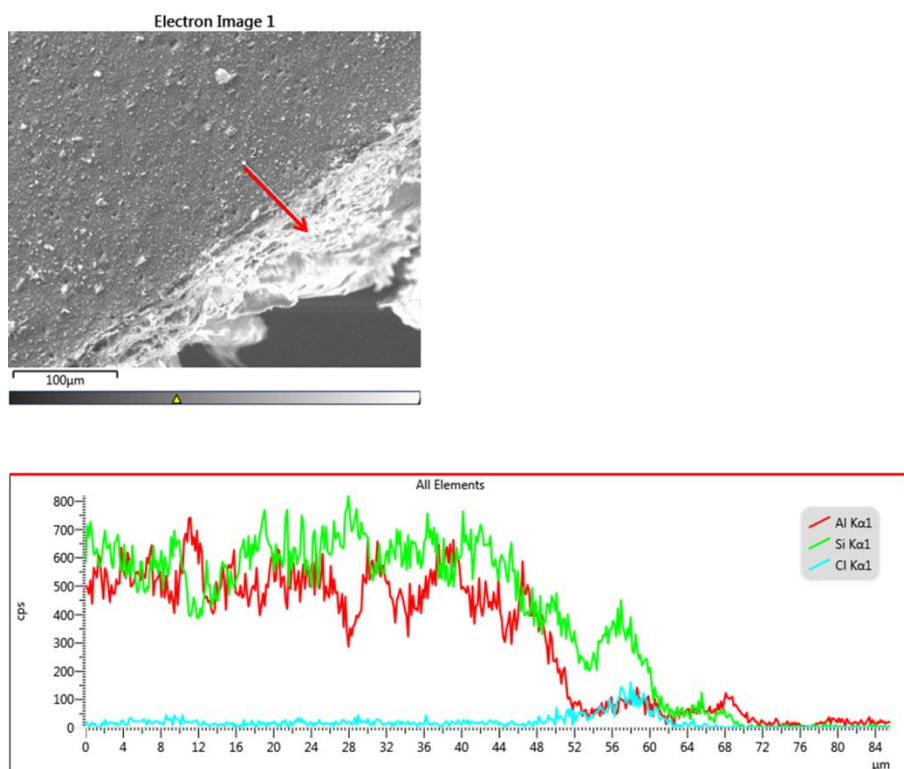
Figure D.19: EDS scan of the ac sample
