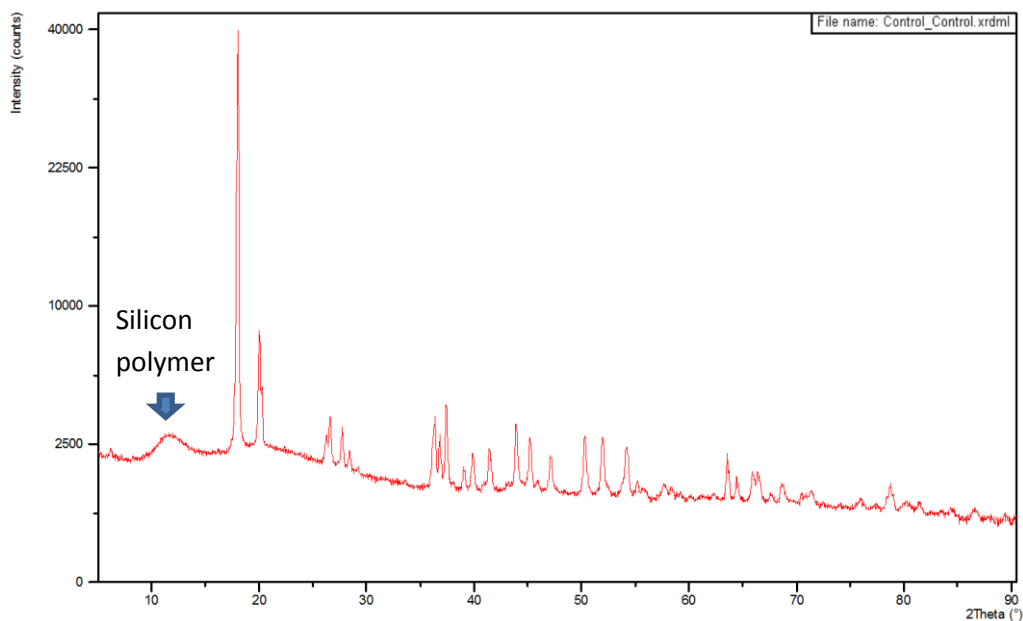
Figure D.24: XRD result for the control sample
