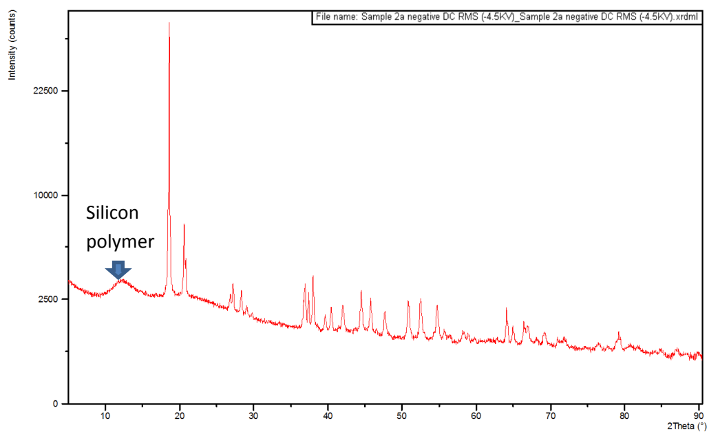
Figure D.27: XRD result for the negative 4.5 kV dc sample
