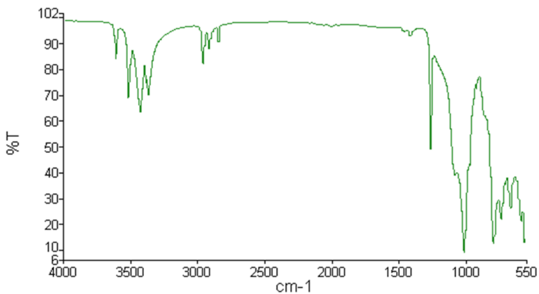
Figure B.9: FTIR spectrum of the control sample of HTV silicone rubber
