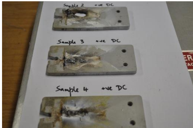
Figure 9: All three samples showing signs of severe erosion
