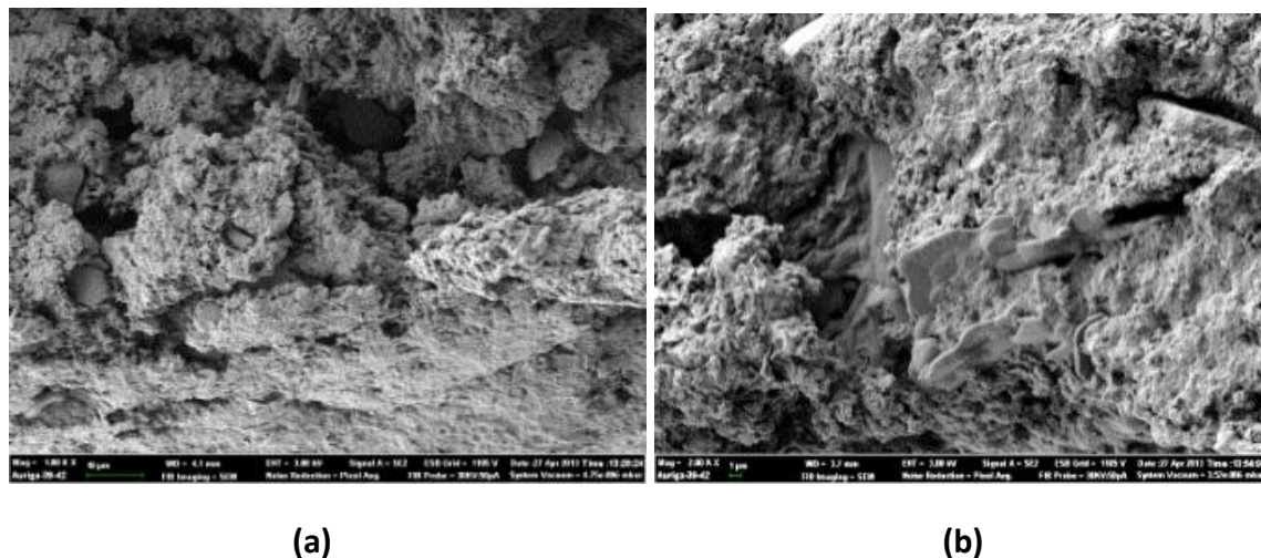
Figure 18: Cross-sectional views of (a) +6.3 kV dc and (b) -6.3 kV dc
