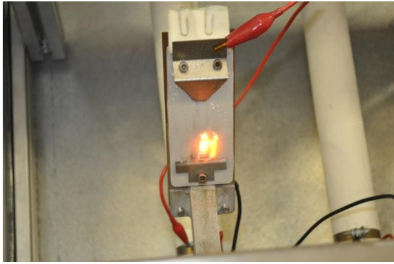
Figure C.49: Formation of arc roots
