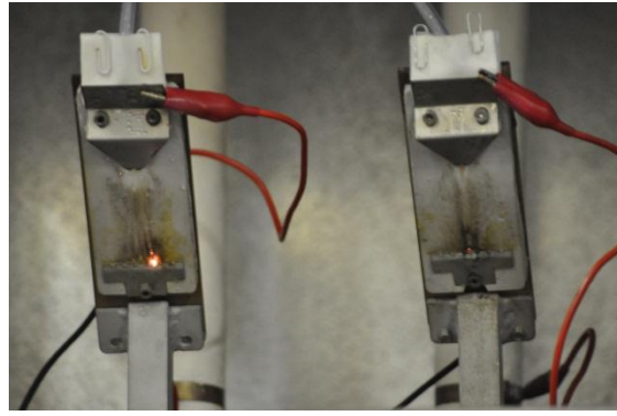
Figure C.9: Yellow-brown discolouration
