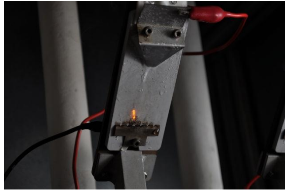
Figure C.31: Beginning of arc root on sample 2
