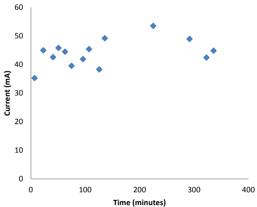
Figure C.55: Leakage current graph
