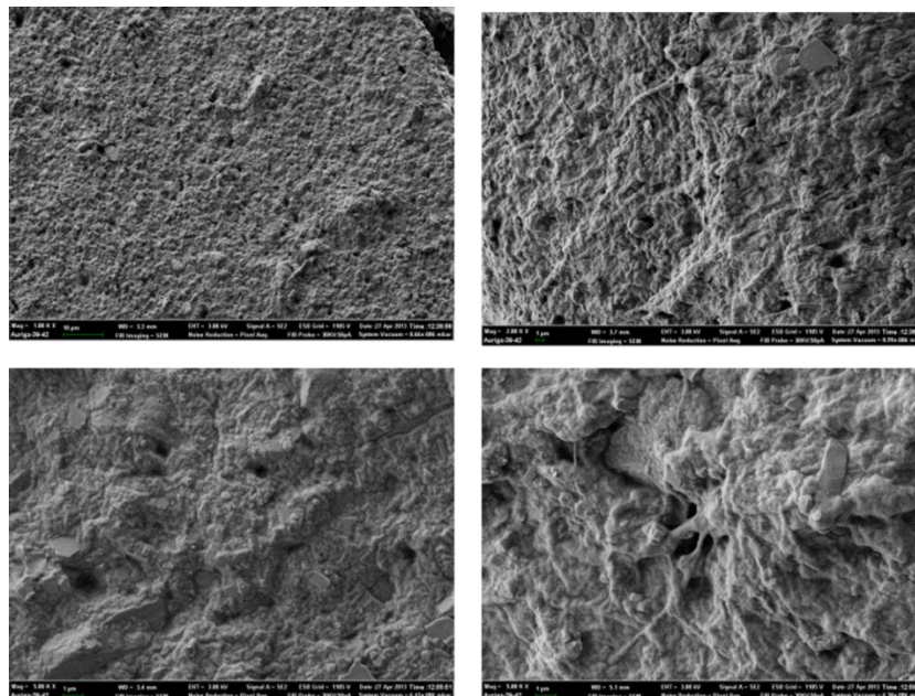
Figure B.7: SEM images of the silicone rubber control sample
