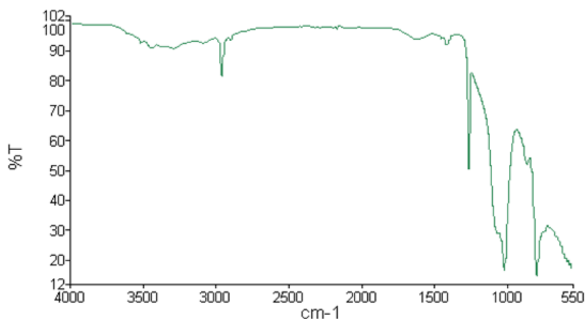
Figure D.12: FTIR of negative 4.5 kV dc sample – 1cm away from damage area
