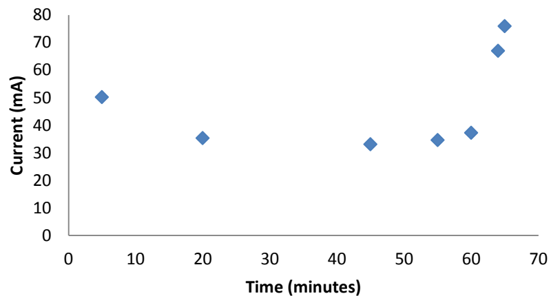
Figure C. 27: Leakage current graph
