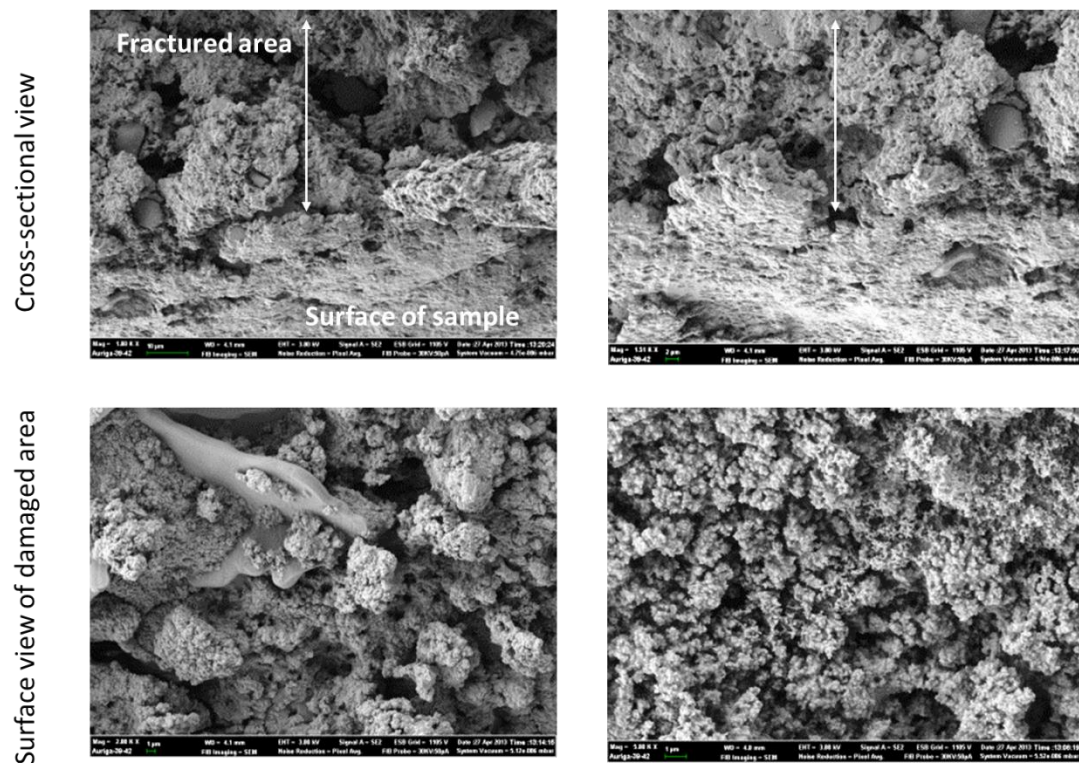
Figure D.5: SEM analysis of positive 6.3 kV dc sample
