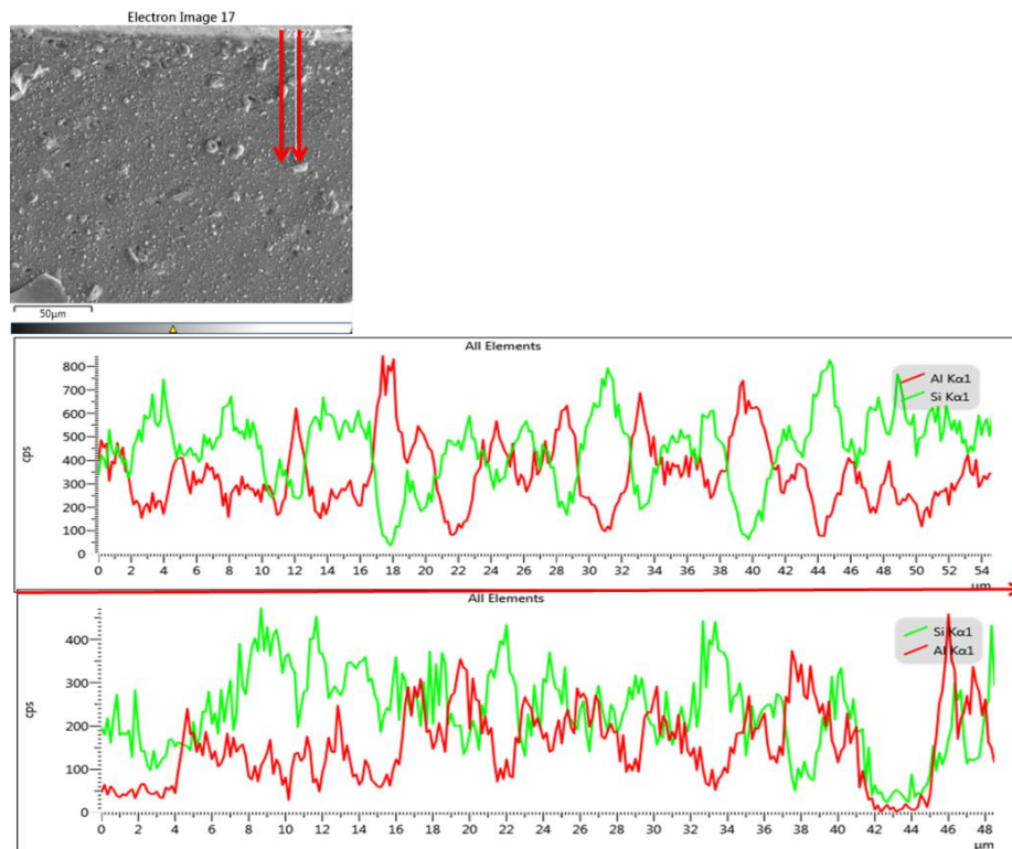
Figure B.10: EDS scan of the silicone rubber control sample used for the IPT tests
