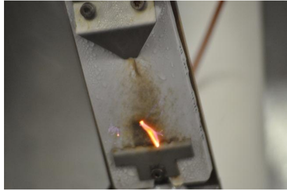
Figure C.18: Development of arc
