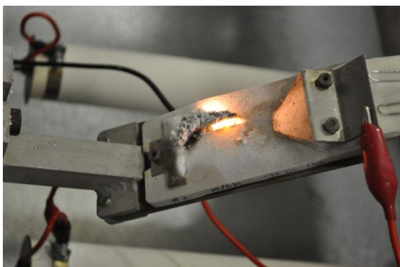
Figure C.34: Erosion approx. 50% of gap
