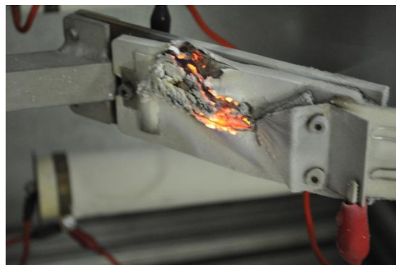
Figure C.35: Sample 2 after 42 minutes
