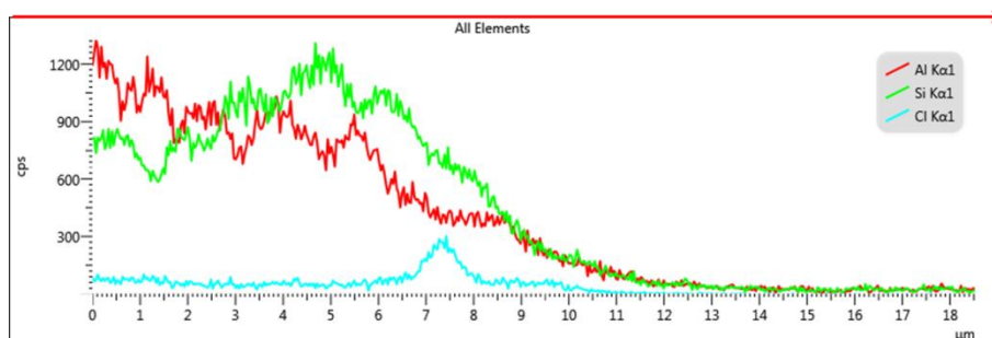
Figure D.23: EDS Scan of negative 6.3 kV dc sample
