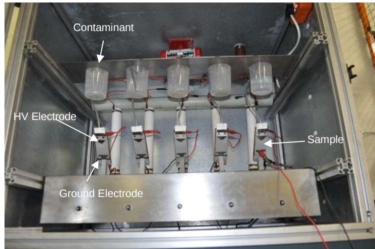
Figure 1: Inclined plane test setup
