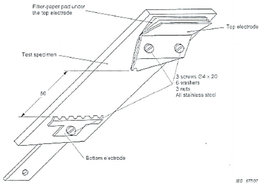
Figure B.1: Assembly of the electrodes – contaminant flows from top to bottom
