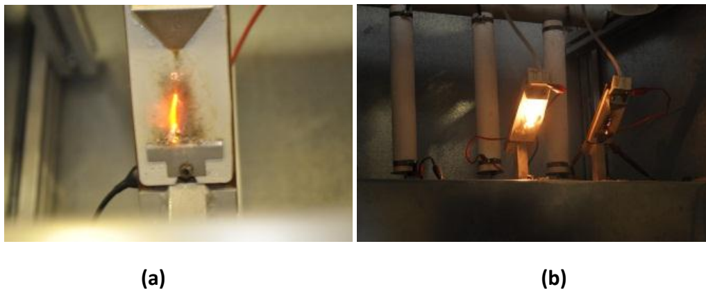
Figure 14: (a) Arcing and the starting of erosion in sample 2, and (b) small flames observed after 40 minutes
