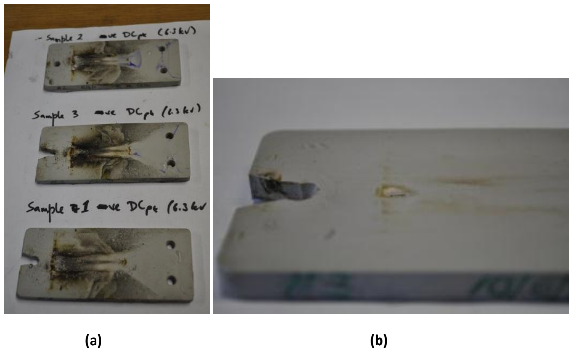
Figure 17: (a) The samples at the end of the negative 6.3 kV dc test and, (b) sample 3 after cleaning.
