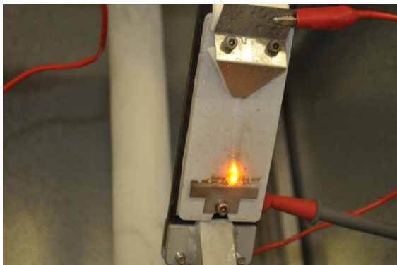
Figure C.32: Arc root on Sample 1
