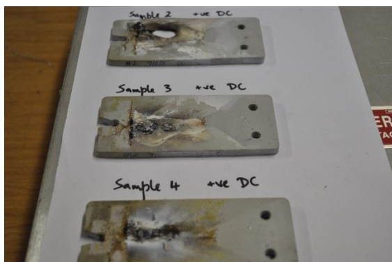
Figure C.26: Samples after testing
