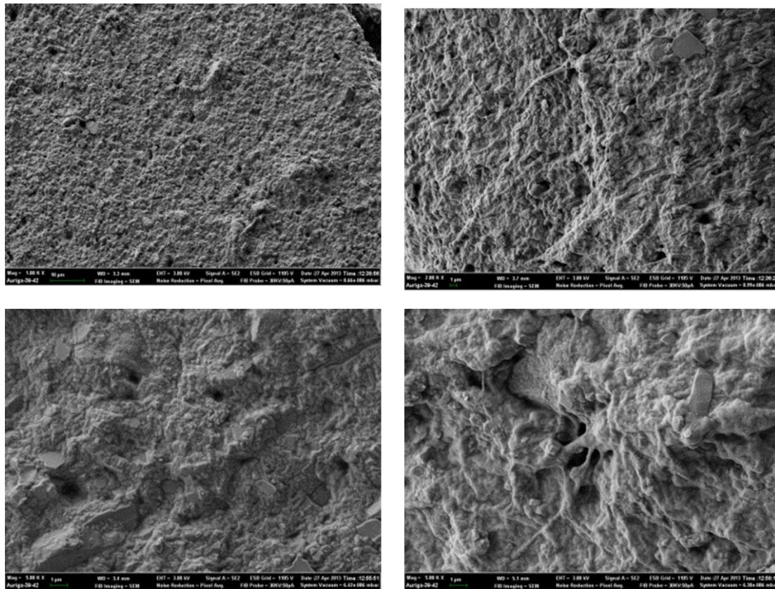
Figure D.1: SEM analysis of the control sample
