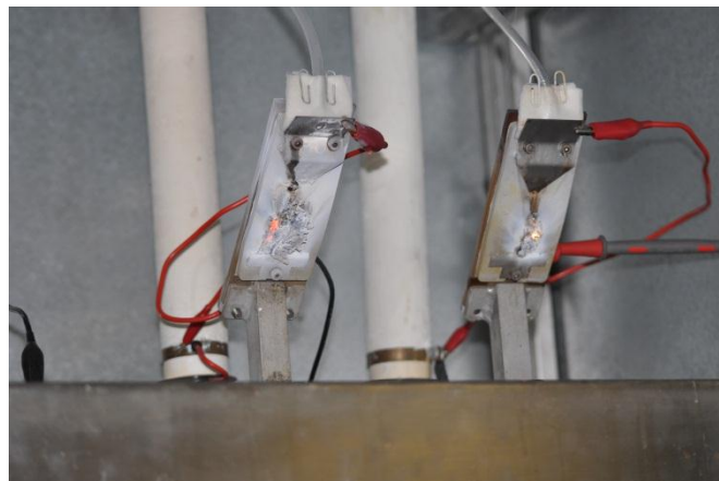
Figure C.23: Erosion on sample 2 (left) and sample 3 (right)
