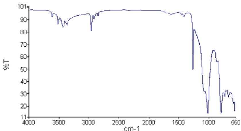
Figure D.10: FTIR of positive 4.5 kV dc sample – 1 cm away from damage area
