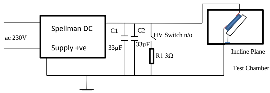
Figure B.3: Circuit diagram for positive dc setup
