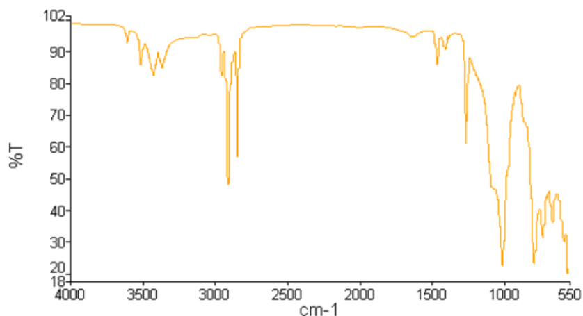
Figure D.14: FTIR of positive 6.3 kV dc sample – 1 cm away from damage area
