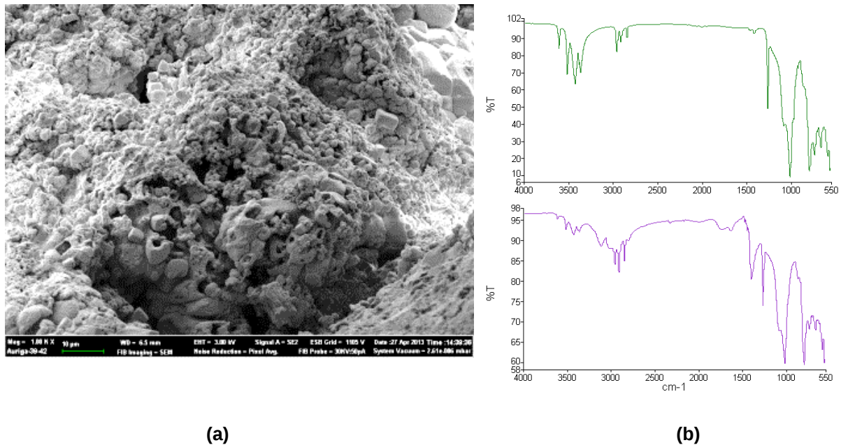
Figure 7: (a) Cross-sectional view of the ac sample and (b) the comparison in FTIR scan
