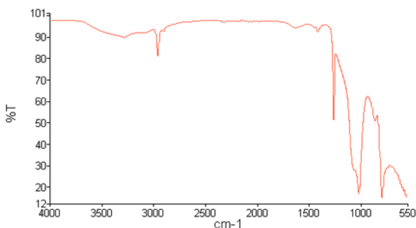
Figure D.11: FTIR of positive 4.5 kV dc sample – damage area
