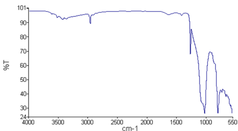
Figure D.13: FTIR of negative 4.5 kV dc sample – damage area
