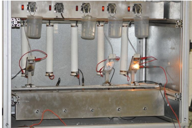
Figure C.22: Formation of arc root on sample 3, TP1
