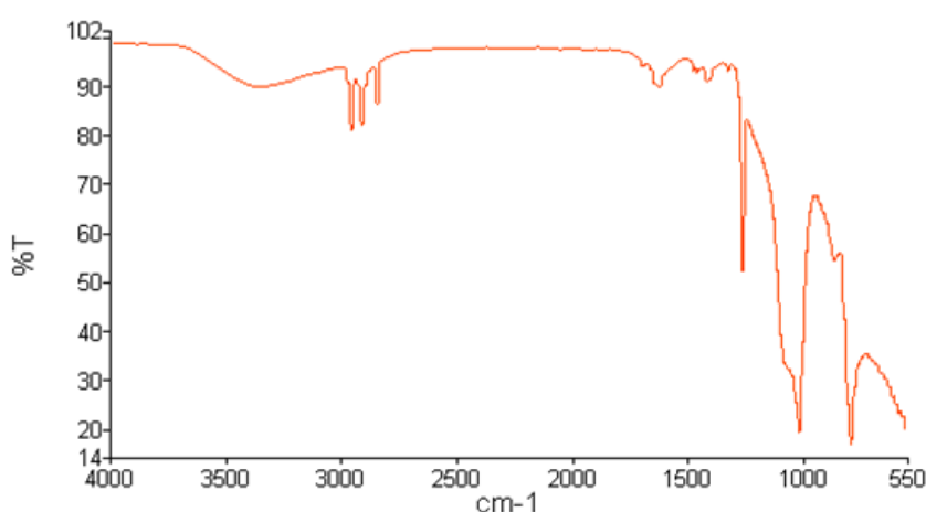
Figure D.15: FTIR of positive 6.3 kV dc sample – damage area
