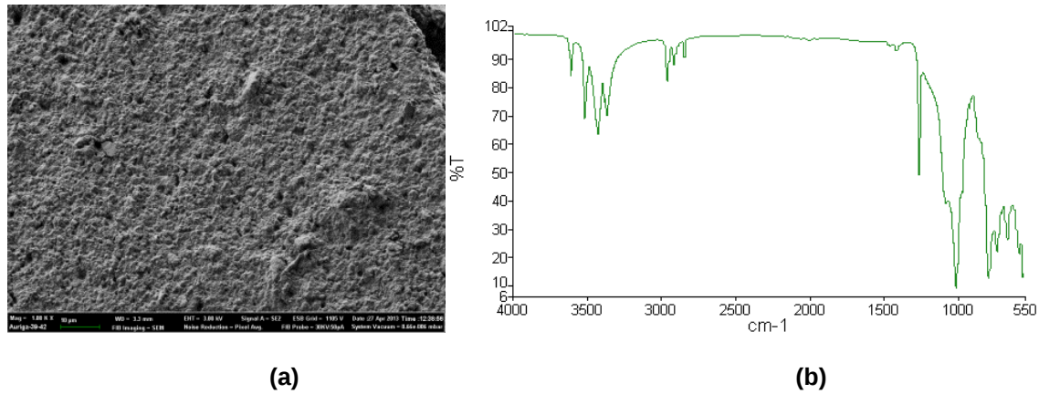
Figure 3: (a) Cross-sectional view of the control sample and (b) the FTIR spectrum
