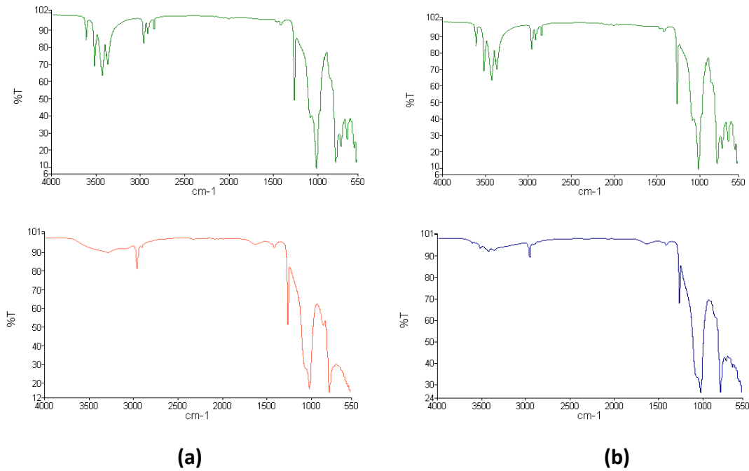
Figure 13: FTIR comparisons between (a) +4.5 kV dc (pink) and (b) -4.5 kV dc (blue) against the control (green)
