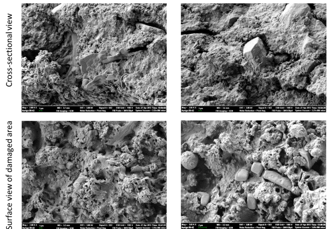
Figure D.6: SEM analysis of negative 6.3 kV sample
