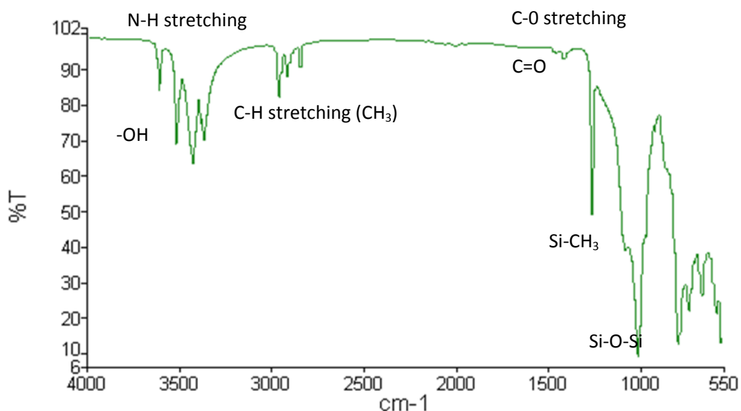
Figure D.7: FTIR spectra of the control sample
