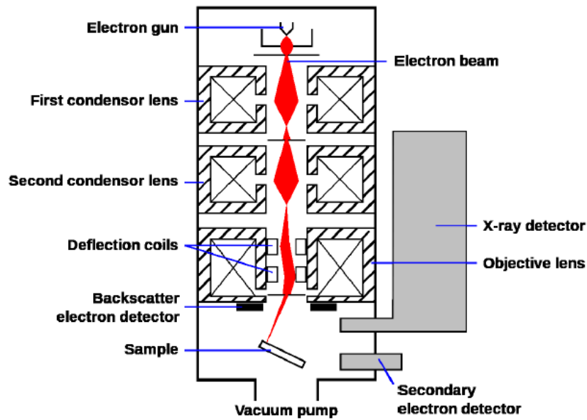
Figure B.6: Schematic diagram of a SEM
