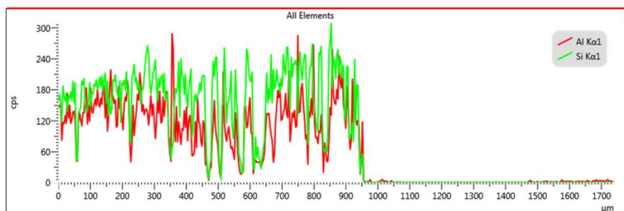
Figure D.21: EDS scan of negative 4.5 kV dc sample
