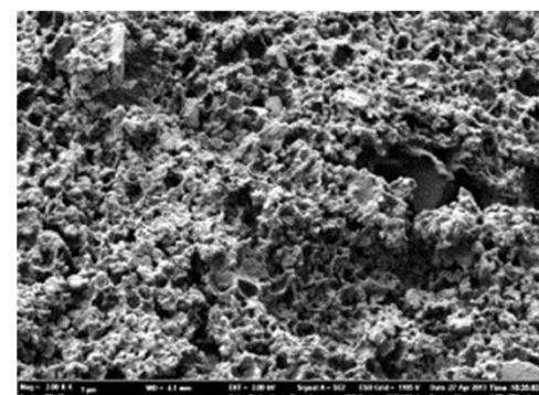
Figure D.4: SEM analysis of negative 4.5 kV dc sample
