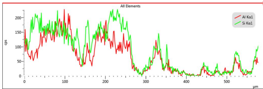
Figure D.20: EDS Scan of positive 4.5 kV dc sample
