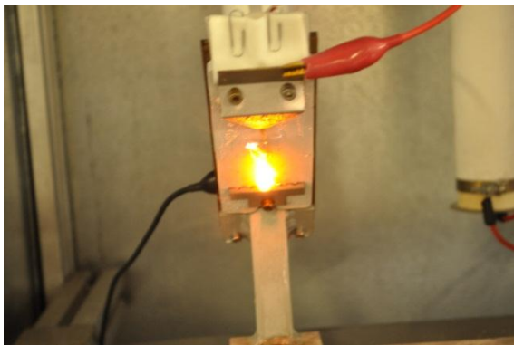
Figure C.40: Brighter arcs
