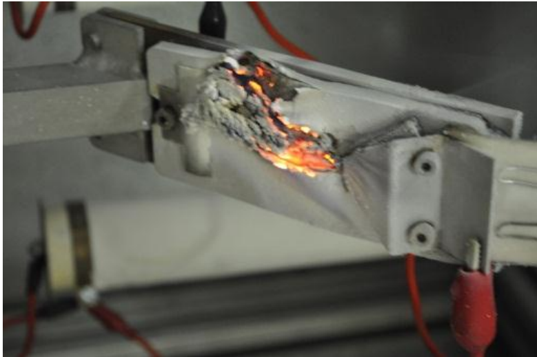
Figure 11: Severe erosion on sample 2 after 42 minutes
