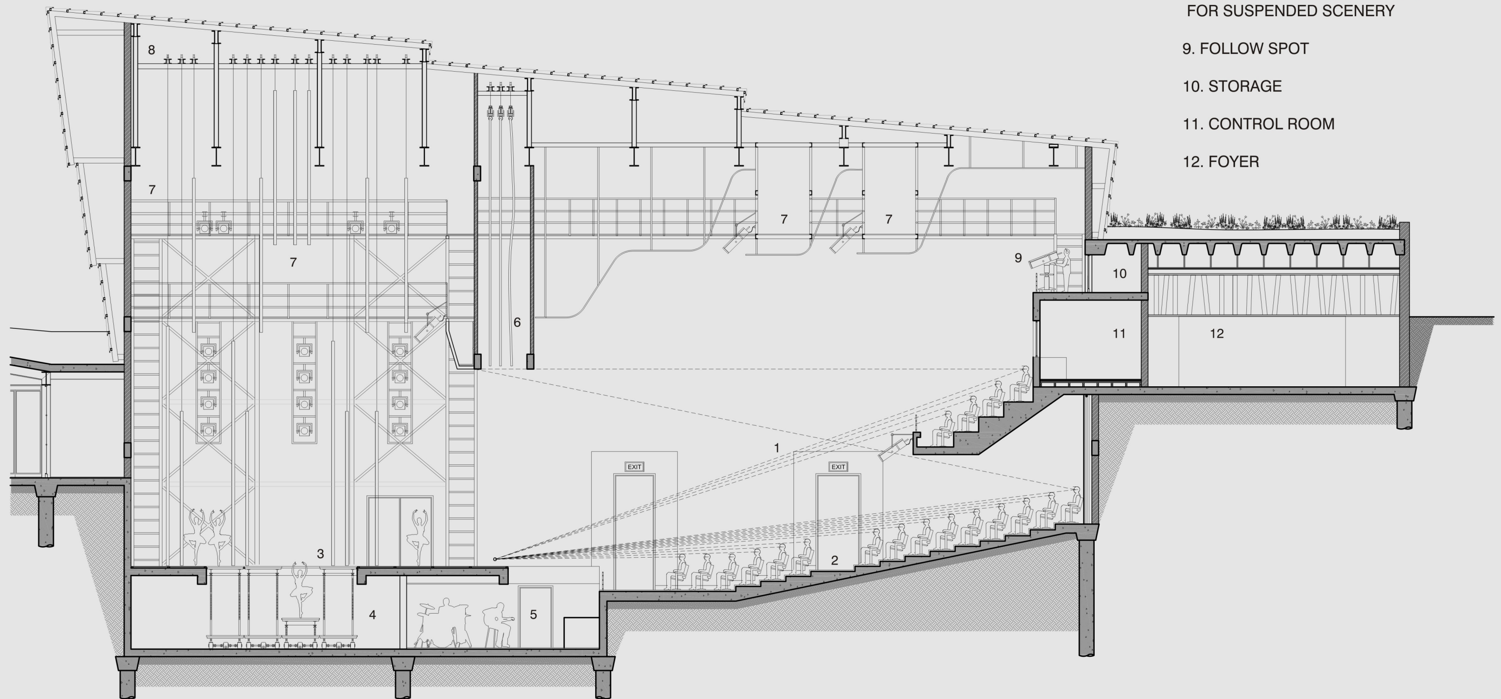
DETAIL SECTION THROUGH AUDITORIUM
