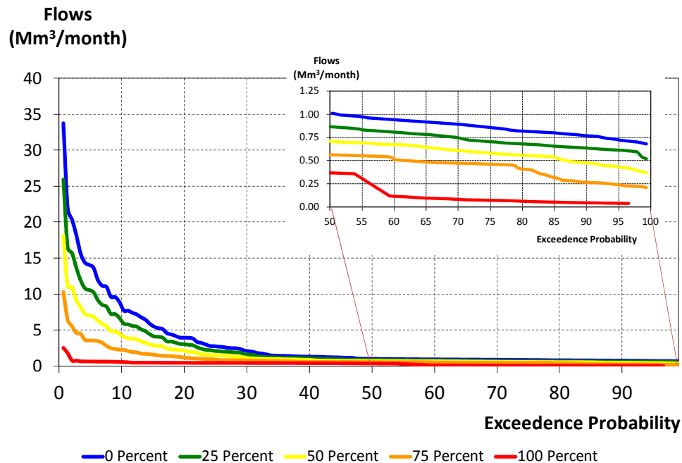
Figure 5.10 Flow Duration Curves for different levels of IRWH adoption in C52A obtained using WRSIM (Sejamoholo et al., 2008).
