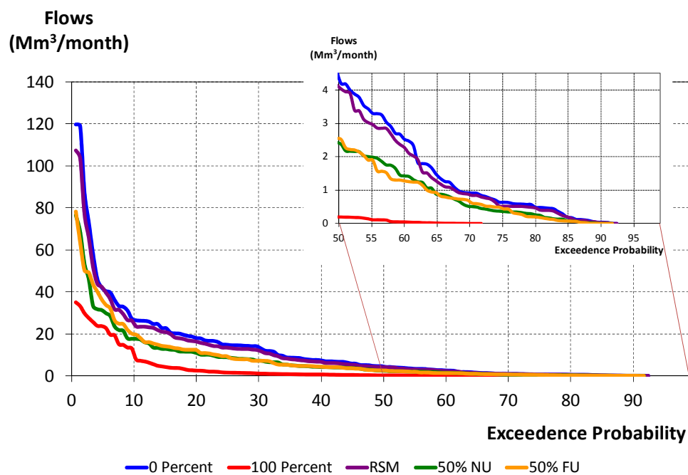
Figure 5.9 Flow Duration Curves for different levels of IRWH adoption in C52A obtained using SWAT.
