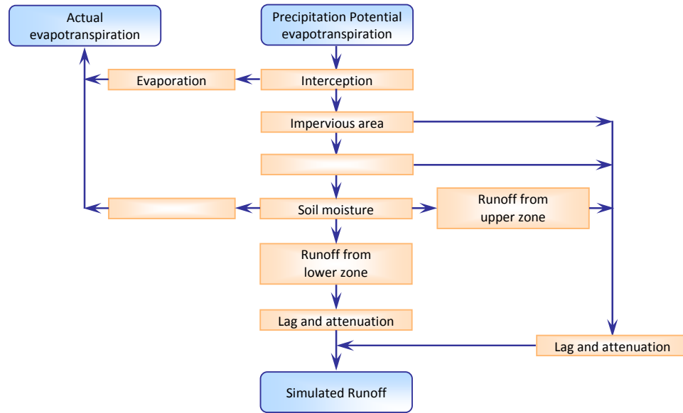
Figure 5.8 Core structure of the Pitman model (Pitman, 1973).
