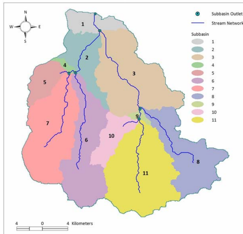
Figure 5.3 Stream network and Subbasins delineated by SWAT.
