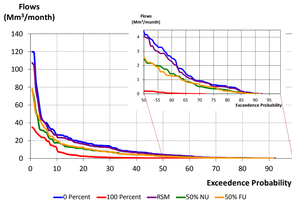
Figure 5.6 Flow Duration Curves for different levels of IRWH adoption C52A (SWAT).
