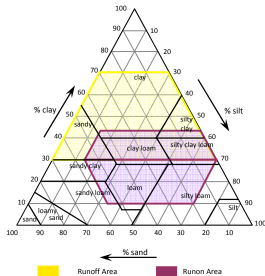
Figure 4.2. Soil texture triangle with RWH Runon and Runoff area (FAO, 2003).
