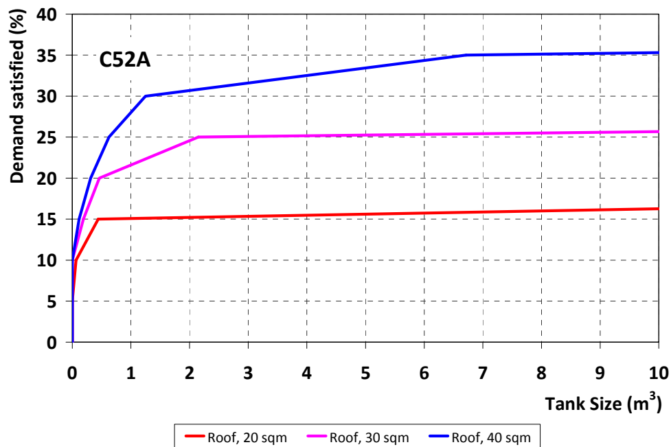
Figure 6.4 Percentage of demand satisfied for varying tank size and different roof areas in C52A.
