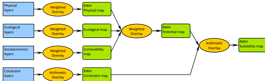
Figure 4.3 Schematic of the RSM showing the Potential model and Constraint sub-models.
