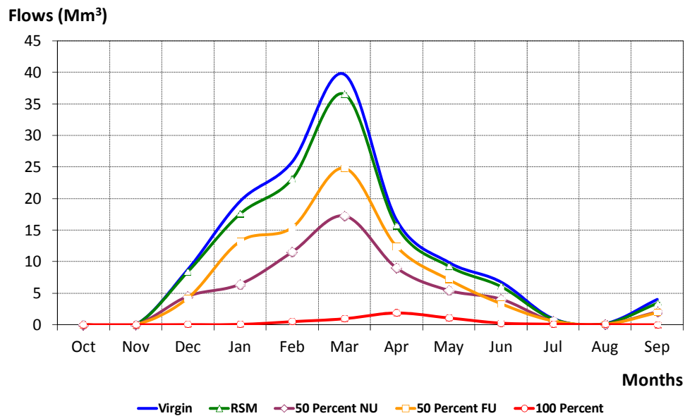
Figure 5.7 Median monthly hydrograph (October 1990 to September 1991) of different levels of IRWH adoption in C52A (SWAT).
