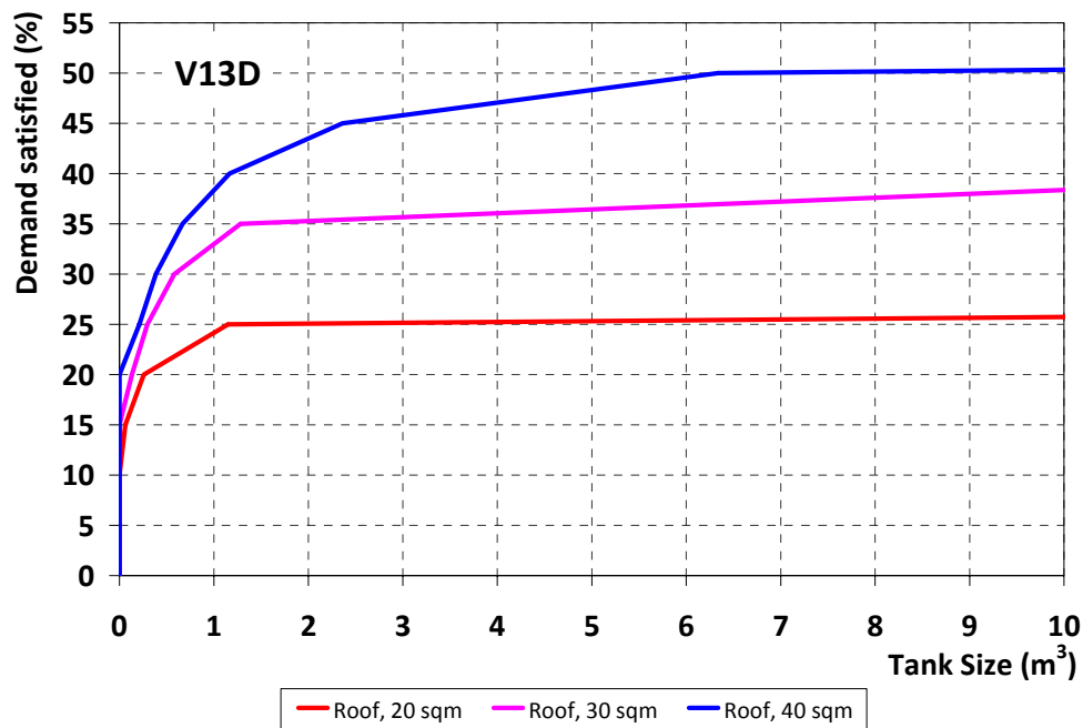
Figure 6.5 Percentage of demand satisfied for varying tank size and different roof areas in C52A.
