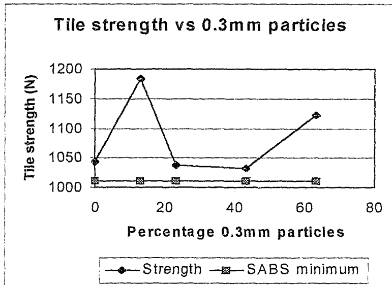
GRAPH H: Tile strengths relative to concentrations of 300 \mu m particles in river sand
