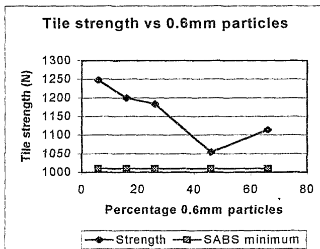
GRAPH G: Tile strengths relative to concentrations of 600 \mu m particles in river sand
