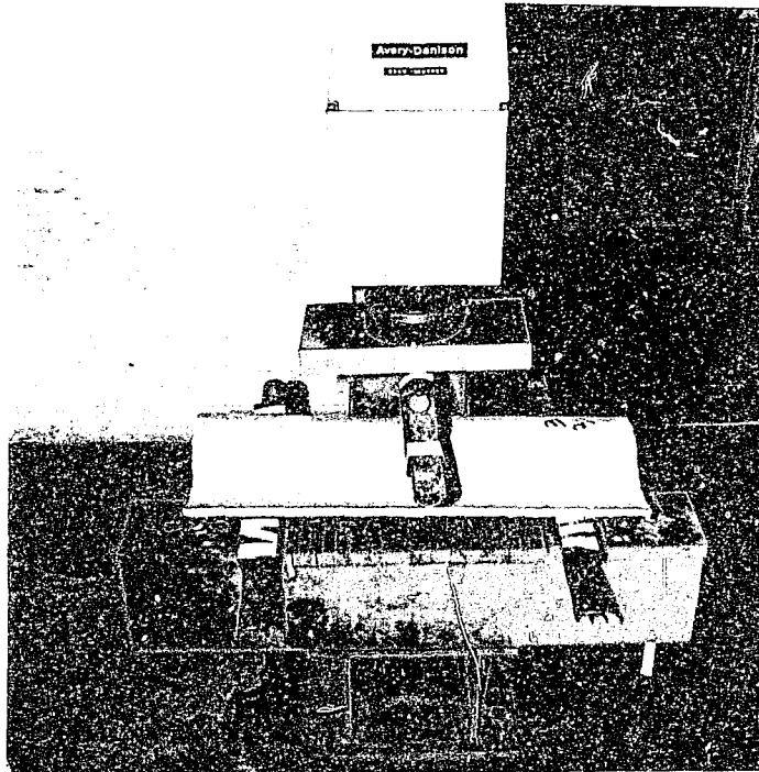
Figure 1: The beam crusher used to establish the transverse strength of the tiles
