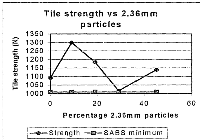
GRAPH E: Tile strengths relative to concentrations of 2360 \mu m particles in river sand
