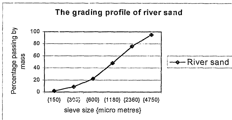
Graph.C: The natural grading profile of river sand
