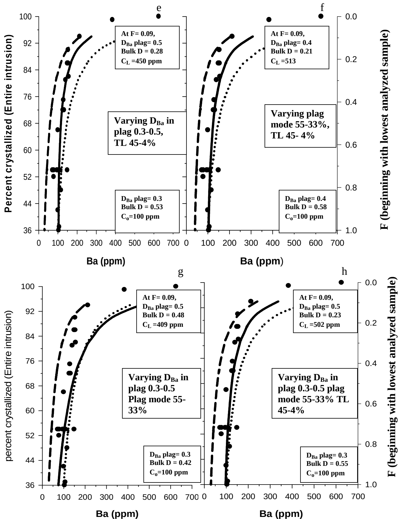
Fig. 5.5. cont. Calculated trends for barium in the Skaergaard intrusion from varying different parameters with crystallization.
