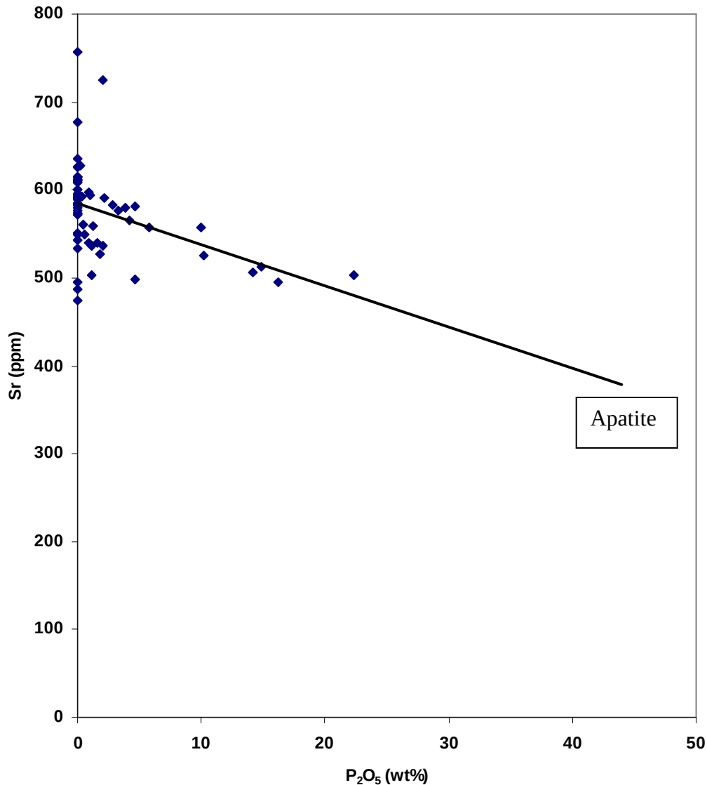
Fig. 4.3 Sr vs. P 2 O 5 contents for samples from 1400 m upward (which include the apatite-bearing interval) showing how a calculation can be made to correct for the presence of apatite.
