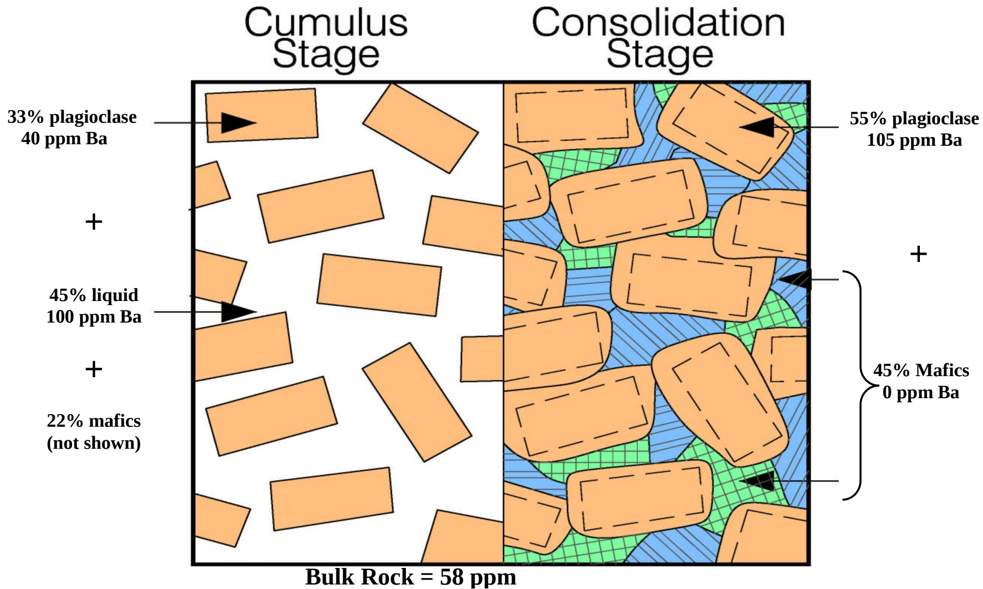
Fig. 5.1 Trapped Liquid Shift effect for barium in plagioclase showing its enormous effect. Original cumulus and re-equilibrated compositions differ by a factor of nearly three.
