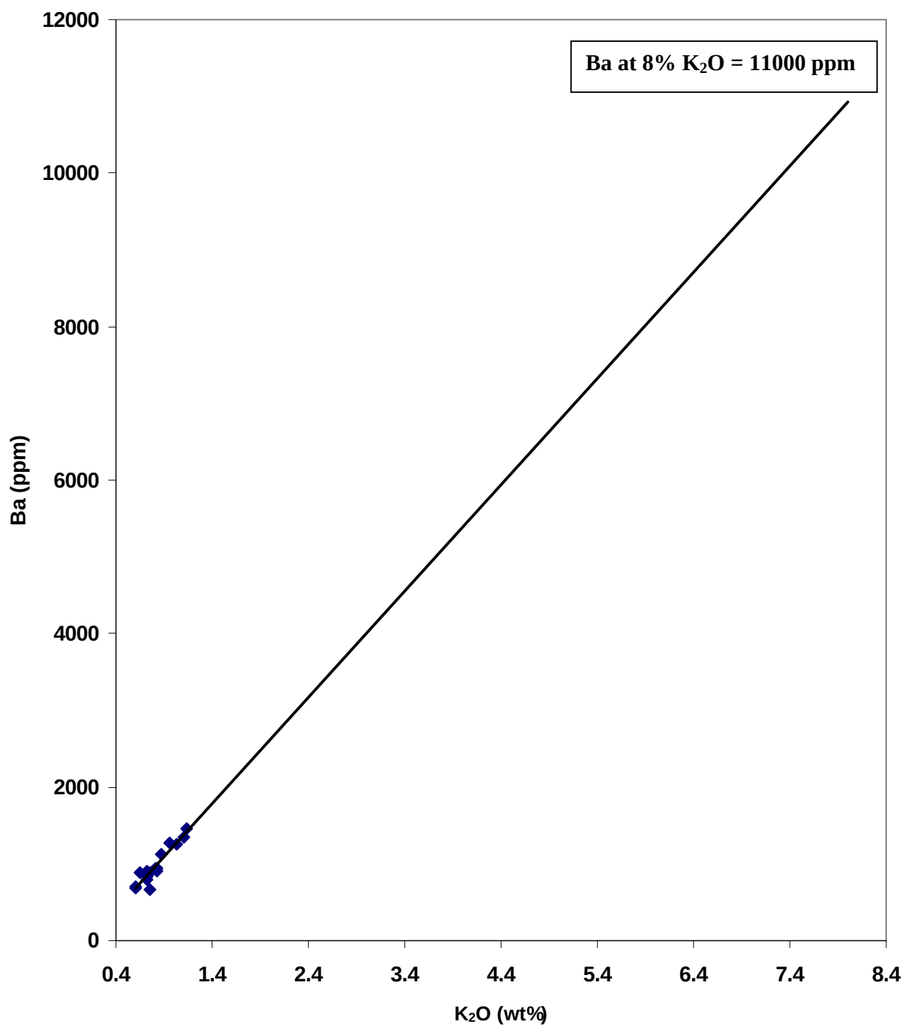
Fig. 4.6 Barium vs. K 2 O from analyses. Samples which report high K 2 O also have high Ba values hence contain significant alkali feldspar.
