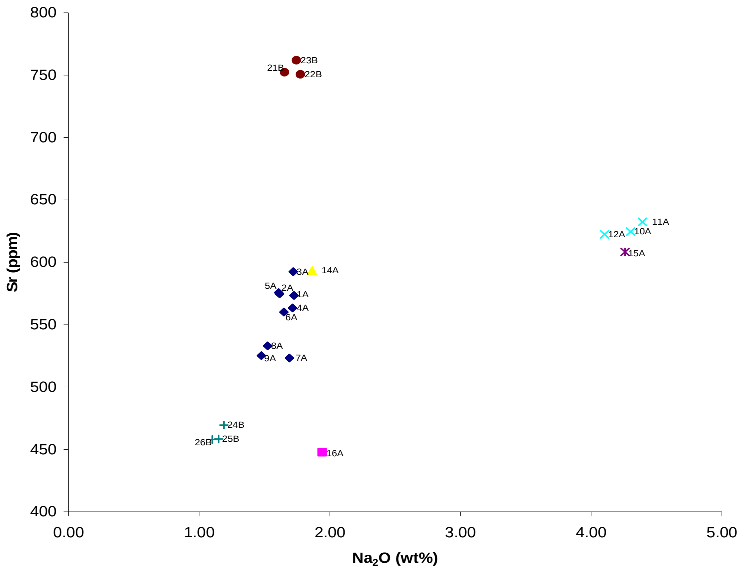
Fig.2B: Na 2 O vs Sr decrease for Citric acid dissolution experiments
