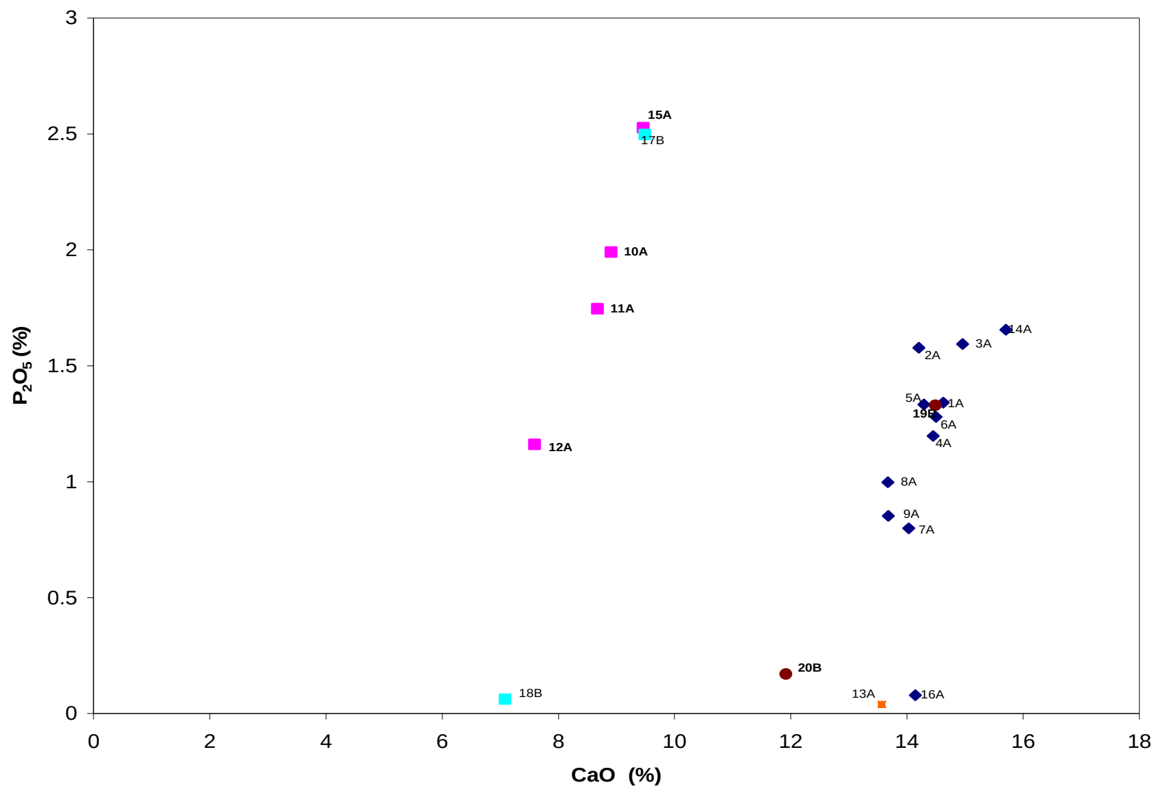
Fig. 1B:P 2 O 5 change with CaO from Citric acid Leaching. 2
