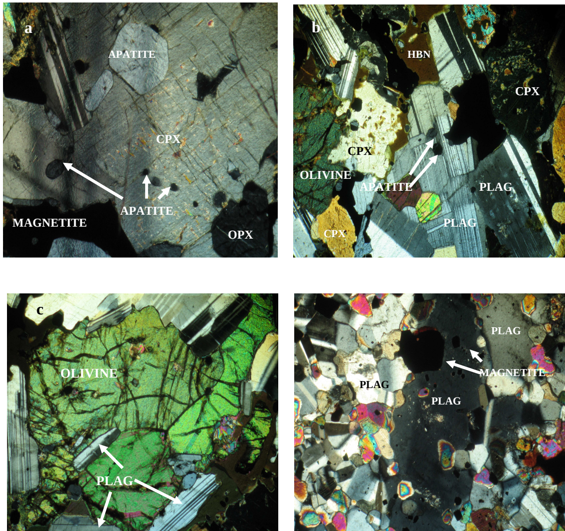
Fig. 3.3. Inclusions and composite grains a.)-1W604.5; apatite included in cpx b.)-1W545.7 apatite included in plagioclase c.)-1W545.7 plagioclase on grain boundary of olivine d.) Subhedral plagioclase and disseminated magnetite grains.
