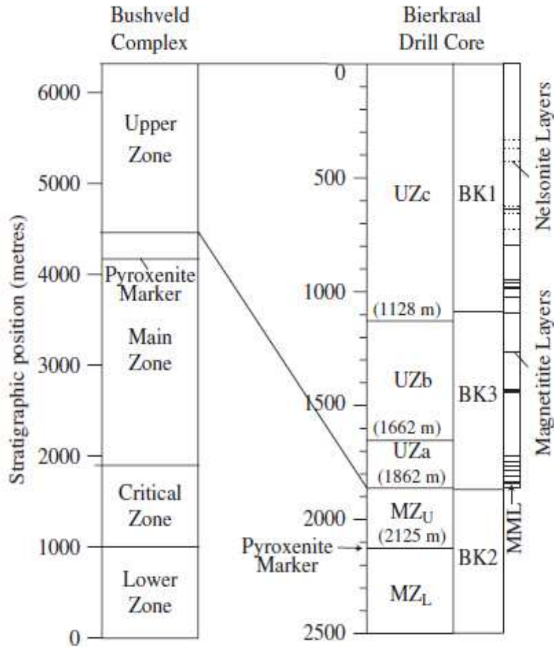
Fig. 2.2. Generalized stratigraphic section of the Bushveld Complex and combined Bierkraal drill cores. Subzones have been divided based on the appearance and disappearance of cumulus minerals (Tegner et al., 2006). BK1 and BK3 samples = 1W and 3W respectively for sample numbers.
