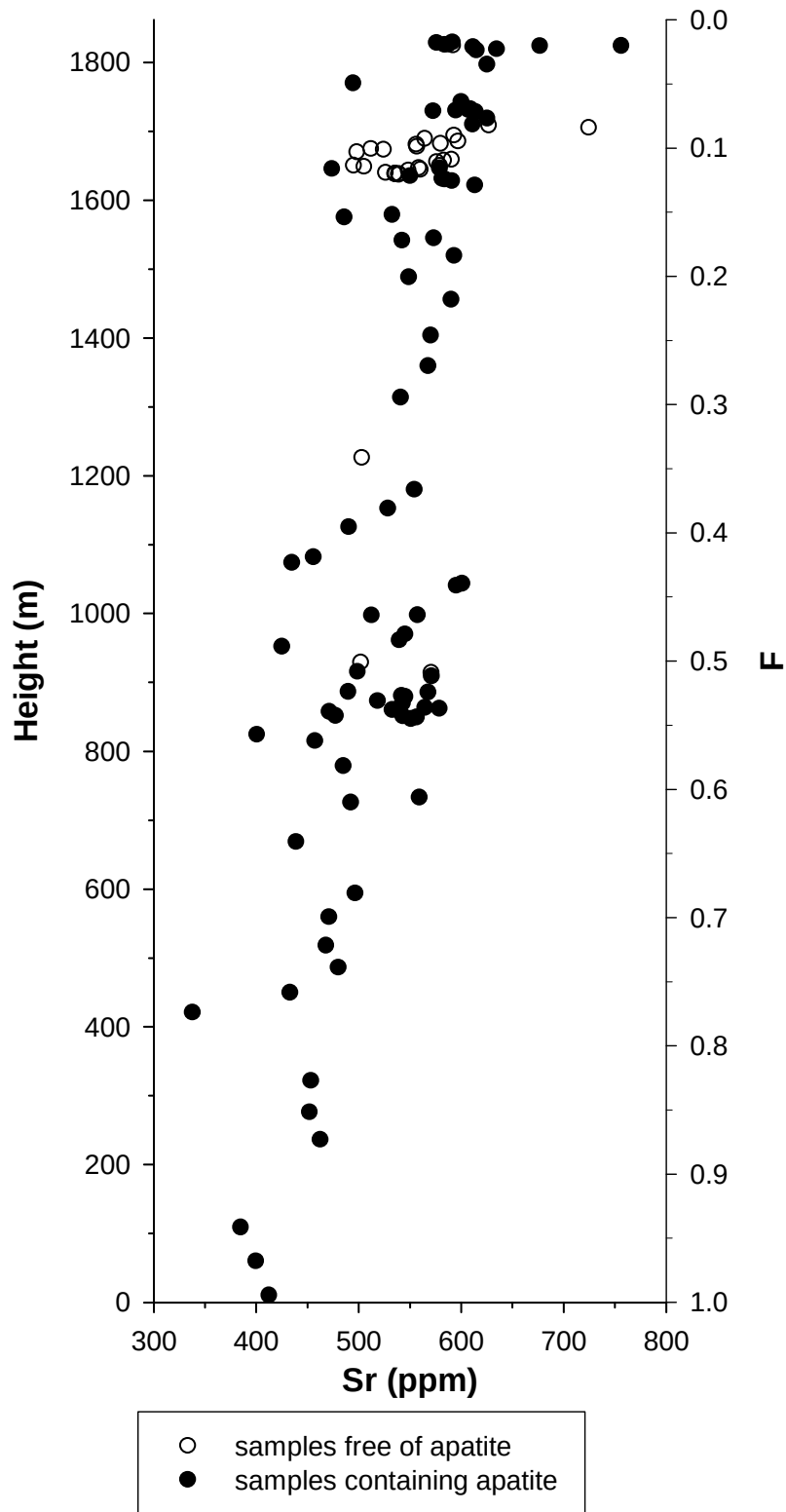
Fig. 4.2 Plots of Sr content vs. height and fraction of magma remaining showing the samples which contain apatite. Data are not corrected for the presence of apatite.
