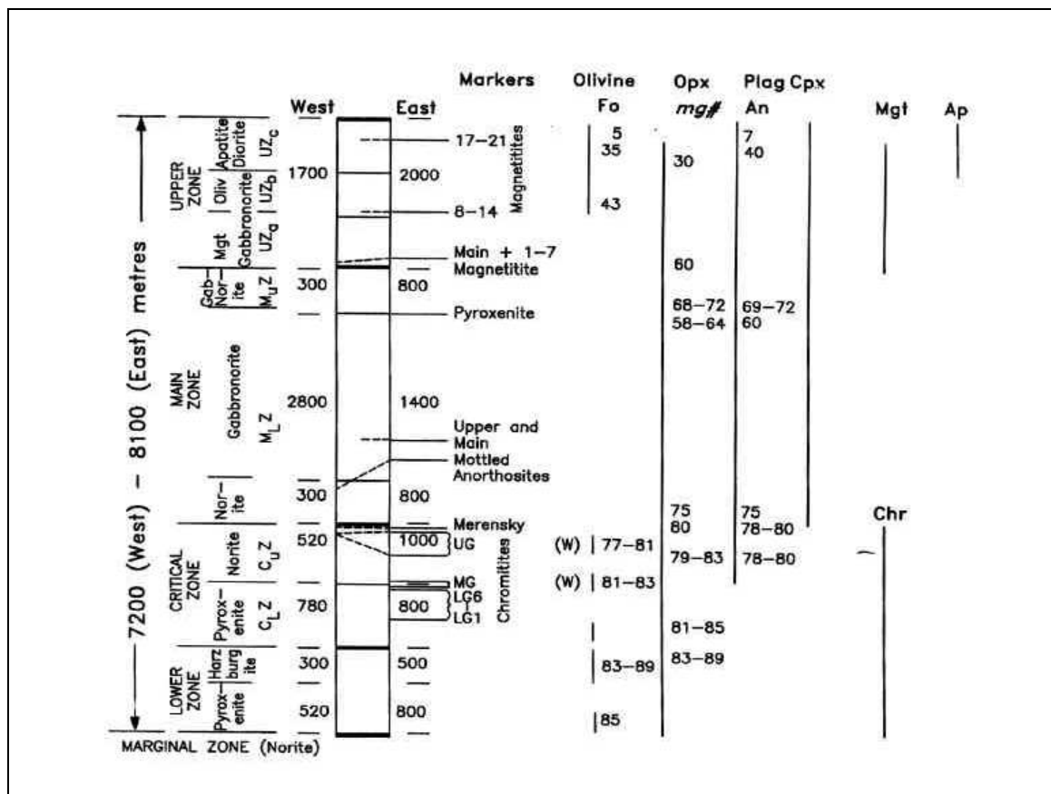
Fig. 1.2 Stratigraphy of the Eastern and Western limbs of the Bushveld Complex showing rock types and appearance of cumulus minerals (Eales and Cawthorn, 1996)
