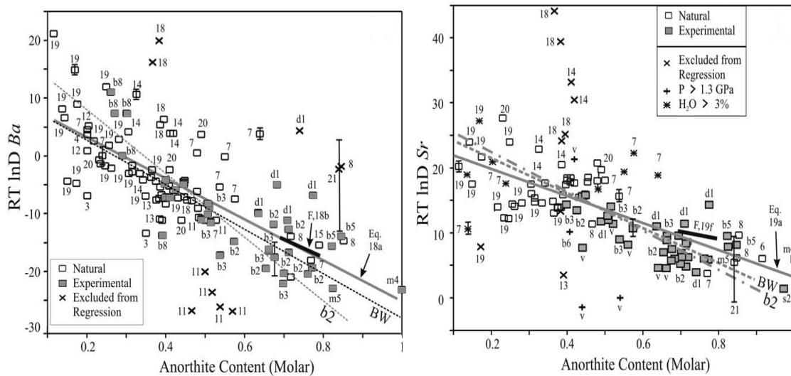
Fig. 5.4. Relationship between D for Sr and Ba into plagioclase and anorthite content (Bedard, 2006)
