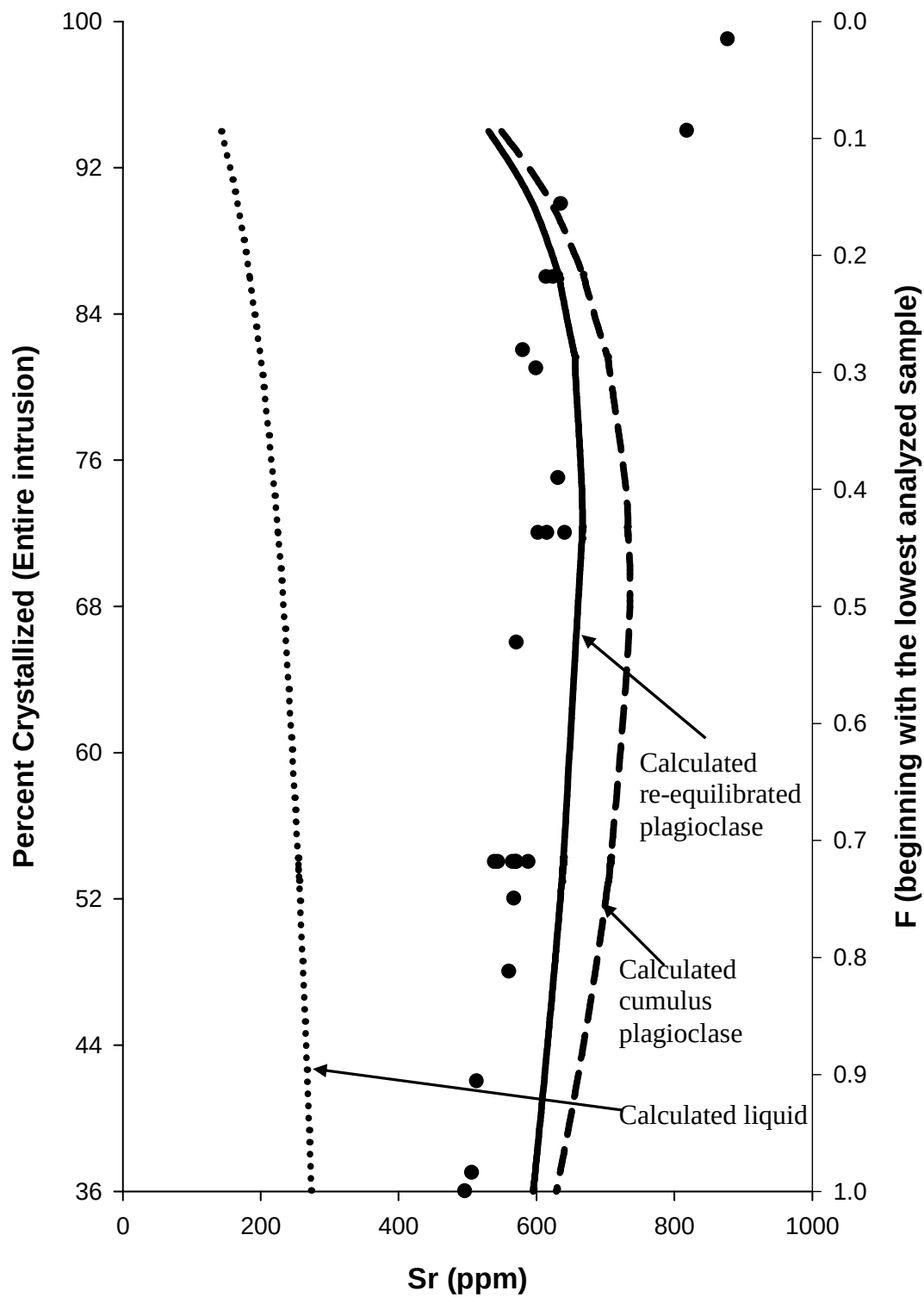
Fig. 5.7 Sr contents of liquid, cumulus and re-equilibrated plagioclase calculated from D values of Blundy and Wood (1991)
