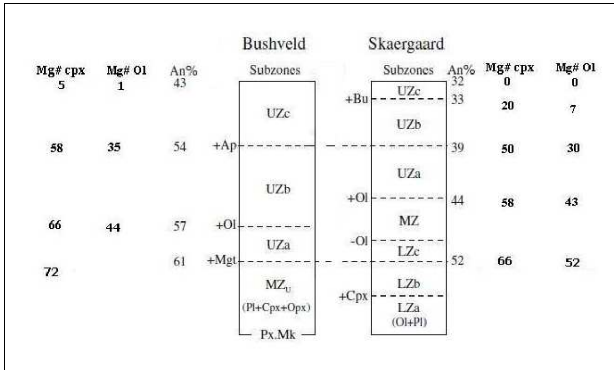
Fig. 2.1. Mineral compositions in the Bushveld Complex, above the Pyroxenite Marker and the Skaergaard Layered Series (Modified after Tegner and Cawthorn, 2009). Data for the Bushveld from Tegner et al. (2006) and for the Skaergaard from Thy et al. (2009)
