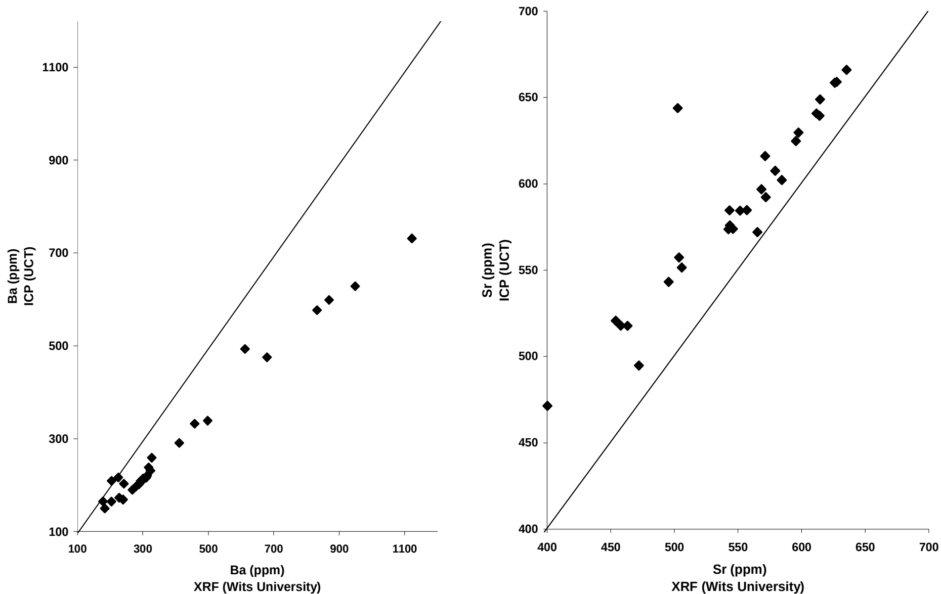
Fig. 1B. Comparison of Sr and Ba contents from analyses by both XRF at Wits University and the ICP at the University of Cape Town.
