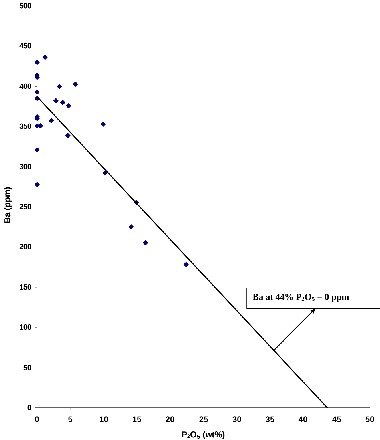
Fig. 4.4 Ba vs. P 2 O 5 Correlation. Extrapolation to the P 2 O 5 concentration of apatite shows that apatite does not concentrate Ba.
