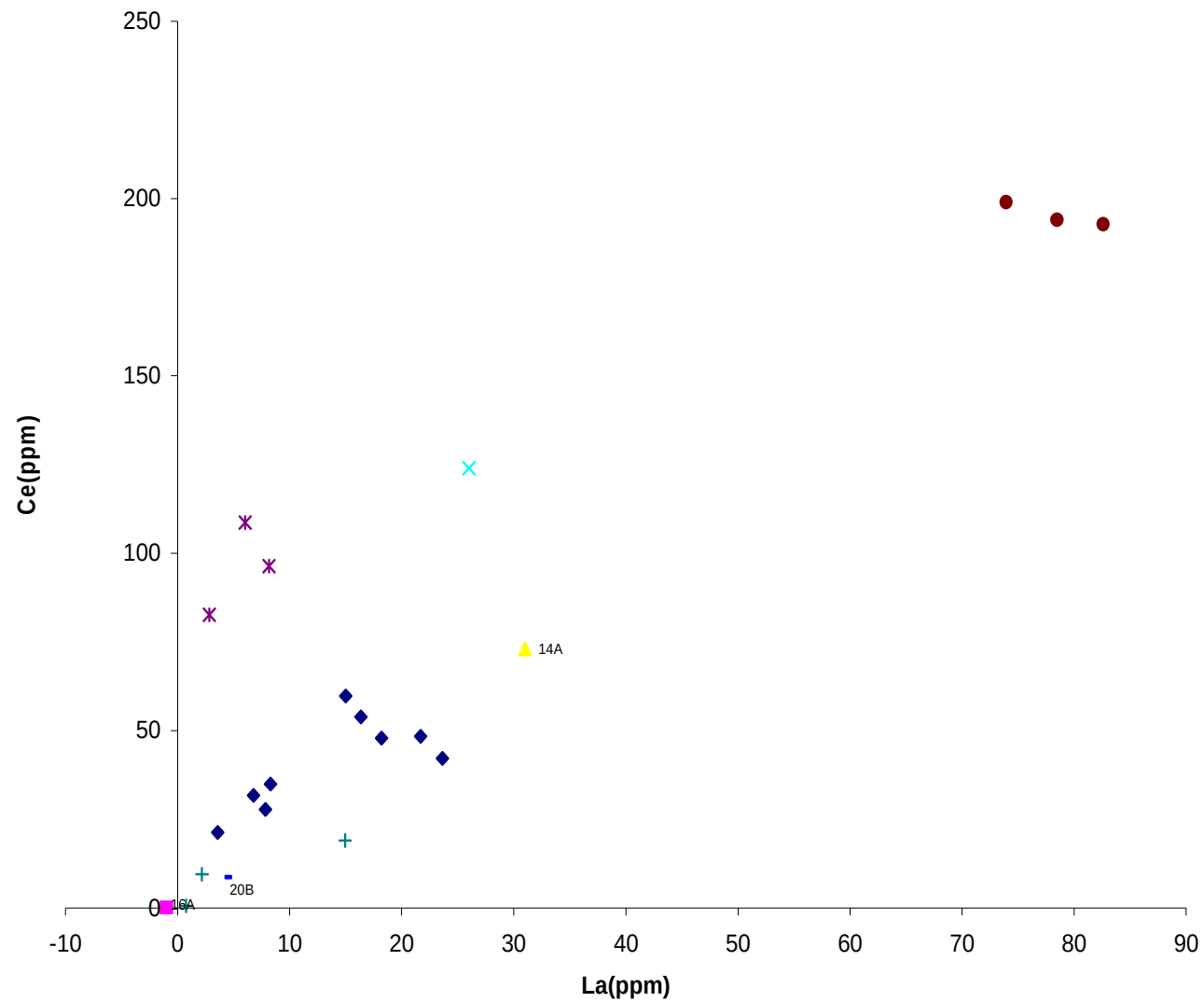
Fig. 3B :La change with Ce for Leaching experiments
