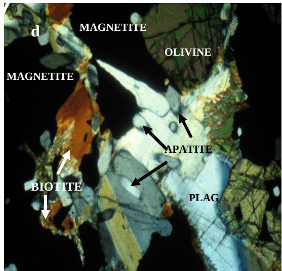
Fig. 3.2. Intercumulus minerals a.)- 1W443.8; Hornblende poikilitic to cpx, plagioclase and magnetite. b.)- 1W443.8; Alkali feldspar poikilitic to plagioclase and apatite c.)-1W443.8; Intergranular quartz. d.) -1W636.2; Intercumulus biotite. All views are taken with a x4 lens under crossed polars, field of view is 3 mm.
