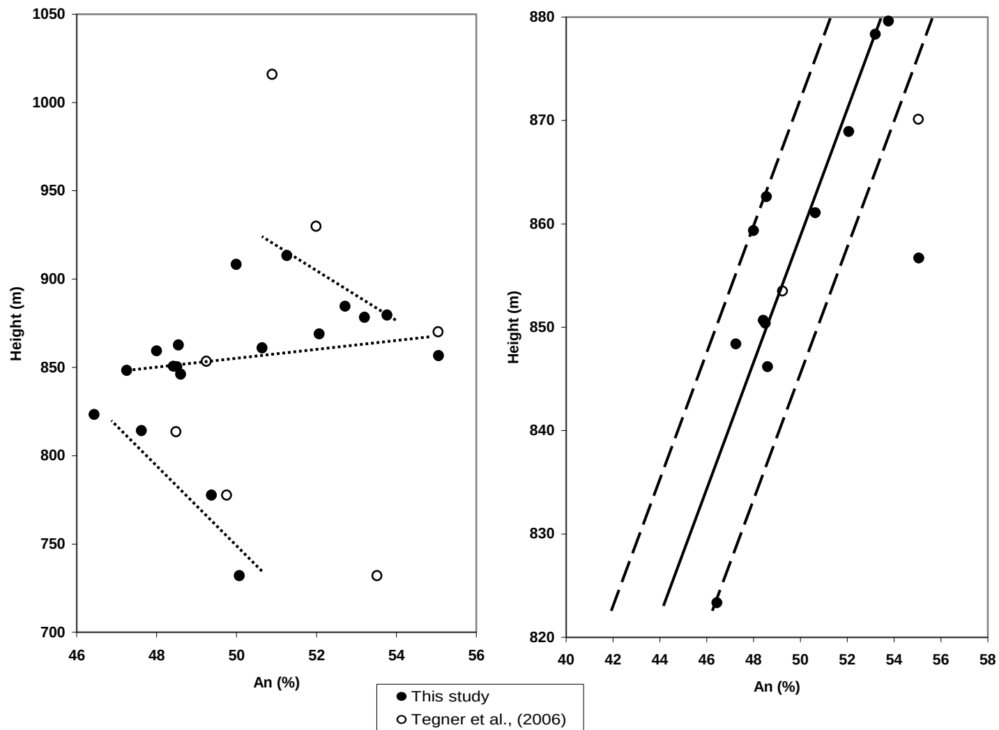
Fig. 4.9 Plot of An content in plagioclase versus height for the biggest reversal a) Section from 700 to 1050 m showing the most prominent reversal in plagioclase An. b) Section from 820 to 880 m; a best fit line (continuous) and 2% An uncertainty (dashed lines) are included.
