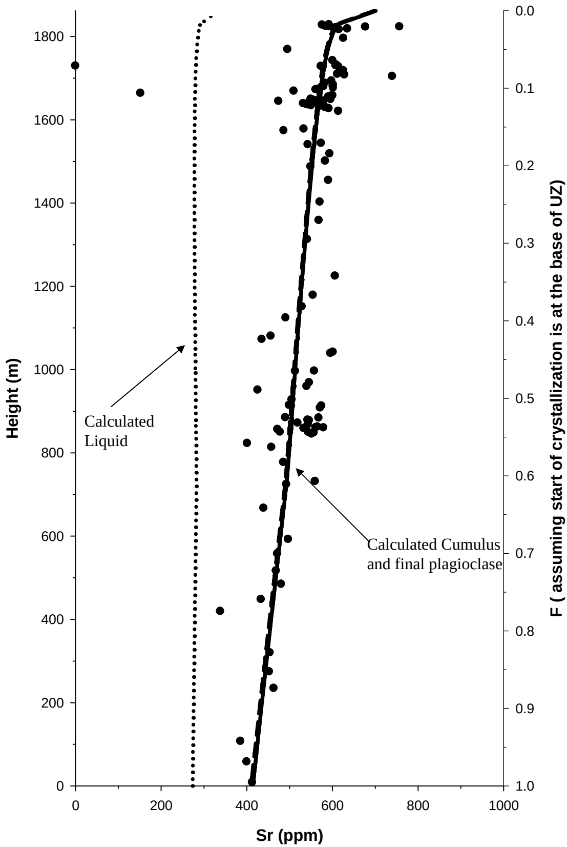
Fig. 6.3 Plots of Sr in liquid, original cumulus and re-equilibrated plagioclase vs. F(fraction of magma remaining) and height for the Upper Zone assuming a changing D_{Sr} value from 1.5 to 2.1 at the end of crystallization.
