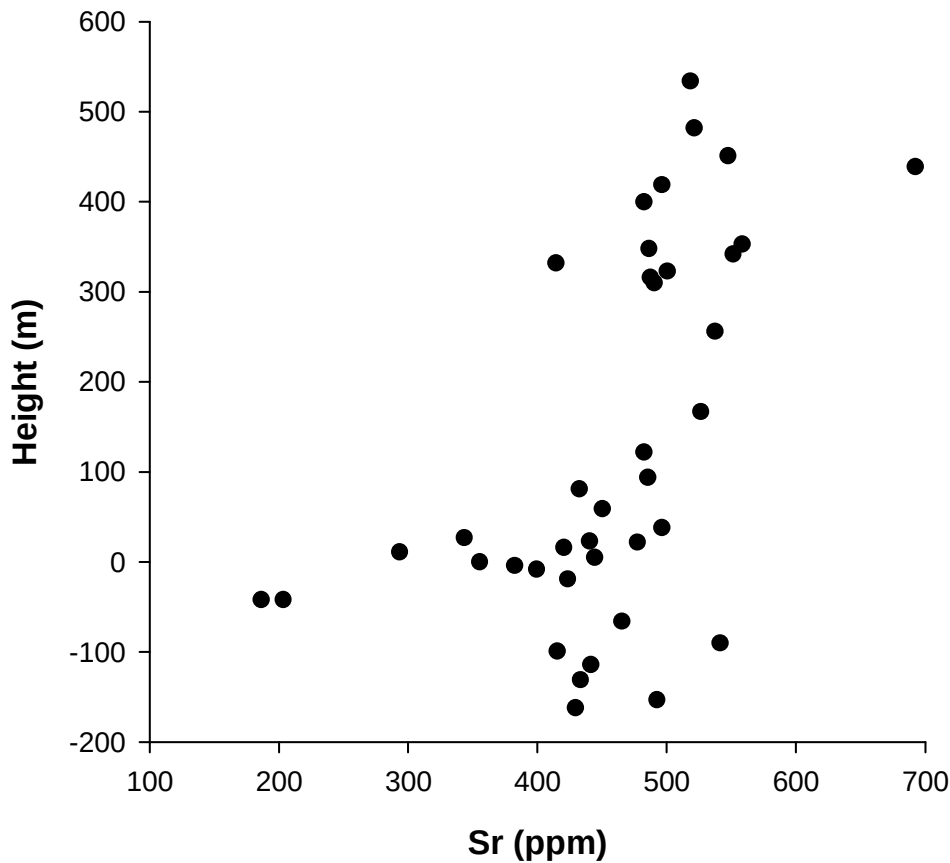
Fig. 6.5 Sr contents of plagioclase across the Lower- Upper Critical Zone boundary. Height is quoted relative to the base of the Upper Critical Zone (Reichardt, 1989)
