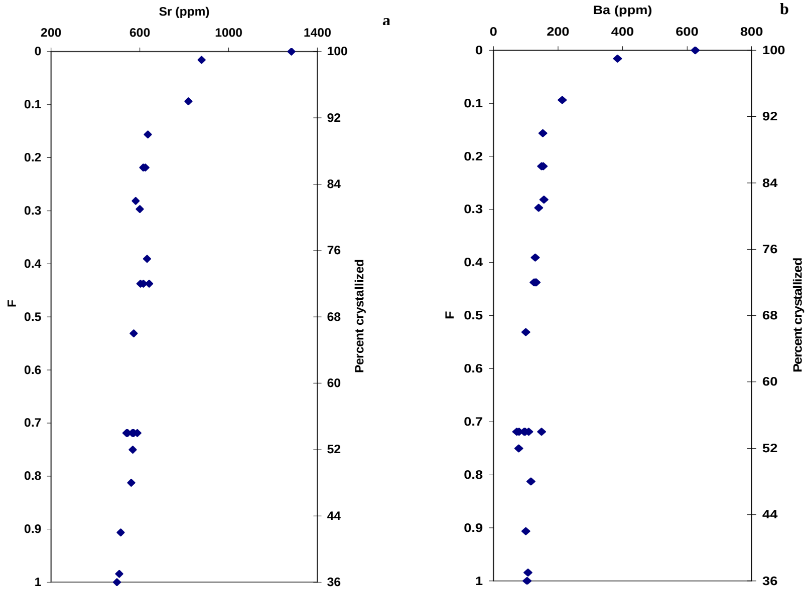
Fig. 4.11 Ba and Sr contents of plagioclase for the Skaergaard Layered Series.
