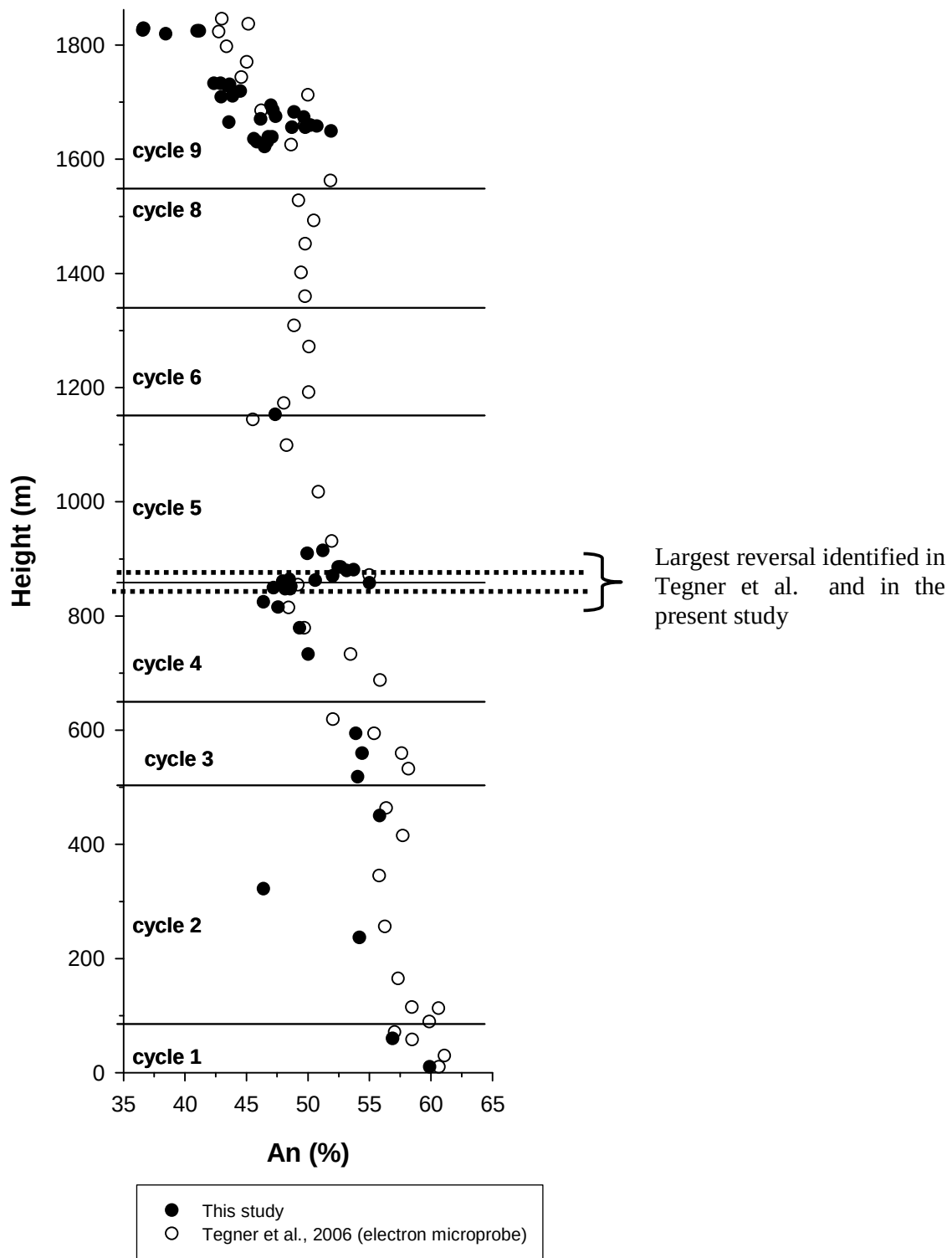
Fig. 4.8 Variation of plagioclase An content with Height in the Bierkraal drill cores. Data have been corrected for the presence of apatite by leaching or calculation and probe data are from Tegner et al. (2006). Location of cycles are from Tegner et al.
