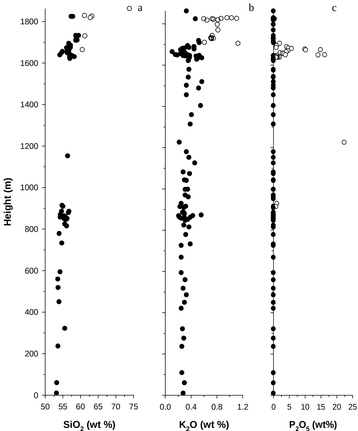
Fig. 4.7 \text{SiO}_2 , \text{K}_2\text{O} and \text{P}_2\text{O}_5 contents from analyses of separates plotted against height. Empty circles are a) samples which contain quartz, b) samples that contain significant alkali feldspar and c.) Samples which contain apatite. The sections in b and c contain more samples than in section a because these plots are created from XRF analyses on pellets in which all samples were analyzed.
