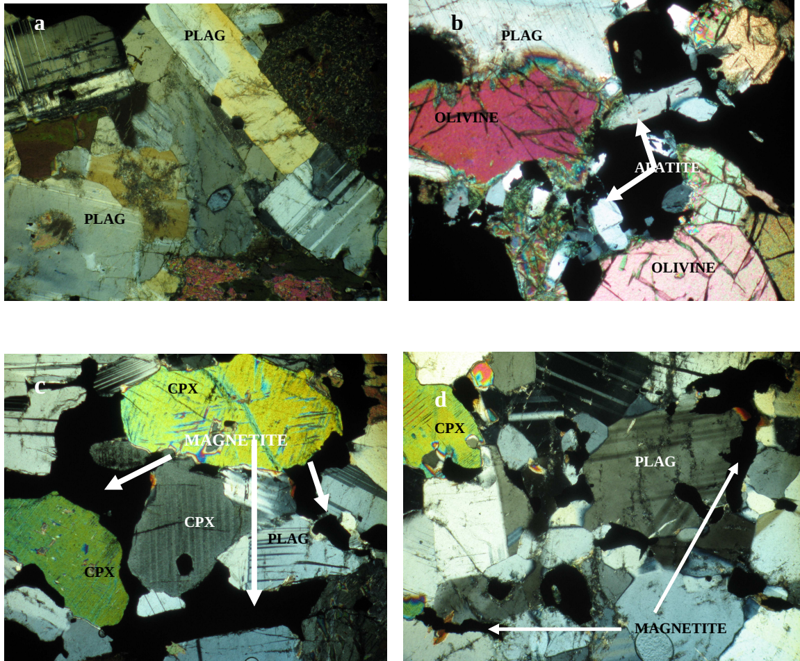
Fig. 3.1. Microphotographs showing the major cumulus phases in the Upper Zone. a.) -1W443.8; Plagioclase grains, some altered to sericite. b.)-1W636.2; Olivine altered along the rims and cracks to bowlingite. c.)-1W1473 Subhedral cpx with anhedral magnetite d.)- 1W1498.7; Cumulus and interstitial magnetite as inclusions and composite grains. All views are taken with a x4 lens under crossed polars, field of view is 3 mm.
