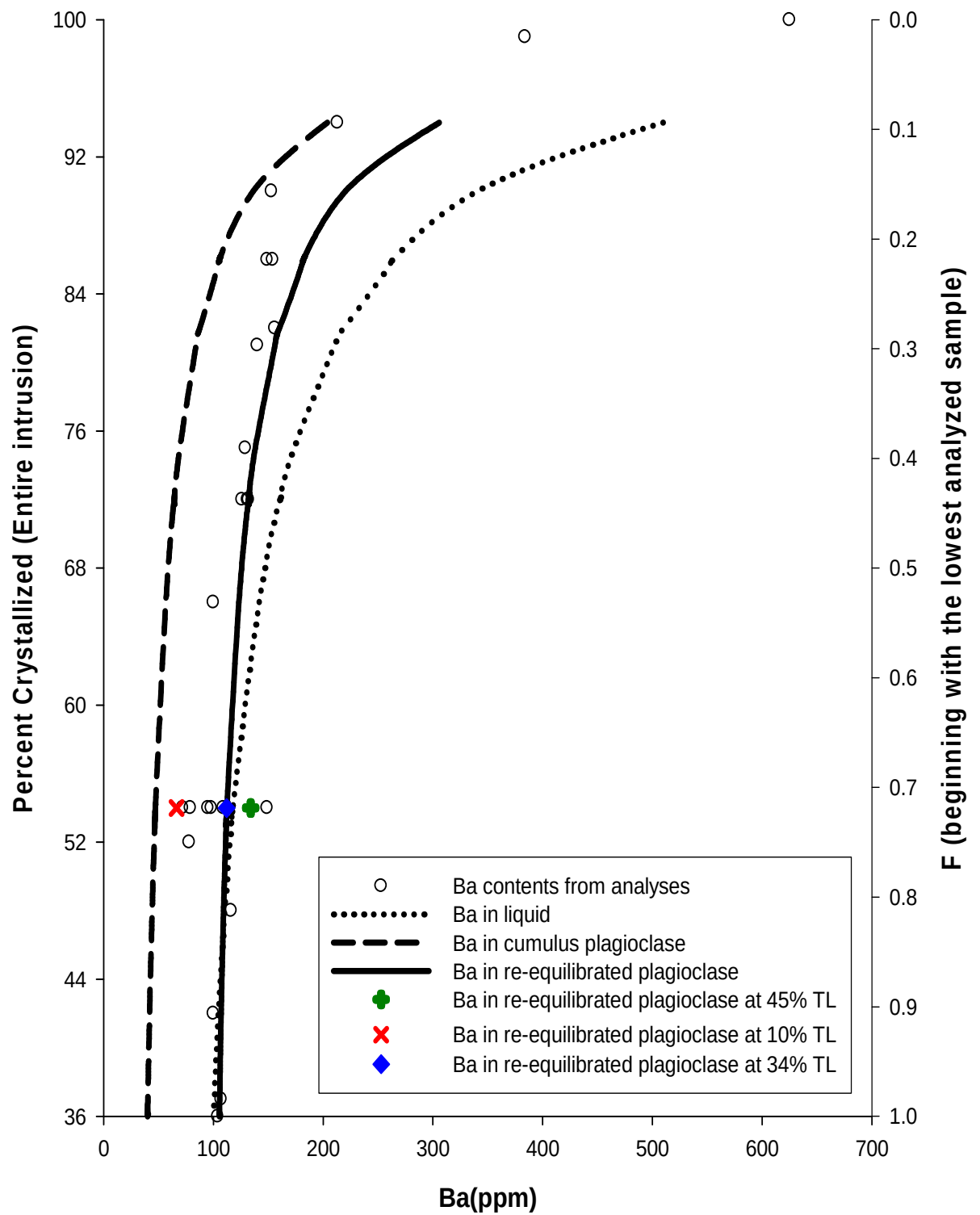
Fig. 5.3. Variation in re-equilibrated plagioclase Ba resulting from varying Trapped Liquid fractions at the same stratigraphic sample
