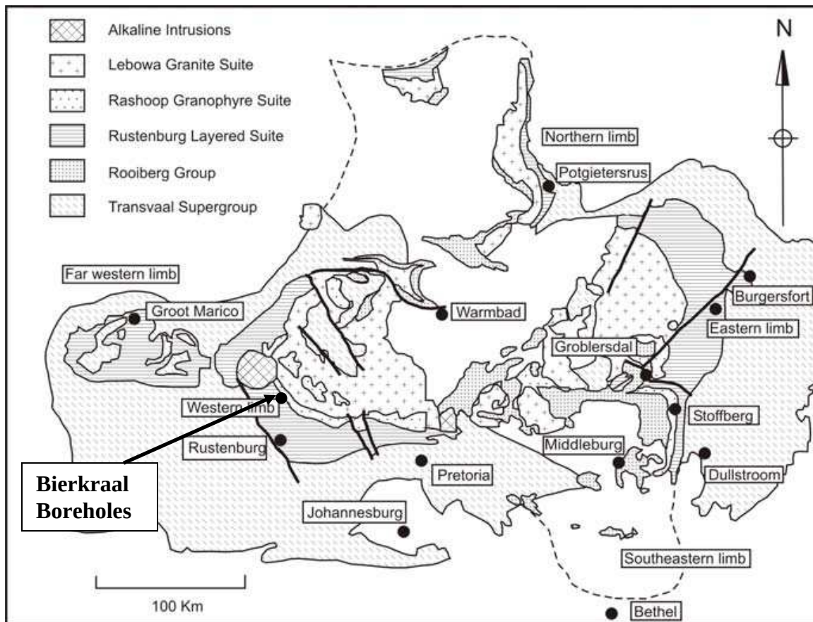
Fig. 1.1 Simplified Geological Map of the Bushveld Complex showing the location of the Bierkraal boreholes (based on Eales and Cawthorn, 1996)
