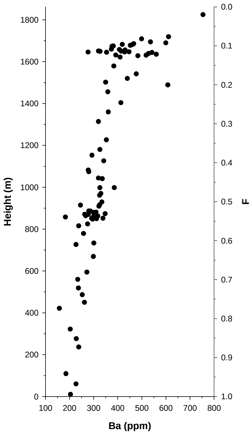
Fig. 4.13 Barium contents of plagioclase plotted against height for the Bushveld Upper Zone. Data exclude samples which contain significant alkali feldspar.
