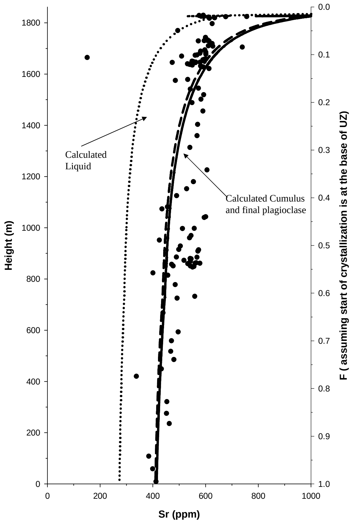
Fig. 6.2 Plots of Sr in liquid, original cumulus and re-equilibrated plagioclase vs. F(fraction of magma remaining) and height for the Upper Zone assuming a constant D_{Sr} in plagioclase of 1.5. The cumulus and final re-equilibrated plagioclase compositions do not differ significantly because the TLS effect is small for Sr .
