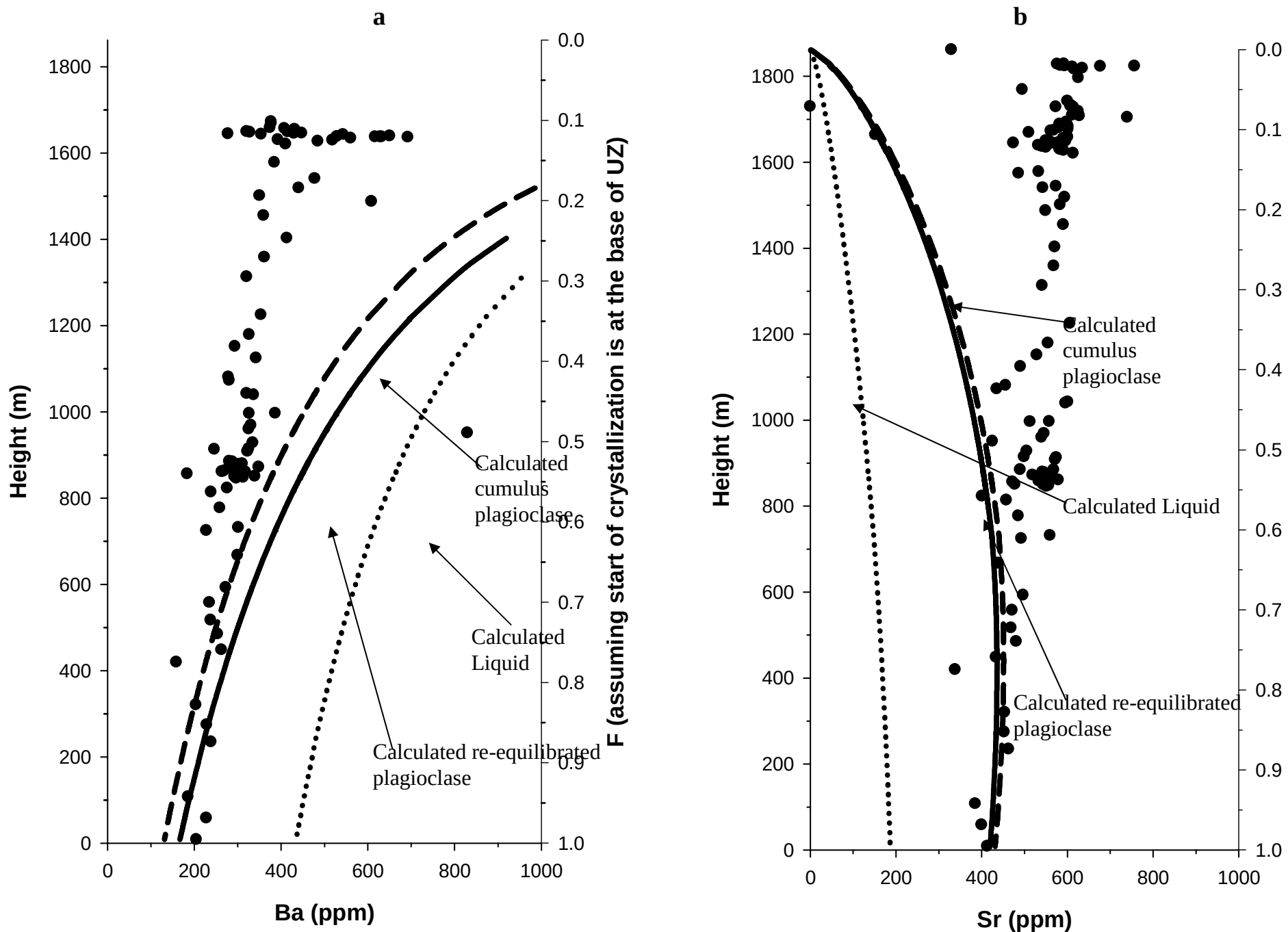
Fig. 6.4 Trends for Sr and Ba contents of liquid, cumulus and re-equilibrated plagioclase for the Bushveld intrusion calculated from equations by Blundy and Wood (1991)
