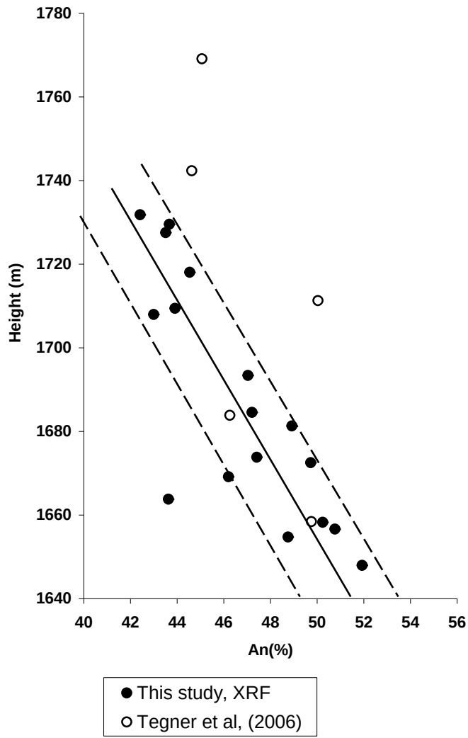
Fig. 4.10 Plot of An content in plagioclase vs. height for the section in which the second biggest reversal in the data of Tegner et al. occurs. The best fit line is indicated with a continuous line and 2% uncertainty on both sides indicated with dashed lines.
