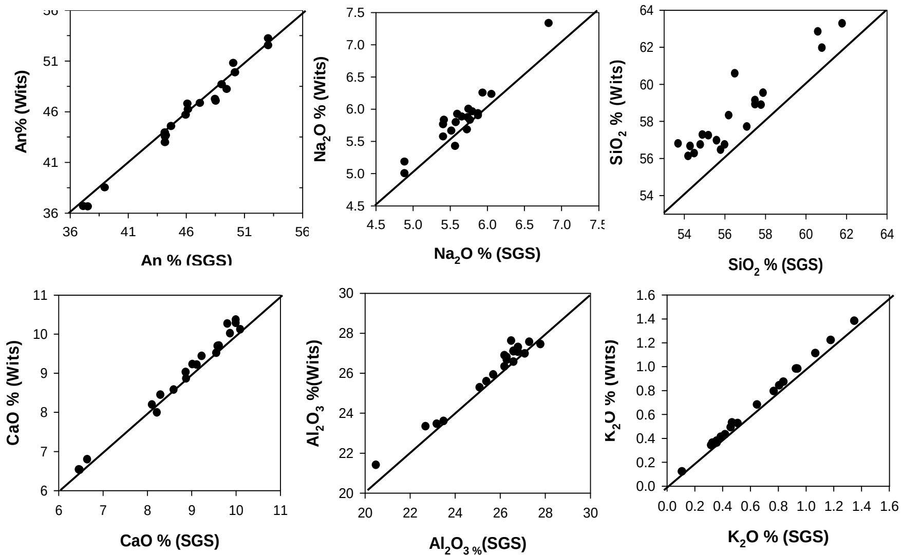
Fig 1A. Comparison of major element compositions for samples analyzed by both Wits University and SGS Lakefields
