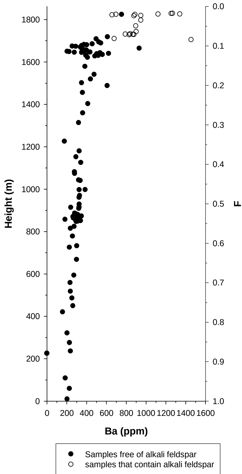
Fig. 4.5 Barium contents of plagioclase plotted against height for the Bushveld Upper Zone showing samples which are rich in alkali feldspar.
