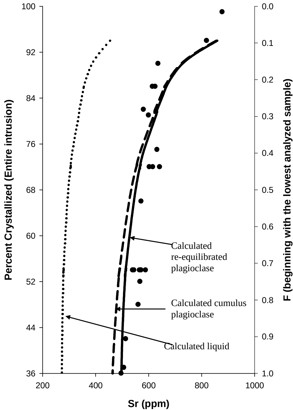
Fig. 5.6 Calculated trends based on Rayleigh fractionation with the Sr content of the Skaergaard parental liquid (Nielson, 2004) and allowing for the trapped liquid shift effect. Solid dots are data from Jang and Naslund (2001).
