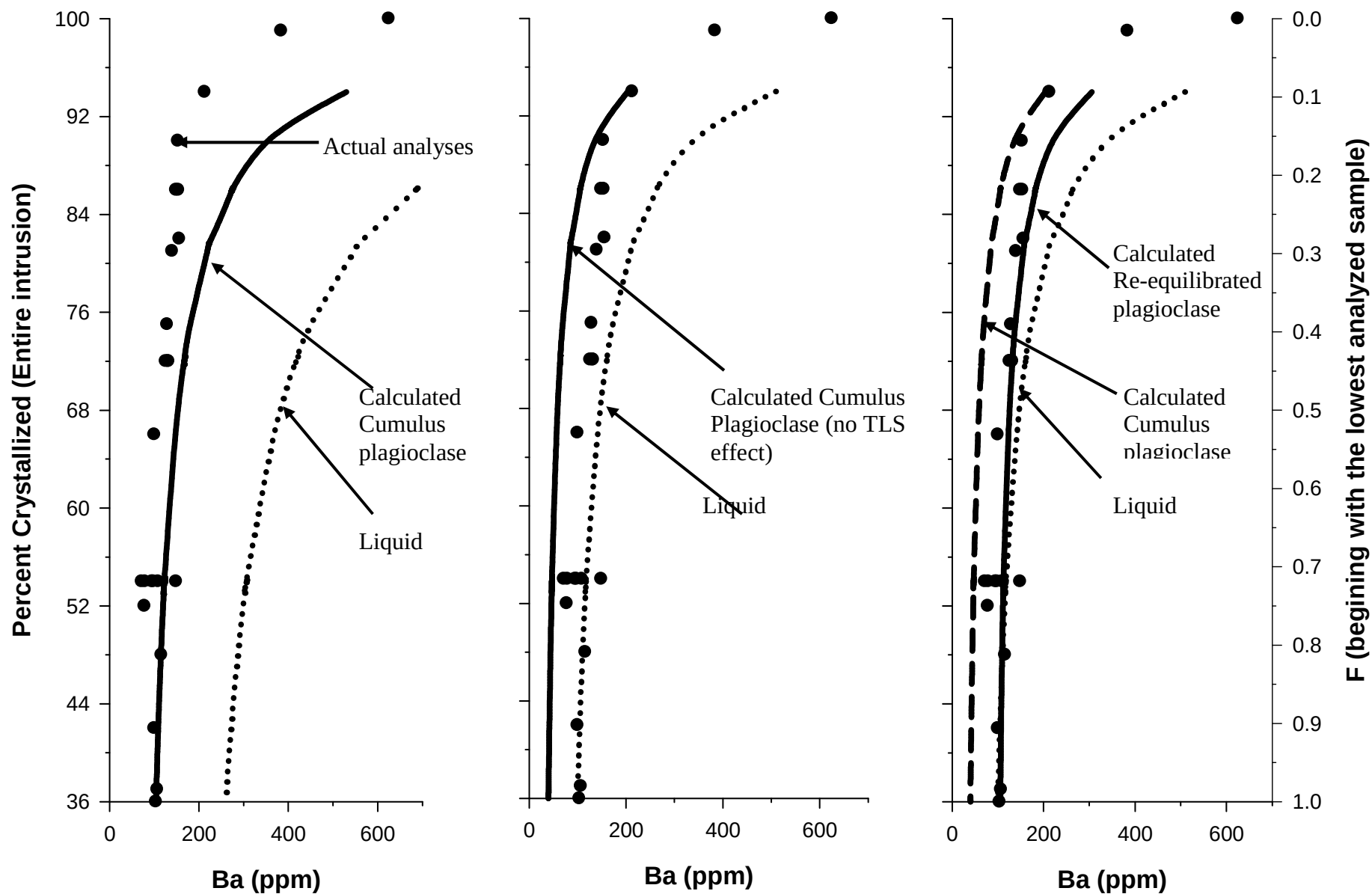
Fig. 5.2 Trends for barium in the Skaergaard intrusion showing the difference in calculated compositions (liquid, cumulus and re-equilibrated plagioclase) from the three different models. a) Compositions modeled as described in section 5.2.1a. b) Modeled as in 5.2.1b and data are from Table 5.2 c) Modeled as described in section 5.2.2 and re-equilibrated plagioclase Ba contents agree a lot better with observed plagioclase Ba.
