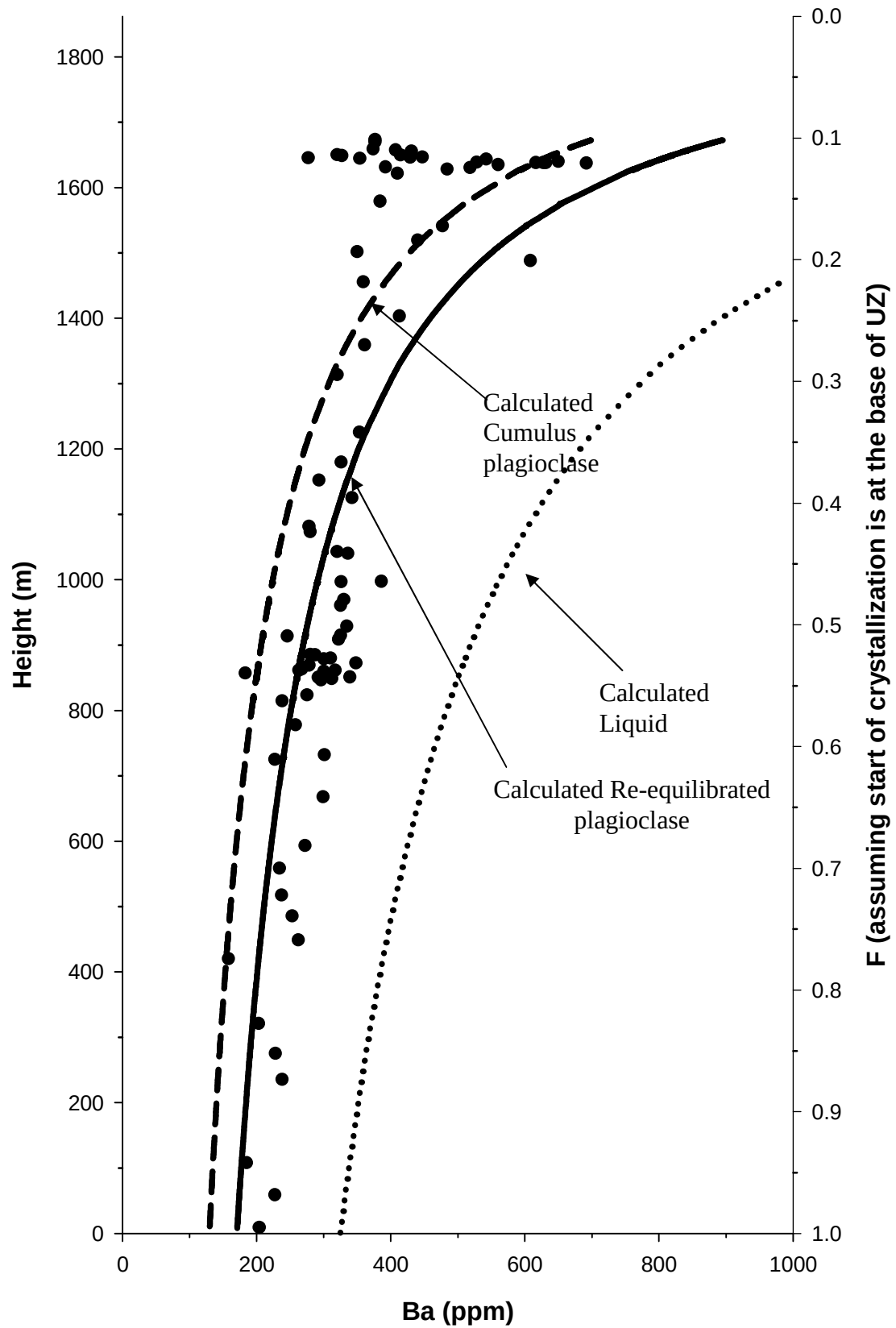
Fig. 6.1 Plots of Ba in liquid, original cumulus and re-equilibrated plagioclase vs. F (fraction of magma remaining) and height for the Upper Zone, Bushveld intrusion. Filled circles represent analytical data
