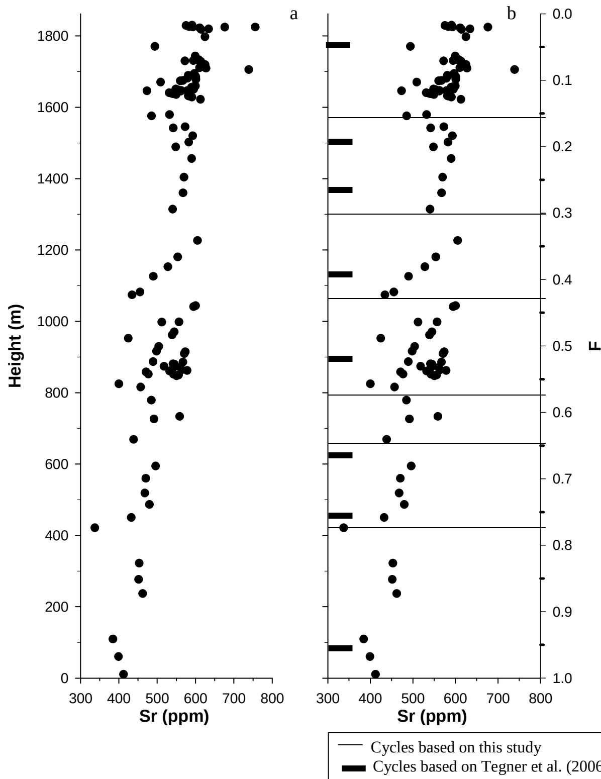
Fig. 4.12 Plots of Sr contents of plagioclase for the Upper Zone of the Bushveld Complex. Data have been corrected for the presence of apatite. Two y-axes values are shown, one for the height relative to the base of the Upper Zone and the section that can be modeled (referred to as F). The section in b includes fractionation cycles for the present study and for Tegner et al.
