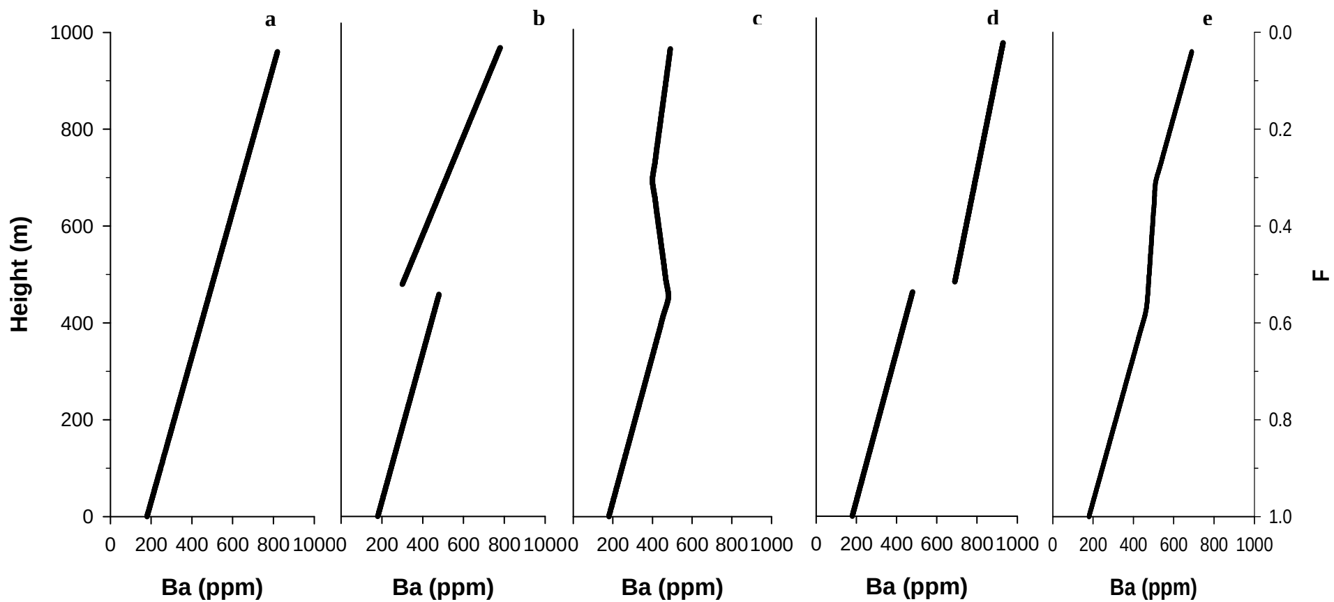
Fig. 6.6 Possible trends in the Ba contents of plagioclase plotted against height and fraction of magma remaining
