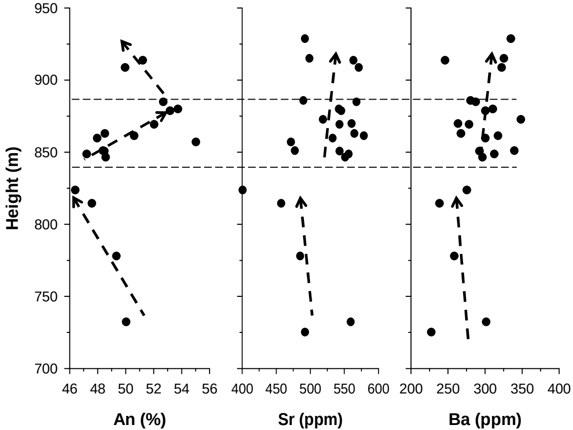
Fig. 6.7 Sr and Ba contents of the section over which the largest reversal in plagioclase An occurs in the Upper Zone of the Bushveld Complex
