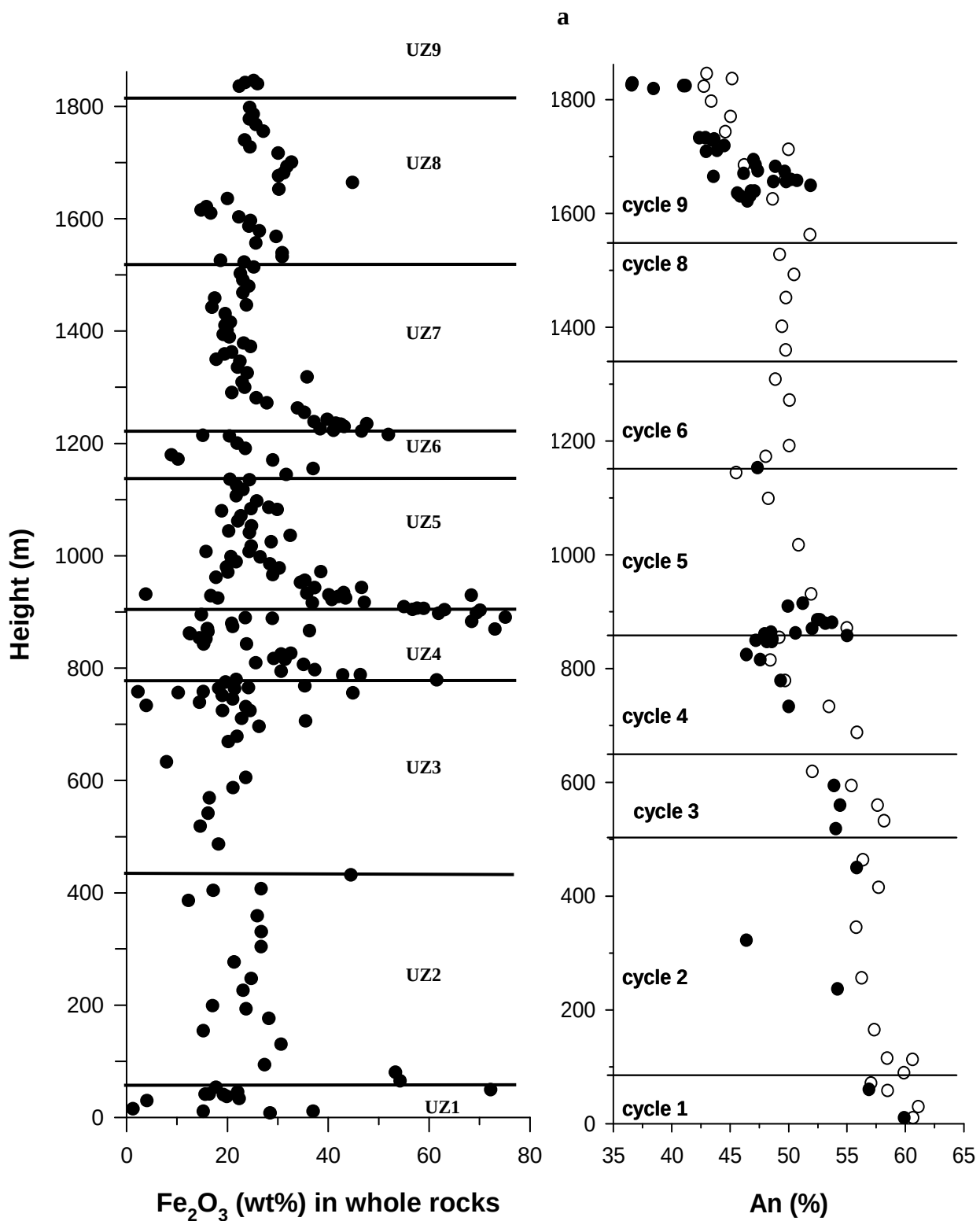
Fig. 6.8 Comparison of cycles based on increase in \text{Fe}_2\text{O}_3 in whole rocks with reversals in plagioclase An content identified by Tegner et al (2006). Filled circles are An contents from this study and empty circles are An contents from Tegner et al. \text{Fe}_2\text{O}_3 data are from Roberts (2005)
