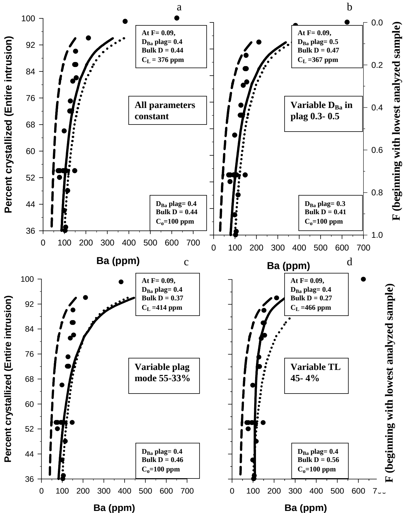
Fig. 5.5 Calculated trends for barium in the Skaergaard intrusion from varying different parameters with crystallization. F values start at LZa; percent crystallized is for entire intrusion from Jang and Naslund (2001) and C_L is the liquid composition at F = 0.1 . Dotted curves represent Ba in the liquid and solid curves are Ba in the modeled plagioclase, dashed curve in c represents Ba in the original cumulus plagioclase.
