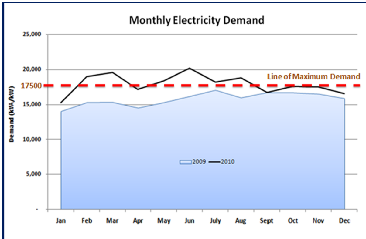
Figure 29: Monthly electricity demand profiles of NDC for the year 2009 and 2010 (NDC, 2011 and NDC, 2010).
