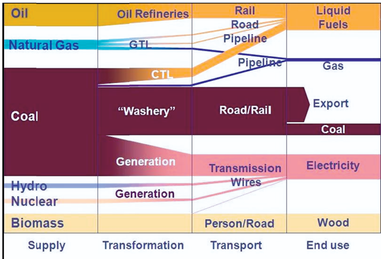
Figure 1: Flow of energy chart (DME, 2008).
