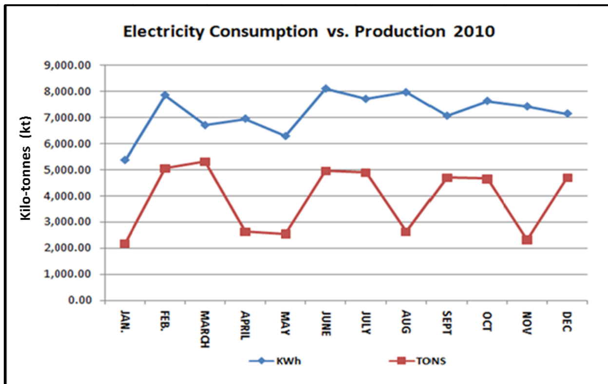
Figure 34: Production versus electrical power consumed for the year 2010 (NDC, 2010)
