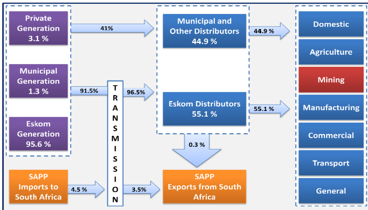
Figure 10: Energy flow through the electricity supply industry (Winkler, 2009).
