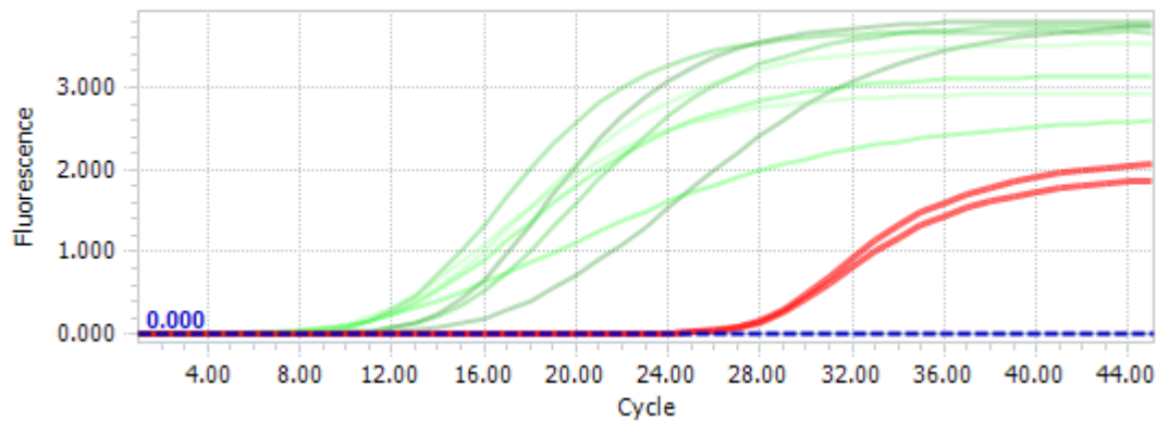
Figure 13: CNP standard curve of 10ng/ \mu l to 0.08ng/ \mu l. The green curves are the standard curve values. The red curves are the test samples that were used. This shows that the samples do not fall within the curve.
