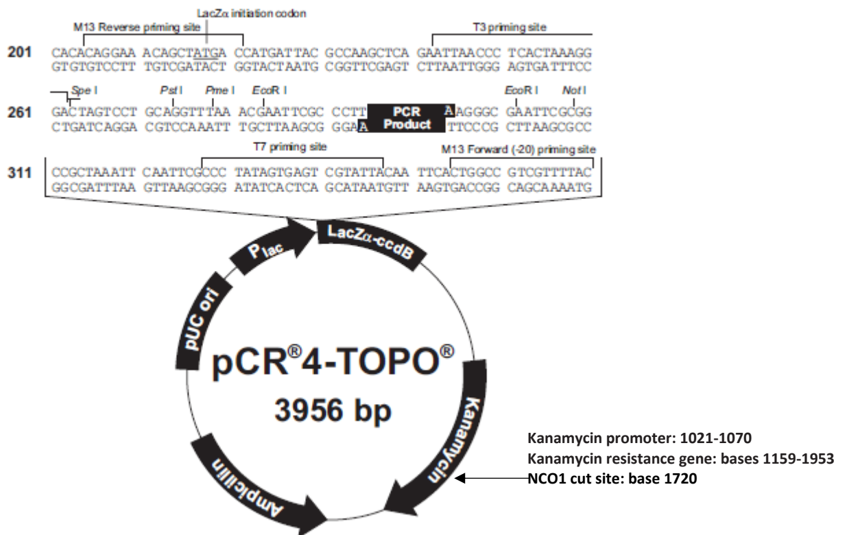
Figure 14: TOPO vector with restriction enzyme cut sites (Invitrogen life technologies, TOPO TA manual)
