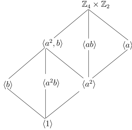
Figure 4.2: lattice of subgroups of \mathbb{Z}_4 \times \mathbb{Z}_2
