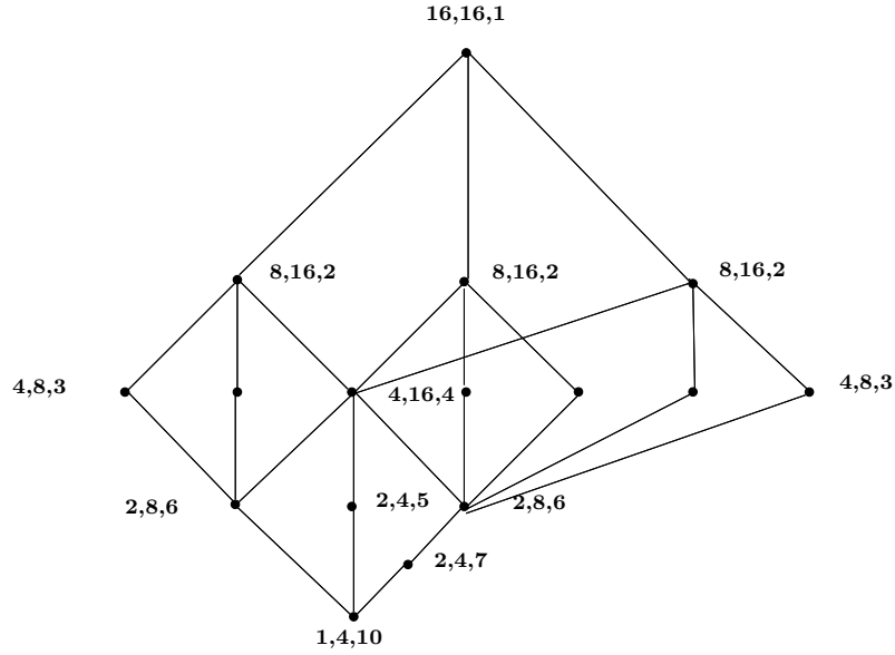
Figure 8.6: lattice of optimal partitions of \mathbb{Z}_4 \rtimes \mathbb{Z}_4
