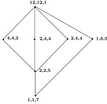
Figure 6.2: lattice of optimal partitions of \mathbb{Z}_3 \rtimes \mathbb{Z}_4
