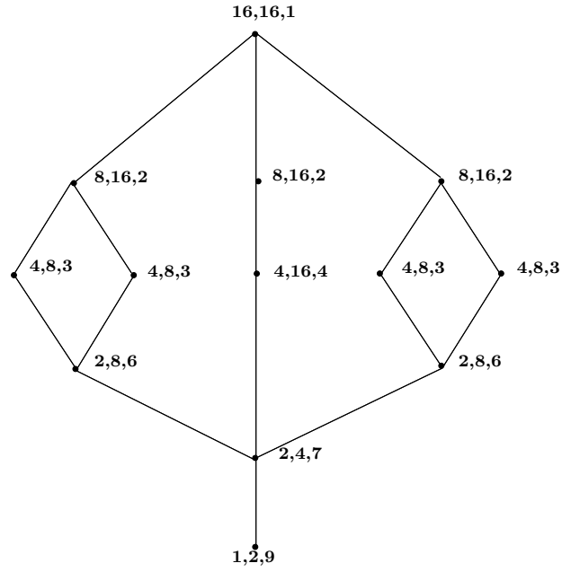
Figure 8.2: lattice of optimal partitions of Q_{16}
