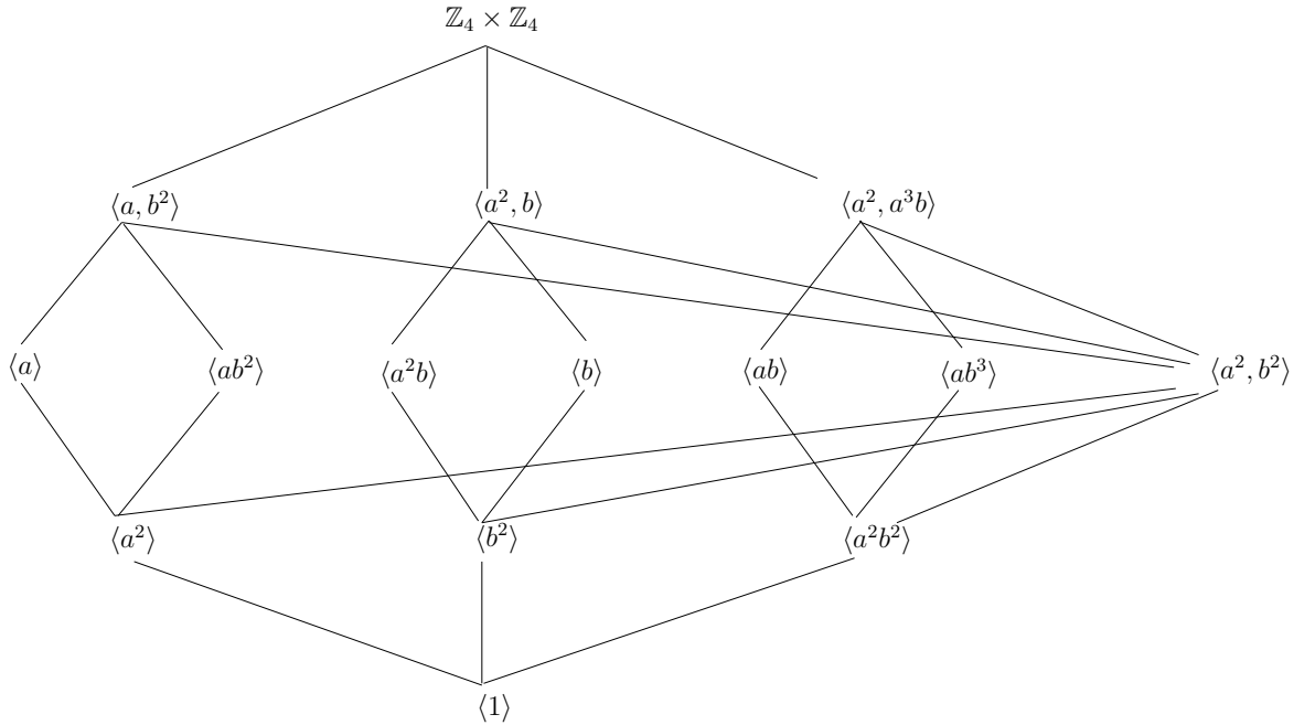
Figure 4.5: lattice of subgroups of \mathbb{Z}_4 \times \mathbb{Z}_4
