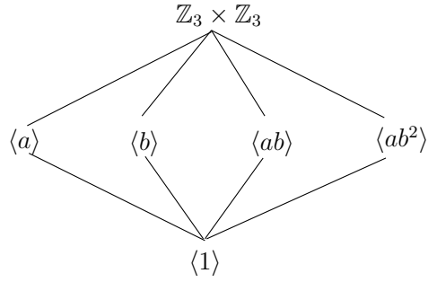
Figure 4.3: lattice of subgroups of \mathbb{Z}_3 \times \mathbb{Z}_3
