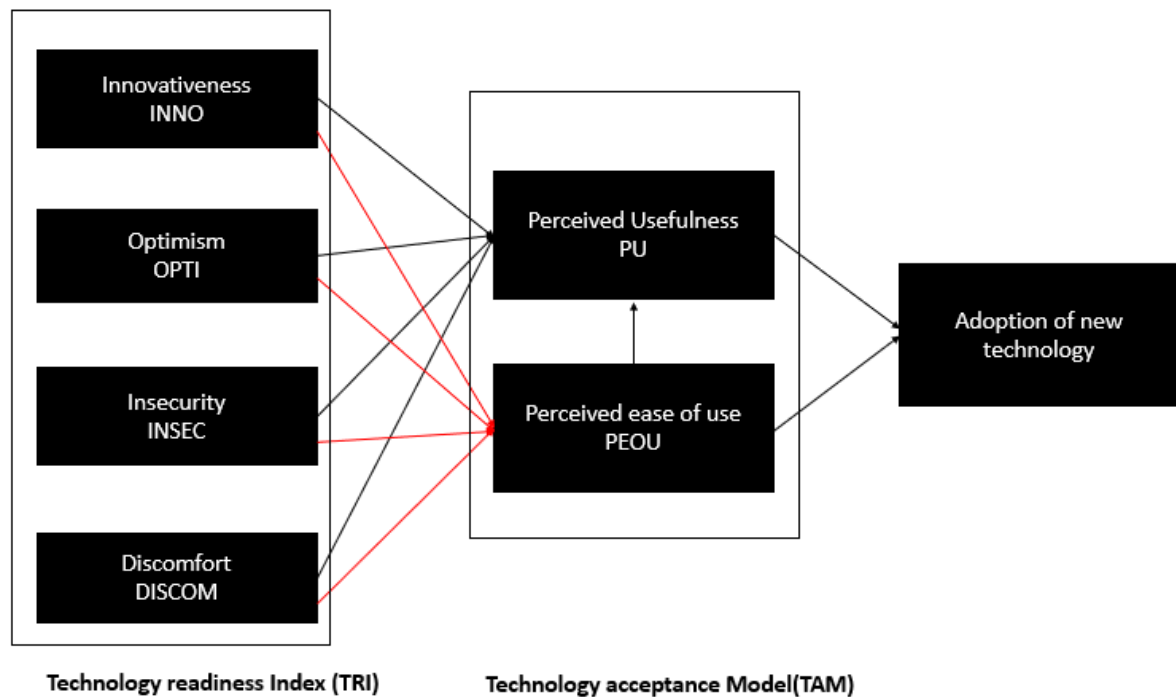
Figure 2. 7: TRAM model
