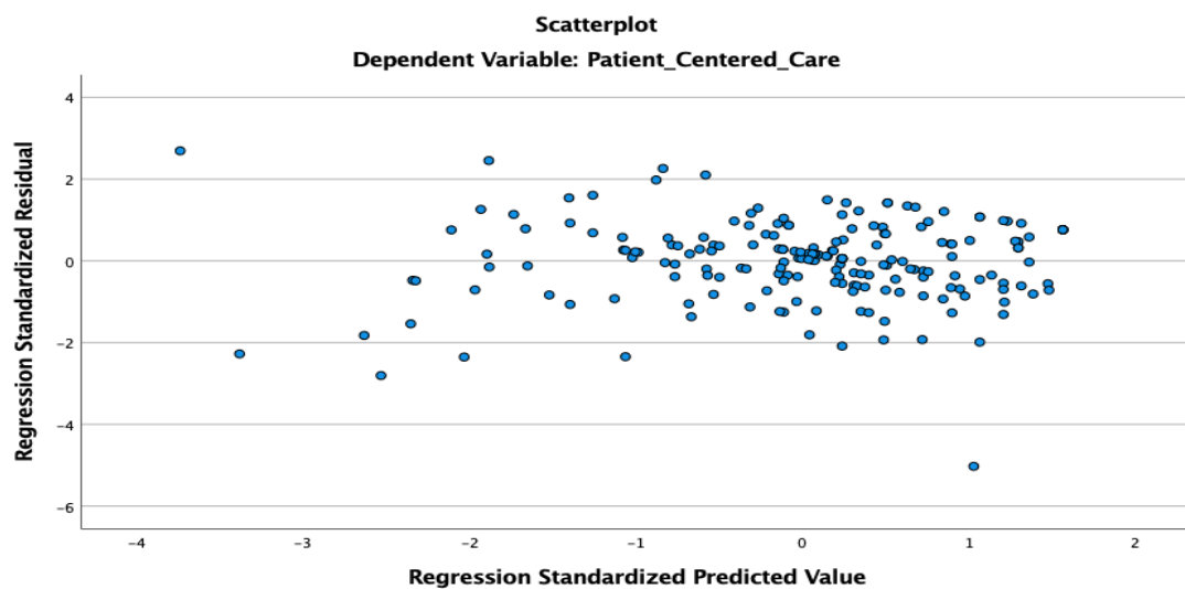
Figure 17: Scatterplot
