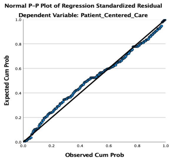
Figure 15: P-P Plot
