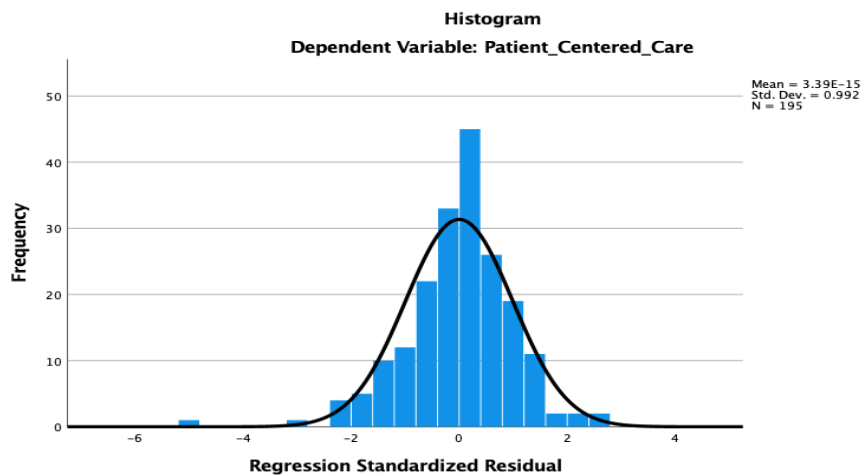
Figure 16: Histogram
