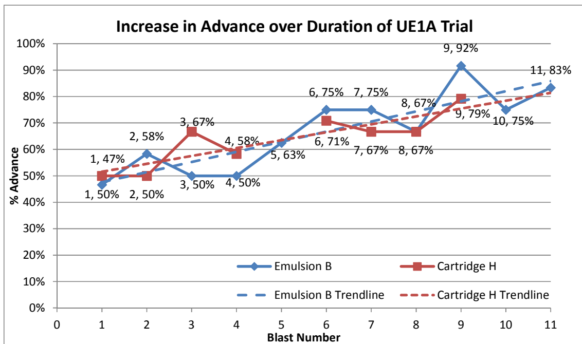
Figure 43, Increase in Advance over Duration of Trial
