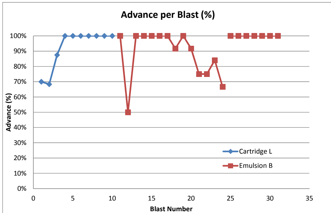
Figure 41, Face advance per blast as a percentage of drilled length, Panel 3 South
