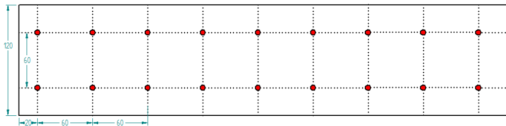
Figure 42, Round Design – Panel North 6, UE1A reef, Rand Uranium
