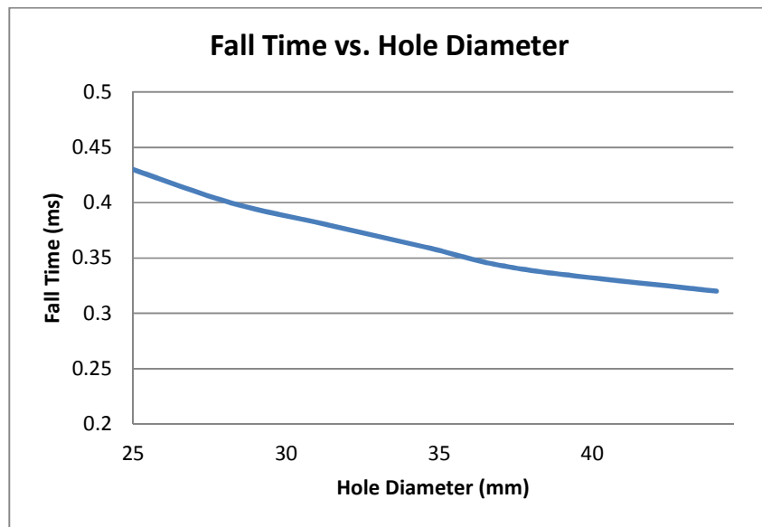
Figure 16, Fall Time measured by Saffy at 230mm (9 inches) from the blasthole for a fully coupled charge in increasing hole diameters (Saffy, 1961)
