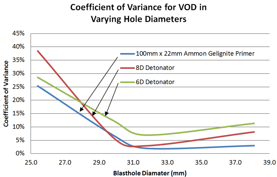
Figure 8, Coefficient of variance for VOD in increasing hole diameters (Mulke, 1966)
