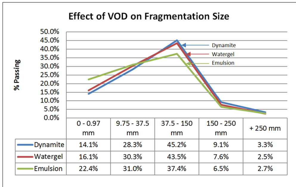
Figure 18, Influence of VOD on fragment size in blast results (Brinkmann, 1994)
