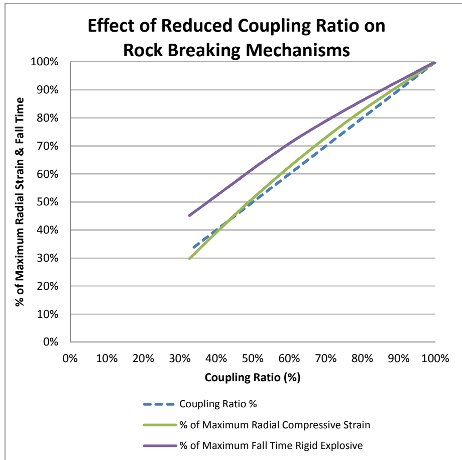
Figure 10, Effect of coupling ratio on Radial Compressive Strain and Fall Time (Saffy, 1961)
