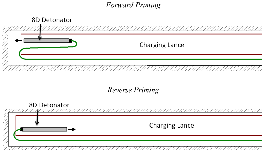
Figure 33, Method for forward and reverse priming of closed end VOD test pipes
