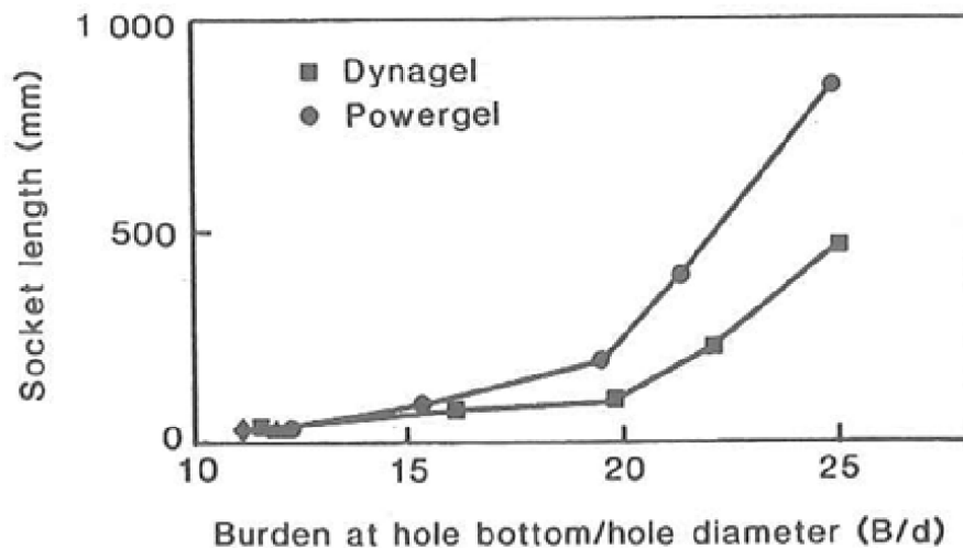
Figure 6, Comparison of socket length blasted with higher and lower VOD explosives with consistent energy (Brinkmann, 1990)
