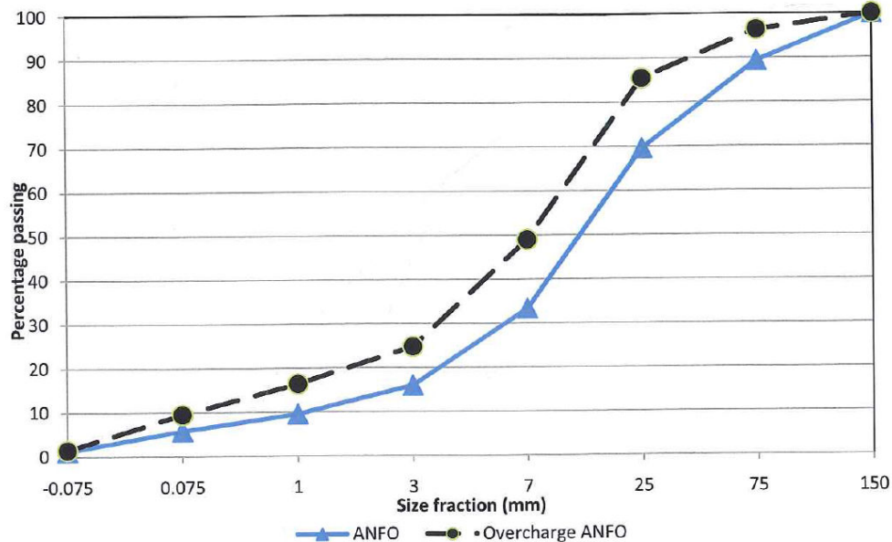
Figure 20, Effect of overcharging with ANFO on the size of fragmentation (Prout, 2010)
