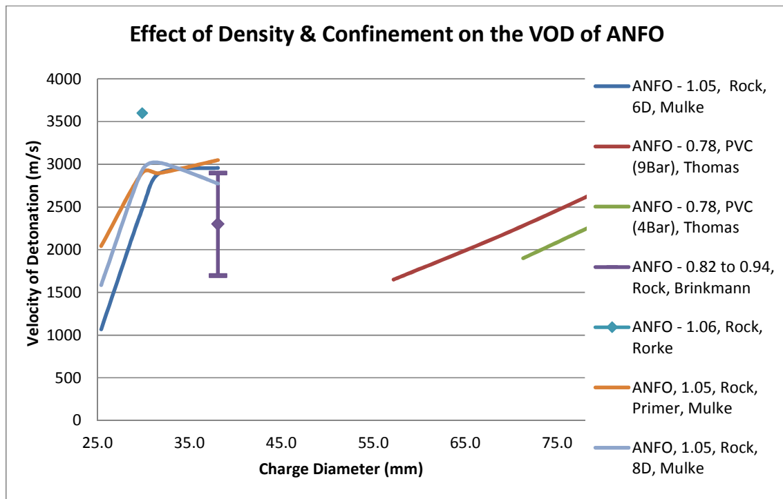
Figure 7, Effect of density and confinement on the VOD of ANFO (Thomas, 2005; Rorke, 1996; Brinkmann, 1990; Mulke, 1966)
