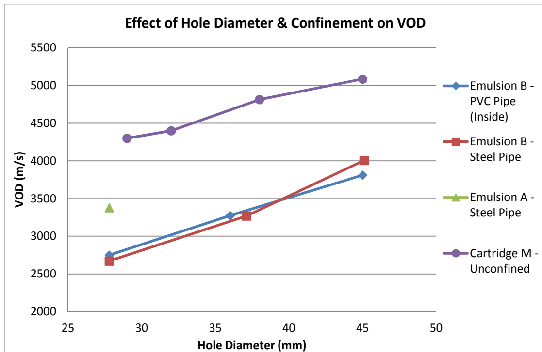
Figure 36, Velocity of detonation (VOD) for Emulsion B and cartridged emulsion plotted against pipe diameter
