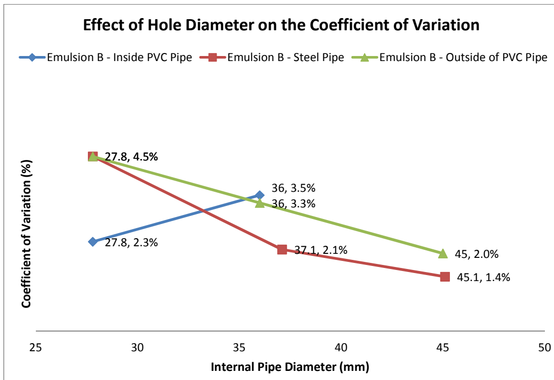
Figure 35, Coefficient of Variation for Emulsion B VOD results
