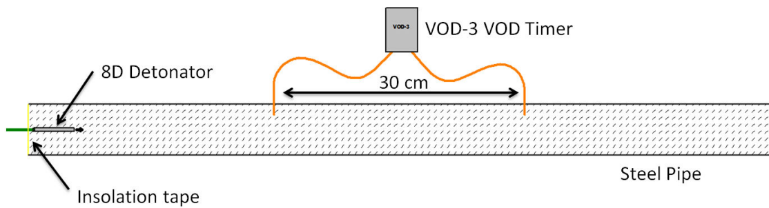
Figure 29, Test 1 – Recording of VOD in steel pipe with AECE VOD-3 VOD timer
