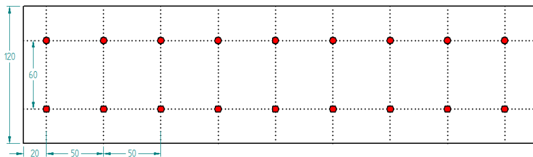
Figure 40, Round Design – Panel 3 South, RMDC
