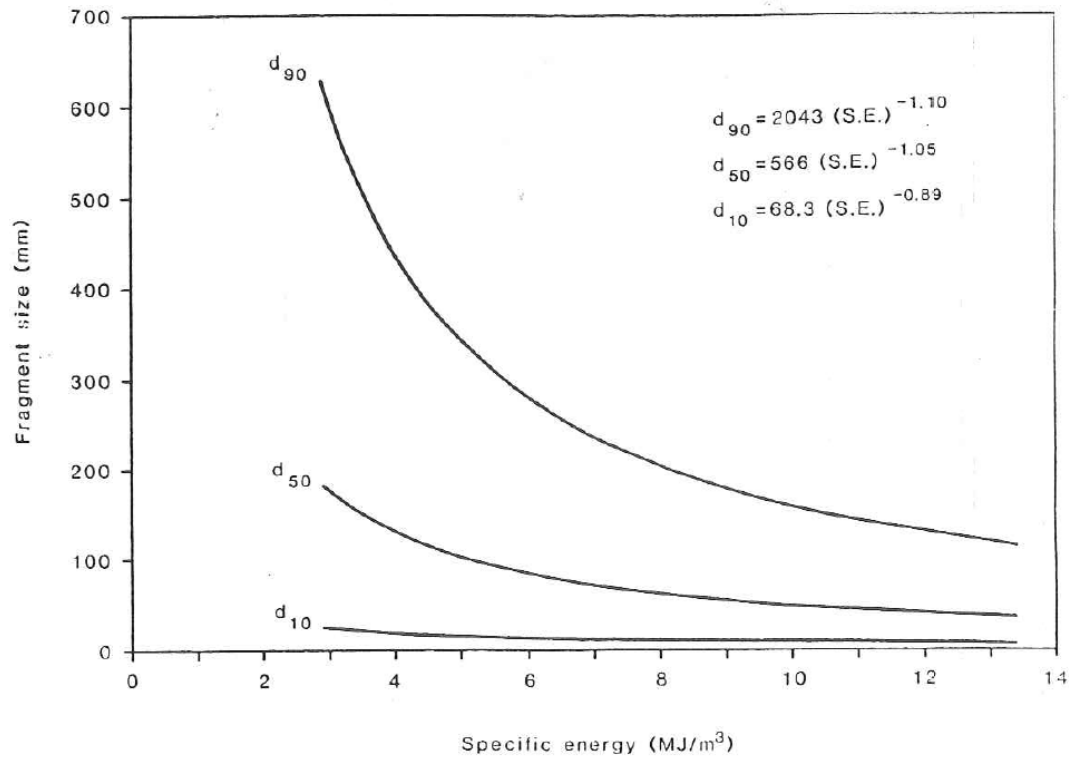
Figure 17, Influence of specific energy on fragment size in blast results (Brinkmann, 1994)
