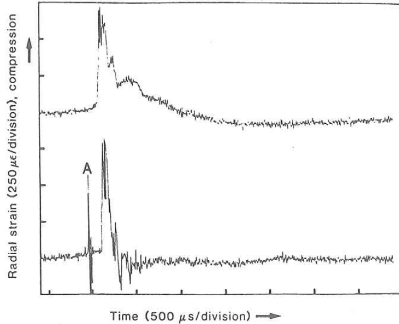
Figure 15, Radial strain measured at a distance of 600mm from the blasthole using cartridged emulsion. (Upper - Normal blasthole, Lower - Lined blasthole, A - Electrical noise) (Brinkmann, 1994)
