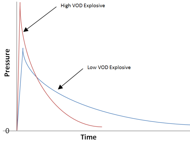
Figure 4, Comparative borehole pressures for higher and lower VOD explosives from time of detonation
