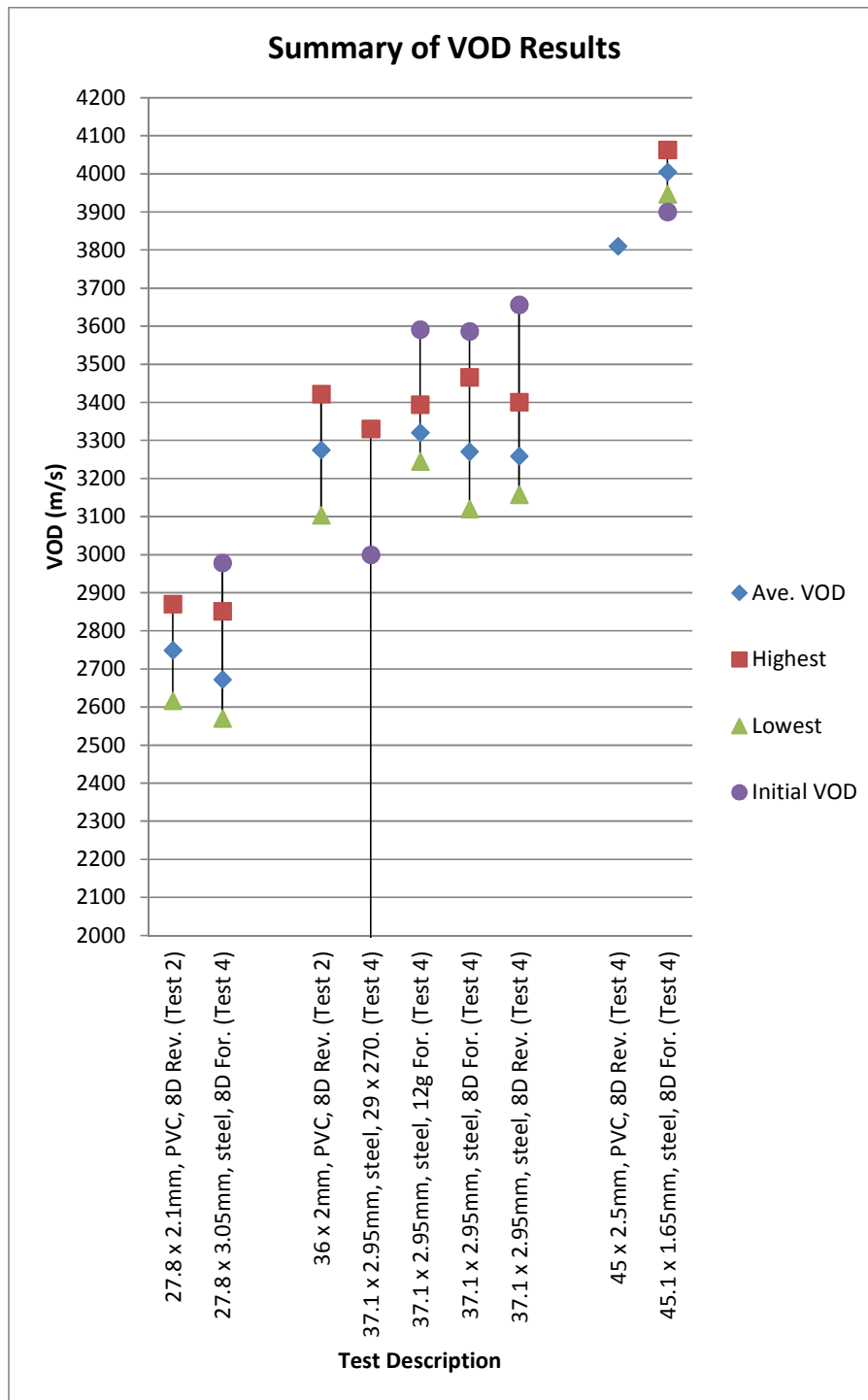
Figure 34, Summary of VOD Results for VOD Test 2 and VOD Test 4
