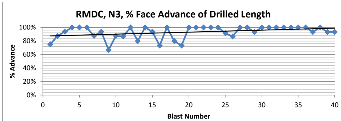
Figure 39, Emulsion B on North 3 raise RMDC – Percentage face advance of drilled length
