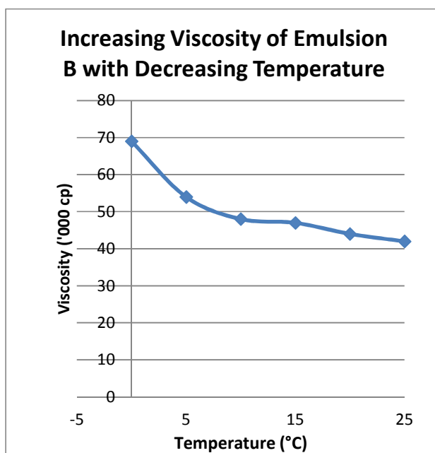
Figure 25, Effect of temperature variations on the viscosity of Emulsion B
