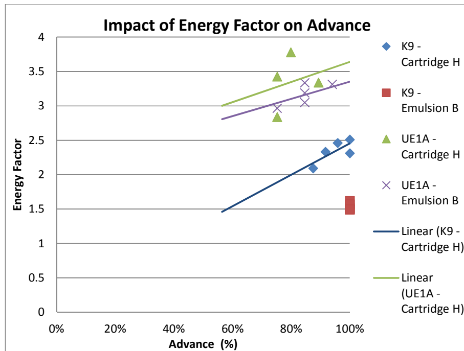
Figure 46, Comparison of energy factor and advance for Emulsion B and Cartridge H, RU
