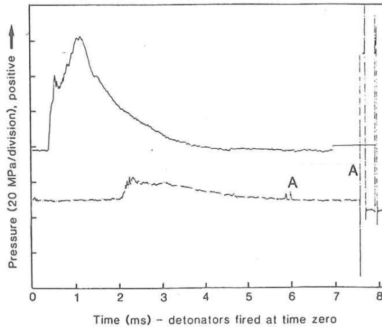
Figure 12, Exhaust pressure measured at the blast hole collar, single-hole blast with emulsion explosive. Trends on vertical axis offset for comparison (Upper un-stemmed; Lower clay stemmed.) (Brinkmann, 1994)
