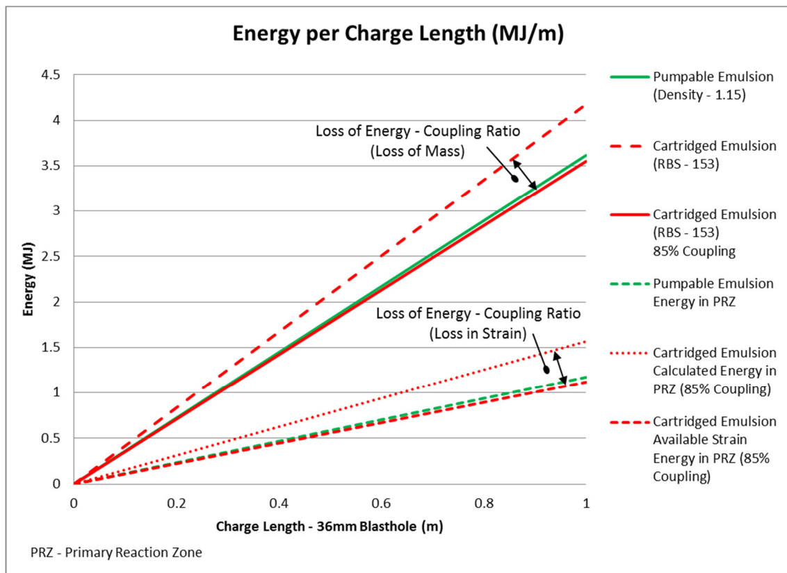
Figure 11, Theoretical energy comparison of a fully coupled bulk emulsion charge with a decoupled cartridged emulsion in 36mm blastholes.
