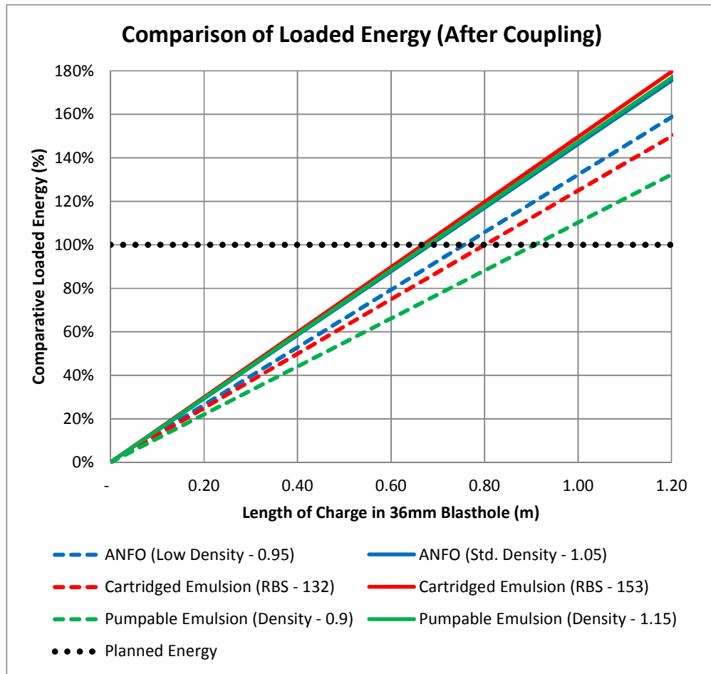
Figure 19, Propensity for the overcharging of blastholes with varying explosives. The planned energy within the 36mm blasthole represents a fully coupled 800 gram charge of ANFO at a density of 1.05, resulting in a charge length of 68cm.
