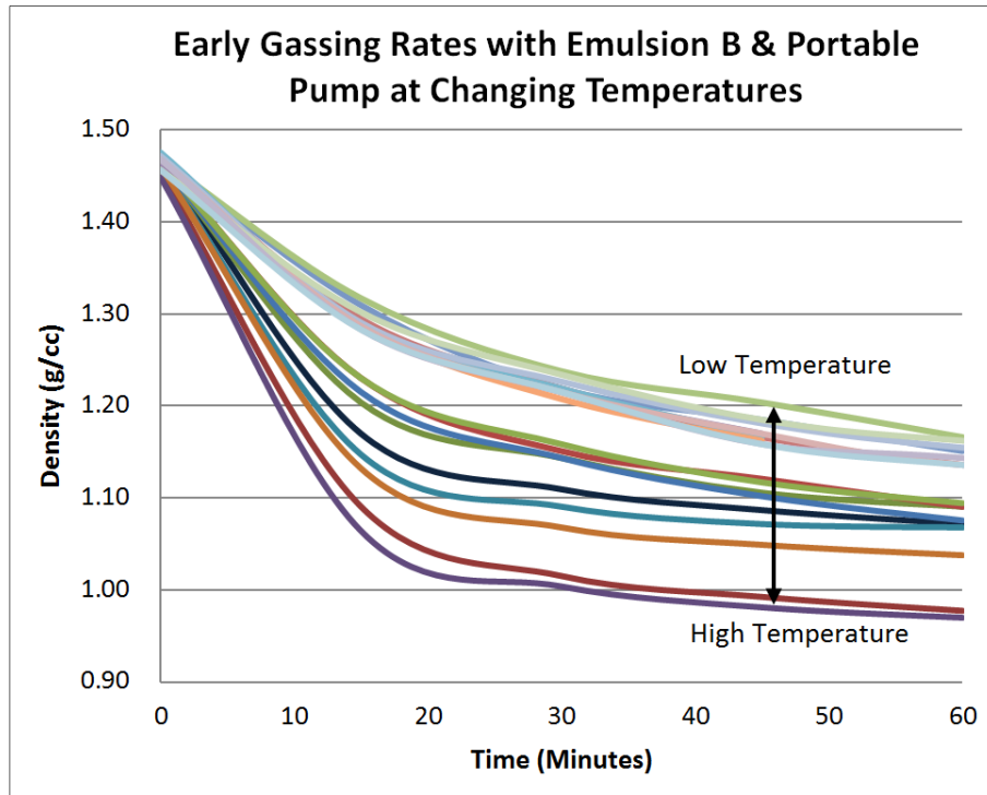
Figure 24, Effect of temperature variations on the gassing rate of an early Emulsion B formulation prior to optimisation.
