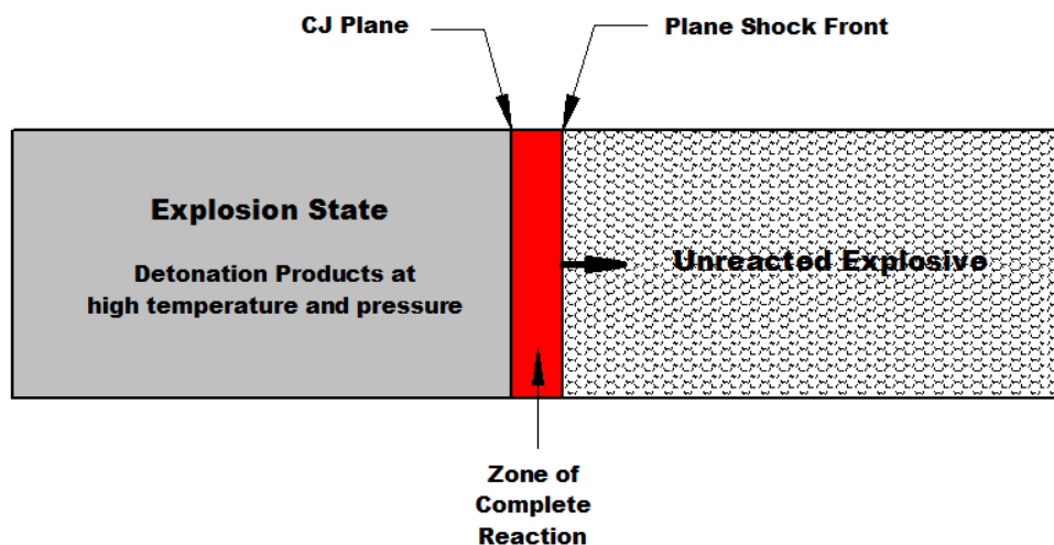
Figure 1, Ideal Detonation Front (Brinkmann, 1990)
