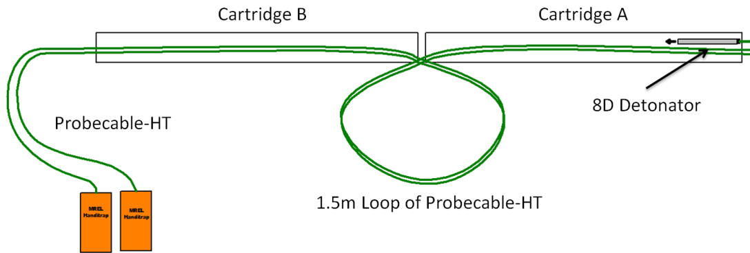
Figure 32, Test 4 – Calibration of MREL Handitrap VOD Recorders
