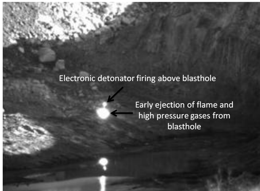
Figure 13, Blasthole detonated with no stemming material. Electronic detonators fired simultaneously inside explosive column and above the blasthole (Brits, 2010)
