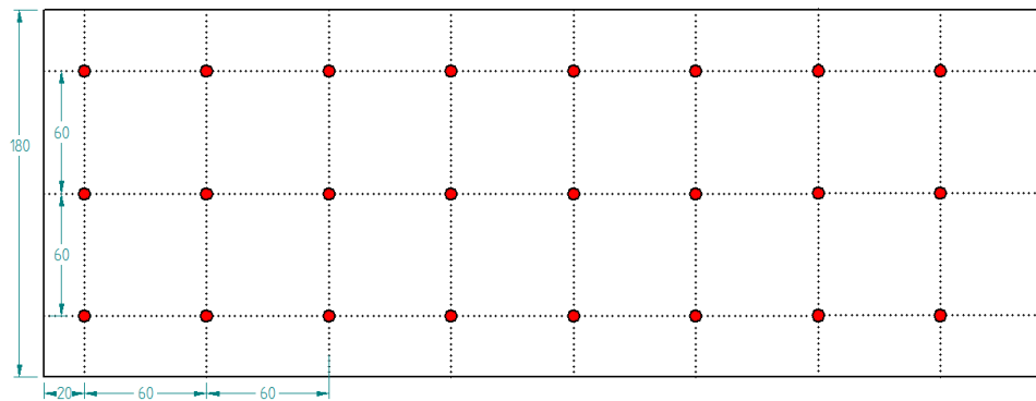
Figure 45, Round Design – Panel 2 West, K9 reef, Rand Uranium
