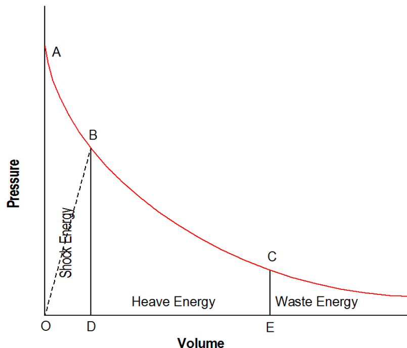
Figure 3, Energy partition in blasting (Lownds, 1991)
