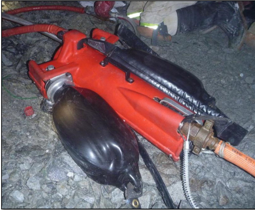
Figure 26, Portable Pump as implemented in the Rand Uranium narrow reef trial
