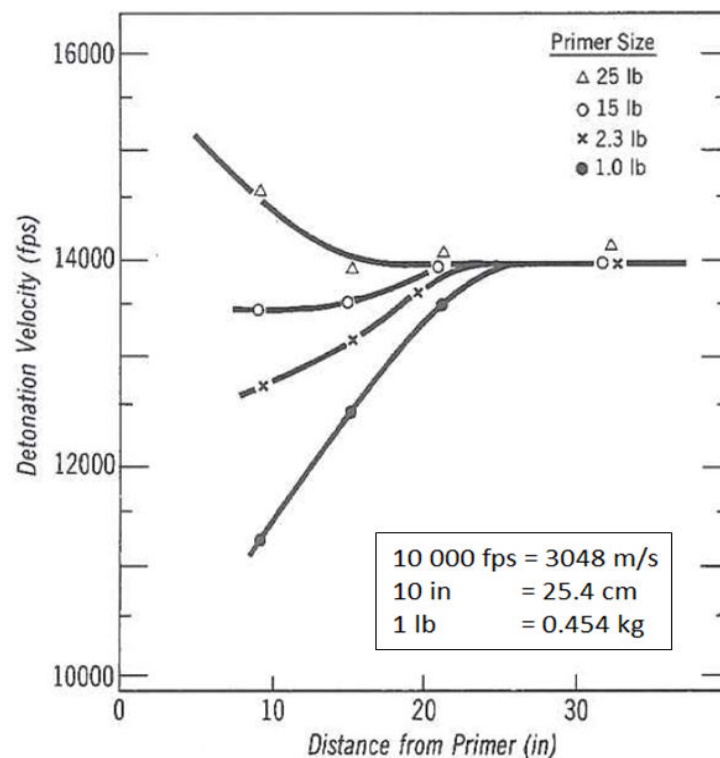
Figure 9, Effect of primer size on the run up of VOD in ANFO (230mm pipe diameter) (ISEE, 1998)
