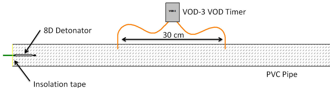
Figure 30, Test 2 – Recording of VOD in PVC pipe with VOD-3 VOD timer
