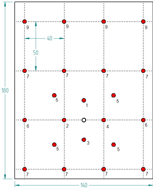
Figure 38, RMDC - Raise Blast Design and Timing Sequence
