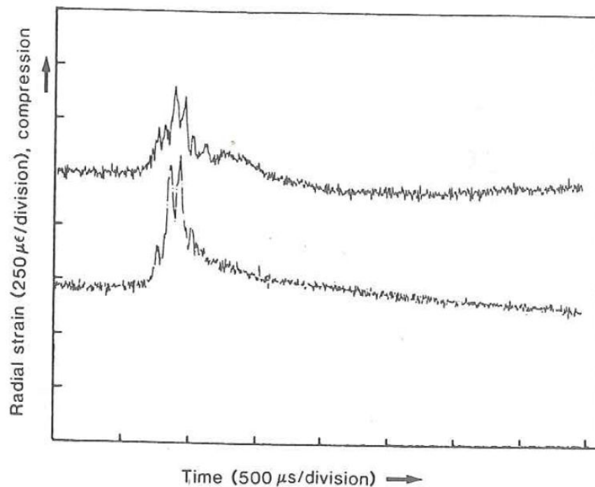
Figure 14, Radial strain measured at a distance of 600mm from the blasthole using dynamite.
