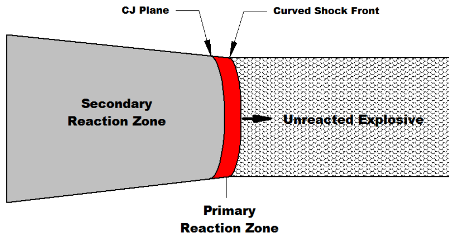
Figure 2, Non-ideal Detonation Theory (Brinkmann, 1990)
