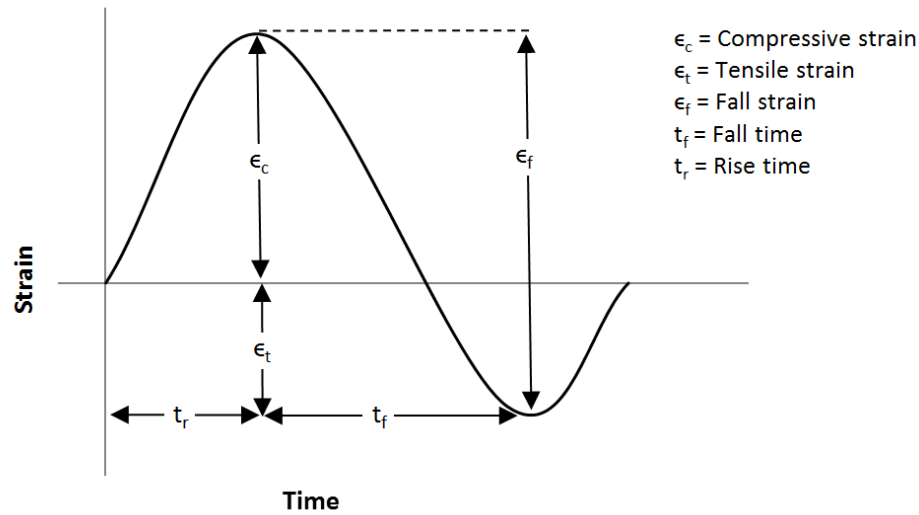
Figure 5, Shape of a measured strain wave generated through the detonation of a blasthole (Saffy, 1961)
