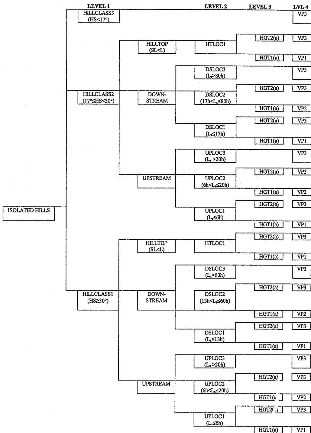
Figure 6.8 Designation of meso-ventilation potentials (VPs) based on: hill slope angle (HS) (level 1), source location with regard to horizontal recirculation zones (level 2), and source height with regard to inner layer depth (level 3).
