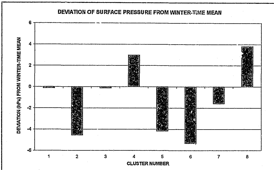
Figure 6.1 Deviation of average surface pressure for each cluster identified for Irene from the wintertime mean surface pressure for this station (1989-1992).
