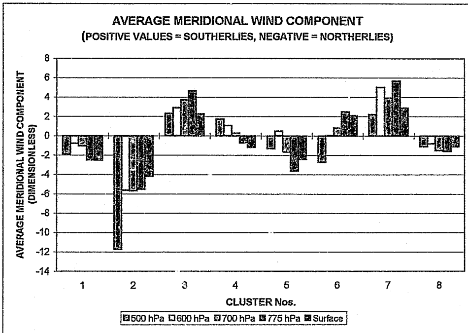
Figure 6.5 Average meridional wind component (at various pressure levels) for each of the clusters identified at Irene (1989-1992).
