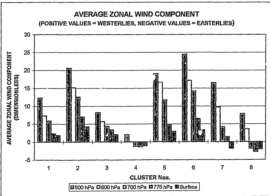
Figure 6.4 Average zonal wind component (at various pressure levels) for each of the clusters identified at Irene (1989-1992).
