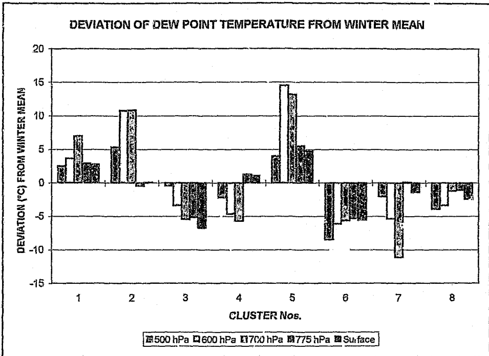
Figure 6.3 Deviation of average dew point temperature (at various pressure levels) for each cluster identified for Irene from the winter mean dew point temperature.
