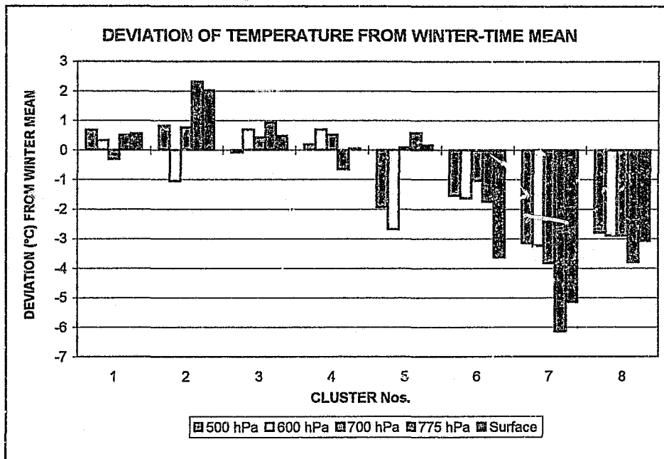
Figure 6.2 Deviation of average temperature (at various pressure levels) for each cluster identified for Irene from the wintertime mean temperature for this station (1989-1992).
