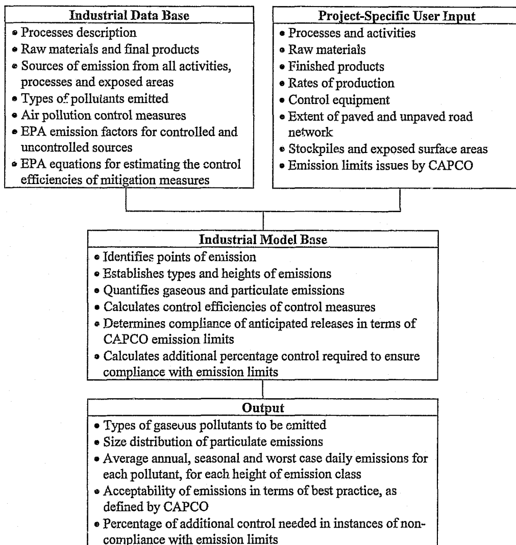
Figure 1.2 Structure of the industrial data base, model base and user interface.
