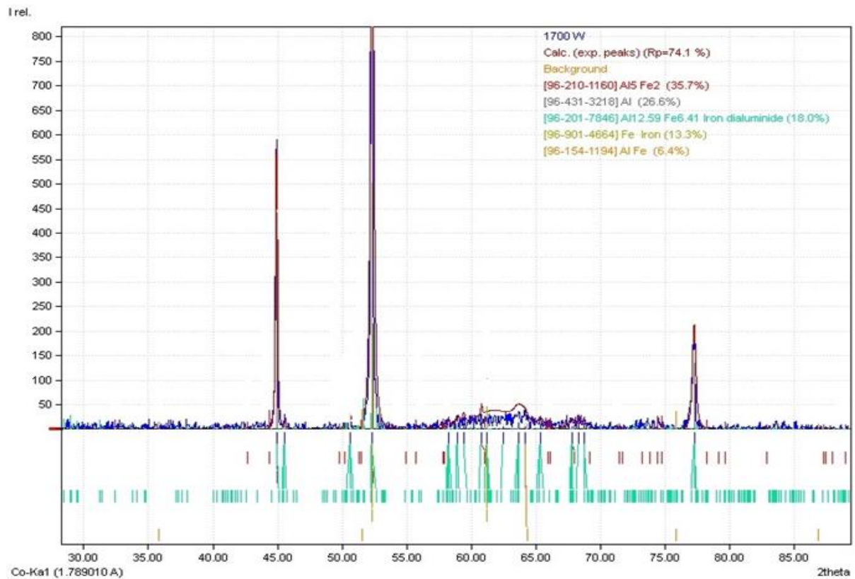
Figure 6.7: XRD pattern for 1700 W showing the quantity of elements and IMC phases
