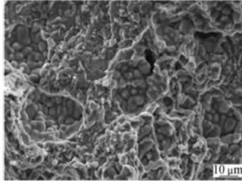
Figure 2.6: SEM image showing surface fracture of aluminium [75].
