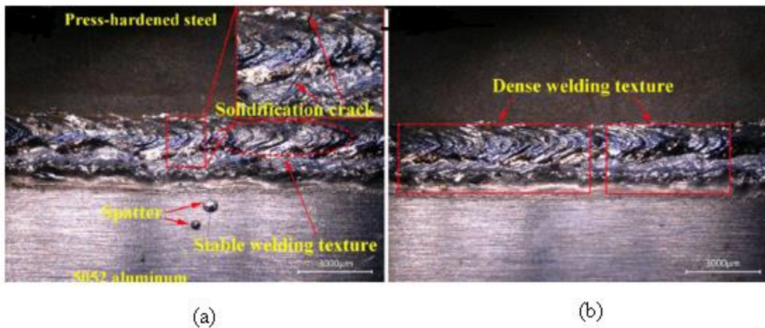
Figure 2.8: The appearance of the weld at various laser offsets: (a) 0.1 mm, (b) 0.2 mm [88].
