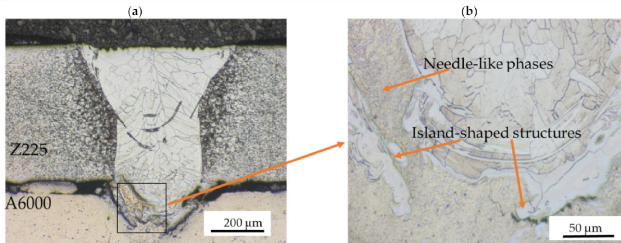
Figure 5. Optical micrographs for 1200 W and 3 m/min showing (a) columnar grain structure at 20×; (b) weld interface with irregular phases at 50×.
