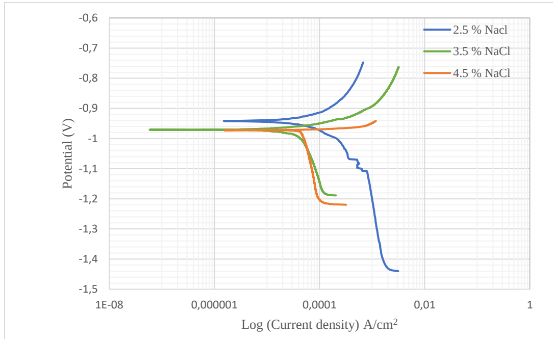
Figure 4.17: Polarization curves indicating the effect of NaCl concentration on the corrosion properties of dissimilar weld joints between Z225 and Al 5754.
