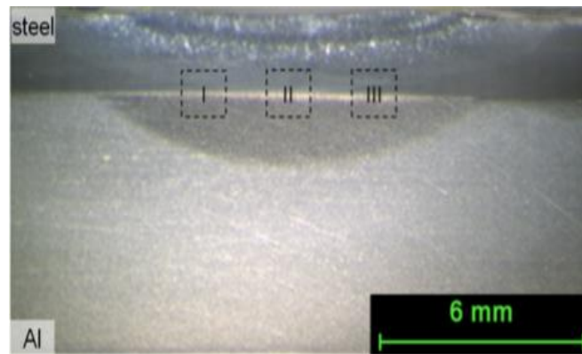
Figure 2.14: Microsection of the IMC layer thickness [106].
