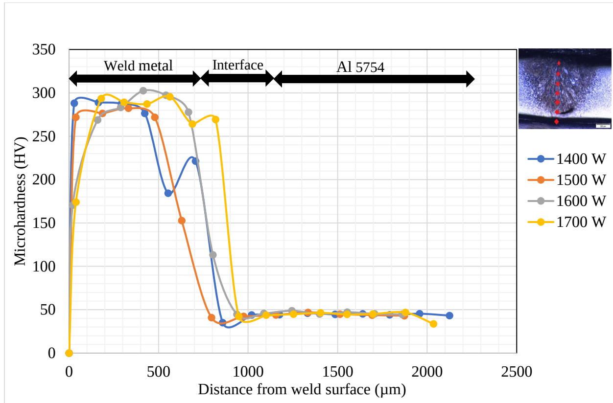
Figure 4.19: Effect of laser welding power on WM microhardness
