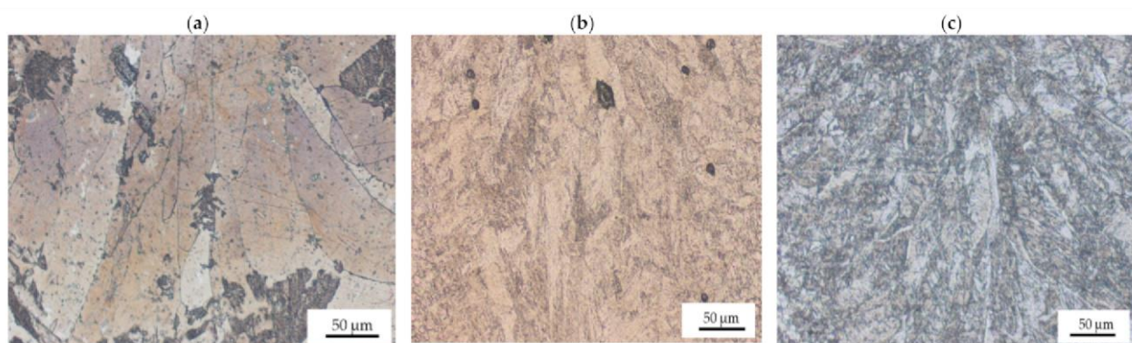
Figure 7. Optical micrographs for 950 W and different laser welding speeds at 50× magnification showing (a) large columnar grain structure at 2 m/min; (b) micropores at 3 m/min; (c) fine equiaxed grain structure at 4 m/min.
