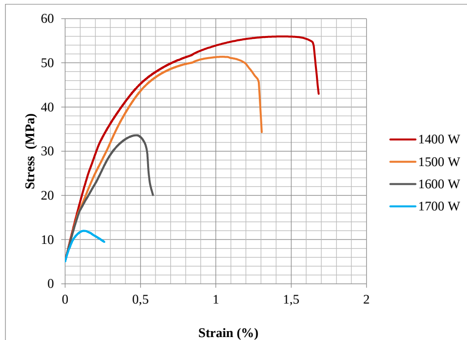
Figure 4.24 : Stress-strain curves for different laser powers and constant speed of 3.0 mm/s.
