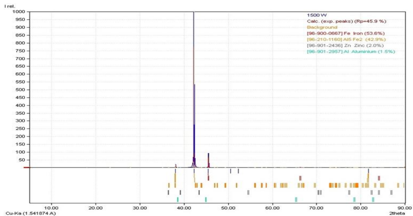
Figure 6.5: XRD pattern for 1500 W showing the quantity of elements and IMC phases
