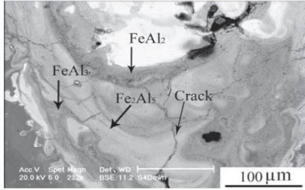
Figure 2.4: Weld zone showing brittle IMCs and a crack [72].
