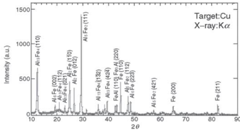
Figure 2.13: Various types of IMCs shown on XRD pattern of a fracture surface [105].
