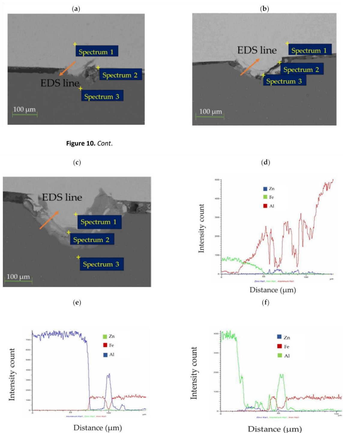
Figure 10. SEM images showing direction of EDS line scan and EDS points; (a,d) 800 W; (b,e) 1000 W; (c,f) 1200 W.
