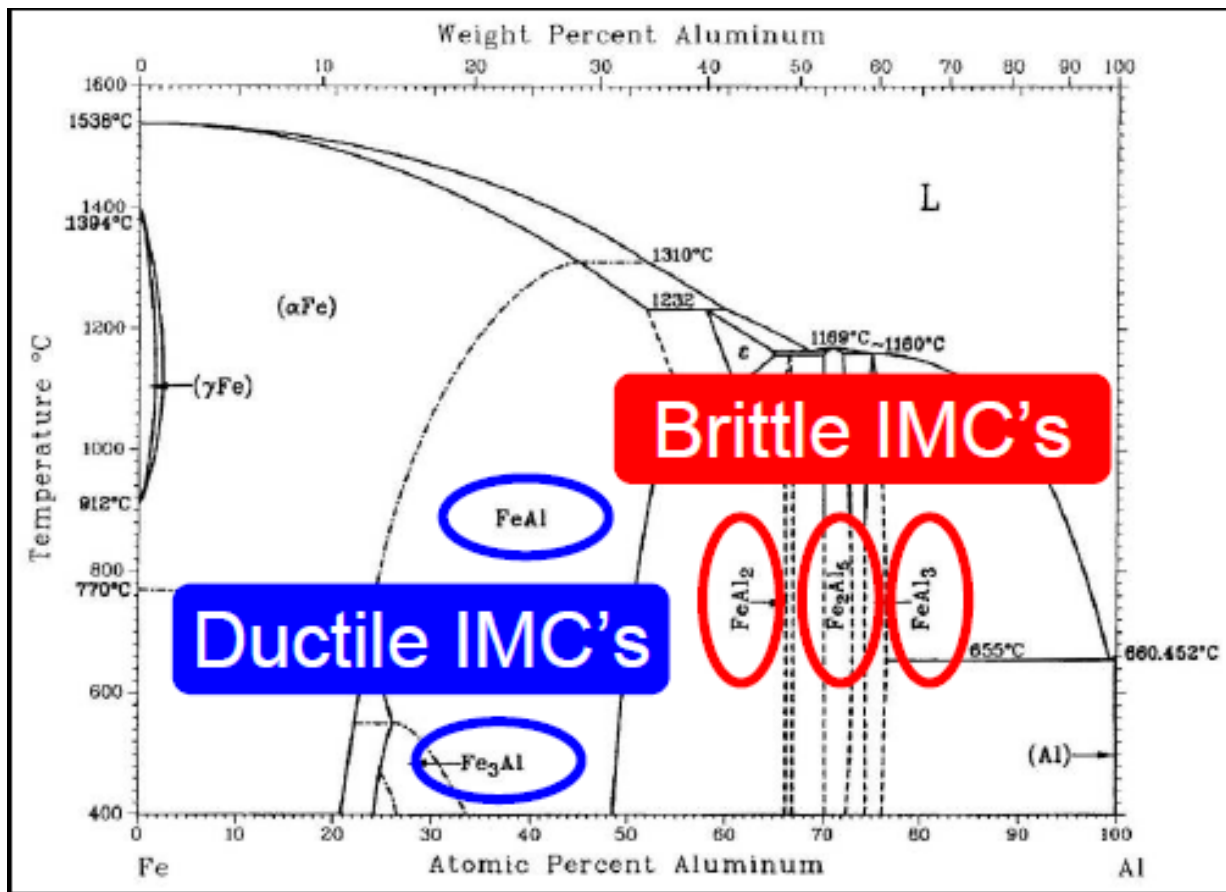
Figure 1.1: Binary equilibrium phase diagram of Fe and Al [6].
