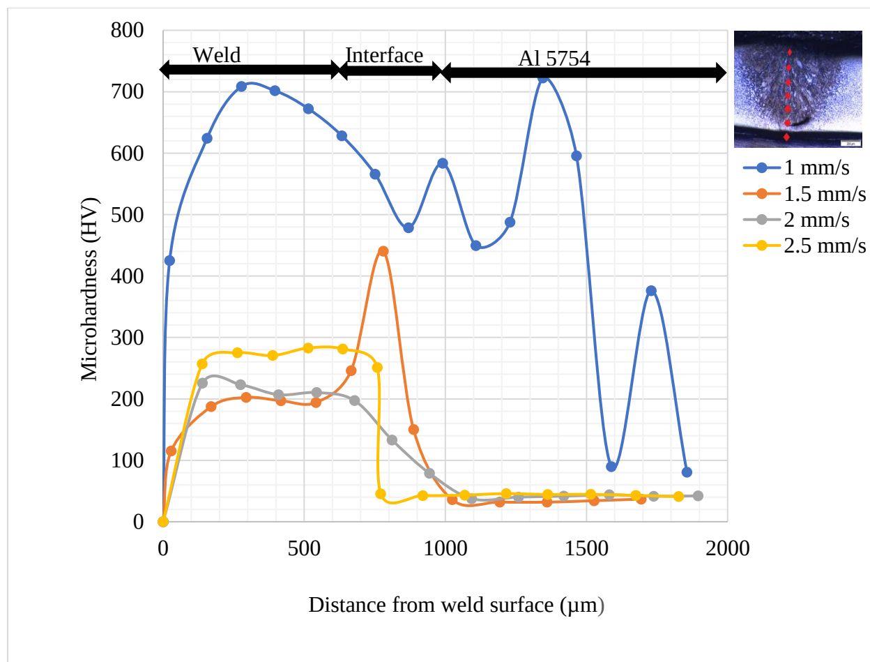
Figure 4.20: Effect of laser welding speed on weld metal microhardness
