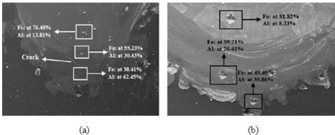
Figure 2.11: EDS analysis points at varying heat input. (a) 33.3 J/mm, (b) 28.5 J/mm [104].
