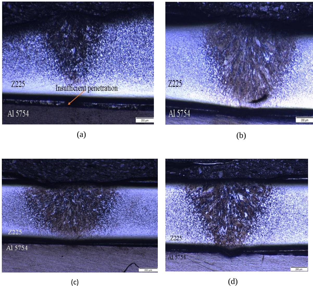
Figure 4.2: Optical micrographs for dissimilar joints produced at a constant laser welding speed of 3.0 mm/s and laser welding power of (a) 1400 W, (b) 1500 W, (c) 1600 W and (d) 1700 W.
