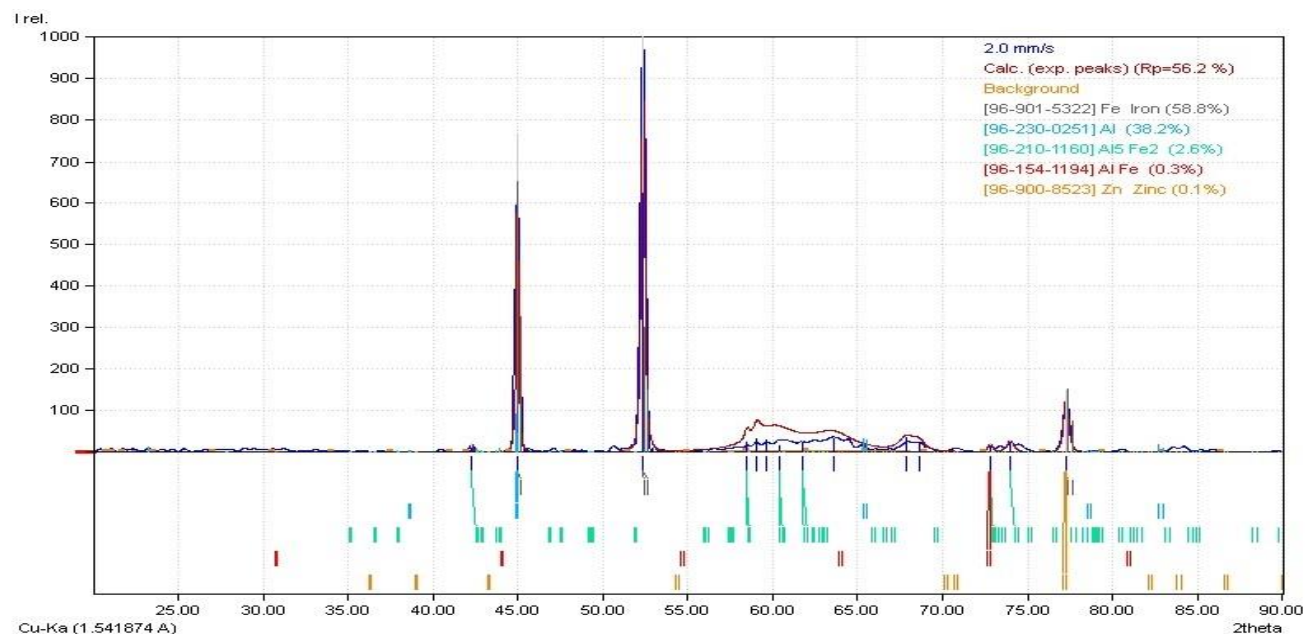
Figure 6.2: XRD pattern for 2.0 mm/s showing the quantity of elements and IMC phases
