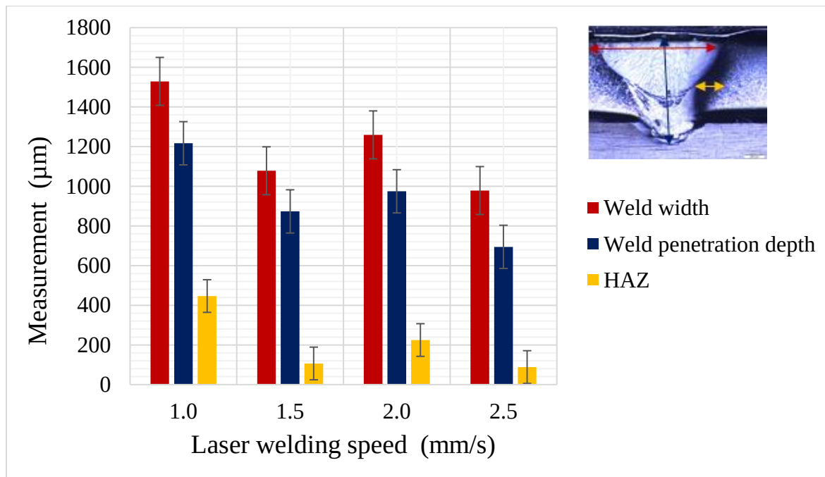
Figure 4.4: Effect of laser welding speed on the weld bead dimensions
