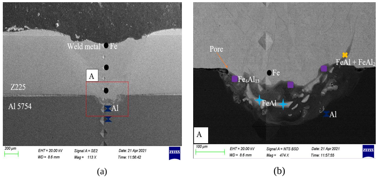
Figure 4.11: SEM images of IMCs at 1700 W. (a) Weld cross-section, (b) Interfacial region (A).
