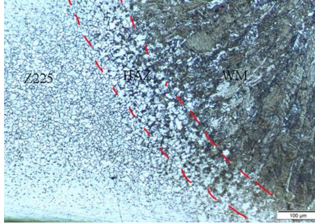
Figure 4.7: Transition of grains from BM to WM.
