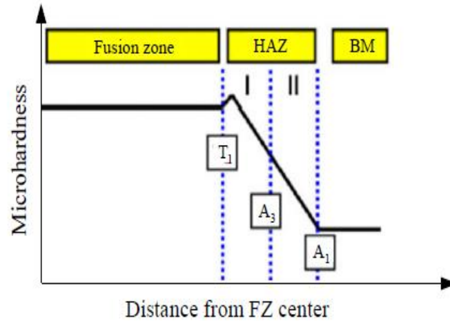
Figure 2.19: Schematic of a representative hardness profile of steel-Al fusion welds [111].
