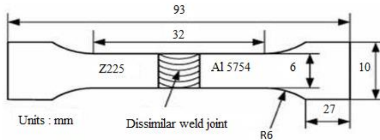
Figure 3.3: Tensile shear strength test specimen (modified from) [123].
