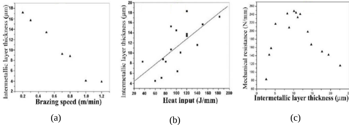
Figure 2.9: Influence of welding parameters on the IMC thickness (a) Laser brazing speed, (b) Heat input, (c) Influence of IMC layer thickness on mechanical resistance [90].
