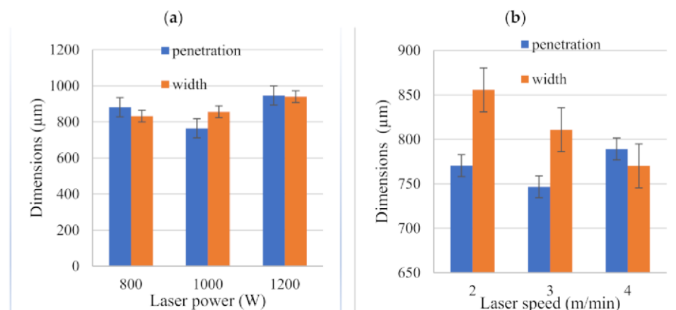
Figure 8. Effect of system parameters on the weld bead dimensions, (a) effect of laser power; (b) effect of laser welding speed.
