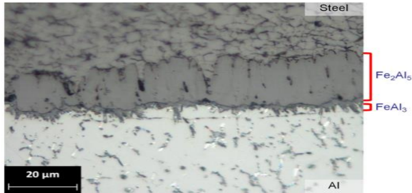
Figure 2.16: Two different IMC layers [106].
