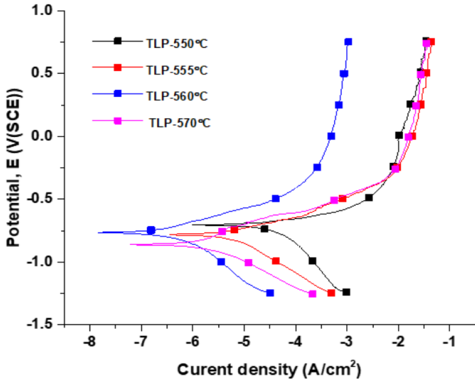
Figure 2.18: Polarization curves of joints produced at different TLP bonding temperatures [110].
