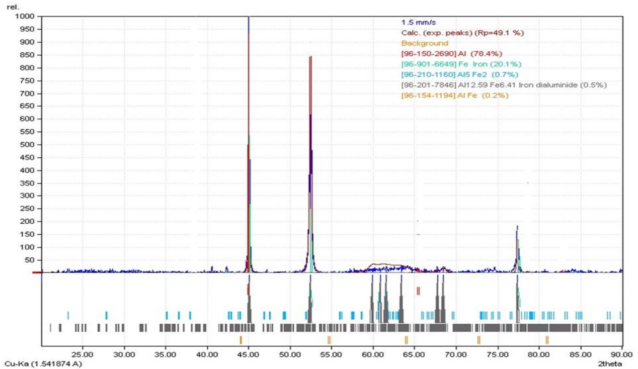
Figure 6.1: XRD pattern for 1.5 mm/s showing the quantity of elements and IMC phases
