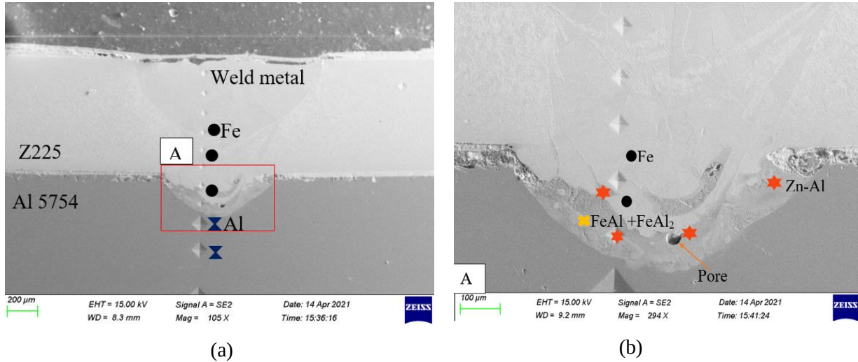
Figure 4.14: SEM images of IMCs at 2.0 mm/s. (a) Weld cross-section, (b) Interfacial region (A).
