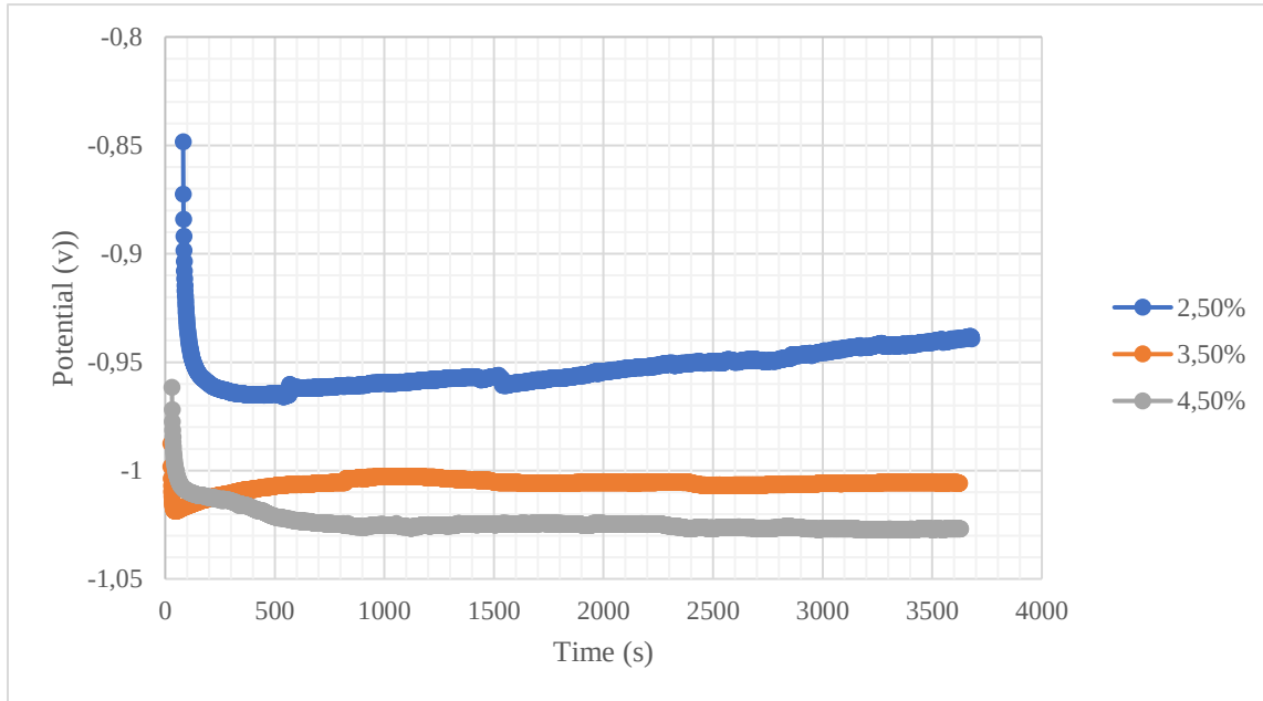
Figure 6.8: Impact of NaCl concentration on the OCP values
