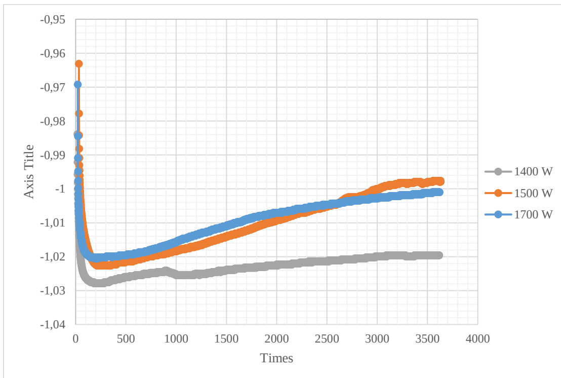
Figure 6.9: Impact of laser welding power on OCP values
