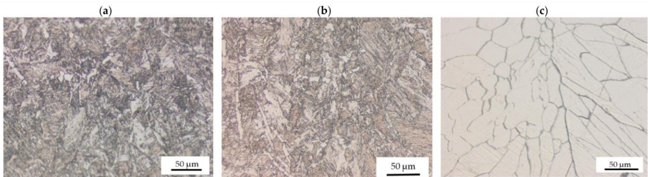
Figure 5. Optical micrographs for 1200 W and 3 m/min showing (a) columnar grain structure at 20×; (b) weld interface with irregular phases at 50×.
