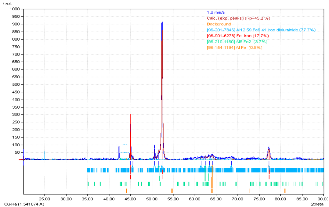
Figure 4.16: XRD pattern for 1.0 mm/s showing the detected elements and IMC phases detected.
