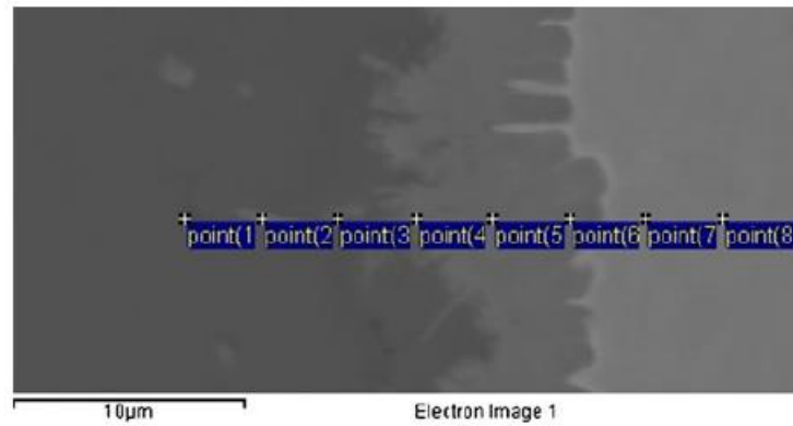
Figure 2.12: Points of EDS performed on the micrograph [10].
