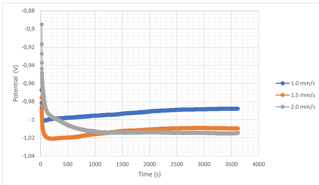
Figure 6.9: Impact of laser welding speed on OCP values
