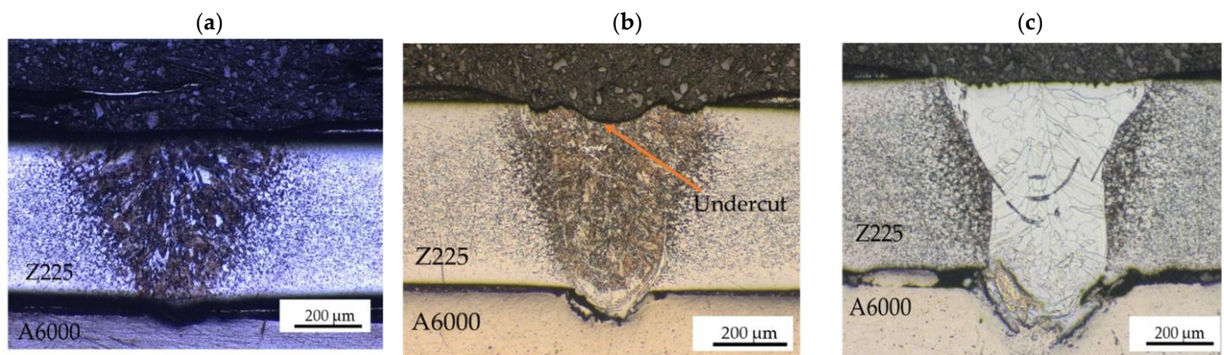
Figure 3. Optical micrographs for 3 m/min and different laser powers at 20× showing: (a) insufficient fusion at 800 W; (b) undercutting at 1000 W; (c) columnar grain structure at 1200 W.
