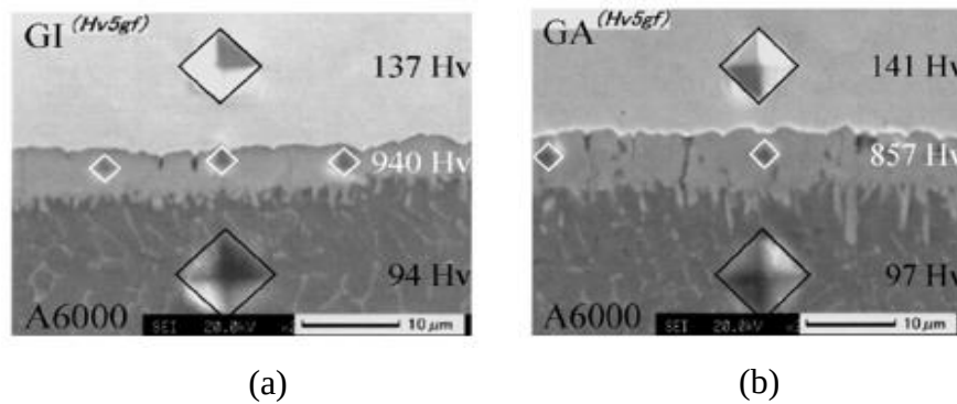
Figure 2.21: Measurements of Vickers hardness indentations at the joint interface [8].
