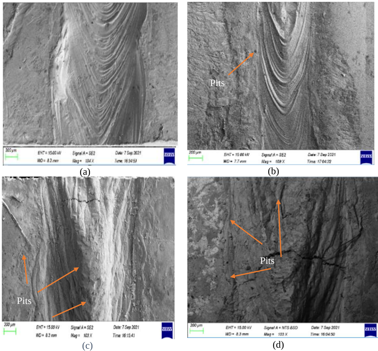
Figure 6.10: Z225/Al 5754 surface before and after being exposed to different NaCl concentrations. (a) before exposure, (b) after being exposed to 2.5 % NaCl, (c) 3.5 % NaCl, (d) 4.5 % NaCl
