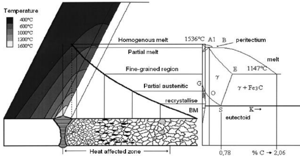
Figure 2.10: Relationship between the microstructure of welded structural steel and thermal cycle [95].
