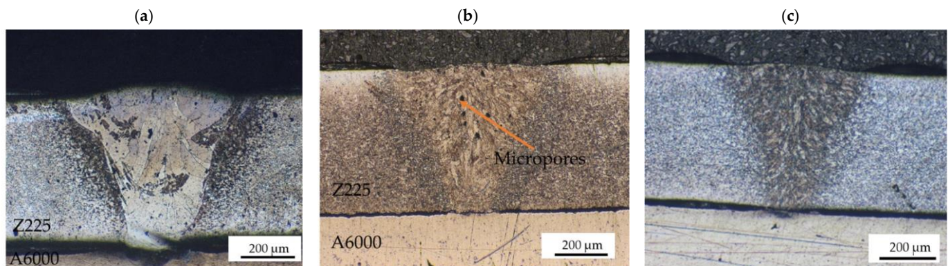
Figure 4. Optical micrographs for 950 W and different laser welding speeds at 20× magnification showing (a) columnar grain structure at 2 m/min; (b) micropores at 3 m/min; (c) insufficient fusion at 4 m/min.
