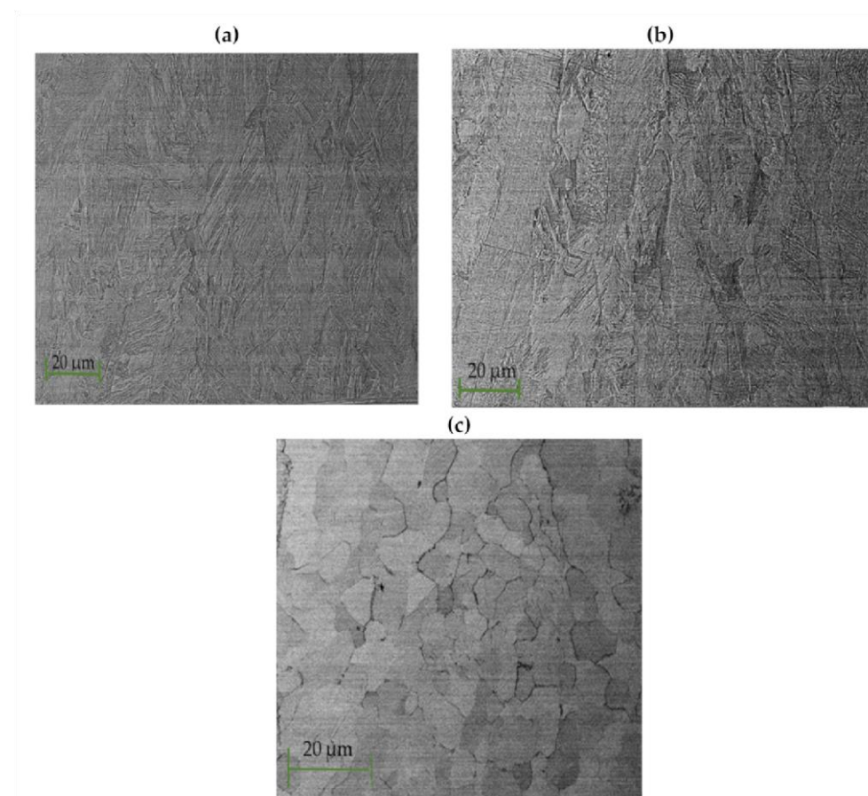
Figure 9. SEM images showing the effect of laser welding power on the microstructure of the weld metal, (a) 800 W; (b) 1000 W; (c) 1200 W.
