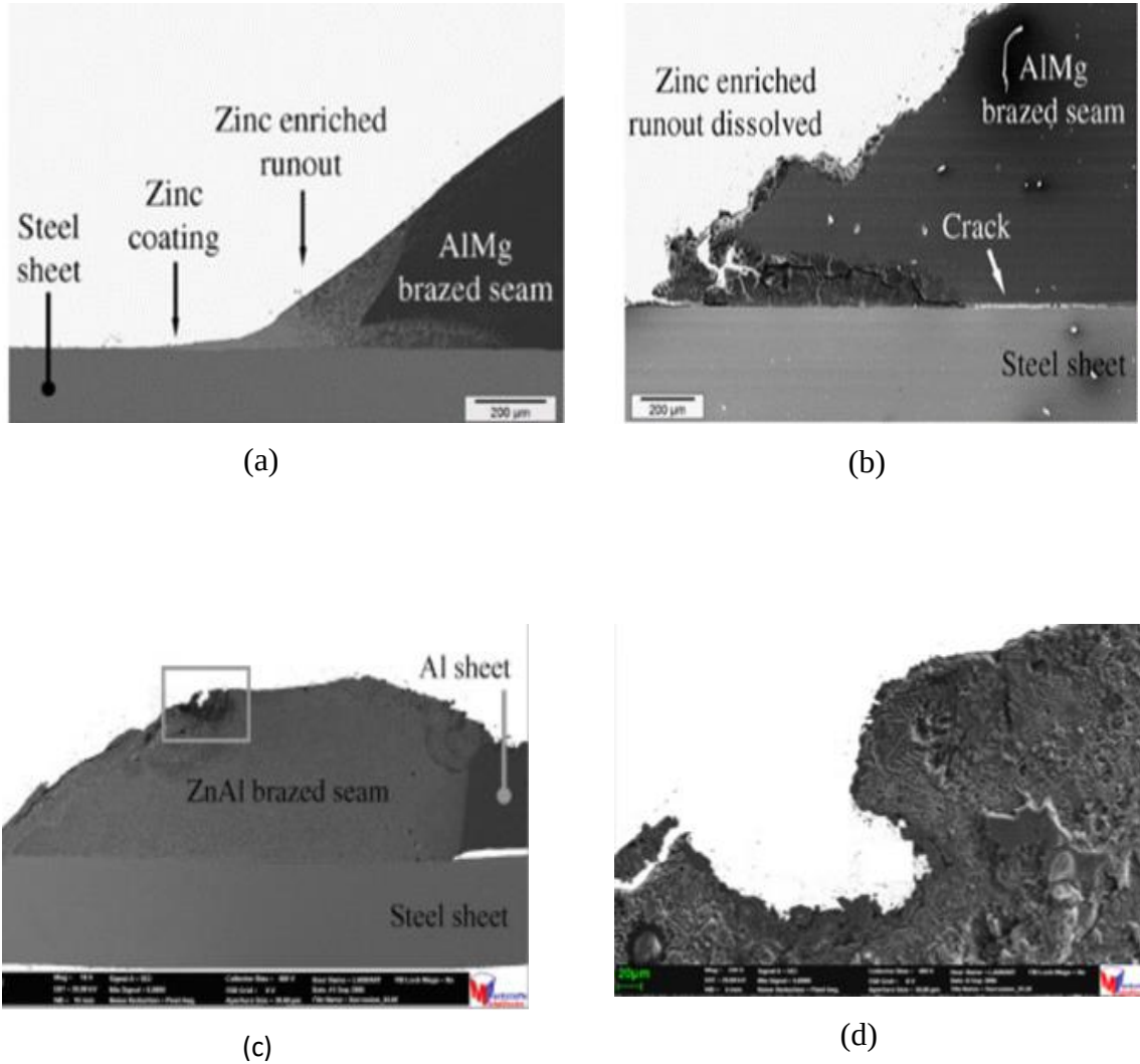
Figure 2.17: Weld joint produced from \text{AlMg}_6\text{Mn} filler material (a) before corrosion, (b) after corrosion and weld joint produced from \text{ZnAl}_2 filler material (c) before corrosion, (d) after corrosion [109].
