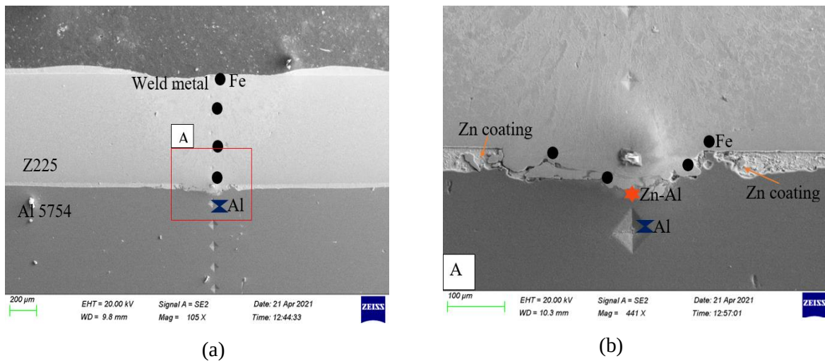
Figure 4.15: SEM images of IMCs at 2.0 mm/s. (a) Weld cross-section, (b) Interfacial region (A).
