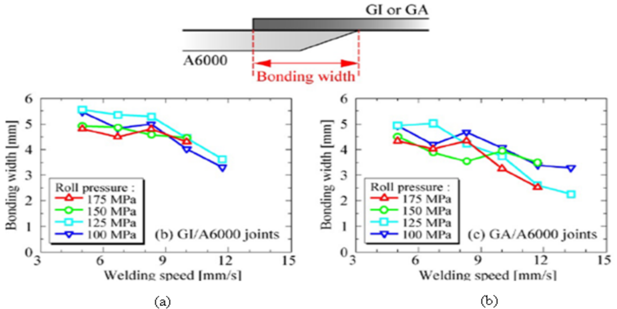
Figure 2.7: Influence of welding speed on bonding width at varying roll pressures; (a) GI-A6000 joint, (b) GA-A6000 joint [8].
