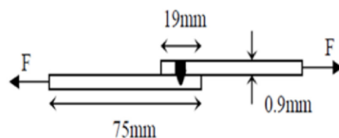
Figure 1. Specimen used for tensile shear strength test indicating direction of applied stress [16].
