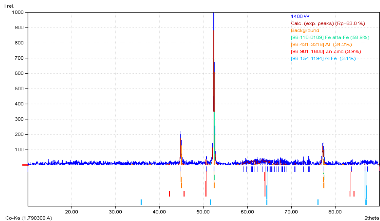
Figure 6.4: XRD pattern for 1400 W showing the quantity of elements and IMC phases
