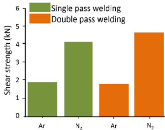
Figure 2.22: Influence of Ar and \text{N}_2 on shear strength using single and double pass welding [117].
