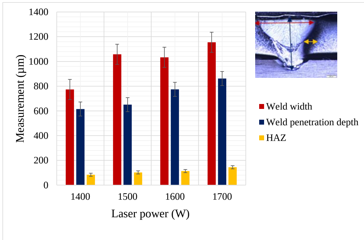
Figure 4.3: Effect of laser welding power on the weld bead dimensions
