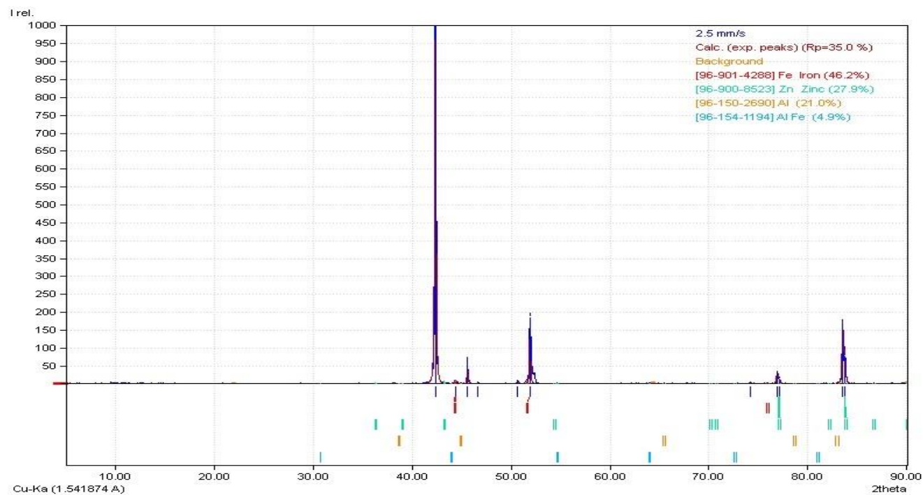
Figure 6.3: XRD pattern for 2.5 mm/s showing the quantity of elements and IMC phases
