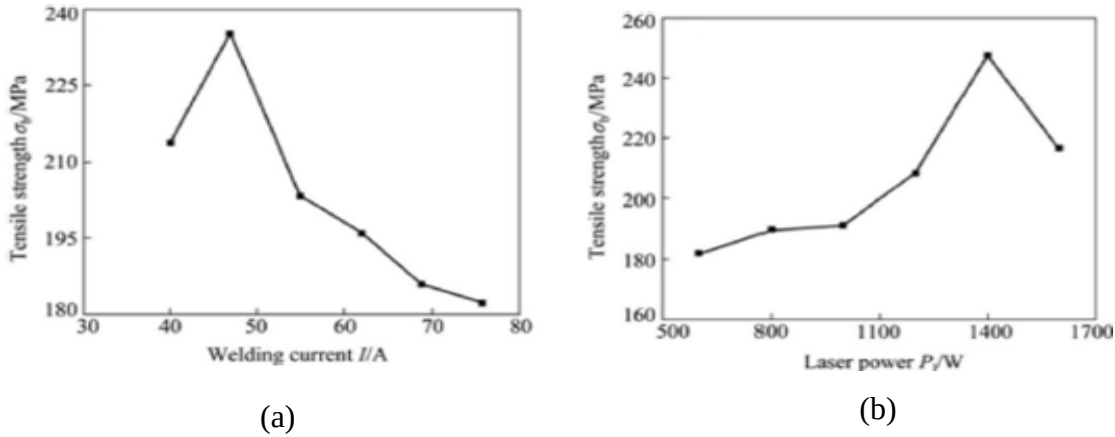
Figure 2.5: Tensile strength of the weld; (a) Varying welding current (b) Varying laser power [75].
