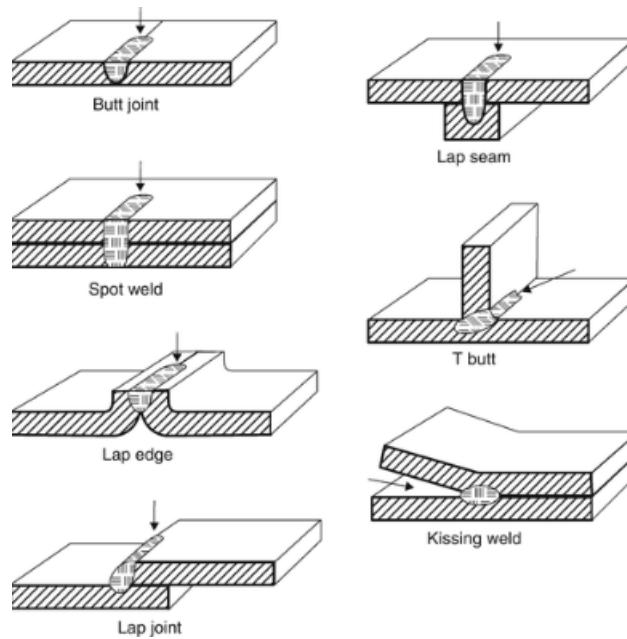
Figure 2.2: Possible laser welding configurations [58].
