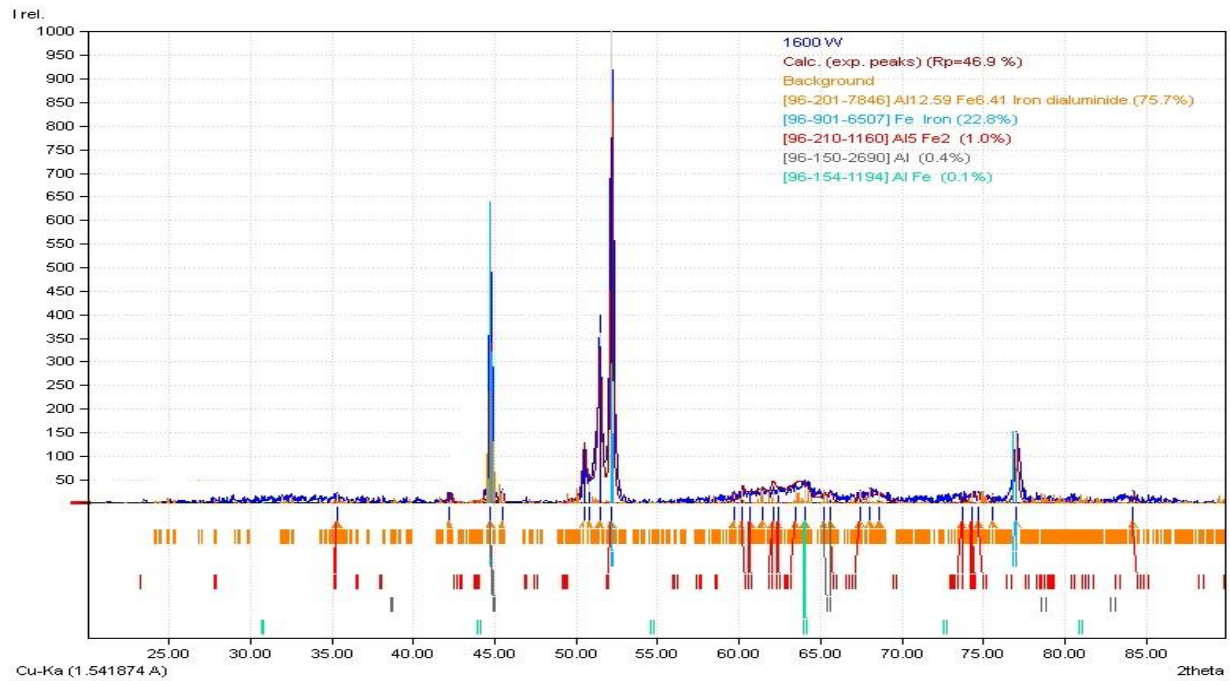
Figure 6.6: XRD pattern for 1600 W showing the quantity of elements and IMC phases
