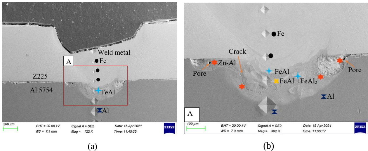
Figure 4.13: SEM images of IMCs at 1.5 mm/s. (a) Weld cross-section, (b) Interfacial region (A).
