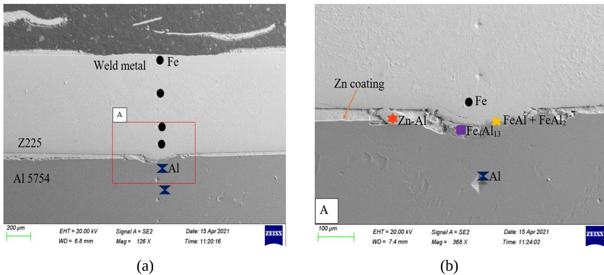
Figure 4.10: SEM images of IMCs at 1600 W. (a) Weld cross-section, (b) Interfacial region (A).
