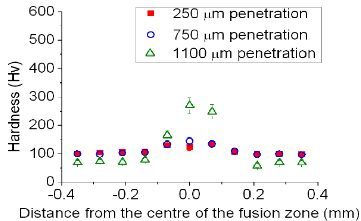
Figure. 2.20: Hardness distribution for single pass welding at different penetration depths [32].
