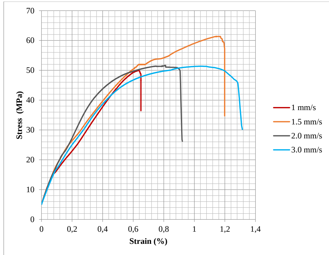
Figure 4.23 : Stress-strain curves for constant laser power of 1500 W and varying laser welding speed.
