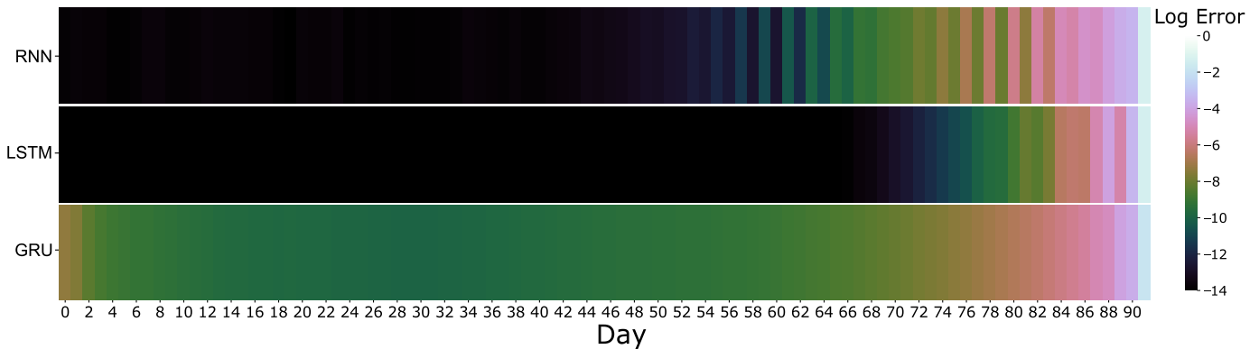
FIGURE 3.2: The log error introduced after adding 1% of noise at each day [1]
