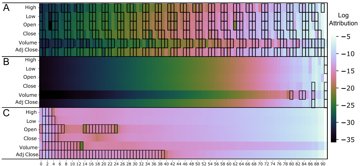
FIGURE 3.3: . The absolute log attributions for A) RNN, B) LSTM and C) GRU neural networks. Bordered areas represent negative attributions [1]
