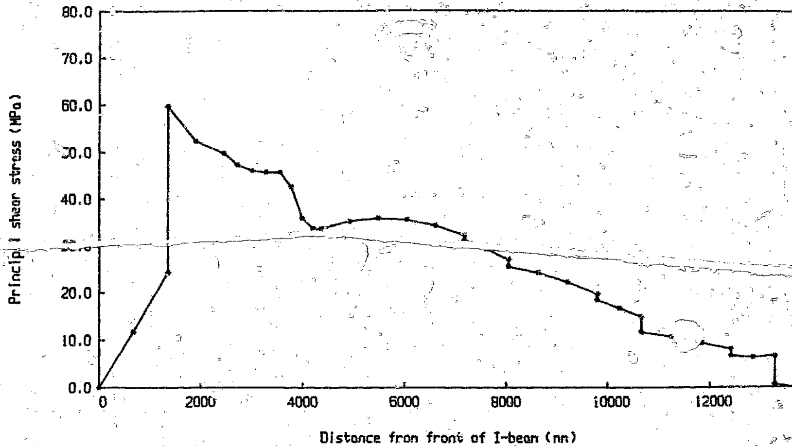
Graph 4.33 Principal shear stress distribution in the main I-beam welds above the neutral axis (Case 1 loading)
