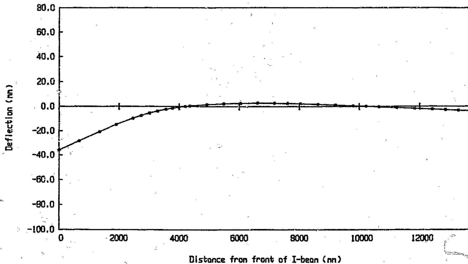
Graph 4.10 Deflection diagram for main chassis I-beam (Case 3 loading)
