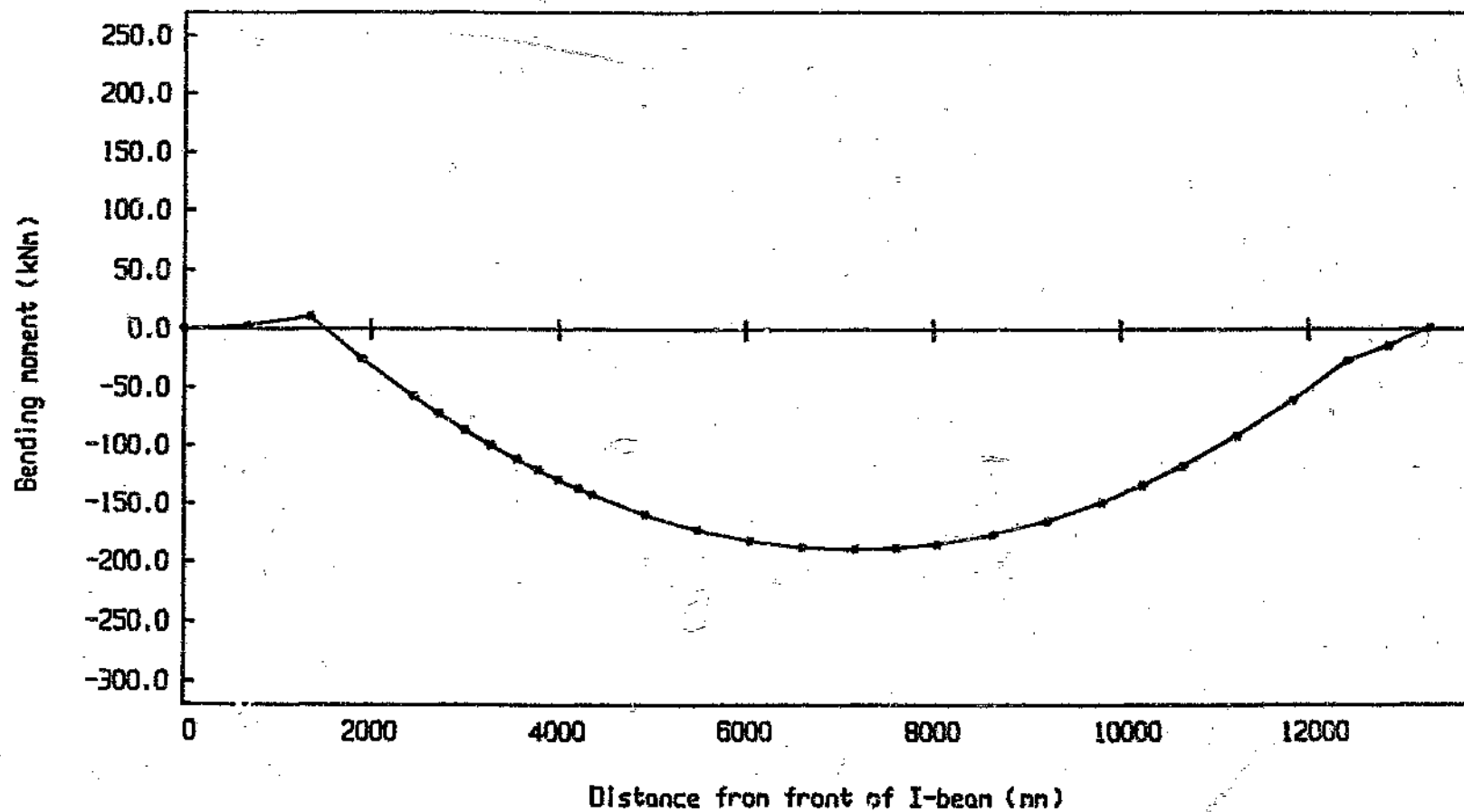
Graph 4.18 Bending moment distribution on main chassis I-beam (Case 6 loading)
