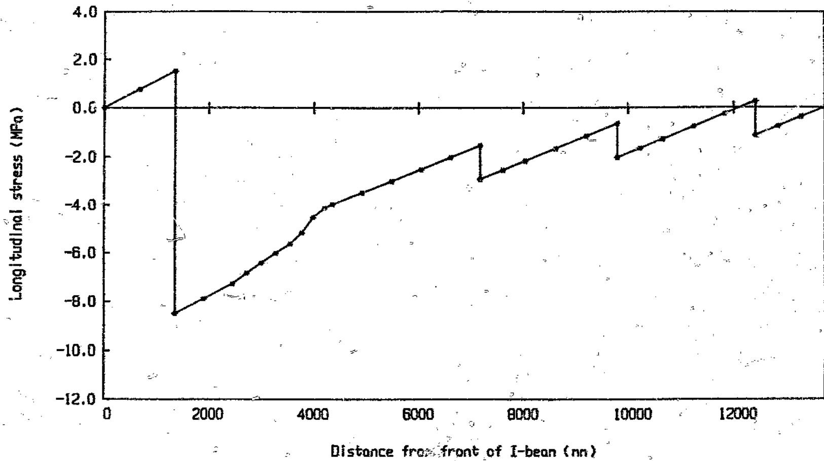
Graph 4.23 Longitudinal direct stress distribution (Case 1 loading)
