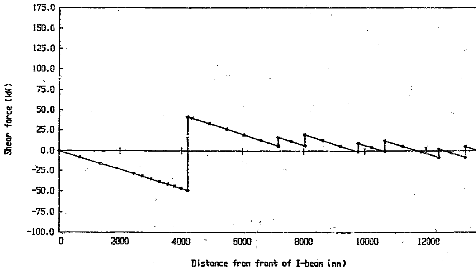
Graph 4.8 Shear force distribution on main chassis I-beam (Case 3 loading)
