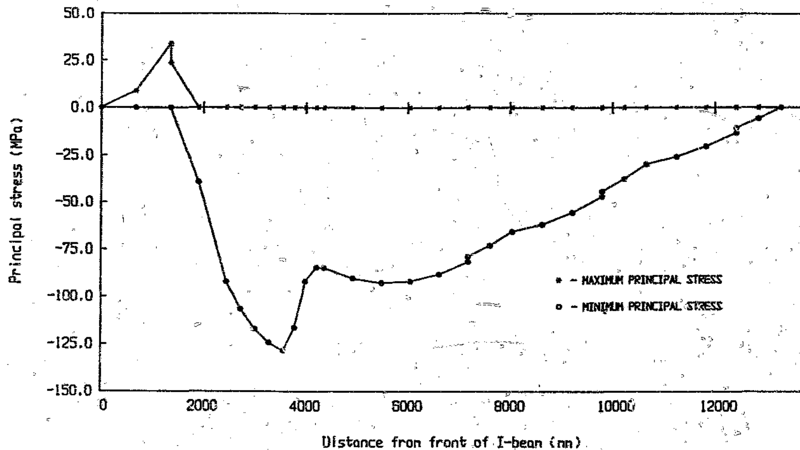
Graph 4.26 Principal stress distribution at the extreme fibres (Upper flange - Case 1 loading)
