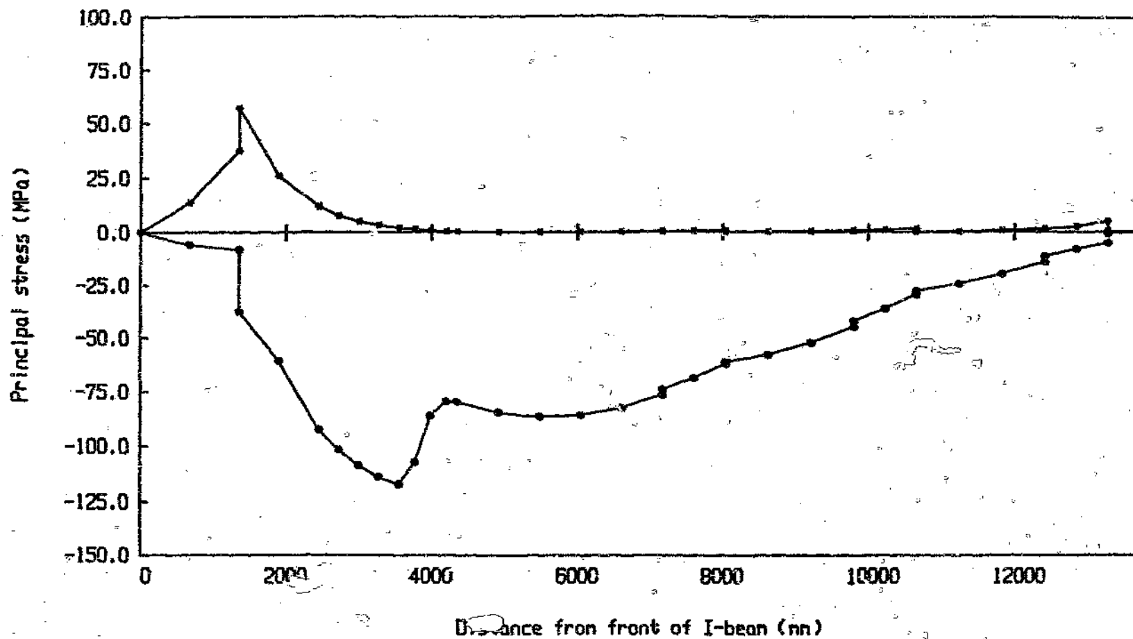
Graph 4.29 Principal stress distribution at the web/flange joint above the neutral axis (Case 1 loading)
