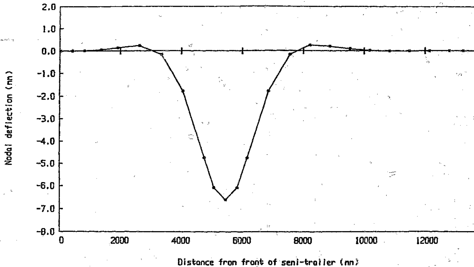
Graph 4.38 Nodal deflection diagram for semi-trailer side rail (Loadcase 1)
