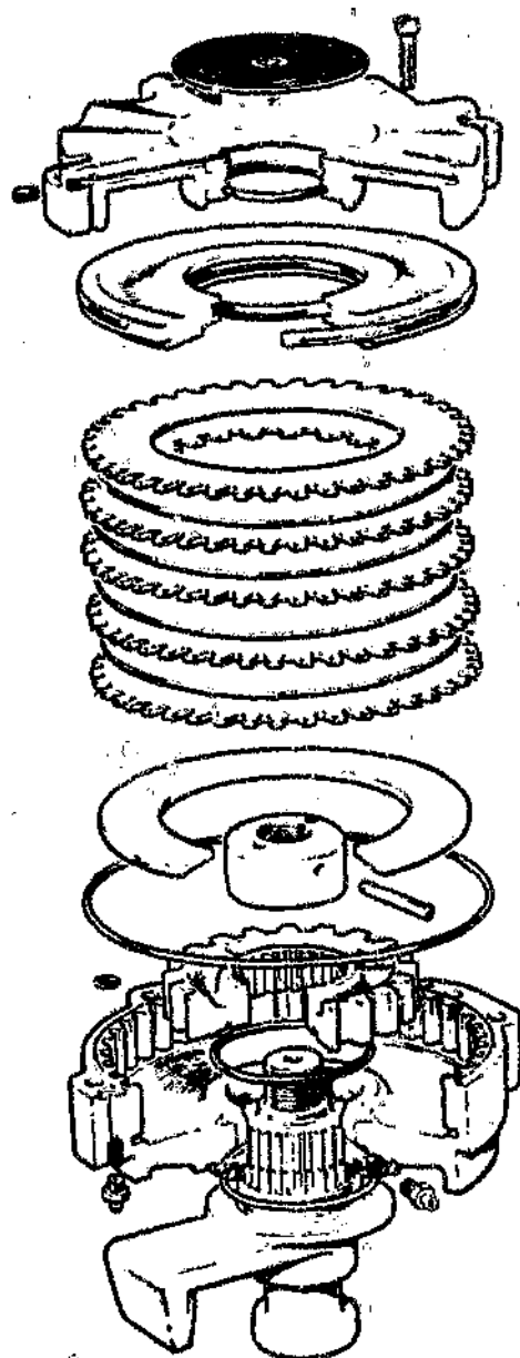
Exploded drawing of Hope anti-jack-knife device.
