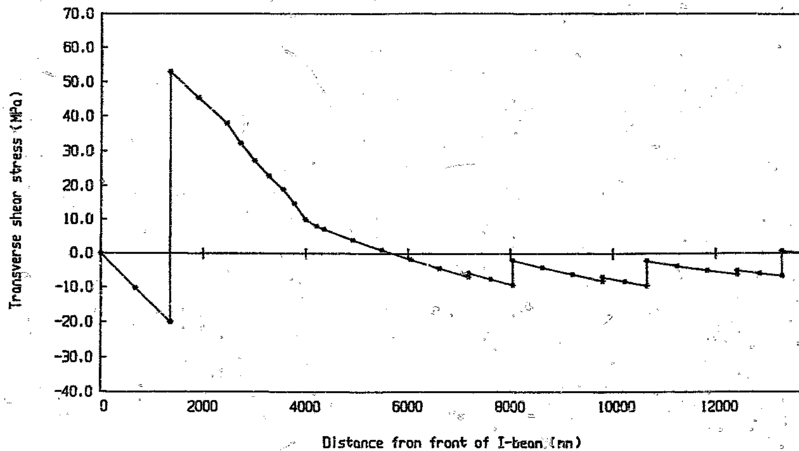
Graph 4.24 Maximum transverse shear stress distribution (Neutral axis - Case 1 loading)
