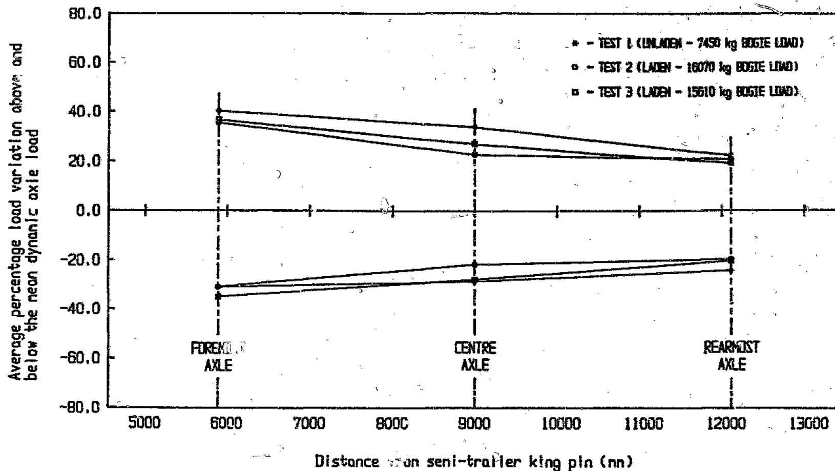
Graph 3.2 Average maximum percentage load variation recorded during the suspension equalization testing of the Henred Fruehauf PET trailer (Freeway at approx. 75 km/h)
