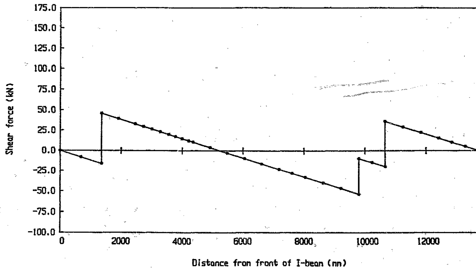
Graph 4.14 Shear force distribution on main chassis I-beam (Case 5 loading)
