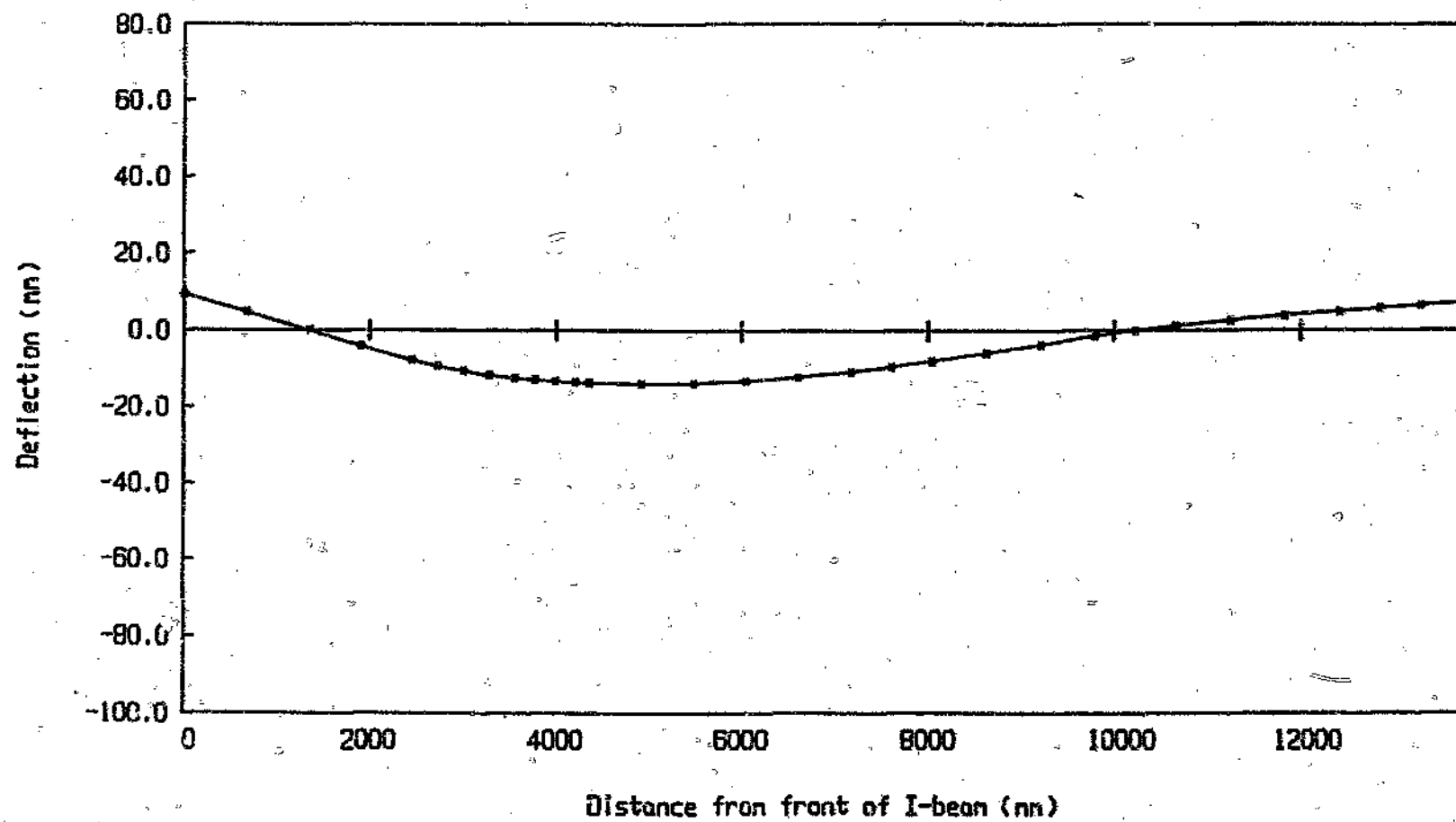
Graph 4.16 Deflection diagram for main chassis I-beam (Case 5 loading)
