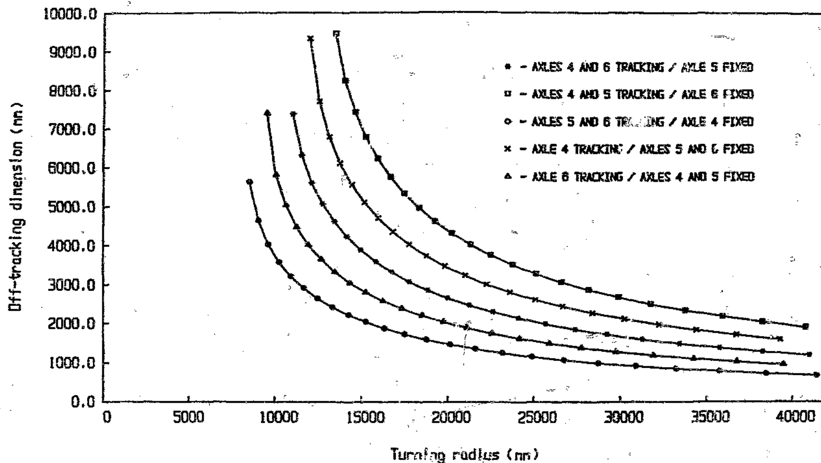
Graph 4.41 Turning radius versus off-tracking dimension for various semi-trailer steering configurations
