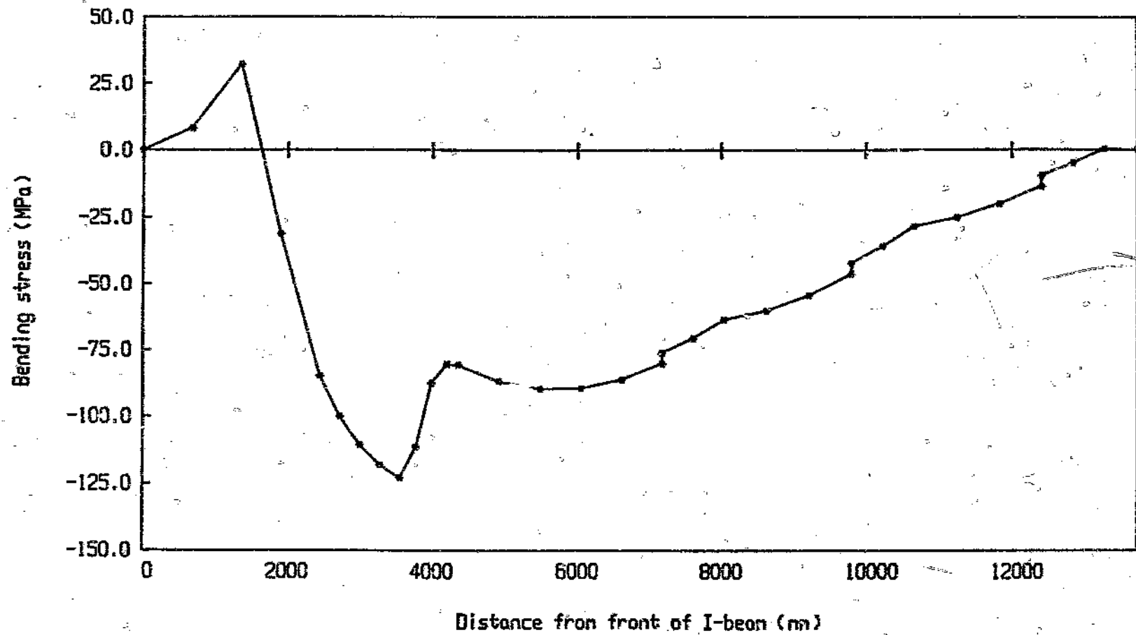
Graph 4.25 Extreme fibre bending stress distribution (Upper flange - Case 1 loading)
