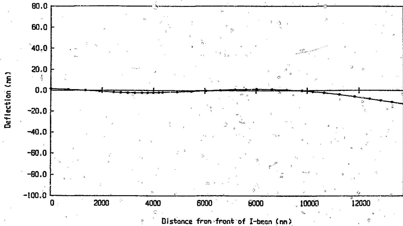
Graph 4.22 Deflection diagram for main chassis I-beam (Case 7 loading)
