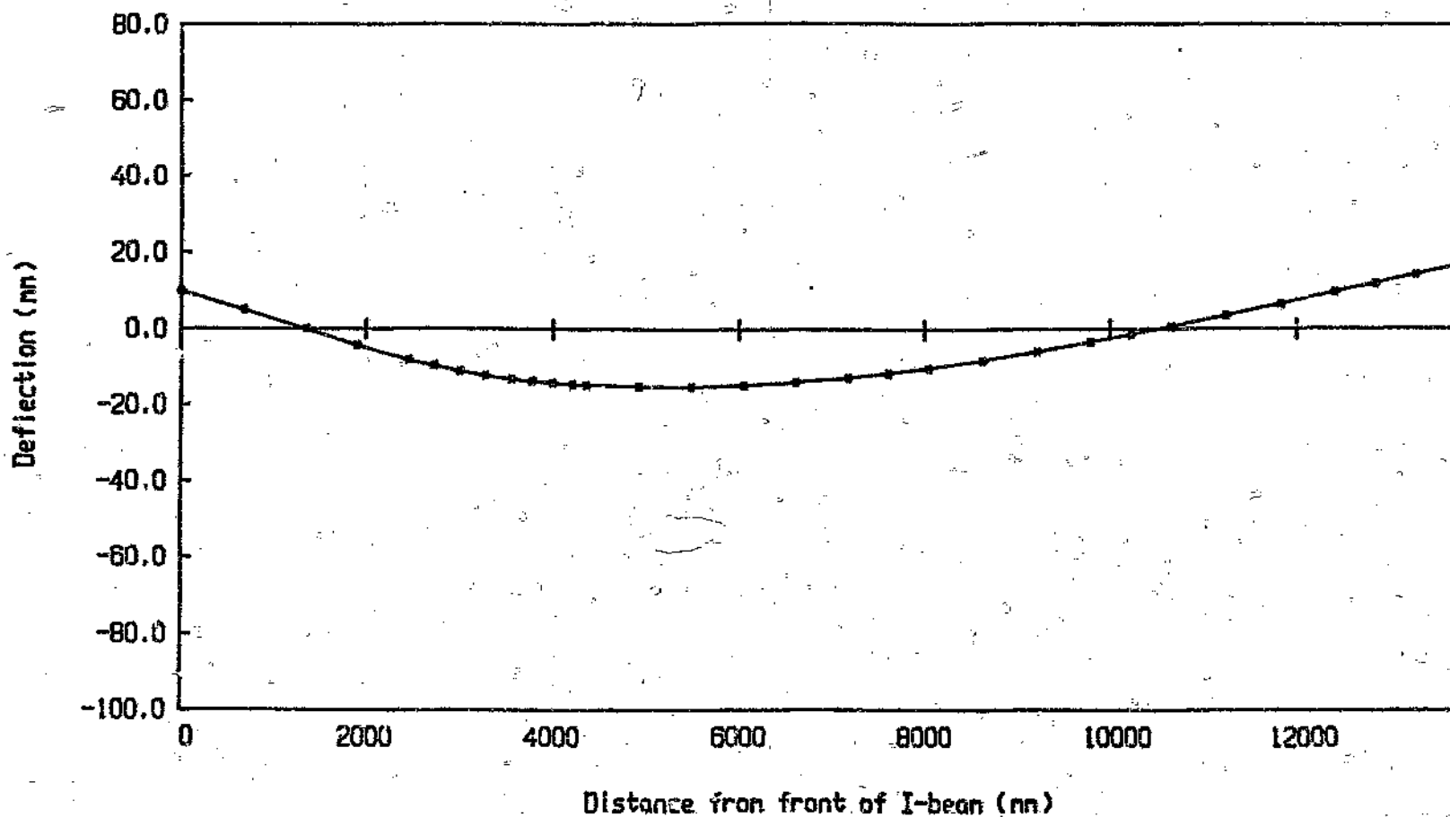
Graph 4.7 Deflection Diagram for main chassis I-beam (Case 2 loading)
