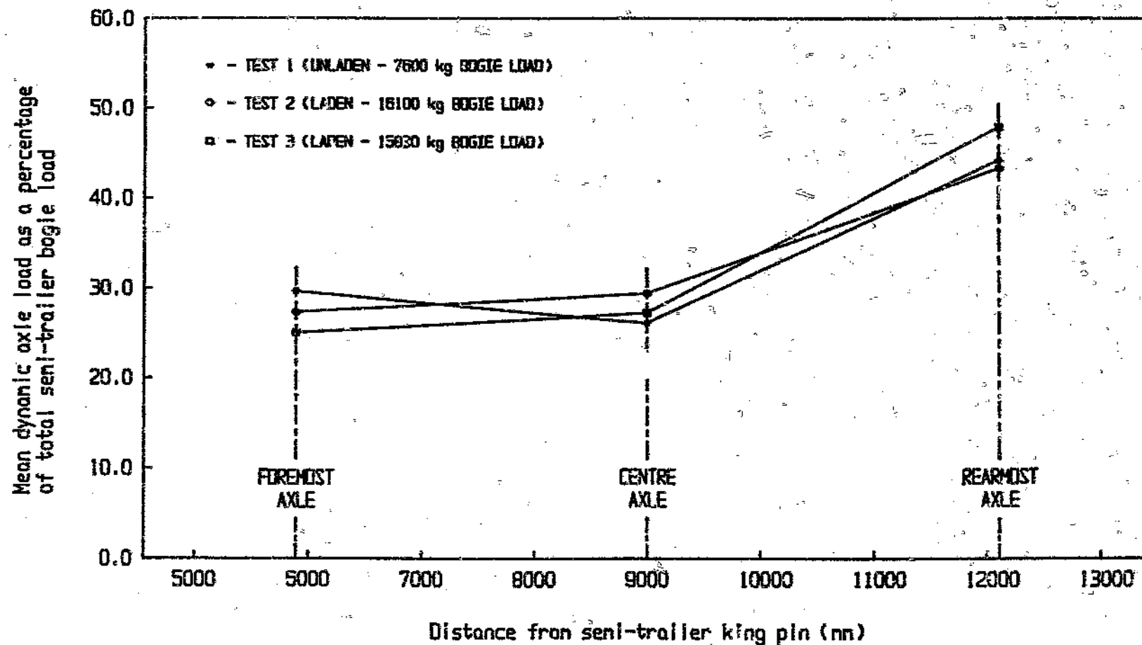
Graph 3.1 Mean dynamic axle loads recorded during the suspension equalization testing of the Henred Fruehauf PET trailer (Freeway at approx. 75 km/h)
