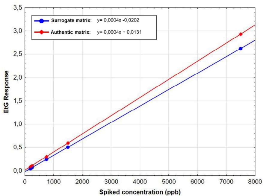
Figure 5.5: The established calibration curves of EtG in surrogate matrix (blue) and authentic matrix (red).
