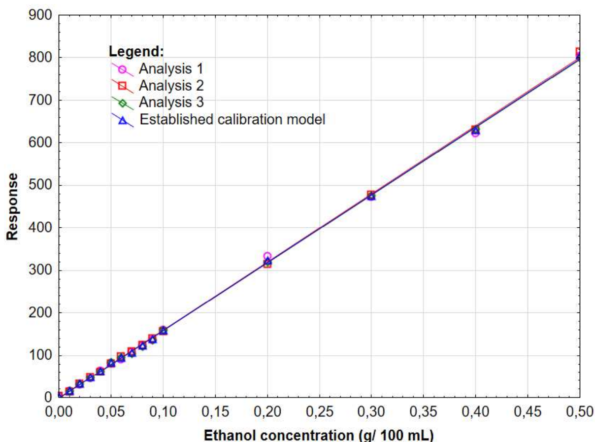
Figure 5.1: A scatterplot illustrating the calibration curves of the three different analytical runs as well as the established calibration model ( r = 0.9996 , y = 1597.9817x - 1.3815 ).
