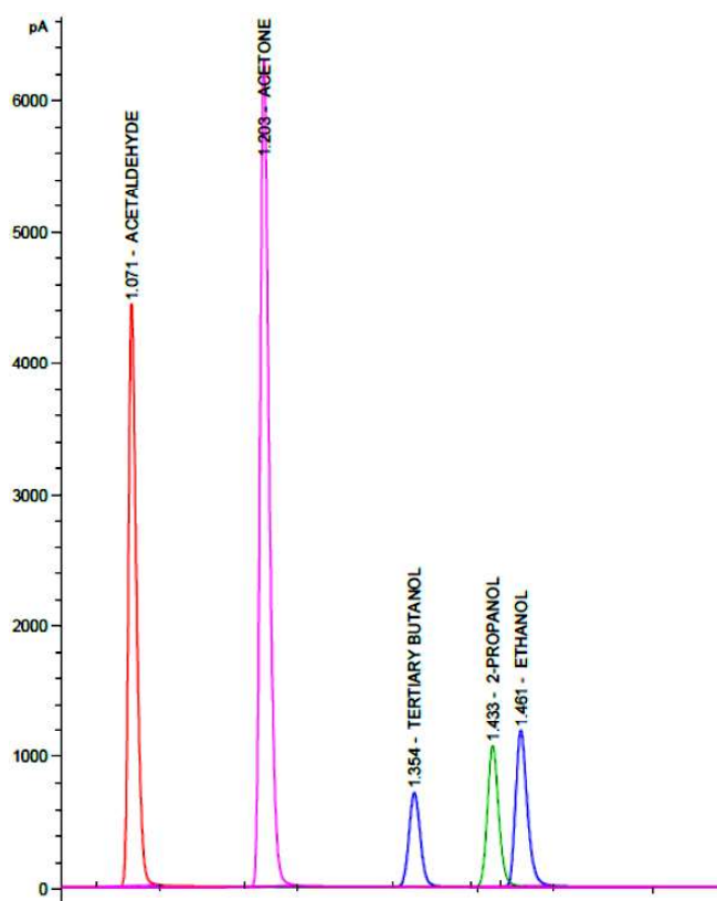
Figure 5.2: A GC-FID chromatogram showing the retention times of acetaldehyde, acetone, tertiary butanol, 2-propanol and ethanol.
