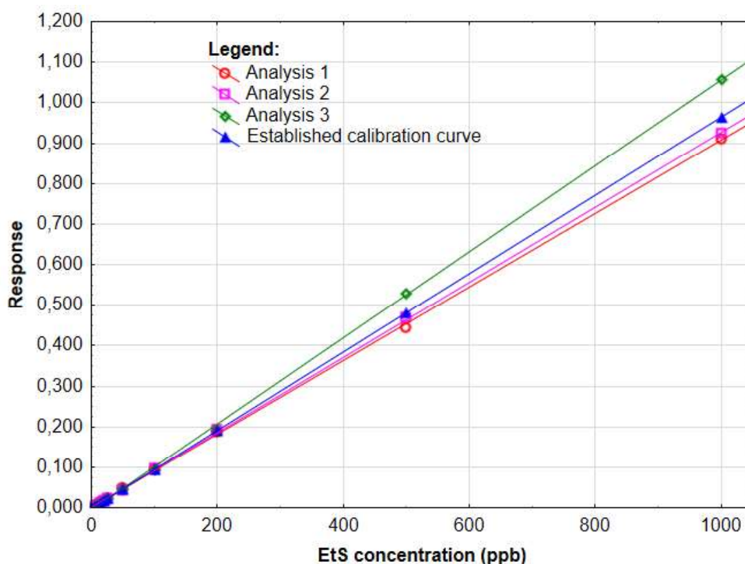
Figure 5.8: A scatterplot illustrating the calibration curves of three different analytical runs as well as the established calibration model for EtS ( r = 0.9999 , y = 0.001x - 0.0017 ) ( n=3 ).
