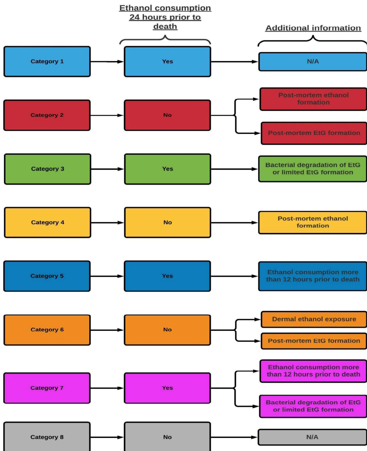
Figure 4.4: A flow diagram describing the process of determining ethanol intoxication 24 hours prior to death, distinguishing between ethanol consumption and post-mortem ethanol formation as well as to determine false positive and false negative results
