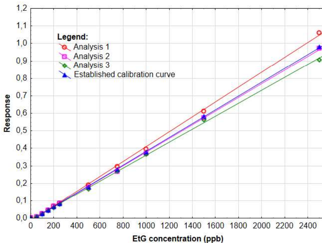
Figure 5.7: A scatterplot illustrating the calibration curves of three different analytical runs as well as the established calibration model for EtG ( r = 0.9998 , y = 0.004x - 0.0128 ) ( n=3 ).
