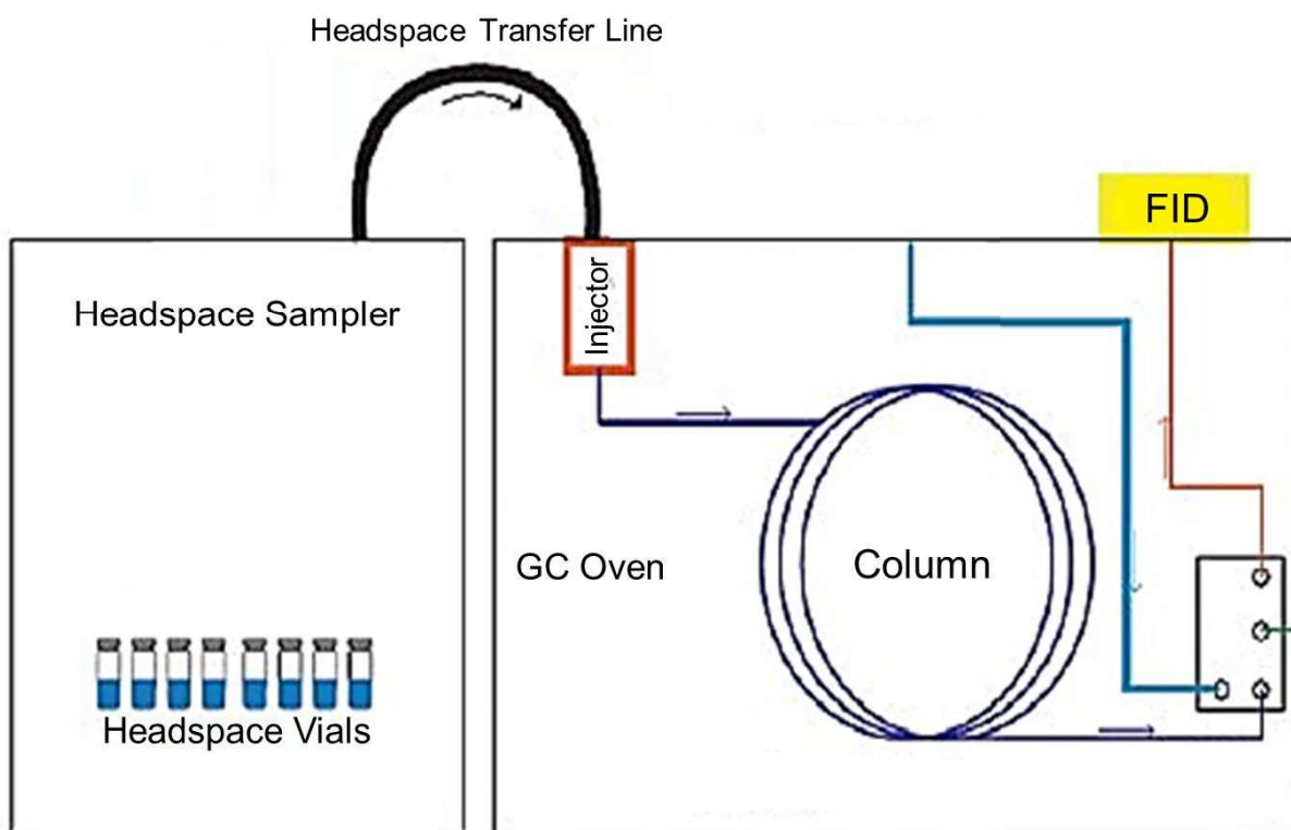
Figure 2.3: HSGC-FID instrument configuration. Figure adapted from (Jacq et al. , 2008)
