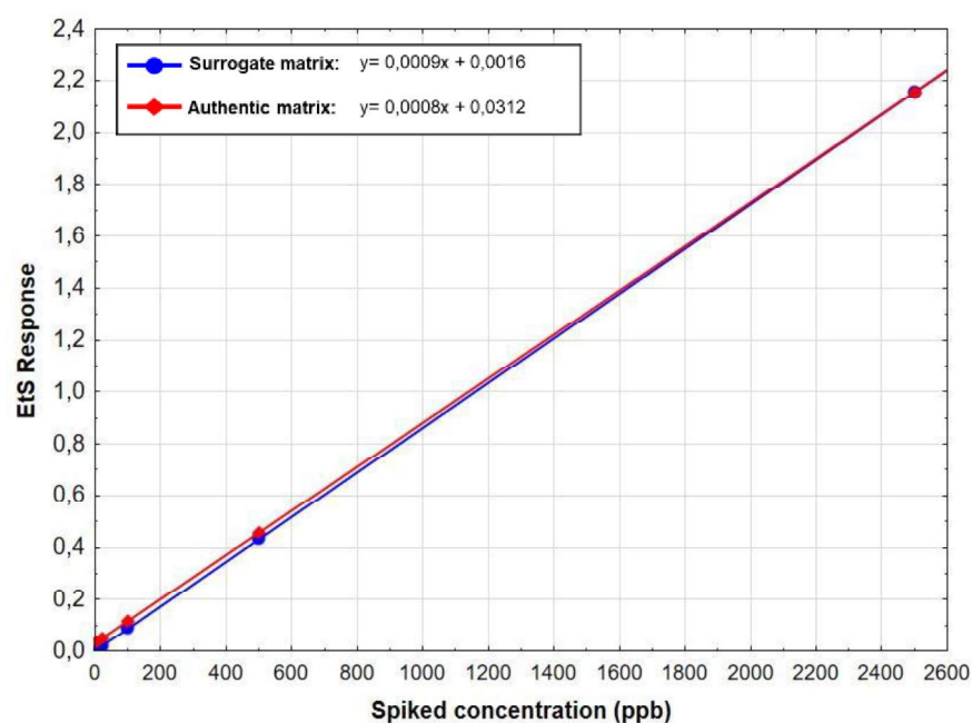
Figure 5.6: The established calibration curves of EtS in surrogate matrix (blue) and authentic matrix (red).
