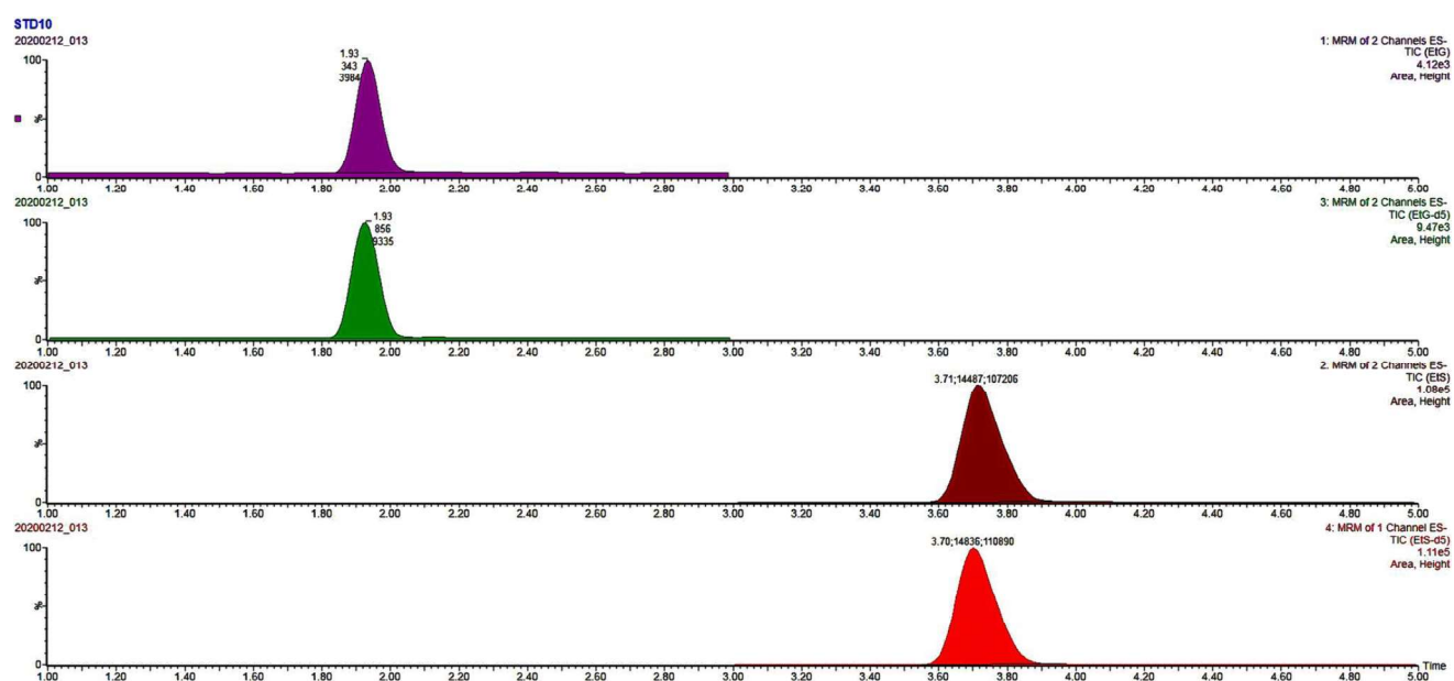
Figure 5.3: A chromatogram indicating the retention times of neat EtG, EtS, EtG-d5 and EtS-d5 standards at a concentration of 5000 ppb.
