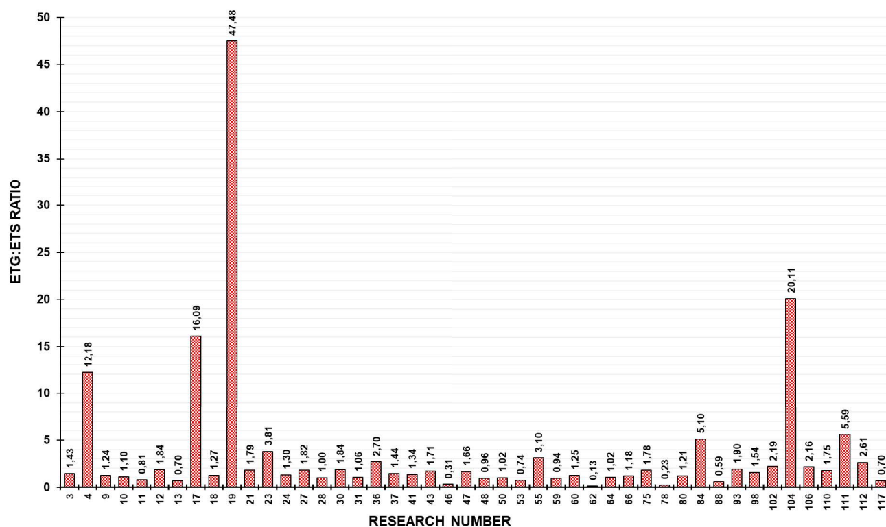
Figure 5.10: A bar graph illustrating the EtG:EtS ratio of the 46 samples positive for both EtG and EtS
