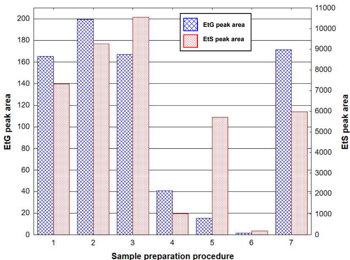
Figure 5.4: The peak area of EtG (left y-axis) and EtS (right y-axis) obtained after performing the various sample preparation procedures on blank vitreous humour samples spiked to a EtG and EtS concentration of 1000 ppb (n=3).
