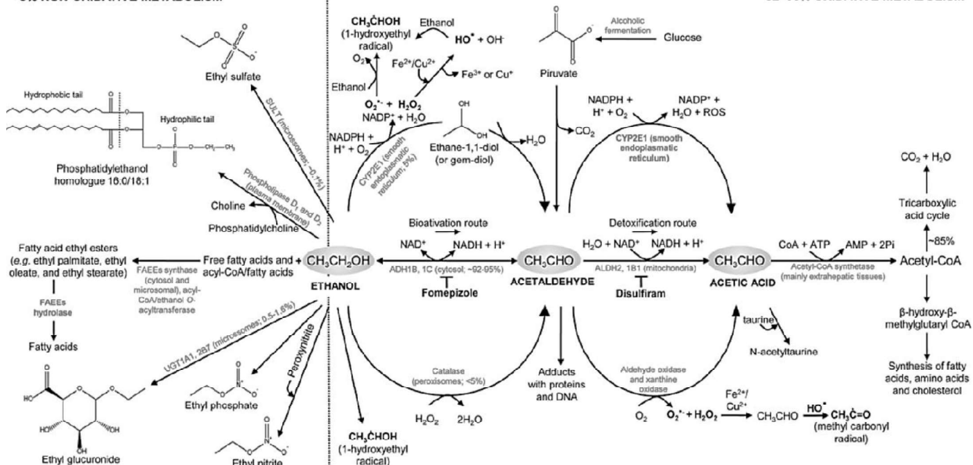
Figure 2.2: The oxidative and non-oxidative metabolism of ethanol. Adapted from (Dinis-Oliveira, 2016), with permission.
