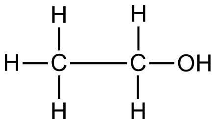
Figure 2.1: The chemical structure of Ethanol (CH 3 CH 2 OH) (Wade, 2019)
