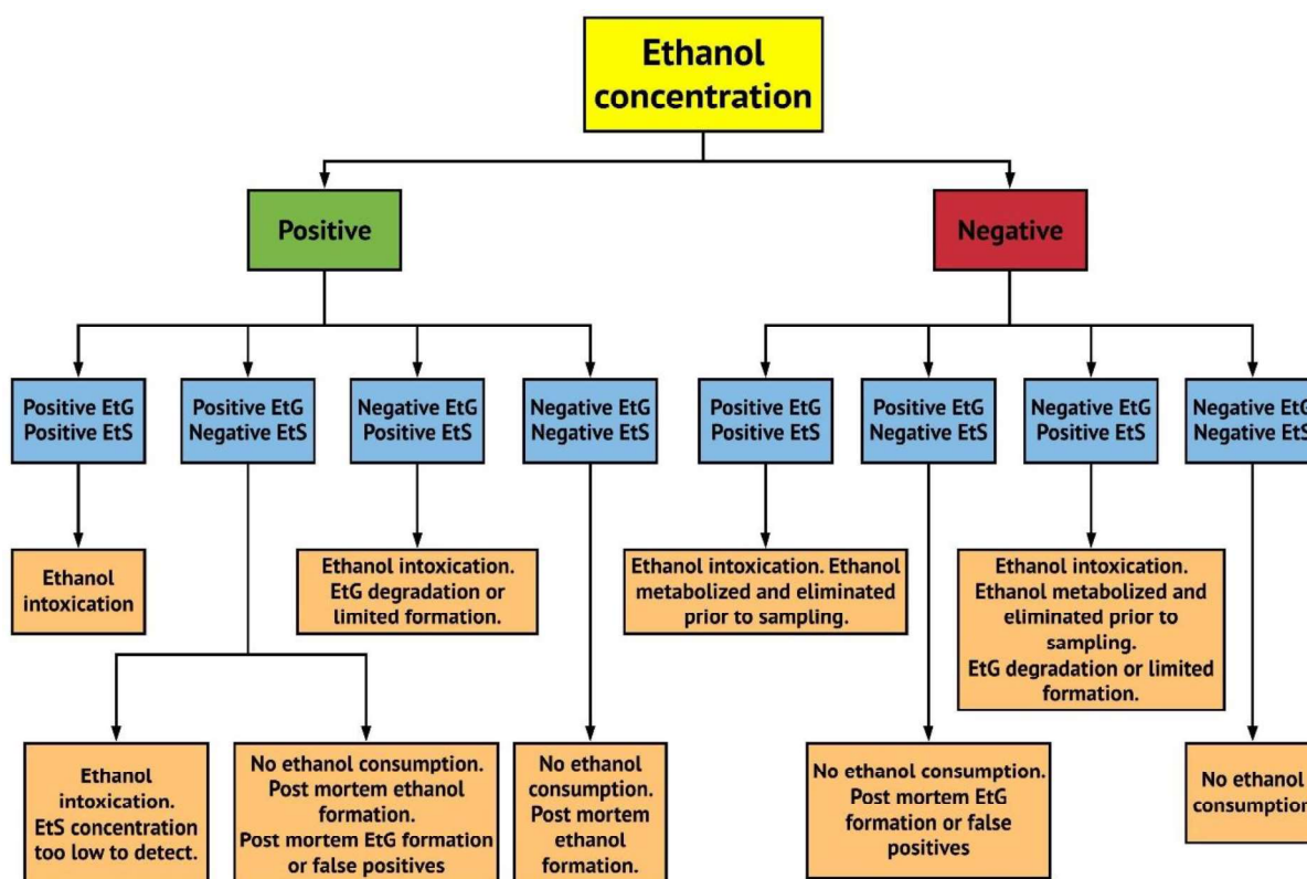
Figure 2.5: A summary of the interpretation of ethanol intoxication using BEC, EtG and EtS results. Information obtained and summarised from (Høiseth et al. , 2007, Armer et al. , 2016, Lostia et al. , 2013, Rainio et al. , 2013).
