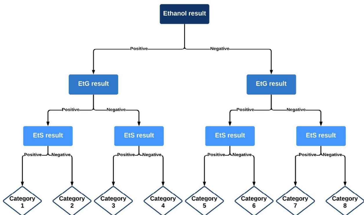
Figure 4.3: The process used to categorize the decedents according to the ethanol, EtG and EtS results of their VH samples
