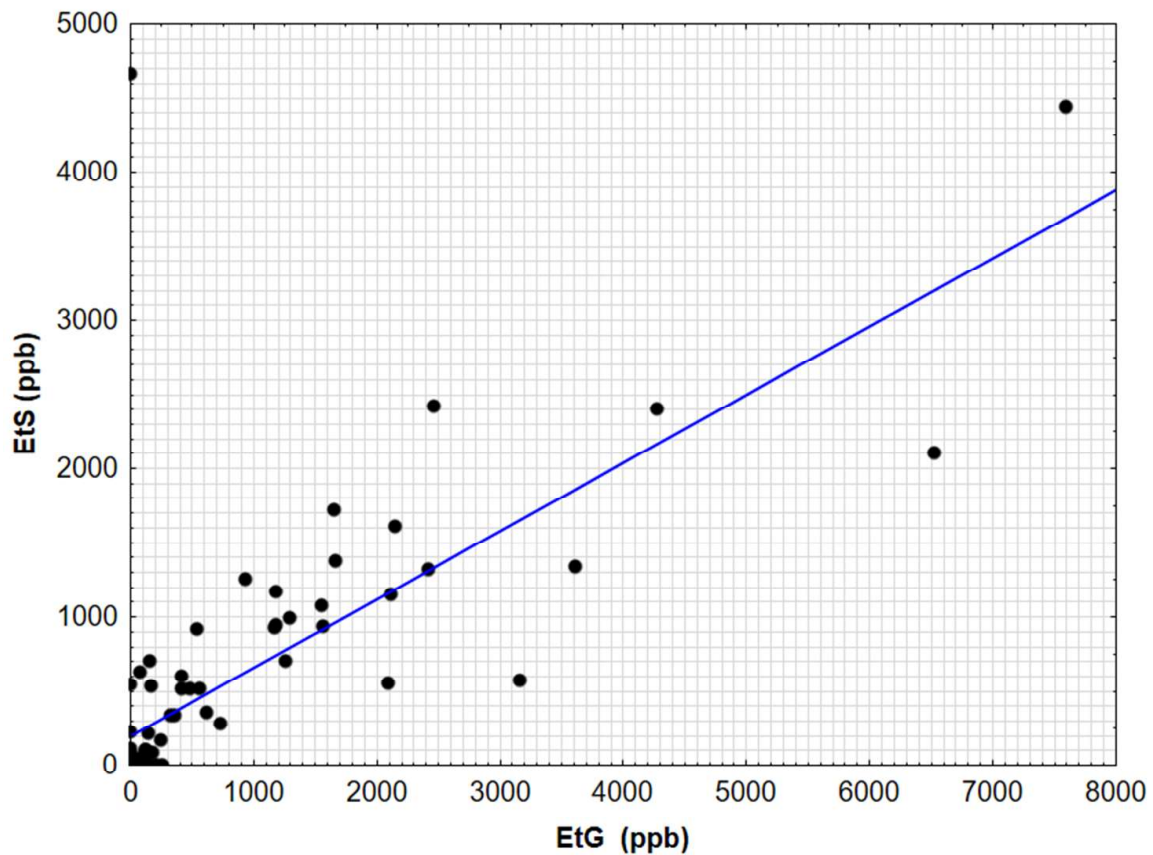
Figure 5.9: A scatterplot of the EtG and EtS concentrations of the 79 positive samples (y = 0.461x + 194.560; r = 0.718; r^2 = 0.516; p < 0.05)
