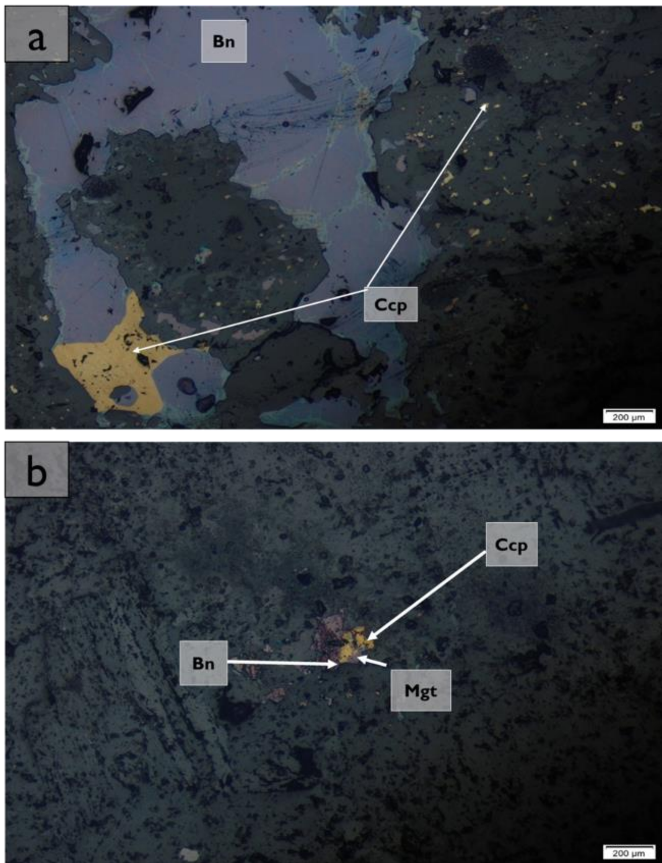
Figure 82: Photomicrographs of the Henderson South matrix: (a) Large chalcopyrite grains that are replaced by bornite. These are adjacent to smaller chalcopyrite and bornite grains. (b) Smaller chalcopyrite replaced by bornite.
