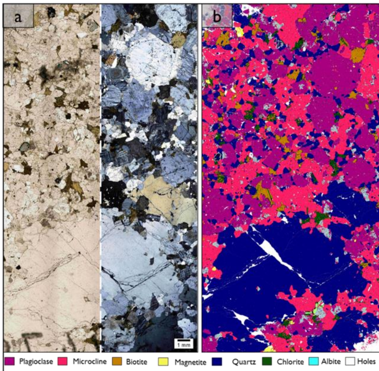
Figure 17: Full thin section photomicrographs of the Diana's Pool matrix: (a) Plane-polarized (left) and cross-polarized light (right) full thin section images of sample BM14780A. (b) TIMA image of the Diana's Pool orbicule sample BM14780A showing a coarse-grained to pegmatitic and granitic matrix comprising feldspars, quartz, biotite and chlorite as predominant phases.
