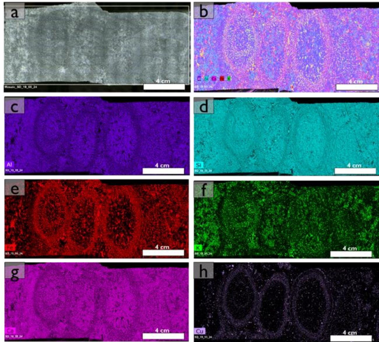
Figure 75: Element maps of Henderson South sample SD-55-24: (a) A mosaic showing the mapped area in a white rectangle. (b) A composite of selected element showing elements detected via the normal map spectrum showing Al (purple), Si (blue), Ca (pink), Fe (red) and K (light green). (c) Element map showing uniform distribution of Al throughout the orbicule sample. (d)Element map showing the highest distribution and intensities of Si in the cores and the matrix. (e) Element map showing the highest distribution and intensities of Fe in shells and matrix. Cores are less ferroan. (f)Element map showing the distribution and concentrations of K in different parts of the orbicules. (g) Uniform Ca distribution throughout the orbicule sample. However, the radiating grains are less sodic (h) Element map showing the distribution and of Cu in different parts of the orbicules. The shells and some parts of the matrix are rich in Cu, and Cu yields the highest intensities in the matrix.
