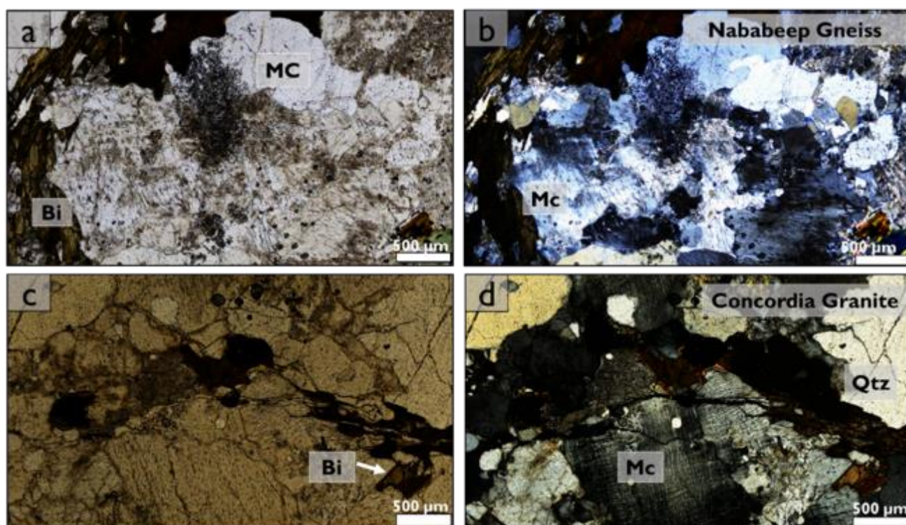
Figure 36: Photomicrographs of samples from Orbicule Koppie and Hoogkraal Lease: (a, b) Photomicrographs of the Nababeep Gneiss showing microcline that exhibits exsolution texture and poikilitic inclusions of magnetite. (c, d) Photomicrographs of the Concordia Granite from Hoogkraal Lease showing subhedral grains of quartz occurring adjacent to biotite and microcline. Microcline contains poikilitic inclusions of biotite, opaque minerals and quartz.
