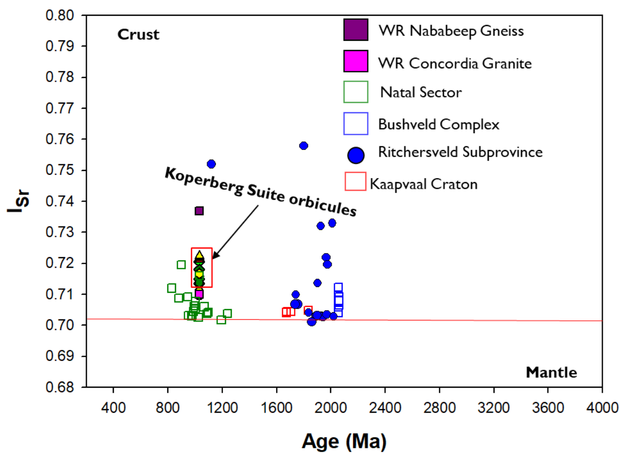
Figure 106: Initial Sr isotope compositions of units from the Koperberg Suite orbicules, Namaqua-Natal (Eglington et al., 1989), Bushveld Complex (Hayes et al., 2018; Scoon et al., 2020; Bourdeau et al., 2022), Richtersveld Subprovince (Reid, 1977; 1979; 1991; 1997) , and the Kaapvaal Craton (Donnelly et al., 2012) relative to the model depleted mantle Eglington, 2006).
