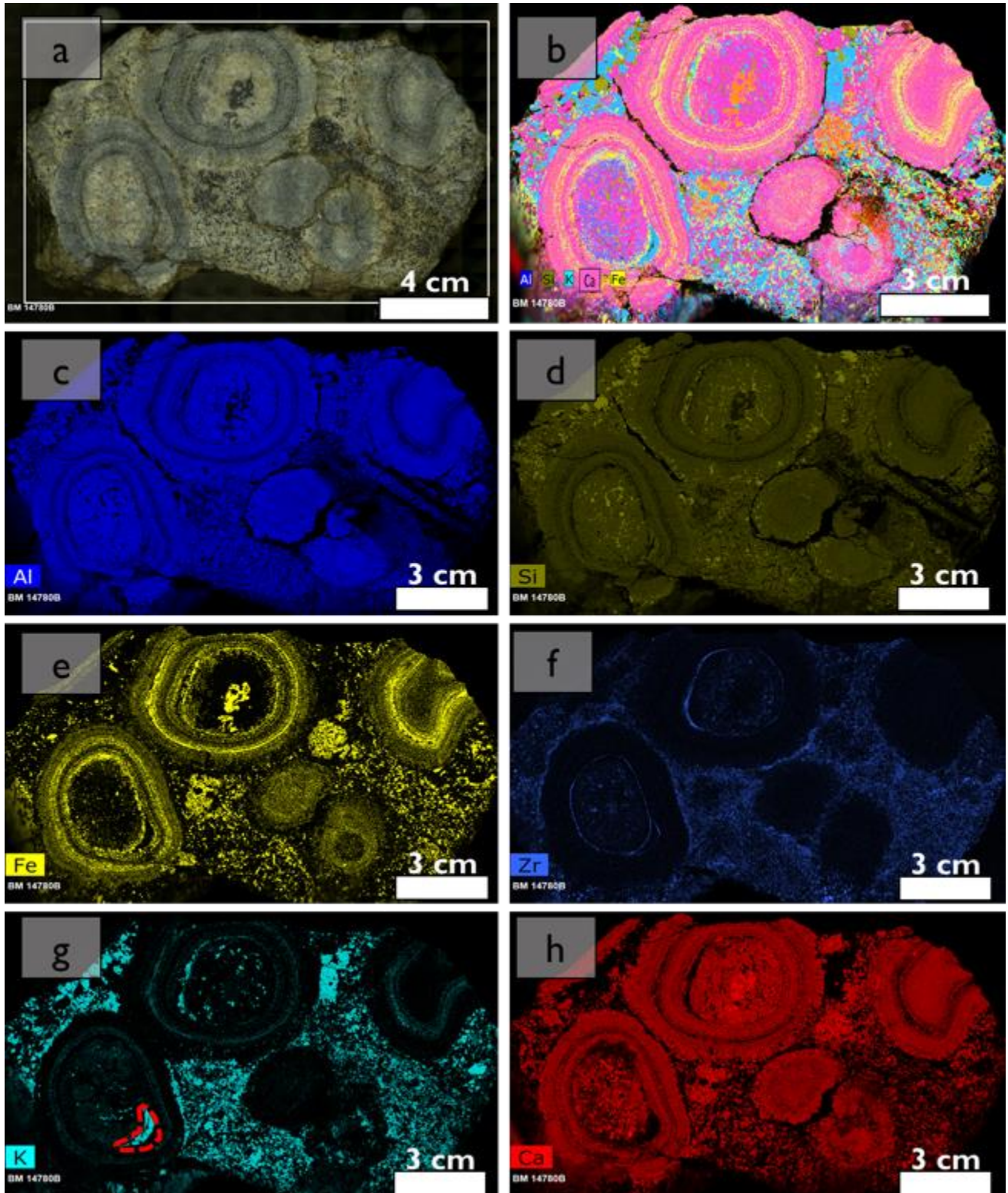
Figure 9: Element maps of the Diana's Pool sample BM 14780B: (a) A mosaic showing the mapped area in white rectangle. (b) A composite of selected elements (Al-dark blue, Si-green, Ca-pink, Fe-yellow and K-light blue) and their distribution shown in a full orbicule sample. (c) Element map showing uniform distribution of Al throughout the sample. However, the dark patches in central cores and some places in shells and matrices do not contain Al. (d) Element map showing uniform distribution of Si in cores and the matrix however, high intensities of Si are observed in the pegmatitic matrix. (e) Element map showing high distribution and intensities of Fe in shells, matrix and some parts of the cores. (f) Element map showing the distribution and concentrations of Zr in different parts of the orbicules. (g) Element map showing the highest concentrations and intensities of K in the matrix, the granitic matrix between the shells (red-dotted area), and some parts of the cores. (h) Element map showing the distribution and concentrations of Ca in different parts of the orbicules.
