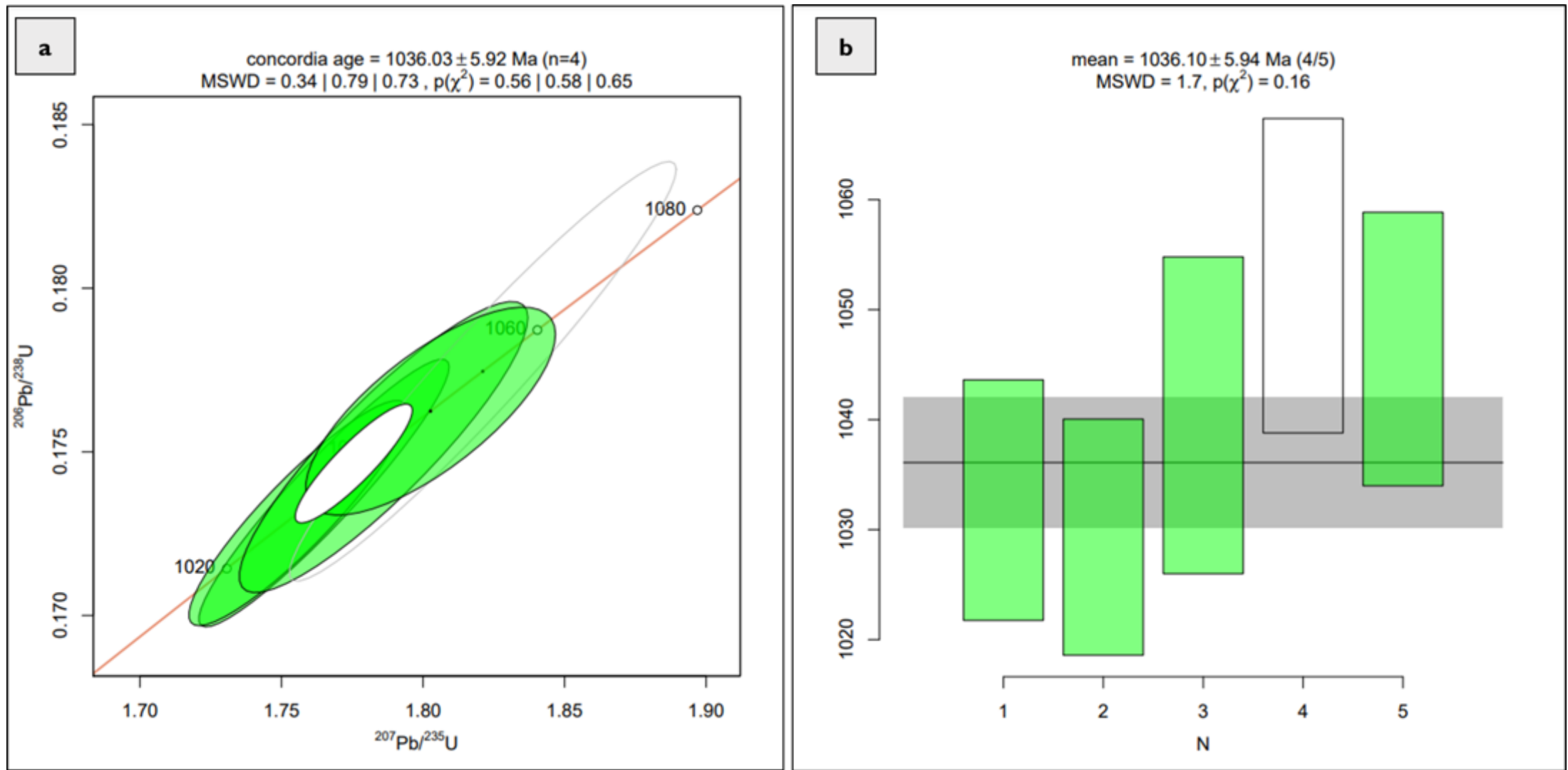
Figure 108: Representative U-Pb geochronology results of zircon (reported to 1\sigma ): (a) Wetherill U-Pb concordia diagram for zircon from Orbicule Koppie matrix sample SD-10-6C. Rejected data are shown in white (outliers and >10\% discordance). (b) Weighted mean diagram showing ^{207}\text{Pb}/^{206}\text{Pb} age of zircon from sample SD-10-6C ( <10\% discordance).
