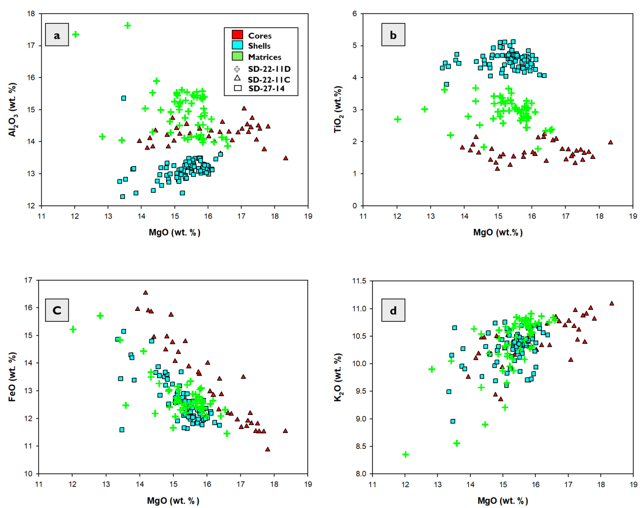
Figure 94: In-situ chemical variation diagrams showing the variation of different oxides in biotite from Hoogkraal Lease orbicular cores, shells, and matrix plotted against MgO (wt. %).
