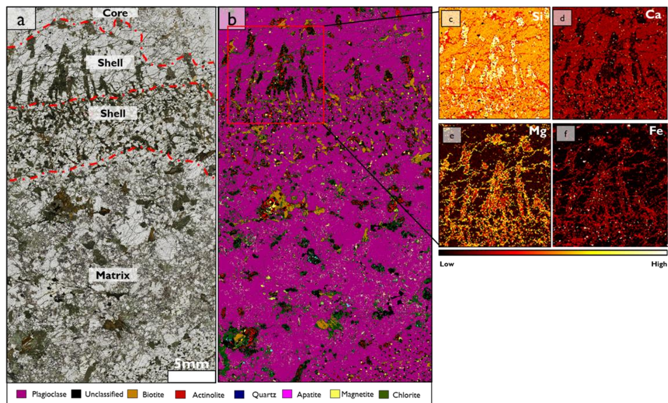
Figure 76: Full thin section photomicrographs of the Henderson South orbicule sample SD-55-24B and the corresponding TIMA images: (a) Plane-polarized full thin section images of sample SD-55-24B. (b) TIMA image of the sample showing a medium-grained core that is composed of plagioclase, quartz and unclassified radiating grains (black). (c) TIMA image of the selected area (red box in image b) showing that the radiating grains have high silica than the surrounding feldspars. (d) TIMA image of the selected area showing that the radiating grains have no calcium and the calcium content in the grains is lower than in the surrounding feldspars. (e, f) TIMA images of the selected area showing that the radiating grains are enriched in iron and magnesium relative to the surrounding calcic plagioclase.
