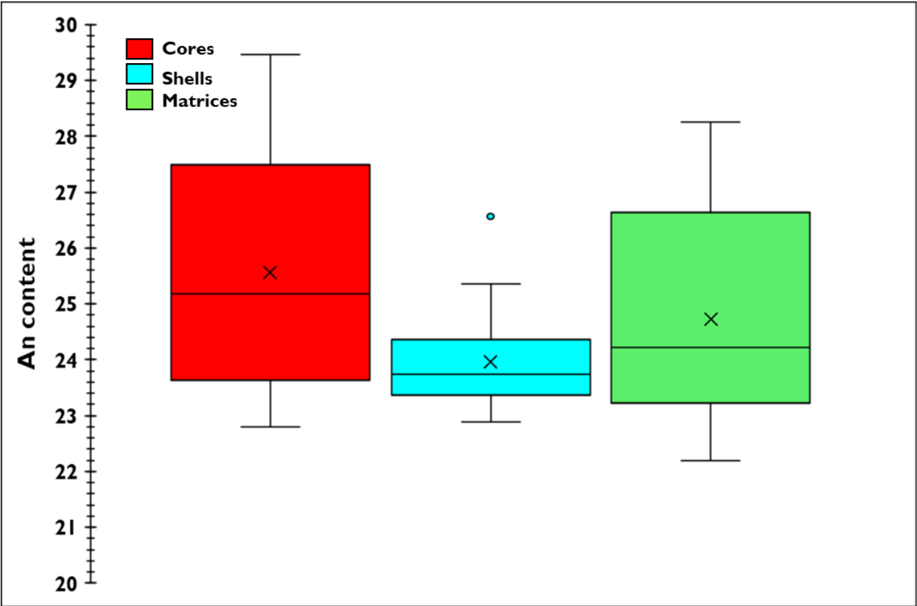
Figure 21: The graph showing the An content in plagioclase from Diana’s Pool orbicular core, shells and matrix from orbicule sample BM14780F (representative of a full orbicule with a core, shells and a matrix). The graph shows little variation in the An contents in the core and matrix, however, the shells have slightly low An contents. The two sigma represent the minimum and maximum values, the box represents the interquartile range, x represents the mean, and the middle straight line represents the median.
