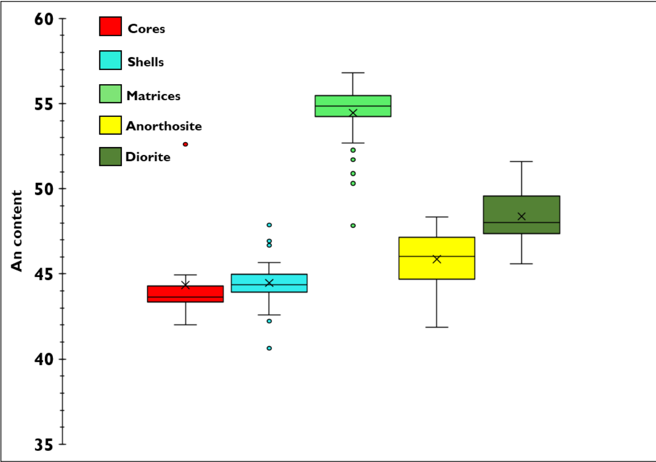
Figure 89: The graph of An content showing a variation in An content in the Orbicule Koppie orbicular core, shells, matrix and the surrounding anorthosite and diorite. Plagioclase in the matrix are more calcic and thus high An contents than plagioclase in the core, shells, diorite and anorthosite. The two sigma represent the minimum and maximum values, the box represents the interquartile range, x represents the mean, and the middle straight line represents the median.
