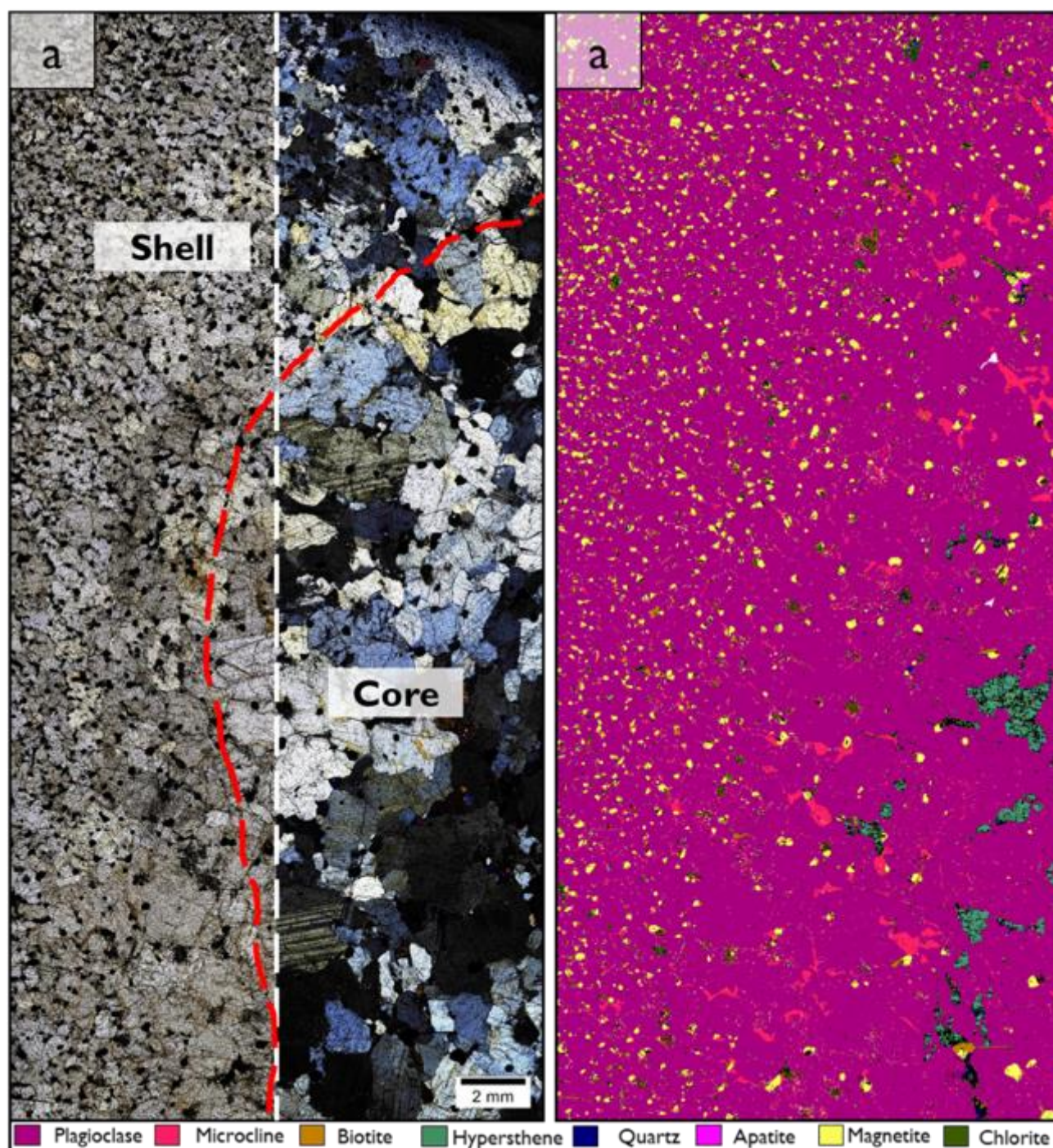
Figure 67: Full thin section photomicrographs of the Henderson North orbicule sample SD-36-18C and corresponding TIMA image: (a) Plane-polarized (left) and cross-polarized light (right) full thin section images of sample SD-36-18C. (b) TIMA image of sample SD-36-18C. (b) TIMA image of sample SD-36-18C showing a medium- to coarse-grained core composed of plagioclase, hypersthene, microcline and magnetite. The red-dotted line marks the gradational contact between the core and the shell. There is a visible increase in magnetite and a decrease in microcline modal abundance in the shell.
