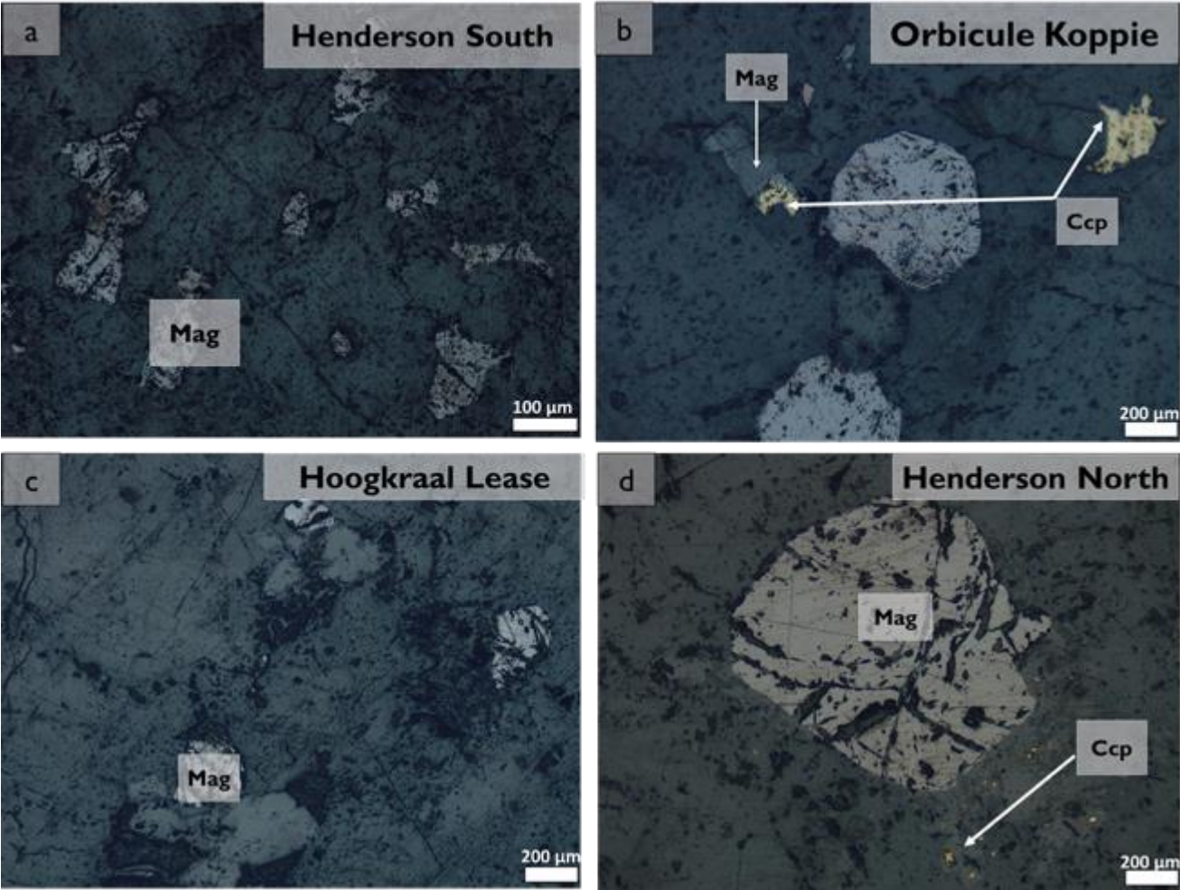
Figure 41: Photomicrographs showing the sulphide mineralization and magnetite in diorites from the Koperberg Suite: (a) Disseminated and anhedral to subhedral grains of magnetite in Henderson South diorite. (b) Subhedral grains of magnetite in the Orbicule Koppie diorite adjacent to smaller and disseminated grains of chalcopyrite. Locally, magnetite replaces chalcopyrite. (c) Small and anhedral magnetite in Hoogkraal Lease diorite concentrated in plagioclase. (d) Large magnetite grains adjacent to small and locally concentrated chalcopyrite grains in the Henderson North diorite.
