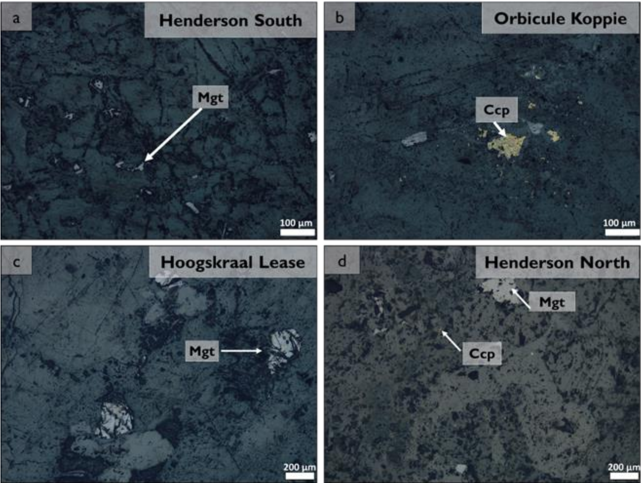
Figure 39: Photomicrographs showing sulphides and oxides in the Koperberg Suite anorthosites: (a) disseminated magnetite grains in anorthosite from the Henderson South adjacent to each other in plagioclase. (b) Disseminated chalcopyrite occurring adjacent to smaller magnetite grains in Orbicule Koppie anorthosite. (c) Larger magnetite grains from Hoogkraal Lease anorthosite. (d) Magnetite grains adjacent to smaller (< 0.1 mm) grains of disseminated magnetite in anorthosite from Henderson North.
