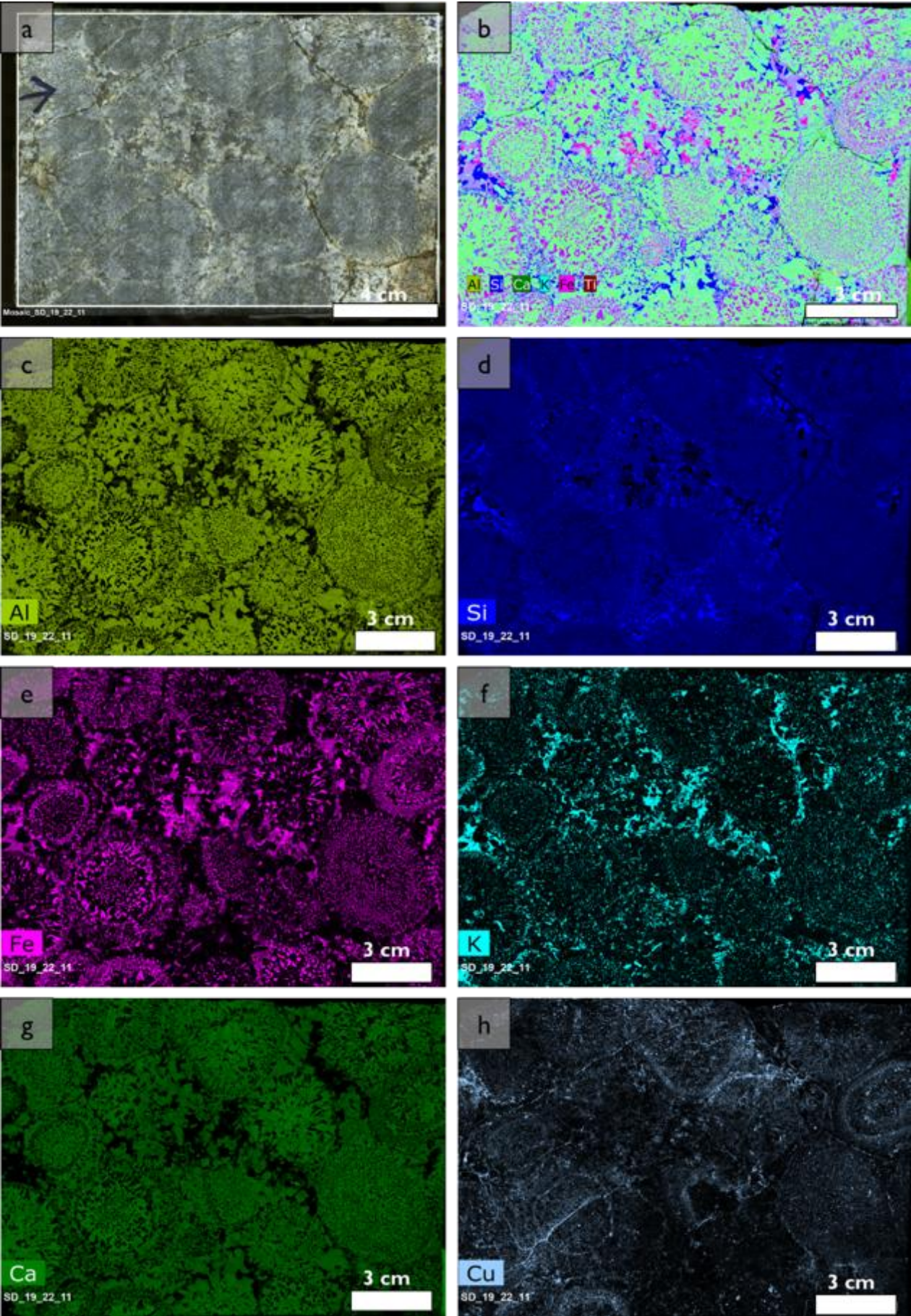
Figure 53: Element maps of Hoogkraal Lease sample SD-22-11: (a) A mosaic showing the mapped area in a white rectangle. (b) A composite of selected element showing elements detected via the normal map spectrum showing the distribution of Al (green), Si (blue), Fe (pink), Ti (red) and Ca (green) in the sample.
