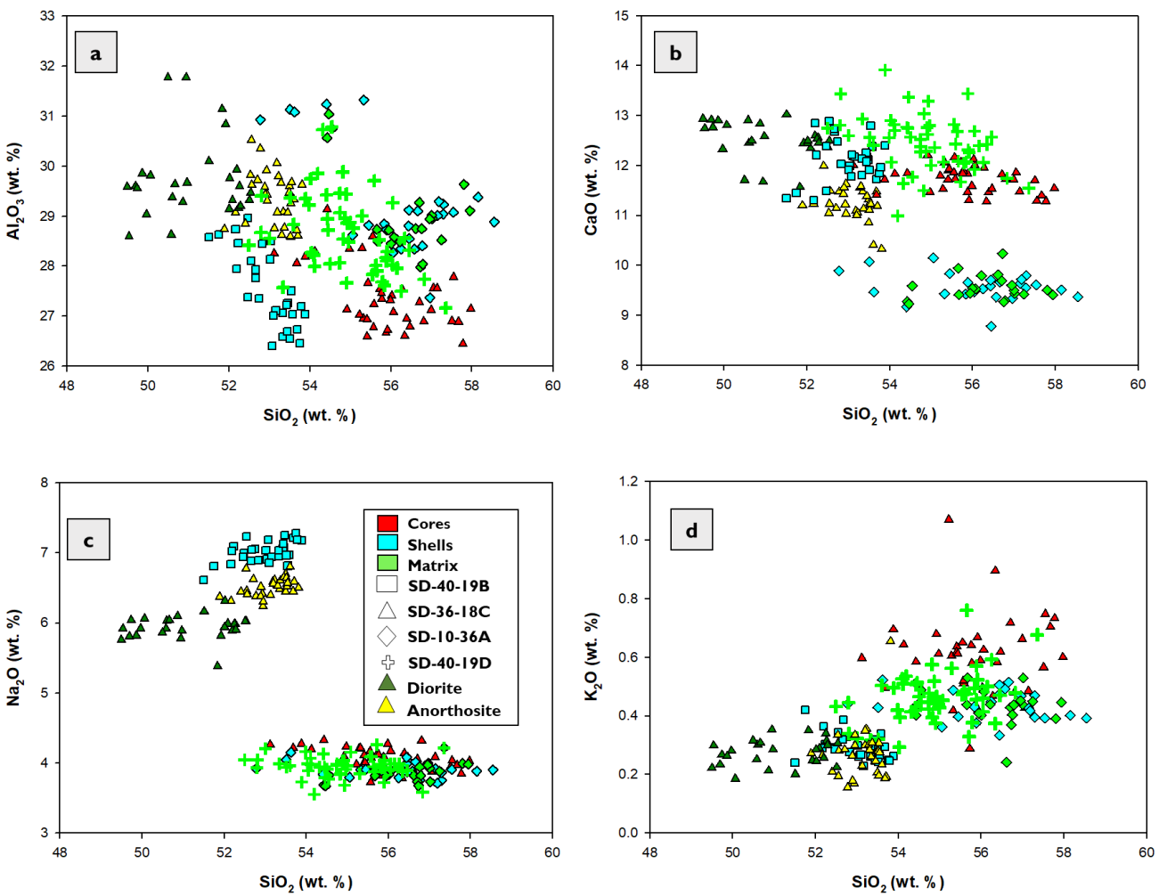
Figure 96: Chemical variation diagrams showing variation of different oxides in plagioclase from the Henderson North orbicular domains, diorite, and anorthosite plotted against SiO 2 (wt. %).
