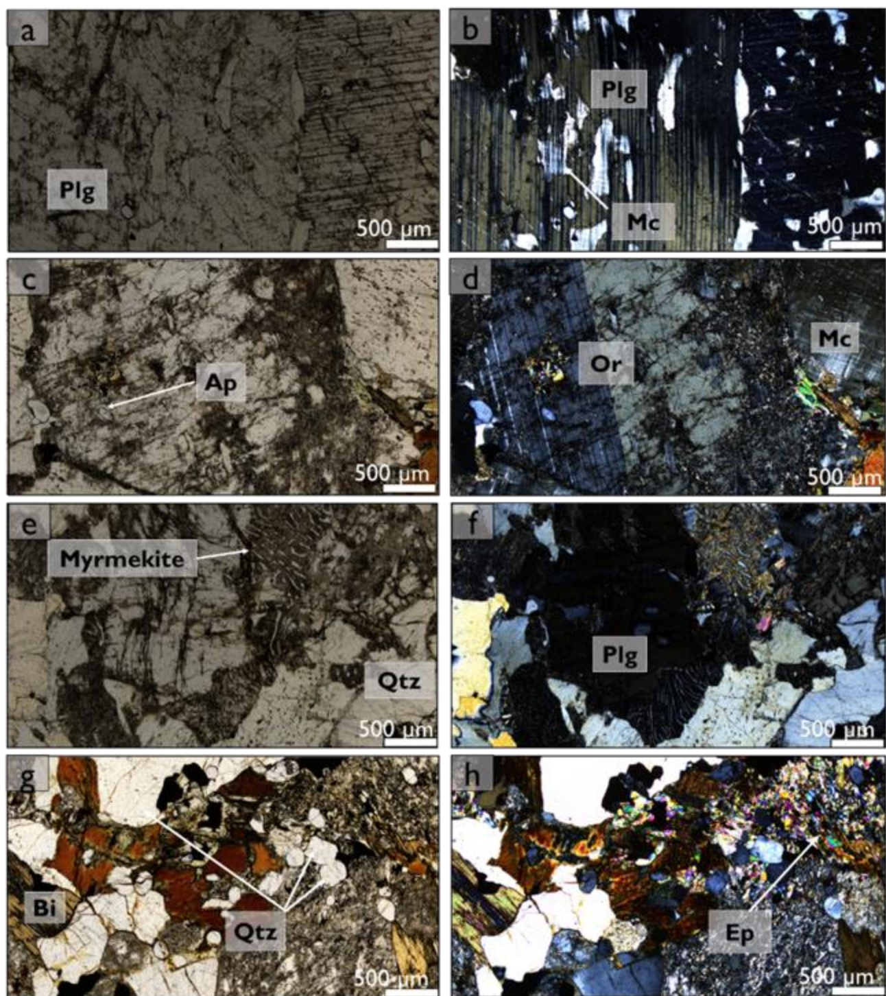
Figure 51: Photomicrographs showing mineral phases and textures in Orbicule Koppie matrix: (a, b) Large plagioclase grains containing inclusions of microcline lamellae that follows the orientation of the albite twinning (antiperthite). (c, d) Plagioclase altered to sericite occurring adjacent to microcline and orthoclase. Orthoclase contains small inclusions of apatite, and it is altered to clay. Biotite occurs adjacent to epidote and they both occur as small inclusions in altered plagioclase. (e, f) Anhydrous quartz grains occurring adjacent to plagioclase. Locally, quartz occurs as vermicular intergrowths in plagioclase (myrmekite texture). Small muscovite grains occur adjacent to quartz and the altered to plagioclase. (g, h) Anhydrous to subhedral quartz grains containing biotite inclusions. Quartz grains occur next to biotite and altered plagioclase. Locally, biotite is altered to chlorite.
