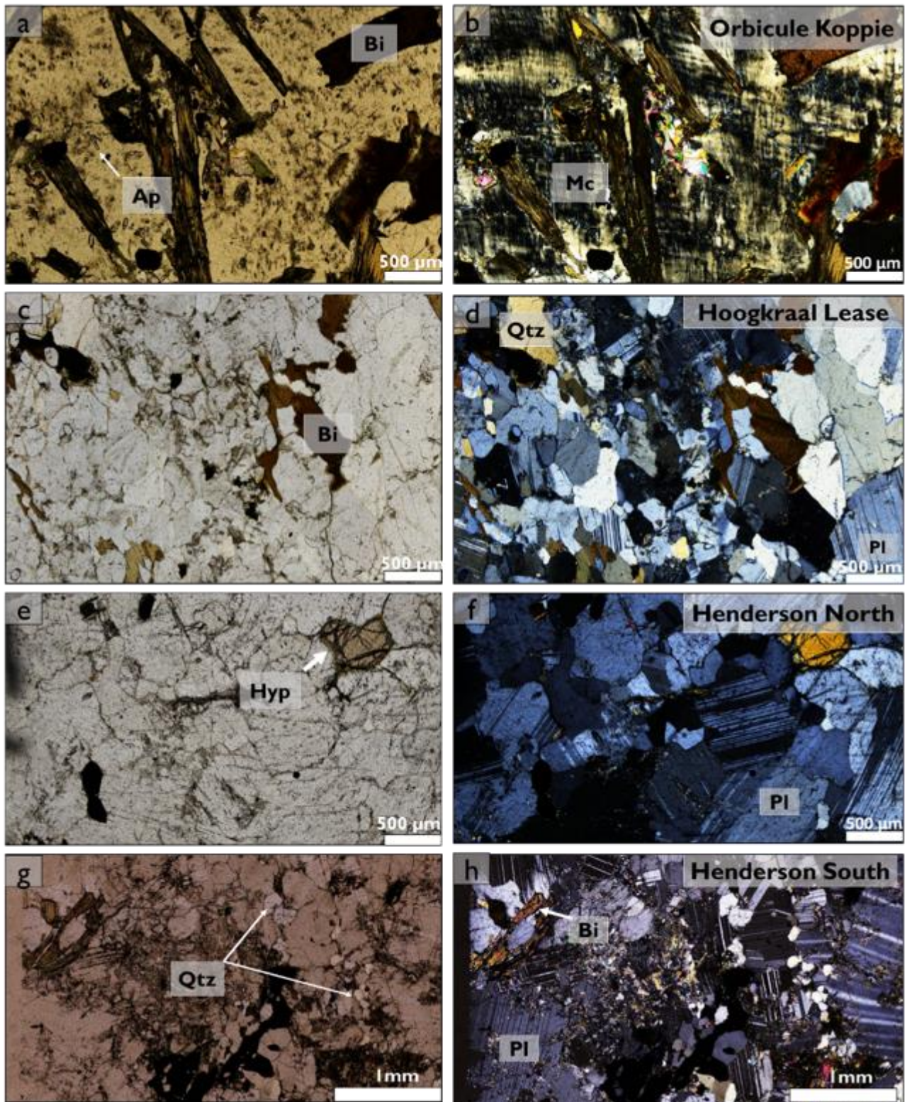
Figure 40: Photomicrographs of diorites from Koperberg Suite illustrating quantitative textural analysis: (a, b) Diorite from Orbicule Koppie composed of large microcline grains that contain poikilitic inclusions of anhedral magnetite and elongated (0.1-0.4 mm) grains of biotite. Microcline displays exsolution textures and it is altered to white mica. (c, d) Diorite from Hoogkraal Lease comprising plagioclase, quartz and biotite grains that occur adjacent to each other. Plagioclase occurs as smaller grains that occur adjacent to quartz and exhibit discontinuous twinning. Locally, plagioclase is surrounded by interstitial biotite. (e, f) Diorite from Henderson North containing small and disseminated hypersthene grains adjacent to plagioclase. Plagioclase locally exhibits discontinuous twinning and occurs adjacent to small biotite grains. (g, h) Diorite from Henderson South containing both unaltered and altered grains of plagioclase (sericite) that contain poikilitic inclusions of quartz and magnetite. Quartz occurs as anhedral grains that occur adjacent to biotite and plagioclase. Locally, quartz occurs as inclusions in biotite.
