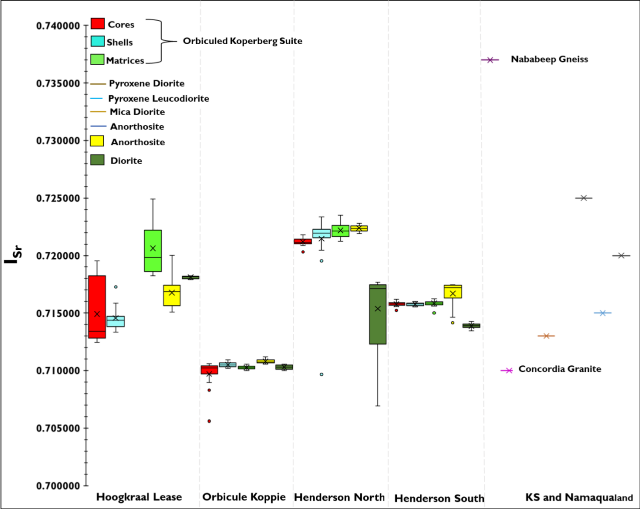
Figure 104: Graph showing a variation in the initial ^{87}\text{Sr}/^{86}\text{Sr} ratios in plagioclase from the Koperberg Suite orbicules and the surrounding Koperberg Suite massive diorites and anorthosite, and the Namaqualand basement rocks. The initial ^{87}\text{Sr}/^{86}\text{Sr} isotopic ratios in orbicules are within range with the initial ^{87}\text{Sr}/^{86}\text{Sr} ratios (adapted from Van Zwieten et al. (1996) of the massive Koperberg Suite and the Namaqualand basement rocks. The two sigma represent the minimum and maximum values, the box represents the interquartile range, x represents the mean, and the middle straight line represents the median.
