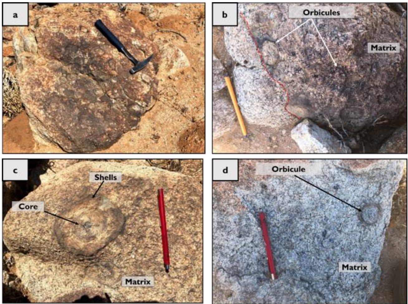
Figure 33: Boulders from the Henderson North orbicular outcrop: (a) A boulder showing spherical orbicules hosted in a coarse-grained pyroxene-bearing diorite. (b) A more coarse-grained pyroxene-bearing diorite characterized by aligned and coarse-grained plagioclase. (c) Orbicule showing alternating mafic and felsic shells lacking the radiating texture. (d) An orbicule hosted in a felsic matrix characterized by a felsic core and mafic shells.
