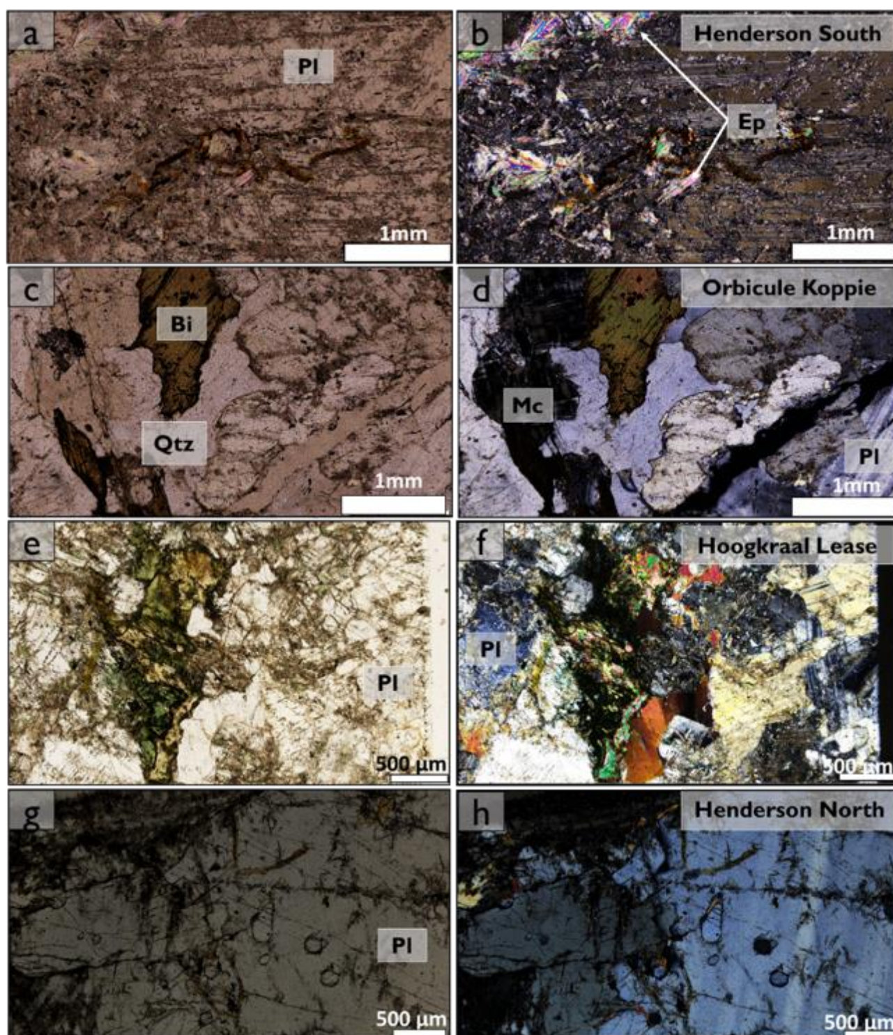
Figure 38: Photomicrographs of anorthosites in contact with the Koperberg Suite orbicules: (a, b) Anorthosite from Henderson South comprising grains of plagioclase that are altered to sericite and comprising poikilitic inclusions of biotite. Microcline and plagioclase are enclosed by interstitial quartz that contains very small inclusions of magnetite. (c, d) Anorthosite from Orbicule Koppie containing grains of microcline, chlorite and plagioclase surrounded by interstitial quartz. Microcline locally exhibits exsolution textures and contains inclusions of magnetite. (e, f) Anorthosite from Hoogkraal Lease comprising plagioclase that exhibits discontinuous twinning and locally altered to sericite. Chloritisation of biotite is observed. (g, h) Anorthosite from Henderson North comprising inclusions of rounded quartz grains in plagioclase. Locally, plagioclase is altered to clay.
