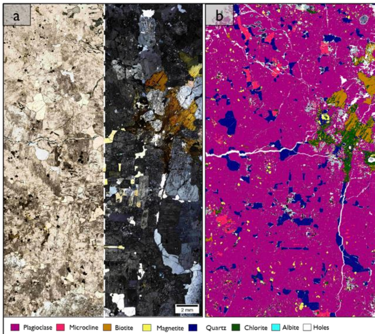
Figure 12: Full thin section photomicrographs and TIMA image of the Diana's Pool orbicular core: (a) Plane-polarized (left) and cross-polarized light (right) full thin section images of sample BM14780D. (b) TIMA image of orbicule sample BM14780D showing a medium-grained core comprising feldspars, quartz, biotite and chlorite.
