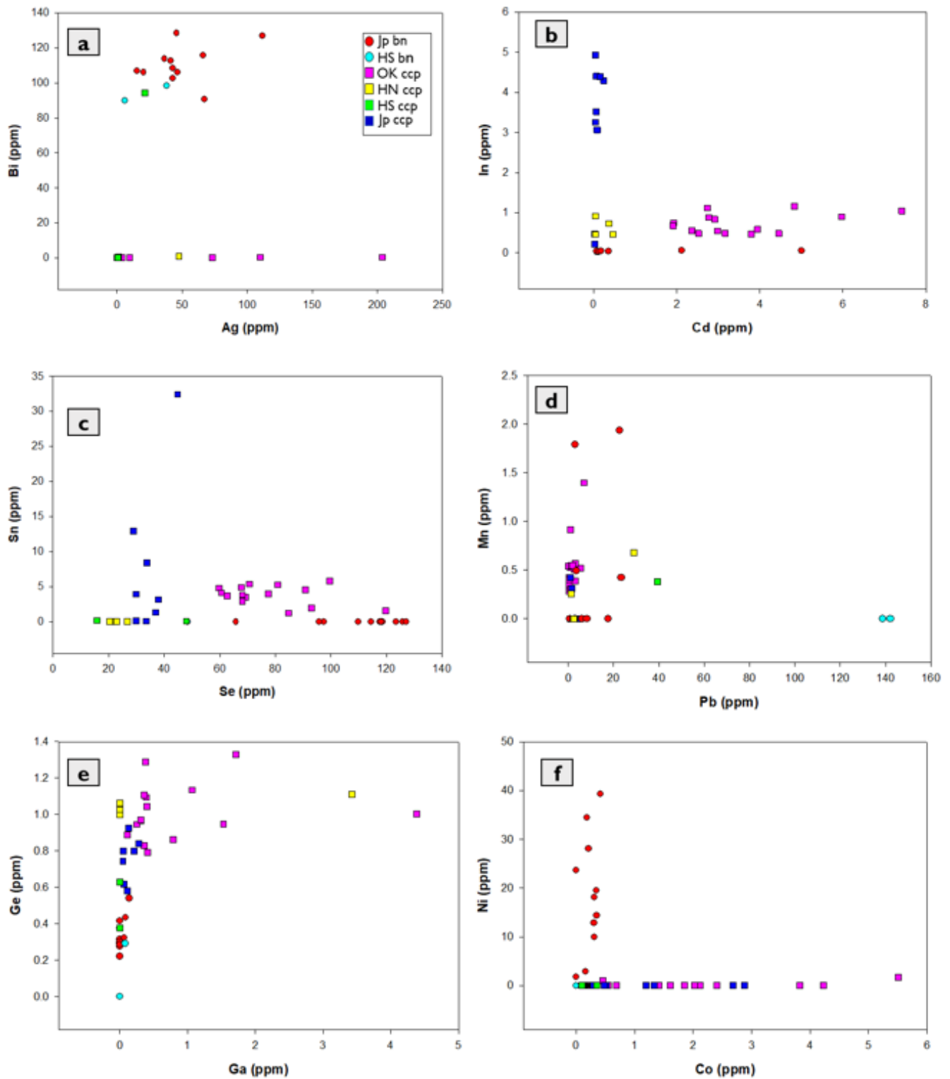
Figure 111: Trace element (ppm) variation diagrams of chalcopyrite (ccp) and bornite (bn) from the Koperberg Suite orbicules: (a) Bi vs Ag diagram showing bornite from different localities enriched in Bi relative to chalcopyrite. Chalcopyrite shows a large variation in Ag. (b) In vs Cd diagram showing that chalcopyrite in the Koperberg Suite is enriched in Cd and depleted in In relative to bornite. (c) Sn vs Se showing that the Koperberg Suite bornite is enriched in Se and depleted in Sn relative to chalcopyrite. (d) Mn vs Pb plot showing high concentrations of Pb and low concentrations of Mn (below detection limit) in the Koperberg Suite bornite. The highest Mn and lowest Pb concentrations are observed in chalcopyrite. (e) Ge vs Ga diagram showing the Koperberg Suite chalcopyrite enriched in Ge relative to bornite. Ga in bornite is below the detection limit (plotted at 0 ppm). (f) Ni in chalcopyrite is below detection limit (plotted at 0); however, the highest concentrations of Ni and lowest concentrations of Co (below the detection limit) are exhibited by the Jubilee Pit bornite. OK=Orbicule Koppie, HS=Henderson South, HN=Henderson North, HL=Hoogkraal Lease and Jp=Jubilee Pit.
