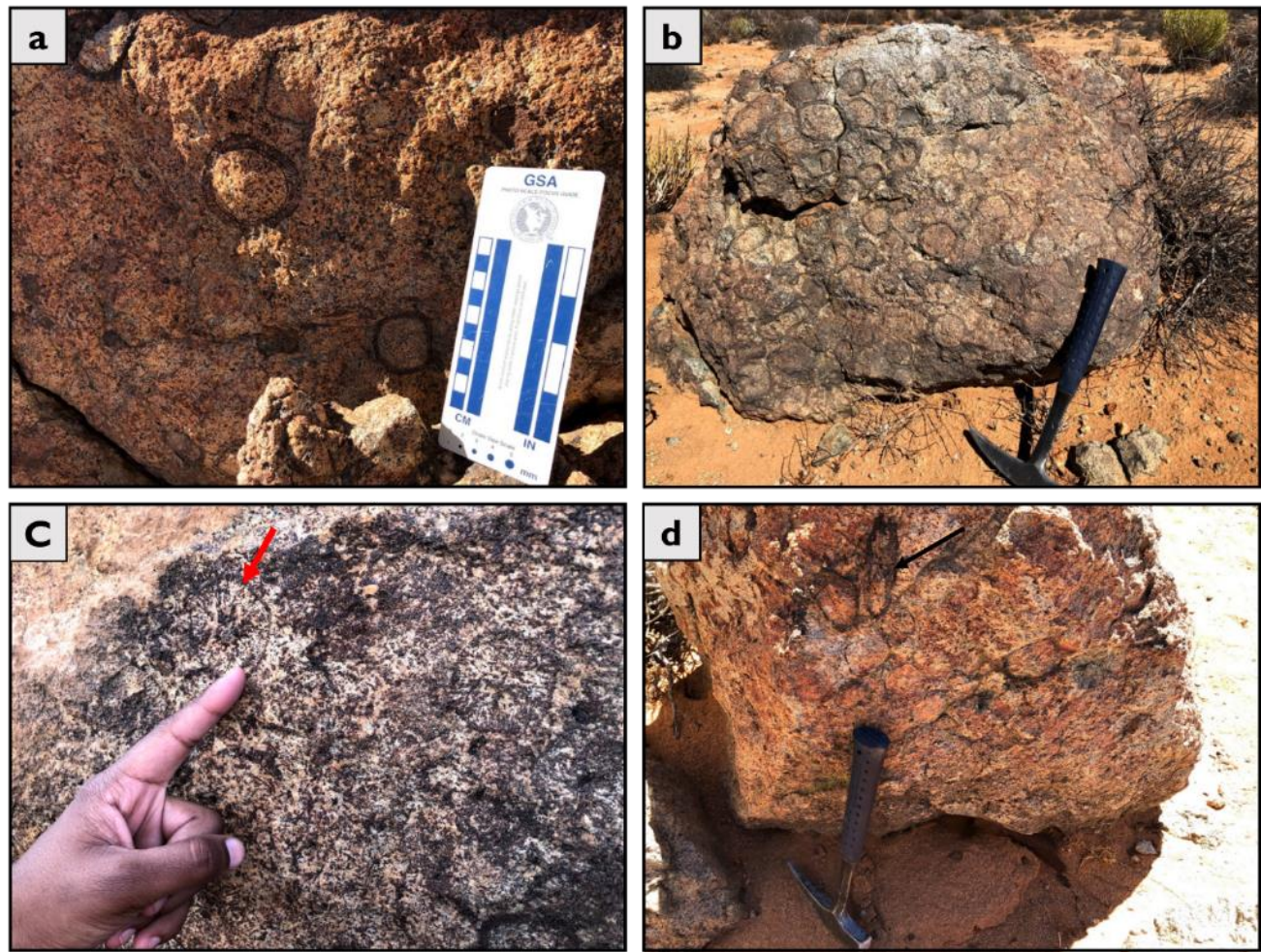
Figure 31: Boulders from the Hoogkraal Lease orbicule outcrop: (a) A boulder showing ~ 30% orbicules to 70% host matrix relative volumes. (b) A boulder showing more orbicules to matrix relative volume. (c) Radiating orthopyroxene texture (red arrow) restricted to the orbicular shells. (d) An outcrop showing different shapes of orbicules, both elongated (black arrow) and spherical.
