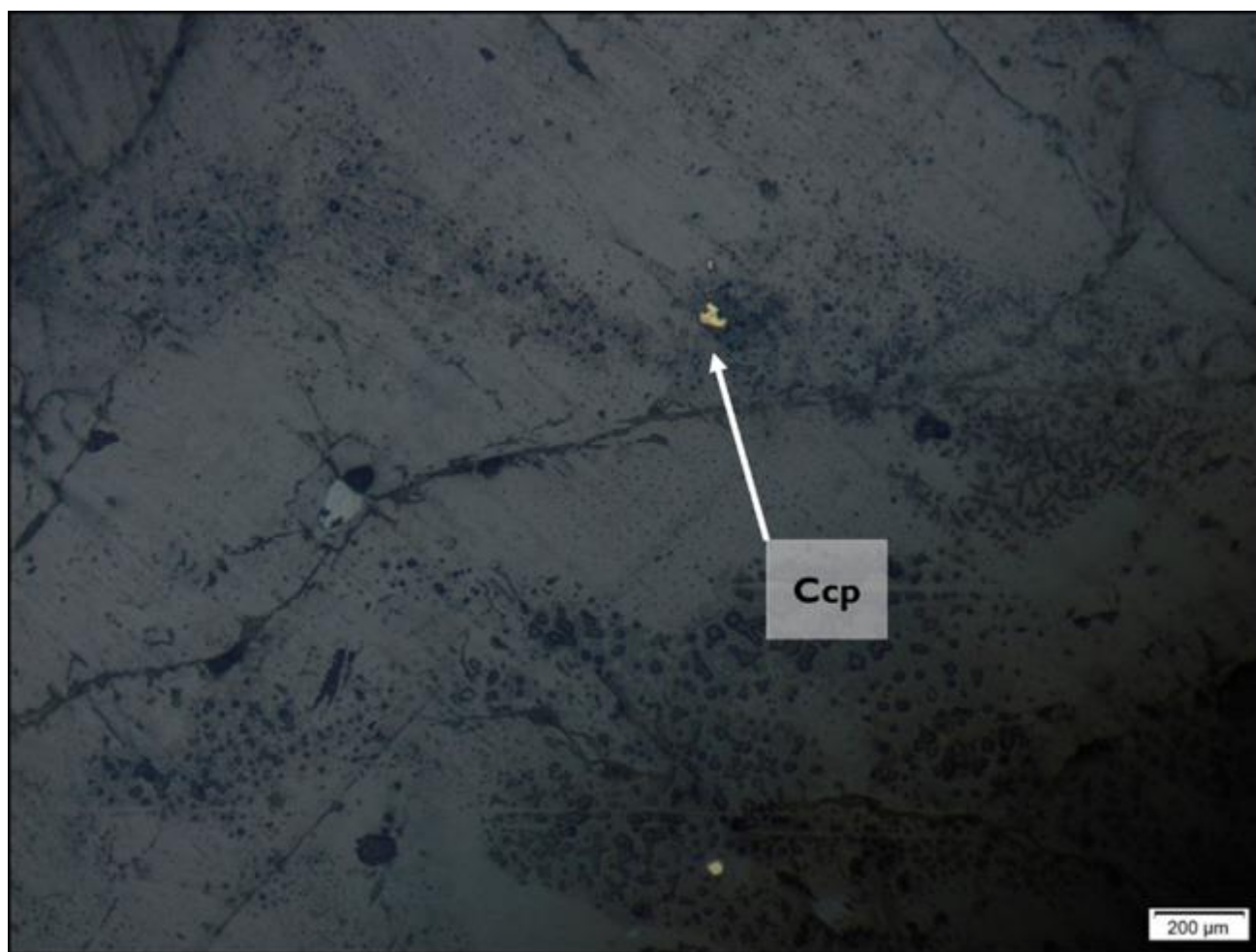
Figure 64: Small, anhedral and disseminated chalcopyrite grain in a matrix from the Hoogkraal Lease orbicules.
