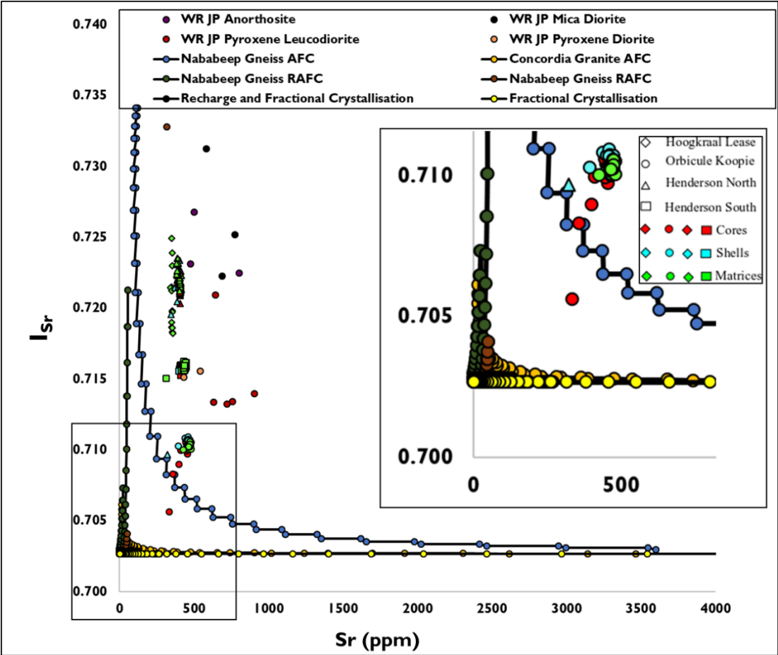
Figure 114: An energy constrained MCS model simulating FC, RFC, AFC with both the NababEEP Gneiss and the Concordia Granite and RAFC using depleted mantle-derived Karoo Large Igneous
