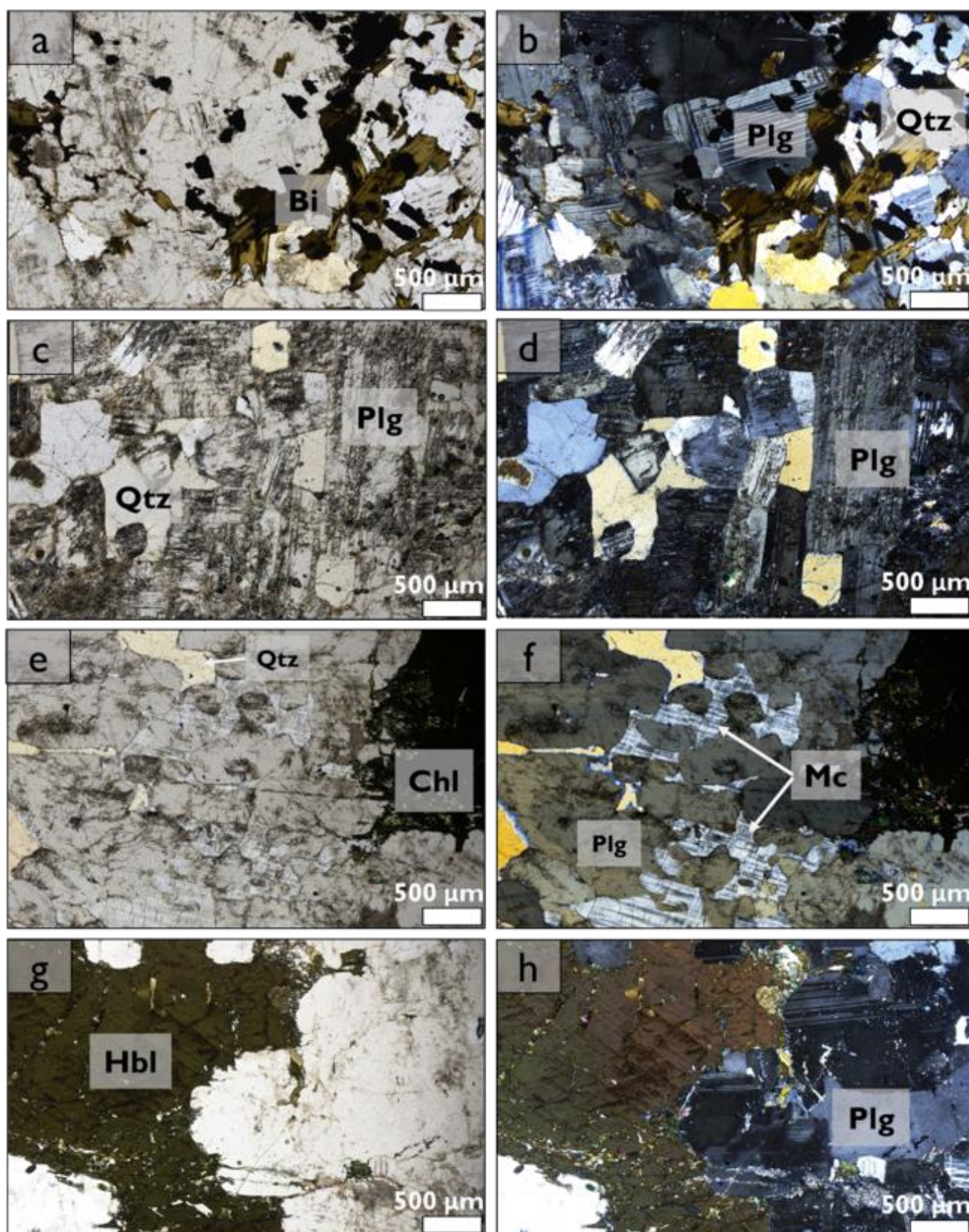
Figure 13: Photomicrographs showing mineral phases and textures in orbicular cores taken from Diana's Pool orbicules: (a, b) Subhedral plagioclase grains occurring adjacent to quartz and biotite. (c, d) Subhedral plagioclase grains occurring adjacent to quartz. Plagioclase is altered to sericite. (e, f) Interstitial microcline enveloping large plagioclase grains that occur adjacent to hornblende. (g, h) Large hornblende grains adjacent to plagioclase and quartz.
