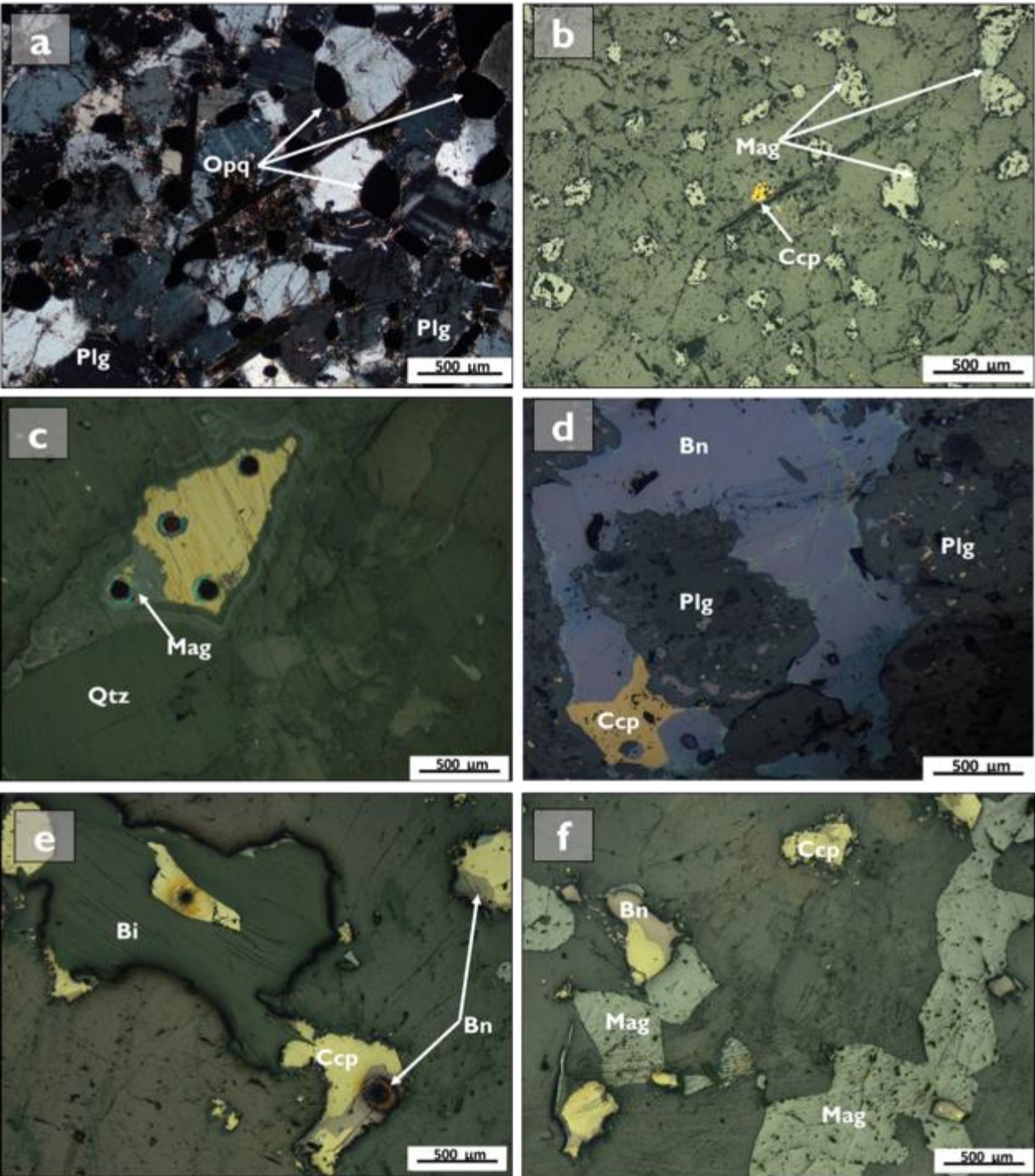
Figure 109: Photomicrographs of representative sulphide phases in the orbicules: (a, b) Photomicrographs in both transmitted and reflected light showing opaque phases occurring along or close to silicate grain boundaries. Smooth and rounded grain boundaries characterize oxides and feathered margins characterize the sulphides. (c) Independent and massive chalcopyrite grain in Orbicule Koppie matrix that is replaced by magnetite. (d) Interstitial bornite and chalcopyrite overgrowths surrounding altered plagioclase that contain small poikilitic inclusions of chalcopyrite. (e) Inclusion of chalcopyrite grains along cleavage planes in biotite surrounded by grains of chalcopyrite and bornite overgrowths. (f) Jubilee Pit sample characterized by bornite and chalcopyrite overgrowths. The grains grow adjacent to magnetite and locally grow along the grain boundaries of magnetite. Some of the photomicrographs (d and e) show the laser spots used for trace element analysis of sulphides.
