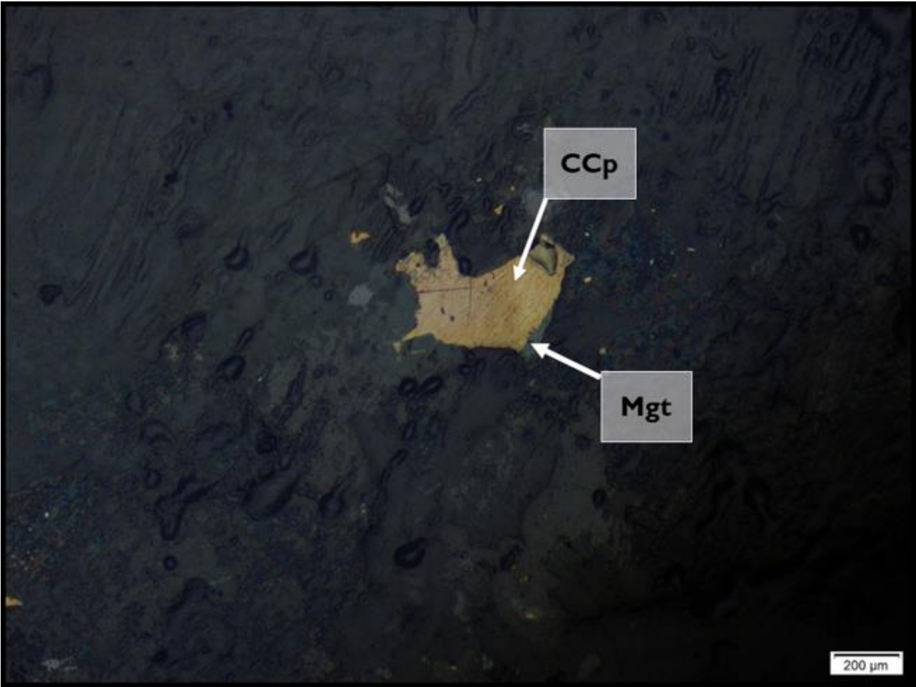
Figure 74: Massive chalcopyrite grain replaced by magnetite. The massive chalcopyrite grain occur adjacent to smaller ( < 0.1 mm) and disseminated chalcopyrite grains.
