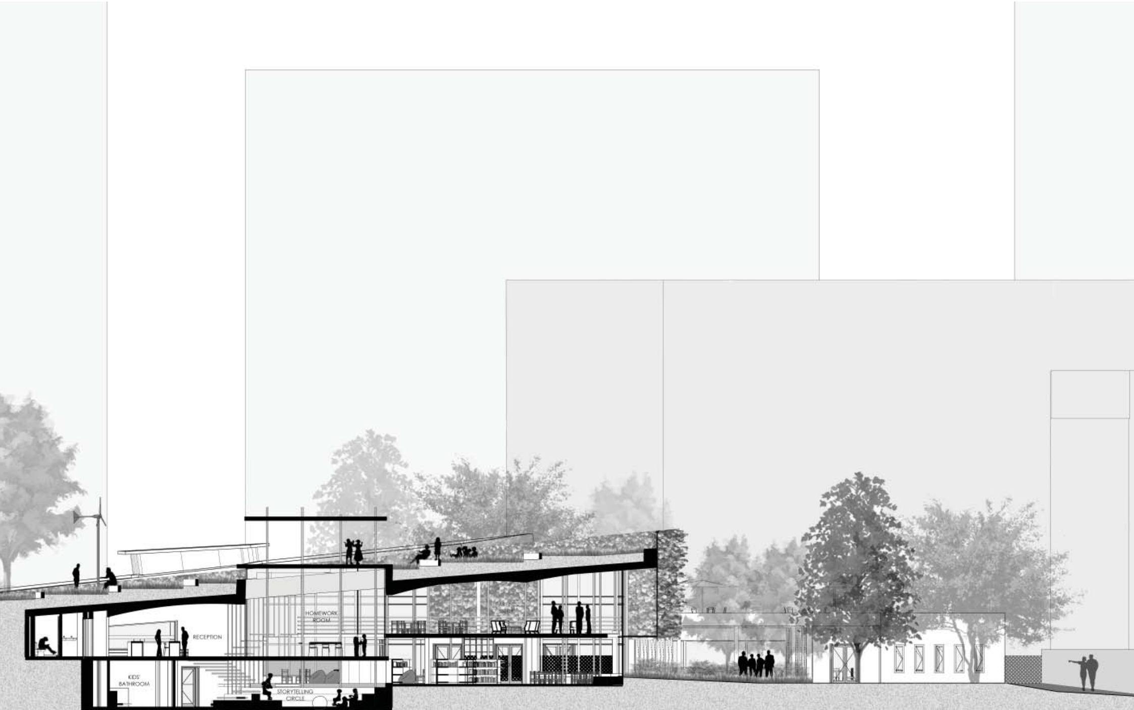
SECTION A-A CHILDREN'S LIBRARY
