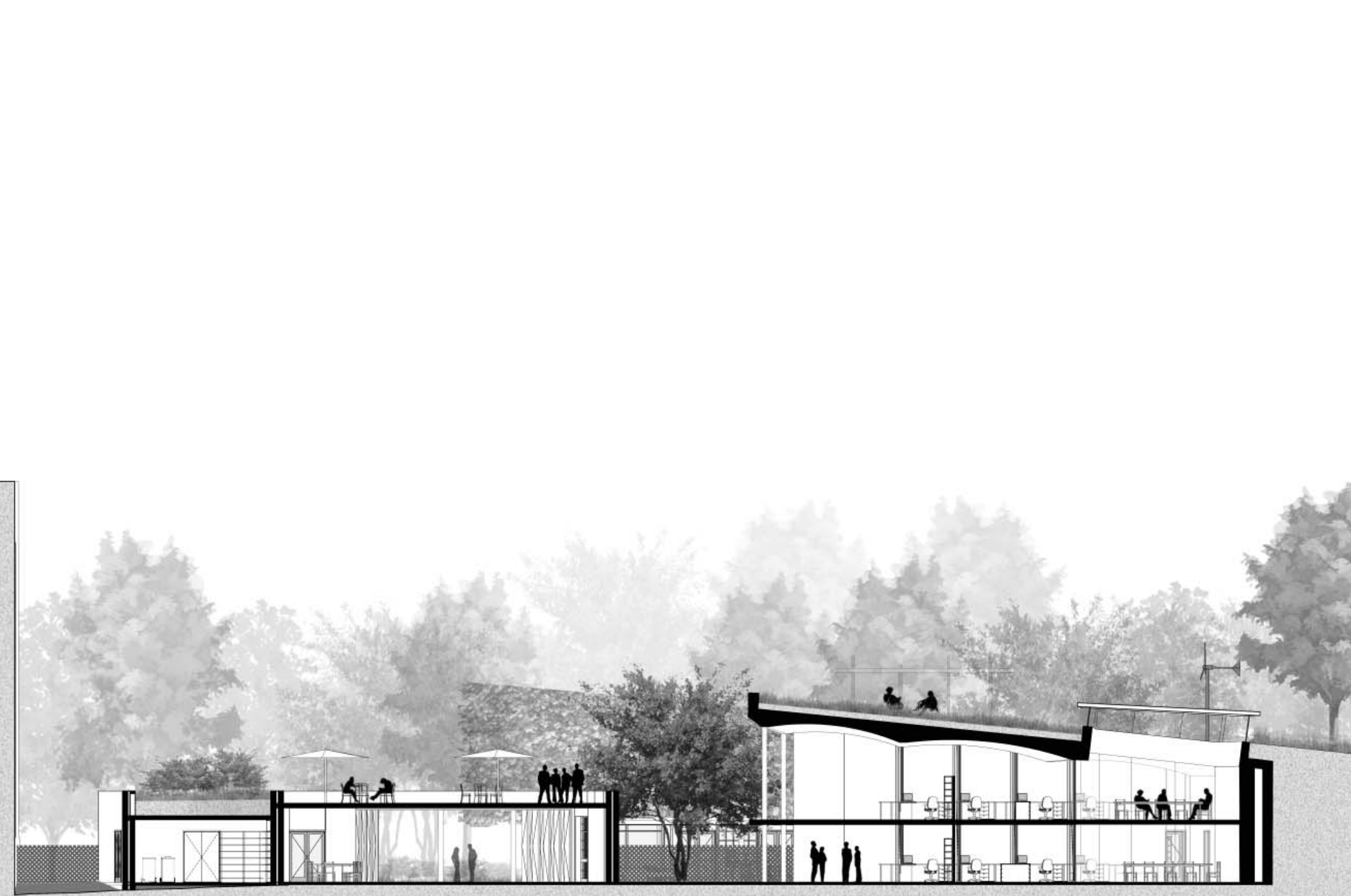
SECTION B-B TOY WORKSHOP & OFFICES
