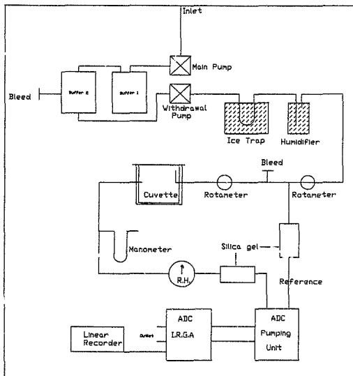
Fig. 5. The gas circuit employed in the determination of photosynthetic \text{CO}_2 uptake using the ADC I.R.G.A.
