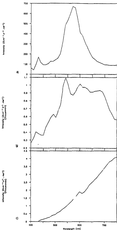
Fig. 4. Spectral analysis of light sources used for: a) Growth of plants; b) Gas exchange studies; c) Oxygen evolution studies.
