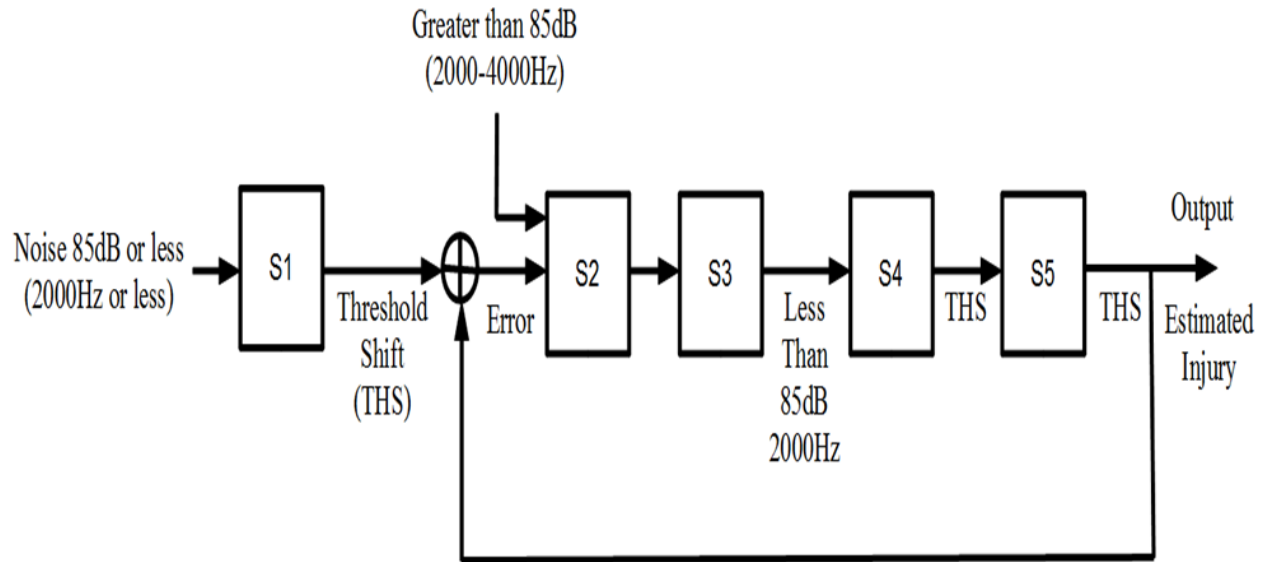
Figure 7: Overall system diagram for a feedback based model for NIHL monitoring (Moroe, Khoza-Shangase, Madahana, & Nyandoro, 2018)
