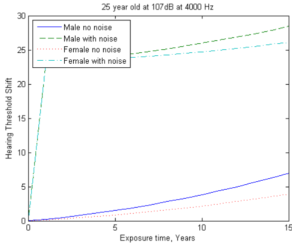
Figure 12: - 25 year old mine worker's threshold shift without protection
