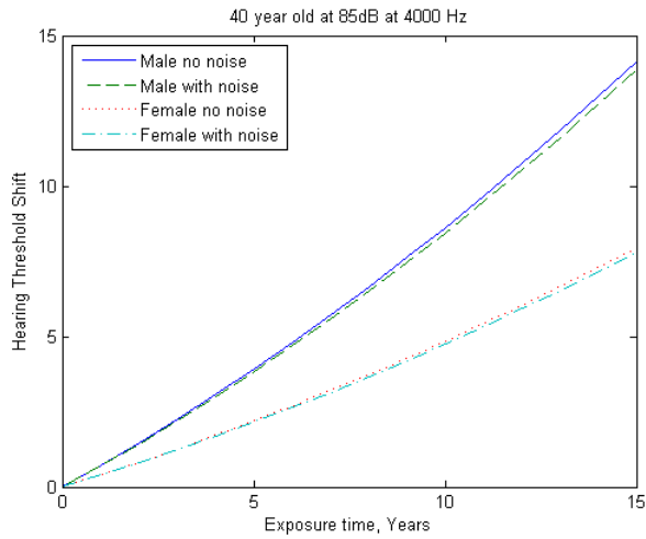
Figure 11: - 40 year old mine worker's threshold shift with protection
