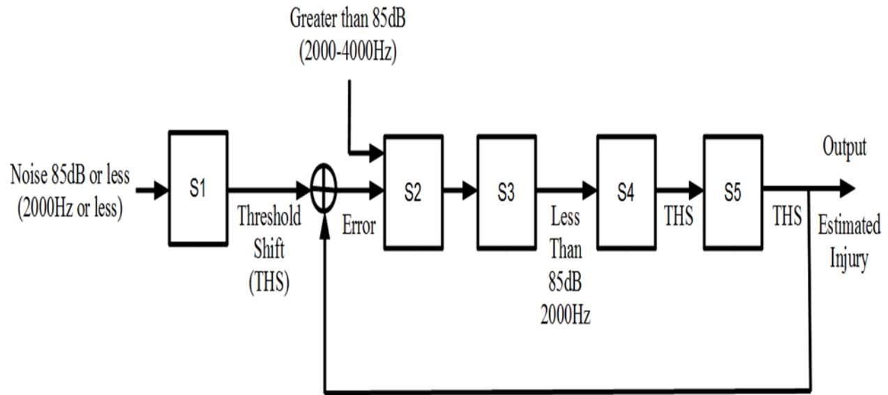
Figure 7: - Overall model diagram for a feedback-based model for ONIHL monitoring
