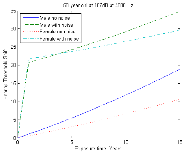
Figure 8: - 50 year old, mine worker's threshold shift without hearing protection
