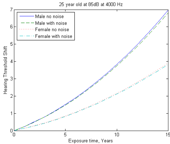
Figure 13: - 25 year old mine worker's threshold shift with protection
