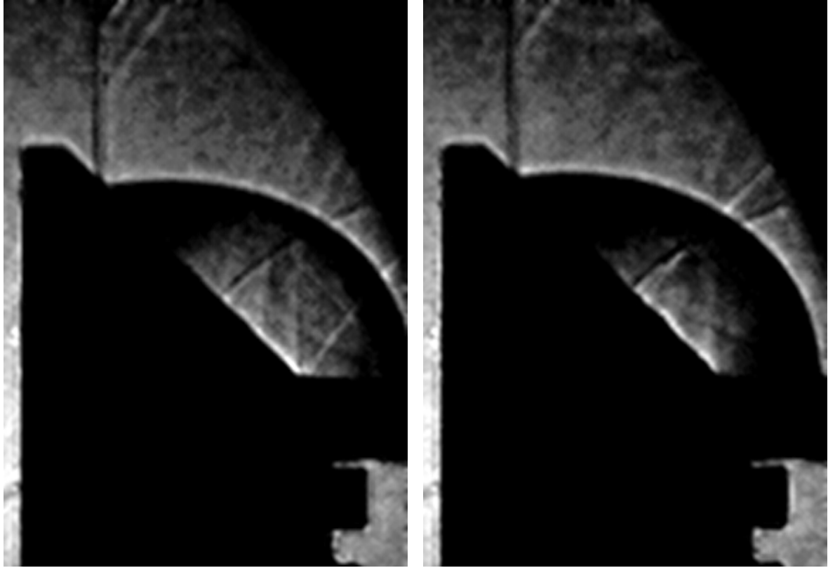
7.11 (e): Convex Profile 50 \mu m M_0 = 1.285
