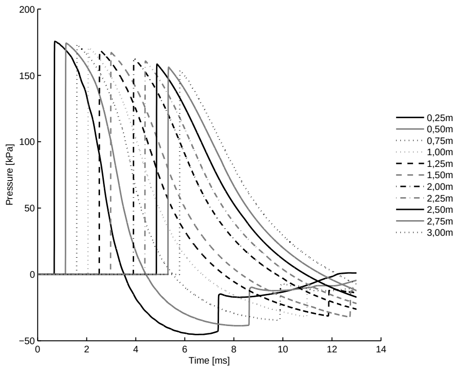
A.1 (b): 75% of Linear Driver Length 10bar
