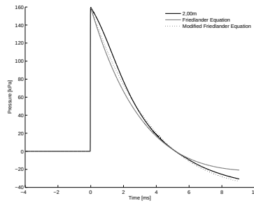
4.33 (e): 75% of Concave Driver Length 10bar 2.00m
