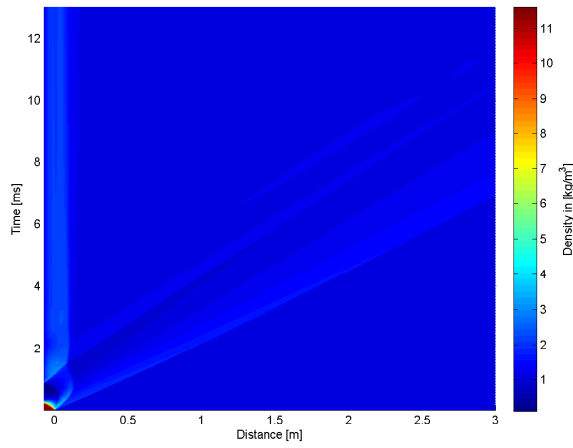
4.42 (a): 50% of Concave Driver and Transition Length 10bar
