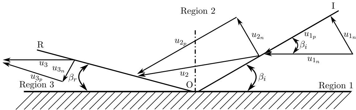
Figure 2.11: Steady Flow counterpart of Oblique Reflection (Skews (1966))
