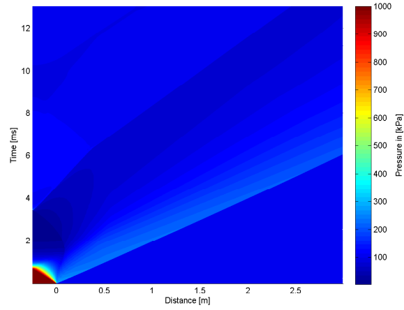
B.4(e): 150% of Linear Driver and Transition Length 10bar
