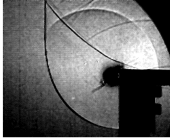
7.5 (d): Linear Profile 100\mu m M_0 = 1.362
