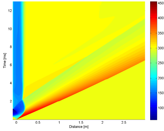
B.6 (a): 50% of Linear Driver and Transition Length 10bar
