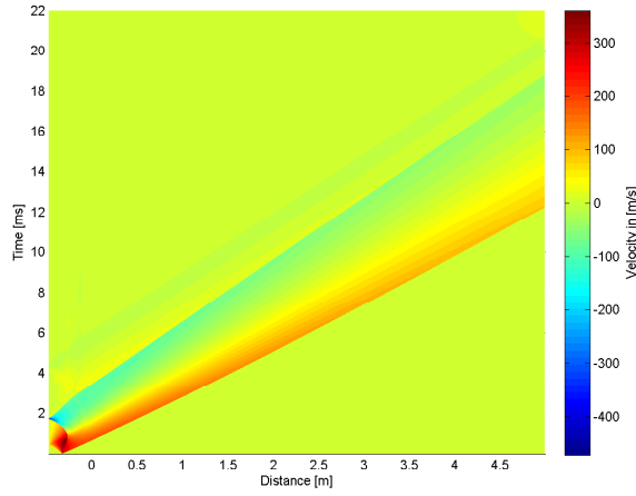
4.54 (a): Concave Profile 10bar
