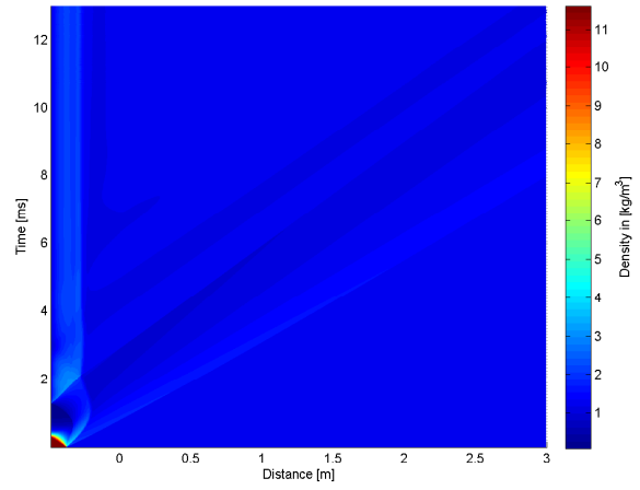
4.35 (d): 25% of Concave Driver Length 10bar
