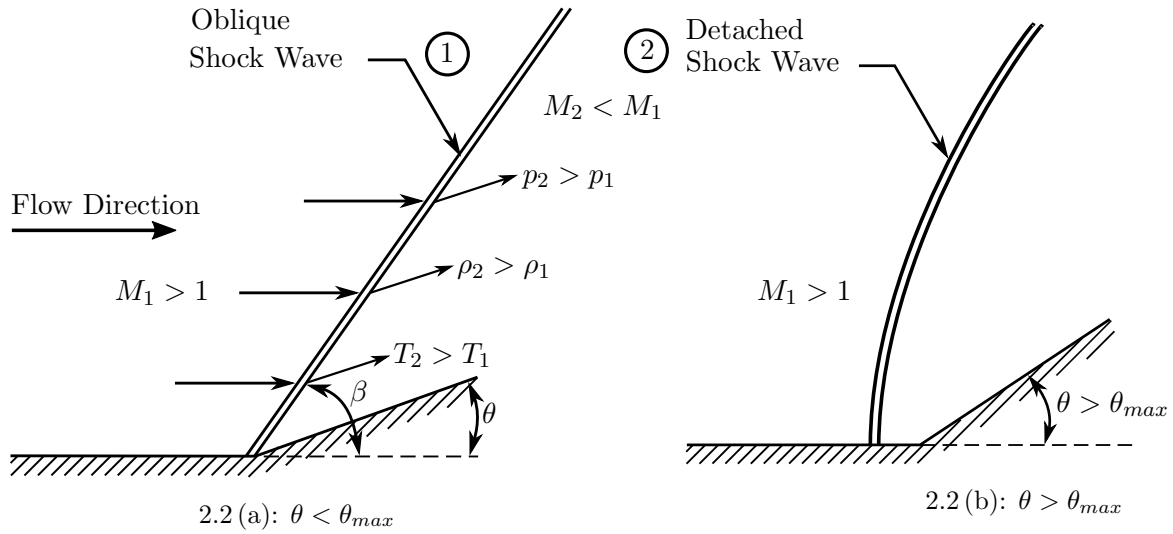
Figure 2.2: Supersonic Flow over a Concave Corner (Anderson (1990))
