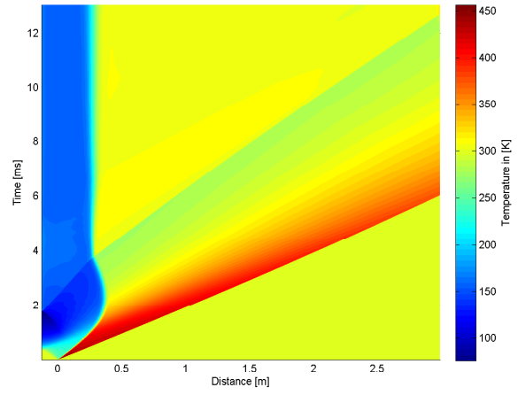
B.13 (b): 75% of Convex Driver and Transition Length 10bar
