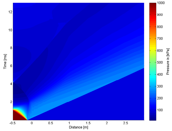
A.4(b): 75% of Linear Driver Length 10bar
