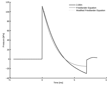
4.33 (h): 50% of Concave Driver Length 10bar 2.00m
