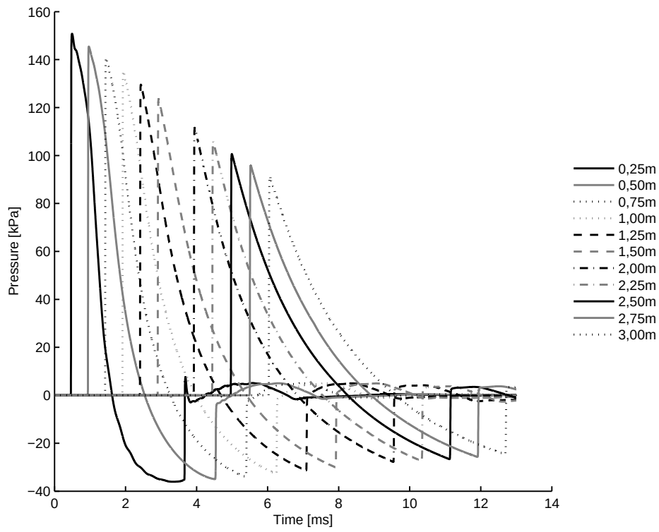
B.8 (b): 75% of Convex Driver and Transition Length 10bar
