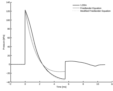
B.3(j): 125% of Linear Driver and Transition Length 10bar 1.00m
