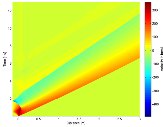
4.44 (c): 100% of Concave Driver and Transition Length 10bar
