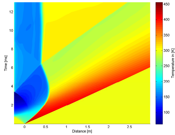
B.6 (e): 150% of Linear Driver and Transition Length 10bar
