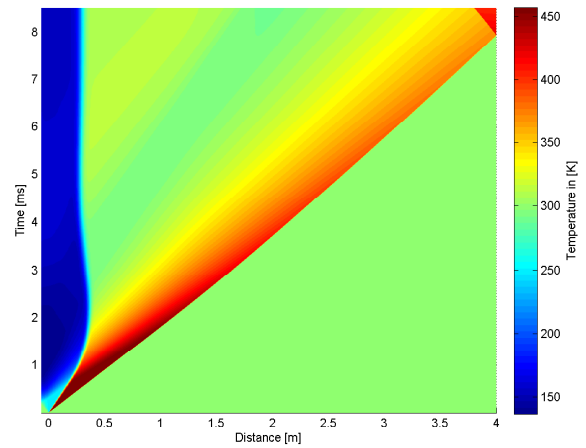
4.26 (b): 65mm 5bar Temperature
