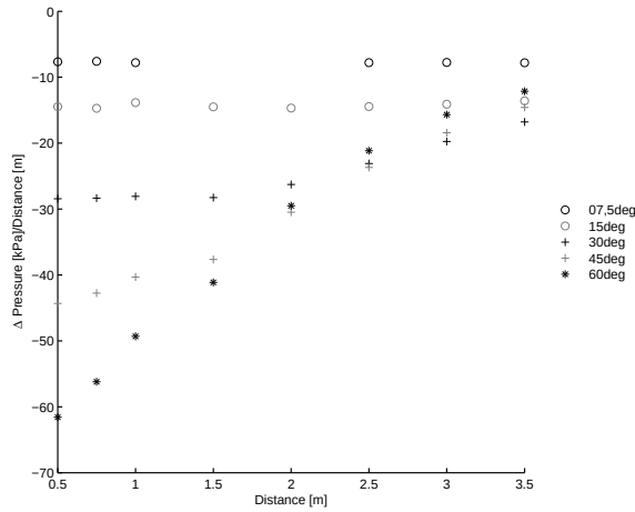
4.7 (a): Rate of Change of Peak Overpressure with Regards to Distance for Diverging Driver Sections
