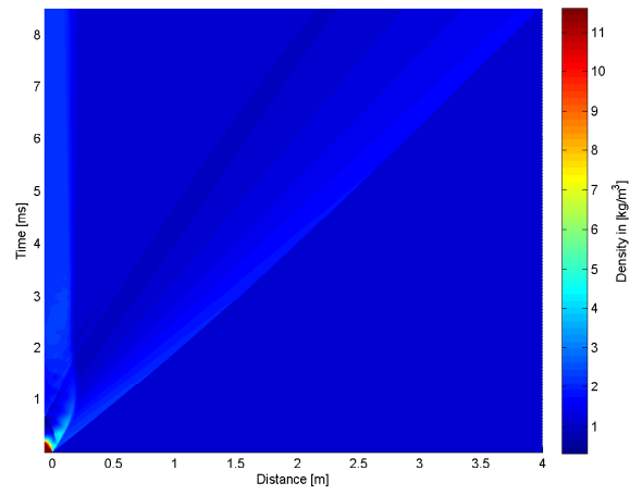
4.10 (e): 60^\circ 10bar
