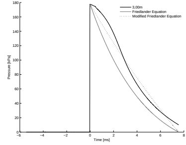
A.10 (c): 100% of Convex Driver Length 10bar 3.00m
