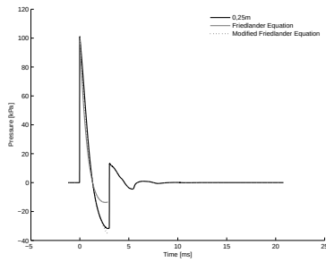
4.48 (a): Concave Profile 10\text{bar} 0.25\text{m}
