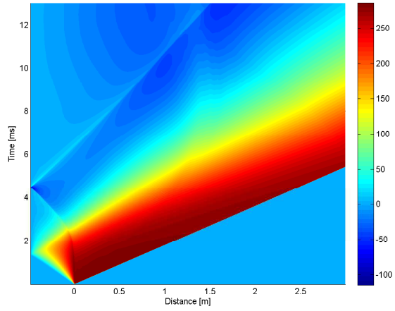
4.37 (a): 100% of Concave Driver Length 10bar
