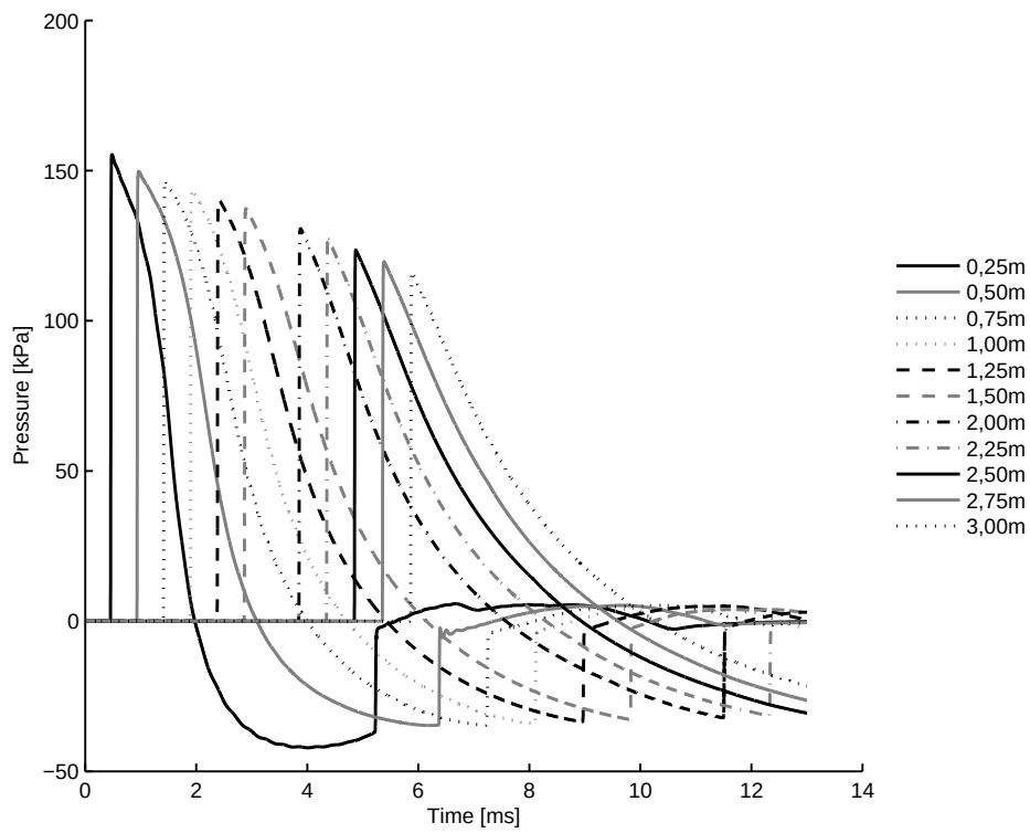
B.8 (d): 125% of Convex Driver and Transition Length 10bar
