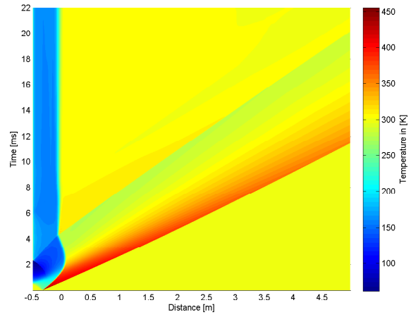
4.53 (b): Linear Profile 10bar
