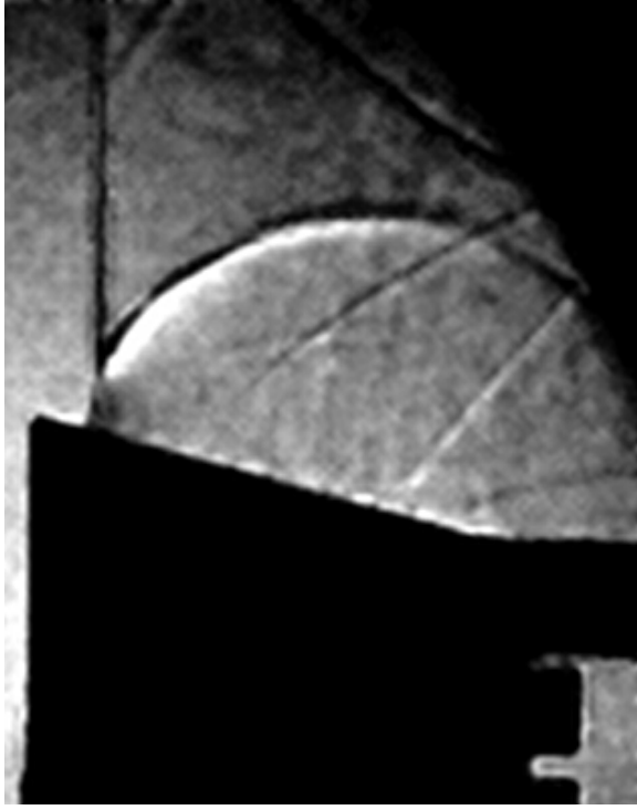
7.7 (e): Convex Profile 50\mu m M_0 = 1.240
