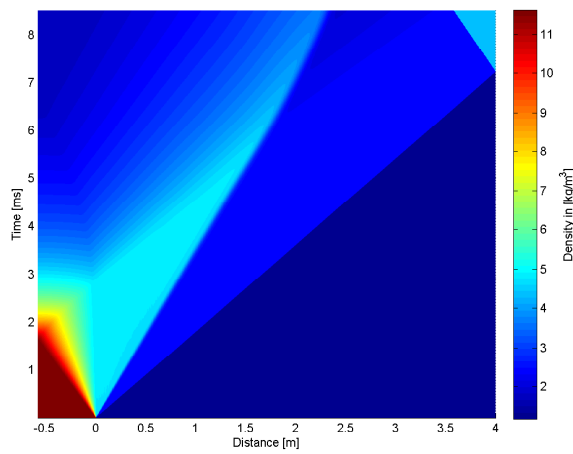
4.22 (a): 580mm 10bar
