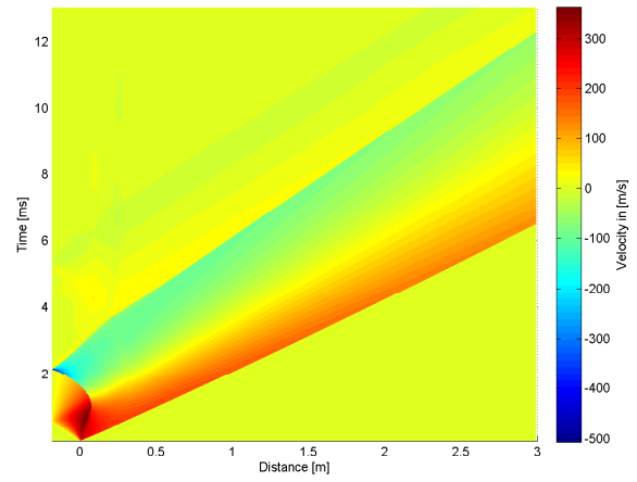
4.44 (d): 125% of Concave Driver and Transition Length 10bar
