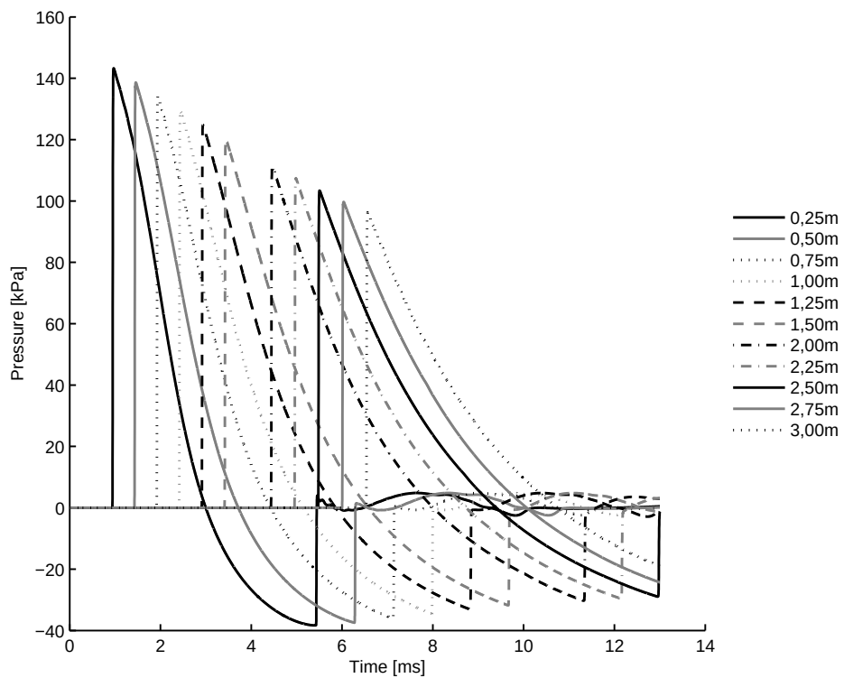
4.31 (c): 50% of Concave Driver Length 10bar
