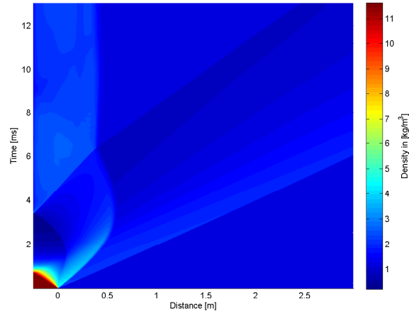
B.5 (e): 150% of Linear Driver and Transition Length 10bar
