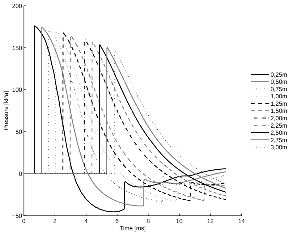
4.31 (b): 75% of Concave Driver Length 10bar
