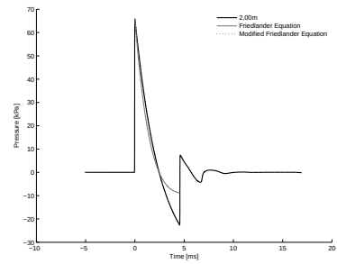
4.48 (c): Concave Profile 10\text{bar} 2.00\text{m}
