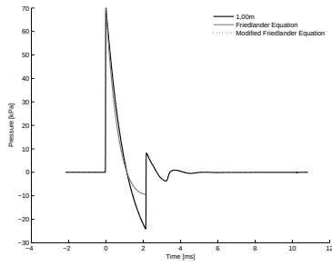
4.40 (a): 50% of Concave Driver and Transition Length 10bar 1.00m
