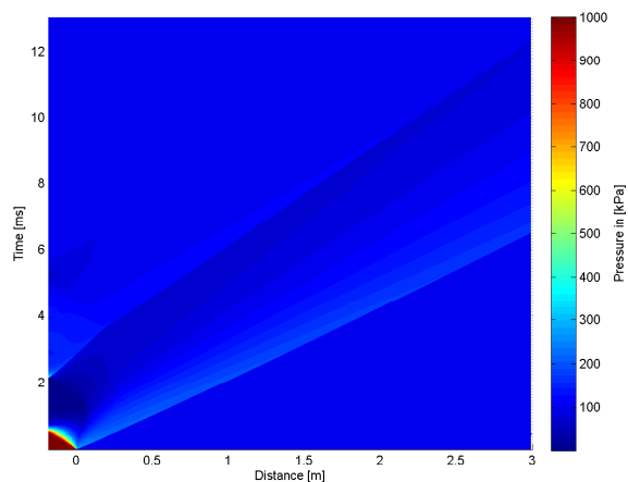
4.41 (d): 125% of Concave Driver and Transition Length 10bar
