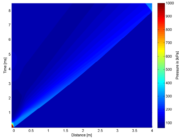
4.26 (a): 65mm 5bar Pressure
