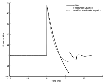
4.48 (e): Concave Profile 10\text{bar} 4.00\text{m}
