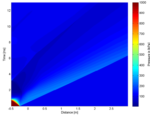
A.4 (c): 50% of Linear Driver Length 10bar
