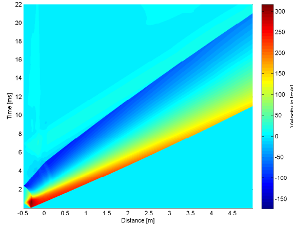
4.54 (c): Convex Profile 10bar
