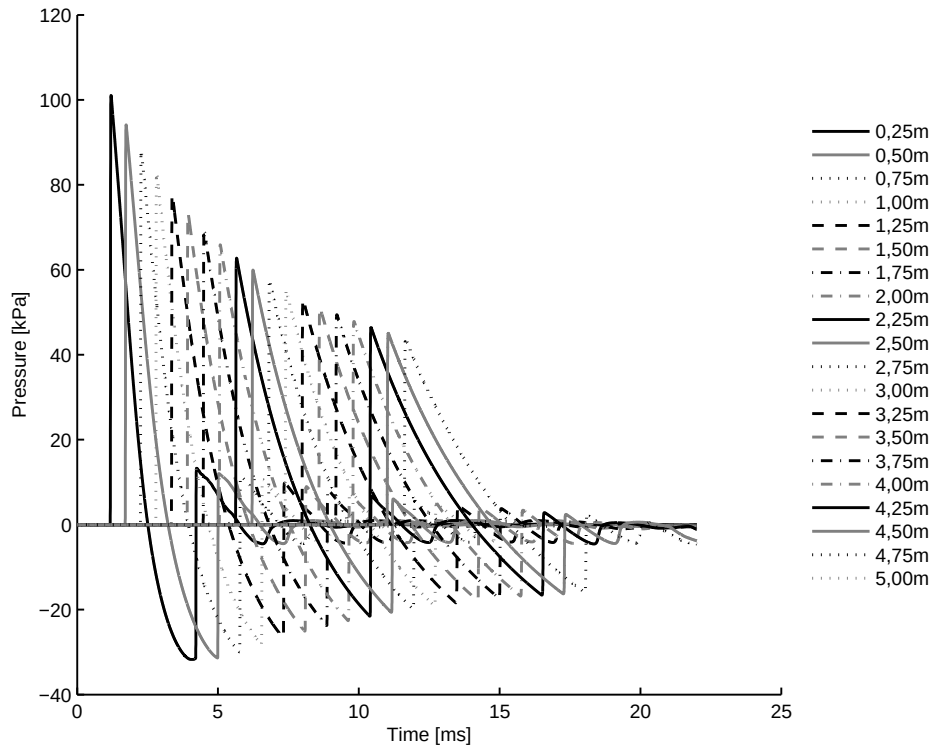
4.47 (a): Concave Profile 10\text{bar}
