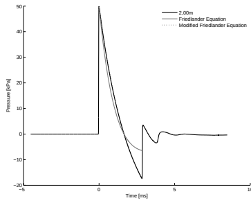
4.40 (b): 50% of Concave Driver and Transition Length 10bar 2.00m
