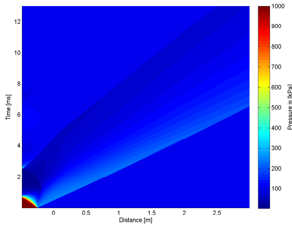
4.34 (c): 50% of Concave Driver Length 10bar
