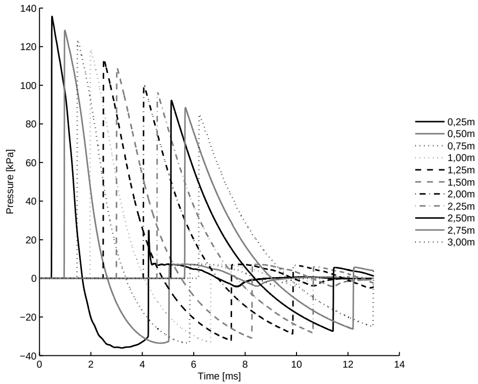
B.1 (c): 100% of Linear Driver and Transition Length 10bar
