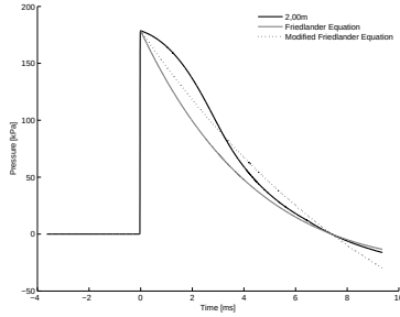
A.3 (b): 100% of Linear Driver Length 10bar 2.00m
