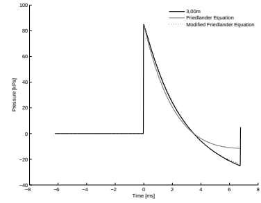
B.3(i): 100% of Linear Driver and Transition Length 10bar 3.00m
