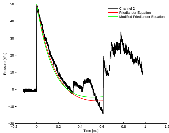
7.2 (e): Linear Profile 50\mu m \approx 600kPa 2.73m
