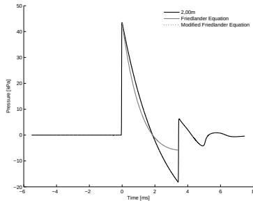
4.33 (k): 25% of Concave Driver Length 10bar 2.00m
