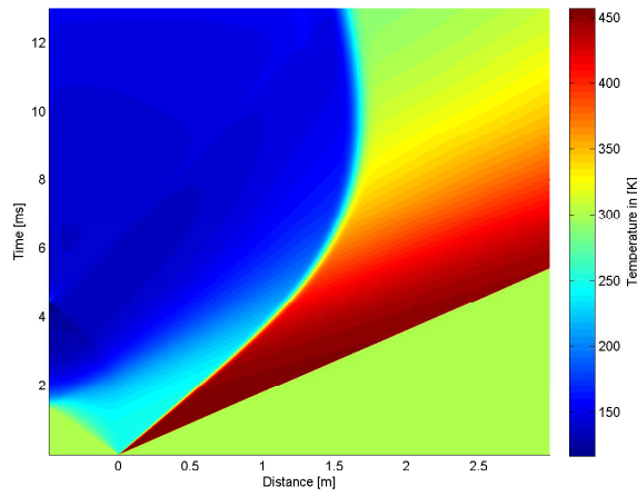
4.36 (a): 100% of Concave Driver Length 10bar
