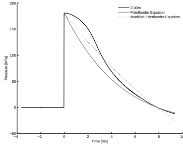
A.10 (b): 100% of Convex Driver Length 10bar 2.00m
