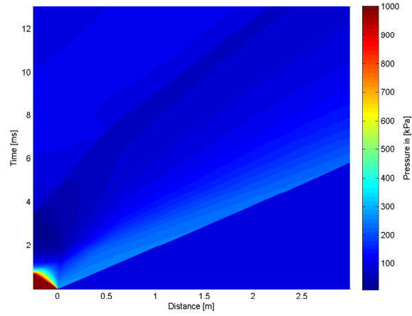
B.11 (e): 150% of Concave Driver and Transition Length 10bar
