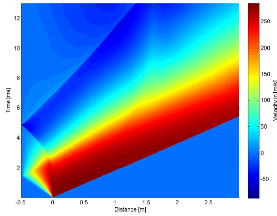
A.7 (a): 100% of Linear Driver Length 10bar
