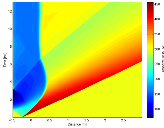
A.6 (c): 50% of Linear Driver Length 10bar
