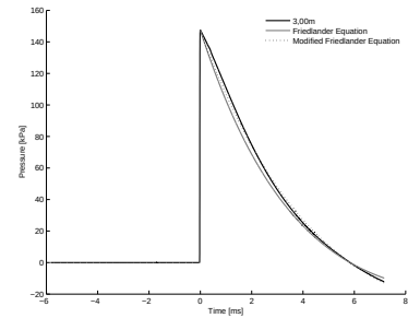
4.33 (f): 75% of Concave Driver Length 10bar 3.00m
