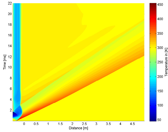
4.53 (a): Concave Profile 10bar
