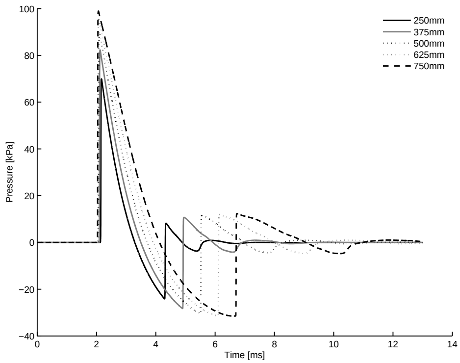
4.39 (b): 1.00m 10bar
