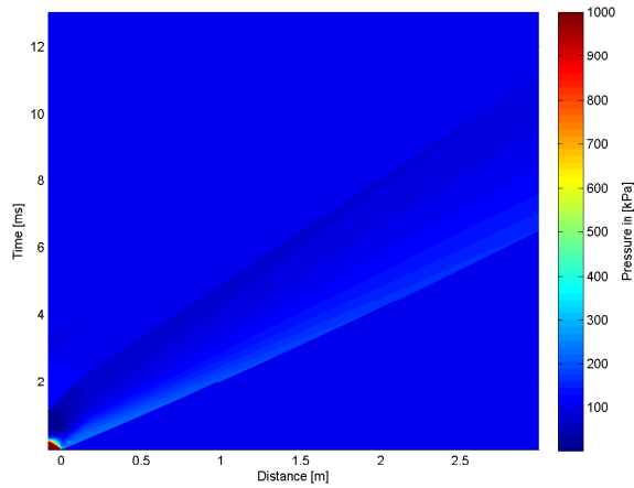
B.4(a): 50% of Linear Driver and Transition Length 10bar
