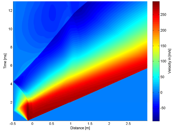
A.14 (b): 75% of Convex Driver Length 10bar
