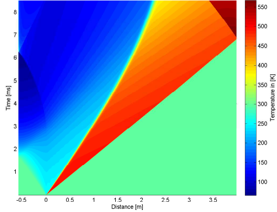
4.15 (b): 7.5° 15bar Temperature
