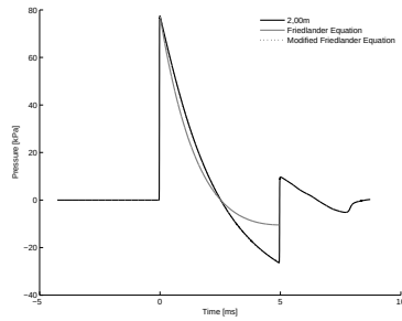
4.40 (k): 125% of Concave Driver and Transition Length 10bar 2.00m
