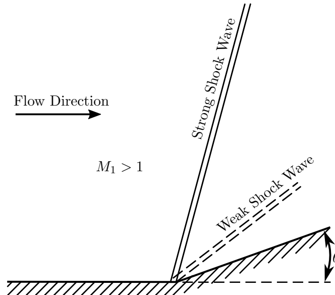
Figure 2.3: Weak and Strong Oblique Shock Waves (adapted from Anderson 1990)
