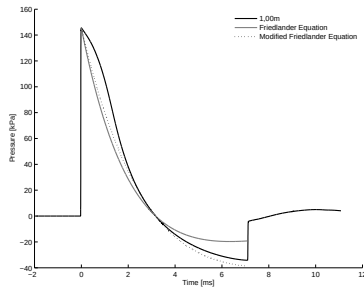
B.10 (m): 150% of Convex Driver and Transition Length 10bar 1.00m
