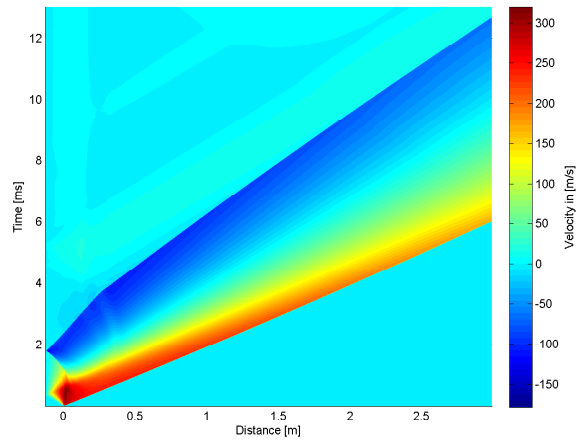
B.14(b): 75% of Convex Driver and Transition Length 10bar
