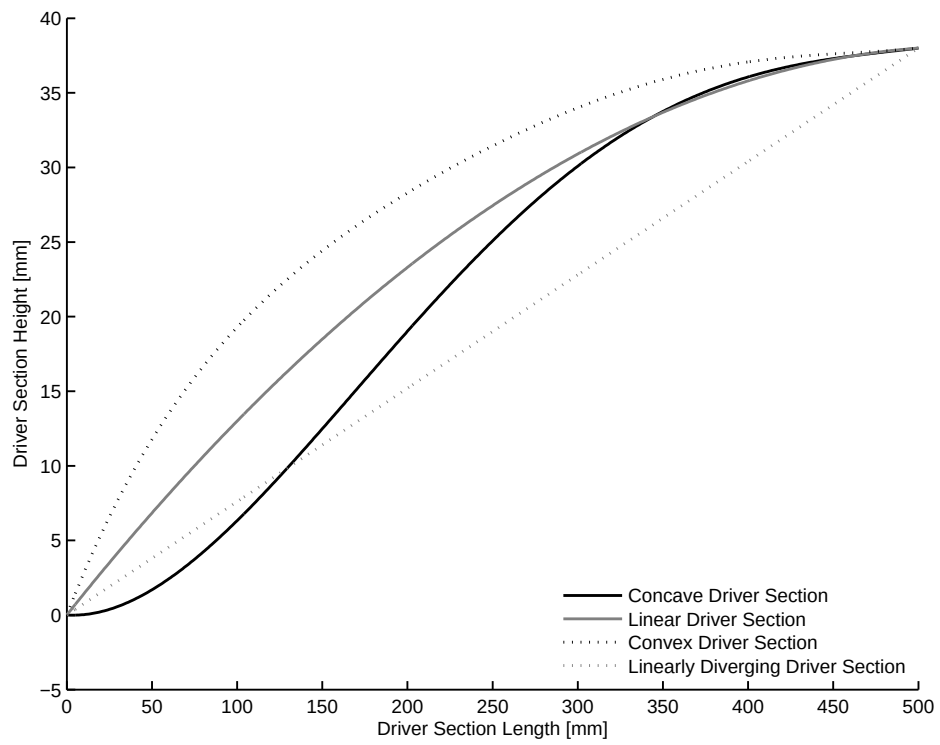
Figure 4.29: The 3 Driver Section Profiles Designed for Further Testing
