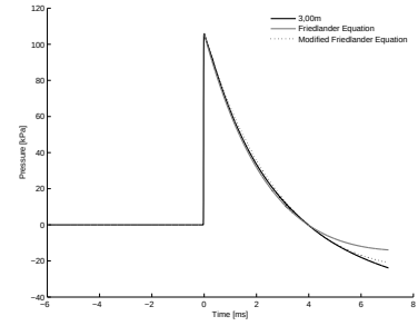
B.10 (i): 100% of Convex Driver and Transition Length 10bar 3.00m
