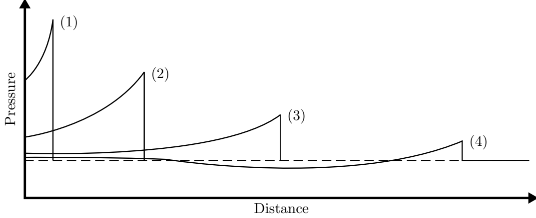
Figure 2.5: Progression of a Pressure-Distance Plot for Typical Point Source Explosion (Kinney (1962))
