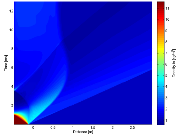
4.35 (b): 75% of Concave Driver Length 10bar
