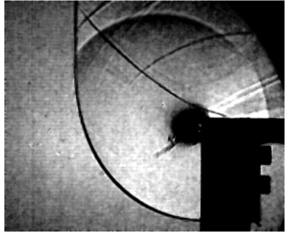
7.5 (f): Convex Profile 100\mu m M_0 = 1.335
