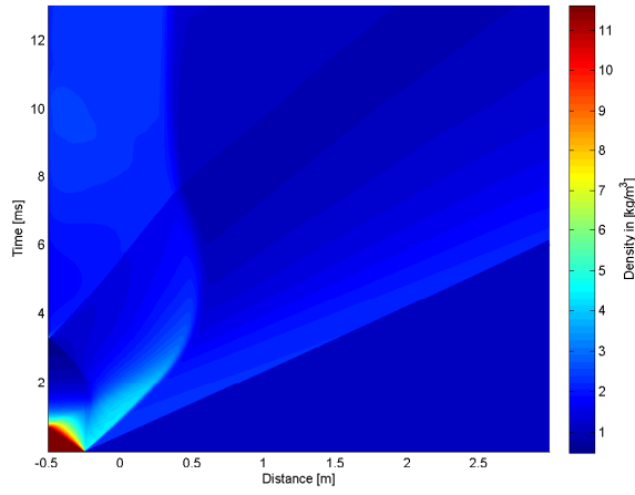
A.12 (c): 50% of Convex Driver Length 10bar
