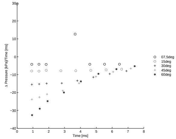
4.7 (b): Rate of Change of Peak Overpressure with Regards to Time for Diverging Driver Sections
