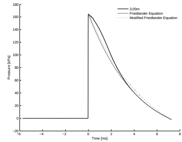
A.10 (f): 75% of Convex Driver Length 10bar 3.00m
