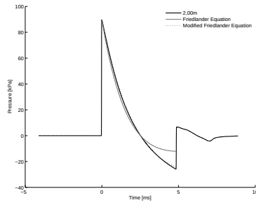
B.3(e): 75% of Linear Driver and Transition Length 10bar 2.00m
