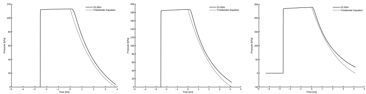
4.20 (a): 580mm 5bar
