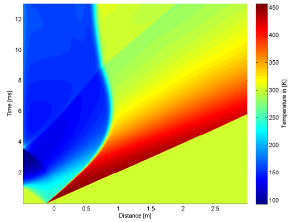
4.36 (b): 75% of Concave Driver Length 10bar
