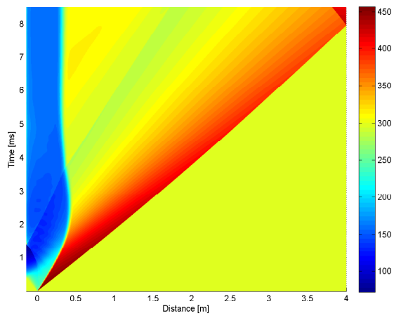
4.11 (c): 30^\circ 10bar
