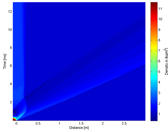
B.12(a): 50% of Convex Driver and Transition Length 10bar
