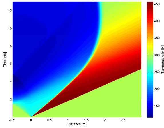
A.6 (a): 100% of Linear Driver Length 10bar
