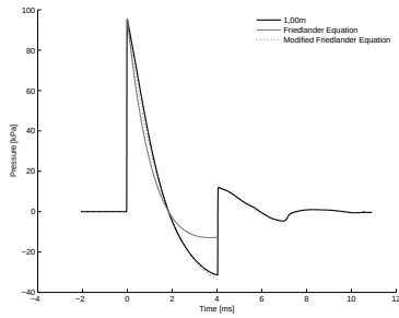
4.40 (j): 125% of Concave Driver and Transition Length 10bar 1.00m
