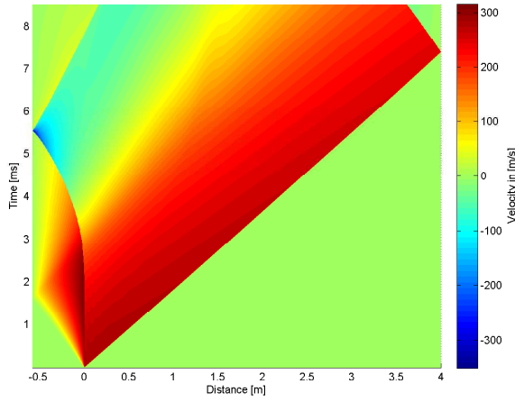
4.12 (a): 07.5^\circ 10bar
