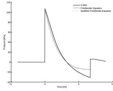
B.3(k): 125% of Linear Driver and Transition Length 10bar 2.00m
