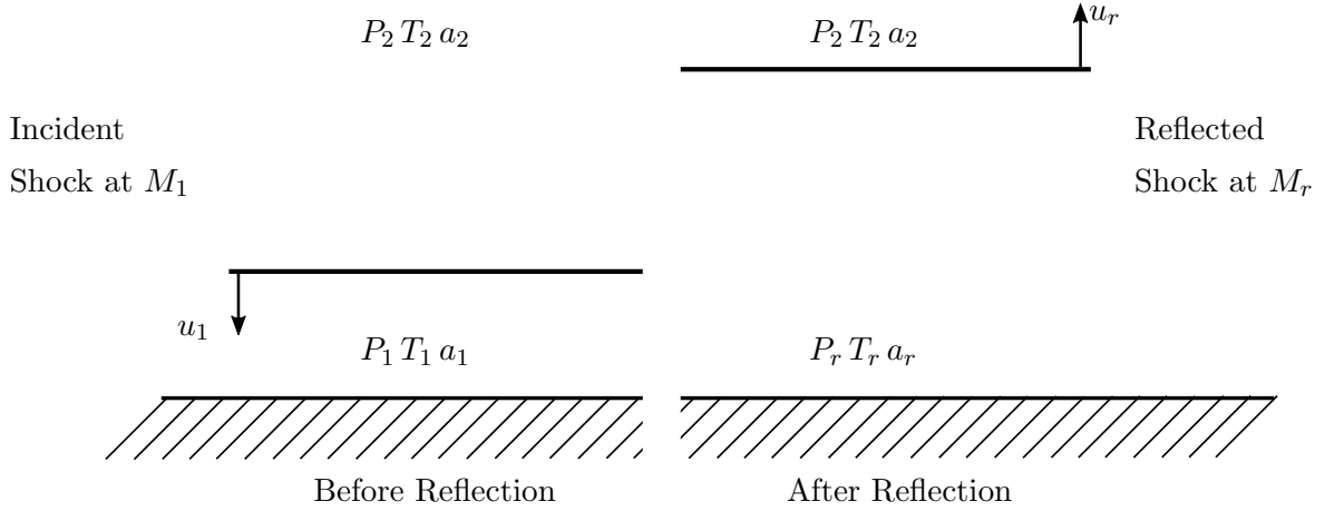
Figure 2.9: Normal Reflection of a Plane Shock (Kinney (1962))
