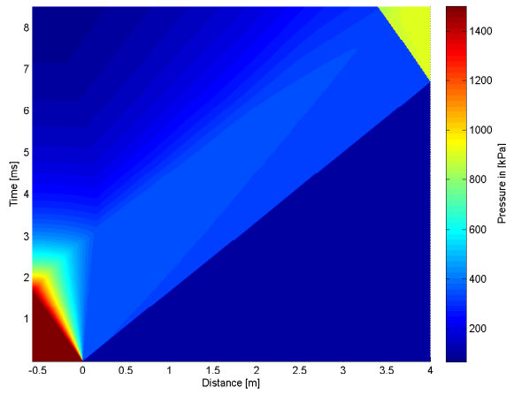
4.27 (a): 580mm 15bar Pressure
