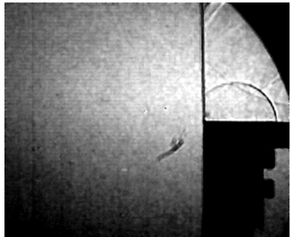
7.3 (d): Linear Profile 100 \mu m M = 1.362
