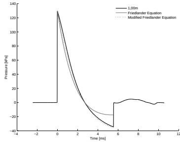
4.33 (g): 50% of Concave Driver Length 10bar 1.00m
