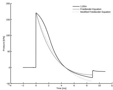
A.3 (d): 75% of Linear Driver Length 10bar 1.00m
