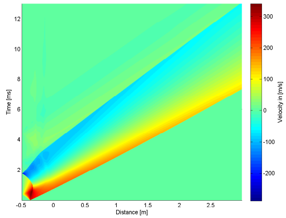
A.7 (d): 25% of Linear Driver Length 10bar
