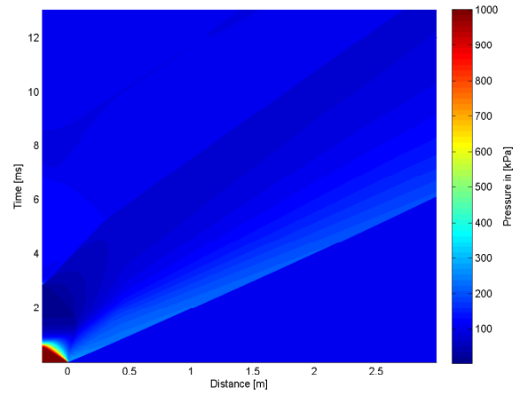
B.4(d): 125% of Linear Driver and Transition Length 10bar
