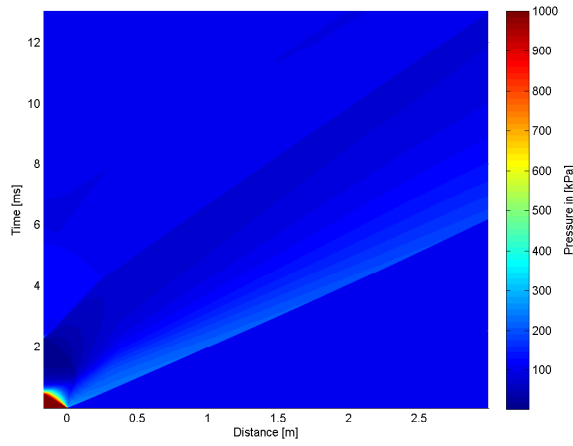
B.4(c): 100% of Linear Driver and Transition Length 10bar
