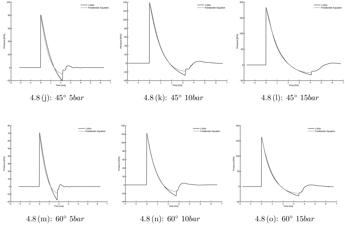
Figure 4.8: Comparing the Effect of Driver Shape and Pressure on Friedlander Pressure Profile
