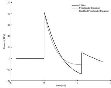
4.40 (n): 150% of Concave Driver and Transition Length 10bar 2.00m
