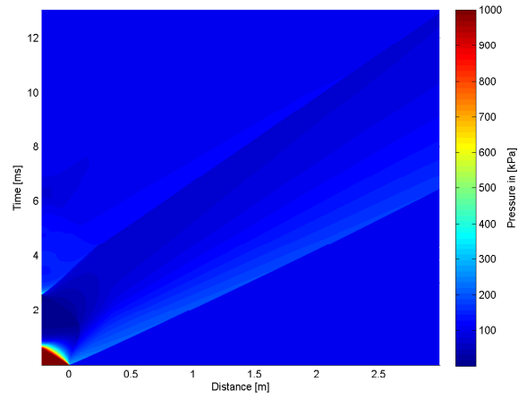
4.41 (e): 150% of Concave Driver and Transition Length 10bar
