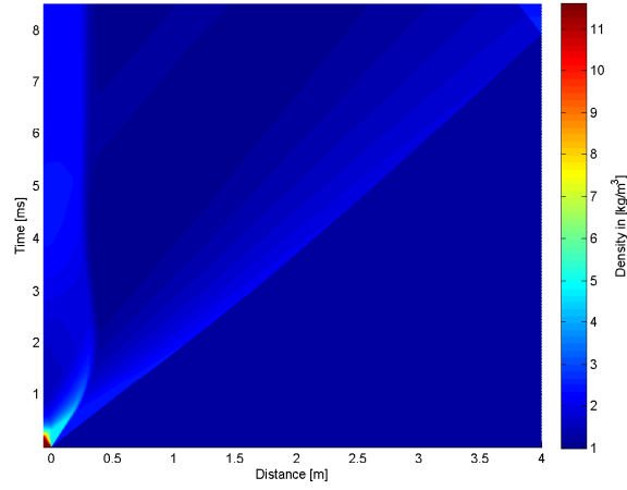
4.22 (e): 65mm 10bar
