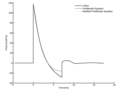
4.50 (c): Convex Profile 10bar 2.00m
