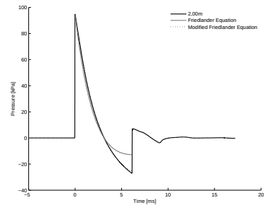
4.49 (c): Linear Profile 10\text{bar} 2.00\text{m}
