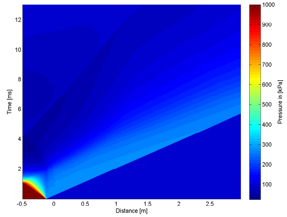
A.11 (b): 75% of Convex Driver Length 10bar
