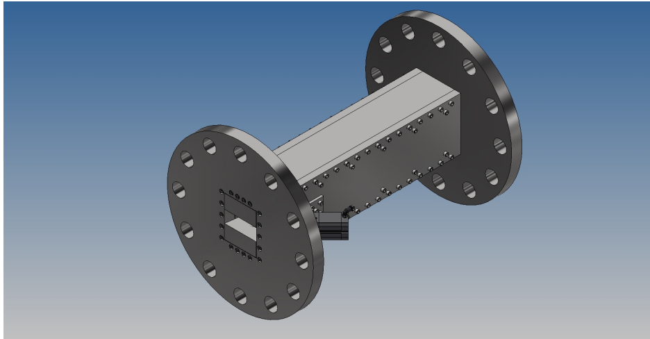
Figure 4.56: Driver Section Assembly
