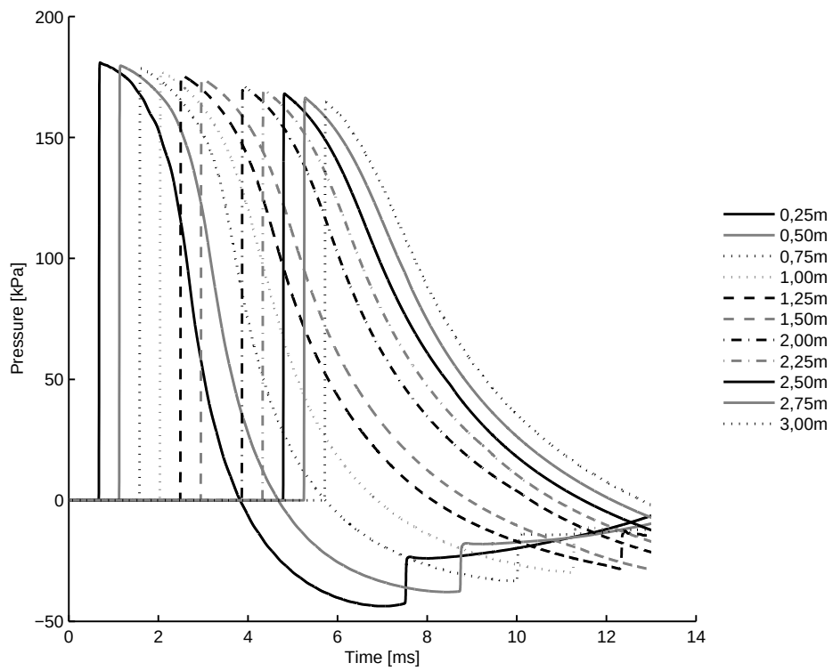
A.8 (b): 75% of Convex Driver Length 10bar
