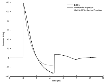
B.3(g): 100% of Linear Driver and Transition Length 10bar 1.00m
