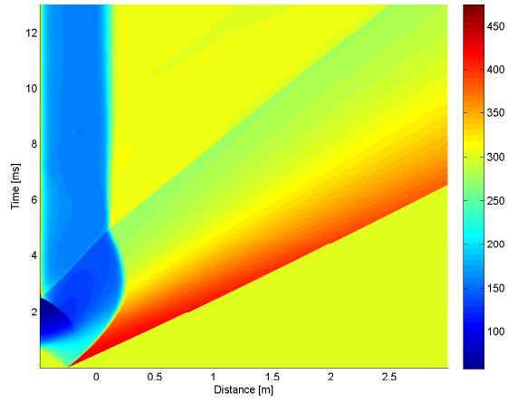
4.36 (c): 50% of Concave Driver Length 10bar
