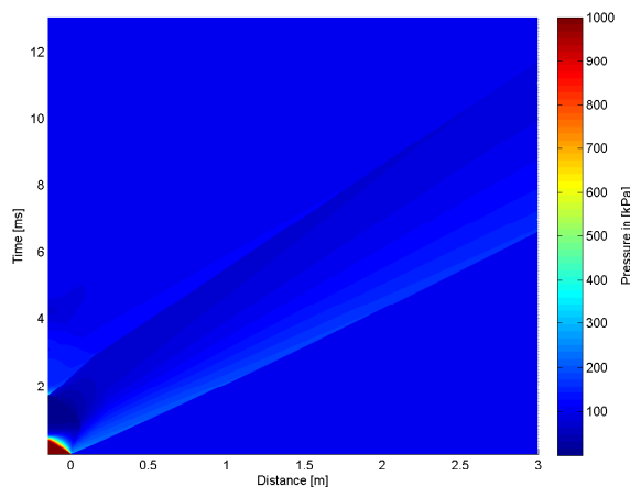
4.41 (c): 100% of Concave Driver and Transition Length 10bar
