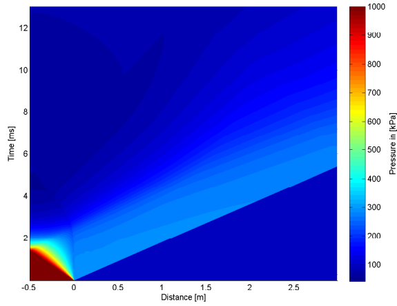
A.11 (a): 100% of Convex Driver Length 10bar
