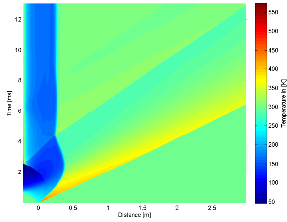
4.43 (e): 150% of Concave Driver and Transition Length 10bar
