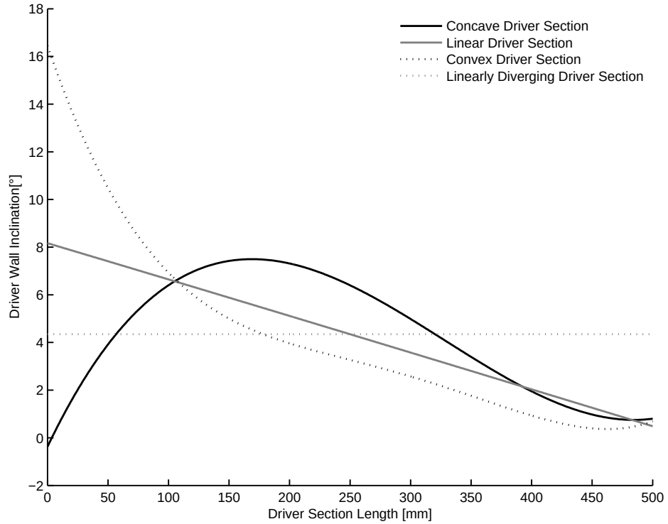
Figure 4.30: The Angle of Inclination of the 3 Driver Section Profiles
