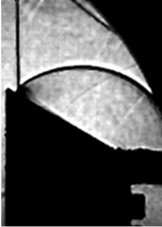
7.9 (c): Linear Profile 50\mu m M_0 = 1.263
