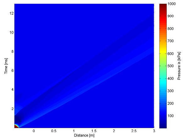
4.34 (d): 25% of Concave Driver Length 10bar
