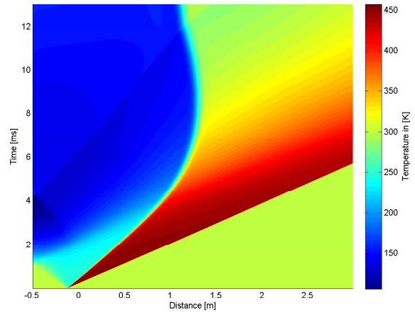
A.13 (b): 75% of Convex Driver Length 10bar
