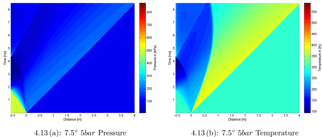
Figure 4.13: X-T Diagram for 7.5° Linearly Diverging Driver Section at 5bar
