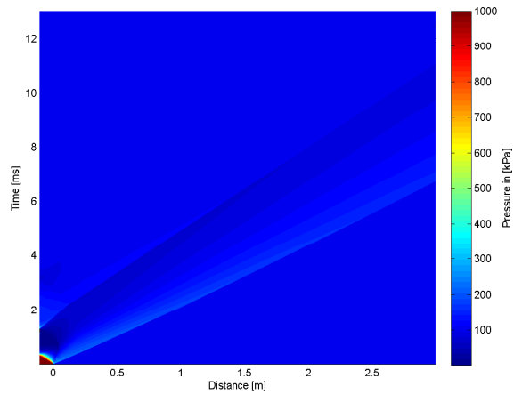
4.41 (b): 75% of Concave Driver and Transition Length 10bar
