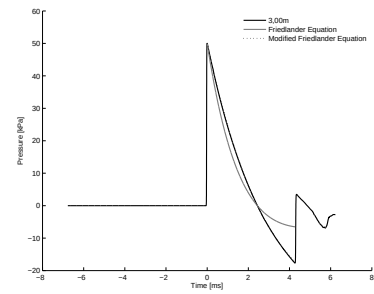
4.40 (f): 75% of Concave Driver and Transition Length 10bar 3.00m
