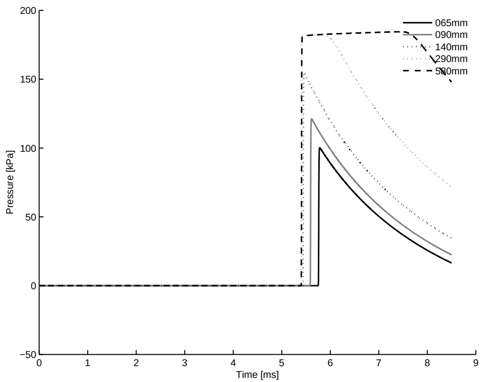
Figure 4.17: The Effect of Driver Length on Pressure
