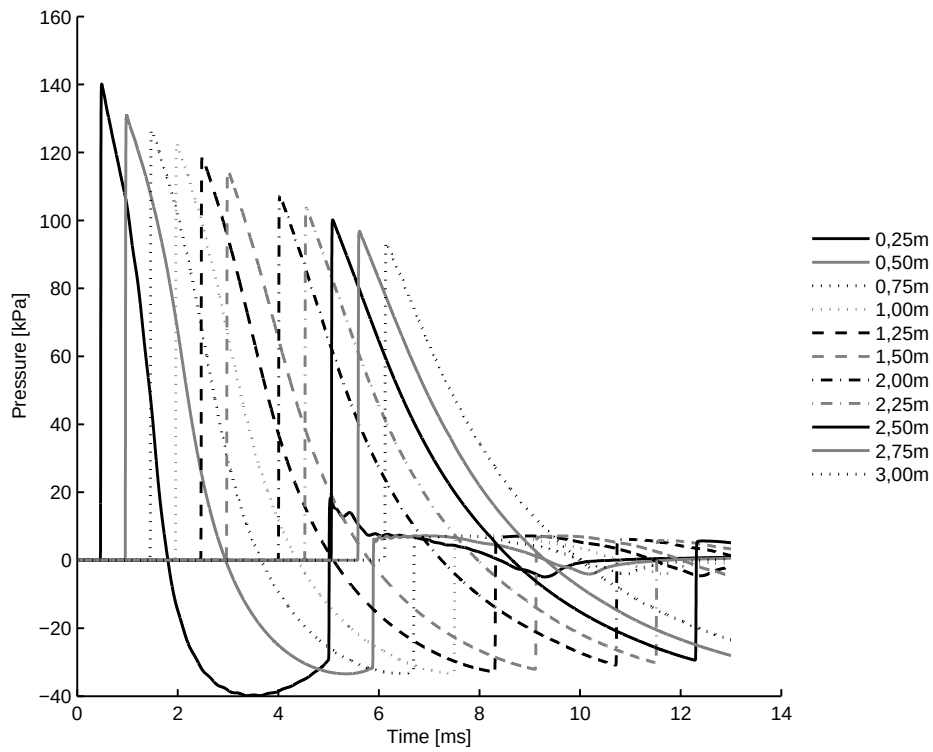
B.1 (d): 125% of Linear Driver and Transition Length 10bar
