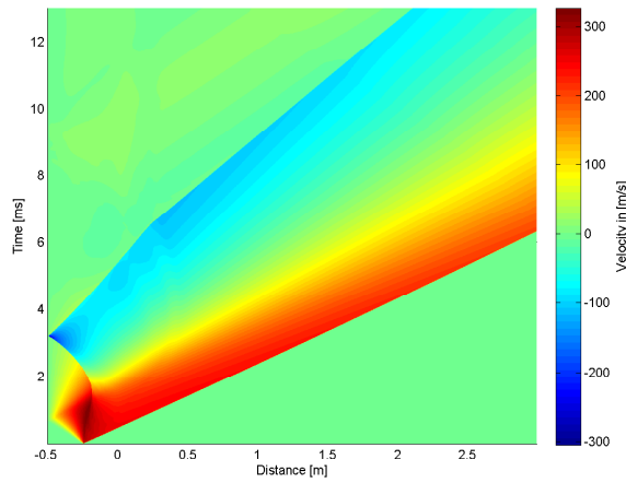
A.7 (c): 50% of Linear Driver Length 10bar
