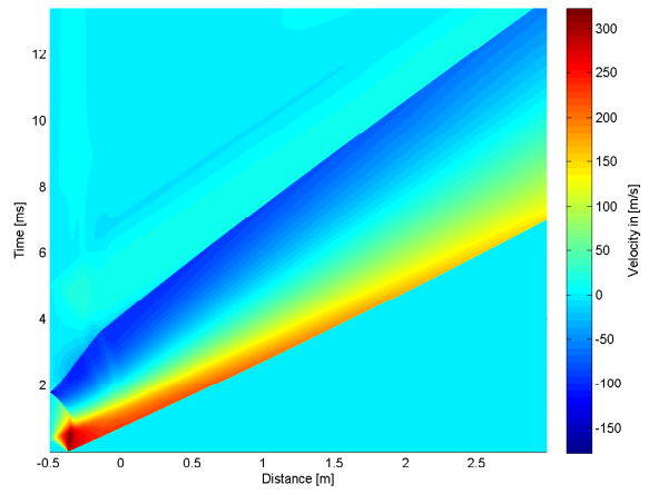
A.14 (d): 25% of Convex Driver Length 10bar
