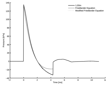
B.10 (d): 75% of Convex Driver and Transition Length 10bar 1.00m
