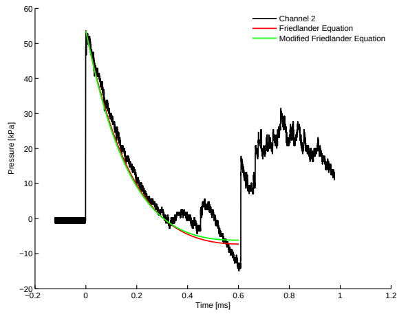
7.2 (i): Convex Profile 50\mu m \approx 500kPa 2.73m
