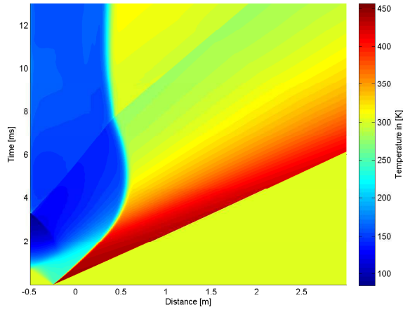
A.13 (c): 50% of Convex Driver Length 10bar
