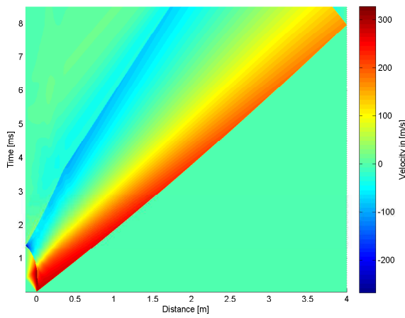
4.12 (c): 30^\circ 10bar
