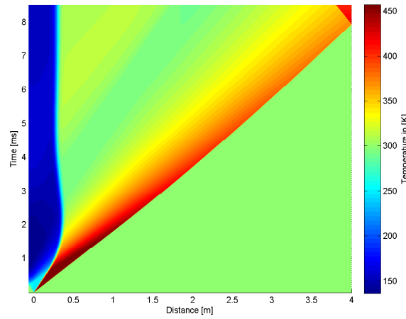
4.23 (e): 65mm 10bar
