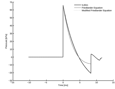
4.49 (f): Linear Profile 10bar 5.00m
