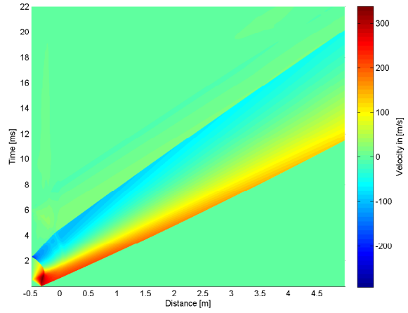
4.54 (b): Linear Profile 10bar
