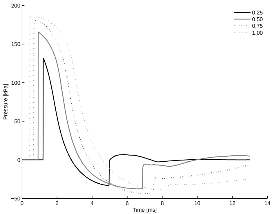
A.9 (a): 0.25m 10bar
