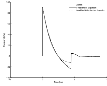
B.10 (b): 50% of Convex Driver and Transition Length 10bar 2.00m
