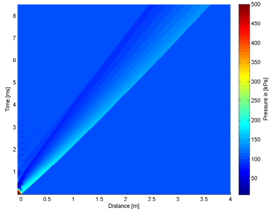
4.14 (a): 60° 5bar Pressure
