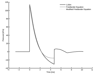
A.10 (j): 25% of Convex Driver Length 10bar 1.00m
