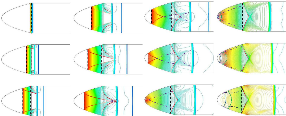
Figure 2.15: The Focusing of Expansion Waves (Whalley (2016))
