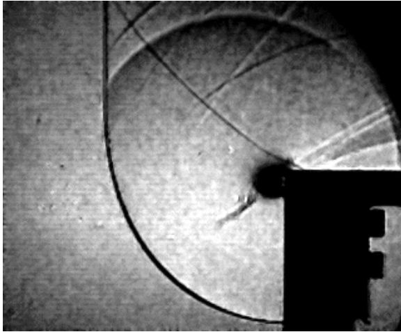
7.5 (e): Convex Profile 50\mu m M_0 = 1.253
