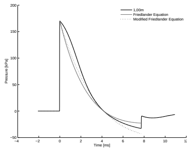
4.33 (d): 75% of Concave Driver Length 10bar 1.00m
