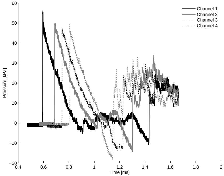
7.1 (b): Linear Profile \approx 600kPa
