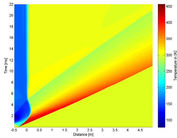
4.53 (c): Convex Profile 10bar
