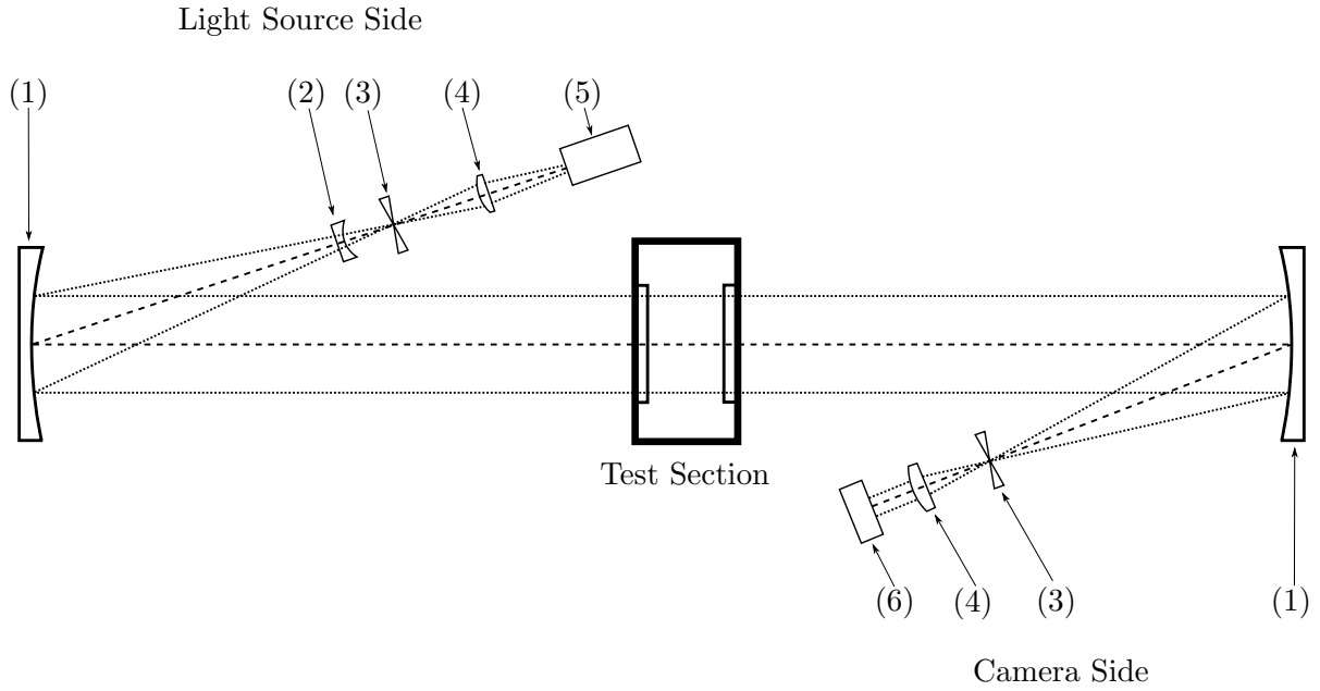
Figure 5.2: Uni-Directional Schlieren Flow Visualisation Set-up
