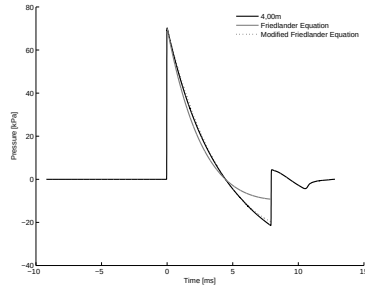
4.49 (e): Concave Profile 10bar 4.00m
