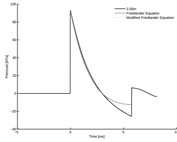
A.10 (k): 25% of Convex Driver Length 10bar 2.00m
