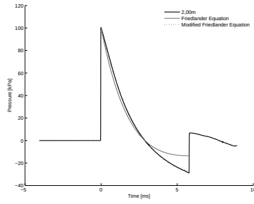
B.3(h): 100% of Linear Driver and Transition Length 10bar 2.00m
