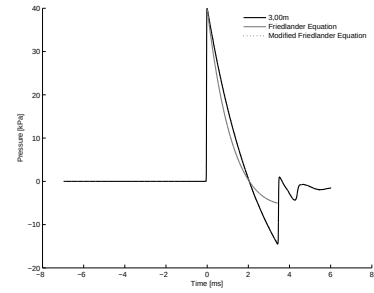
4.40 (c): 50% of Concave Driver and Transition Length 10bar 3.00m
