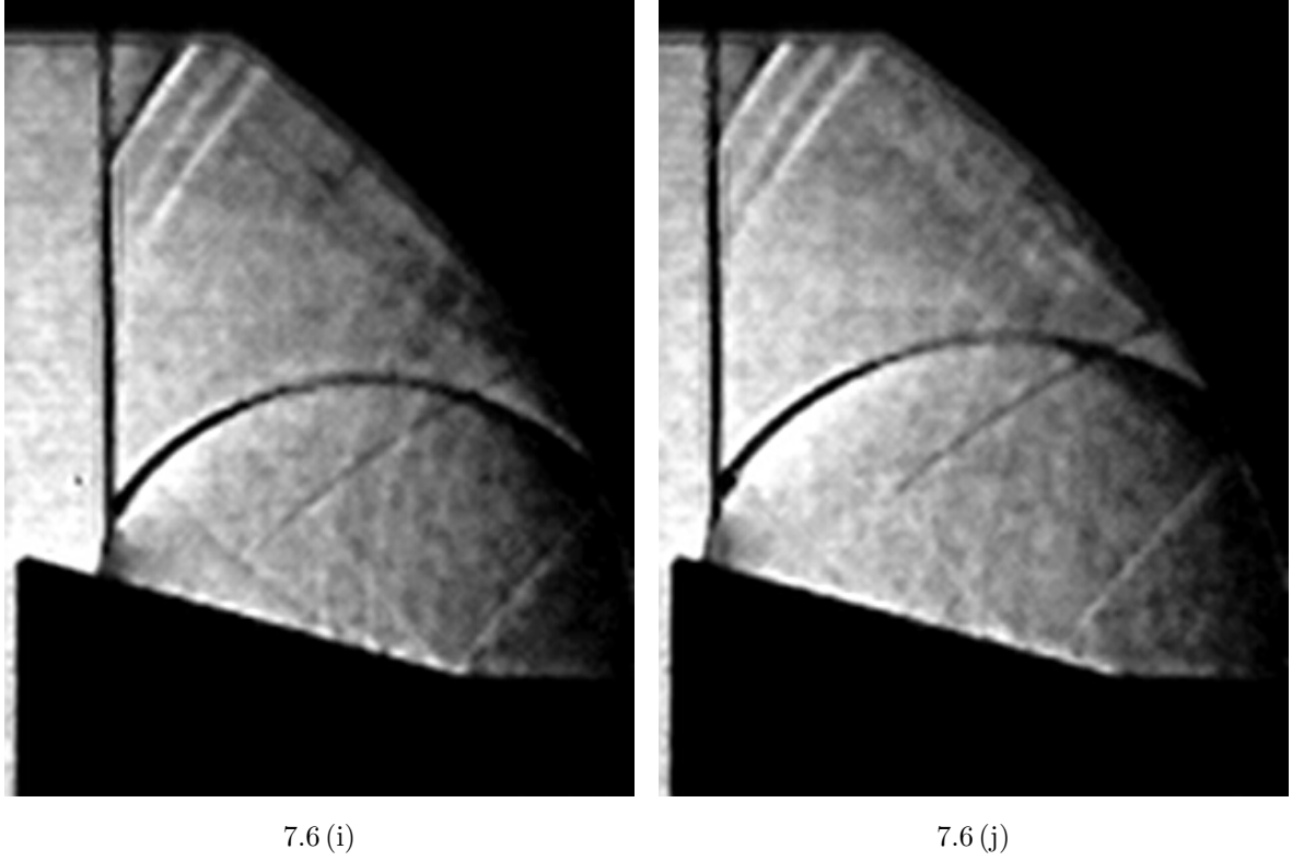
Figure 7.6: Development of a 15° Reflected Blast Wave generated by the Blast Tube having Concave Driver Section 50\mu m M_0 = 1.240
