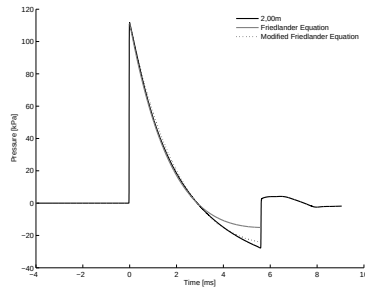
B.10 (e): 75% of Convex Driver and Transition Length 10bar 2.00m
