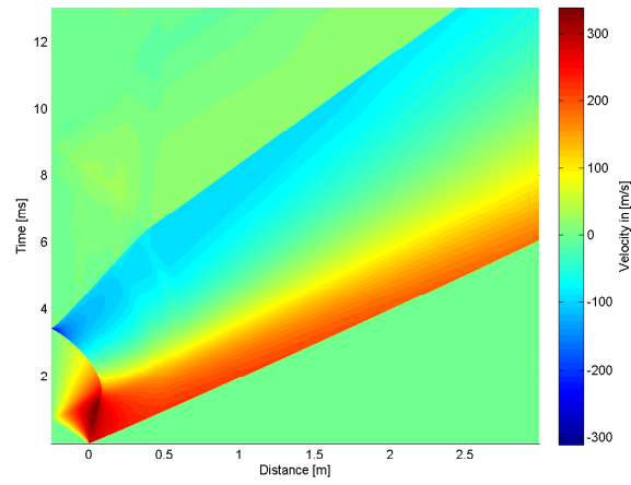
B.7(e): 150% of Linear Driver and Transition Length 10bar
