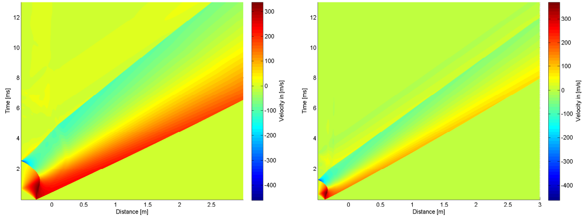
4.37 (c): 50% of Concave Driver Length 10bar
