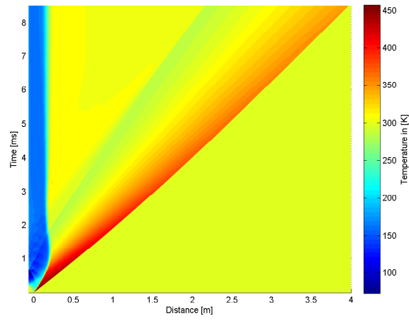
4.11 (e): 60^\circ 10bar
