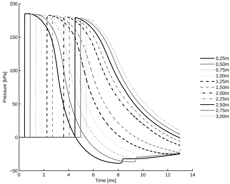
A.8 (a): 100% of Convex Driver Length 10bar
