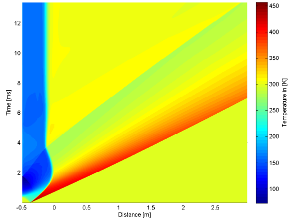
A.13 (d): 25% of Convex Driver Length 10bar
