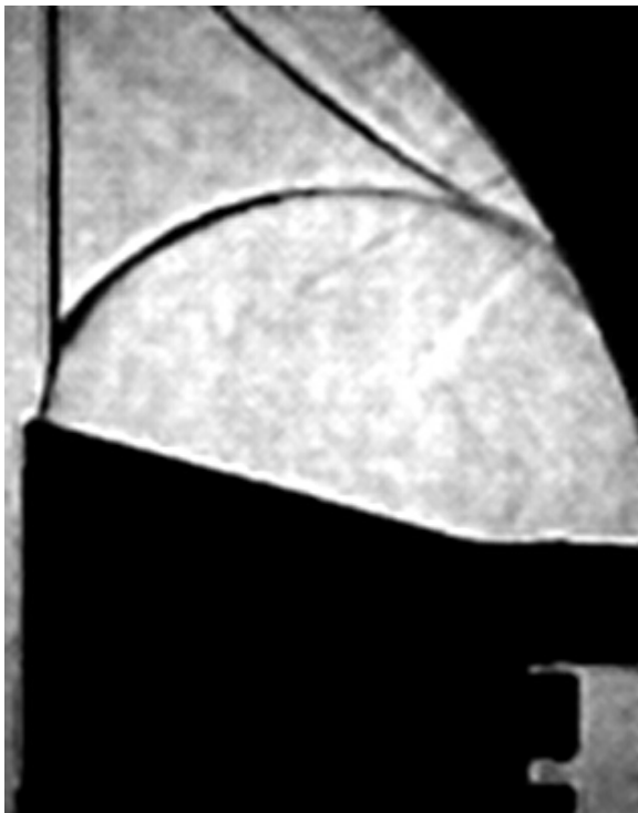
7.7 (c): Linear Profile 50\mu m M_0 = 1.263
