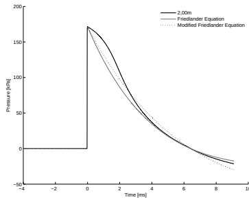
A.10 (e): 75% of Convex Driver Length 10bar 2.00m
