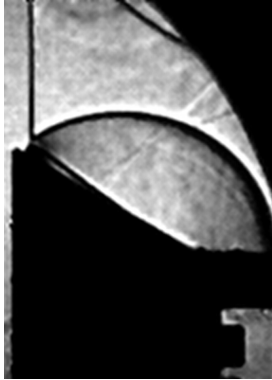
7.9 (d): Linear Profile 100\mu m M_0 = 1.390
