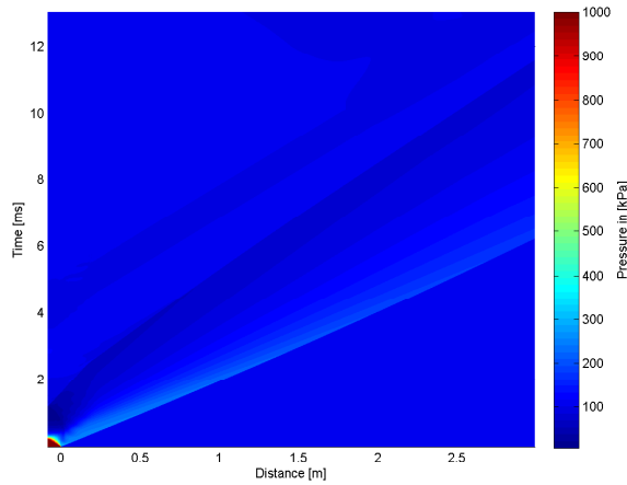
B.11 (a): 50% of Convex Driver and Transition Length 10bar
