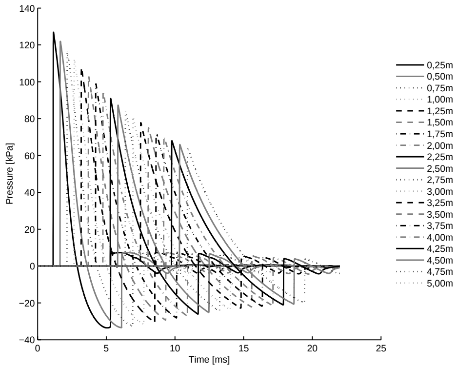
4.47 (b): Linear Profile 10bar
