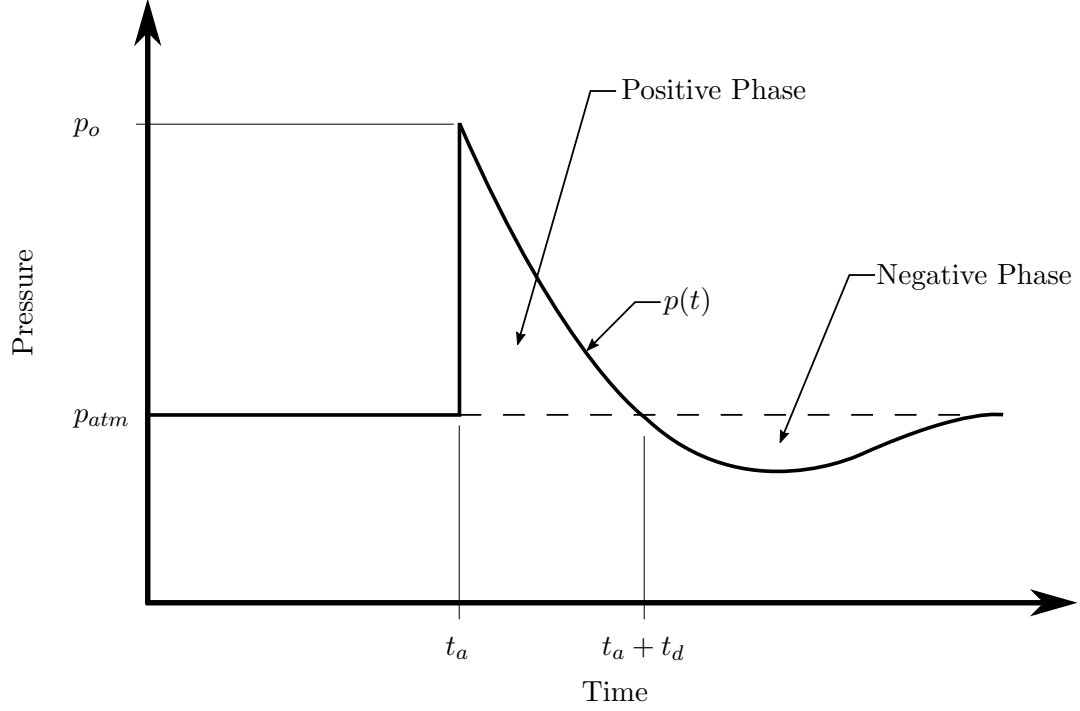
Figure 2.6: Ideal Blast Wave Pressure-Time Curve (Baker (1973))
