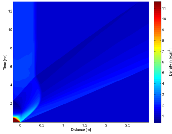
B.12(c): 100% of Convex Driver and Transition Length 10bar
