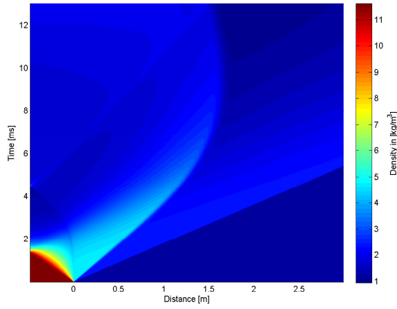
4.35 (a): 100% of Concave Driver Length 10bar
