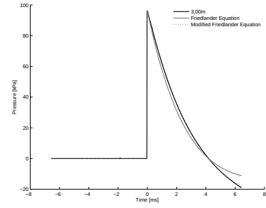
4.33 (i): 50% of Concave Driver Length 10bar 3.00m
