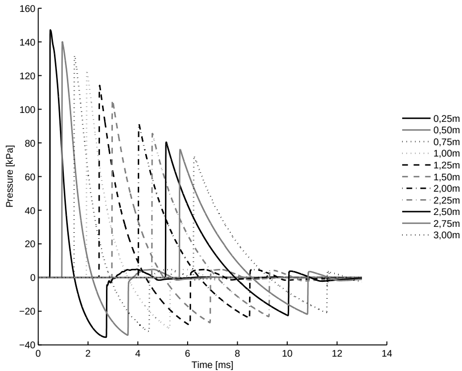
B.8 (a): 50% of Convex Driver and Transition Length 10bar
