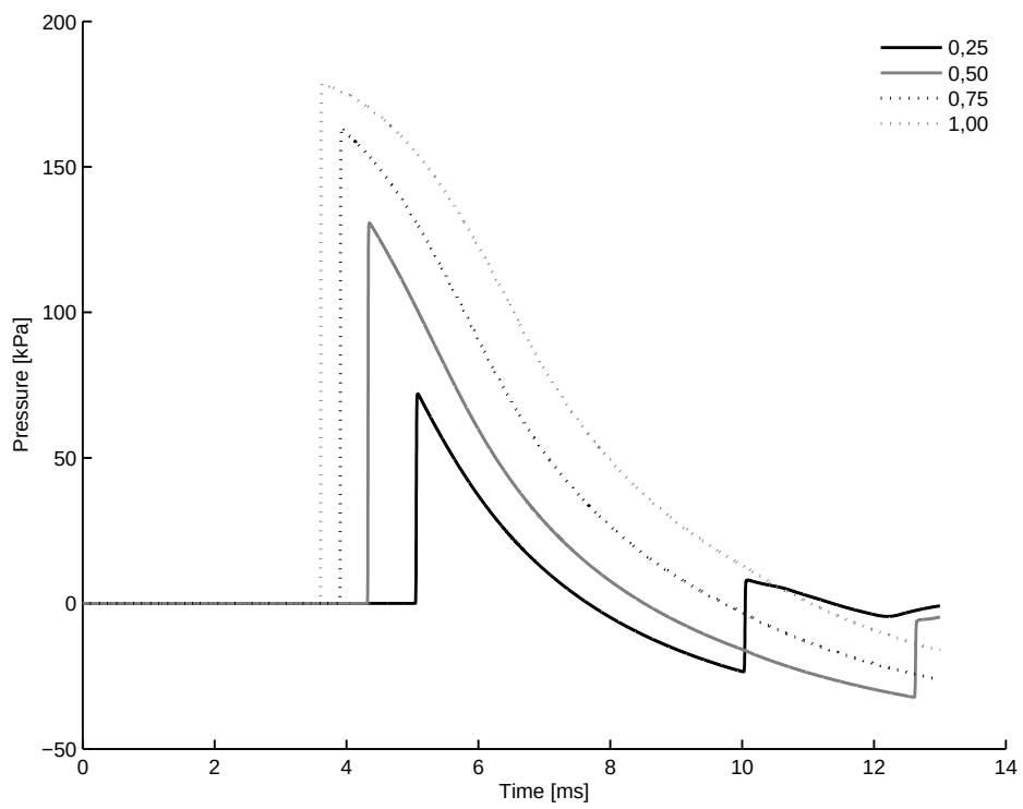
A.2 (c): 2.00m 10bar
