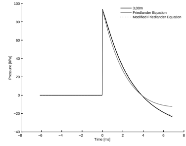
B.3(l): 125% of Linear Driver and Transition Length 10bar 3.00m
