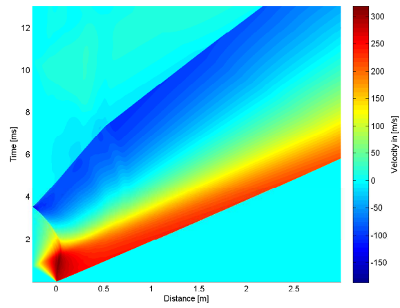
B.14 (e): 150% of Convex Driver and Transition Length 10bar
