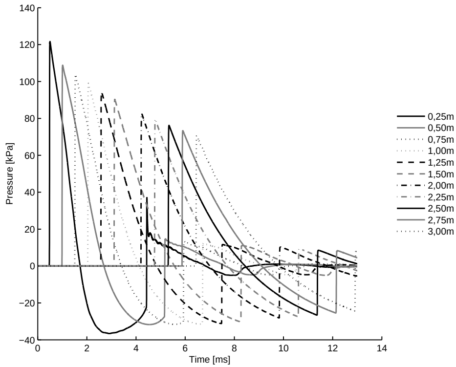
4.38 (e): 150% of Concave Driver and Transition Length 10bar
