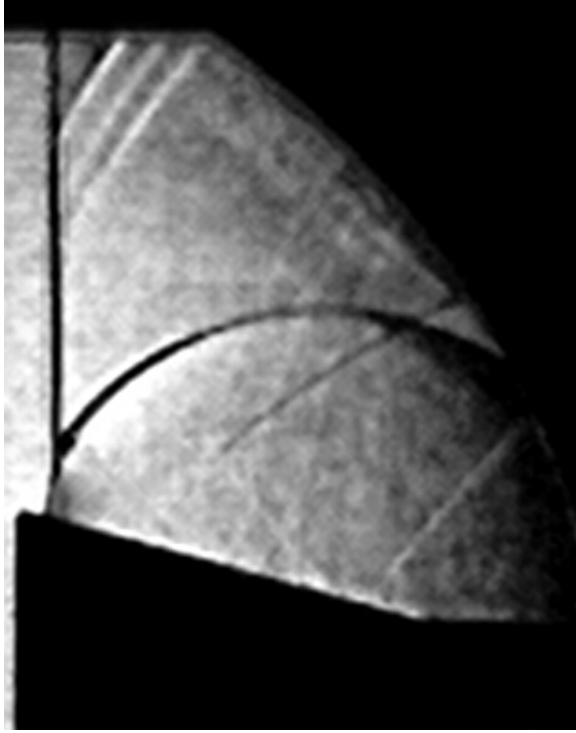
7.7 (a): Concave Profile 50\mu m M_0 = 1.240
