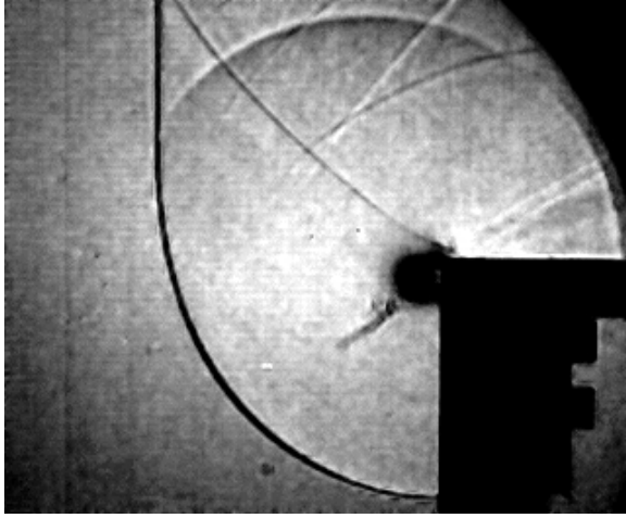
7.5 (a): Concave Profile 50\mu m M_0 = 1.253
