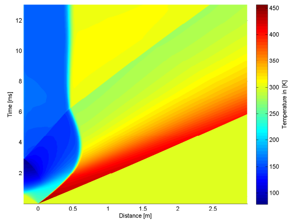
B.13 (d): 125% of Convex Driver and Transition Length 10bar
