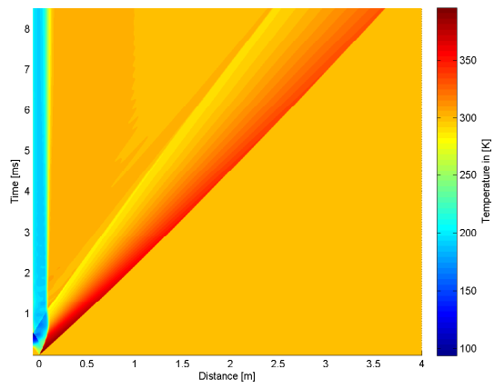
4.14 (b): 60° 5bar Temperature
