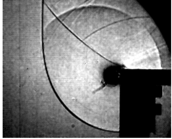
7.5 (b): Concave Profile 100\mu m M_0 = 1.338
