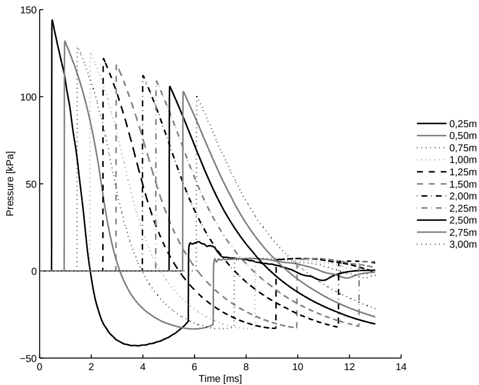
B.1 (e): 150% of Linear Driver and Transition Length 10bar
