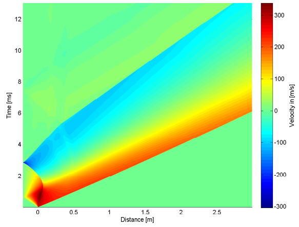
B.7(d): 125% of Linear Driver and Transition Length 10bar
