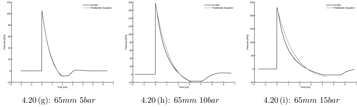
Figure 4.20: Comparing the Effect of Driver Length and Pressure on Friedlander Pressure Profile
