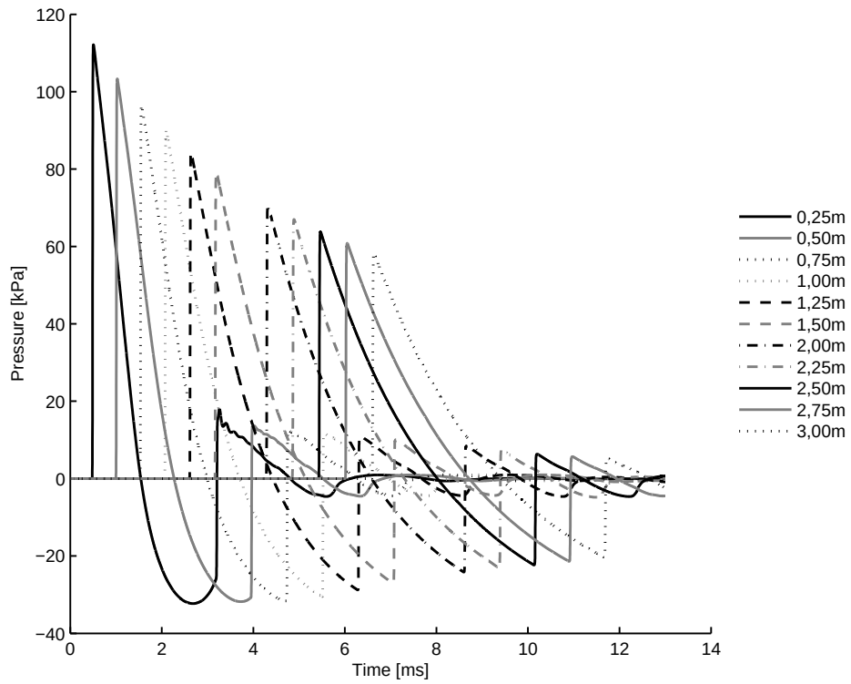
4.38 (c): 100% of Concave Driver and Transition Length 10bar
