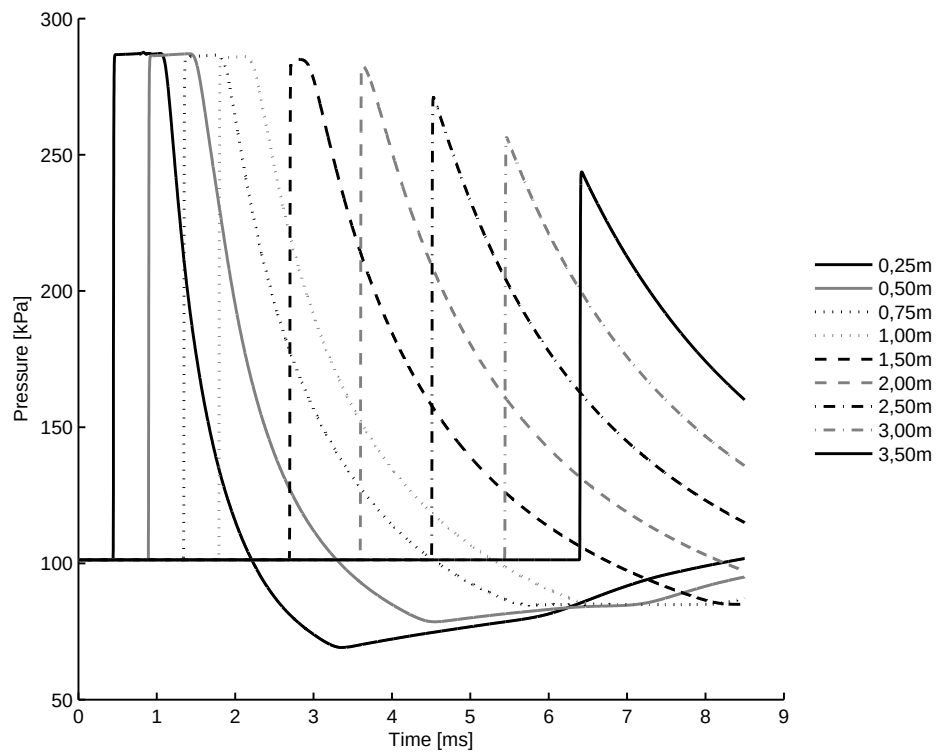
4.19 (c): 140mm 10bar
