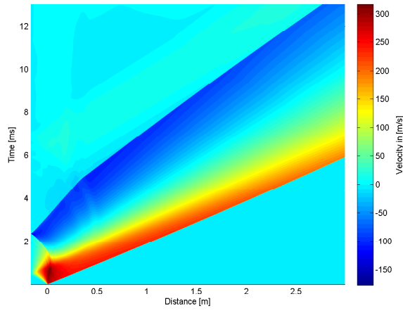
B.14(c): 100% of Concave Driver and Transition Length 10bar
