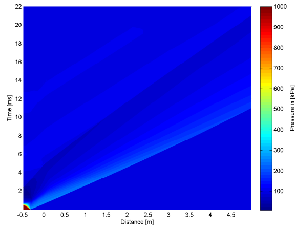
4.51 (c): Convex Profile 10bar
