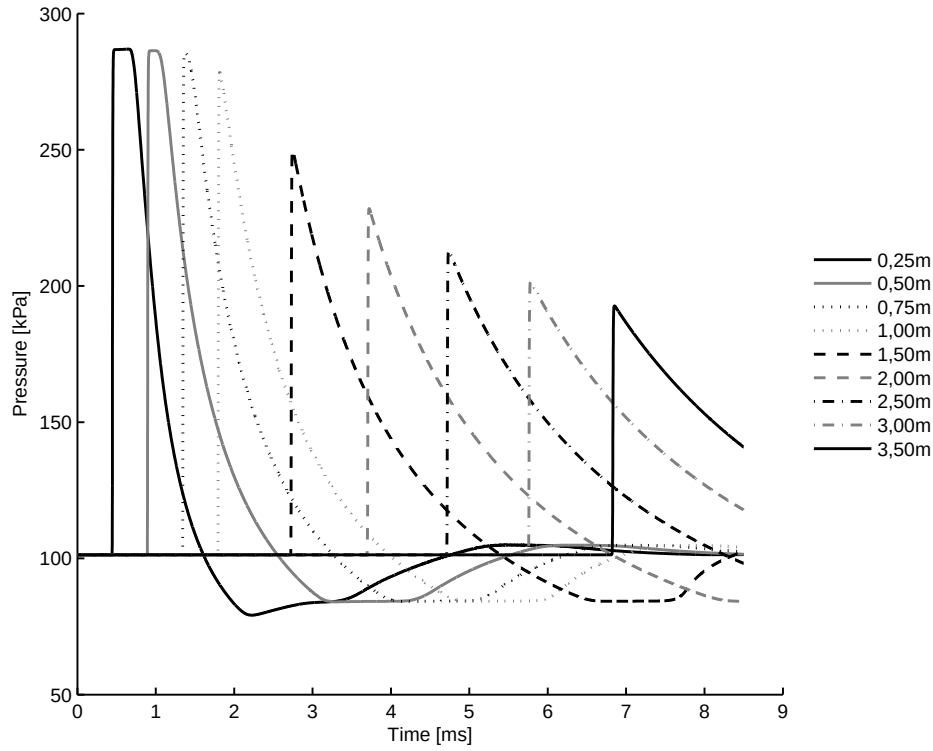
4.19 (e): 65mm 10bar
