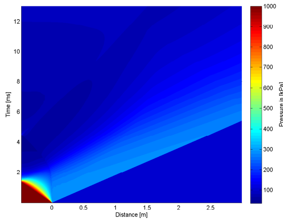
4.34 (a): 100% of Concave Driver Length 10bar
