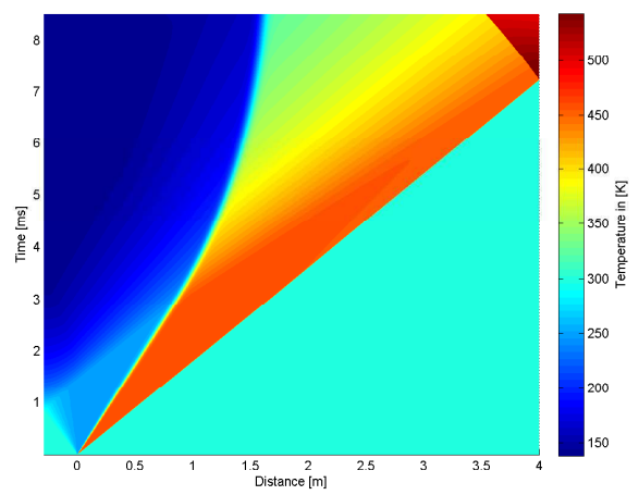
4.23 (b): 290mm 10bar
