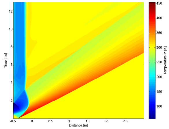
A.6 (d): 25% of Linear Driver Length 10bar
