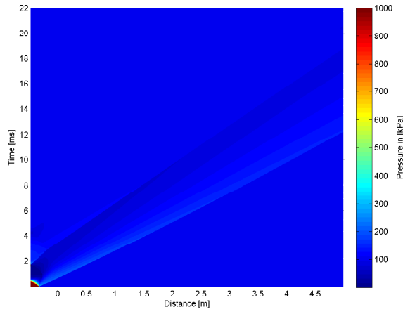
4.51 (a): Concave Profile 10bar
