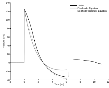
B.3(m): 150% of Linear Driver and Transition Length 10bar 1.00m
