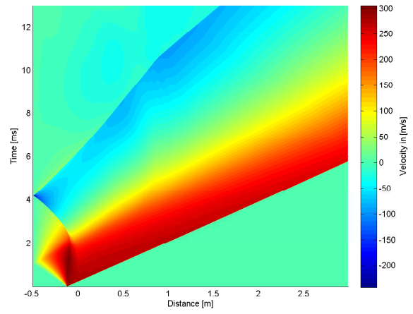
A.7 (b): 75% of Linear Driver Length 10bar
