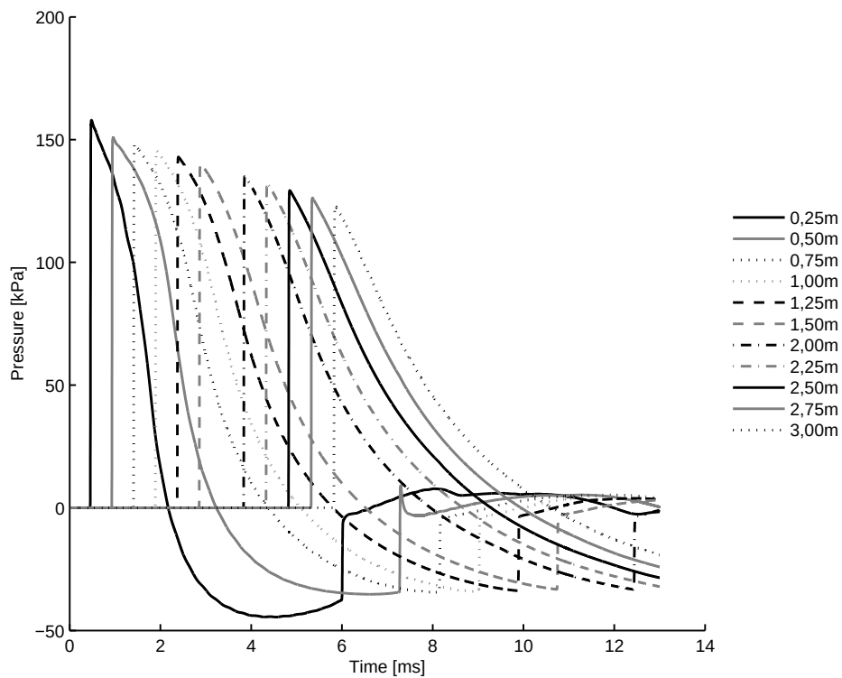
B.8 (e): 150% of Convex Driver and Transition Length 10bar
