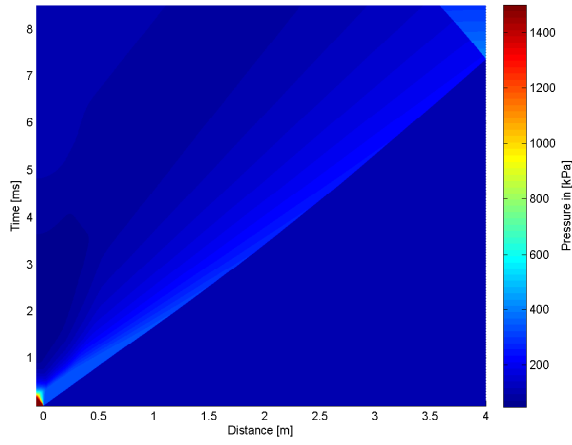
4.28 (a): 65mm 15bar Pressure
