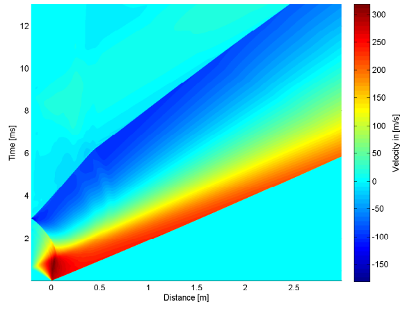
B.14(d): 125% of Convex Driver and Transition Length 10bar
