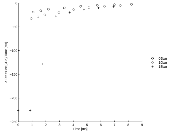
4.6 (b): Rate of Change of Peak Overpressure with Regards to Time
