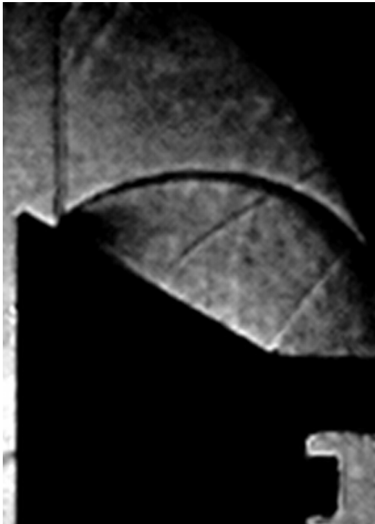
7.9 (e): Convex Profile 50\mu m M_0 = 1.239
