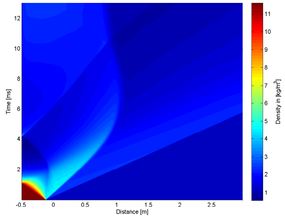
A.5 (b): 75% of Linear Driver Length 10bar
