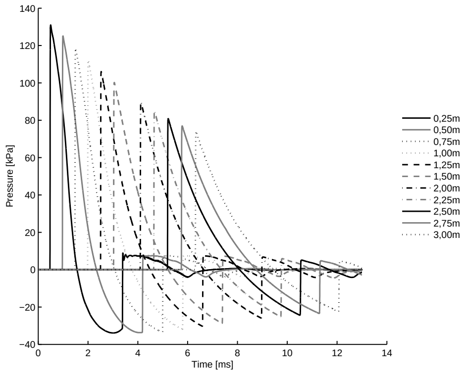
B.1 (b): 75% of Linear Driver and Transition Length 10bar
