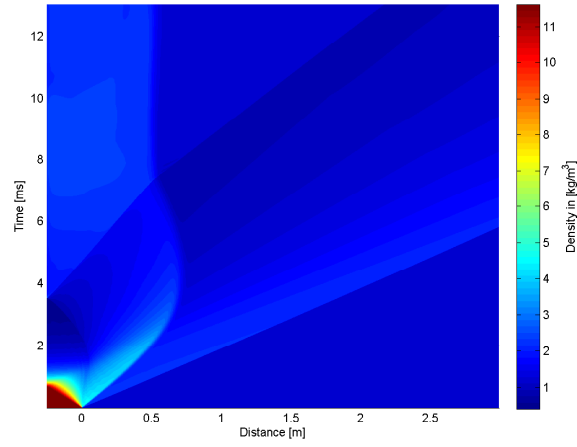
B.12 (e): 150% of Convex Driver and Transition Length 10bar
