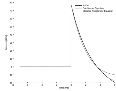
A.10 (l): 25% of Convex Driver Length 10bar 3.00m
