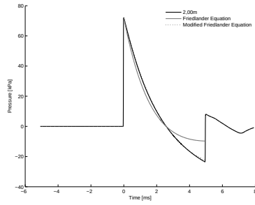
A.3(k): 25% of Linear Driver Length 10bar 2.00m
