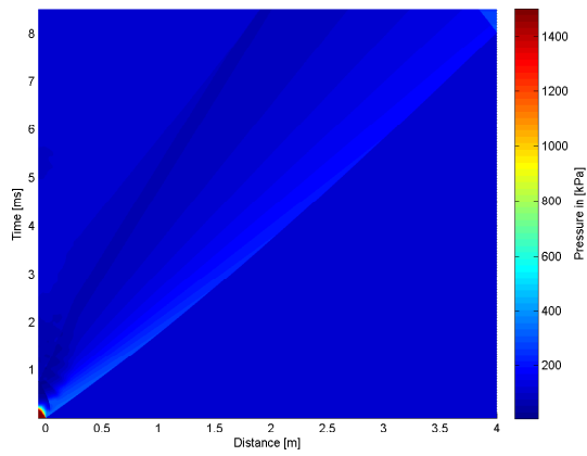
4.16 (a): 60° 15bar Pressure
