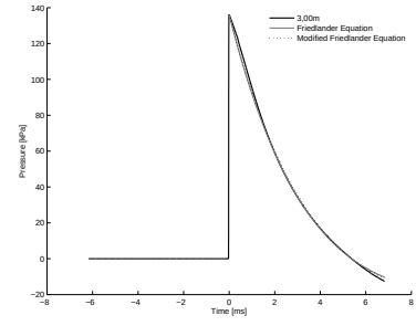
A.10 (i): 50% of Convex Driver Length 10bar 3.00m
