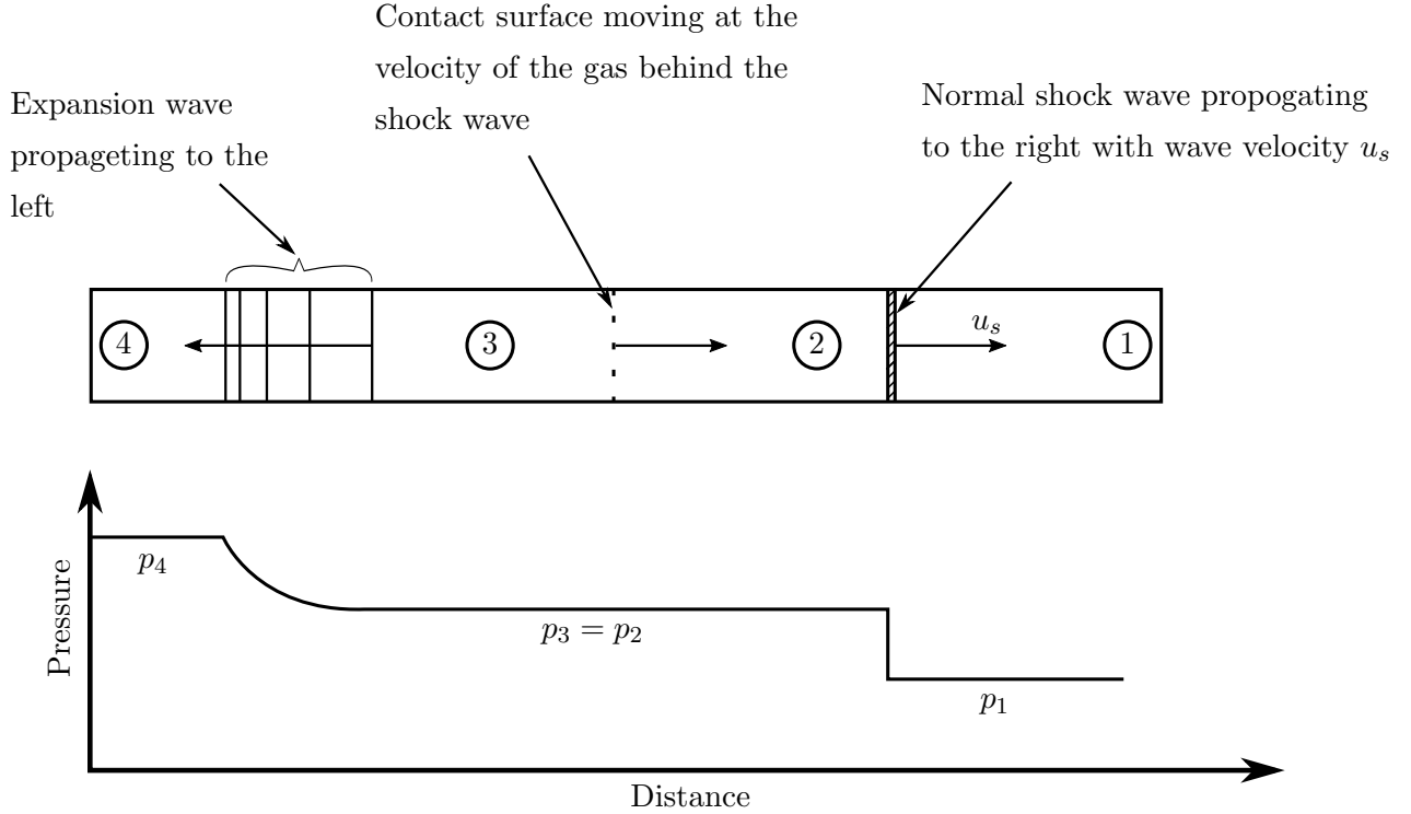
Figure 2.8: Conditions in Shock Tube after Diaphragm is Broken (Anderson (1990))
