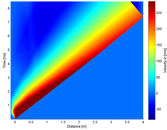
4.24 (c): 140mm 10bar
