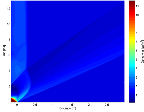
B.5 (c): 100% of Linear Driver and Transition Length 10bar
