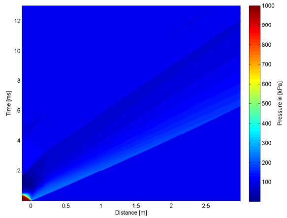
B.4(b): 75% of Linear Driver and Transition Length 10bar
