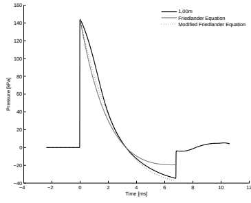
A.3(g): 50% of Linear Driver Length 10bar 1.00m
