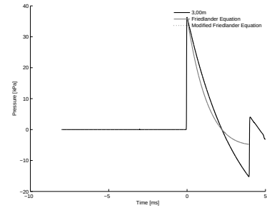
4.33 (l): 25% of Concave Driver Length 10bar 3.00m
