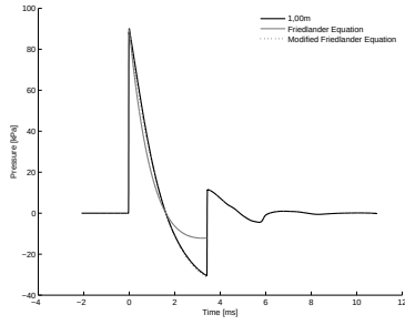
4.40 (g): 100% of Concave Driver and Transition Length 10bar 1.00m
