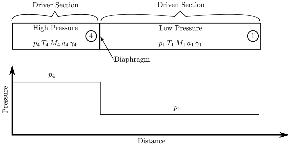
Figure 2.7: Initial Conditions of a Gas Driven Shock Tube (Anderson (1990))
