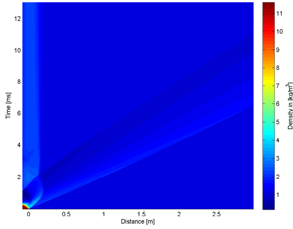
B.5 (a): 50% of Linear Driver and Transition Length 10bar
