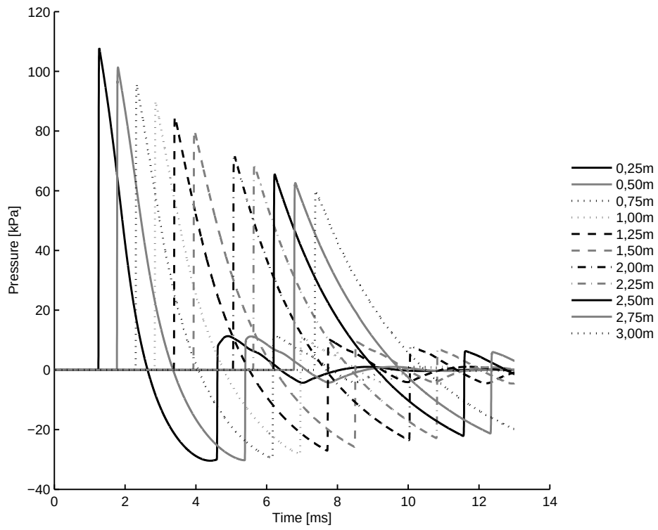
A.1 (d): 25% of Linear Driver Length 10bar
