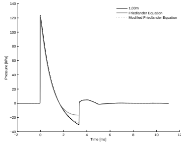
B.10 (a): 50% of Convex Driver and Transition Length 10bar 1.00m
