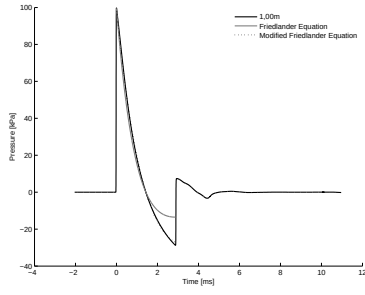
B.3(a): 50% of Linear Driver and Transition Length 10bar 1.00m
