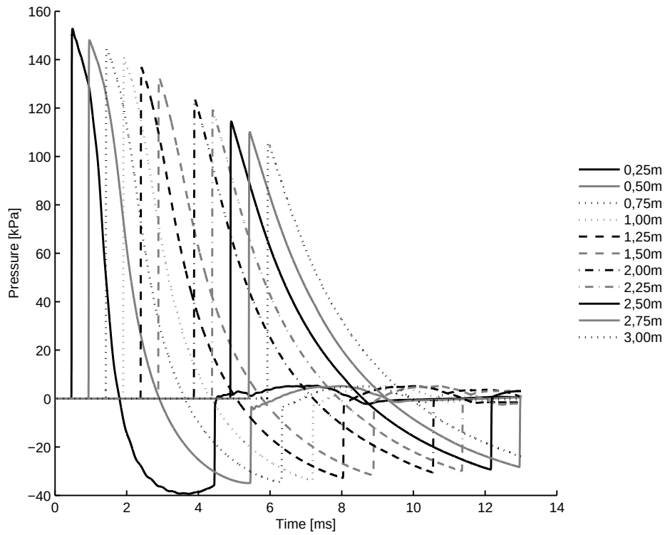
B.8 (c): 100% of Convex Driver and Transition Length 10bar
