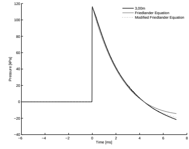
B.10 (l): 125% of Convex Driver and Transition Length 10bar 3.00m
