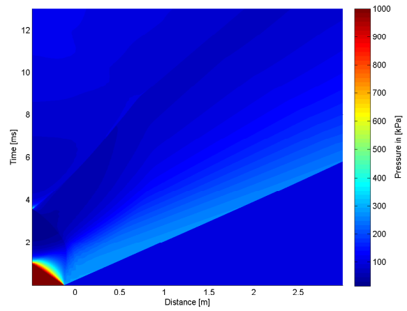
4.34 (b): 75% of Concave Driver Length 10bar
