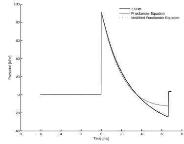
B.10 (f): 75% of Convex Driver and Transition Length 10bar 3.00m
