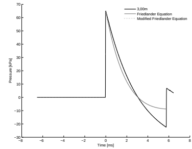
4.40 (l): 125% of Concave Driver and Transition Length 10bar 3.00m
