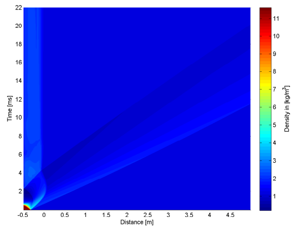
4.52 (b): Linear Profile 10bar
