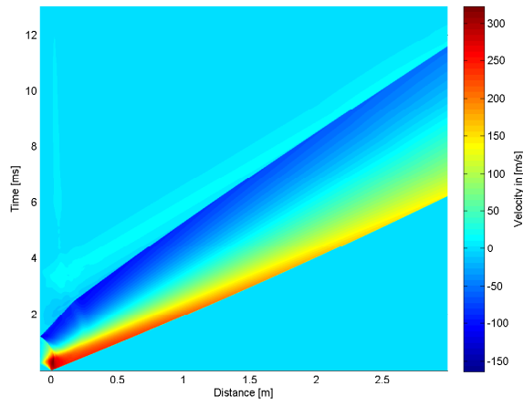
B.14(a): 50% of Convex Driver and Transition Length 10bar
