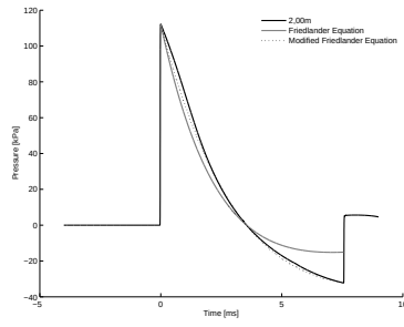
B.3(n): 150% of Linear Driver and Transition Length 10bar 2.00m
