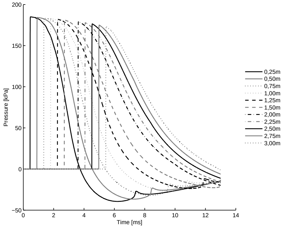
4.31 (a): 100% of Concave Driver Length 10bar
