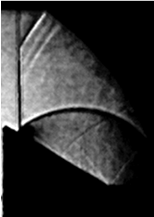
7.9 (a): Concave Profile 50\mu m M_0 = 1.265
