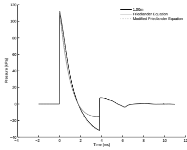
B.3(d): 75% of Linear Driver and Transition Length 10bar 1.00m
