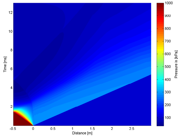
A.4(a): 100% of Linear Driver Length 10bar
