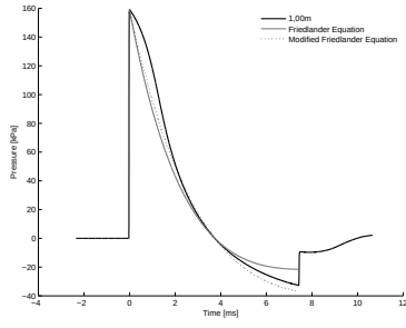
A.10 (g): 50% of Convex Driver Length 10bar 1.00m
