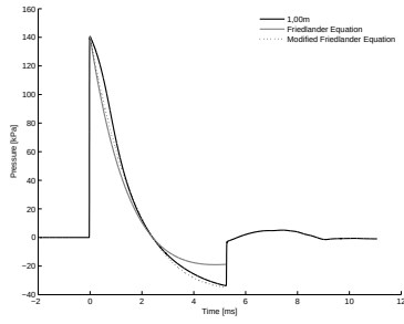
B.10 (g): 100% of Convex Driver and Transition Length 10bar 1.00m
