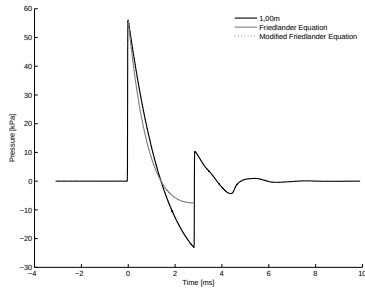
4.33 (j): 25% of Concave Driver Length 10bar 1.00m
