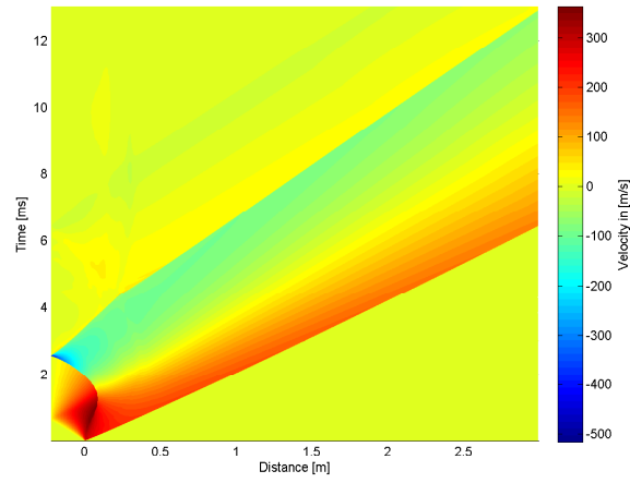
4.44 (e): 150% of Concave Driver and Transition Length 10bar
