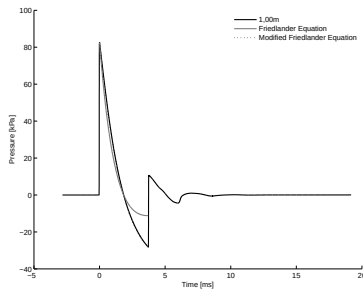
4.48 (b): Concave Profile 10\text{bar} 1.00\text{m}
