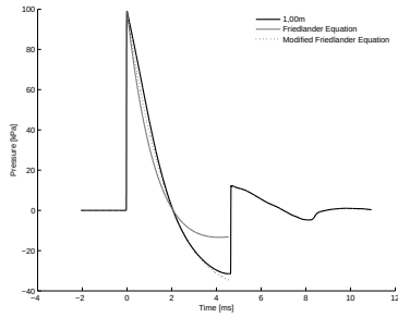
4.40 (m): 150% of Concave Driver and Transition Length 10bar 1.00m
