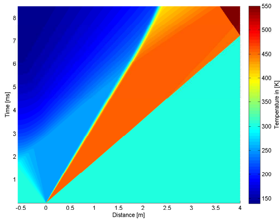
4.23 (a): 580mm 10bar
