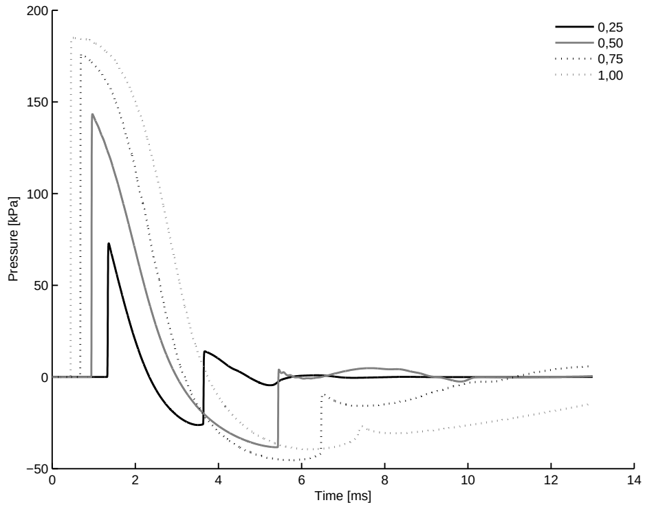
4.32 (a): 0.25m 10bar
