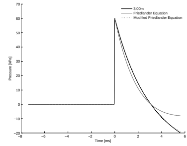
A.3(l): 25% of Linear Driver Length 10bar 3.00m
