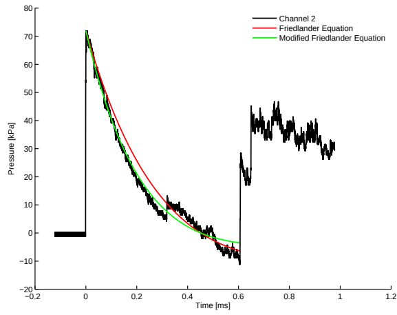
7.2 (g): Linear Profile 100\mu m \approx 1000kPa 2.73m
