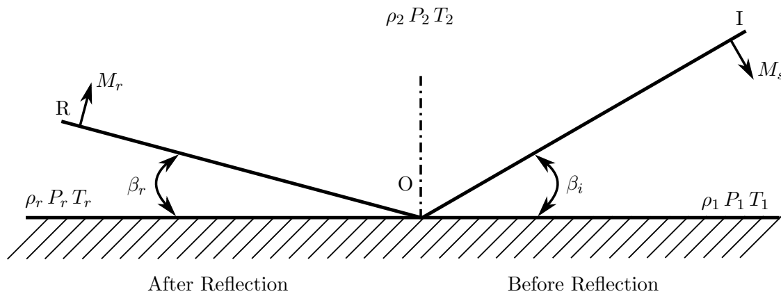
Figure 2.10: Normal Oblique Reflection (Kinney (1962))
