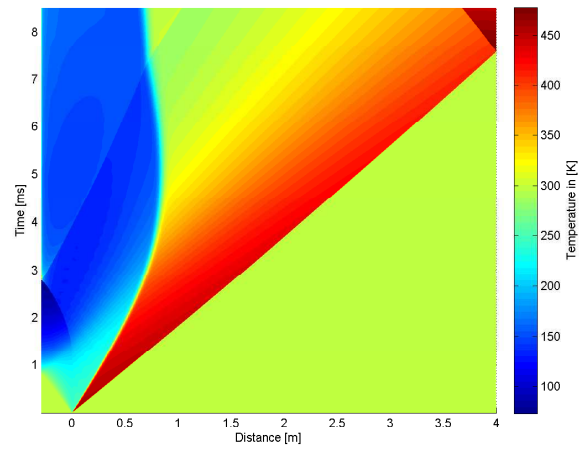
4.11 (b): 15^\circ 10bar
