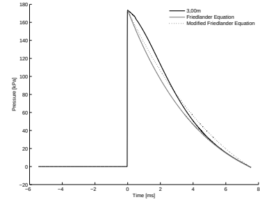
4.33 (c): 100% of Concave Driver Length 10bar 3.00m
