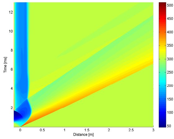
4.43 (c): 100% of Concave Driver and Transition Length 10\bar{b}ar
