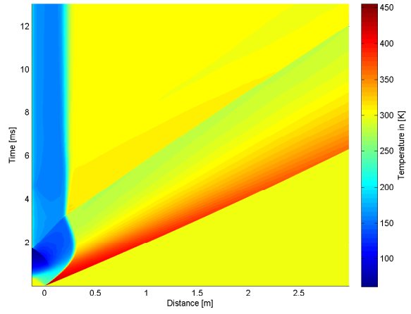
B.6 (b): 75% of Linear Driver and Transition Length 10bar
