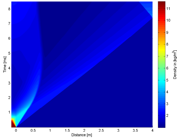
4.22 (c): 140mm 10bar
