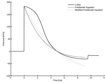
A.3 (a): 100% of Linear Driver Length 10bar 1.00m
