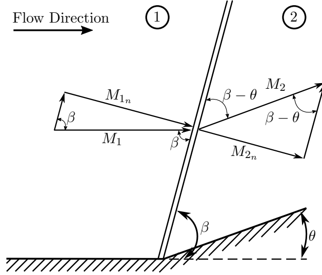
Figure 2.4: Transformation of an Oblique Shock to a Normal Shock (Anderson (1990))
