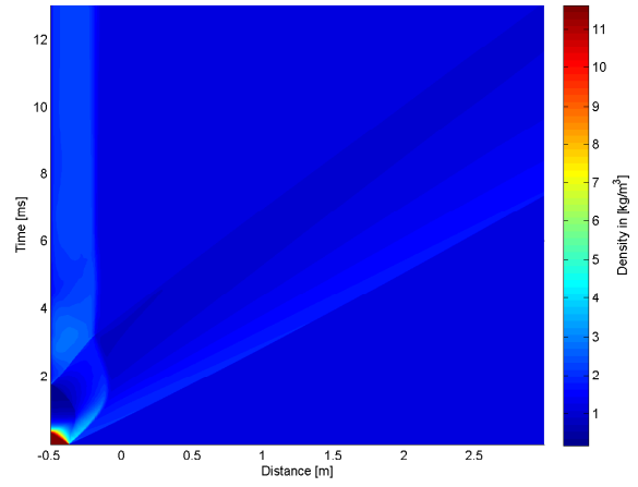
A.5 (d): 25% of Linear Driver Length 10bar
