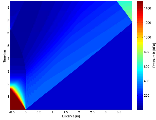
4.15 (a): 7.5° 15bar Pressure
