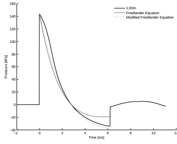
B.10 (j): 125% of Convex Driver and Transition Length 10bar 1.00m
