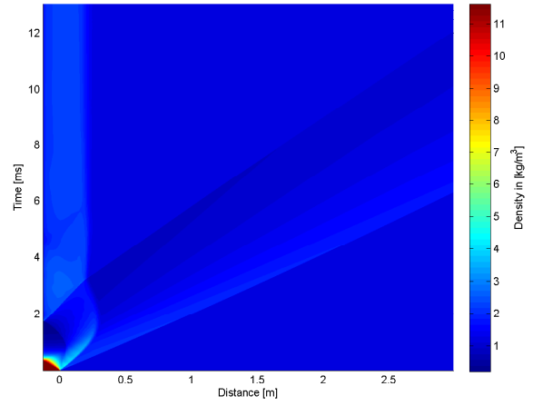
B.5 (b): 75% of Linear Driver and Transition Length 10bar
