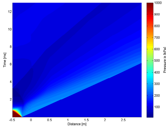
A.11 (c): 50% of Convex Driver Length 10bar
