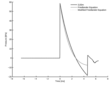
B.3(c): 50% of Linear Driver and Transition Length 10bar 3.00m
