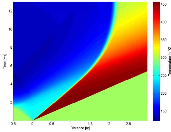
A.13 (a): 100% of Convex Driver Length 10bar
