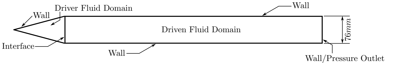
Figure 4.1: The Computational Geometry Configuration
