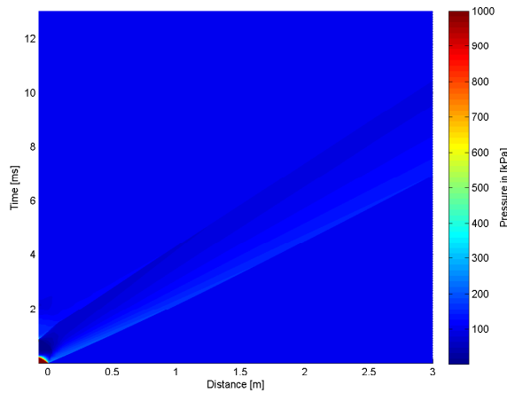
4.41 (a): 50% of Concave Driver and Transition Length 10bar
