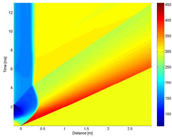
B.6 (c): 100% of Linear Driver and Transition Length 10bar
