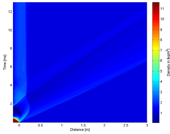
4.42 (c): 100% of Concave Driver and Transition Length 10bar
