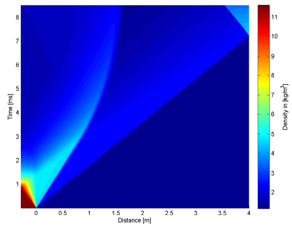
4.22 (b): 290mm 10bar
