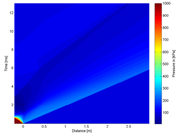
B.11 (d): 125% of Convex Driver and Transition Length 10bar
