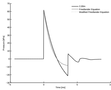
4.40 (e): 75% of Concave Driver and Transition Length 10bar 2.00m
