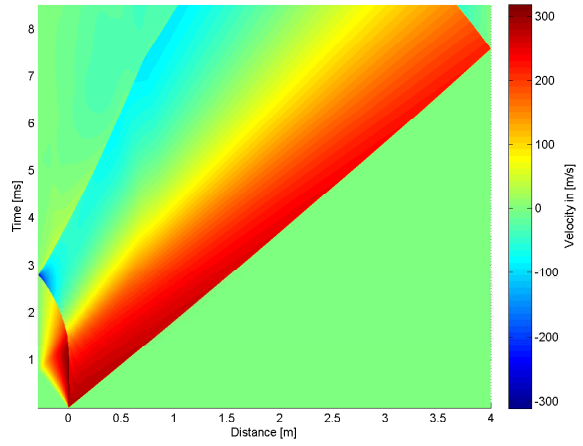
4.12 (b): 15^\circ 10bar
