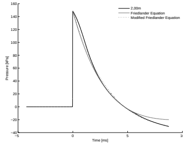
A.10 (h): 50% of Convex Driver Length 10bar 2.00m
