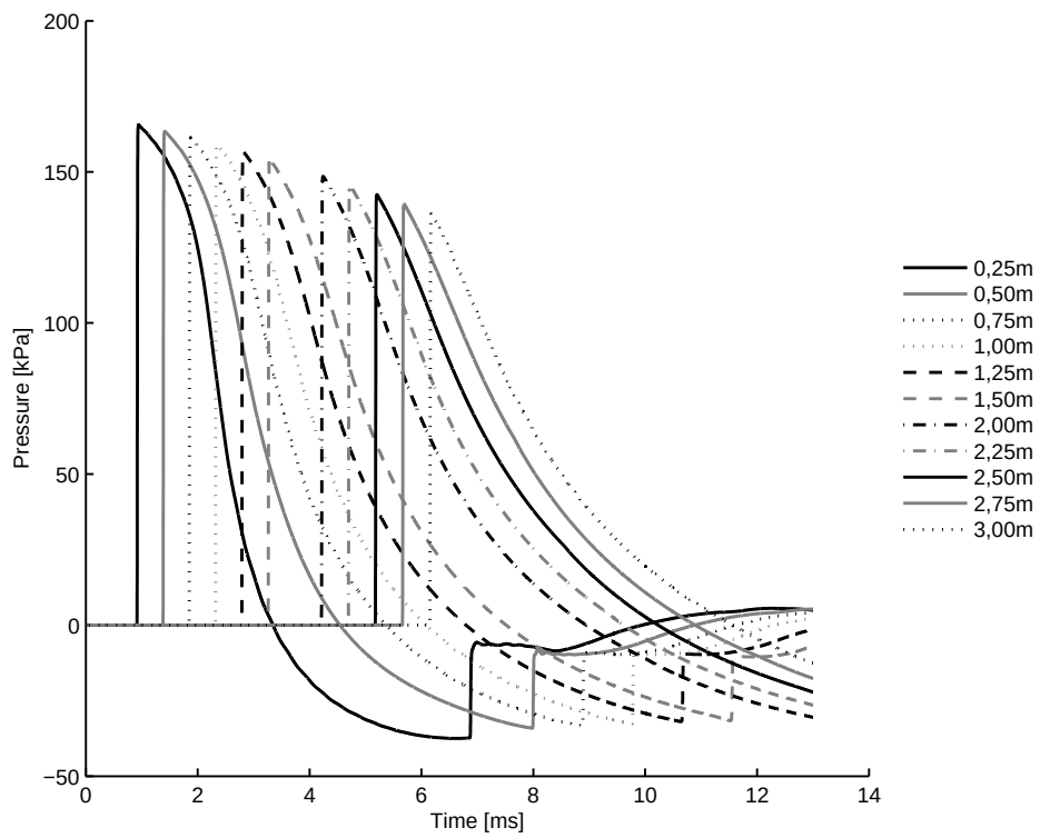
A.8 (c): 50% of Convex Driver Length 10bar
