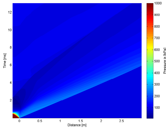
B.11 (c): 100% of Convex Driver and Transition Length 10bar
