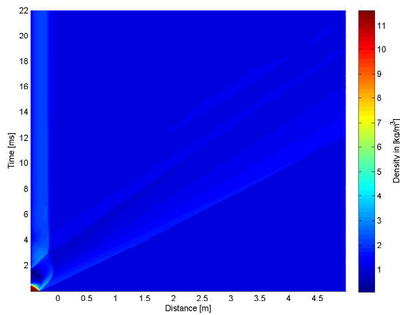
4.52 (a): Concave Profile 10bar
