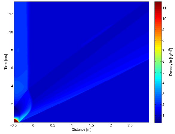
A.12 (d): 25% of Convex Driver Length 10bar
