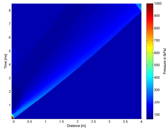
4.21 (e): 65mm 10bar
