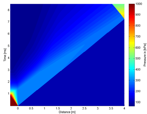
4.21 (b): 290mm 10bar
