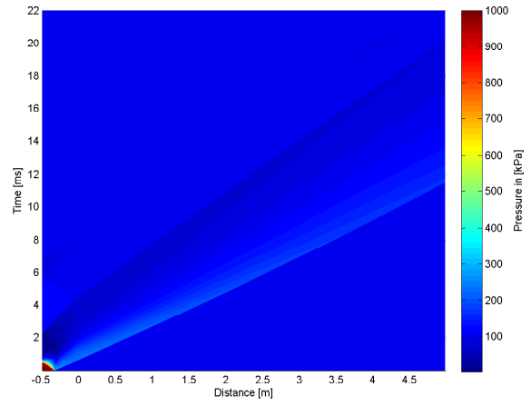
4.51 (b): Linear Profile 10bar
