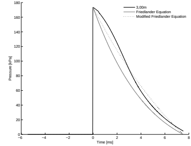
A.3 (c): 100% of Linear Driver Length 10bar 3.00m
