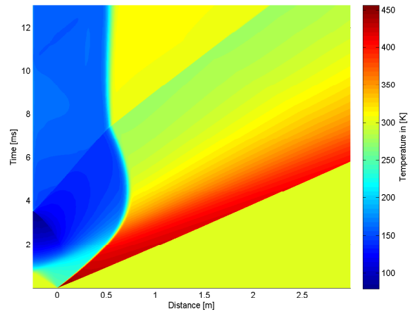
B.13 (e): 150% of Concave Driver and Transition Length 10bar
