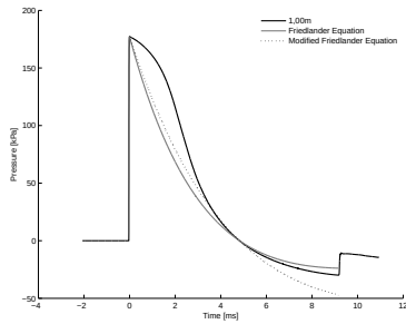
A.10 (d): 75% of Convex Driver Length 10bar 1.00m
