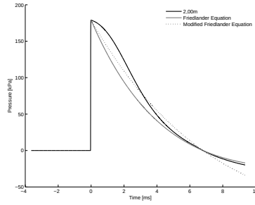
4.33 (b): 100% of Concave Driver Length 10bar 2.00m
