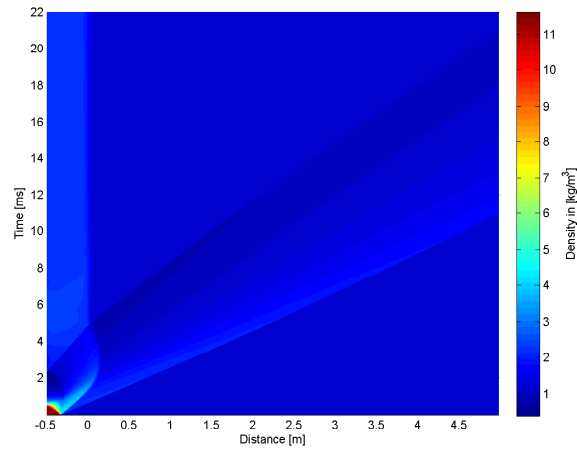
4.52 (c): Convex Profile 10bar
