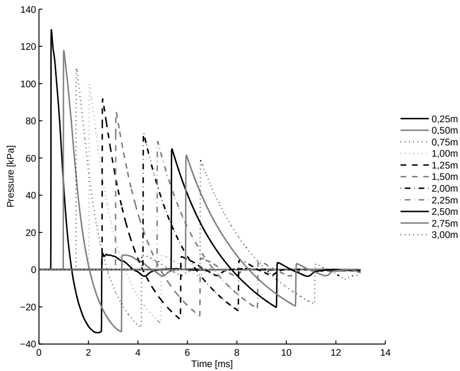
B.1 (a): 50% of Linear Driver and Transition Length 10bar
