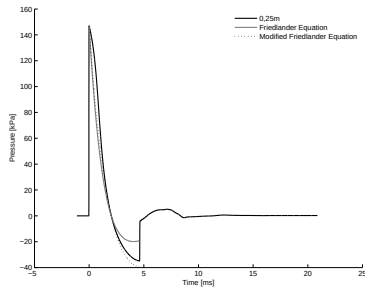
4.50 (a): Convex Profile 10bar 0.25m
