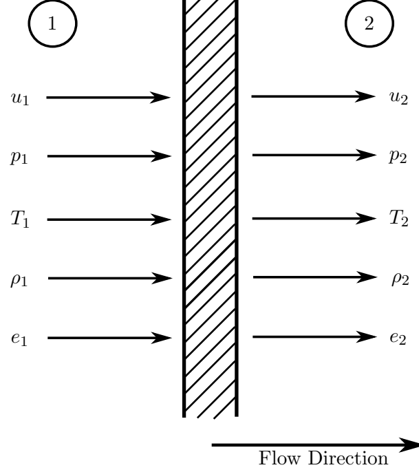
Figure 2.1: Normal Shock Wave Properties adapted from (Anderson (1990))
