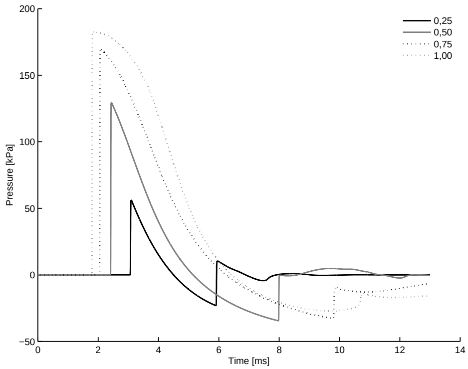
4.32 (b): 1.00m 10bar
