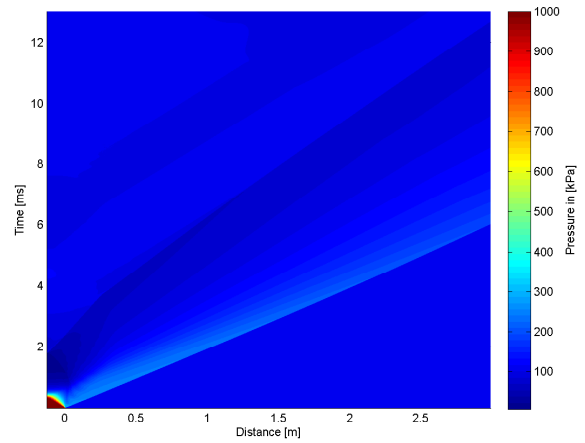
B.11 (b): 75% of Convex Driver and Transition Length 10bar
