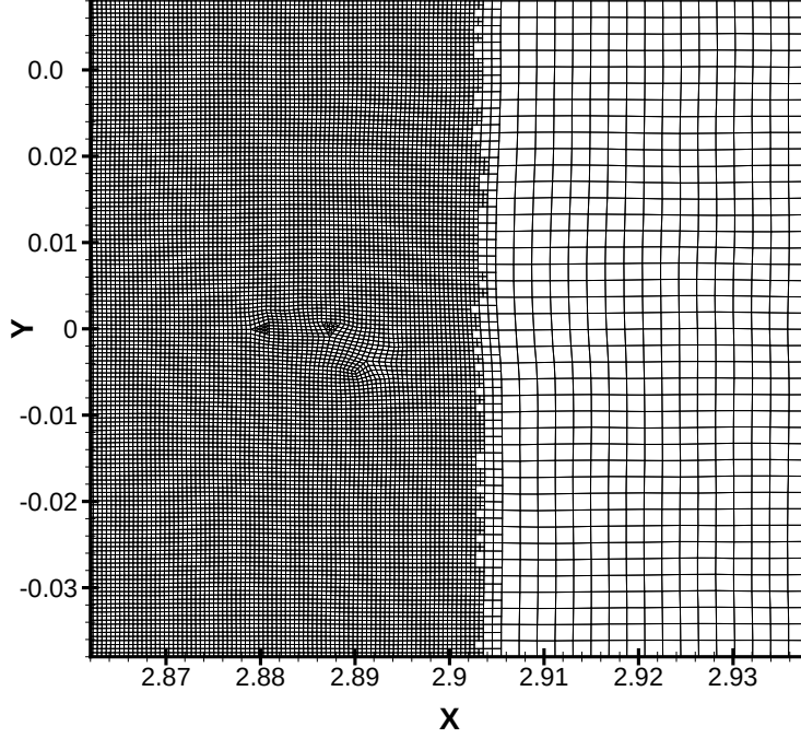
Figure 4.2: Refined Mesh in the Vicinity of the Shock Front
