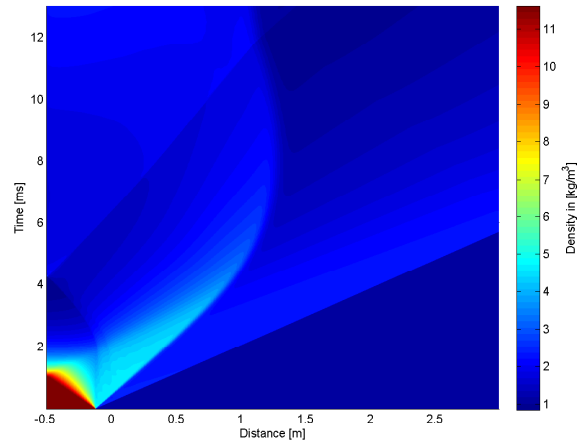
A.12 (b): 75% of Convex Driver Length 10bar
