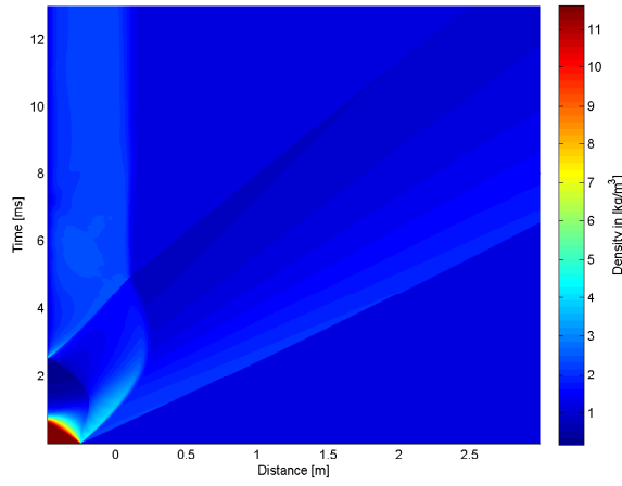
4.35 (c): 50% of Concave Driver Length 10bar
