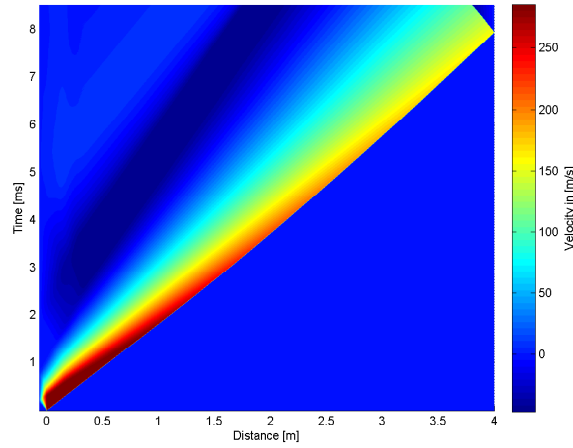
4.24 (e): 65mm 10bar
