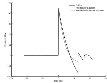
4.48 (f): Concave Profile 10\text{bar} 5.00\text{m}
