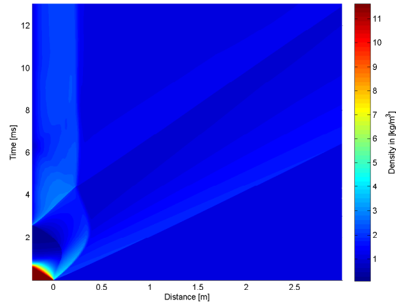
4.42 (e): 150% of Concave Driver and Transition Length 10bar
