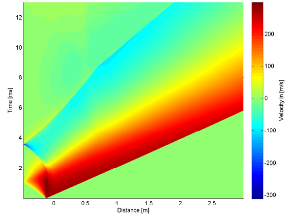
4.37 (b): 75% of Concave Driver Length 10bar
