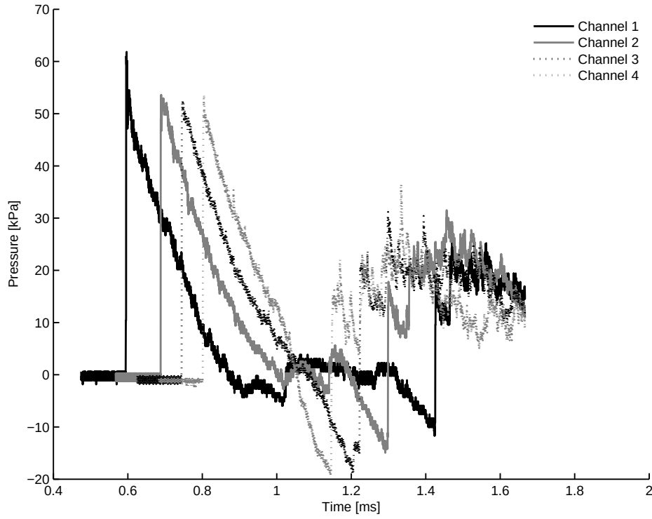
7.1 (c): Convex Profile \approx 500kPa
