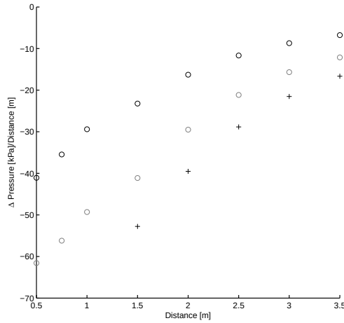
4.6 (a): Rate of Change of Peak Overpressure with Regards to Distance
