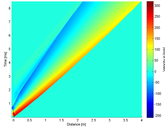
4.12 (e): 60^\circ 10bar
