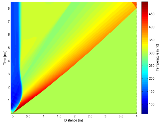
4.16 (b): 60° 15bar Temperature
