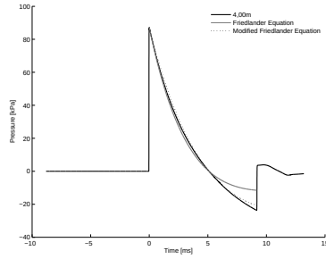
4.50 (e): Convex Profile 10bar 4.00m
