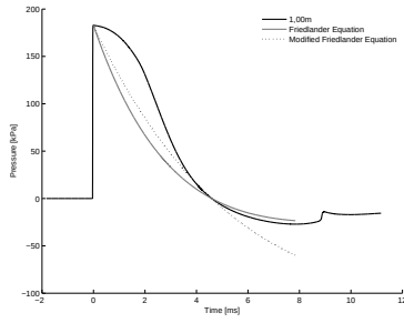
4.33 (a): 100% of Concave Driver Length 10bar 1.00m
