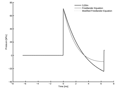
4.40 (o): 150% of Concave Driver and Transition Length 10bar 3.00m
