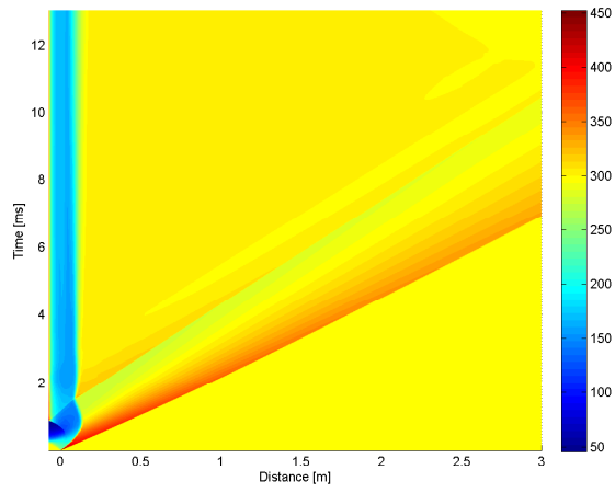
4.43 (a): 50% of Concave Driver and Transition Length 10\bar{b}ar
