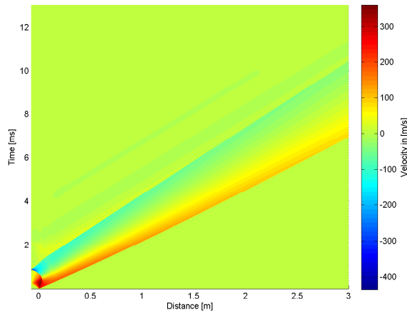
4.44 (a): 50% of Concave Driver and Transition Length 10bar
