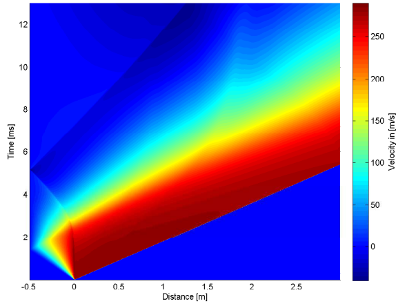
A.14 (a): 100% of Convex Driver Length 10bar
