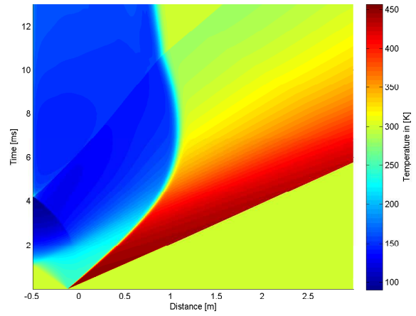
A.6 (b): 75% of Linear Driver Length 10bar
