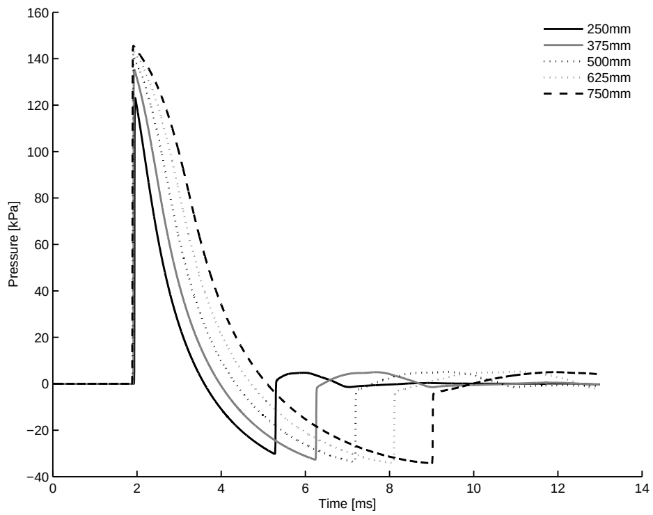
B.9 (b): 1.00m 10bar
