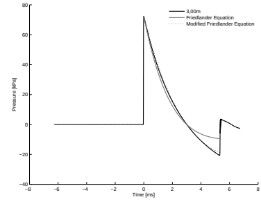
B.10 (c): 50% of Convex Driver and Transition Length 10bar 3.00m
