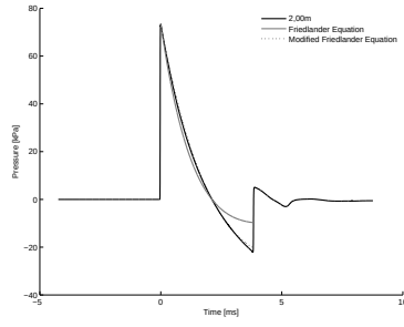
B.3(b): 50% of Linear Driver and Transition Length 10bar 2.00m
