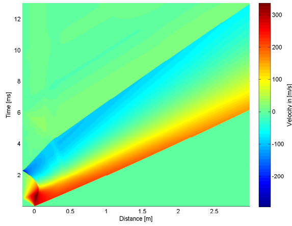
B.7(c): 100% of Linear Driver and Transition Length 10bar
