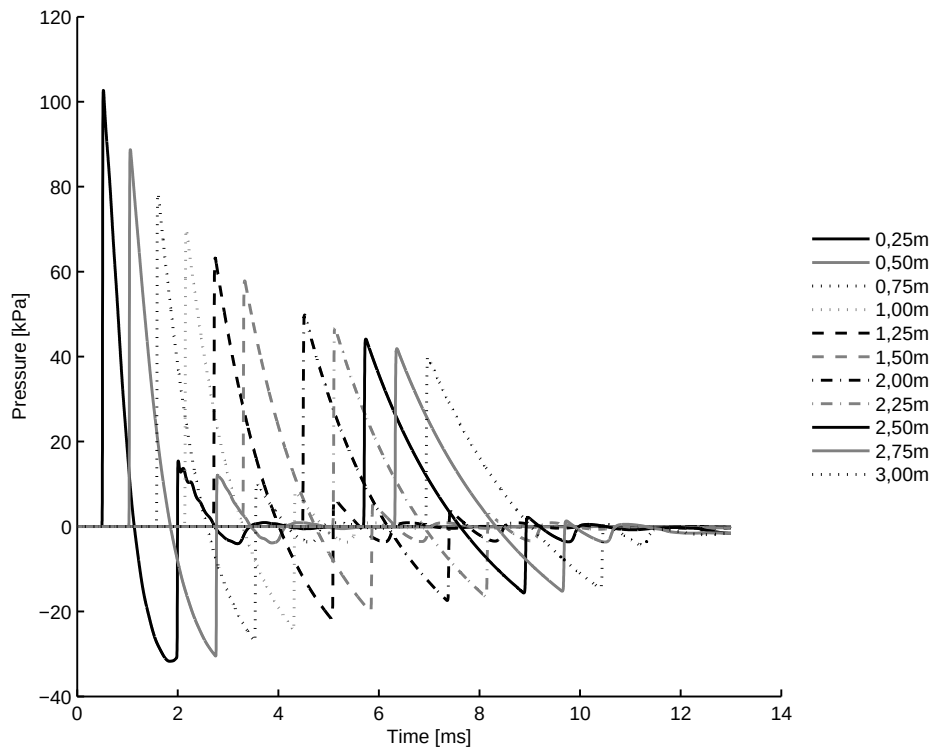
4.38 (a): 50% of Concave Driver and Transition Length 10bar
