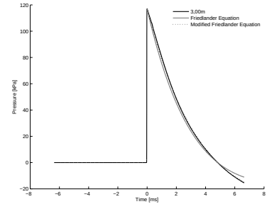
A.3(i): 50% of Linear Driver Length 10bar 3.00m
