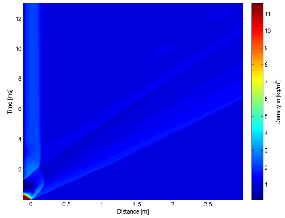
4.42 (b): 75% of Concave Driver and Transition Length 10bar
