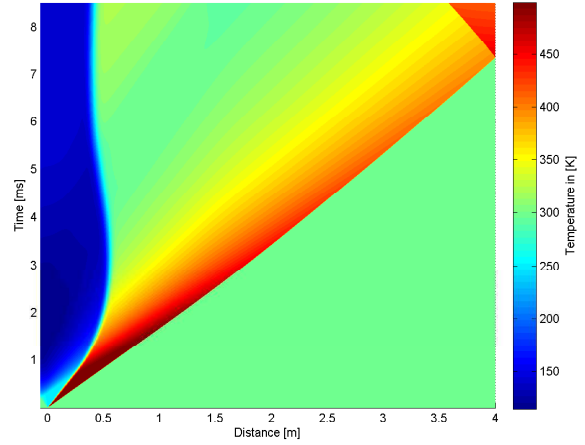
4.28 (b): 65mm 15bar Temperature
