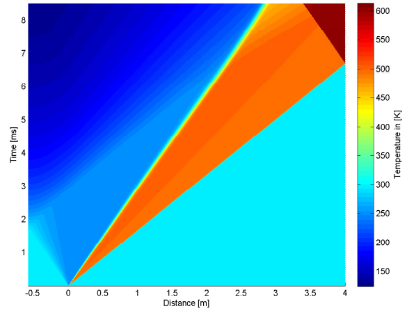
4.27 (b): 580mm 15bar Temperature
