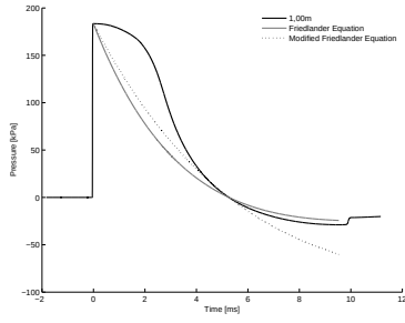
A.10 (a): 100% of Convex Driver Length 10bar 1.00m
