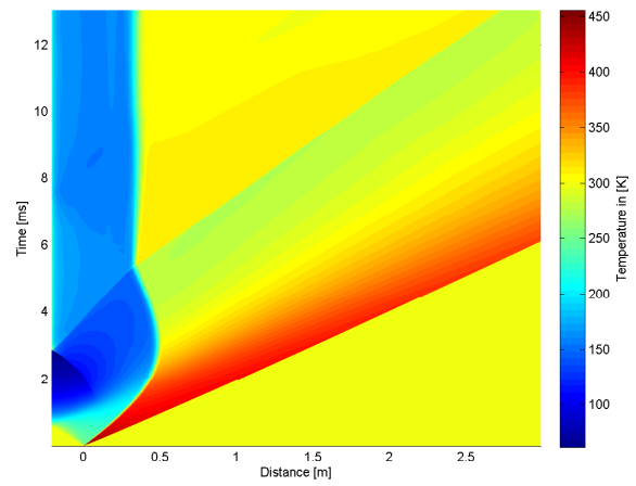
B.6 (d): 125% of Linear Driver and Transition Length 10bar
