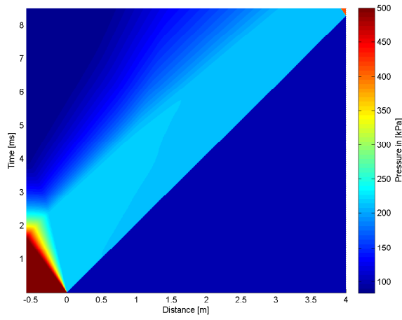
4.25 (a): 580mm 5bar Pressure
