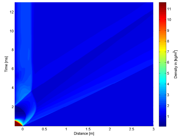
4.42 (d): 125% of Concave Driver and Transition Length 10bar
