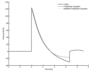
B.10 (h): 100% of Convex Driver and Transition Length 10bar 2.00m
