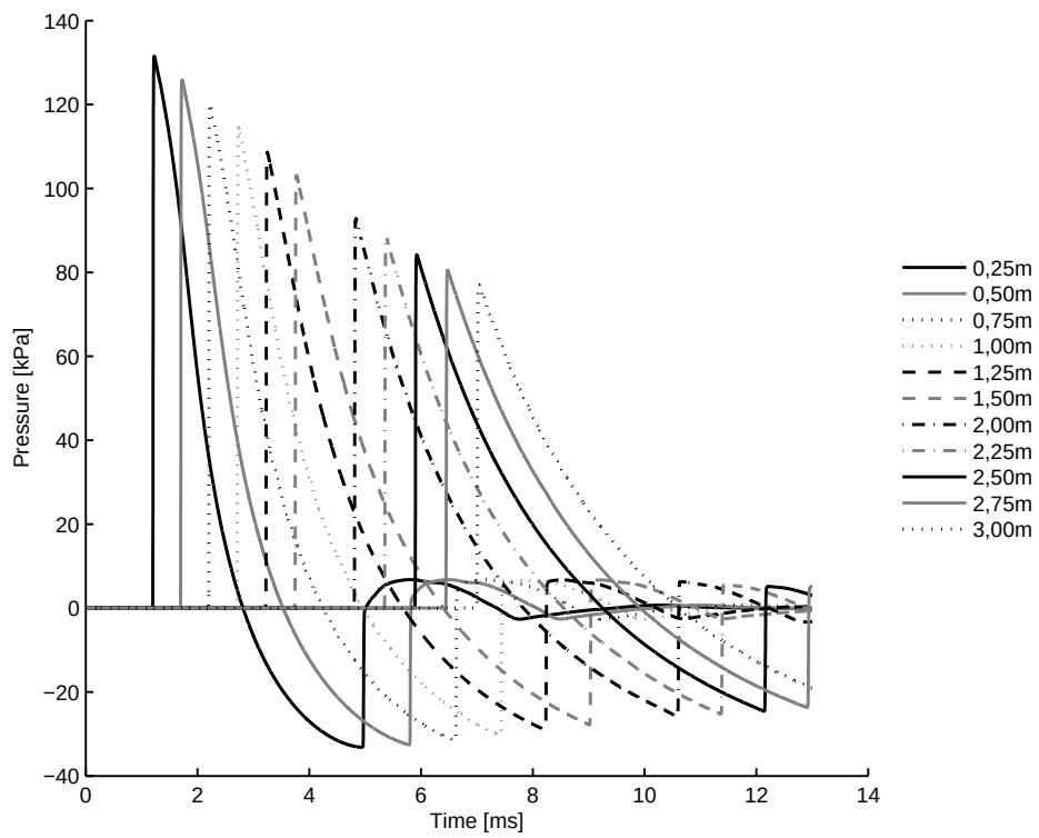
A.8 (d): 25% of Convex Driver Length 10bar
