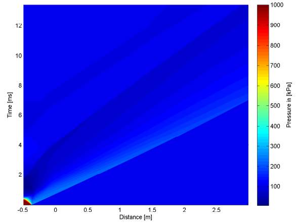
A.11 (d): 25% of Convex Driver Length 10bar
