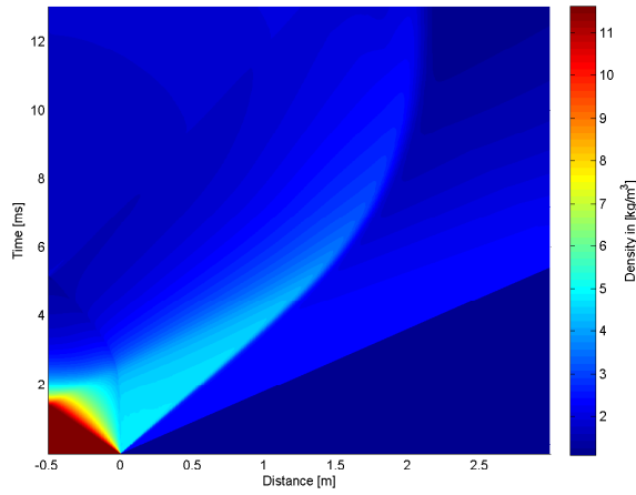
A.12 (a): 100% of Convex Driver Length 10bar
