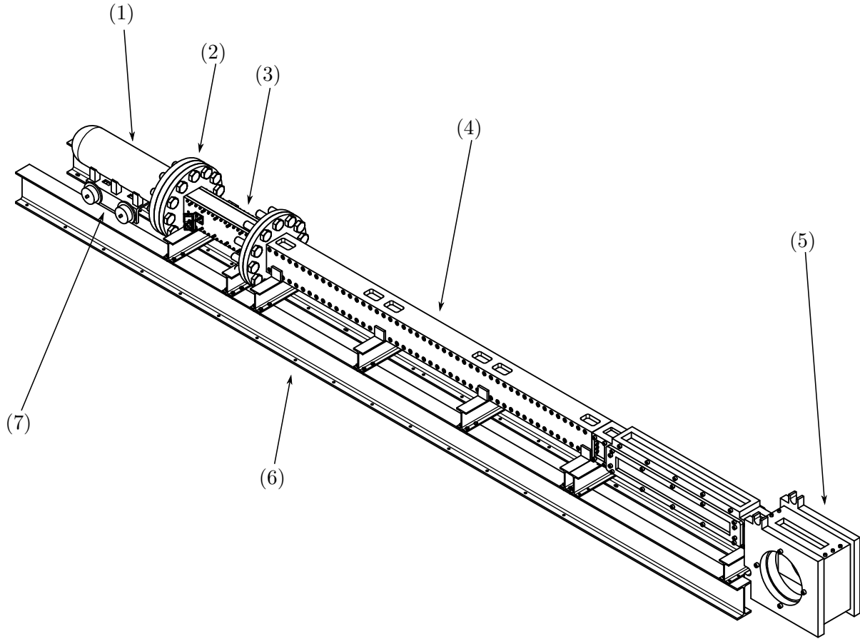
Figure 5.1: Schematic of the Blast Tube Facility
