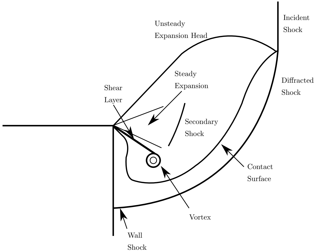
Figure 2.14: The Perturbed Region Behind a Diffracting Shock Wave (Skews (1967b))
