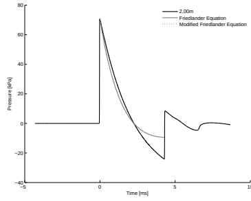
4.40 (h): 100% of Concave Driver and Transition Length 10bar 2.00m
