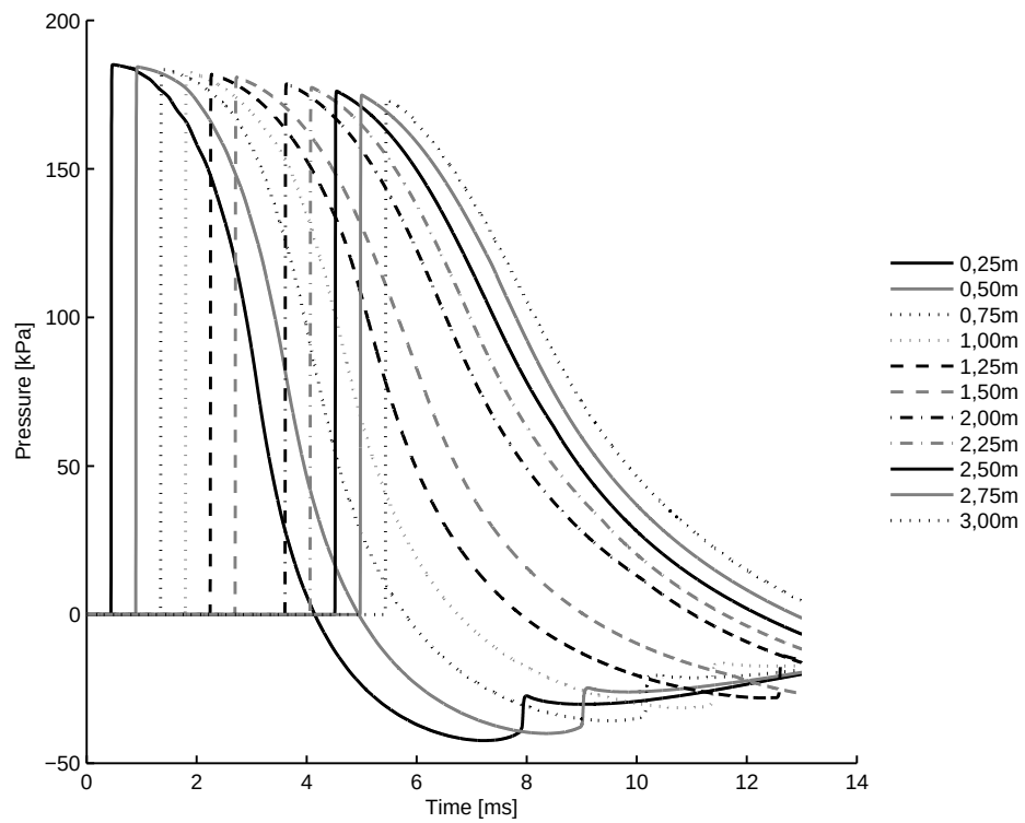
A.1 (a): 100% of Linear Driver Length 10bar
