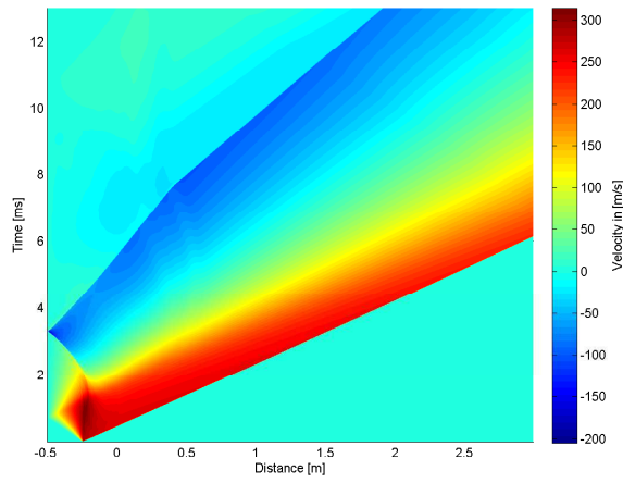
A.14 (c): 50% of Convex Driver Length 10bar
