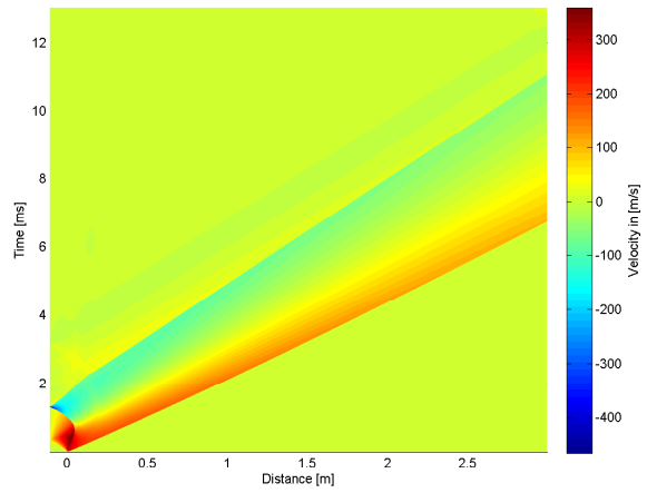
4.44 (b): 75% of Concave Driver and Transition Length 10bar
